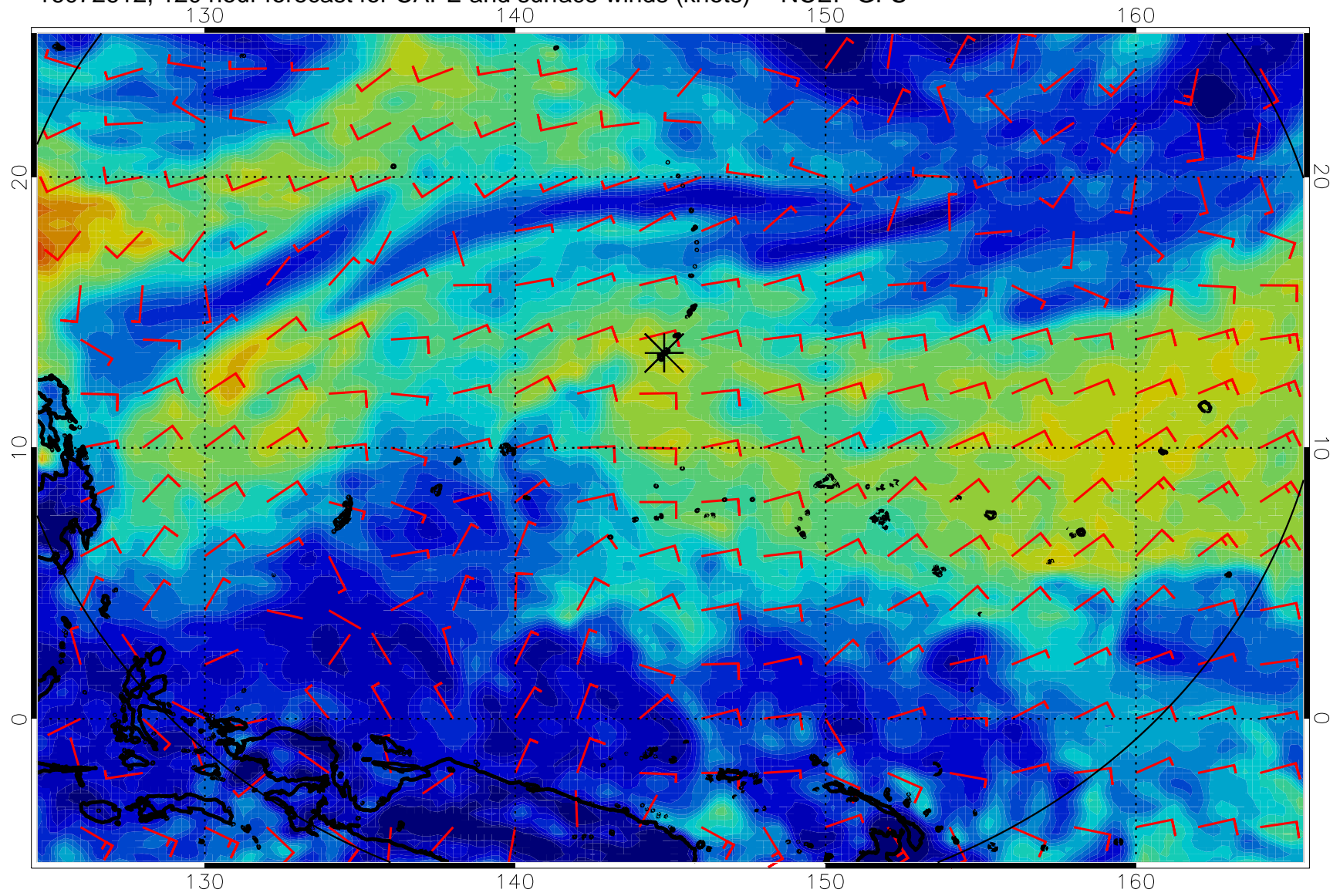
16072612, 120 hour forecast for CAPE and surface winds (knots) -- NCEP GFS
