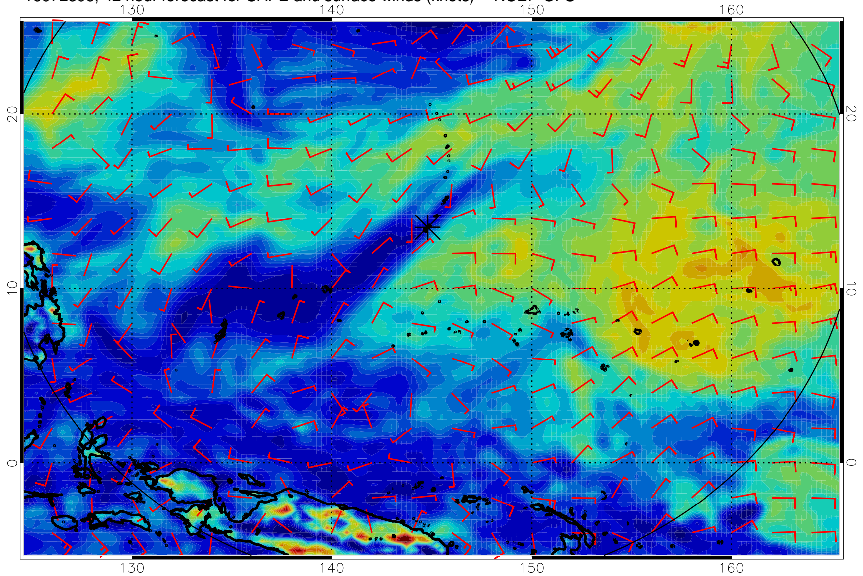
16072306, 42 hour forecast for CAPE and surface winds (knots) -- NCEP GFS
