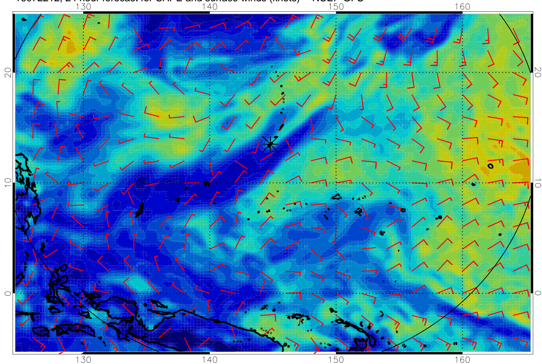
16072212, 24 hour forecast for CAPE and surface winds (knots) -- NCEP GFS
