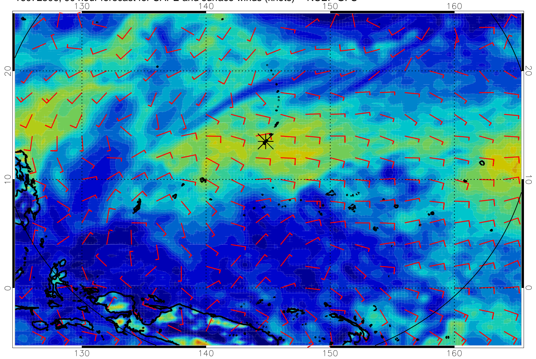
16072506, 90 hour forecast for CAPE and surface winds (knots) -- NCEP GFS
