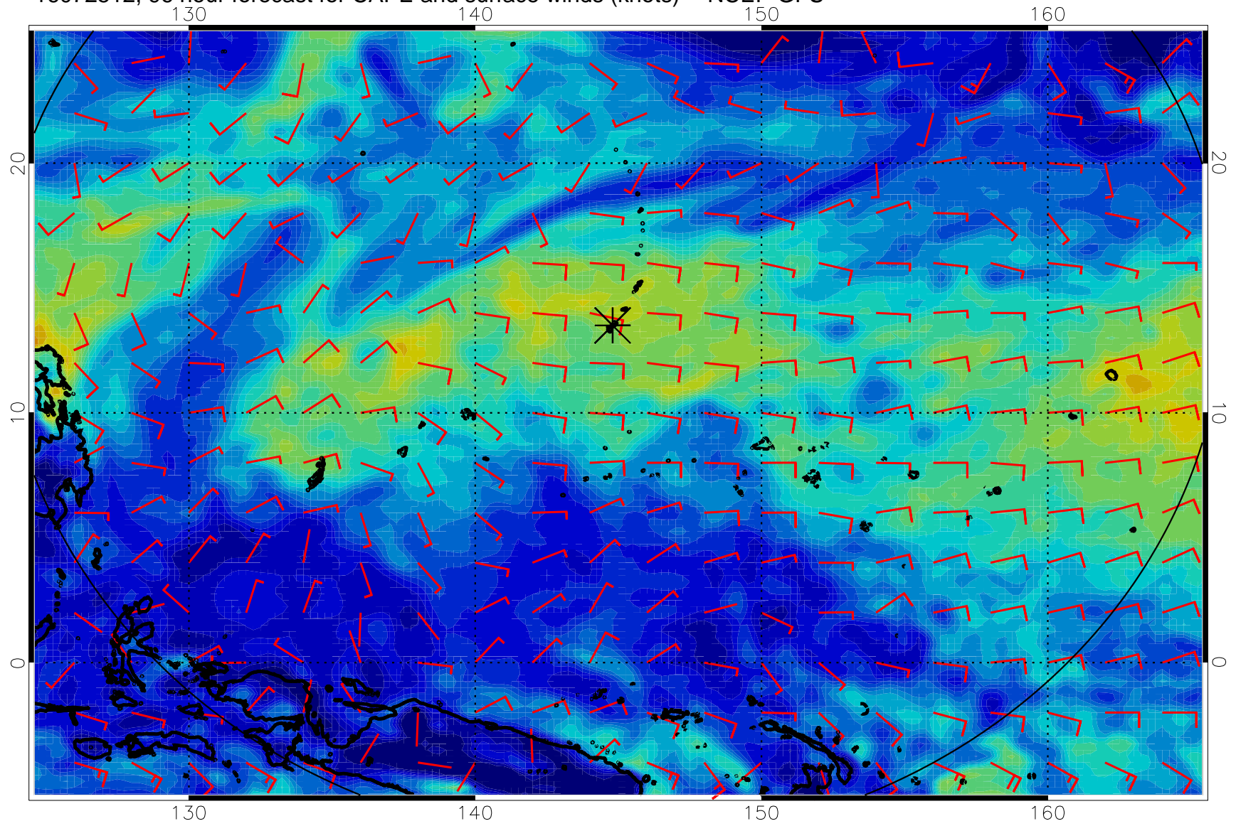
16072512, 96 hour forecast for CAPE and surface winds (knots) -- NCEP GFS
