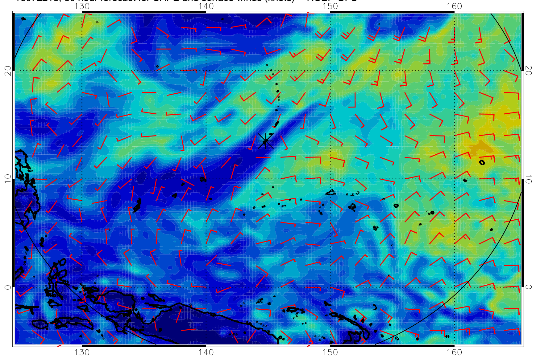
16072218, 30 hour forecast for CAPE and surface winds (knots) -- NCEP GFS
