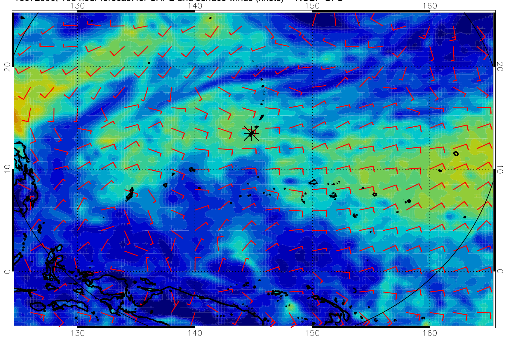
16072600, 108 hour forecast for CAPE and surface winds (knots) -- NCEP GFS
