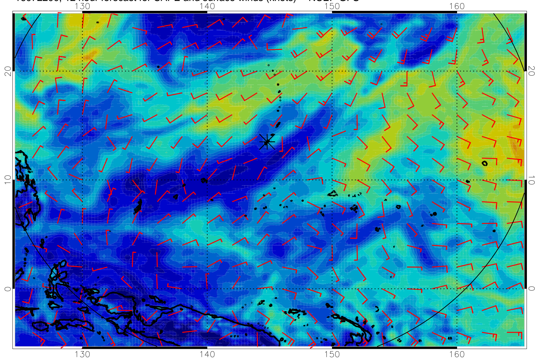
16072200, 12 hour forecast for CAPE and surface winds (knots) -- NCEP GFS
