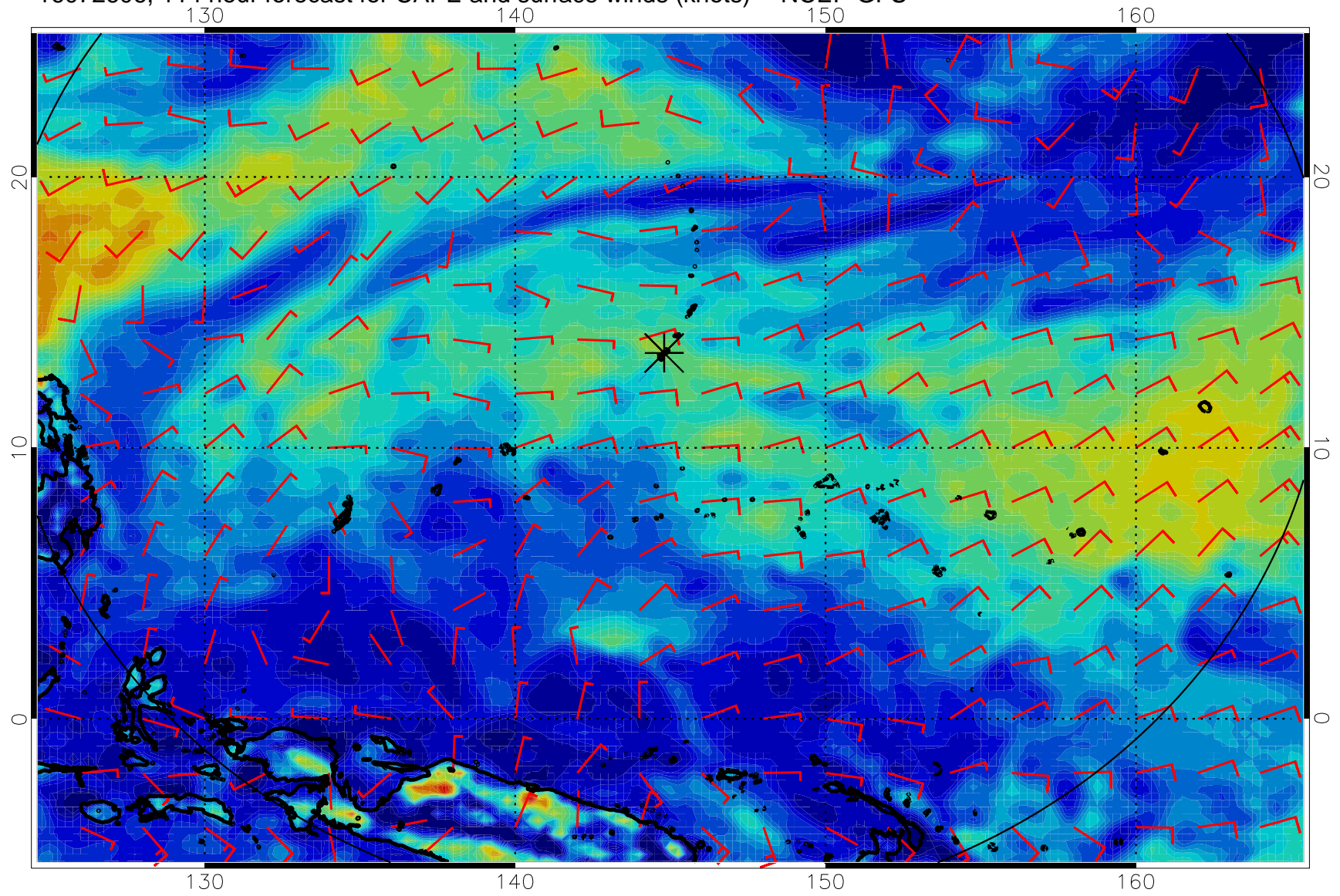
16072606, 114 hour forecast for CAPE and surface winds (knots) -- NCEP GFS
