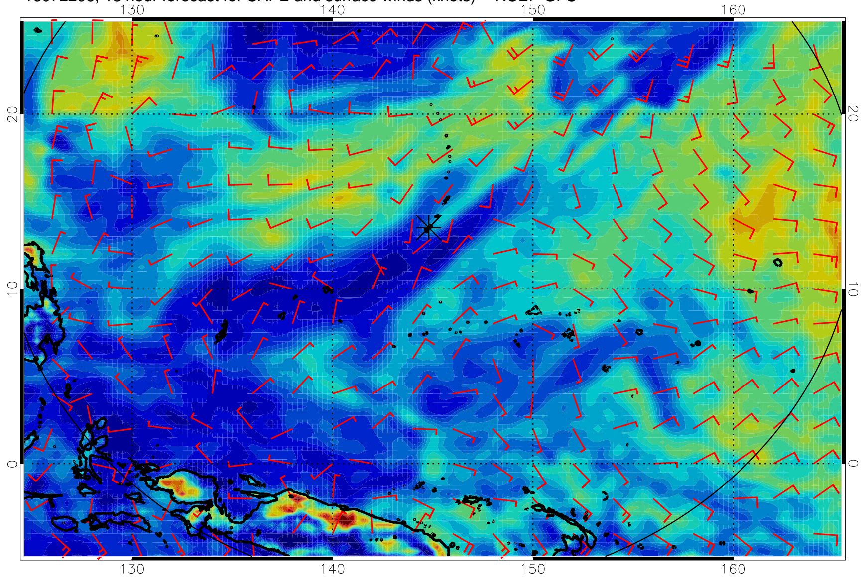
16072206, 18 hour forecast for CAPE and surface winds (knots) -- NCEP GFS
