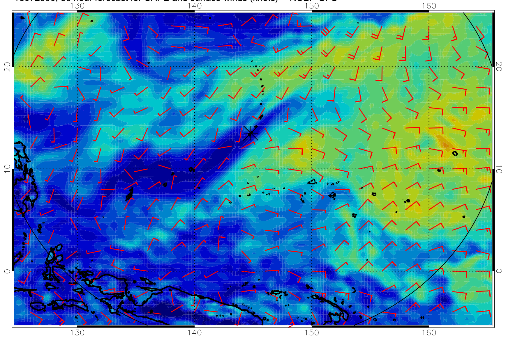
16072300, 36 hour forecast for CAPE and surface winds (knots) -- NCEP GFS
