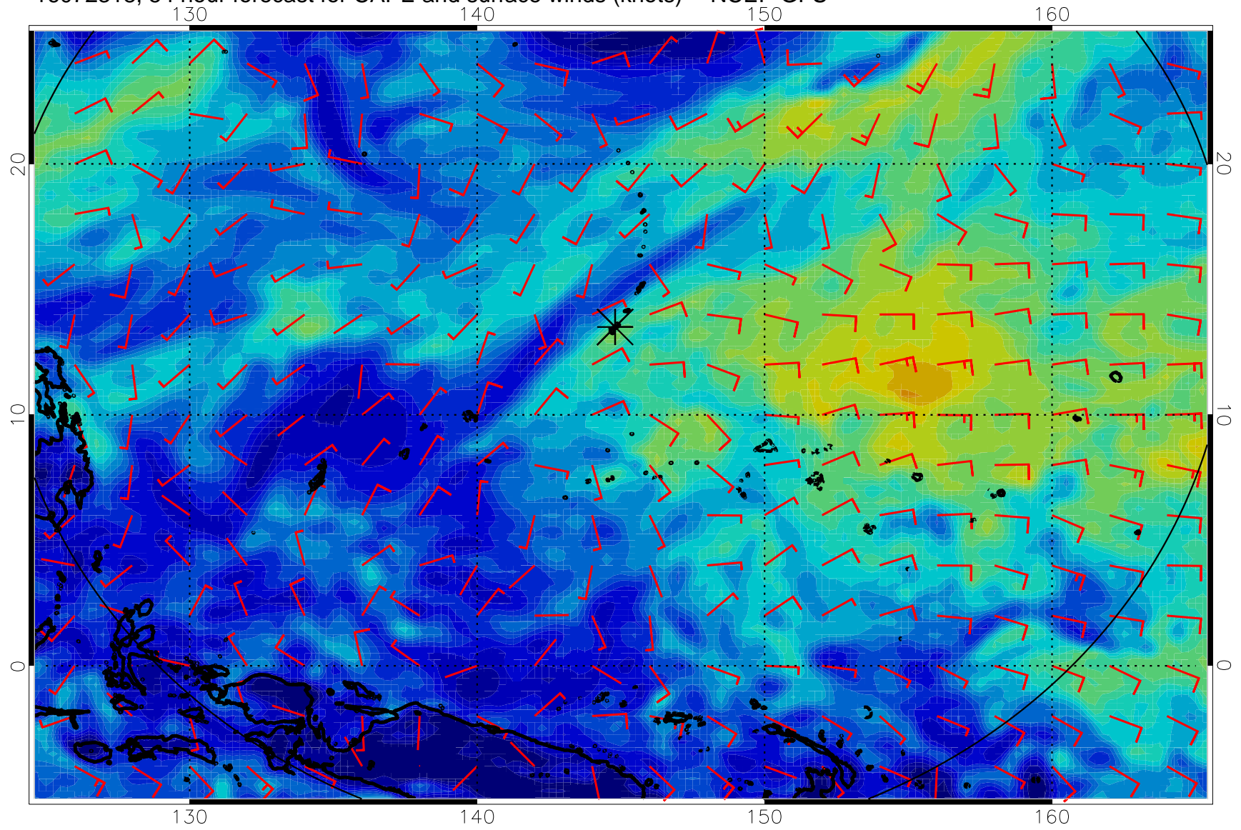
16072318, 54 hour forecast for CAPE and surface winds (knots) -- NCEP GFS
