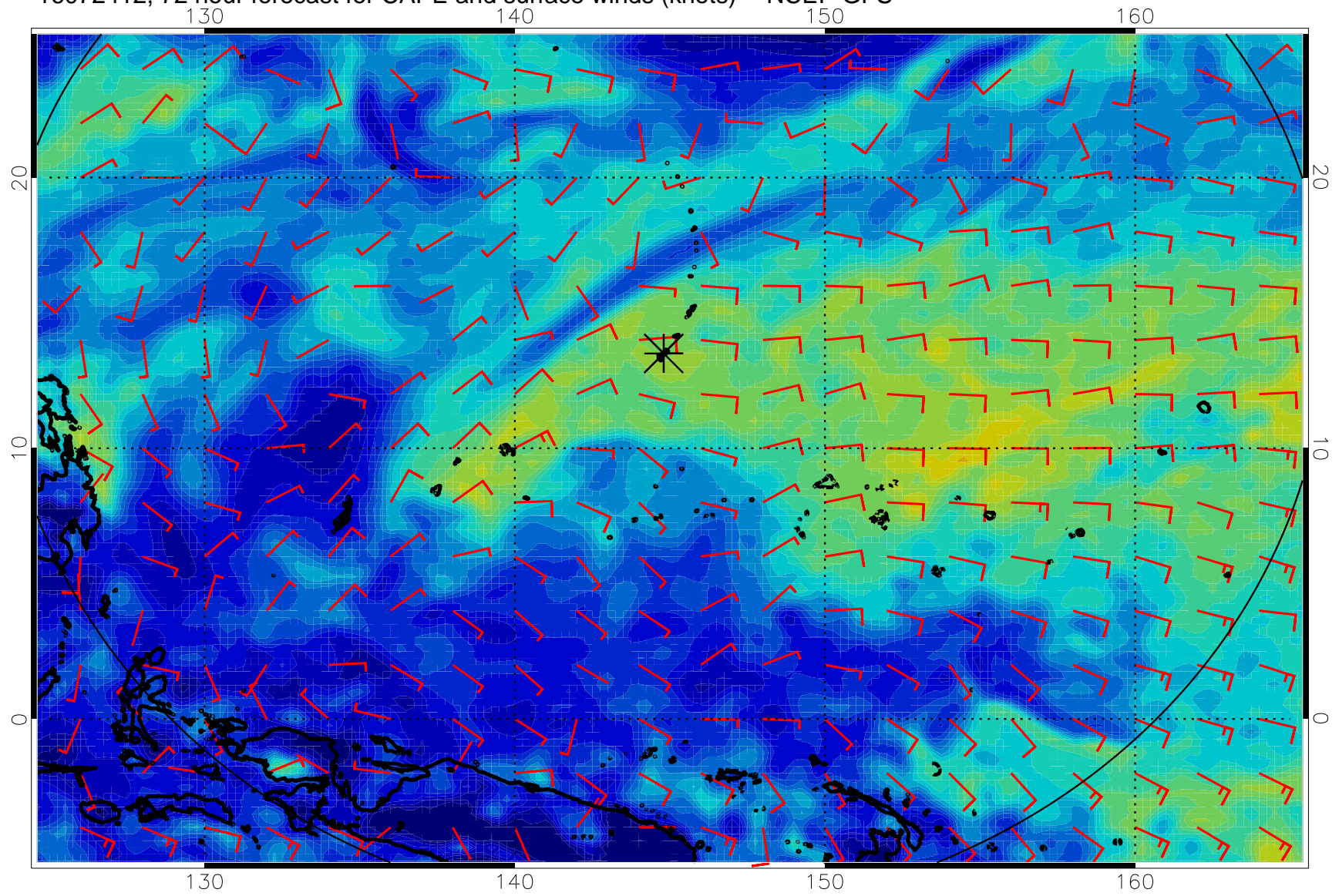
16072412, 72 hour forecast for CAPE and surface winds (knots) -- NCEP GFS
