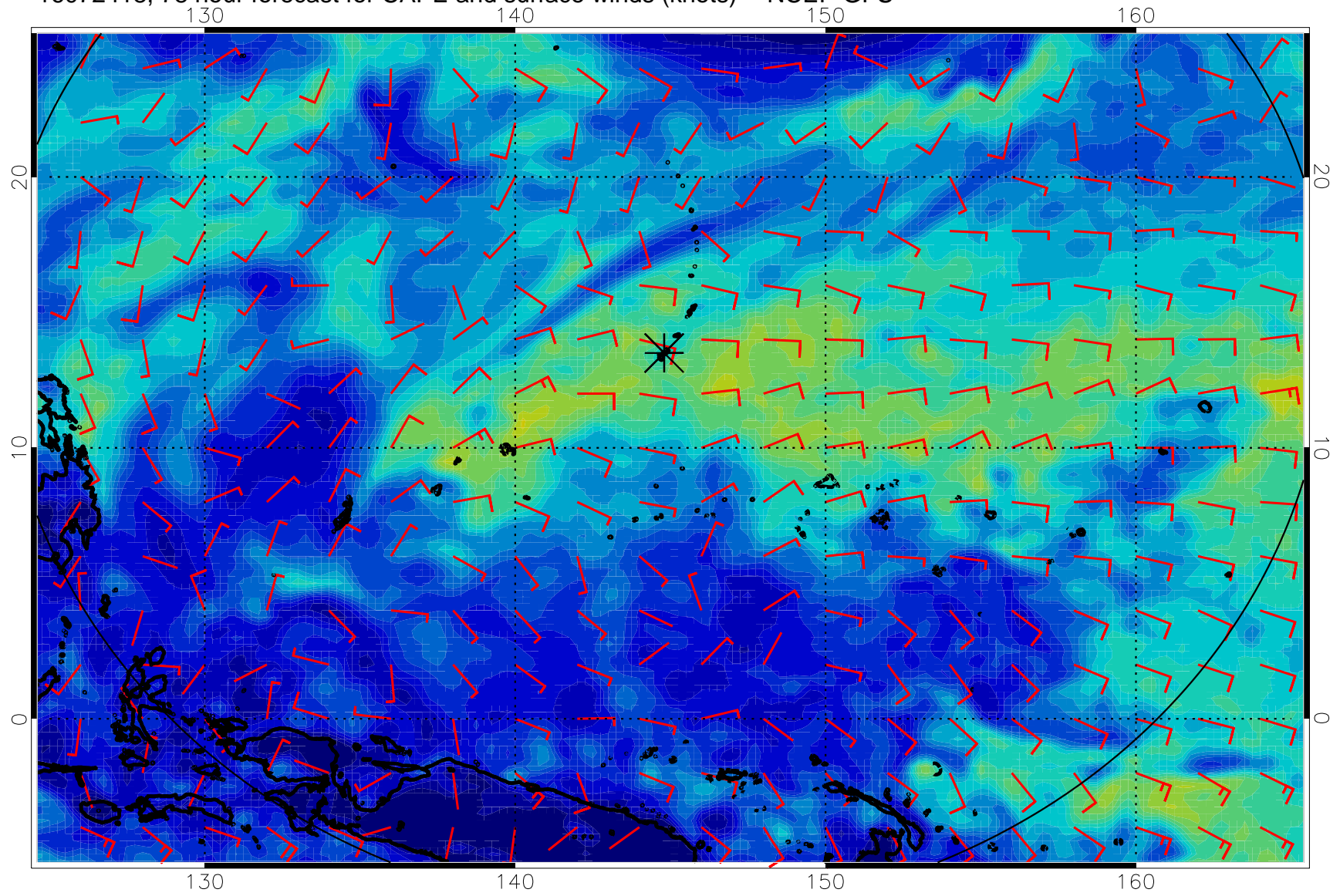
16072418, 78 hour forecast for CAPE and surface winds (knots) -- NCEP GFS
