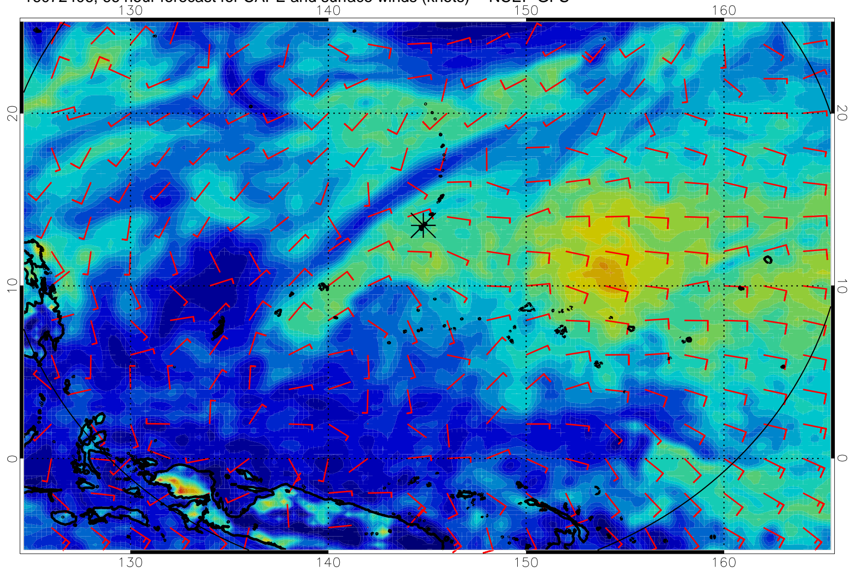
16072406, 66 hour forecast for CAPE and surface winds (knots) -- NCEP GFS
