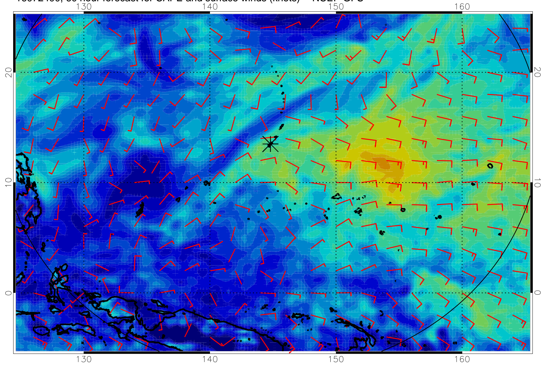
16072400, 60 hour forecast for CAPE and surface winds (knots) -- NCEP GFS
