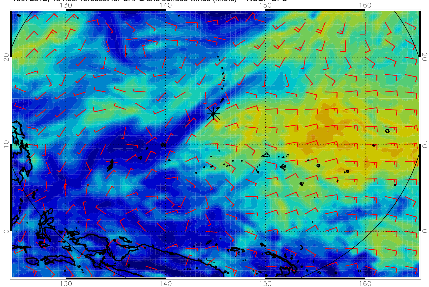
16072312, 48 hour forecast for CAPE and surface winds (knots) -- NCEP GFS
