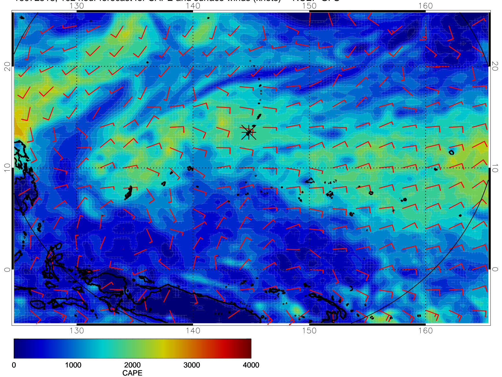
16072518, 102 hour forecast for CAPE and surface winds (knots) -- NCEP GFS
