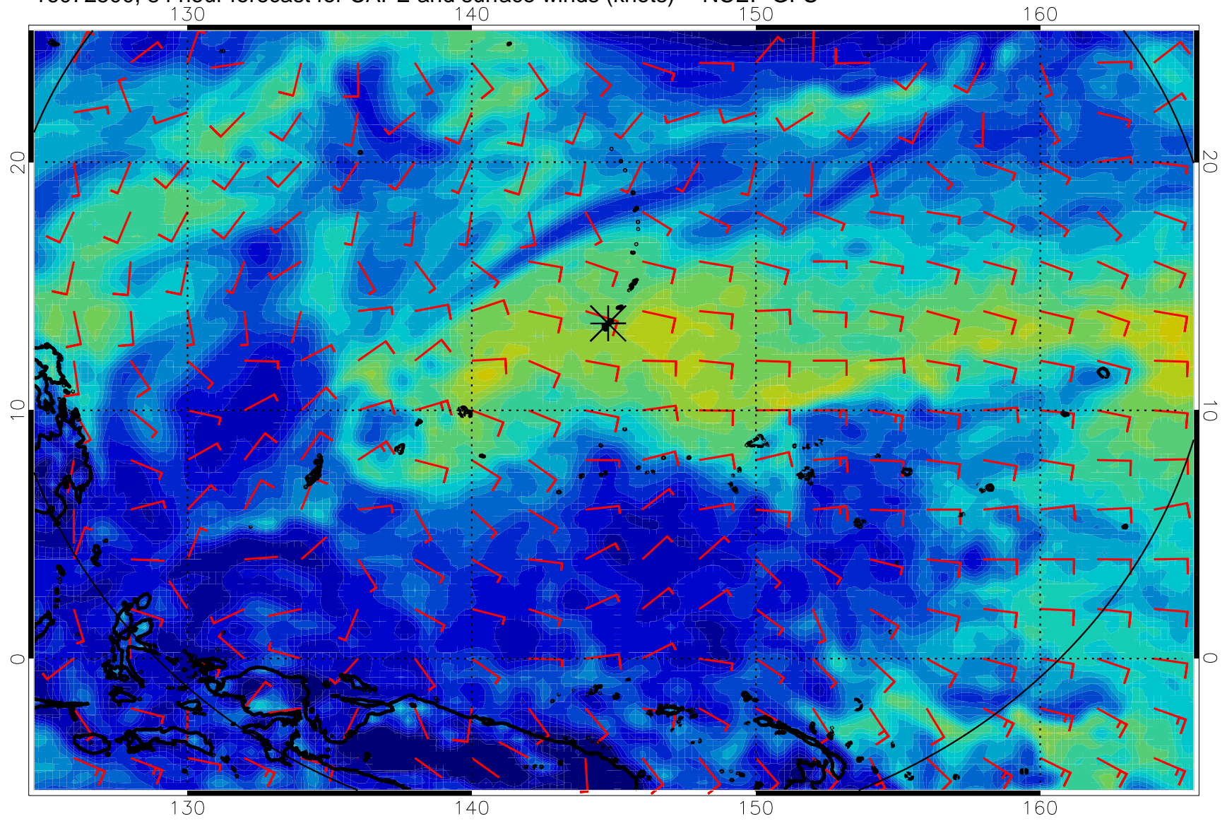
16072500, 84 hour forecast for CAPE and surface winds (knots) -- NCEP GFS
