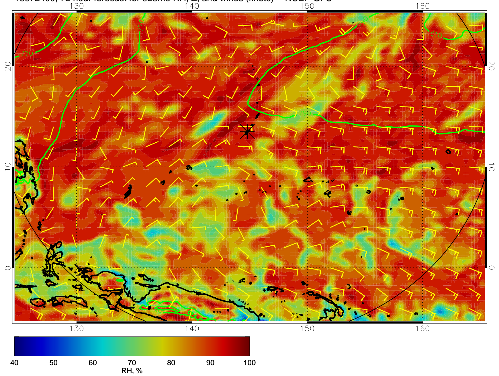
16072400, 72 hour forecast for 925mb RH, Z, and winds (knots) -- NCEP GFS
