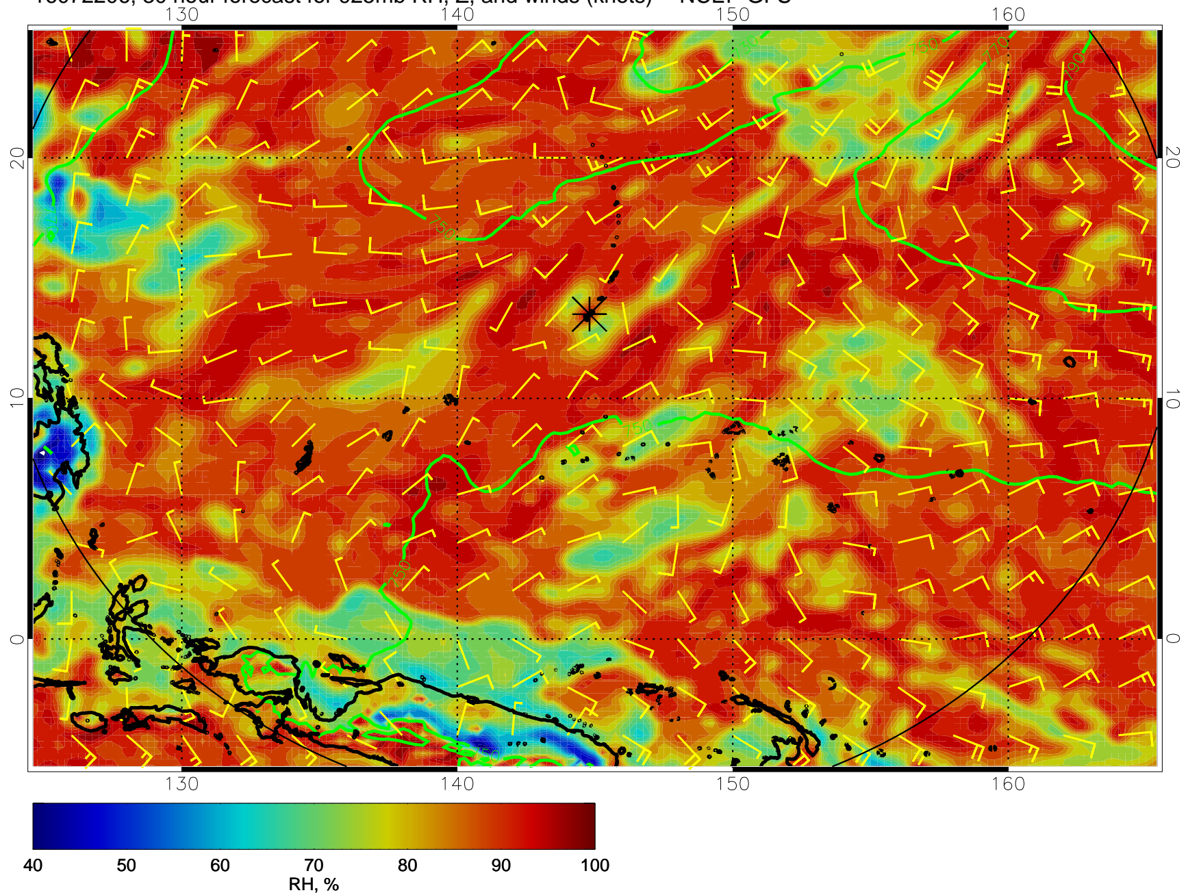
16072206, 30 hour forecast for 925mb RH, Z, and winds (knots) -- NCEP GFS
