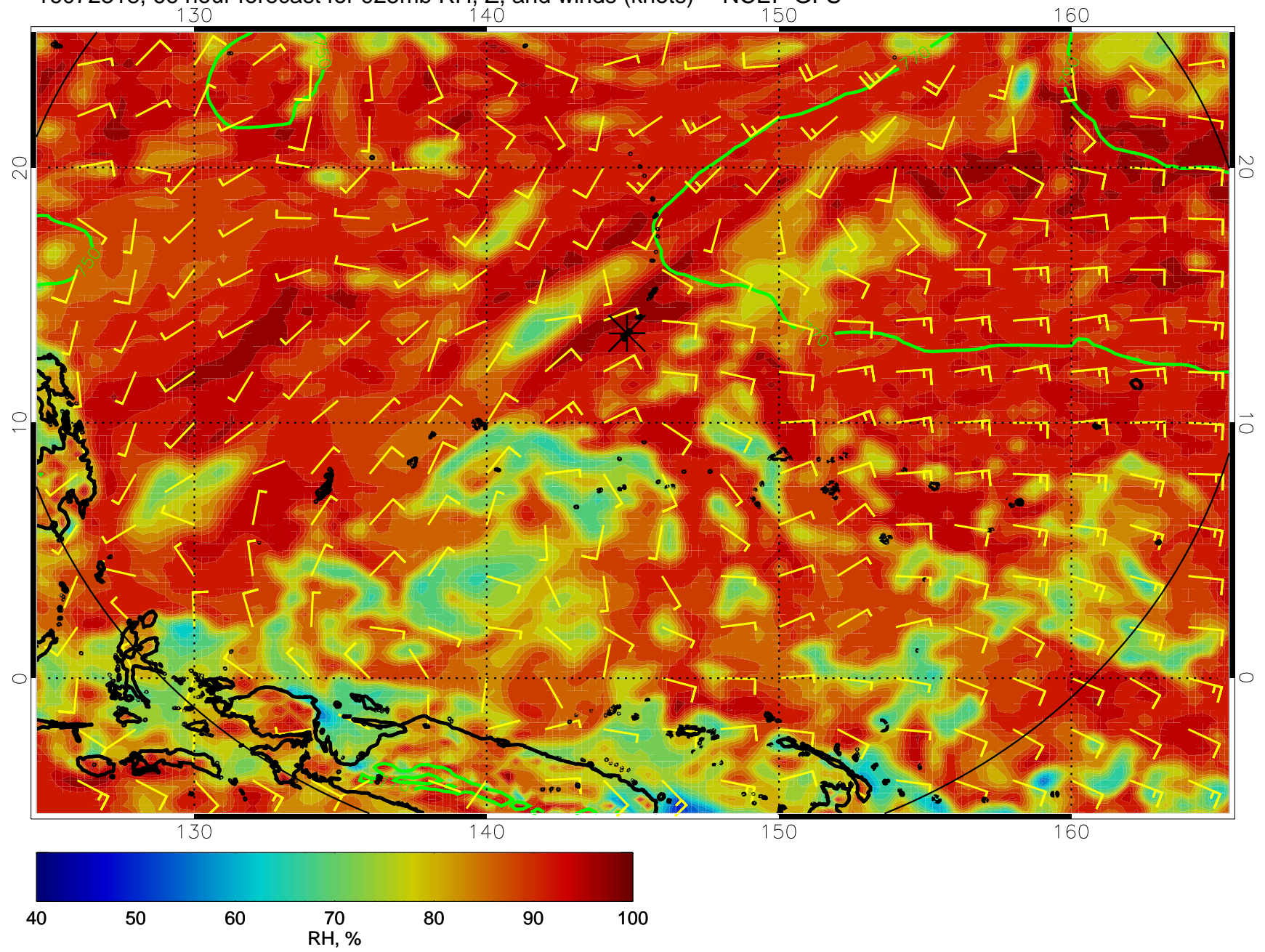
16072318, 66 hour forecast for 925mb RH, Z, and winds (knots) -- NCEP GFS
