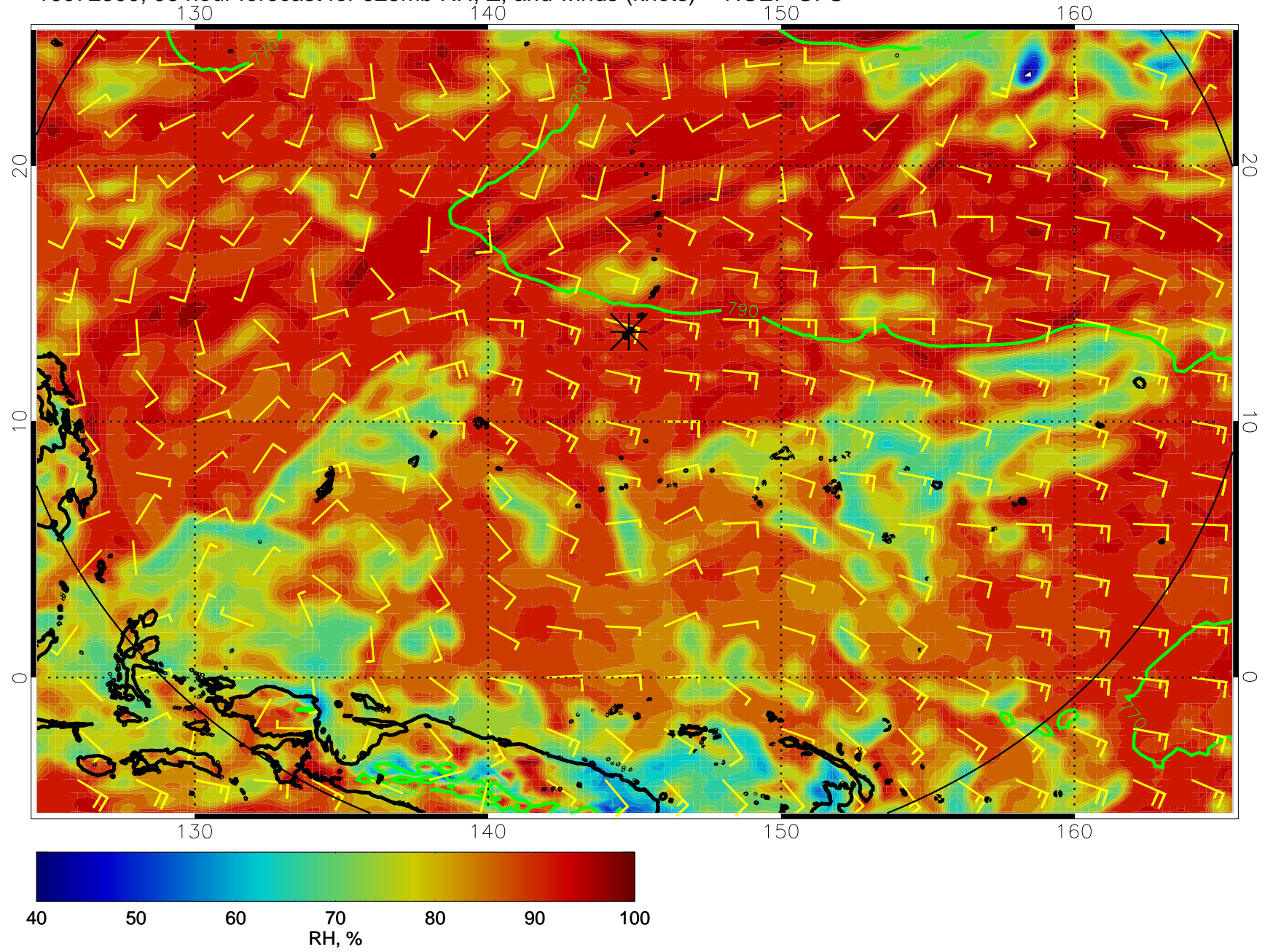
16072500, 96 hour forecast for 925mb RH, Z, and winds (knots) -- NCEP GFS
