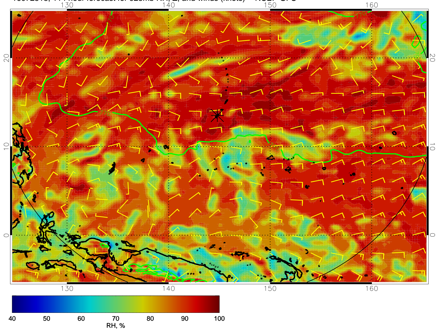
16072518, 114 hour forecast for 925mb RH, Z, and winds (knots) -- NCEP GFS
