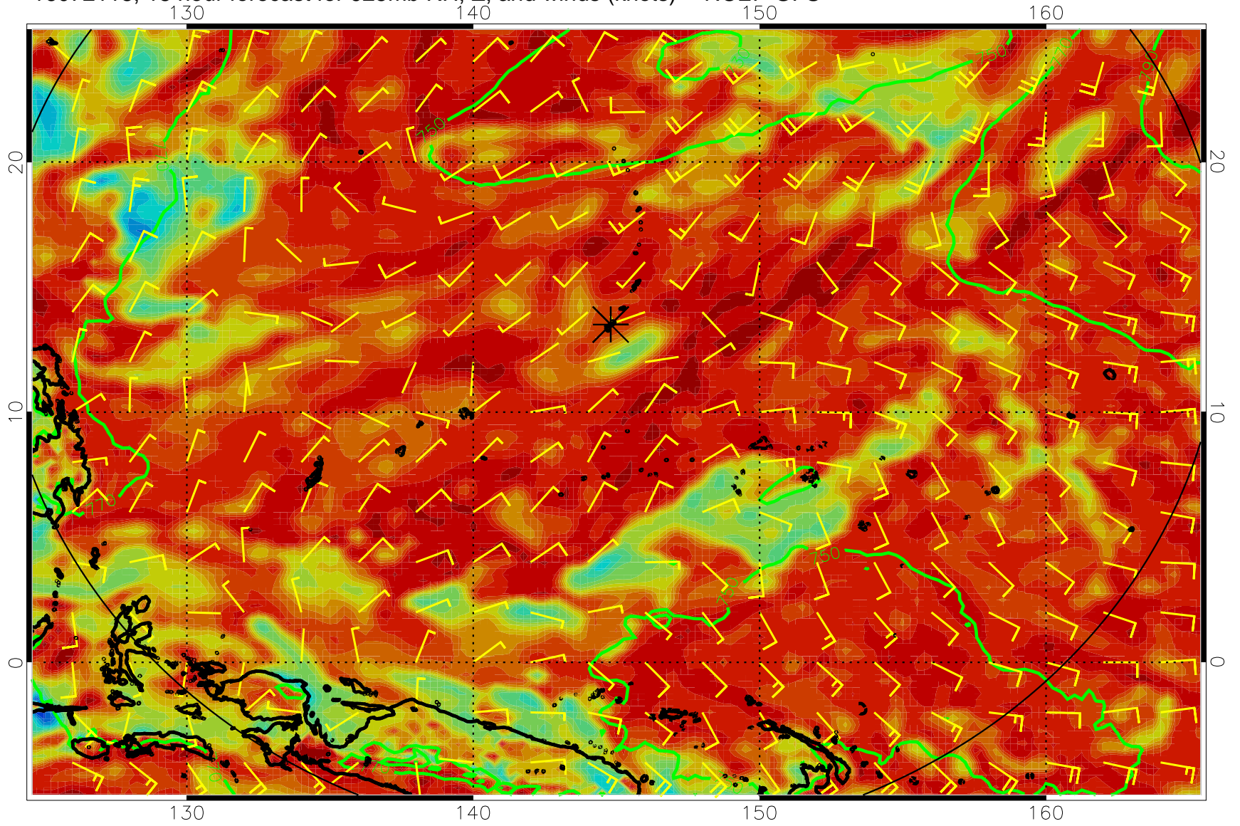
16072118, 18 hour forecast for 925mb RH, Z, and winds (knots) -- NCEP GFS
