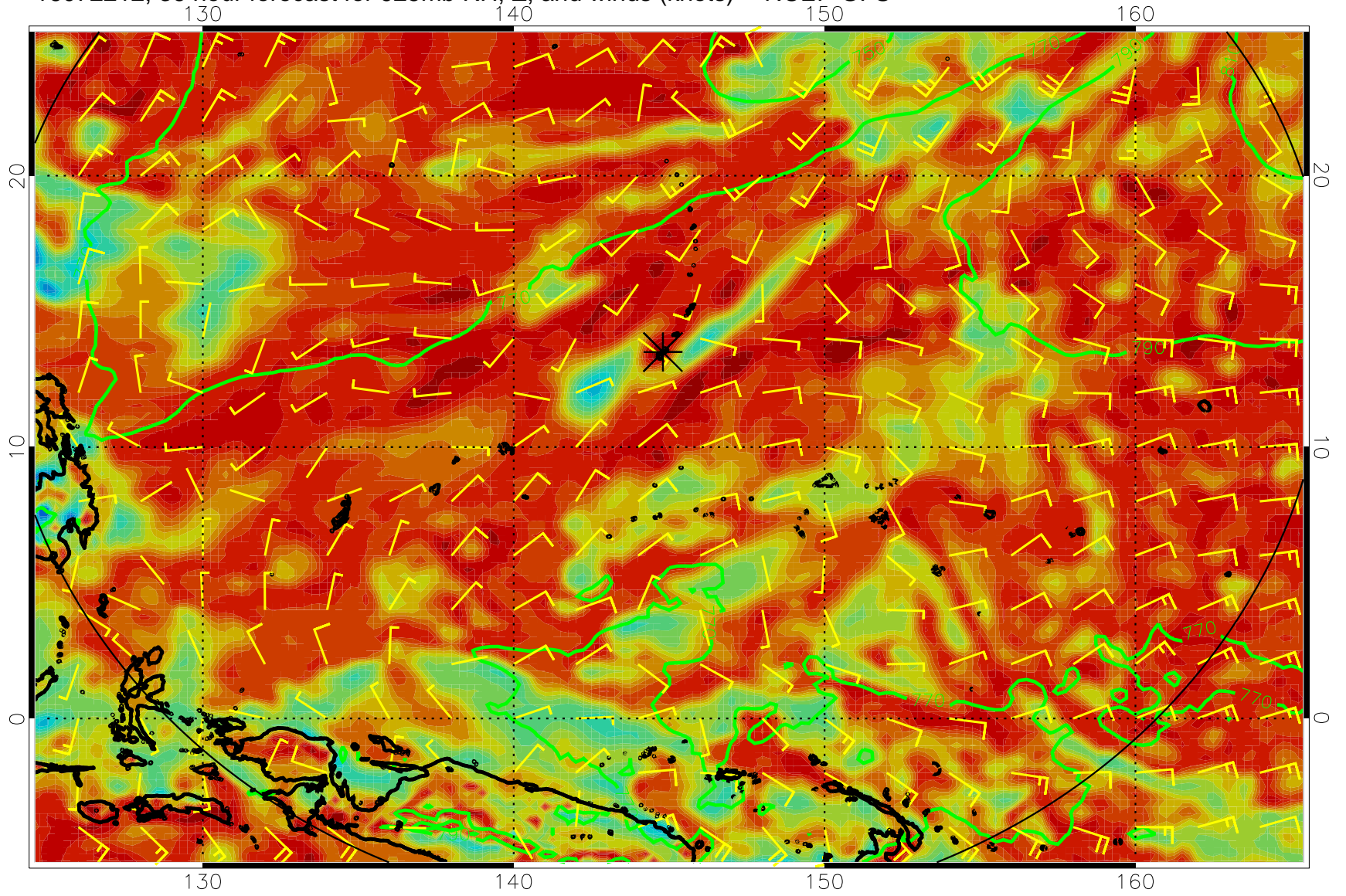
16072212, 36 hour forecast for 925mb RH, Z, and winds (knots) -- NCEP GFS
