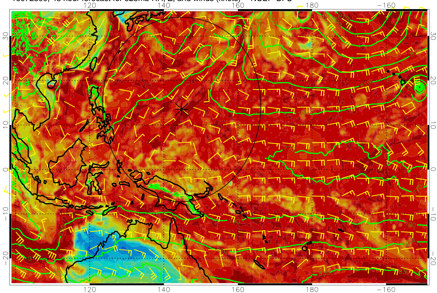
16072300, 48 hour forecast for 925mb RH, Z, and winds (knots) -- NCEP GFS
