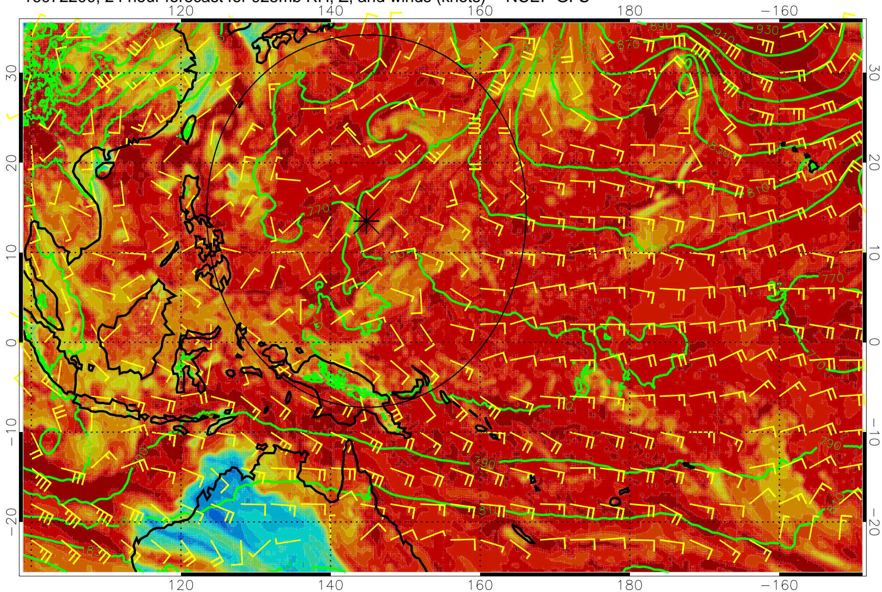
16072200, 24 hour forecast for 925mb RH, Z, and winds (knots) -- NCEP GFS
