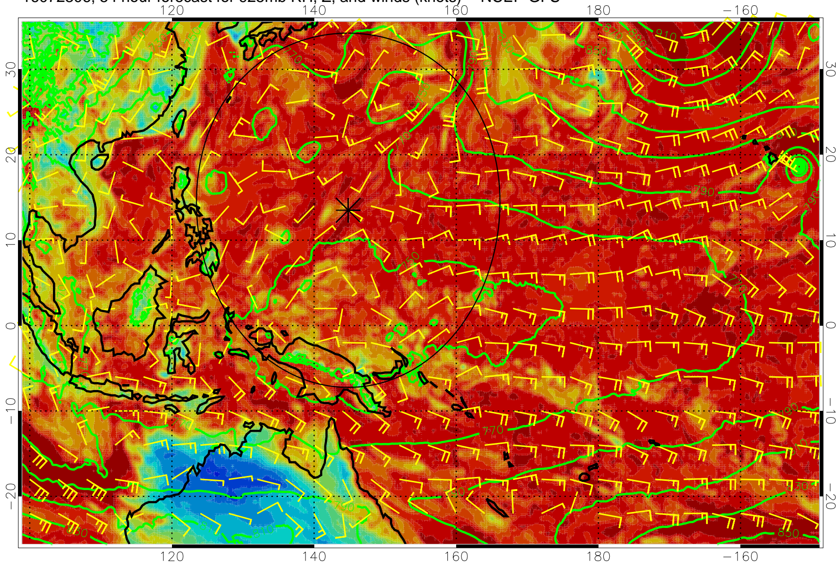
16072306, 54 hour forecast for 925mb RH, Z, and winds (knots) -- NCEP GFS
