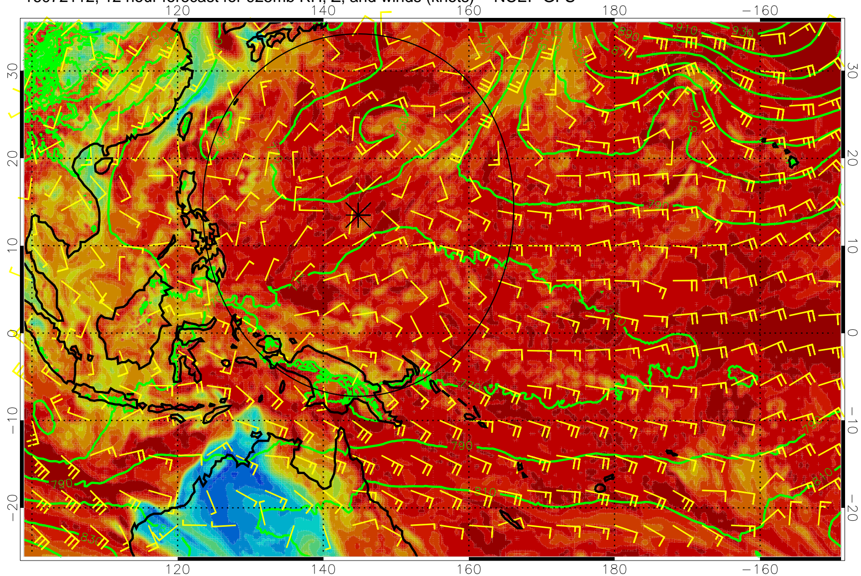
16072112, 12 hour forecast for 925mb RH, Z, and winds (knots) -- NCEP GFS
