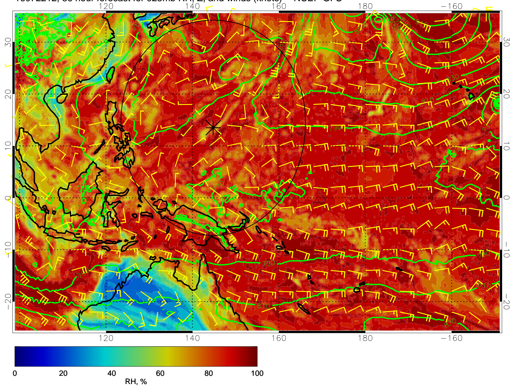
16072212, 36 hour forecast for 925mb RH, Z, and winds (knots) -- NCEP GFS
