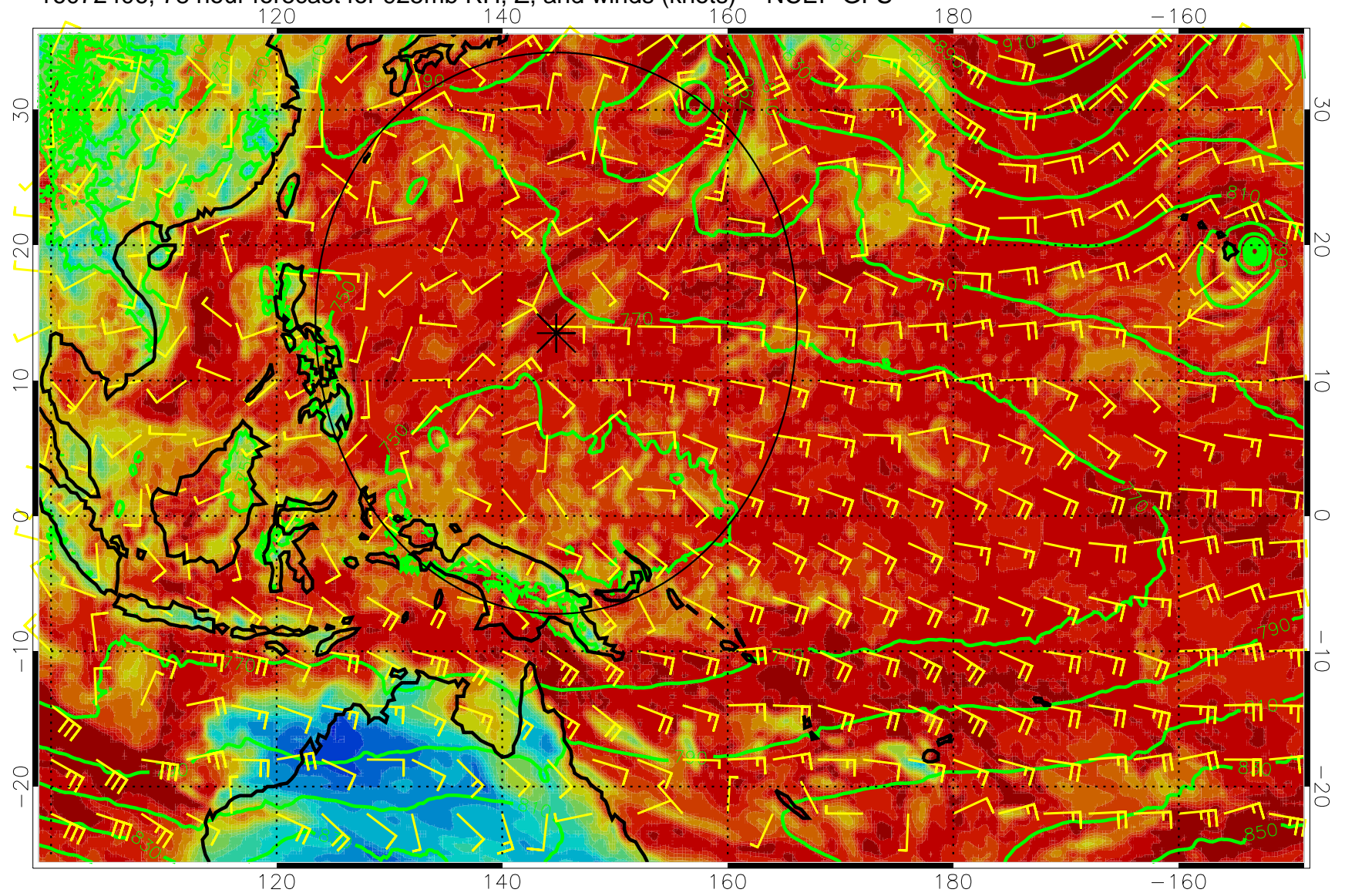
16072406, 78 hour forecast for 925mb RH, Z, and winds (knots) -- NCEP GFS
