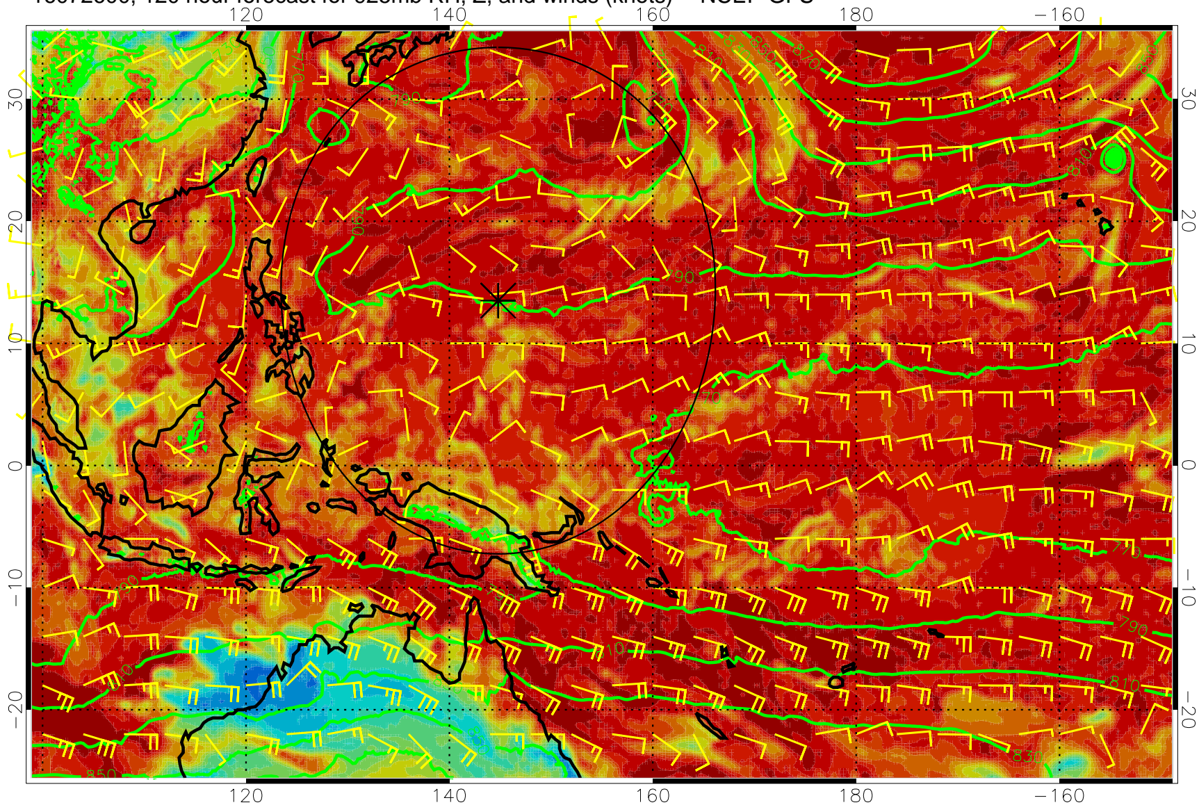
16072600, 120 hour forecast for 925mb RH, Z, and winds (knots) -- NCEP GFS
