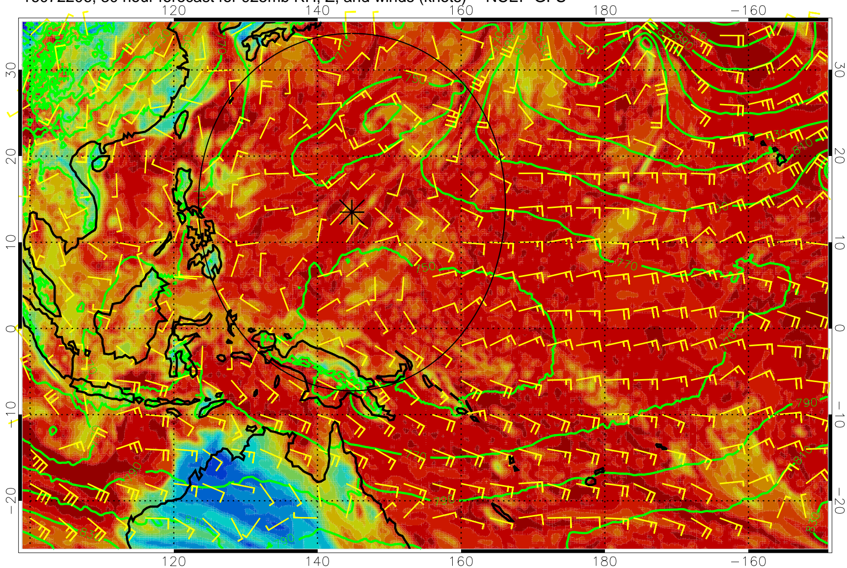
16072206, 30 hour forecast for 925mb RH, Z, and winds (knots) -- NCEP GFS
