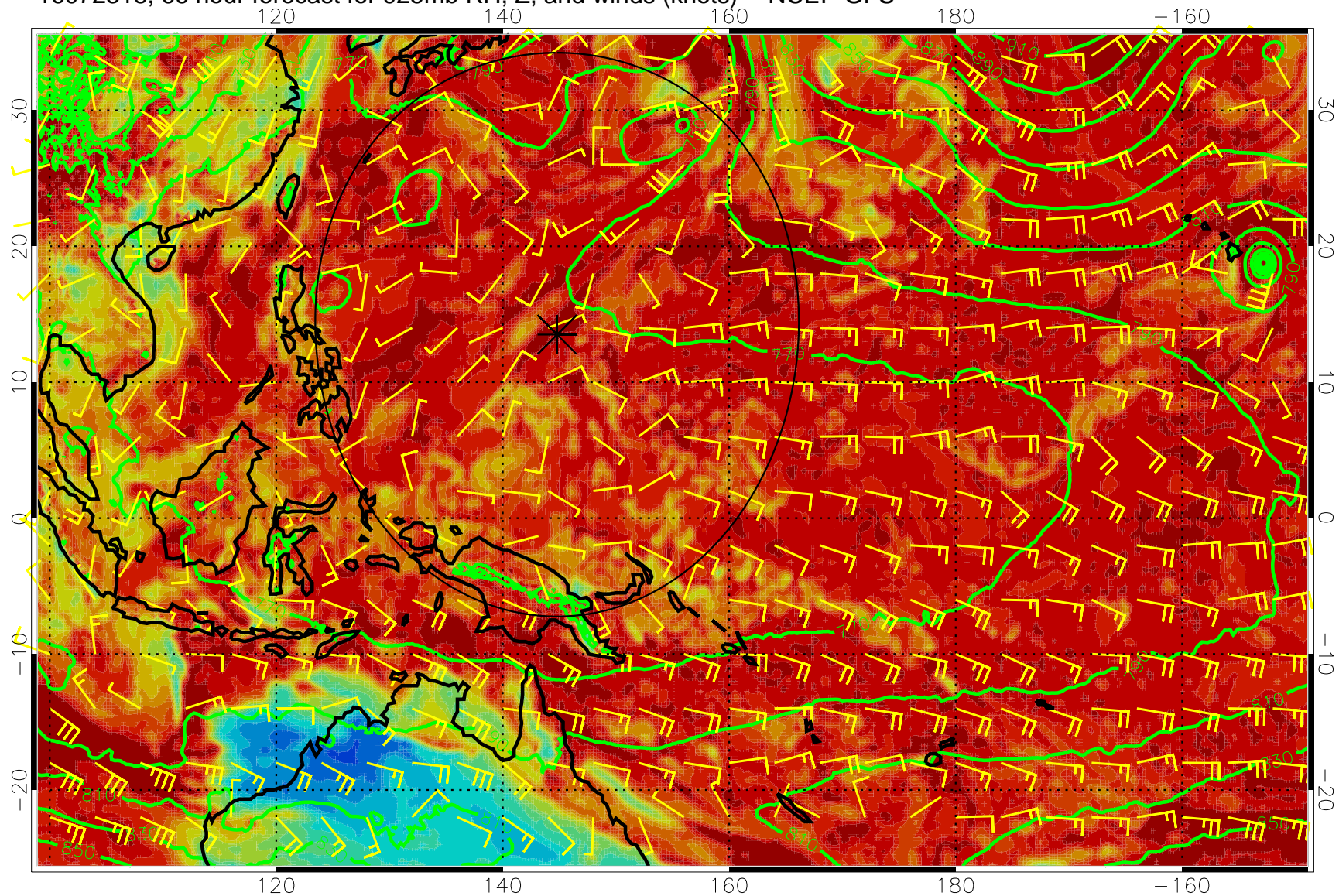
16072318, 66 hour forecast for 925mb RH, Z, and winds (knots) -- NCEP GFS
