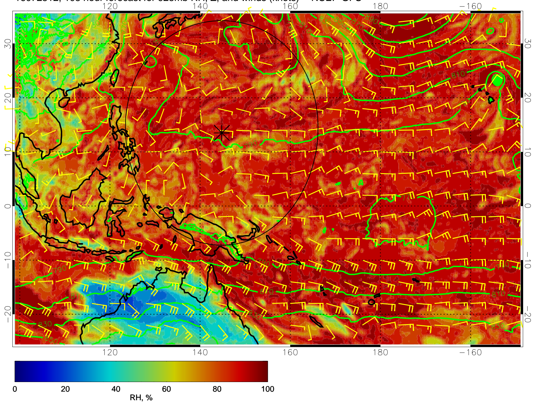
16072512, 108 hour forecast for 925mb RH, Z, and winds (knots) -- NCEP GFS
