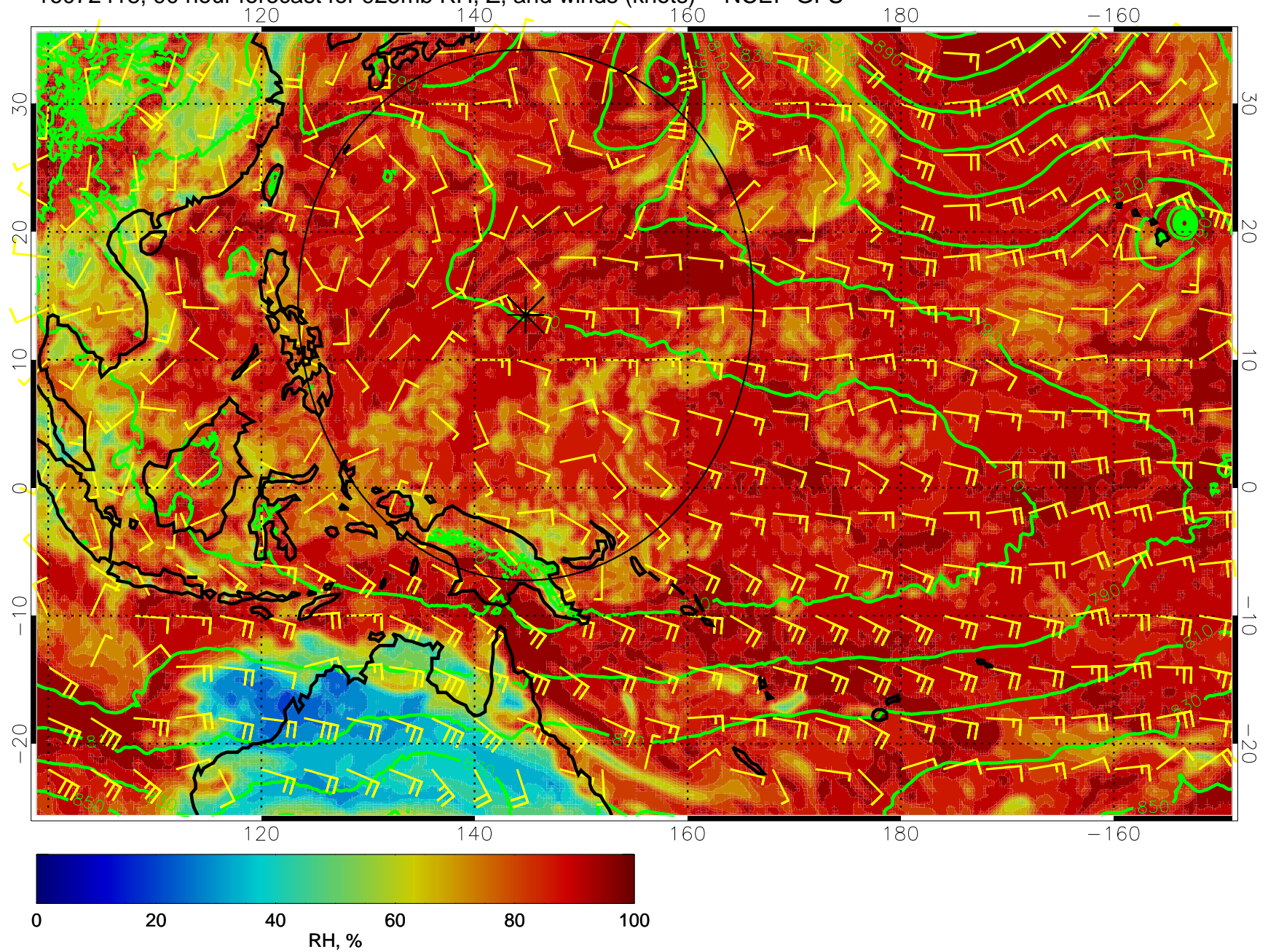
16072418, 90 hour forecast for 925mb RH, Z, and winds (knots) -- NCEP GFS
