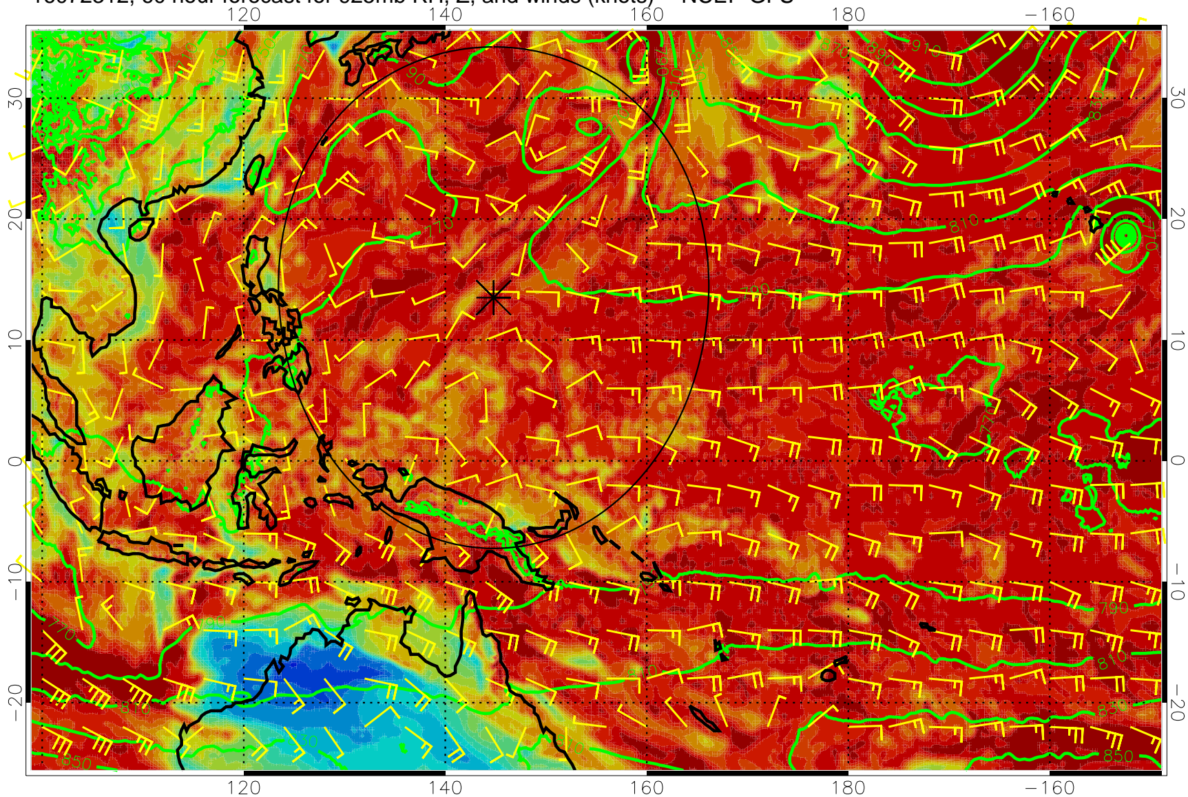
16072312, 60 hour forecast for 925mb RH, Z, and winds (knots) -- NCEP GFS
