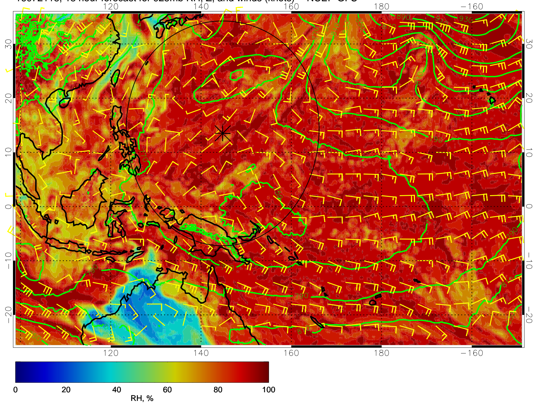
16072118, 18 hour forecast for 925mb RH, Z, and winds (knots) -- NCEP GFS
