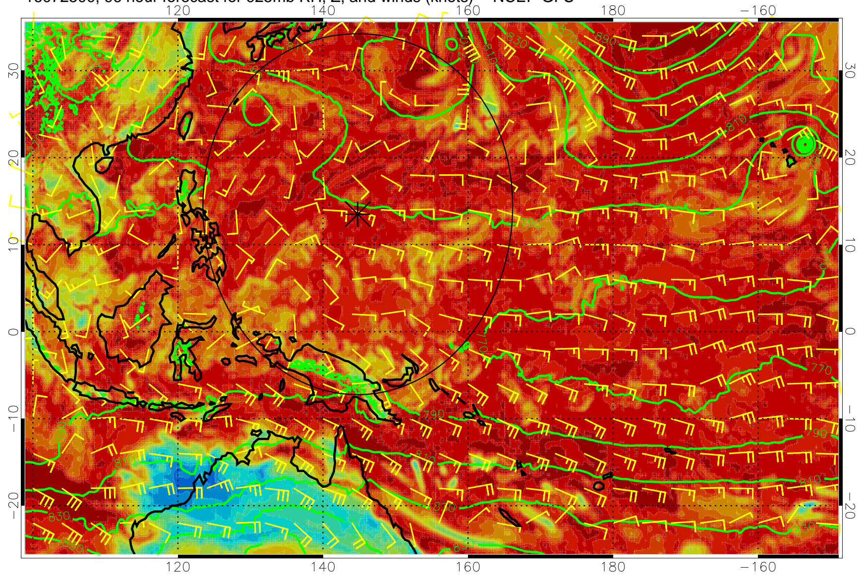
16072500, 96 hour forecast for 925mb RH, Z, and winds (knots) -- NCEP GFS
