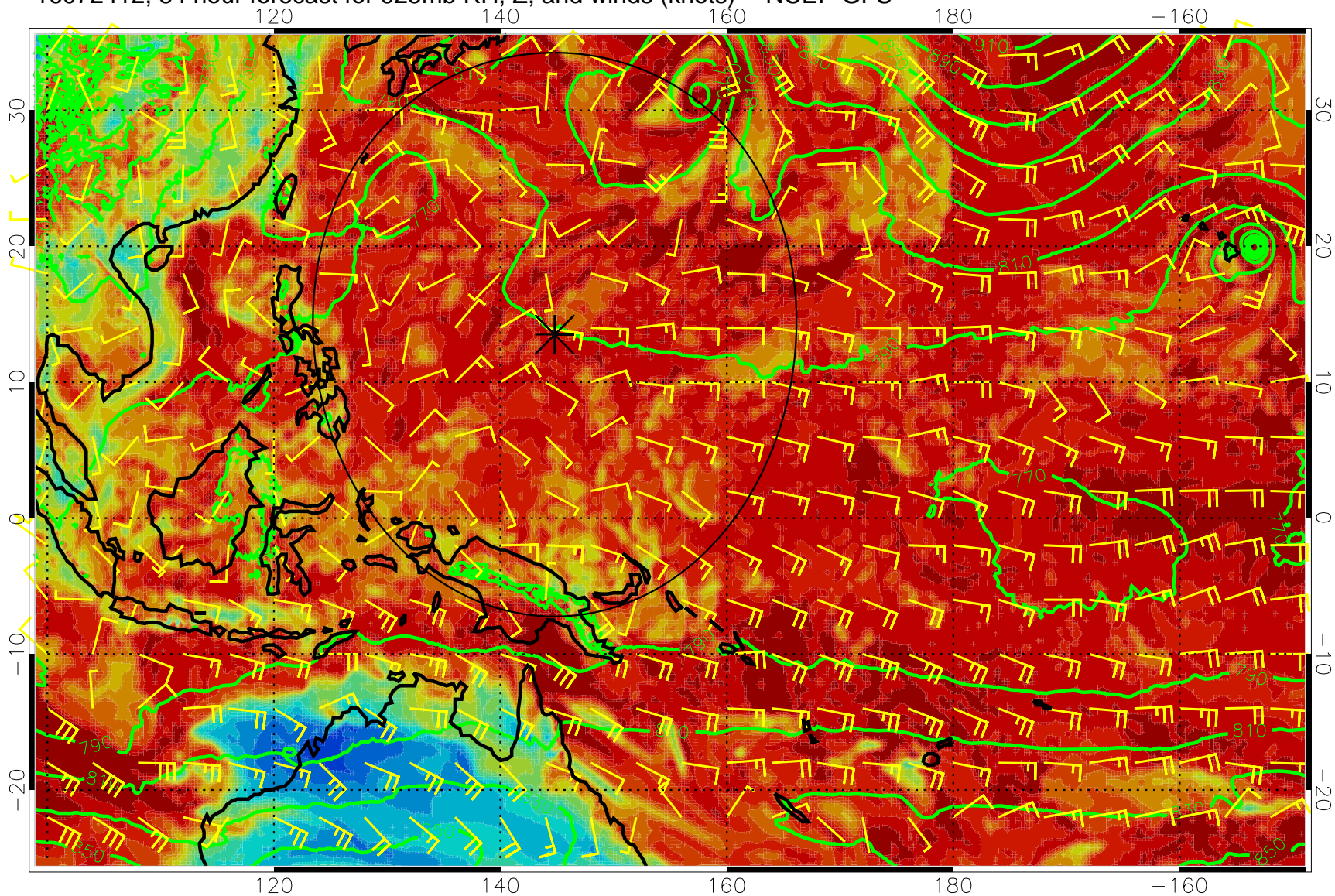
16072412, 84 hour forecast for 925mb RH, Z, and winds (knots) -- NCEP GFS
