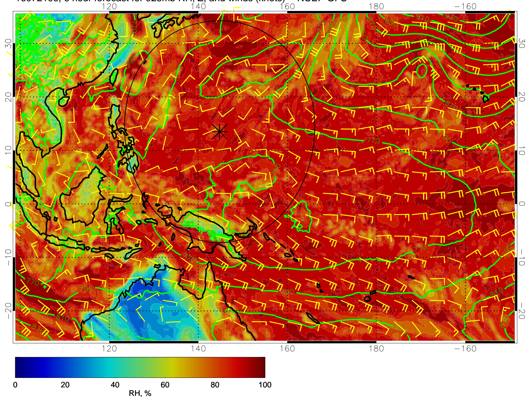
16072106, 6 hour forecast for 925mb RH, Z, and winds (knots) -- NCEP GFS
