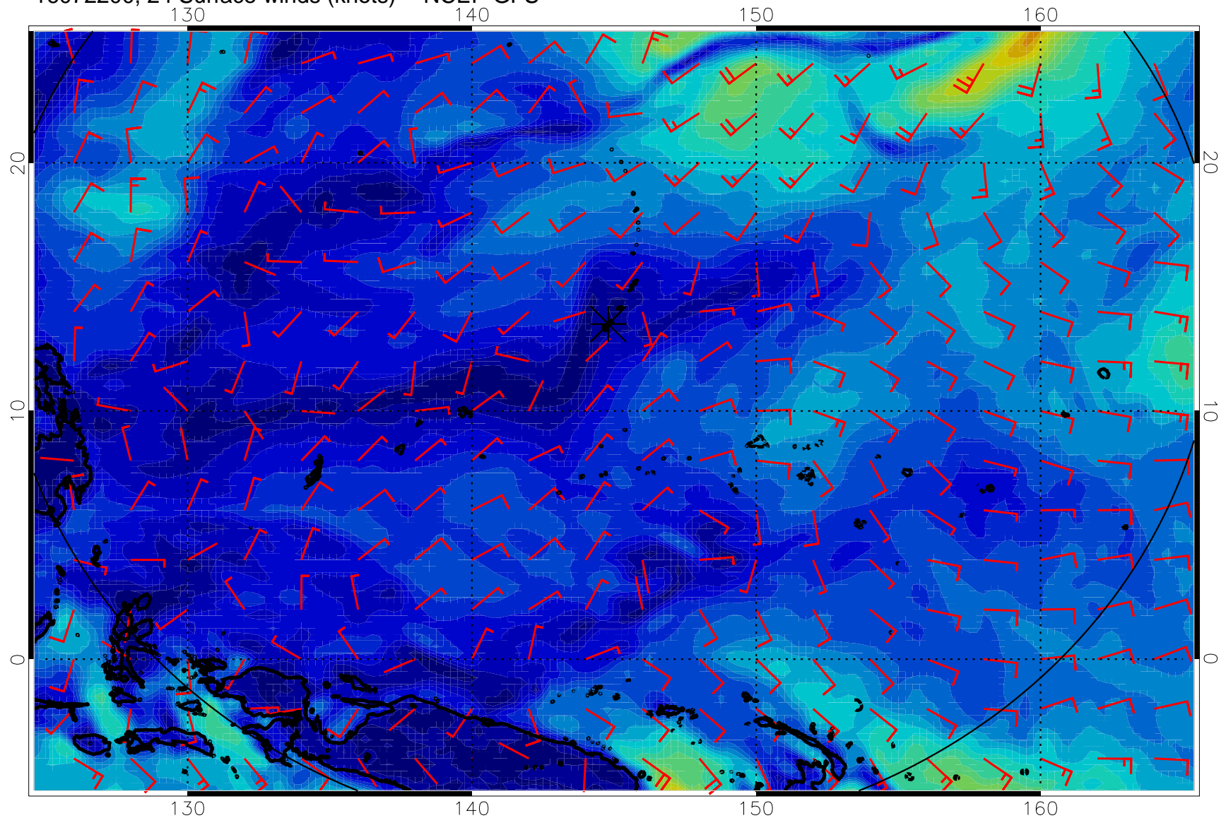
16072200, 24 Surface winds (knots) -- NCEP GFS
