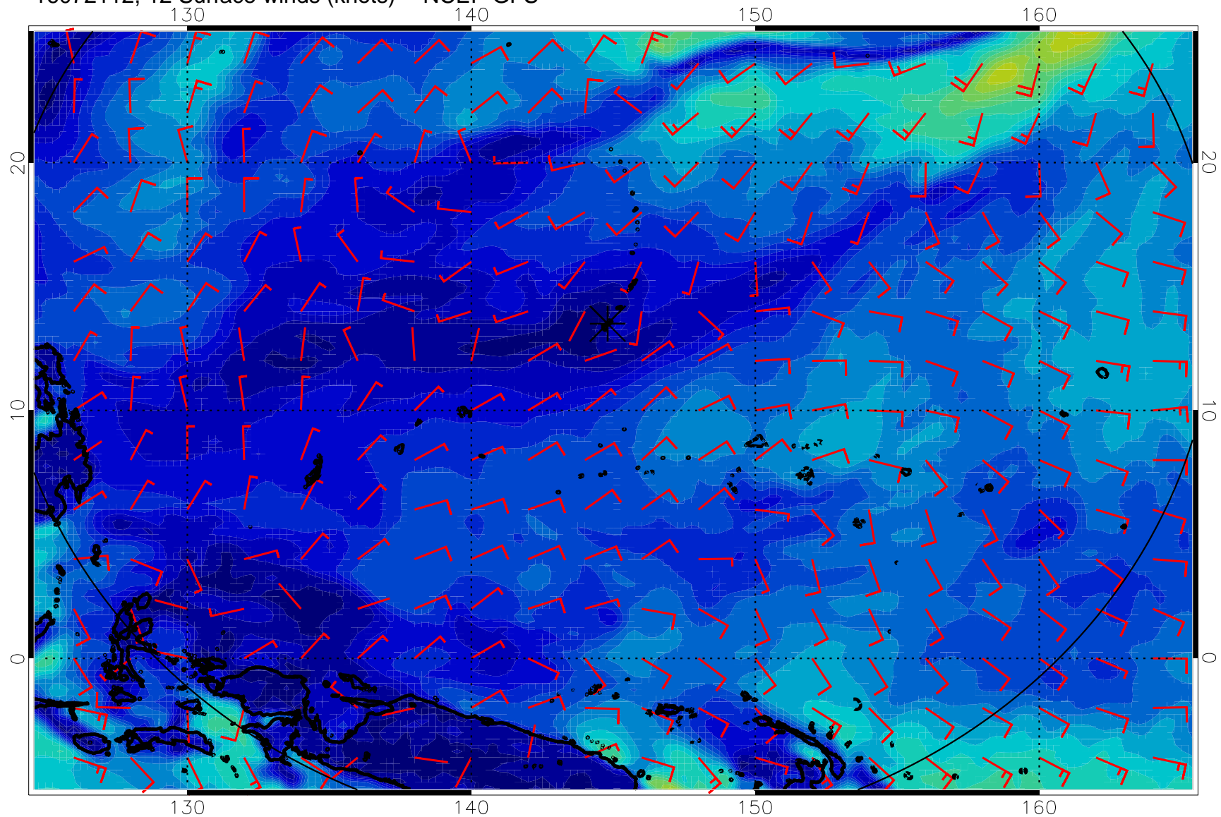
16072112, 12 Surface winds (knots) -- NCEP GFS
