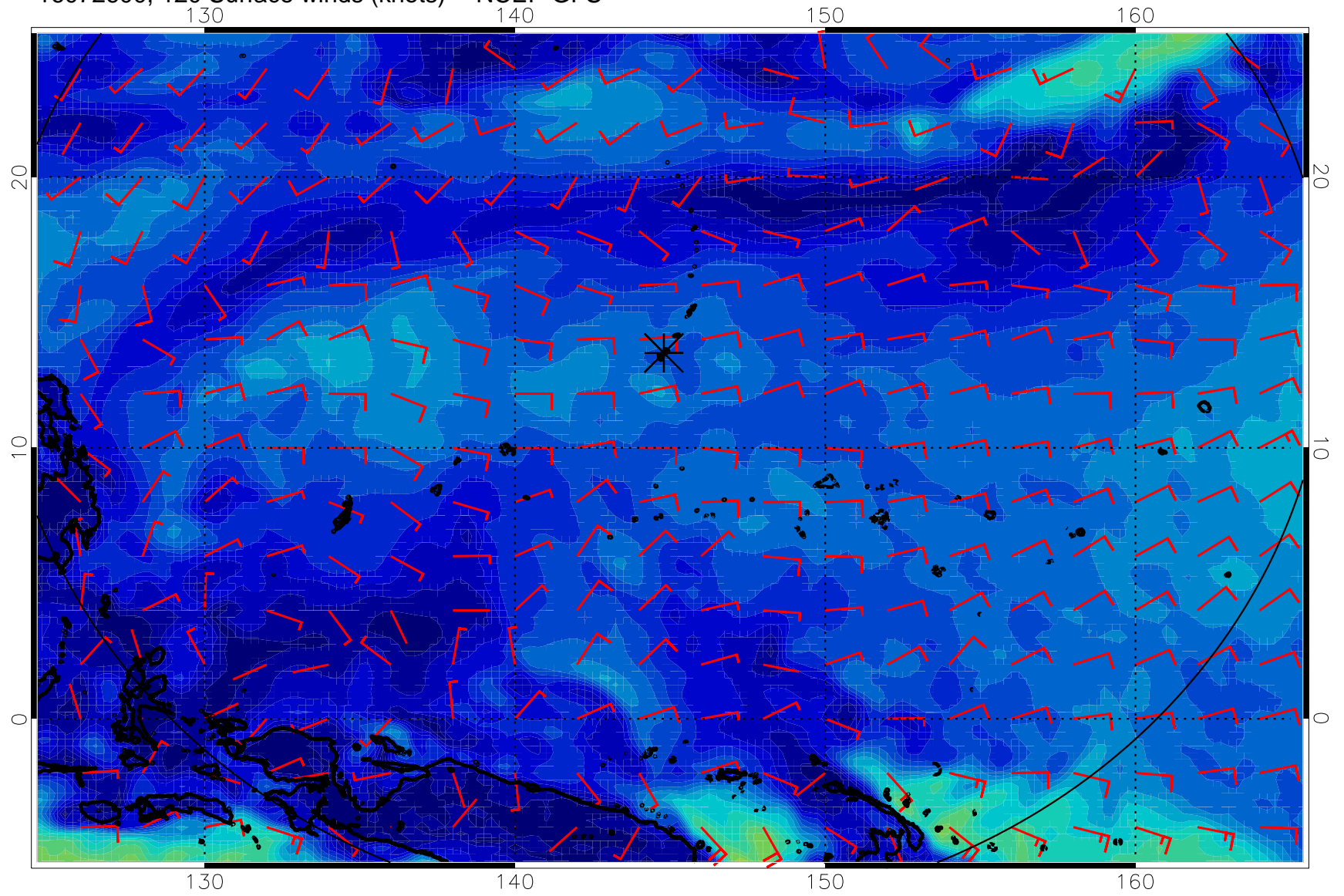
16072600, 120 Surface winds (knots) -- NCEP GFS
