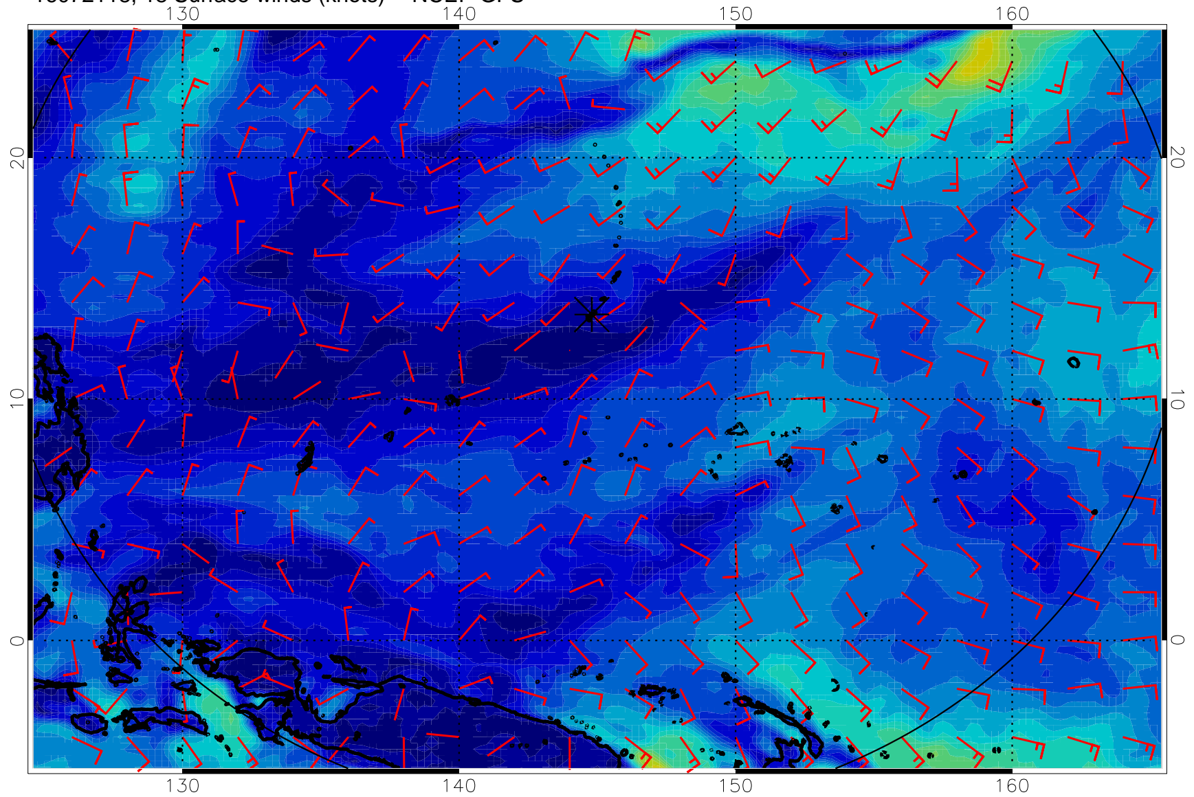
16072118, 18 Surface winds (knots) -- NCEP GFS
