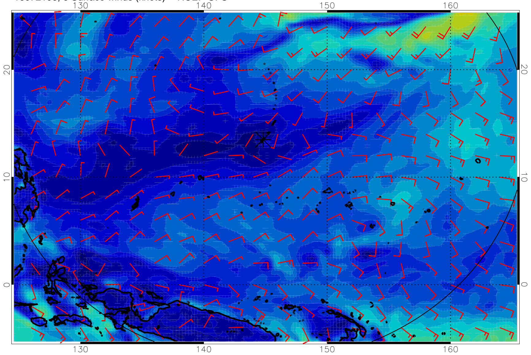
16072106, 6 Surface winds (knots) -- NCEP GFS
