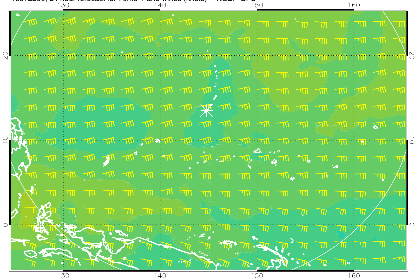
16072200, 24 hour forecast for 70mb T and winds (knots) -- NCEP GFS
