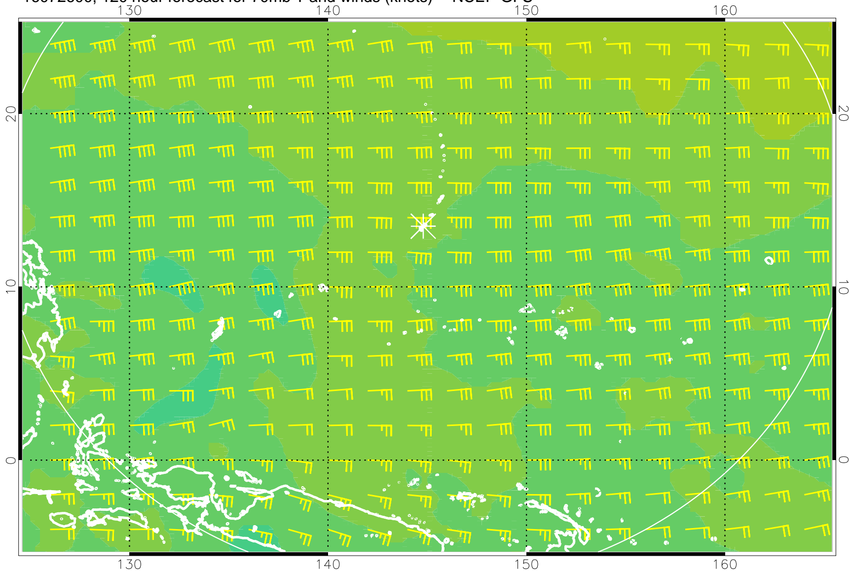
16072600, 120 hour forecast for 70mb T and winds (knots) -- NCEP GFS
