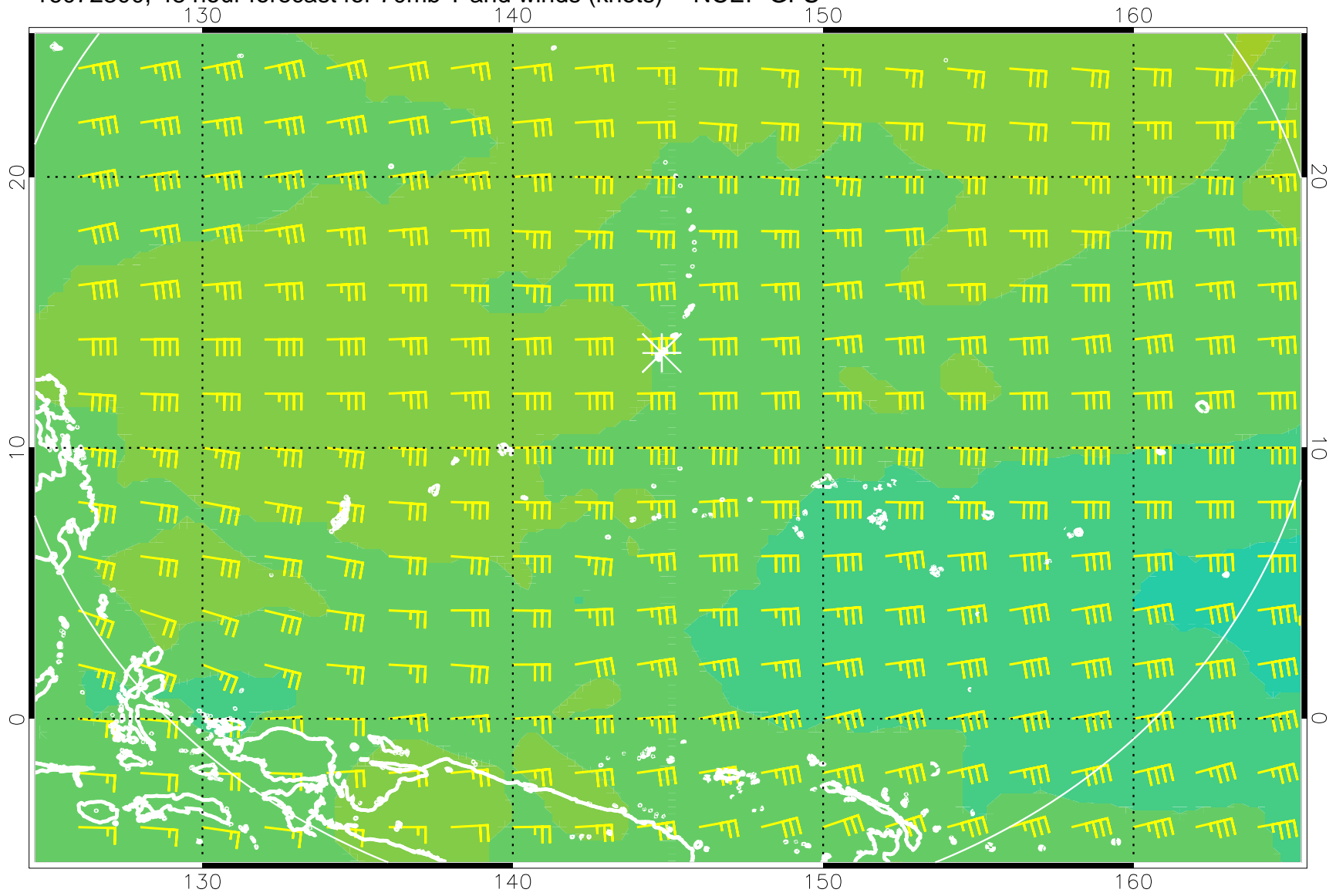
16072300, 48 hour forecast for 70mb T and winds (knots) -- NCEP GFS
