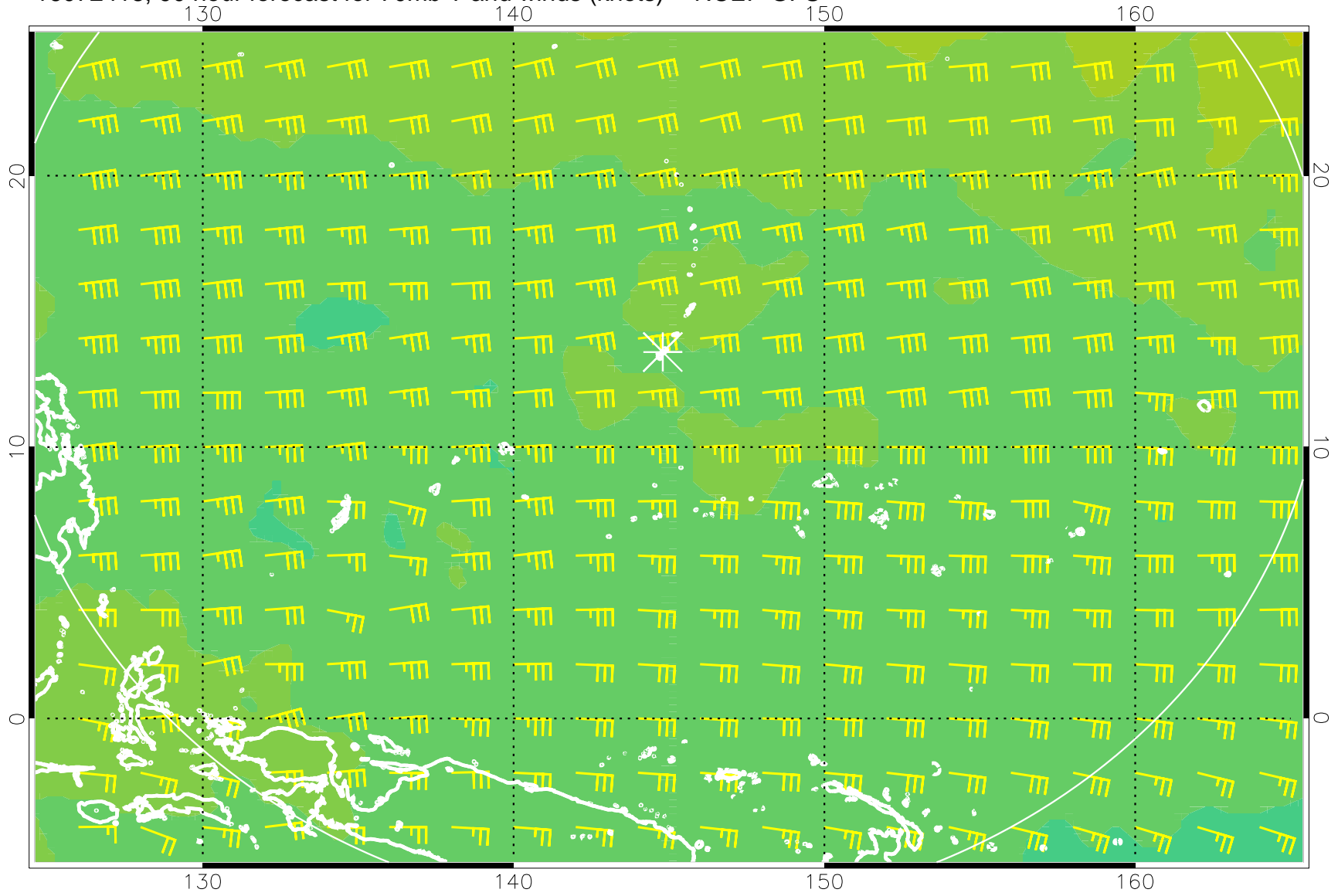
16072418, 90 hour forecast for 70mb T and winds (knots) -- NCEP GFS
