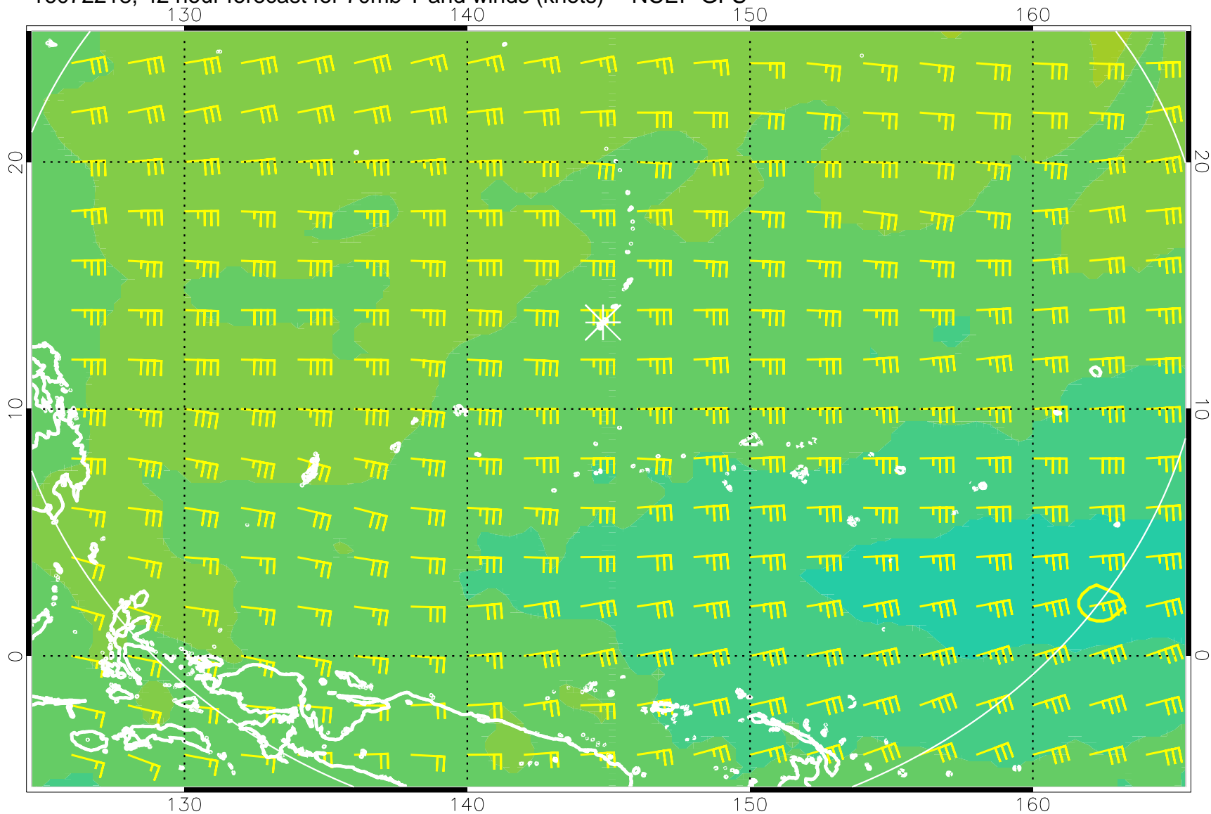
16072218, 42 hour forecast for 70mb T and winds (knots) -- NCEP GFS
