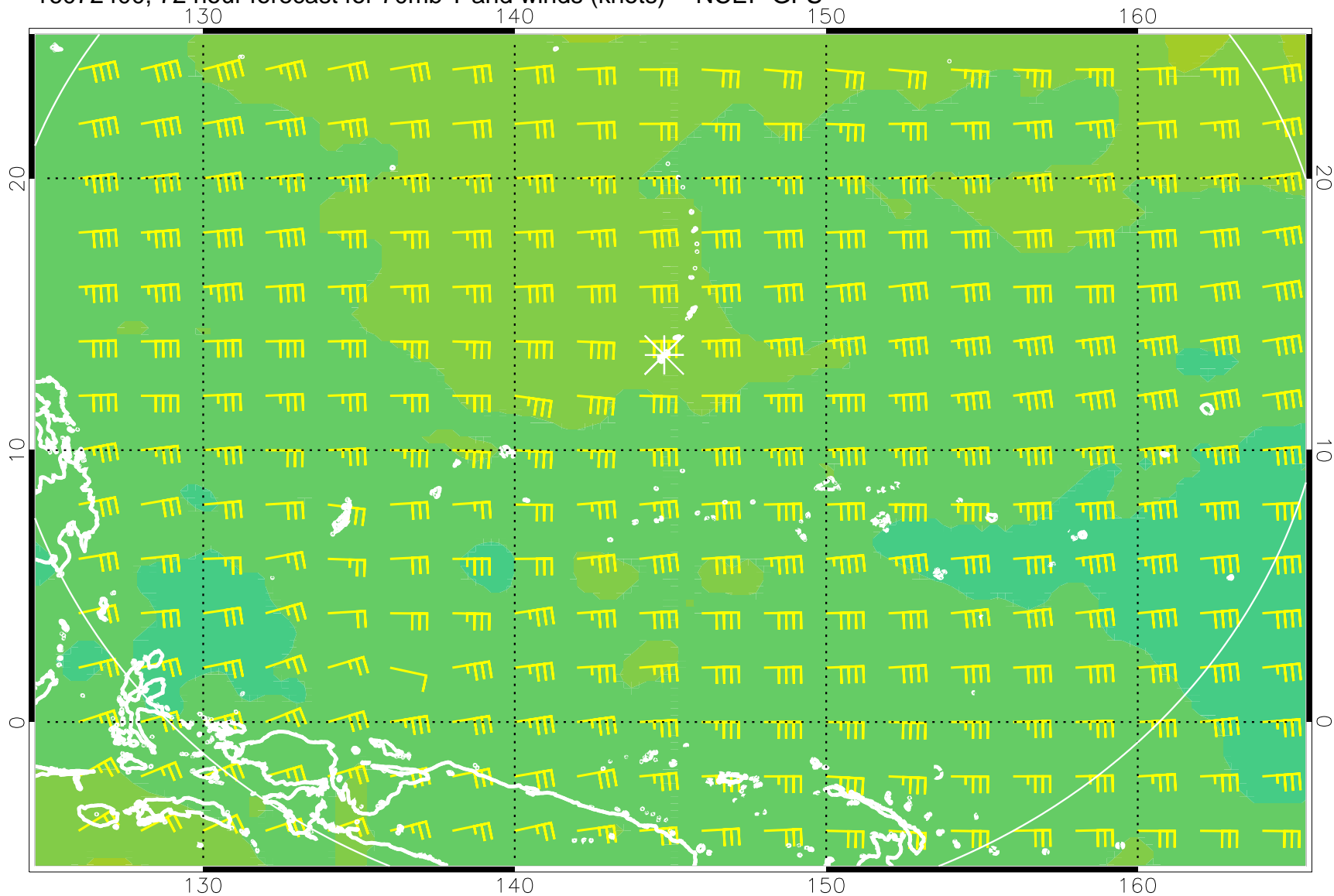
16072400, 72 hour forecast for 70mb T and winds (knots) -- NCEP GFS
