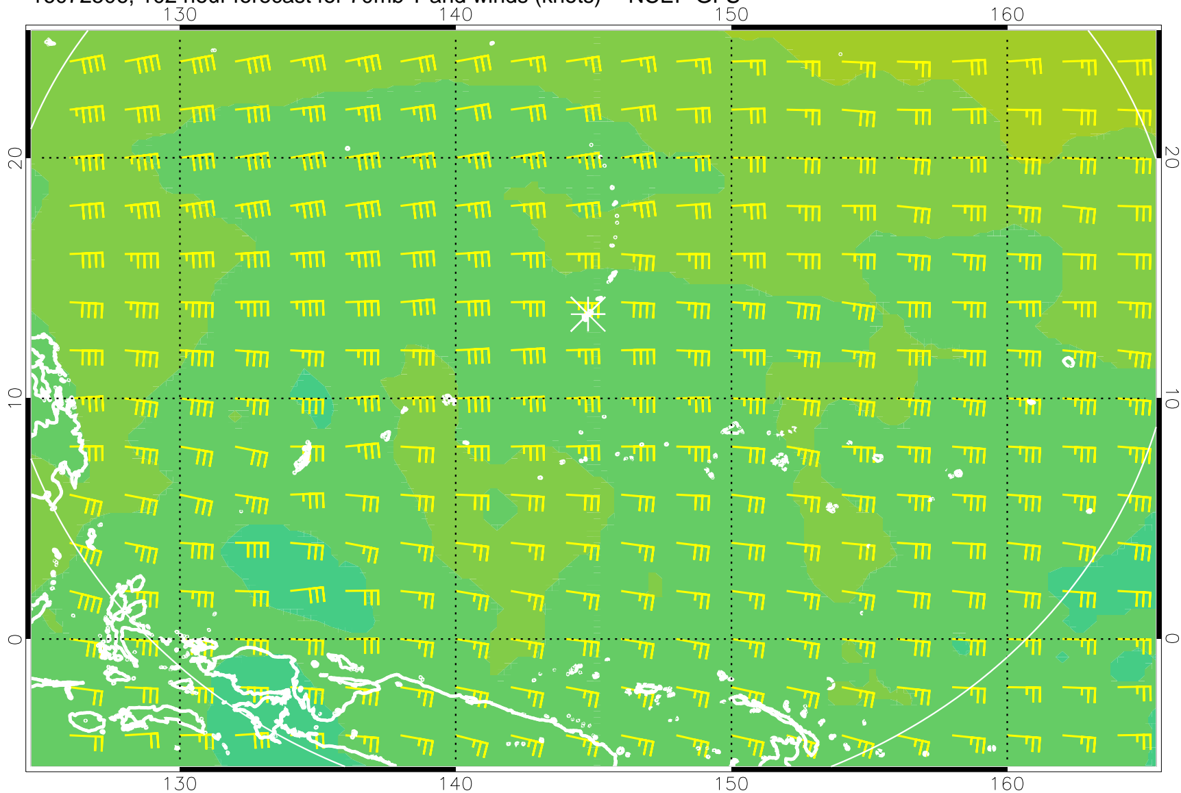
16072506, 102 hour forecast for 70mb T and winds (knots) -- NCEP GFS
