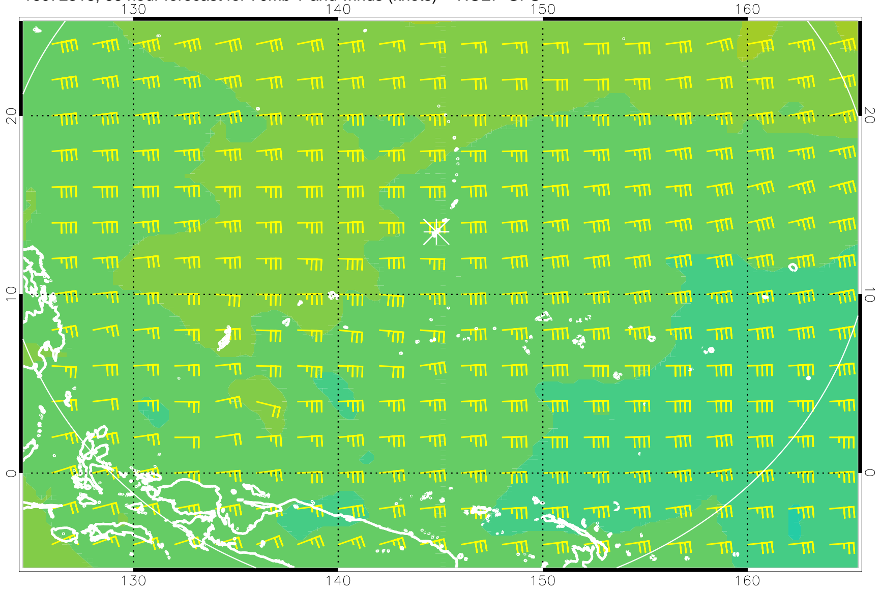
16072318, 66 hour forecast for 70mb T and winds (knots) -- NCEP GFS
