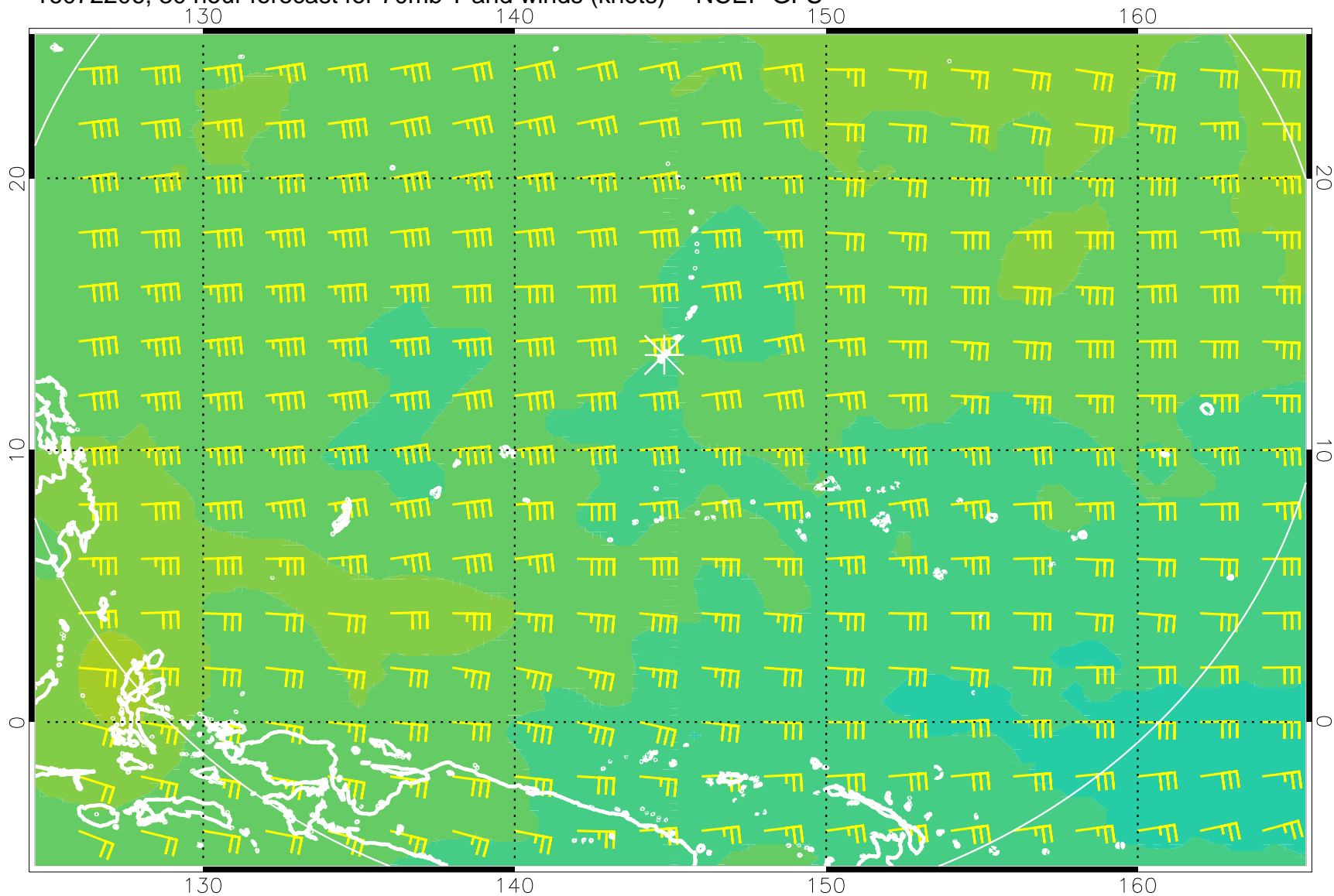
16072206, 30 hour forecast for 70mb T and winds (knots) -- NCEP GFS
