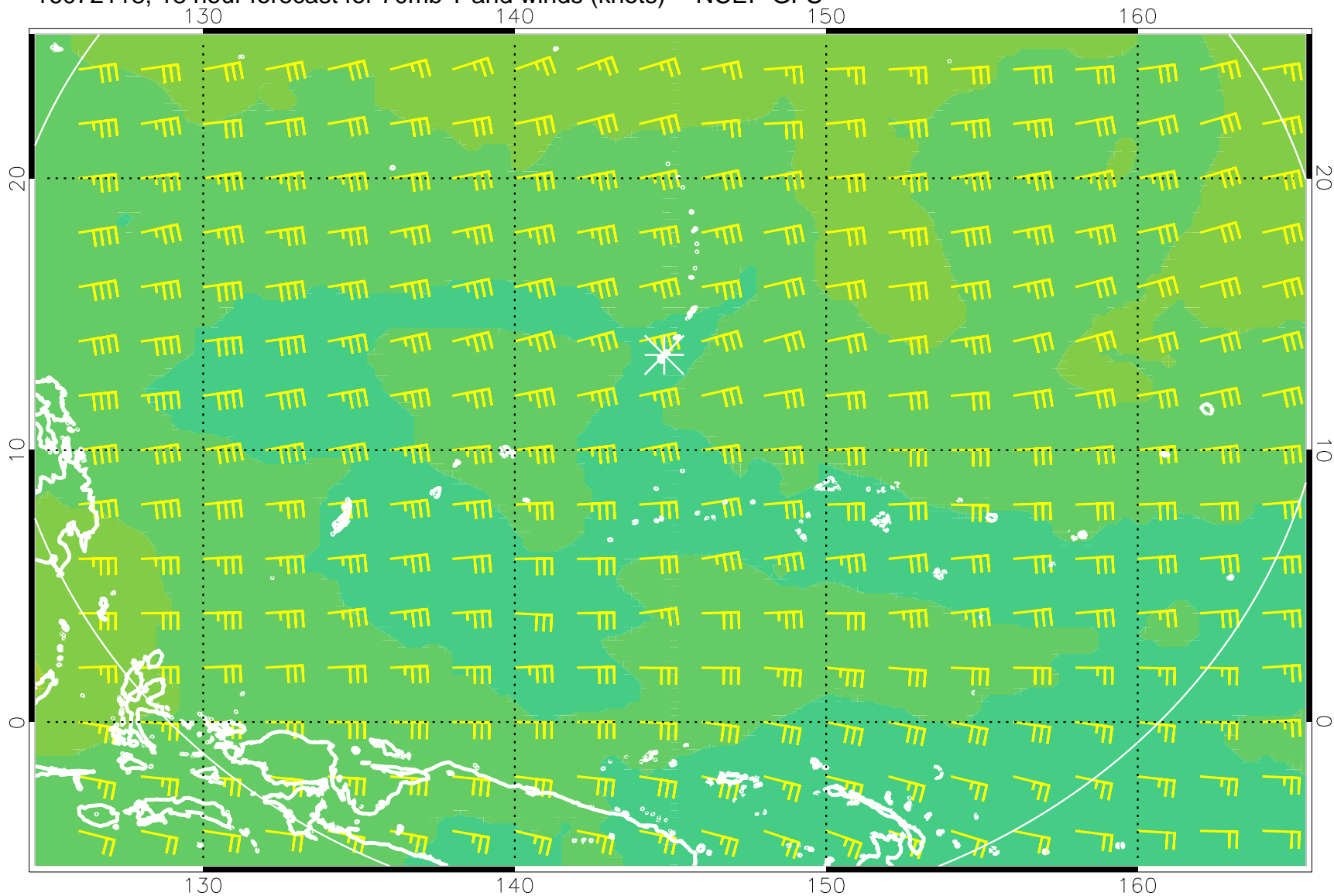
16072118, 18 hour forecast for 70mb T and winds (knots) -- NCEP GFS
