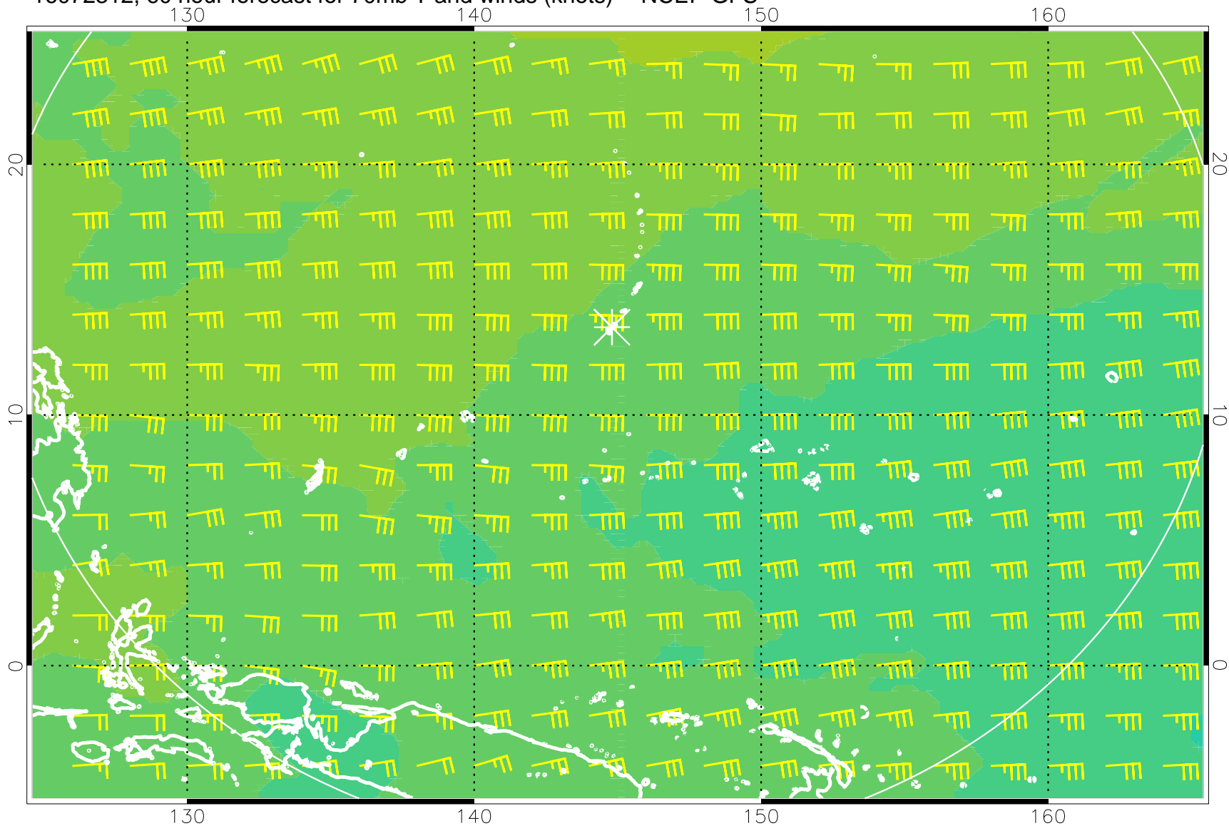
16072312, 60 hour forecast for 70mb T and winds (knots) -- NCEP GFS
