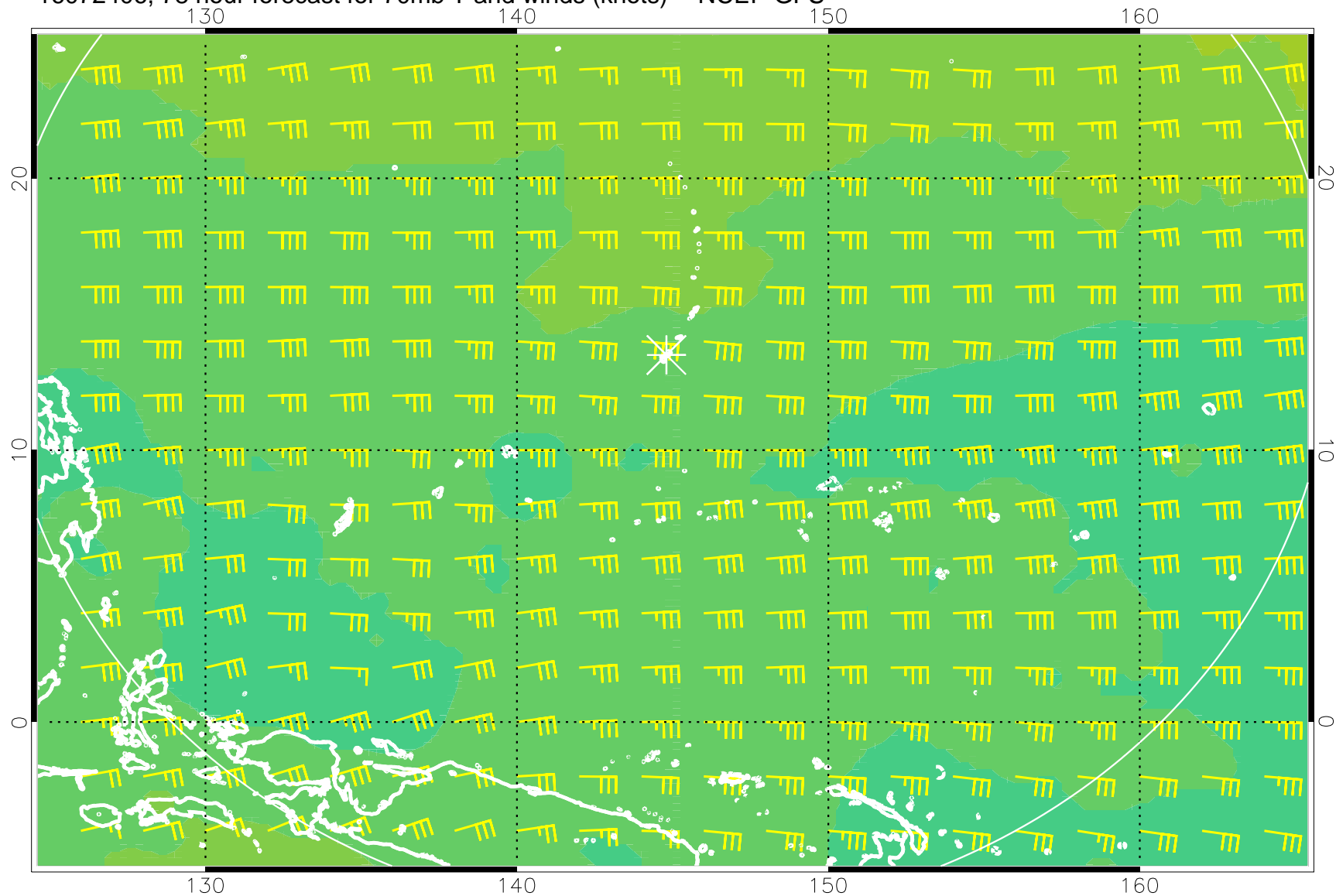
16072406, 78 hour forecast for 70mb T and winds (knots) -- NCEP GFS
