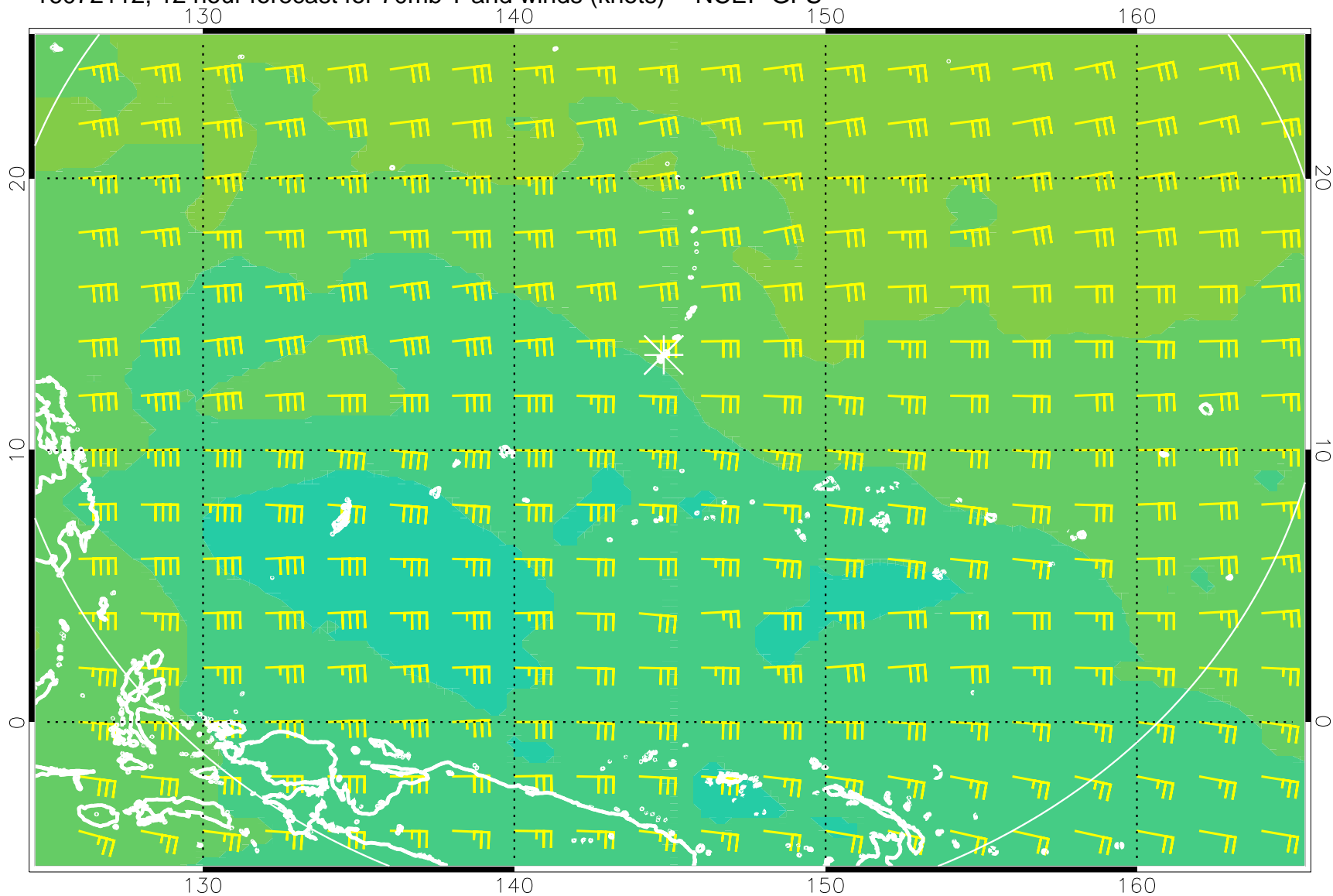
16072112, 12 hour forecast for 70mb T and winds (knots) -- NCEP GFS
