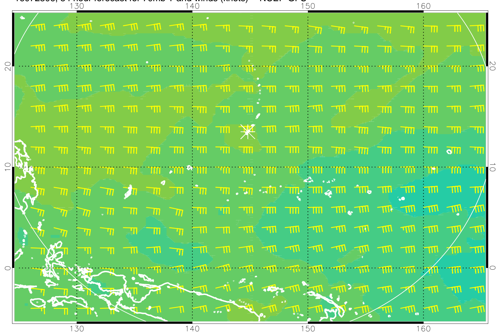
16072306, 54 hour forecast for 70mb T and winds (knots) -- NCEP GFS
