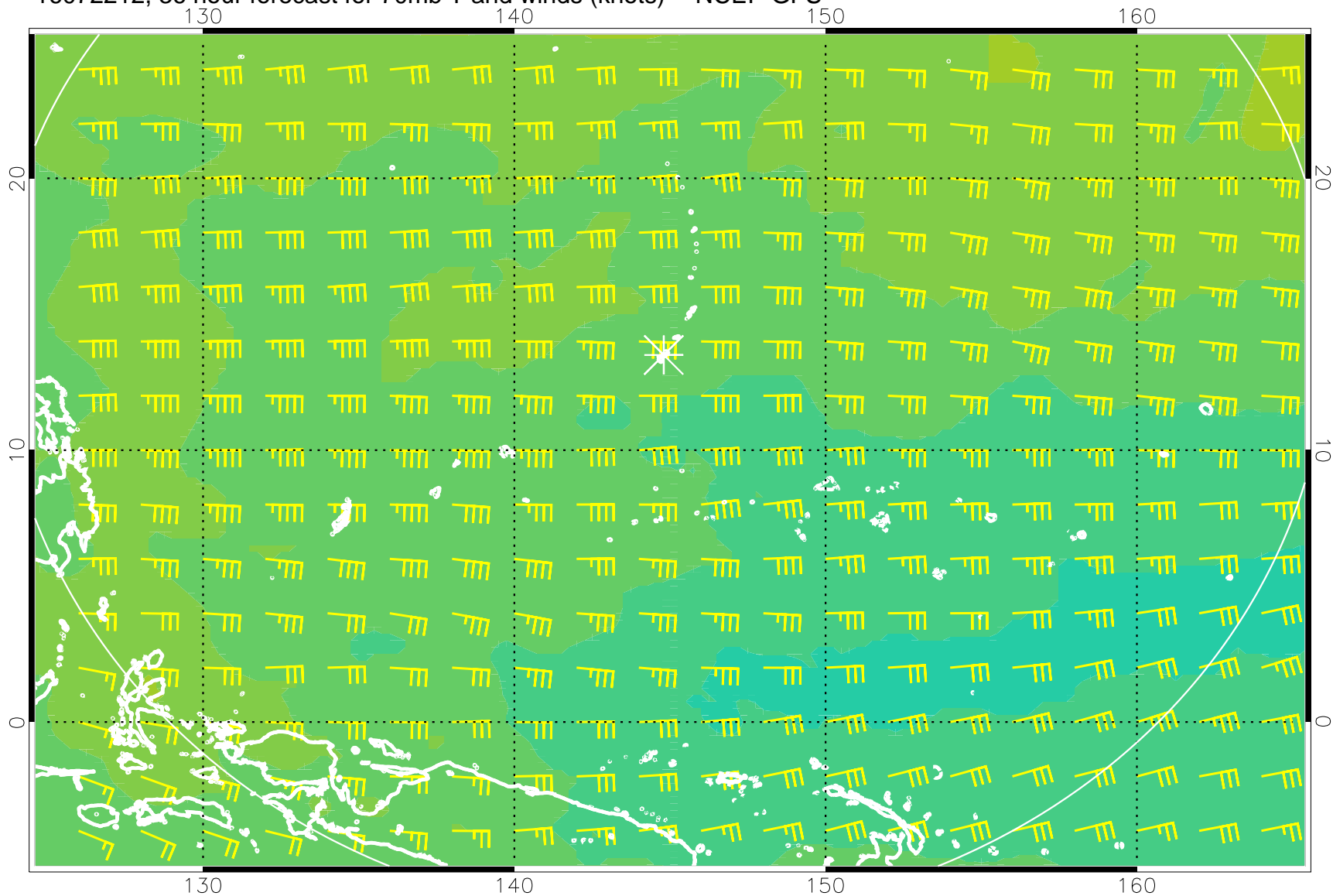
16072212, 36 hour forecast for 70mb T and winds (knots) -- NCEP GFS
