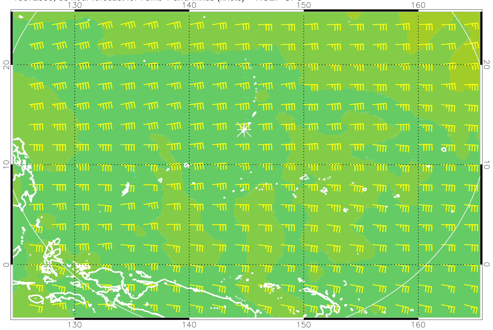
16072500, 96 hour forecast for 70mb T and winds (knots) -- NCEP GFS
