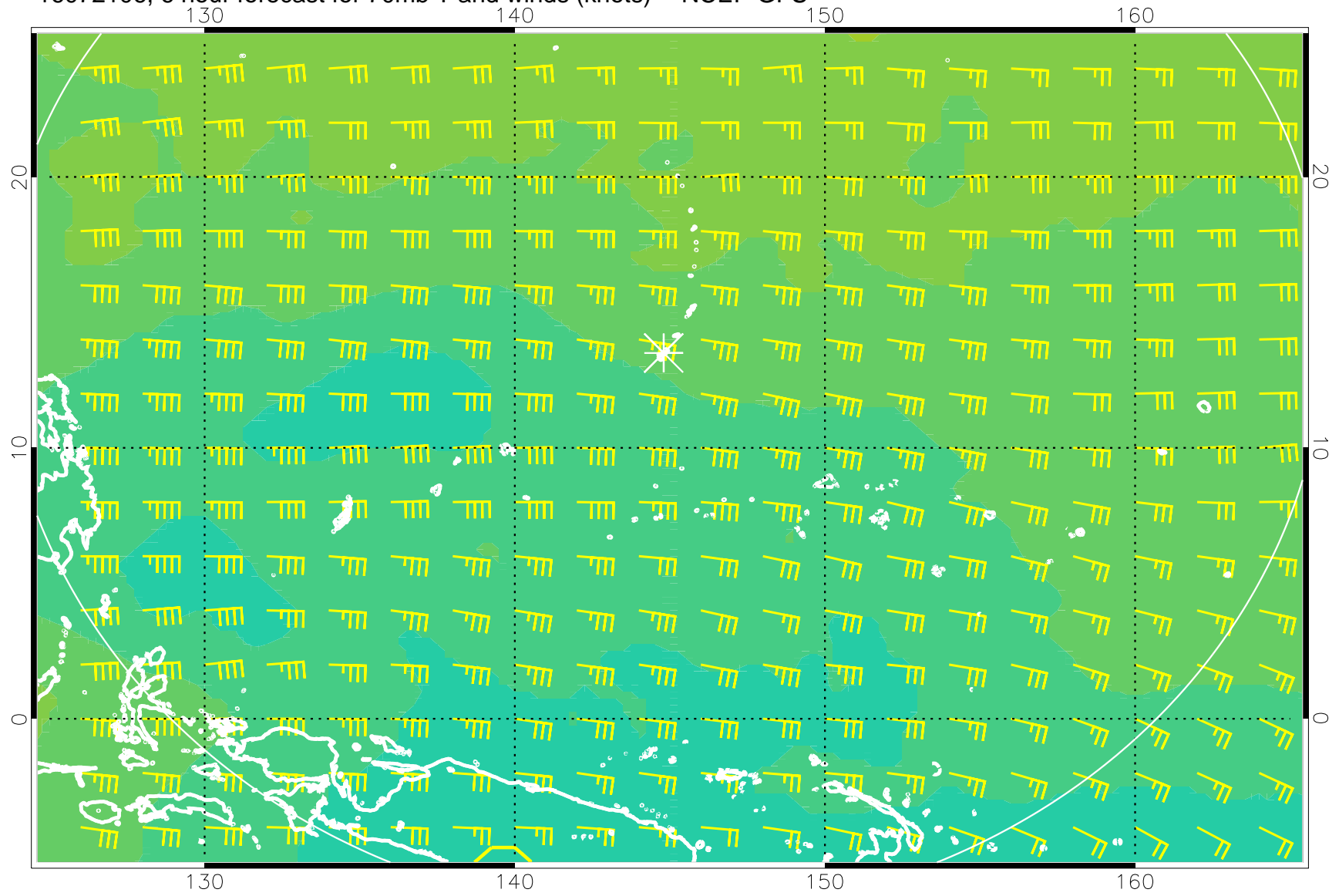
16072106, 6 hour forecast for 70mb T and winds (knots) -- NCEP GFS
