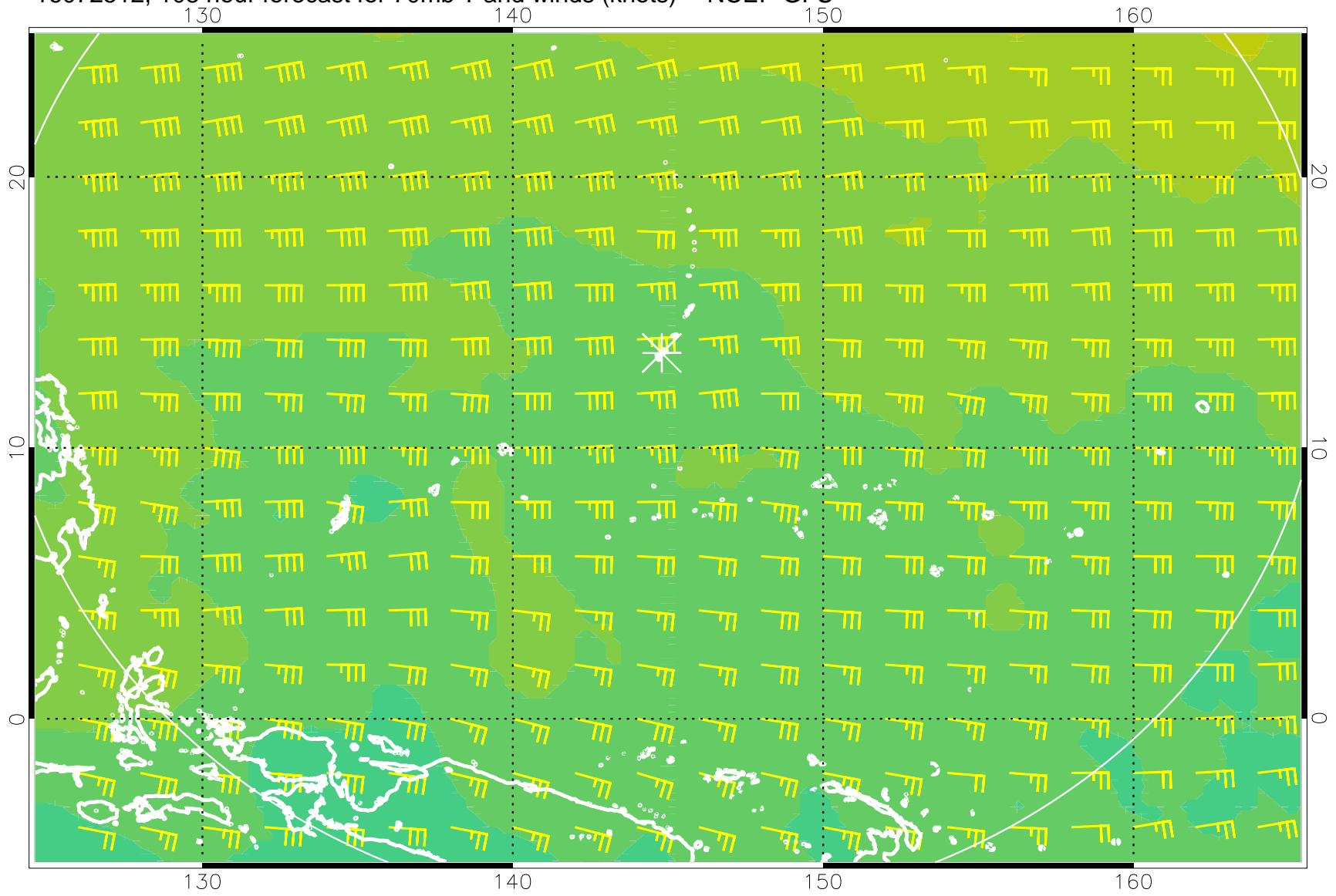
16072512, 108 hour forecast for 70mb T and winds (knots) -- NCEP GFS
