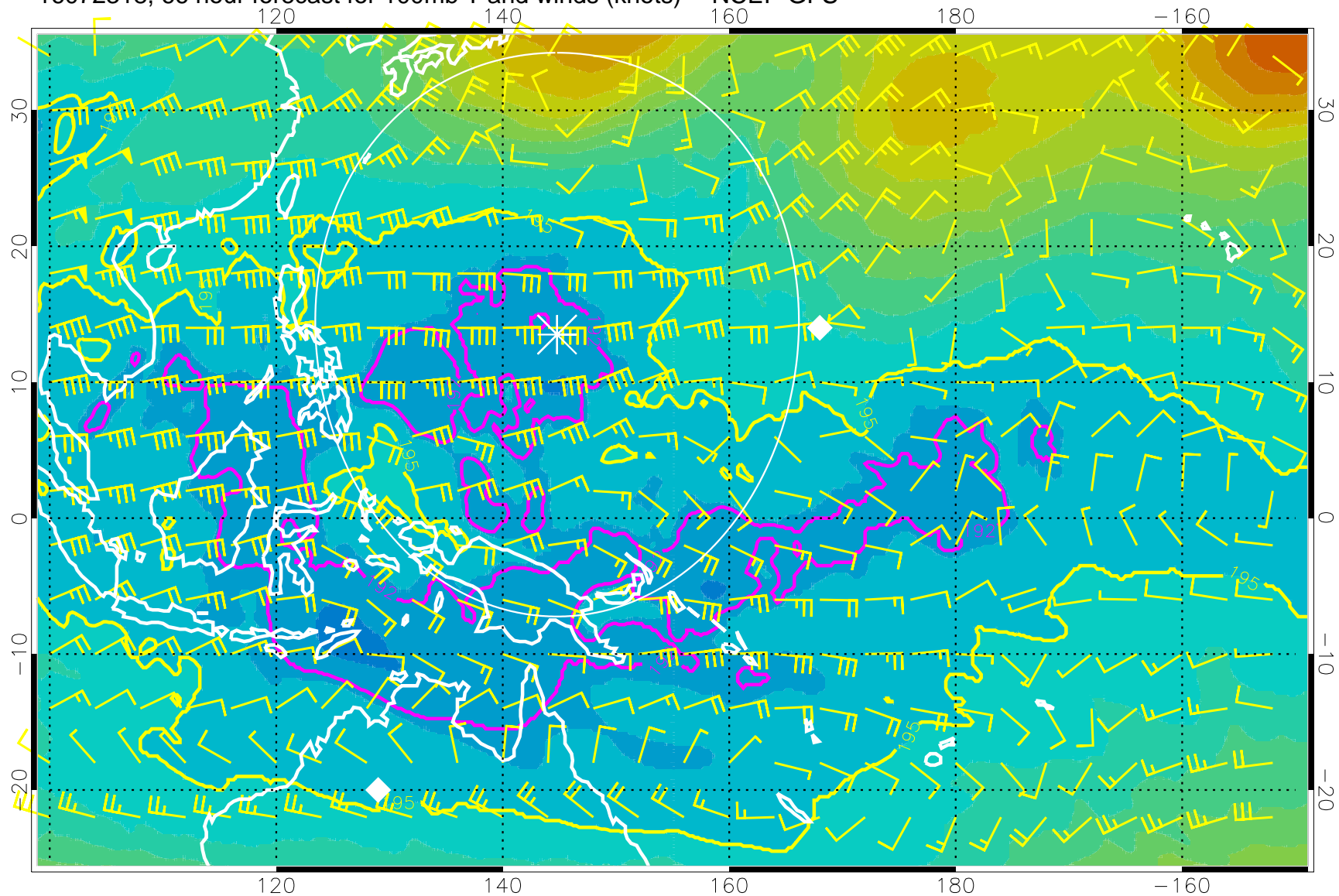
16072318, 66 hour forecast for 100mb T and winds (knots) -- NCEP GFS
