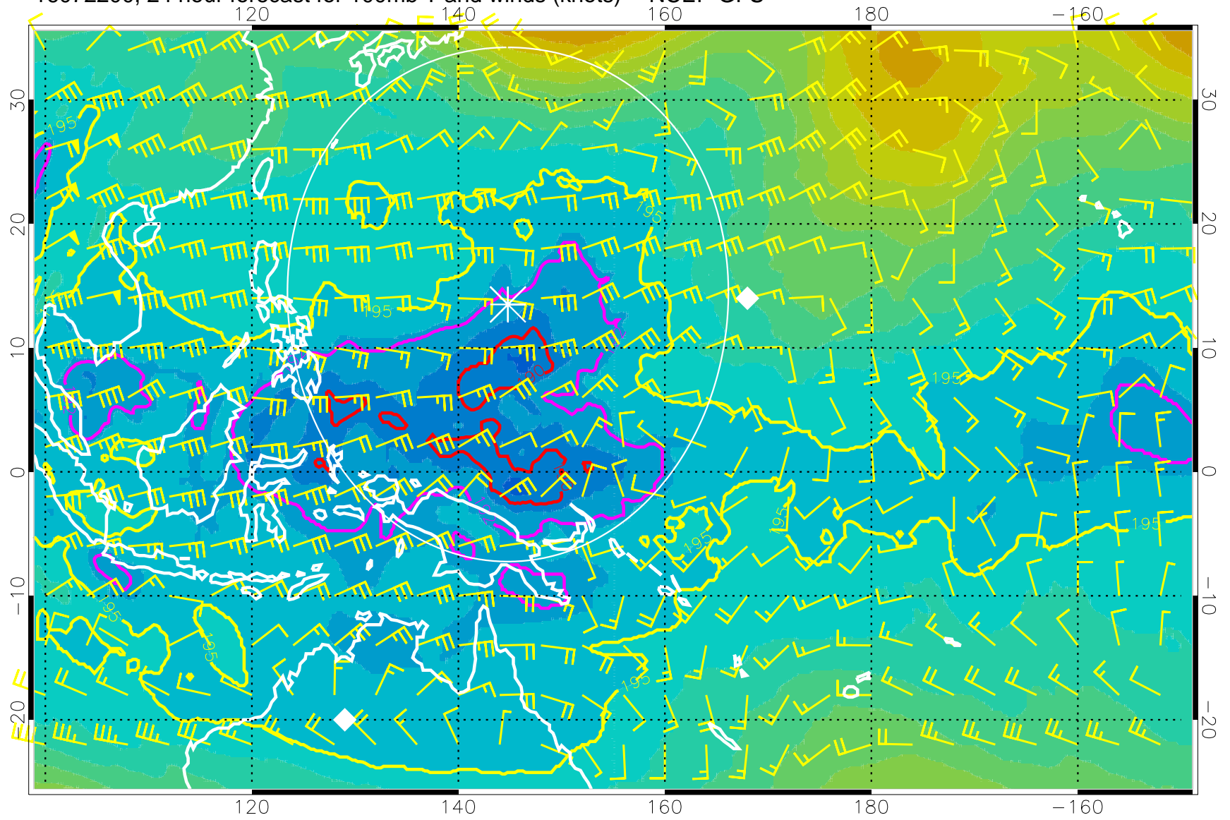
16072200, 24 hour forecast for 100mb T and winds (knots) -- NCEP GFS
