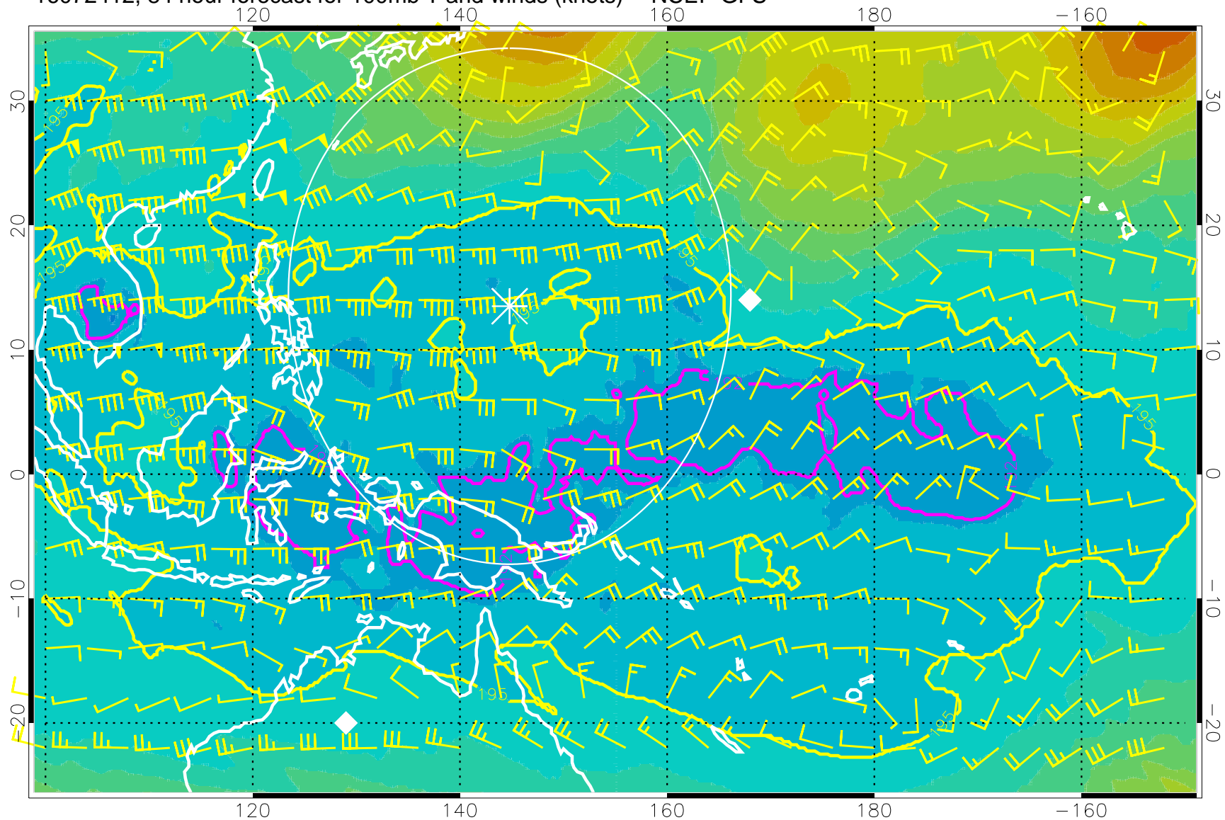
16072412, 84 hour forecast for 100mb T and winds (knots) -- NCEP GFS
