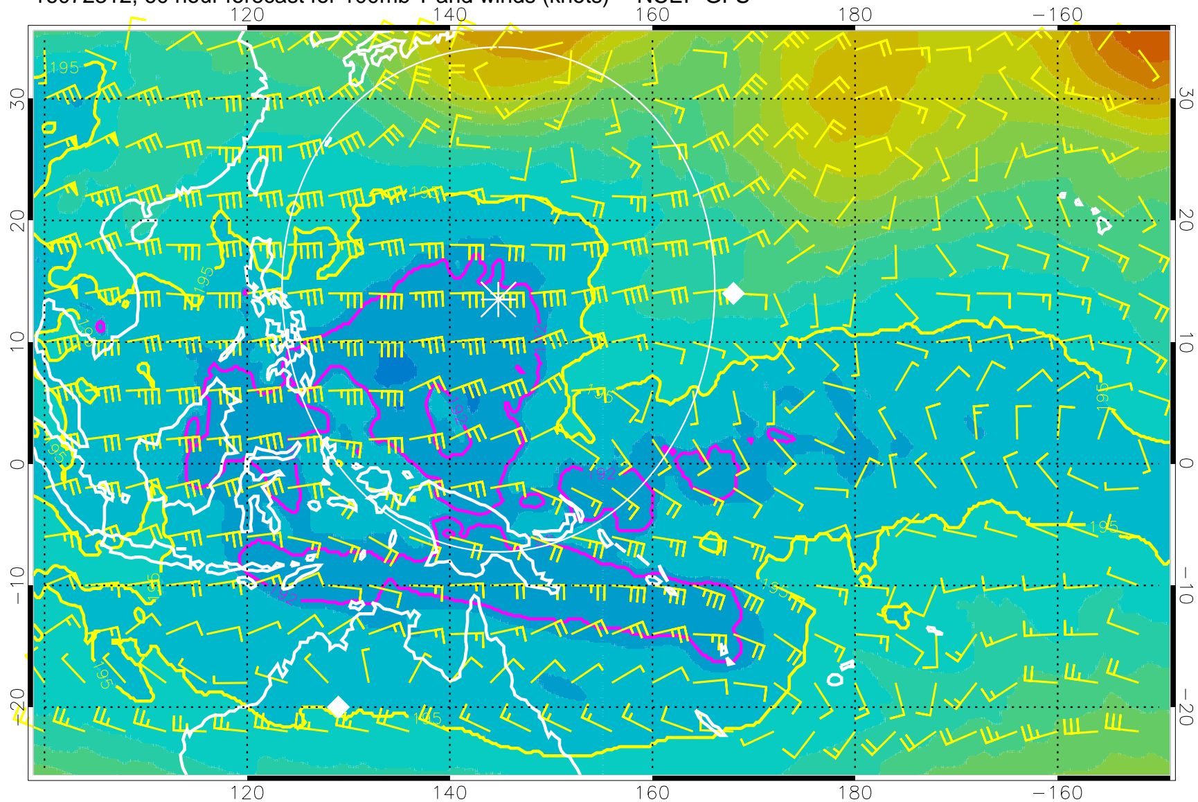
16072312, 60 hour forecast for 100mb T and winds (knots) -- NCEP GFS
