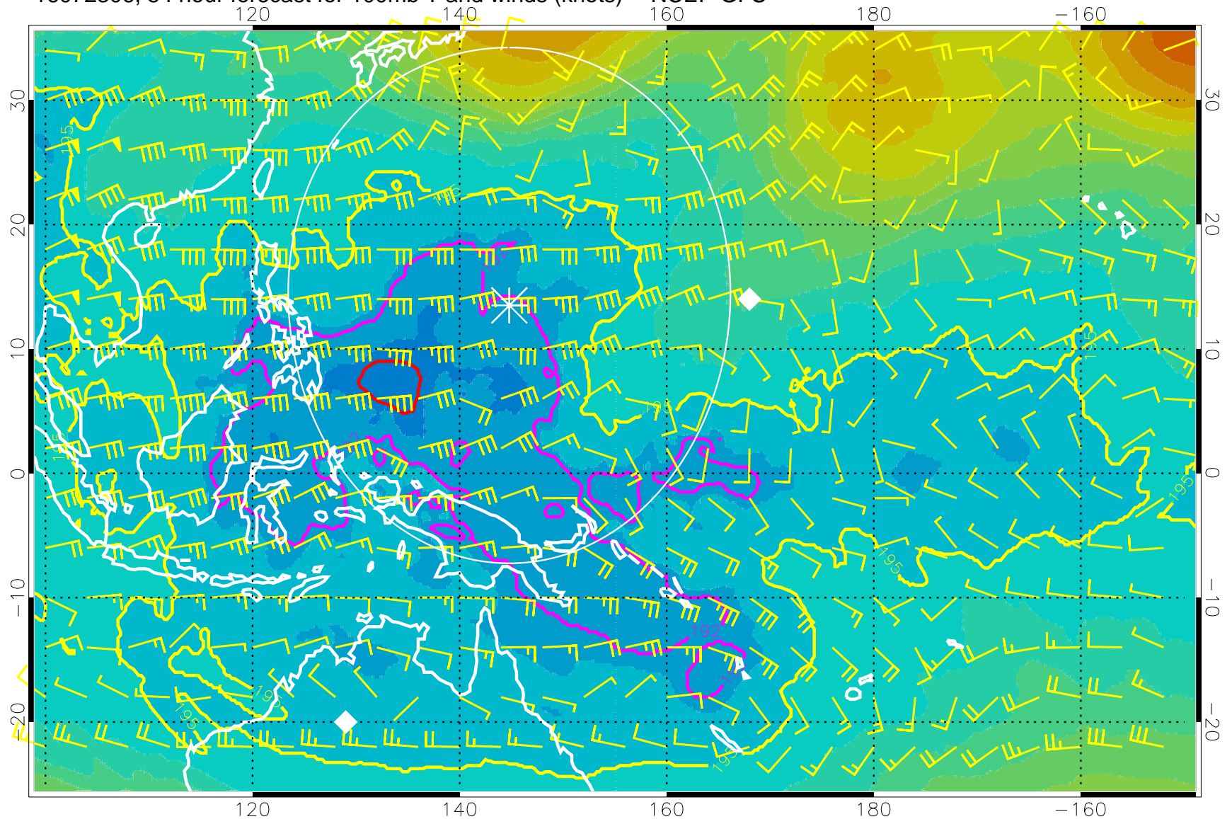
16072306, 54 hour forecast for 100mb T and winds (knots) -- NCEP GFS
