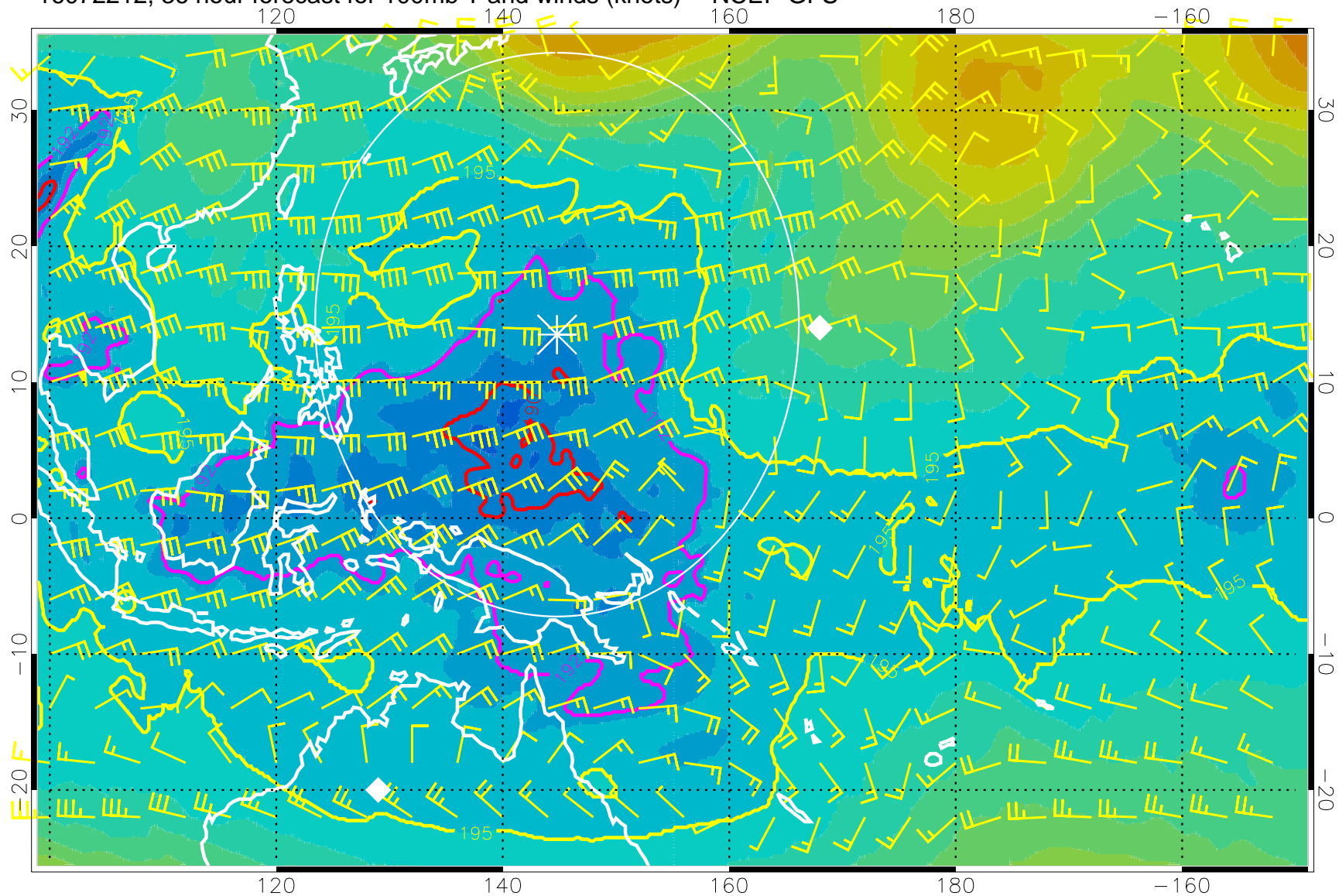
16072212, 36 hour forecast for 100mb T and winds (knots) -- NCEP GFS
