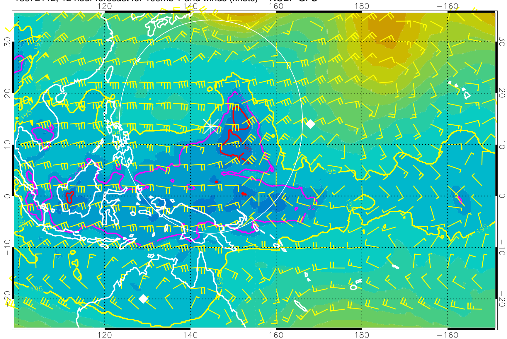
16072112, 12 hour forecast for 100mb T and winds (knots) -- NCEP GFS
