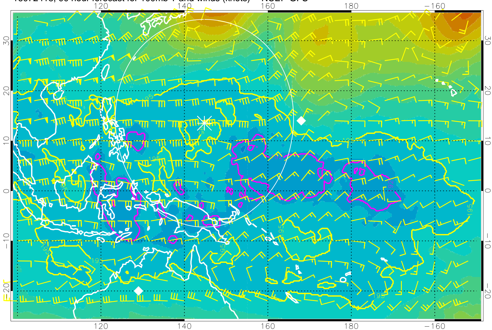
16072418, 90 hour forecast for 100mb T and winds (knots) -- NCEP GFS
