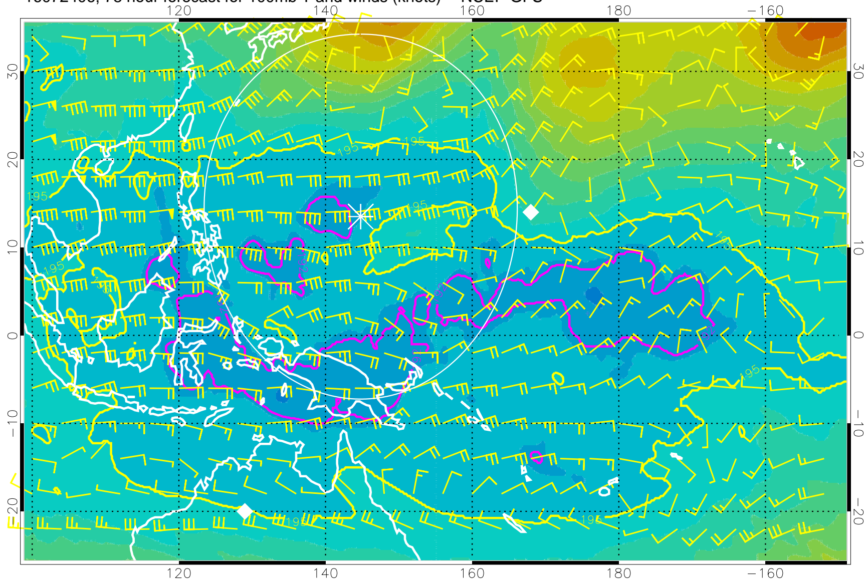
16072406, 78 hour forecast for 100mb T and winds (knots) -- NCEP GFS
