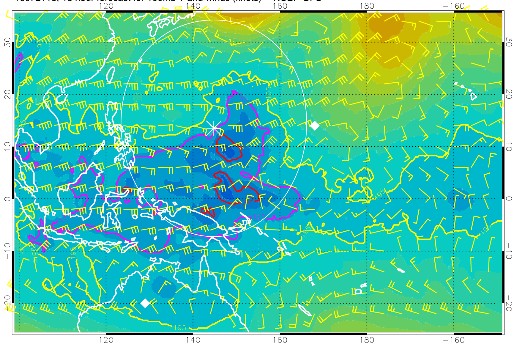
16072118, 18 hour forecast for 100mb T and winds (knots) -- NCEP GFS
