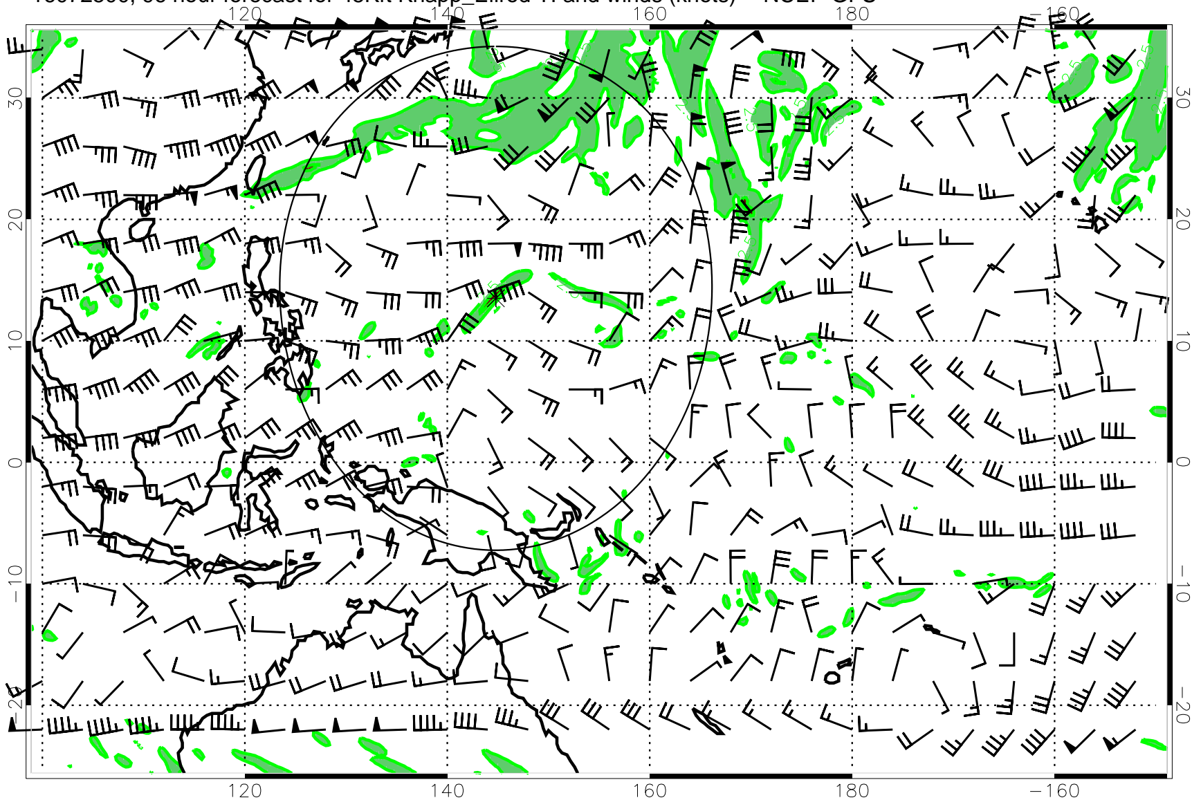
16072500, 96 hour forecast for 45Kft Knapp_Ellrod TI and winds (knots) -- NCEP GFS
