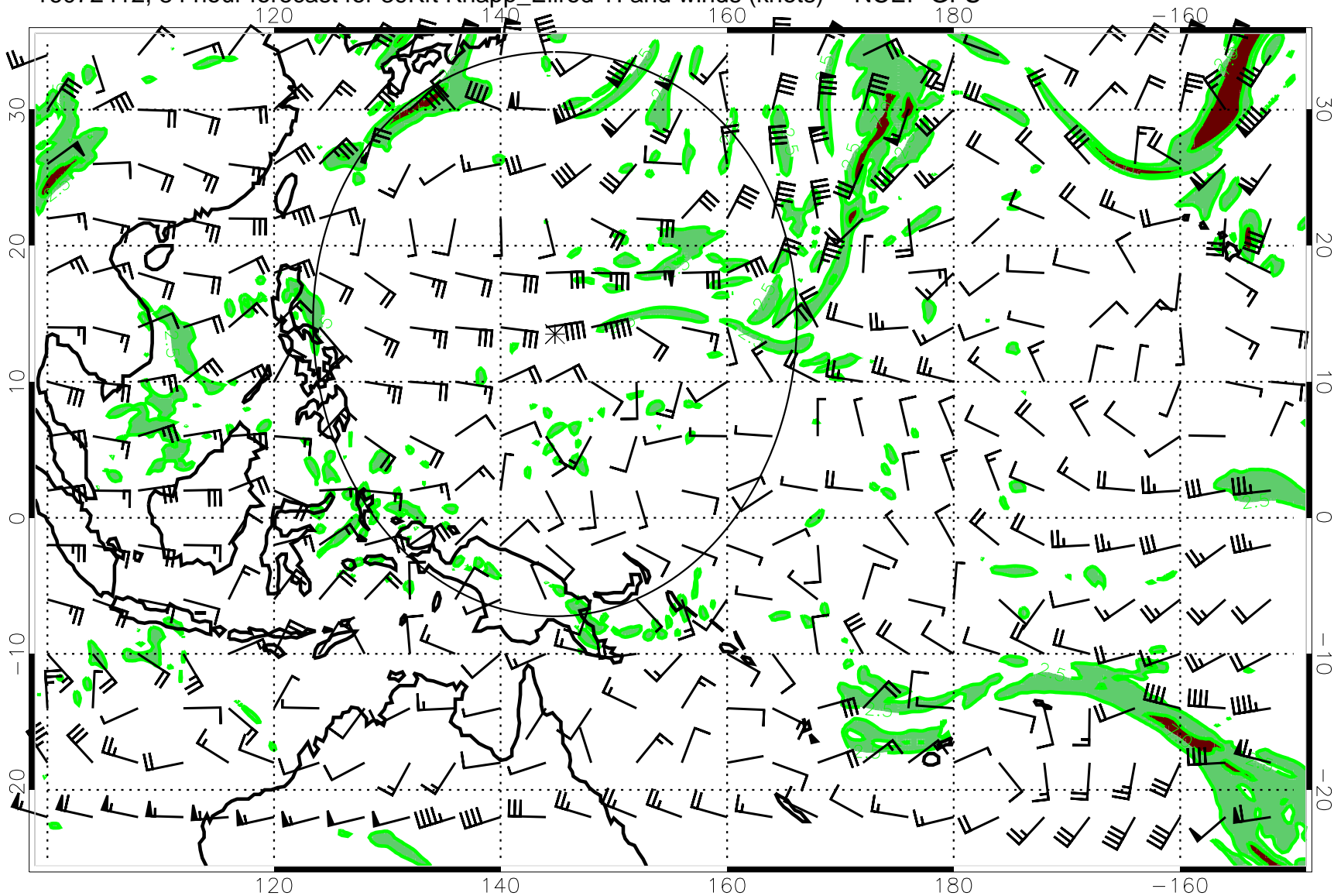
16072412, 84 hour forecast for 39Kft Knapp_Ellrod TI and winds (knots) -- NCEP GFS
