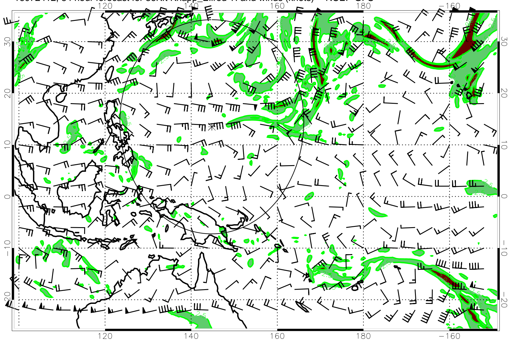
16072412, 84 hour forecast for 36Kft Knapp_Ellrod TI and winds (knots) -- NCEP GFS
