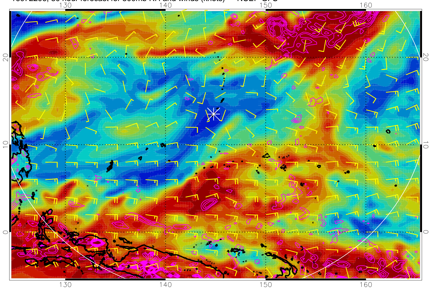
16072206, 30 hour forecast for 500mb RH and winds (knots) -- NCEP GFS
