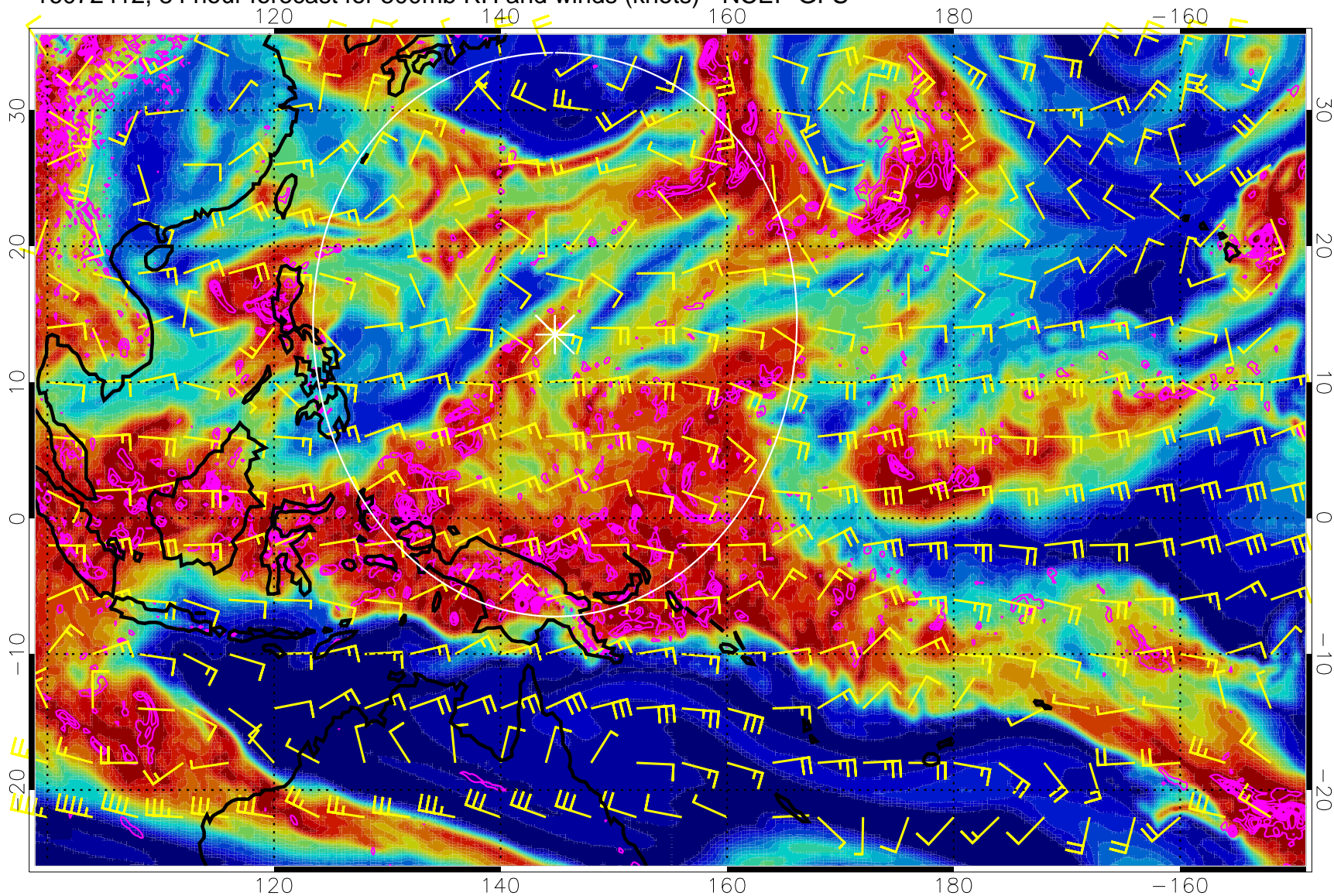
16072412, 84 hour forecast for 500mb RH and winds (knots) - NCEP GFS
