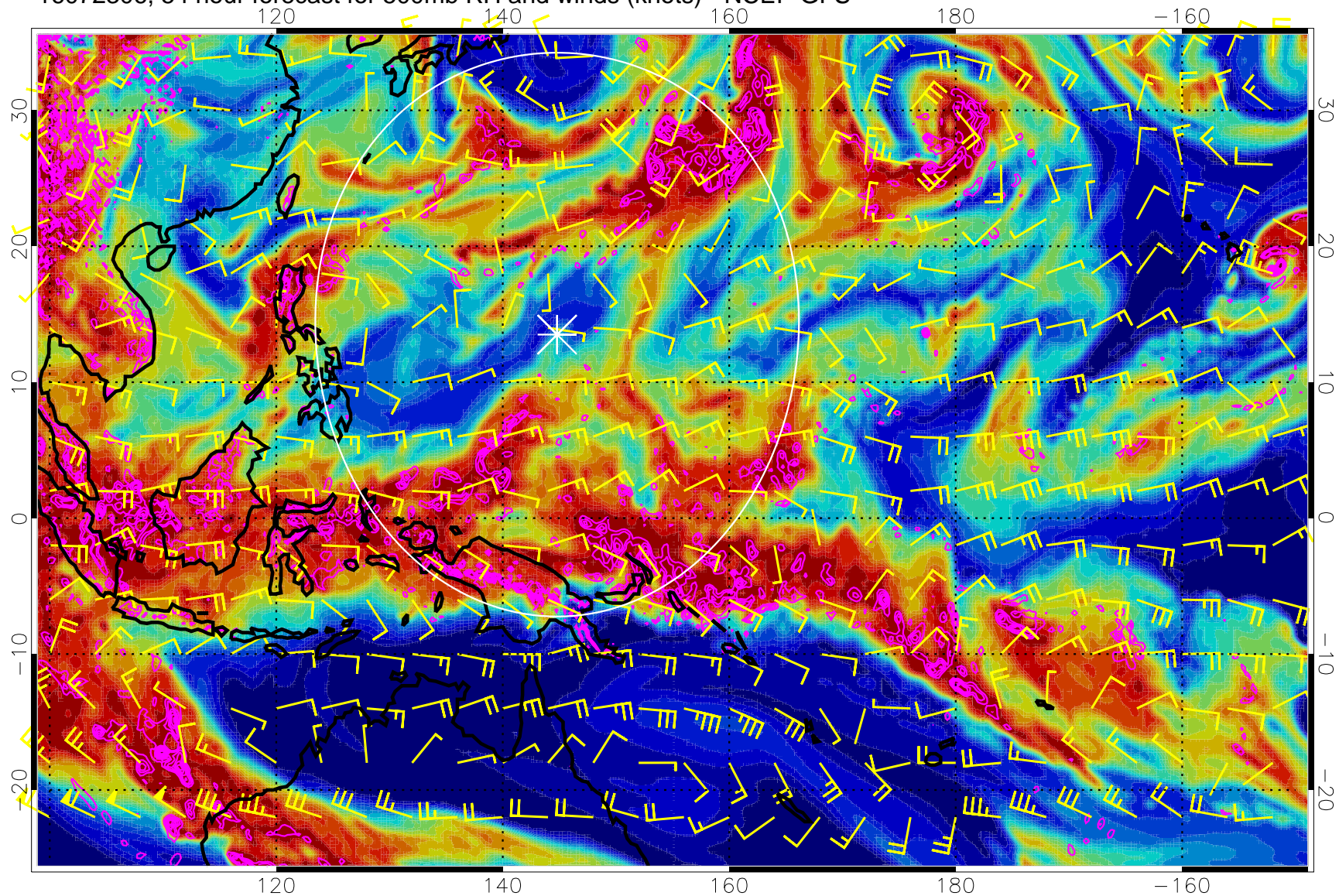
16072306, 54 hour forecast for 500mb RH and winds (knots) - NCEP GFS
