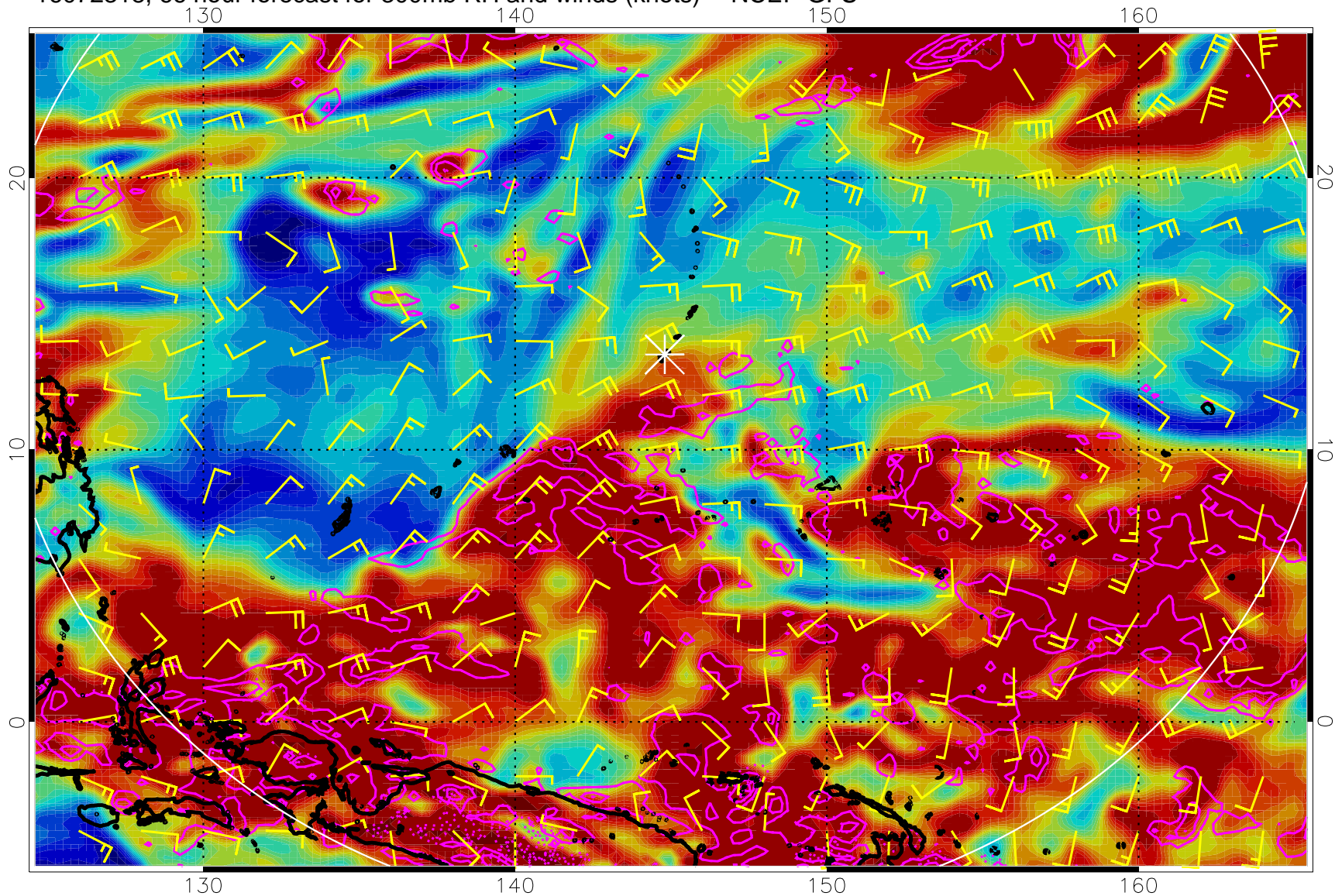
16072318, 66 hour forecast for 300mb RH and winds (knots) -- NCEP GFS
