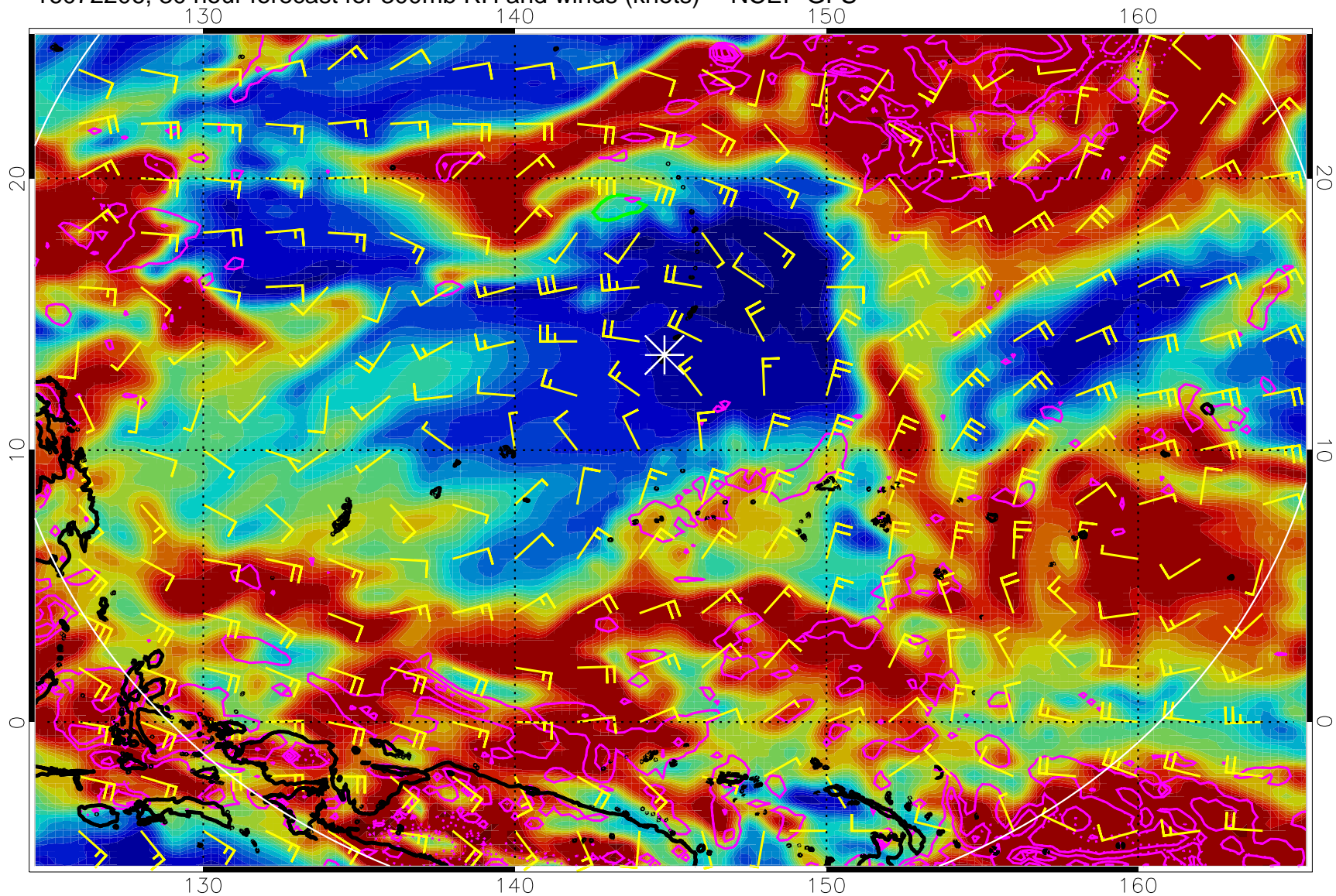
16072206, 30 hour forecast for 300mb RH and winds (knots) -- NCEP GFS
