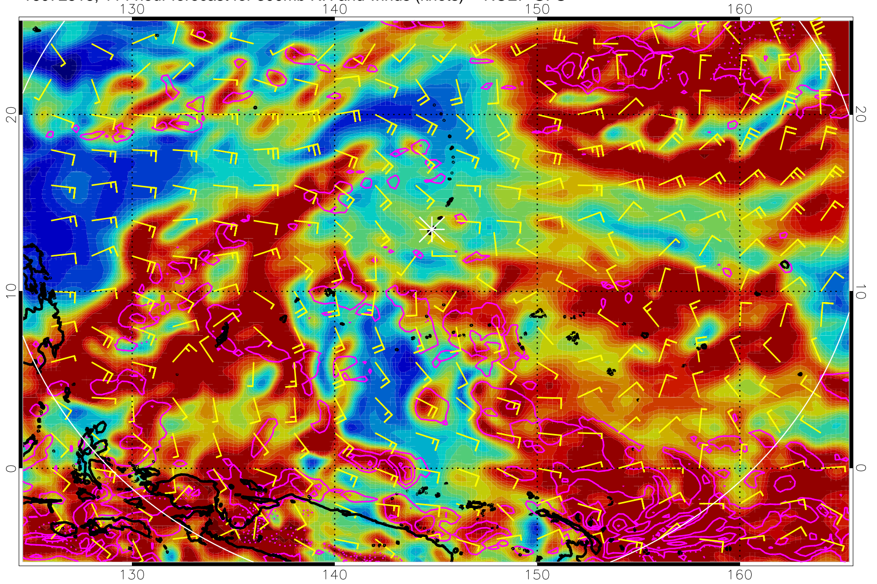
16072518, 114 hour forecast for 300mb RH and winds (knots) -- NCEP GFS
