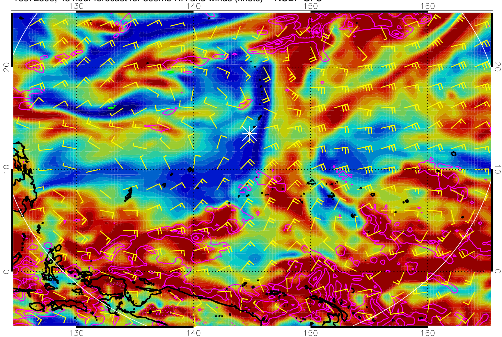
16072300, 48 hour forecast for 300mb RH and winds (knots) -- NCEP GFS
