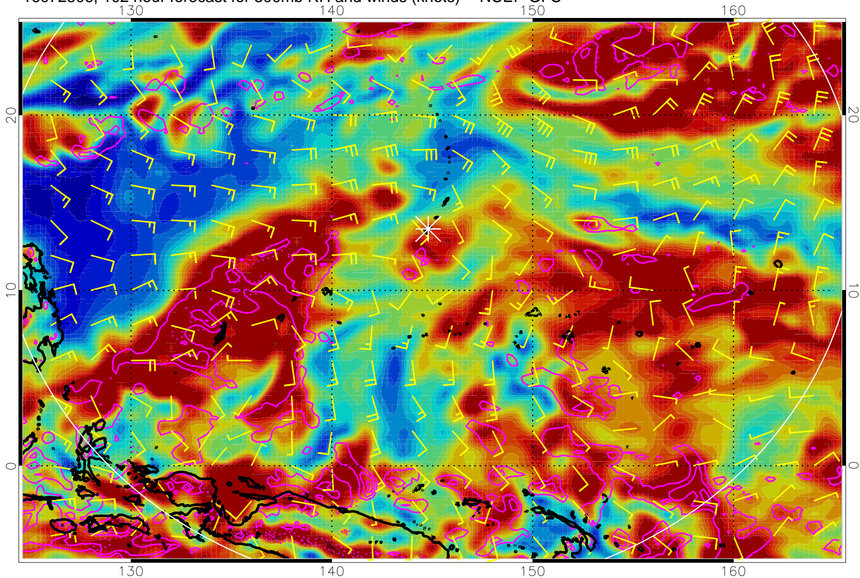
16072506, 102 hour forecast for 300mb RH and winds (knots) -- NCEP GFS
