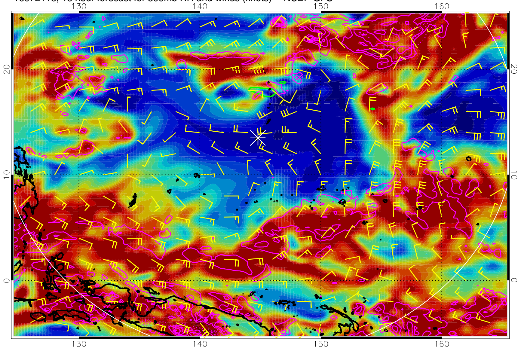
16072118, 18 hour forecast for 300mb RH and winds (knots) -- NCEP GFS
