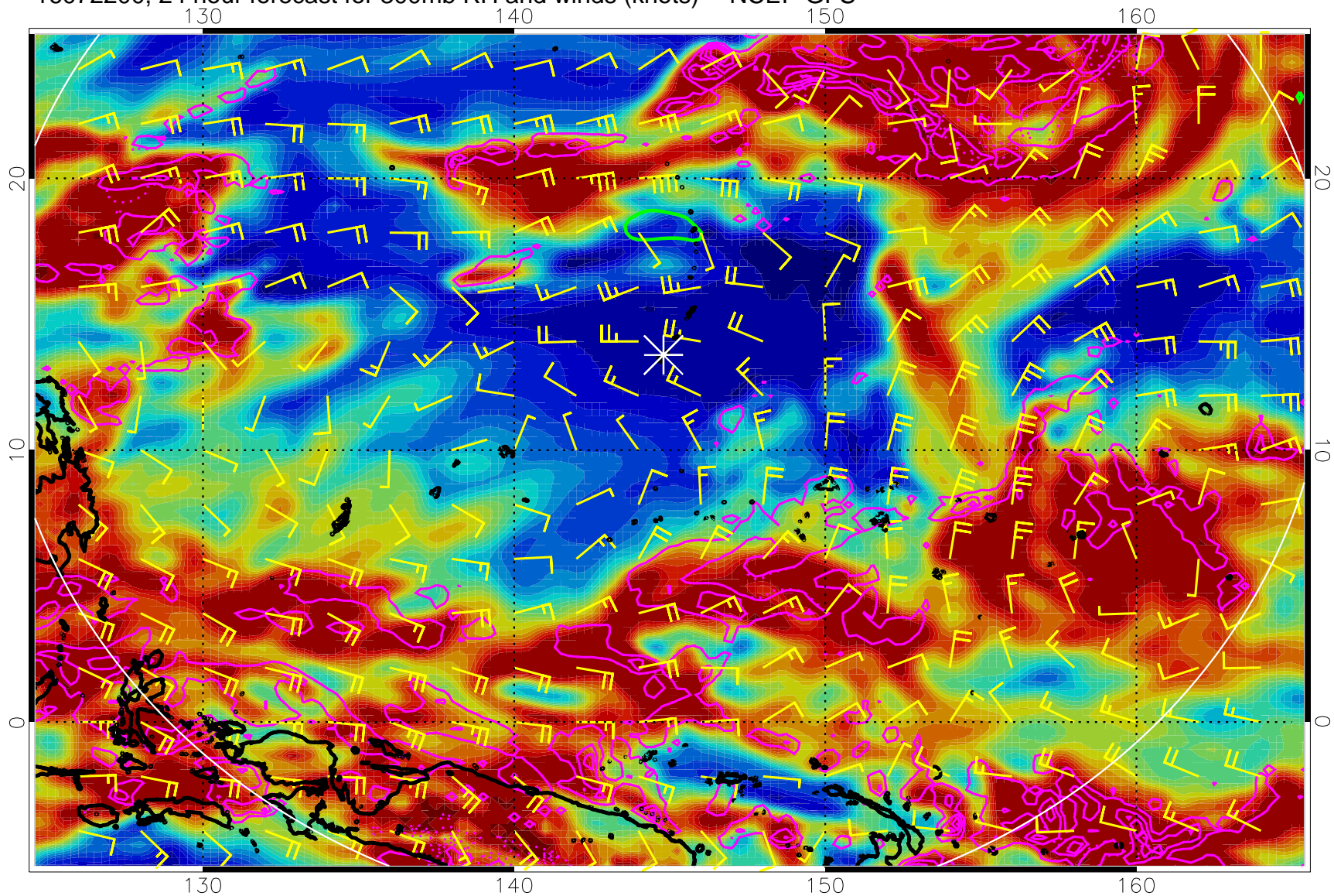
16072200, 24 hour forecast for 300mb RH and winds (knots) -- NCEP GFS
