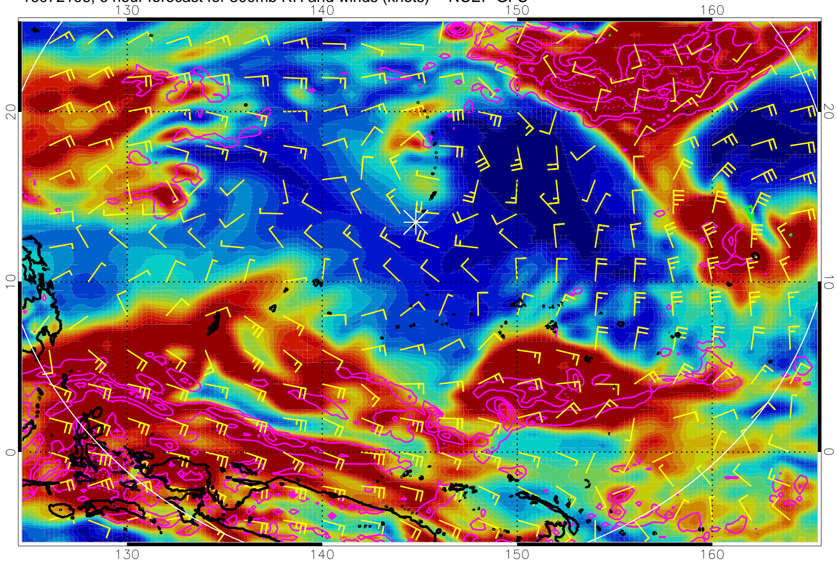
16072106, 6 hour forecast for 300mb RH and winds (knots) -- NCEP GFS
