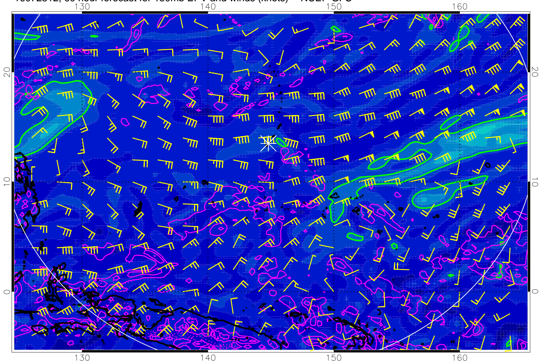
16072312, 60 hour forecast for 150mb EPV and winds (knots) -- NCEP GFS
