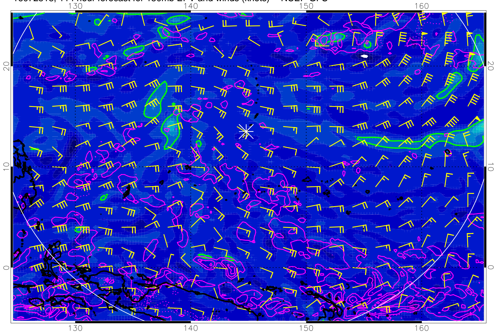
16072518, 114 hour forecast for 150mb EPV and winds (knots) -- NCEP GFS
