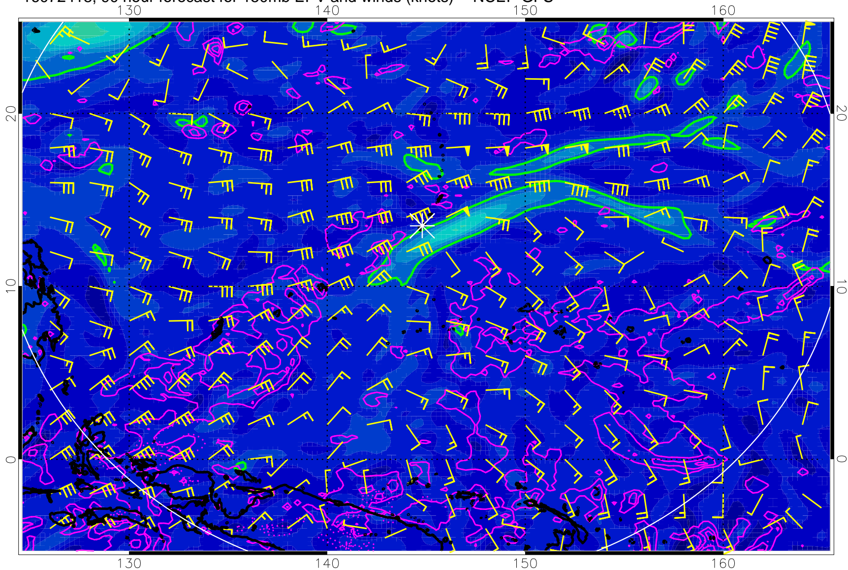
16072418, 90 hour forecast for 150mb EPV and winds (knots) -- NCEP GFS
