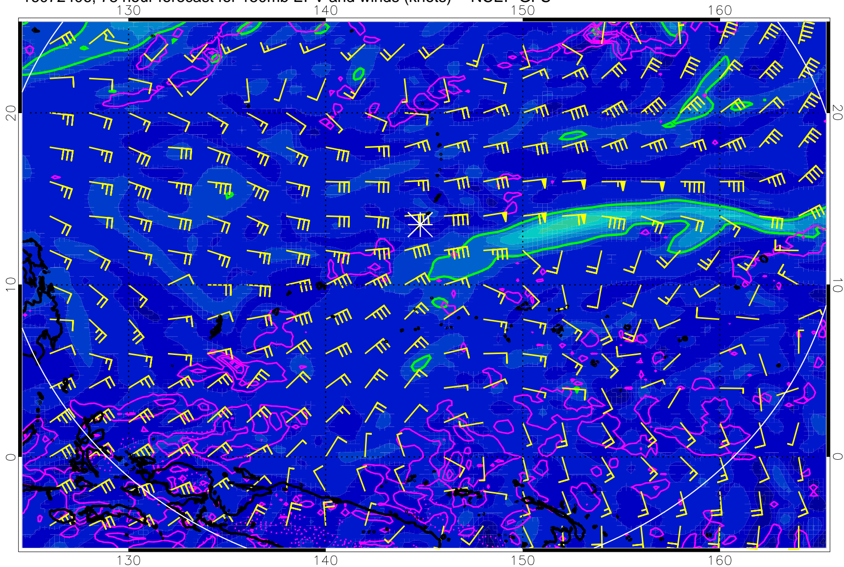
16072406, 78 hour forecast for 150mb EPV and winds (knots) -- NCEP GFS
