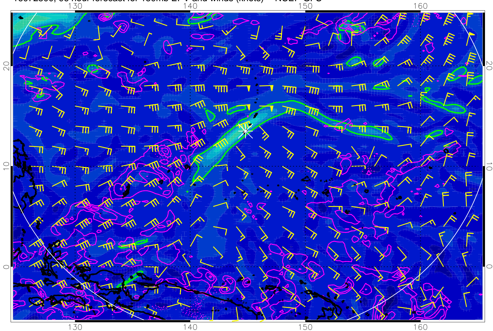
16072500, 96 hour forecast for 150mb EPV and winds (knots) -- NCEP GFS
