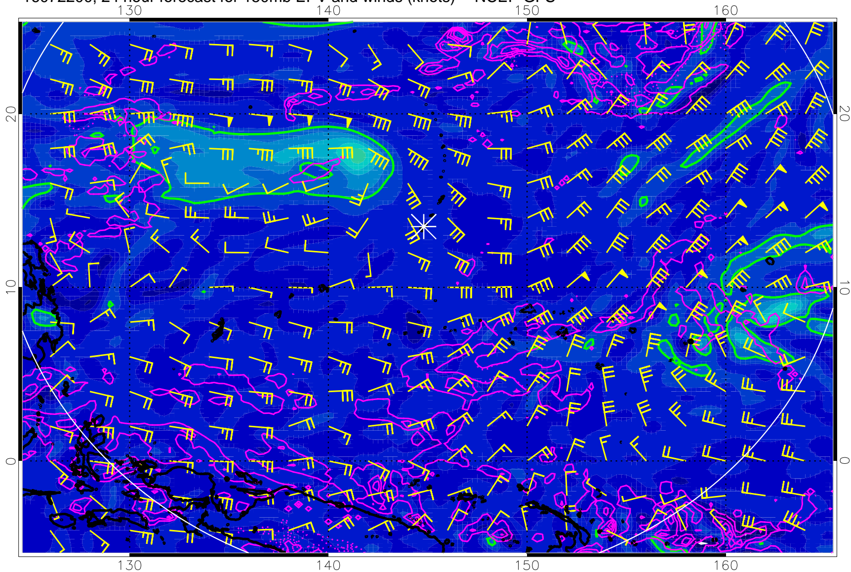
16072200, 24 hour forecast for 150mb EPV and winds (knots) -- NCEP GFS
