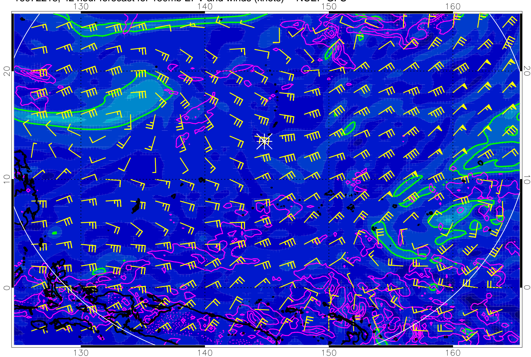
16072218, 42 hour forecast for 150mb EPV and winds (knots) -- NCEP GFS
