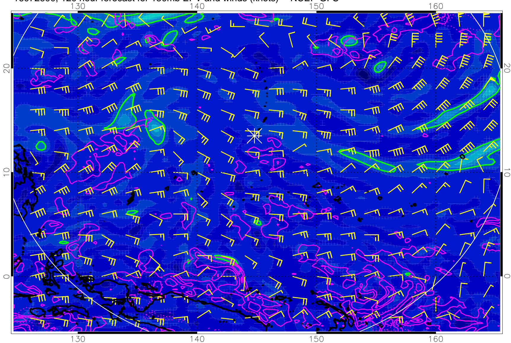
16072600, 120 hour forecast for 150mb EPV and winds (knots) -- NCEP GFS
