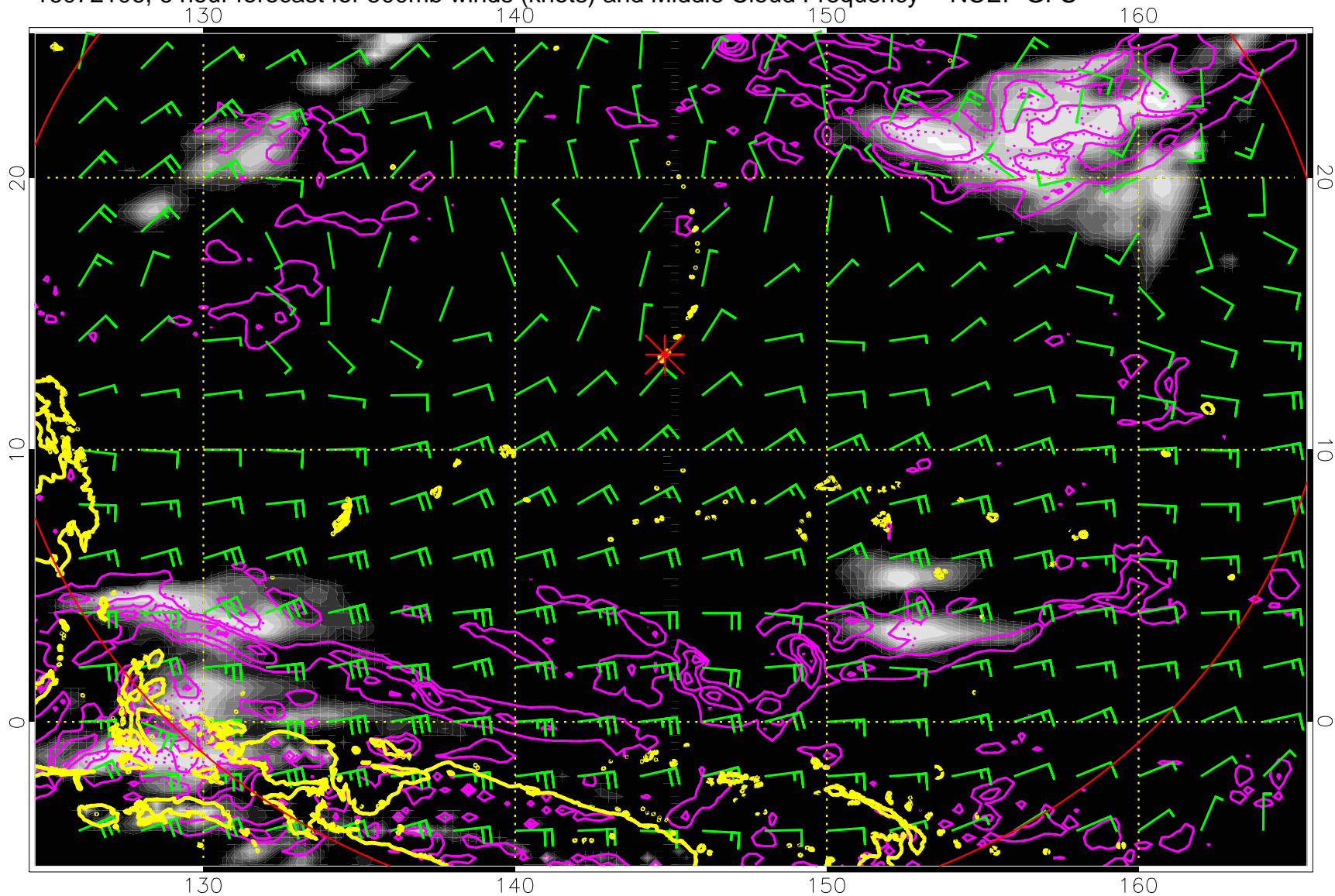
16072106, 6 hour forecast for 500mb winds (knots) and Middle Cloud Frequency -- NCEP GFS
