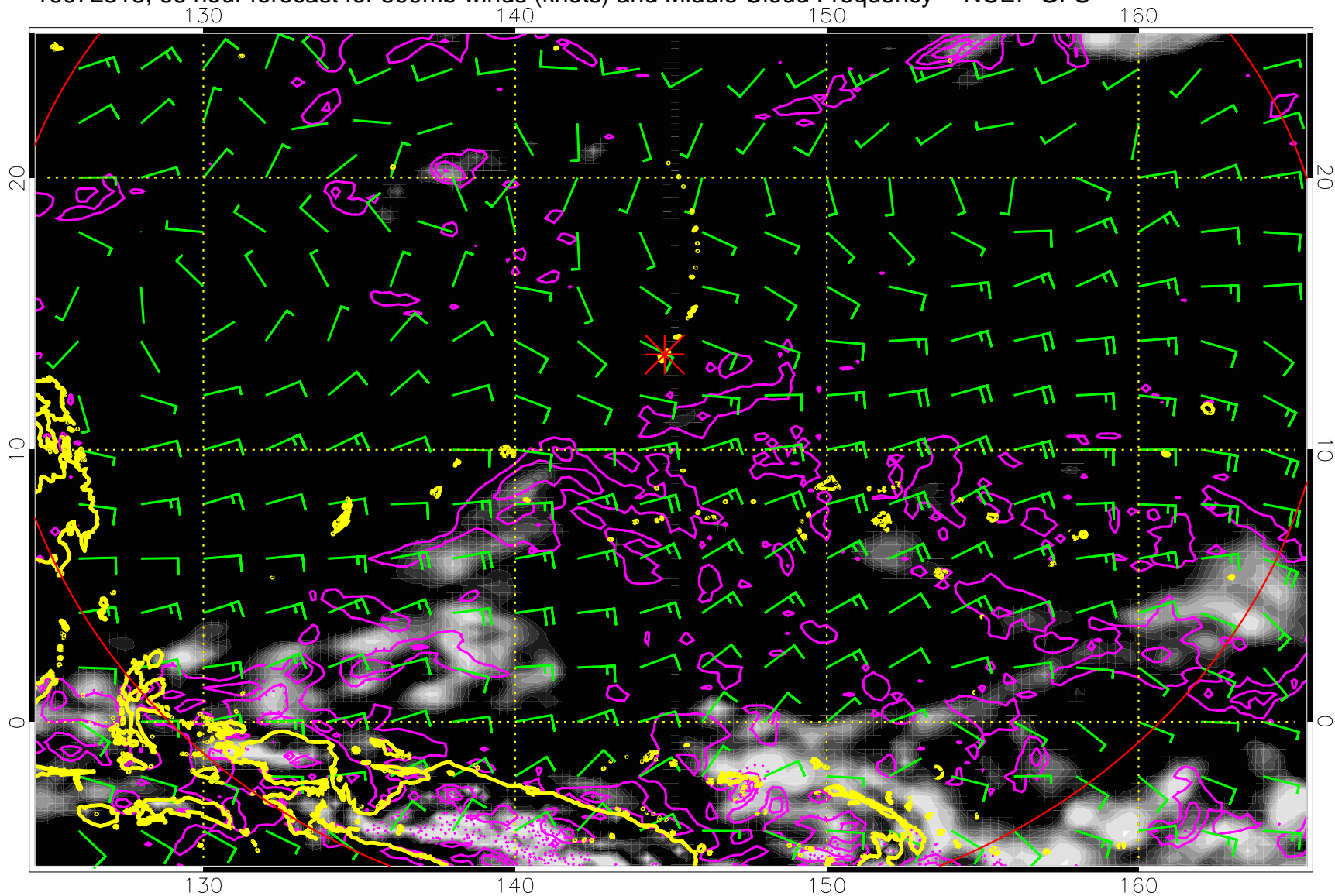
16072318, 66 hour forecast for 500mb winds (knots) and Middle Cloud Frequency -- NCEP GFS
