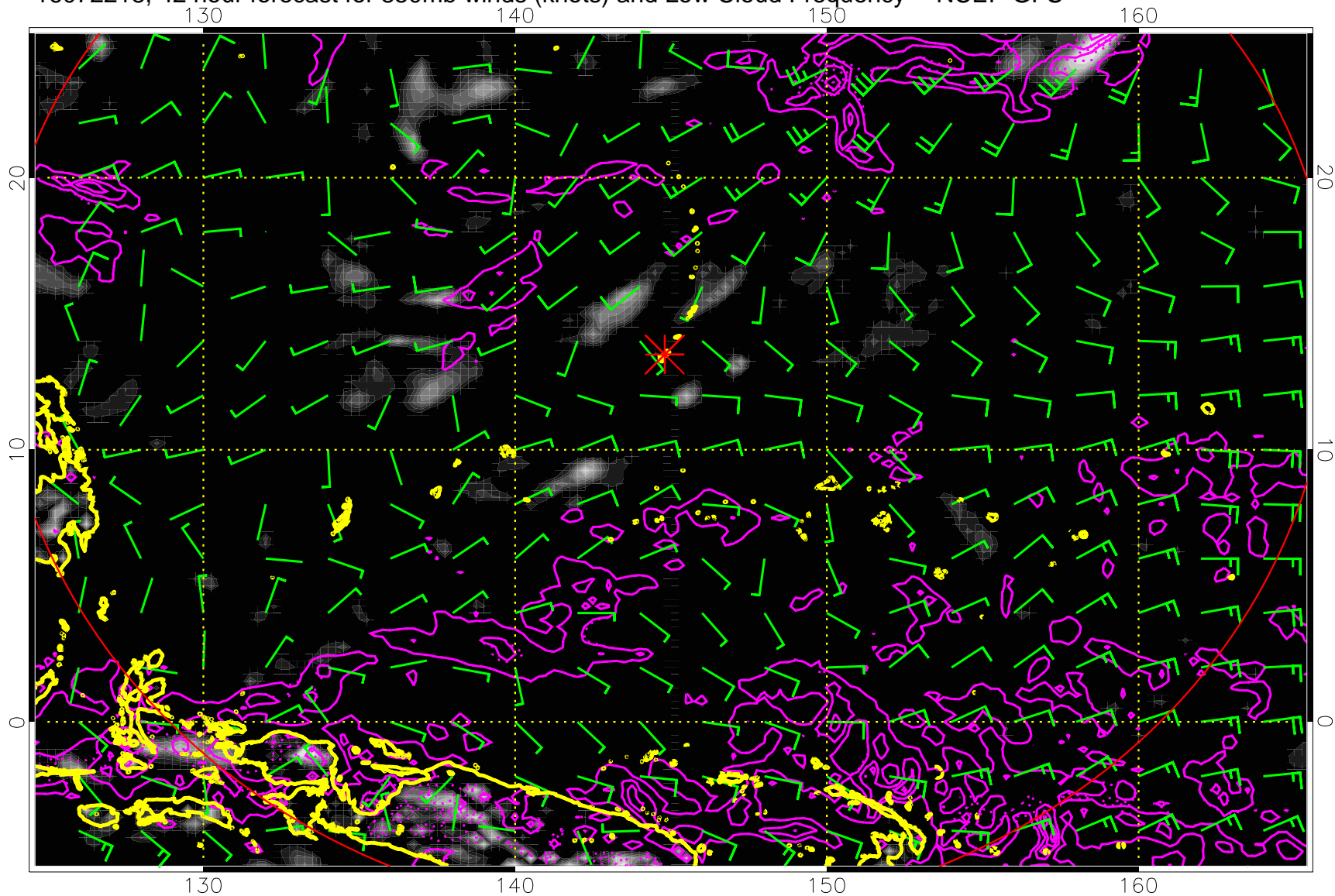
16072218, 42 hour forecast for 850mb winds (knots) and Low Cloud Frequency -- NCEP GFS
