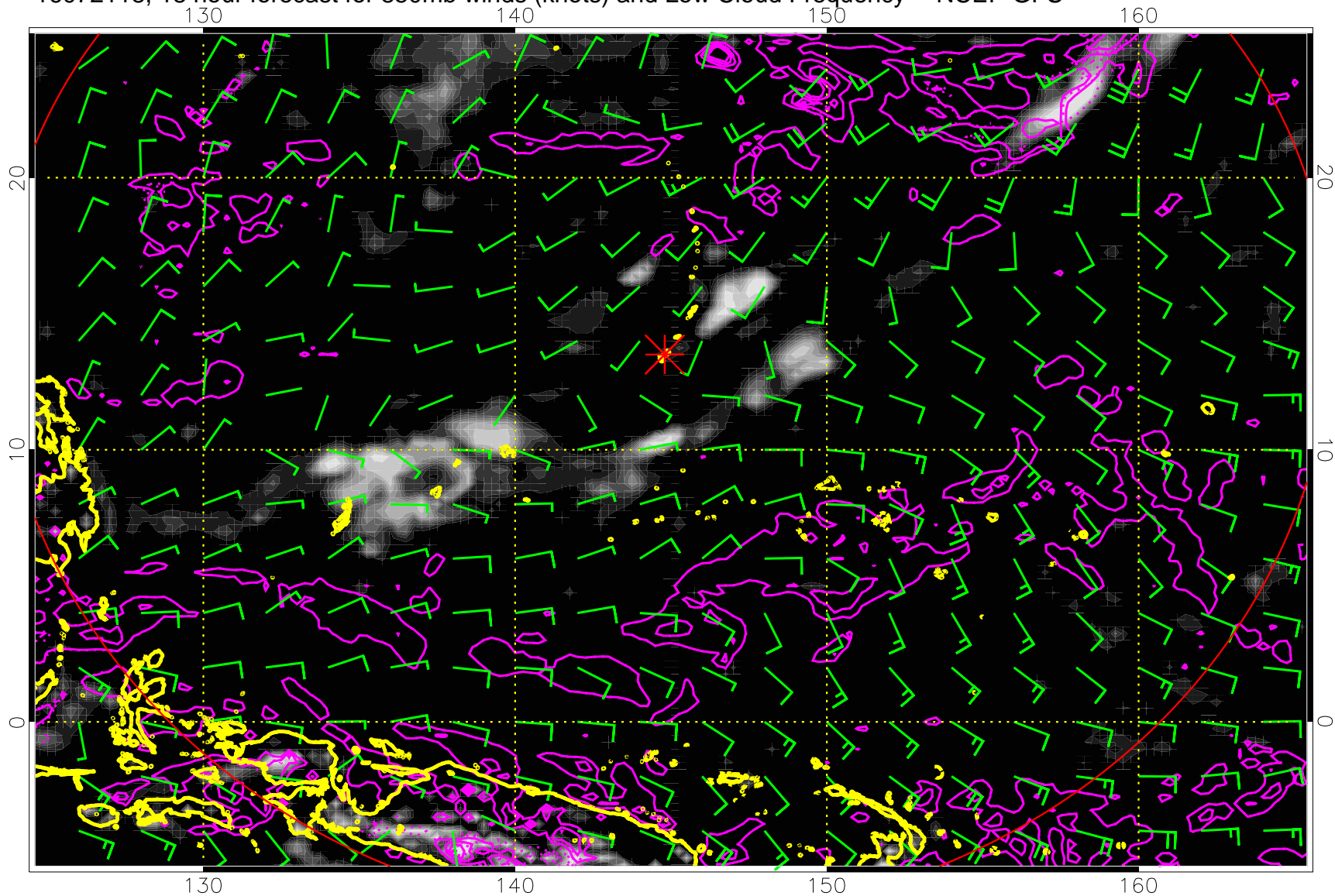
16072118, 18 hour forecast for 850mb winds (knots) and Low Cloud Frequency -- NCEP GFS
