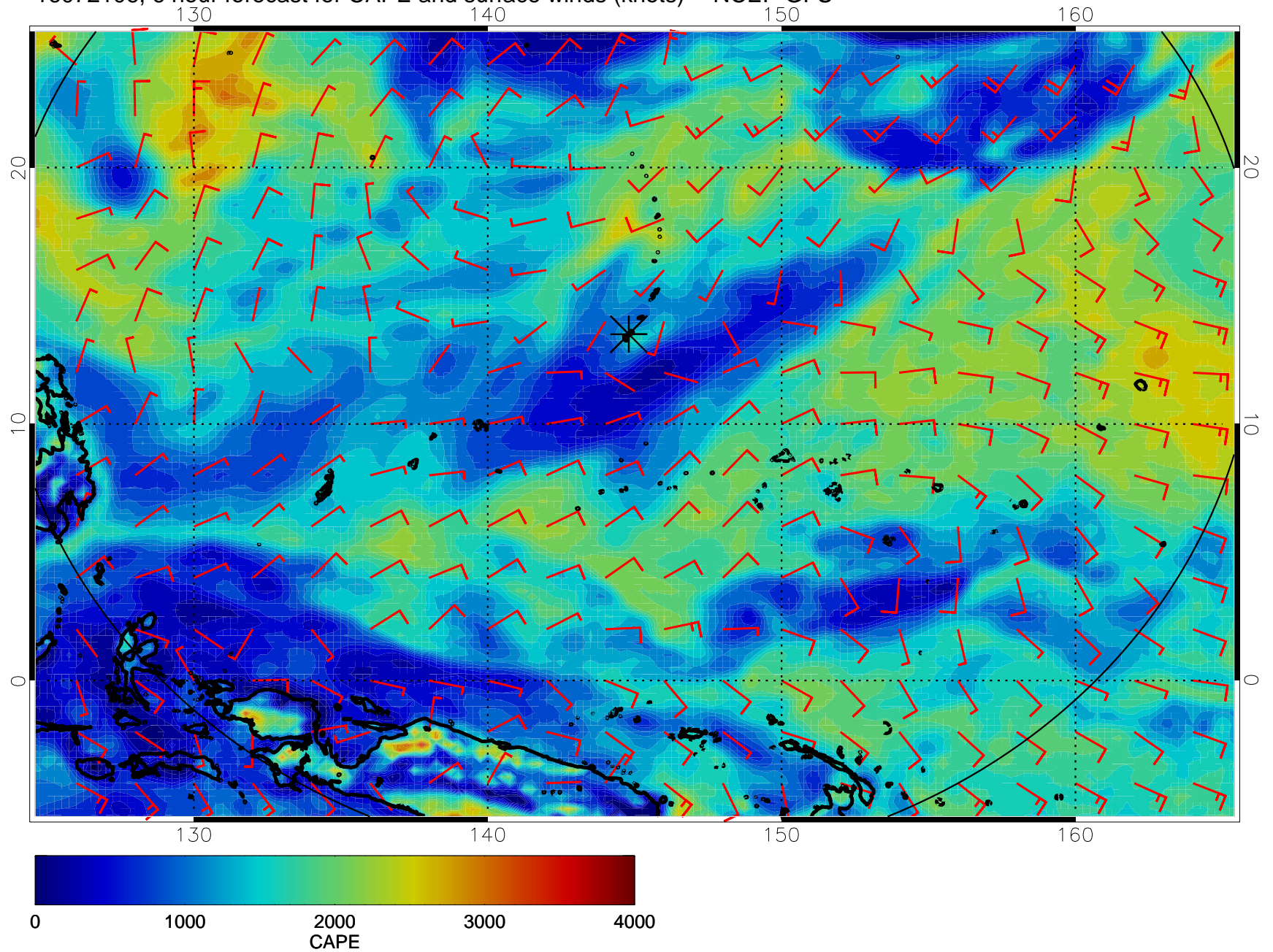
16072106, 6 hour forecast for CAPE and surface winds (knots) -- NCEP GFS
