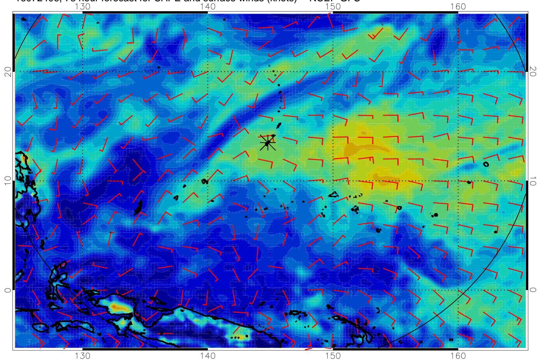
16072406, 78 hour forecast for CAPE and surface winds (knots) -- NCEP GFS
