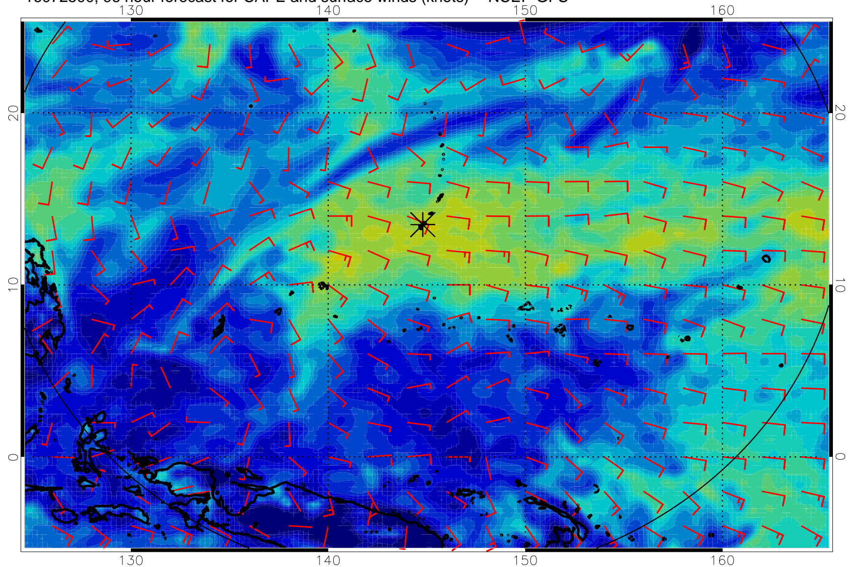
16072500, 96 hour forecast for CAPE and surface winds (knots) -- NCEP GFS
