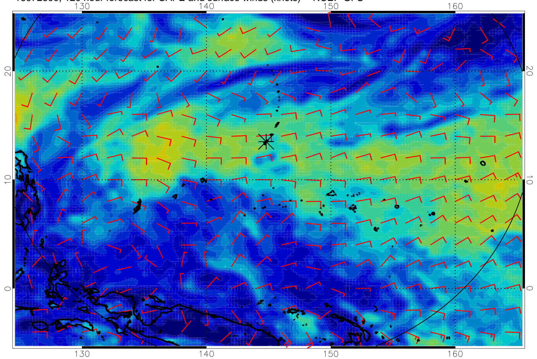
16072600, 120 hour forecast for CAPE and surface winds (knots) -- NCEP GFS
