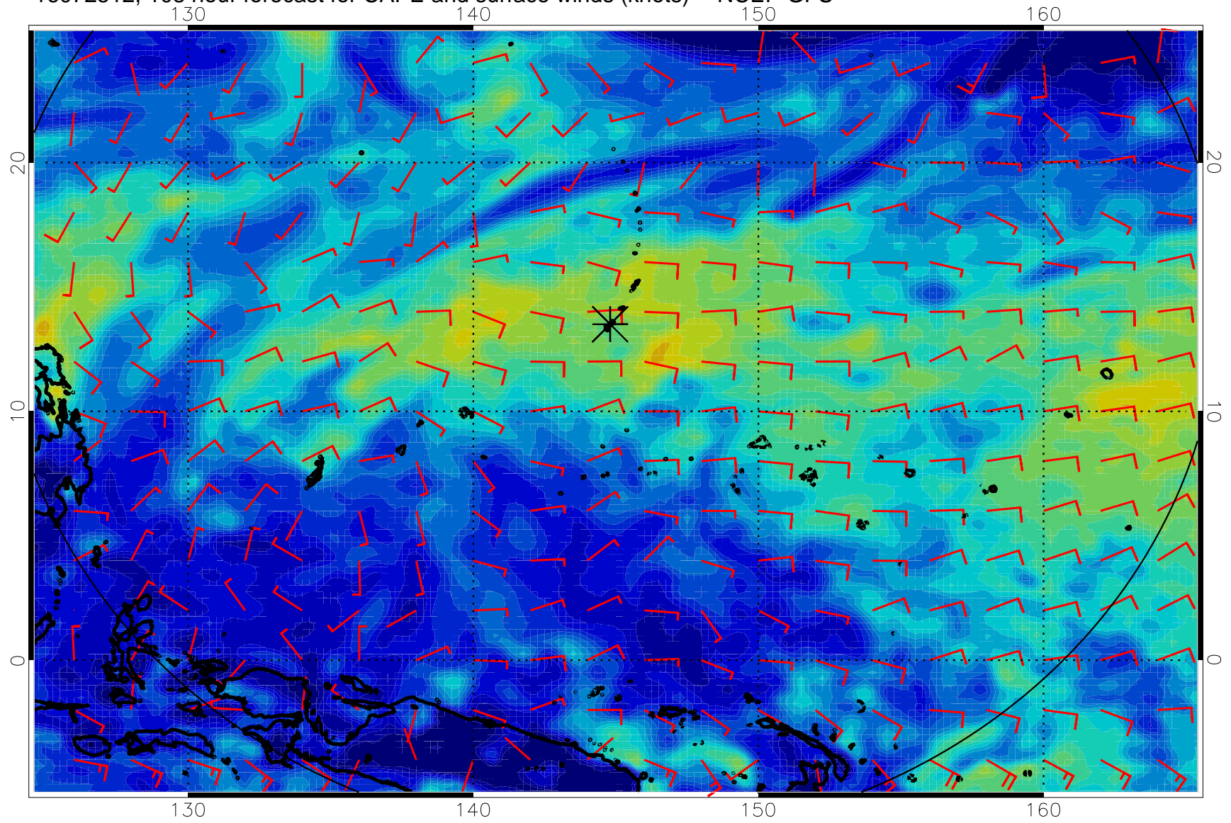
16072512, 108 hour forecast for CAPE and surface winds (knots) -- NCEP GFS
