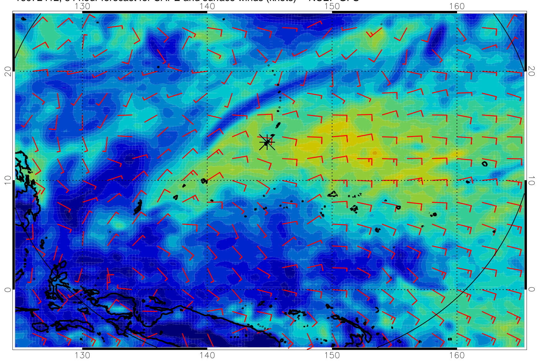
16072412, 84 hour forecast for CAPE and surface winds (knots) -- NCEP GFS
