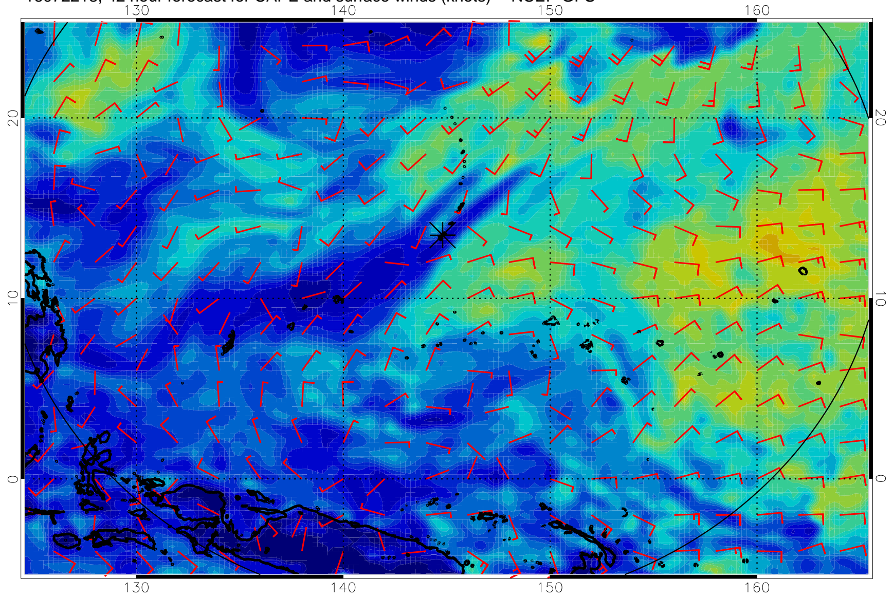
16072218, 42 hour forecast for CAPE and surface winds (knots) -- NCEP GFS
