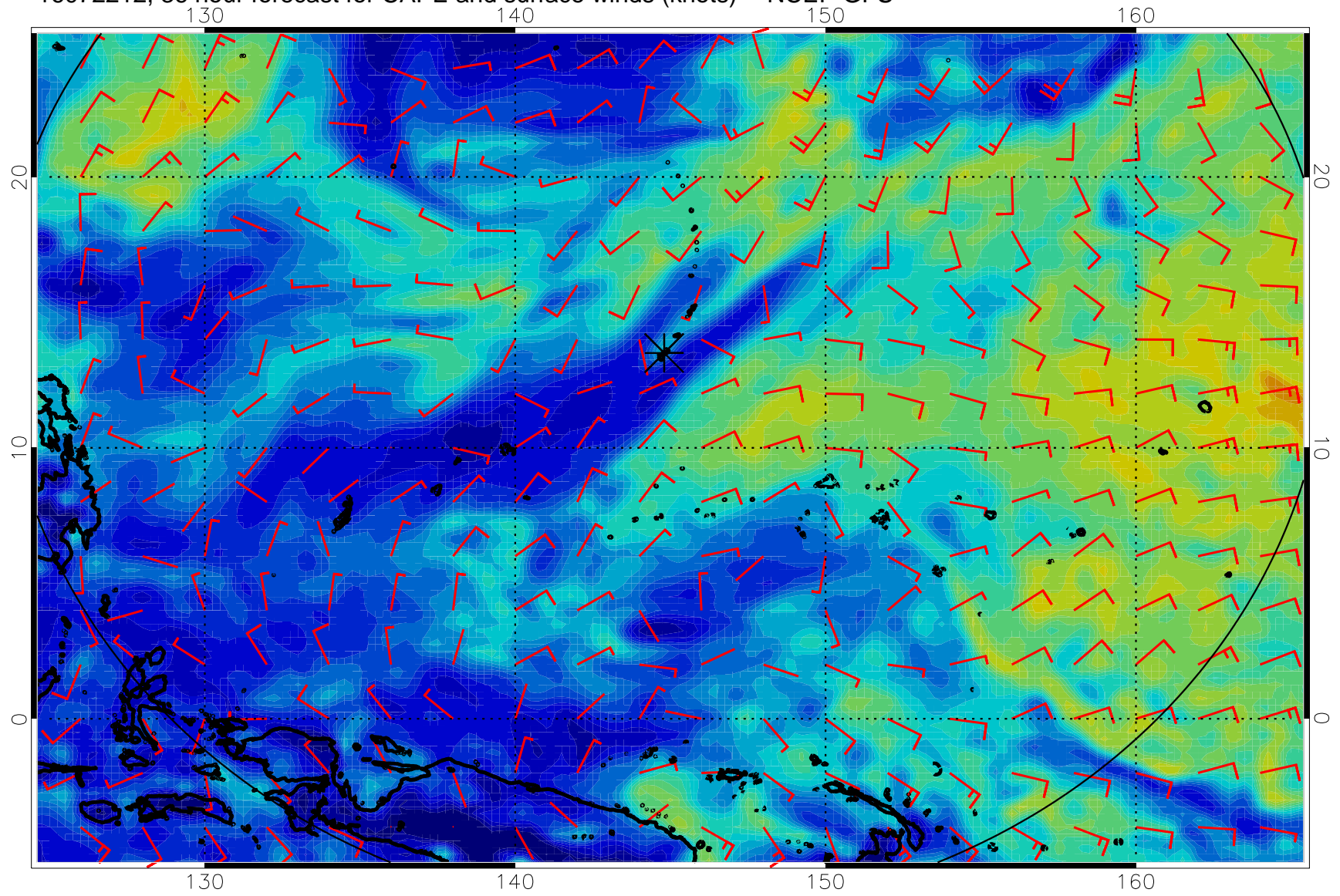
16072212, 36 hour forecast for CAPE and surface winds (knots) -- NCEP GFS
