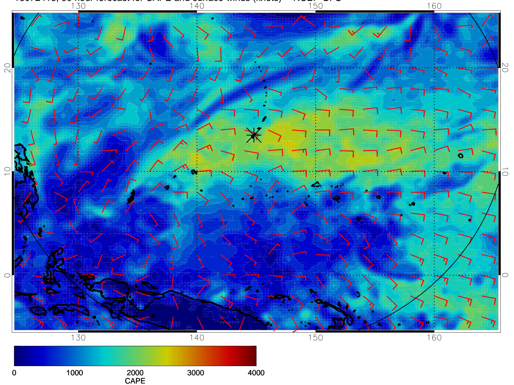
16072418, 90 hour forecast for CAPE and surface winds (knots) -- NCEP GFS
