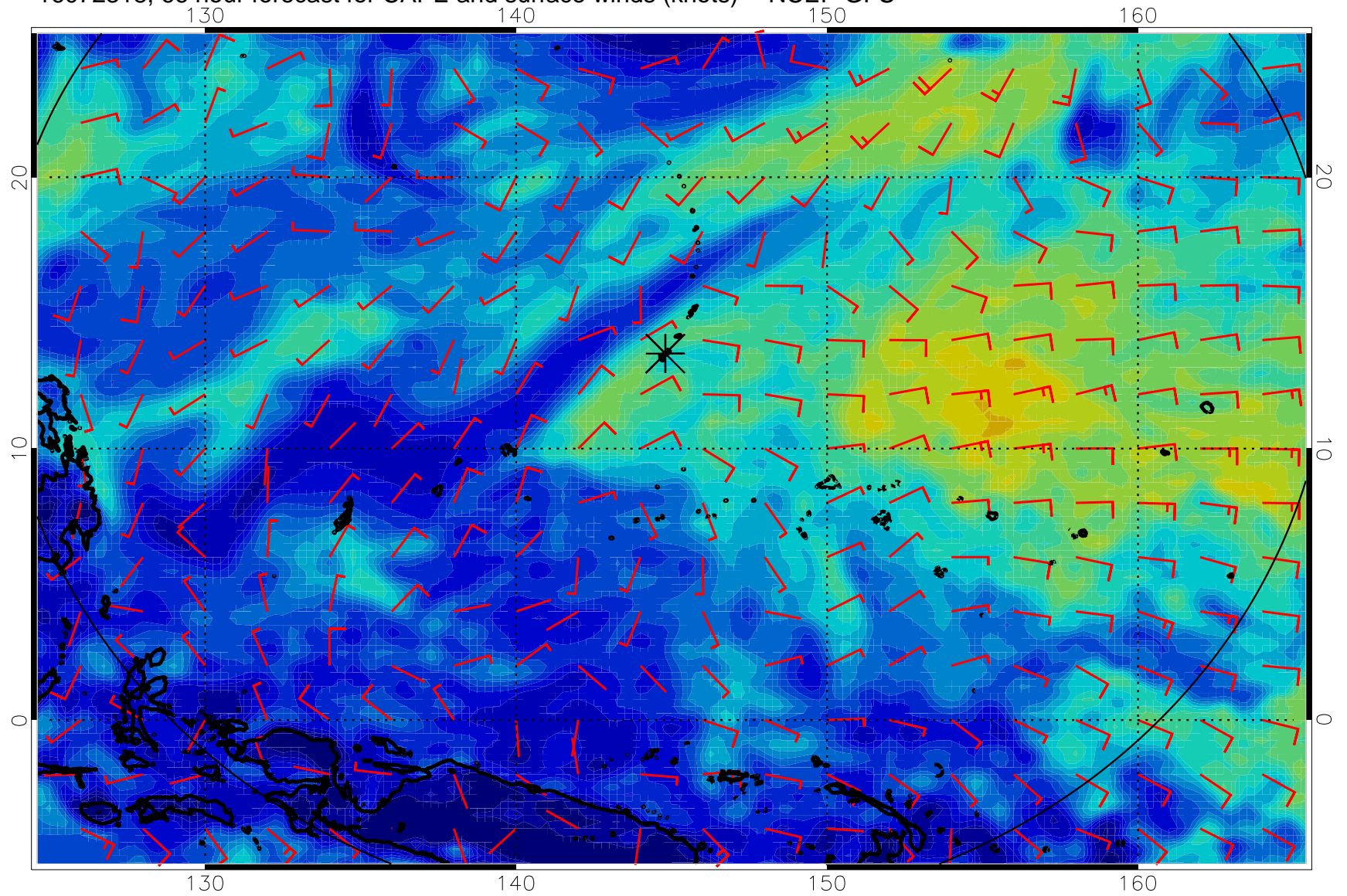
16072318, 66 hour forecast for CAPE and surface winds (knots) -- NCEP GFS
