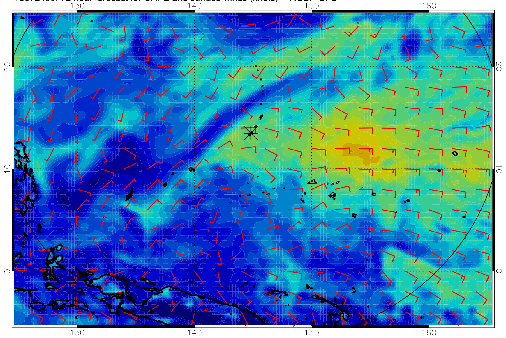
16072400, 72 hour forecast for CAPE and surface winds (knots) -- NCEP GFS
