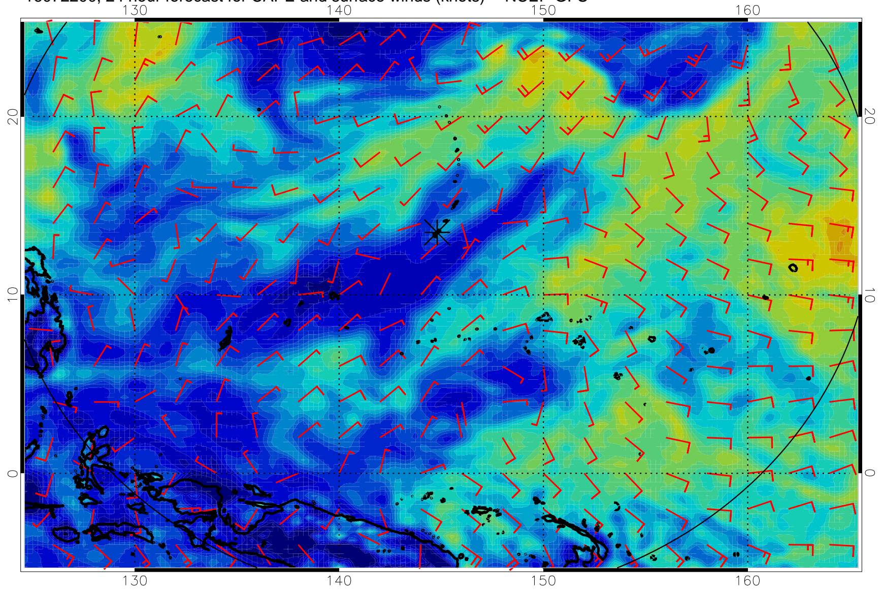
16072200, 24 hour forecast for CAPE and surface winds (knots) -- NCEP GFS
