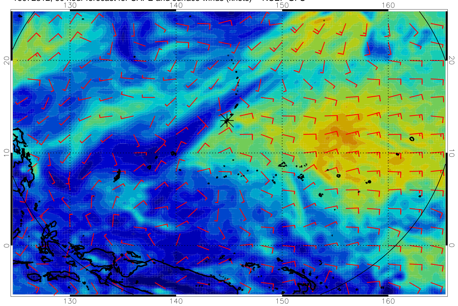
16072312, 60 hour forecast for CAPE and surface winds (knots) -- NCEP GFS
