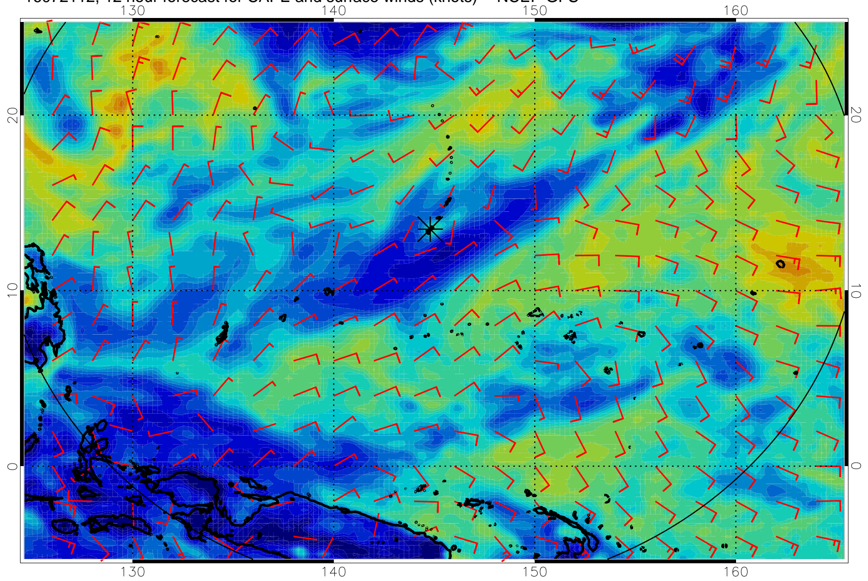
16072112, 12 hour forecast for CAPE and surface winds (knots) -- NCEP GFS
