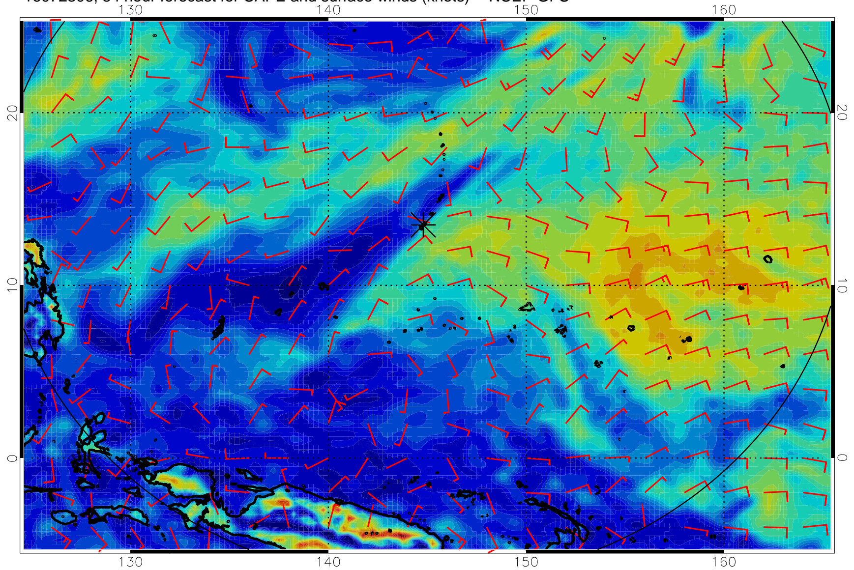
16072306, 54 hour forecast for CAPE and surface winds (knots) -- NCEP GFS
