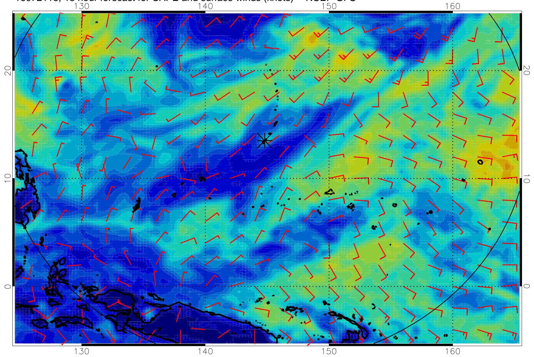
16072118, 18 hour forecast for CAPE and surface winds (knots) -- NCEP GFS
