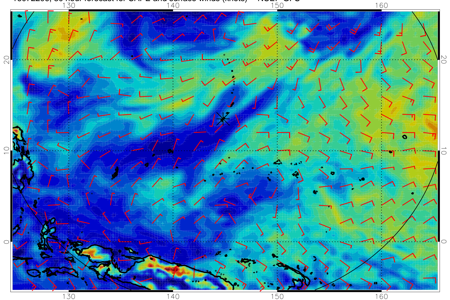
16072206, 30 hour forecast for CAPE and surface winds (knots) -- NCEP GFS
