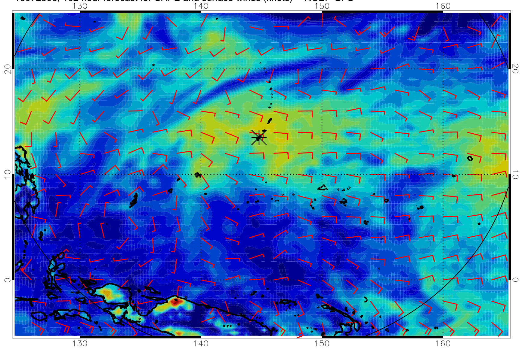
16072506, 102 hour forecast for CAPE and surface winds (knots) -- NCEP GFS
