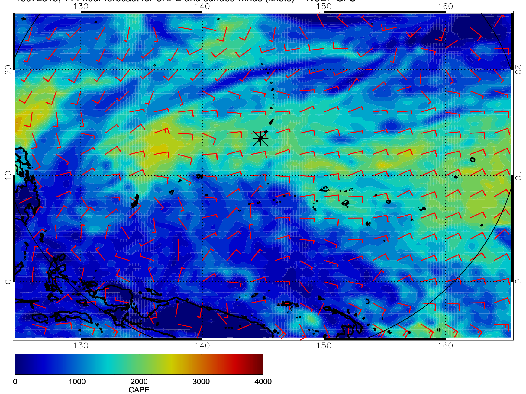
16072518, 114 hour forecast for CAPE and surface winds (knots) -- NCEP GFS
