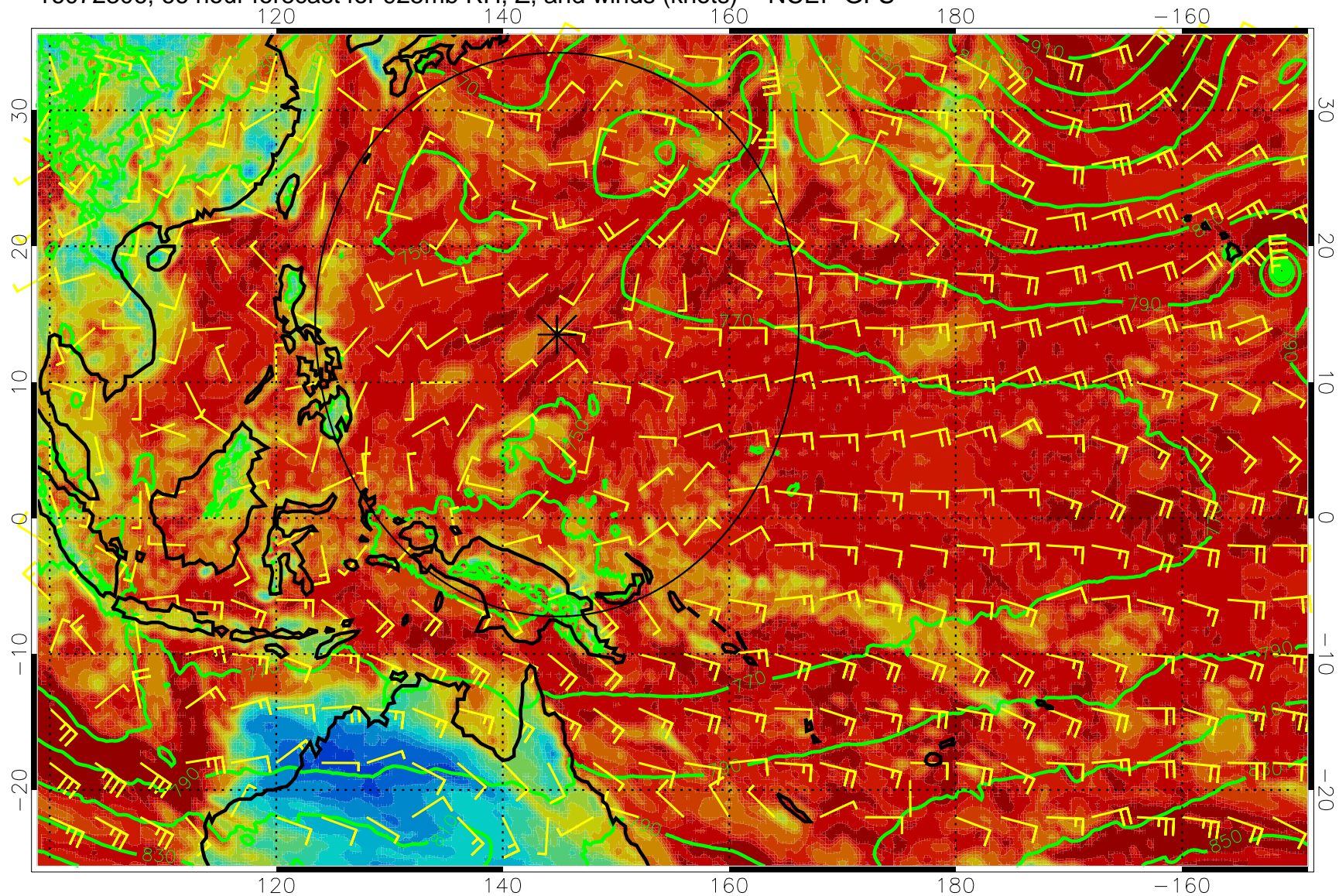
16072306, 66 hour forecast for 925mb RH, Z, and winds (knots) -- NCEP GFS
