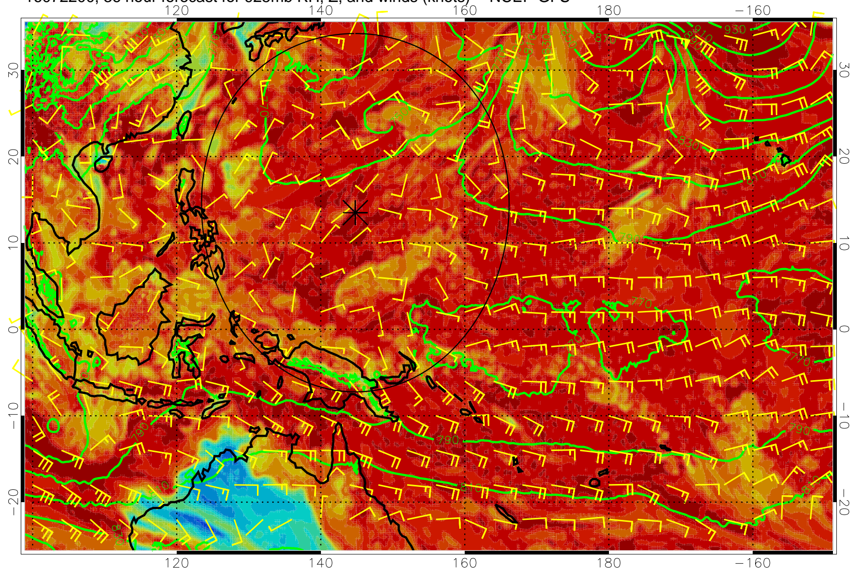
16072200, 36 hour forecast for 925mb RH, Z, and winds (knots) -- NCEP GFS
