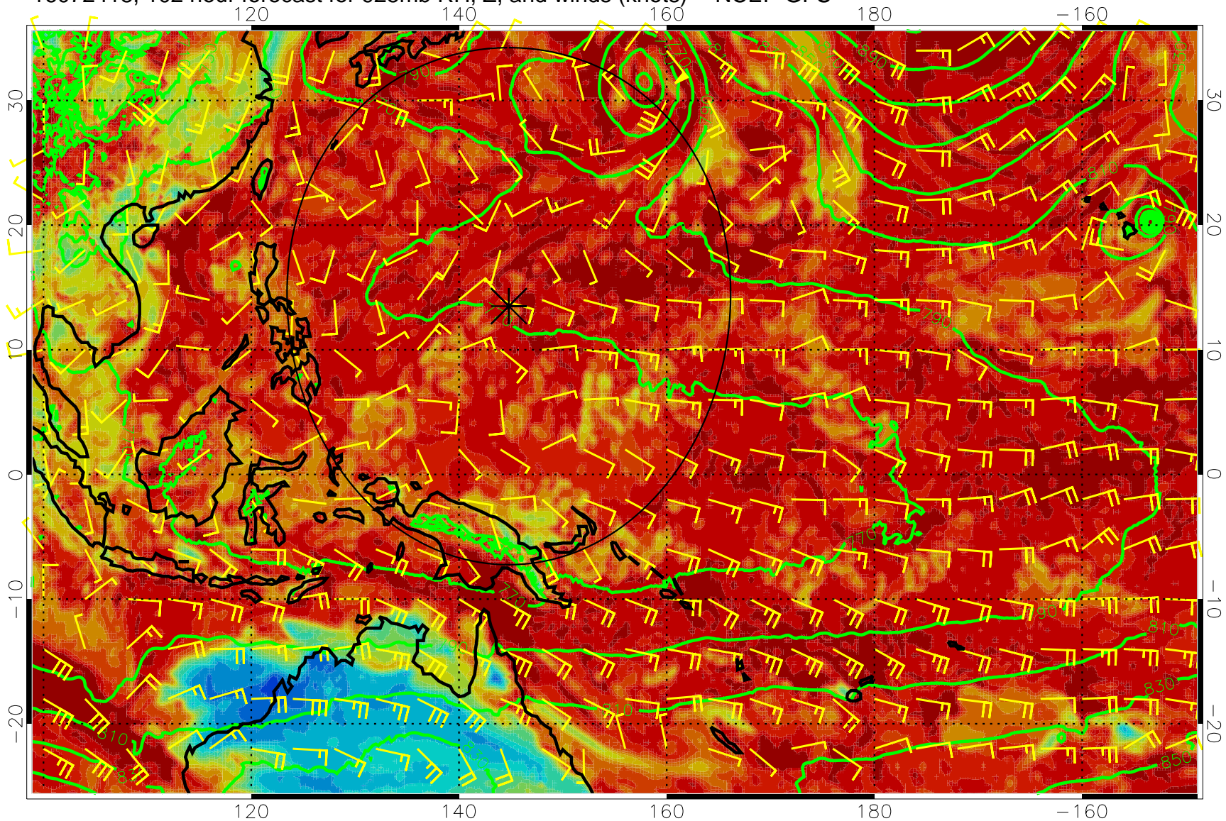
16072418, 102 hour forecast for 925mb RH, Z, and winds (knots) -- NCEP GFS
