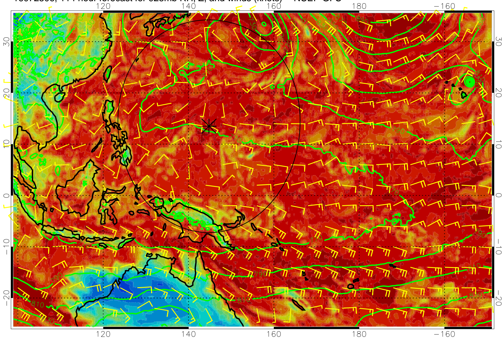
16072506, 114 hour forecast for 925mb RH, Z, and winds (knots) -- NCEP GFS
