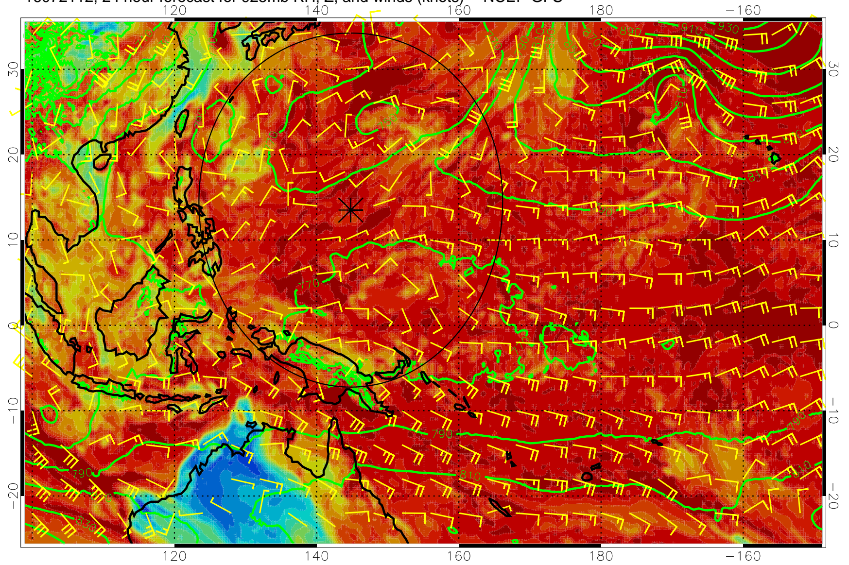
16072112, 24 hour forecast for 925mb RH, Z, and winds (knots) -- NCEP GFS
