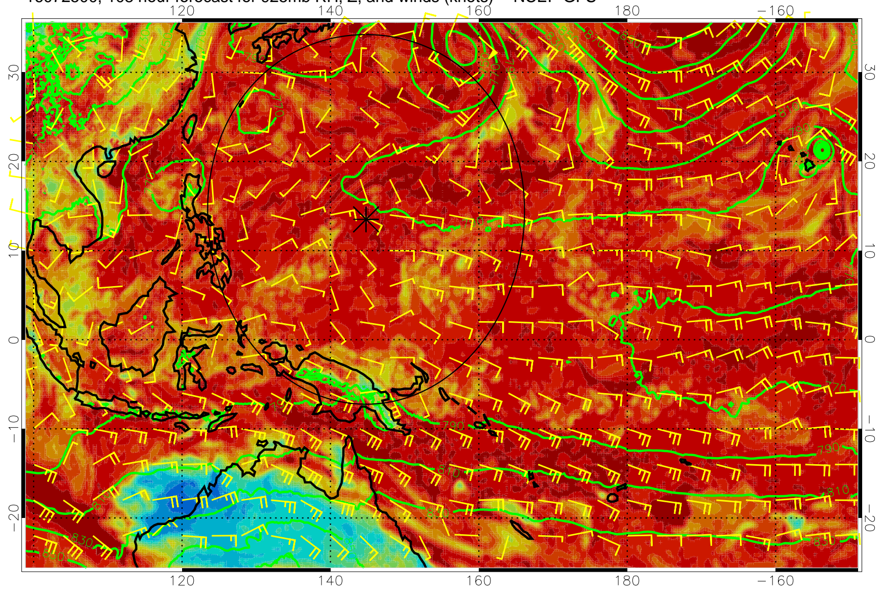
16072500, 108 hour forecast for 925mb RH, Z, and winds (knots) -- NCEP GFS
