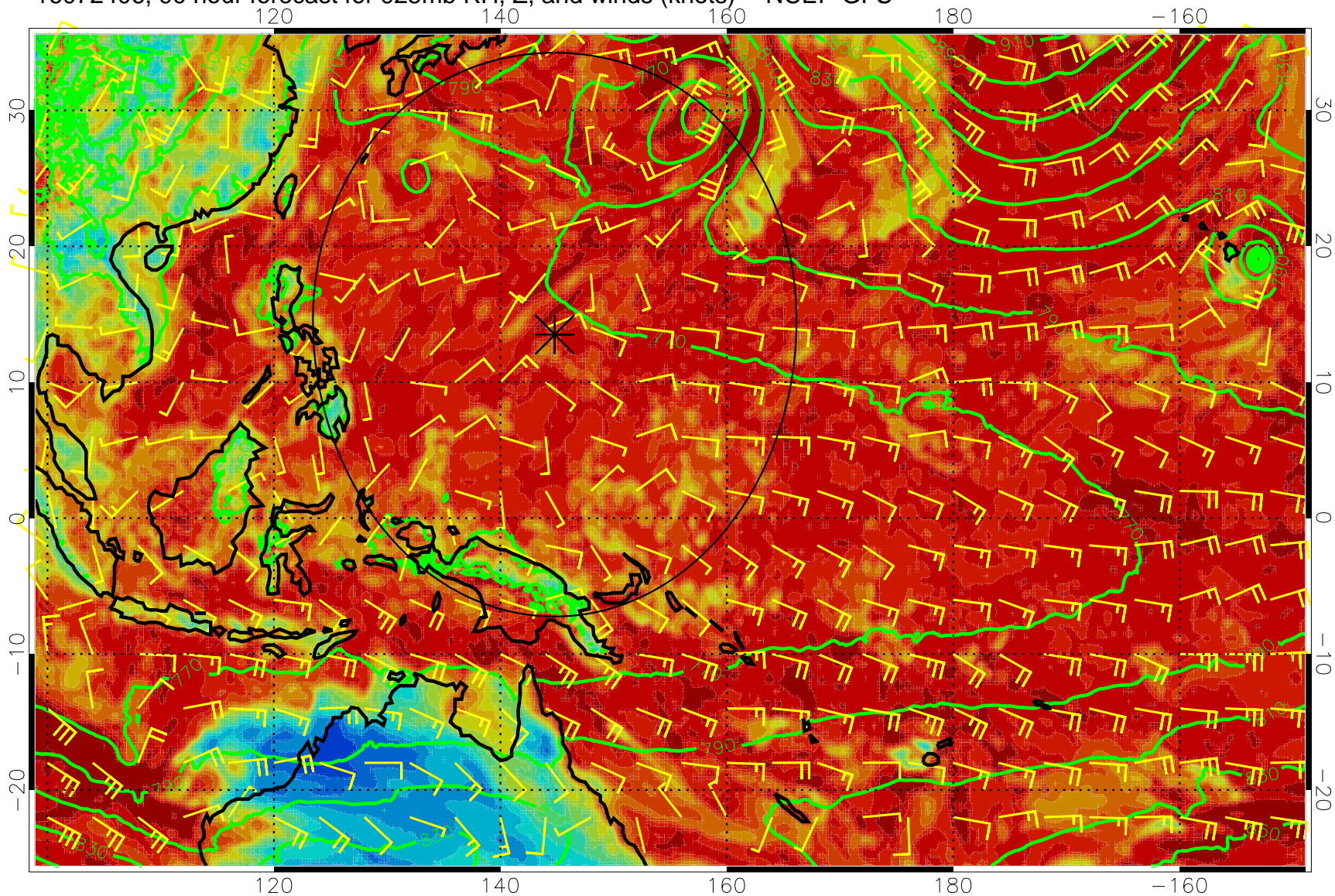
16072406, 90 hour forecast for 925mb RH, Z, and winds (knots) -- NCEP GFS
