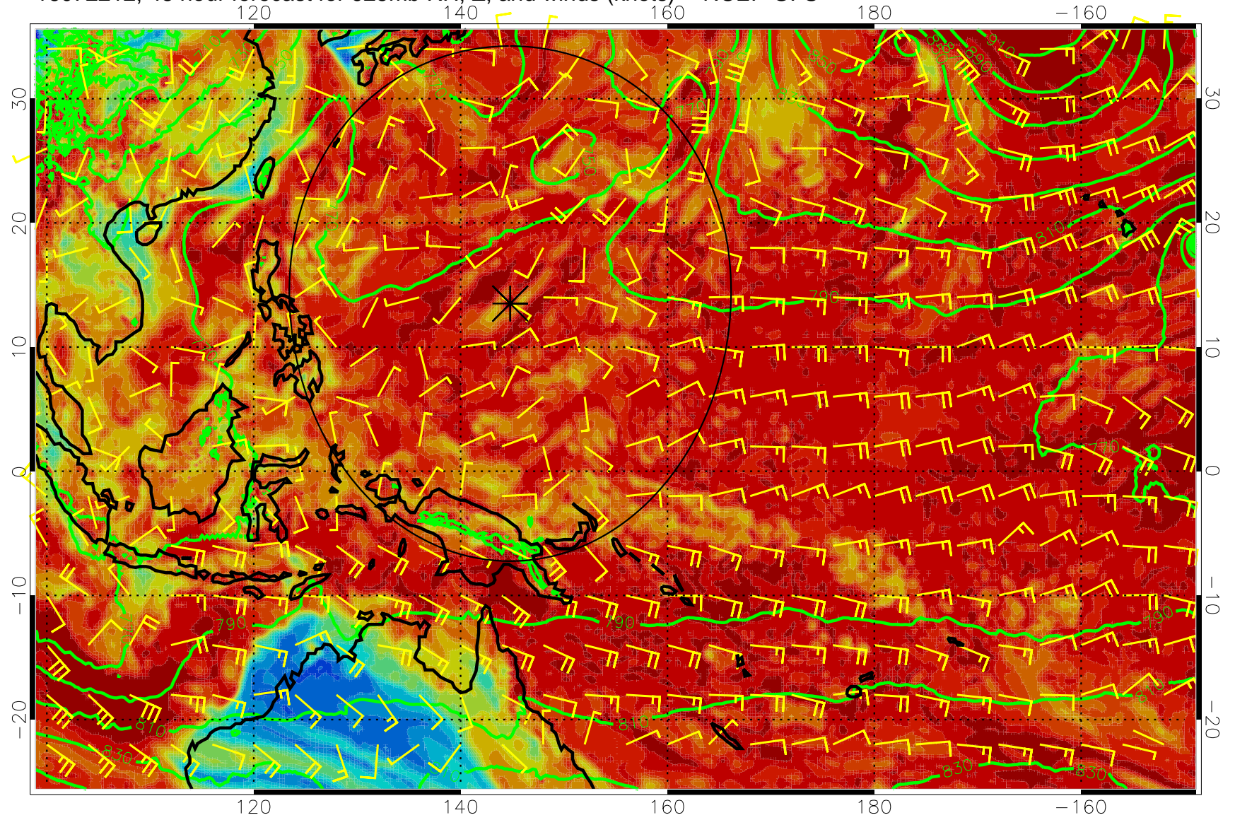
16072212, 48 hour forecast for 925mb RH, Z, and winds (knots) -- NCEP GFS
