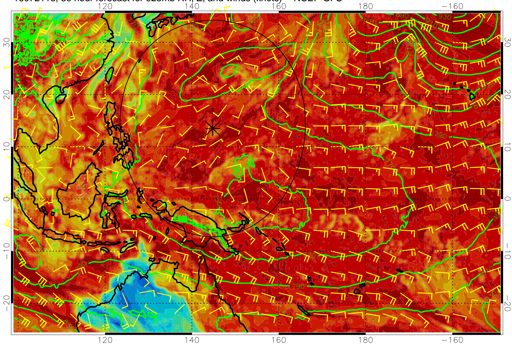
16072118, 30 hour forecast for 925mb RH, Z, and winds (knots) -- NCEP GFS
