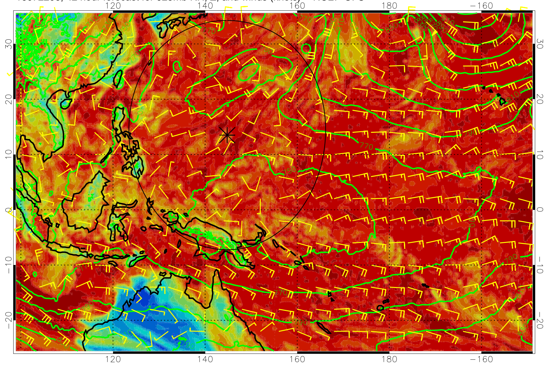
16072206, 42 hour forecast for 925mb RH, Z, and winds (knots) -- NCEP GFS
