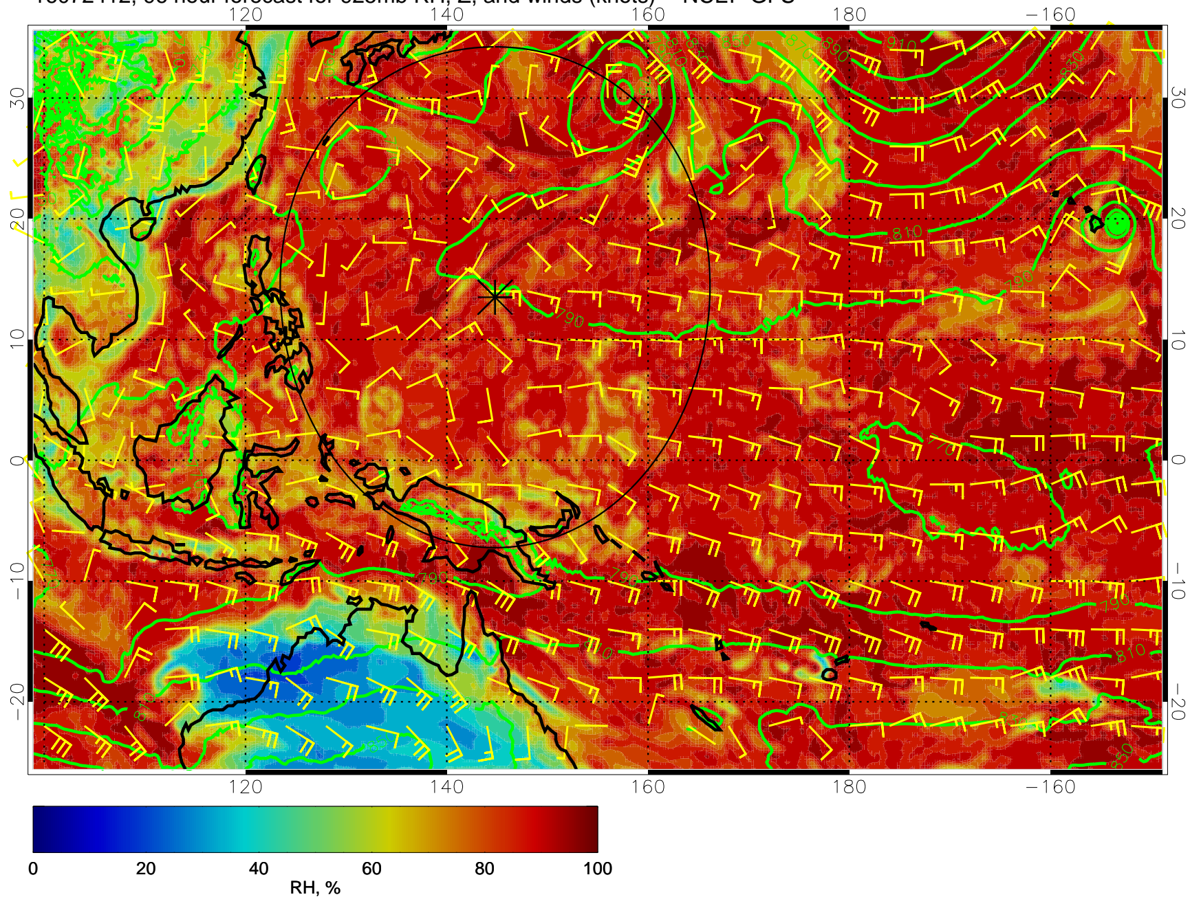
16072412, 96 hour forecast for 925mb RH, Z, and winds (knots) -- NCEP GFS
