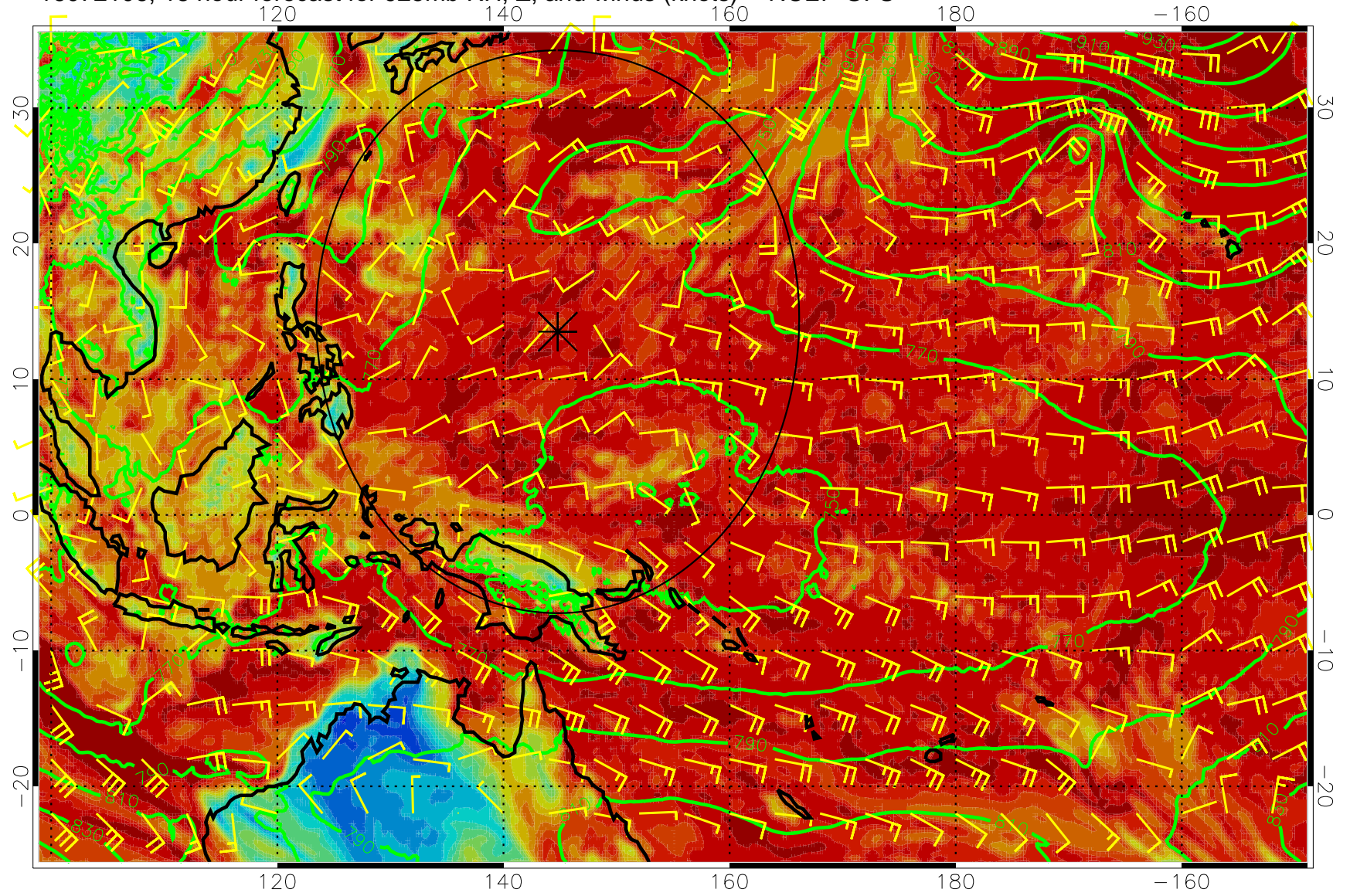
16072106, 18 hour forecast for 925mb RH, Z, and winds (knots) -- NCEP GFS
