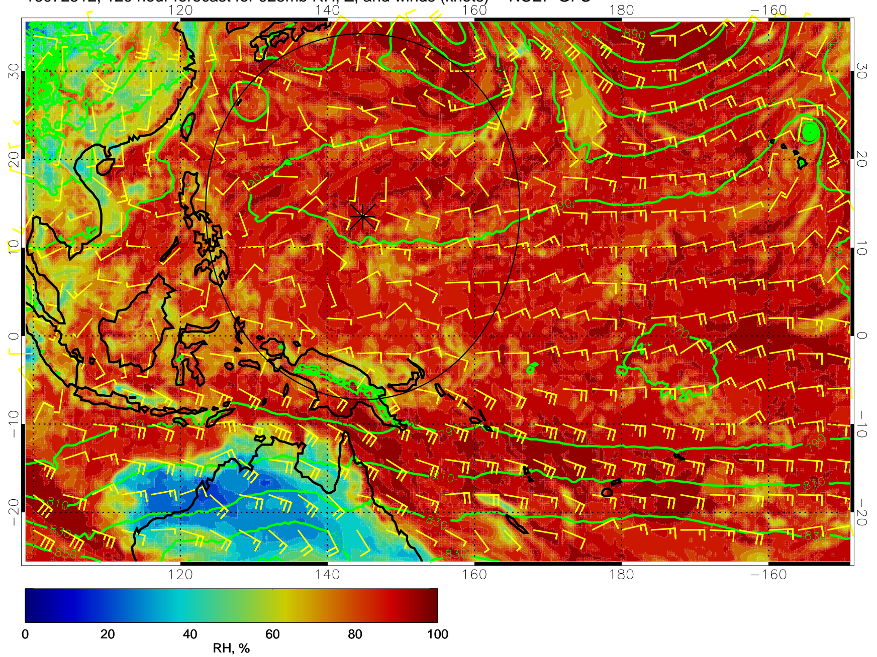
16072512, 120 hour forecast for 925mb RH, Z, and winds (knots) -- NCEP GFS
