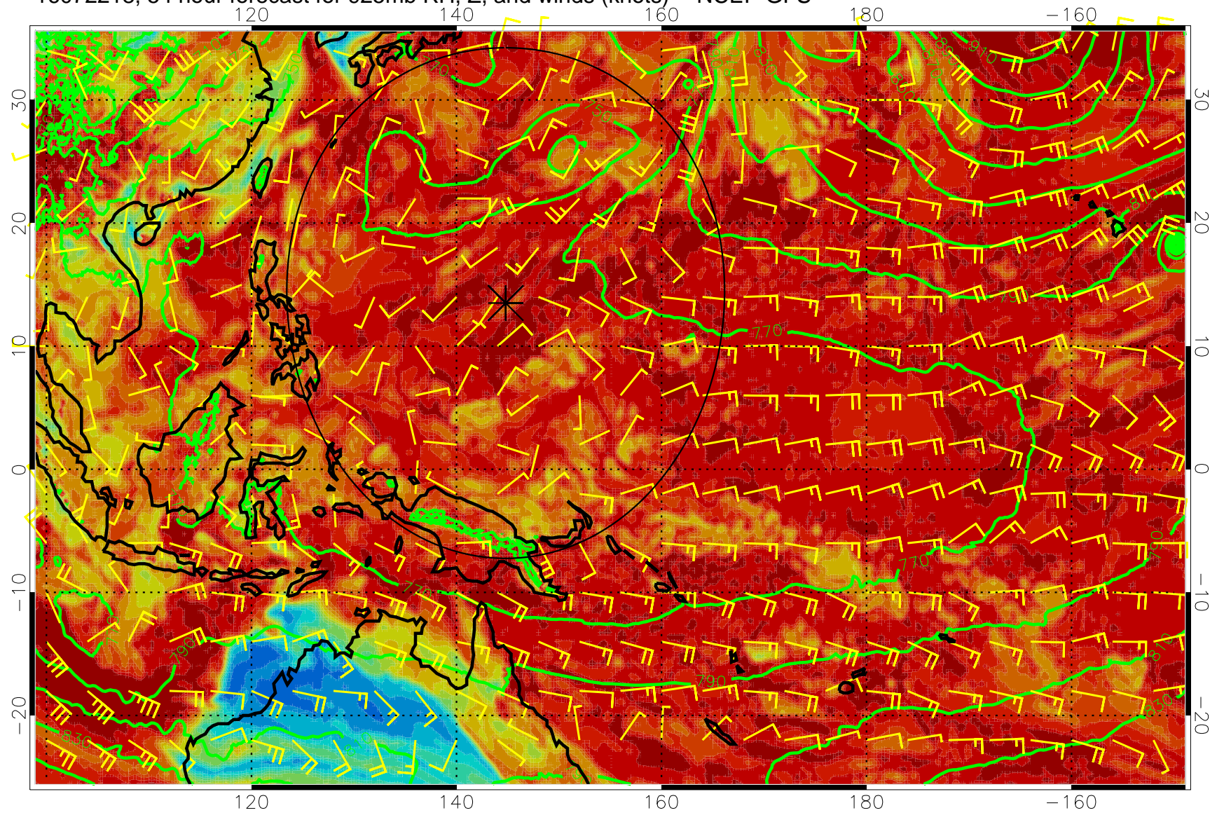
16072218, 54 hour forecast for 925mb RH, Z, and winds (knots) -- NCEP GFS
