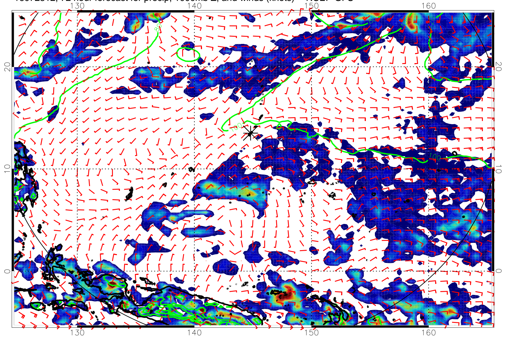
16072312, 72 hour forecast for precip, 1000mb Z, and winds (knots) -- NCEP GFS
