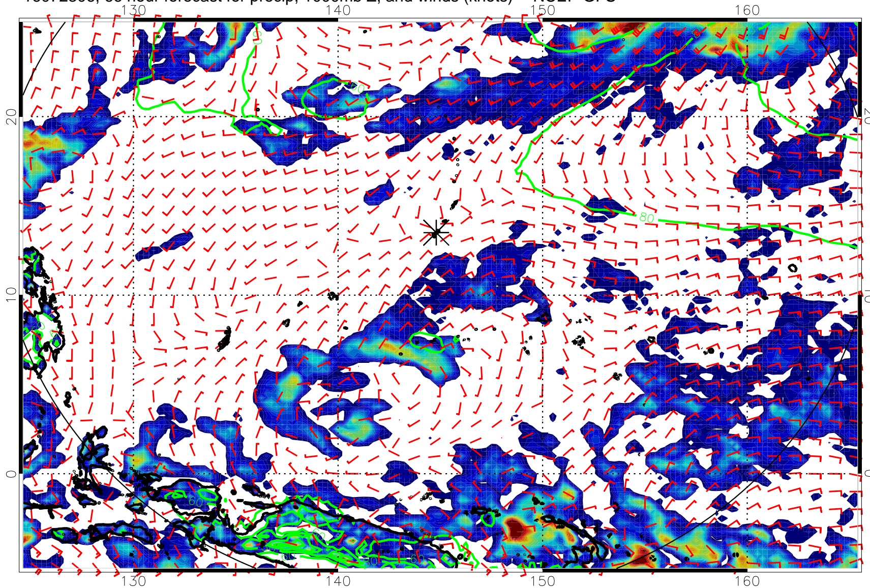
16072306, 66 hour forecast for precip, 1000mb Z, and winds (knots) -- NCEP GFS
