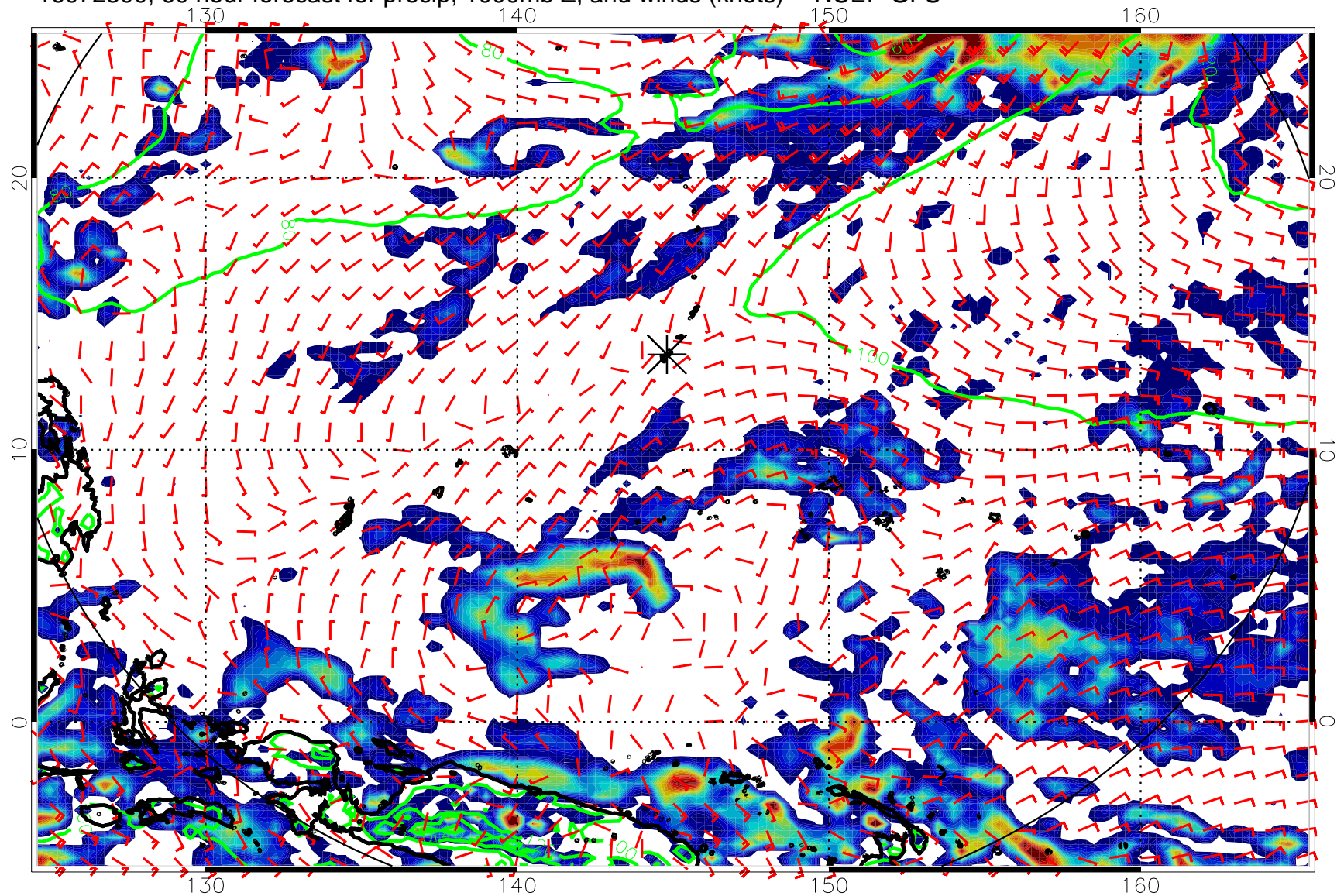
16072300, 60 hour forecast for precip, 1000mb Z, and winds (knots) -- NCEP GFS
