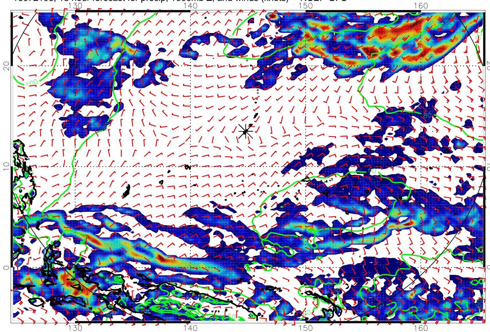
16072106, 18 hour forecast for precip, 1000mb Z, and winds (knots) -- NCEP GFS
