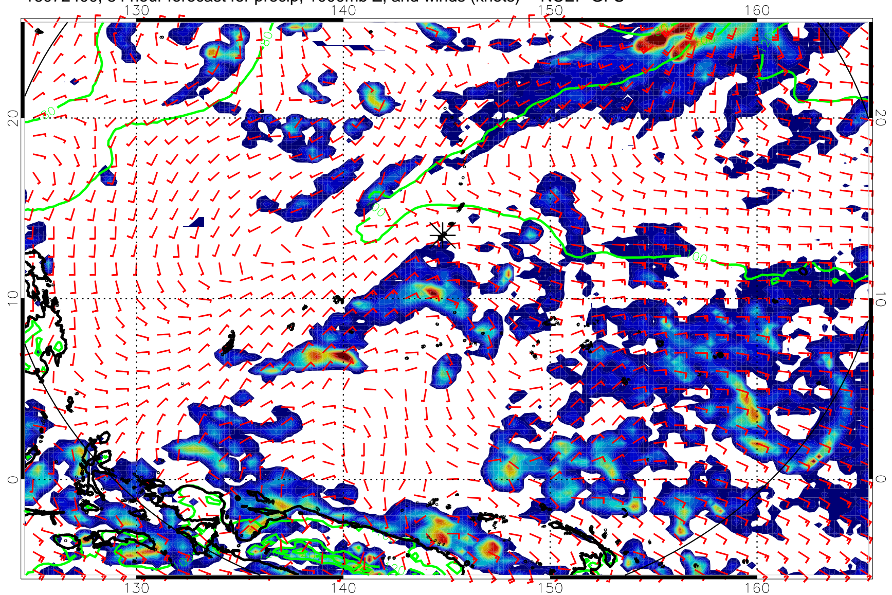
16072400, 84 hour forecast for precip, 1000mb Z, and winds (knots) -- NCEP GFS
