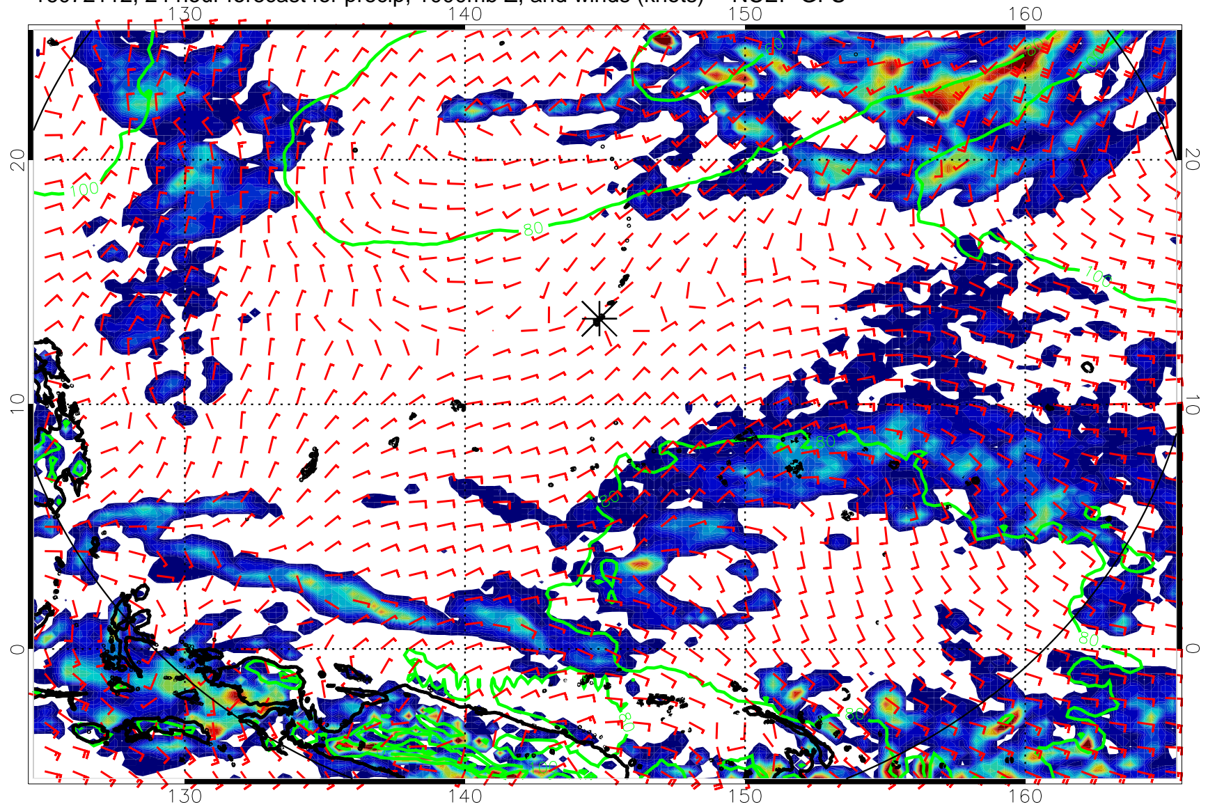
16072112, 24 hour forecast for precip, 1000mb Z, and winds (knots) -- NCEP GFS
