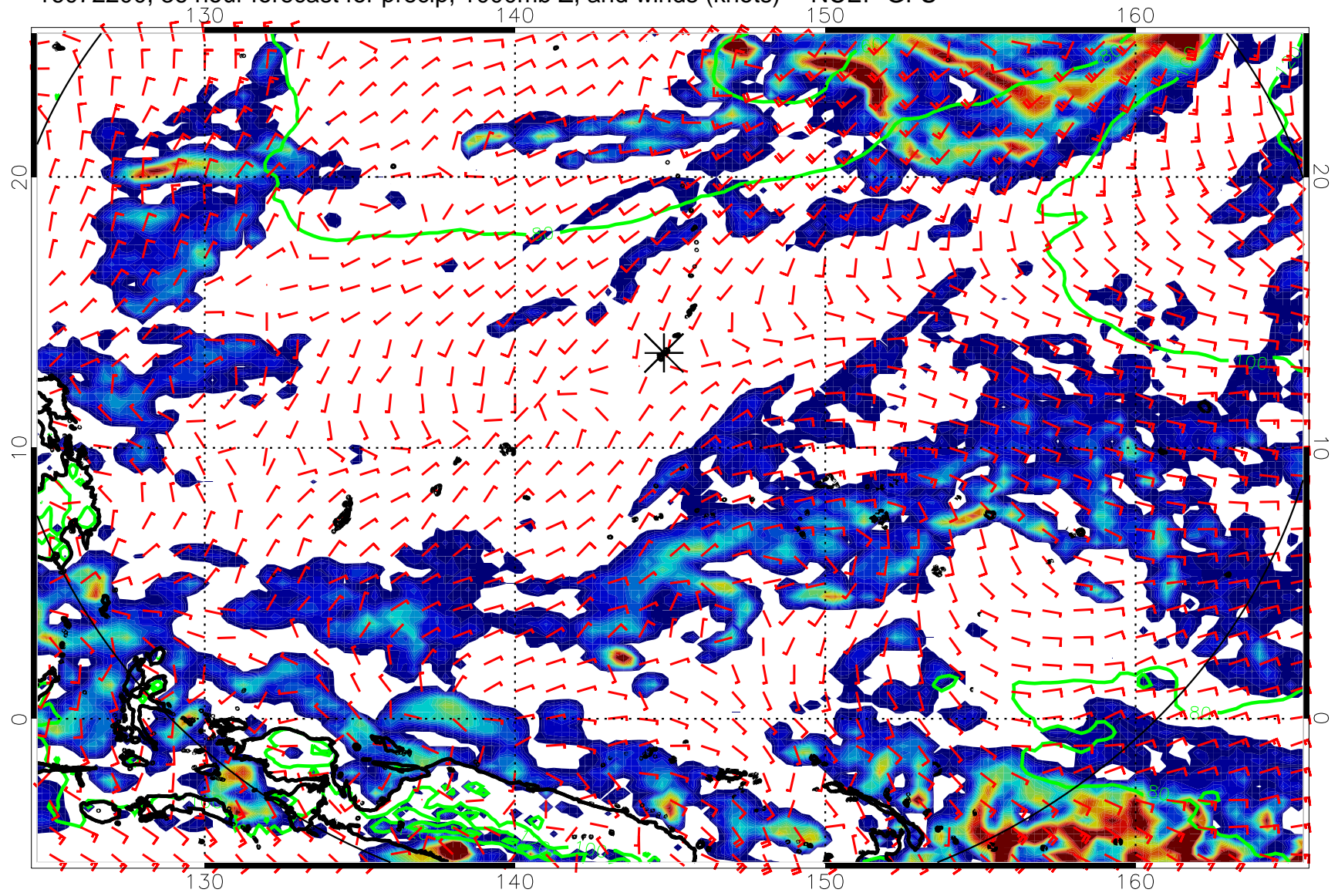
16072200, 36 hour forecast for precip, 1000mb Z, and winds (knots) -- NCEP GFS
