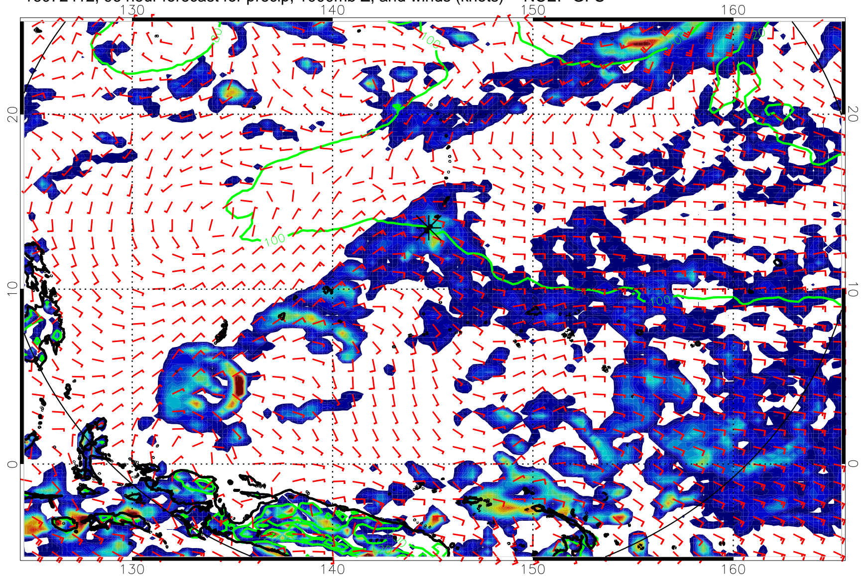
16072412, 96 hour forecast for precip, 1000mb Z, and winds (knots) -- NCEP GFS
