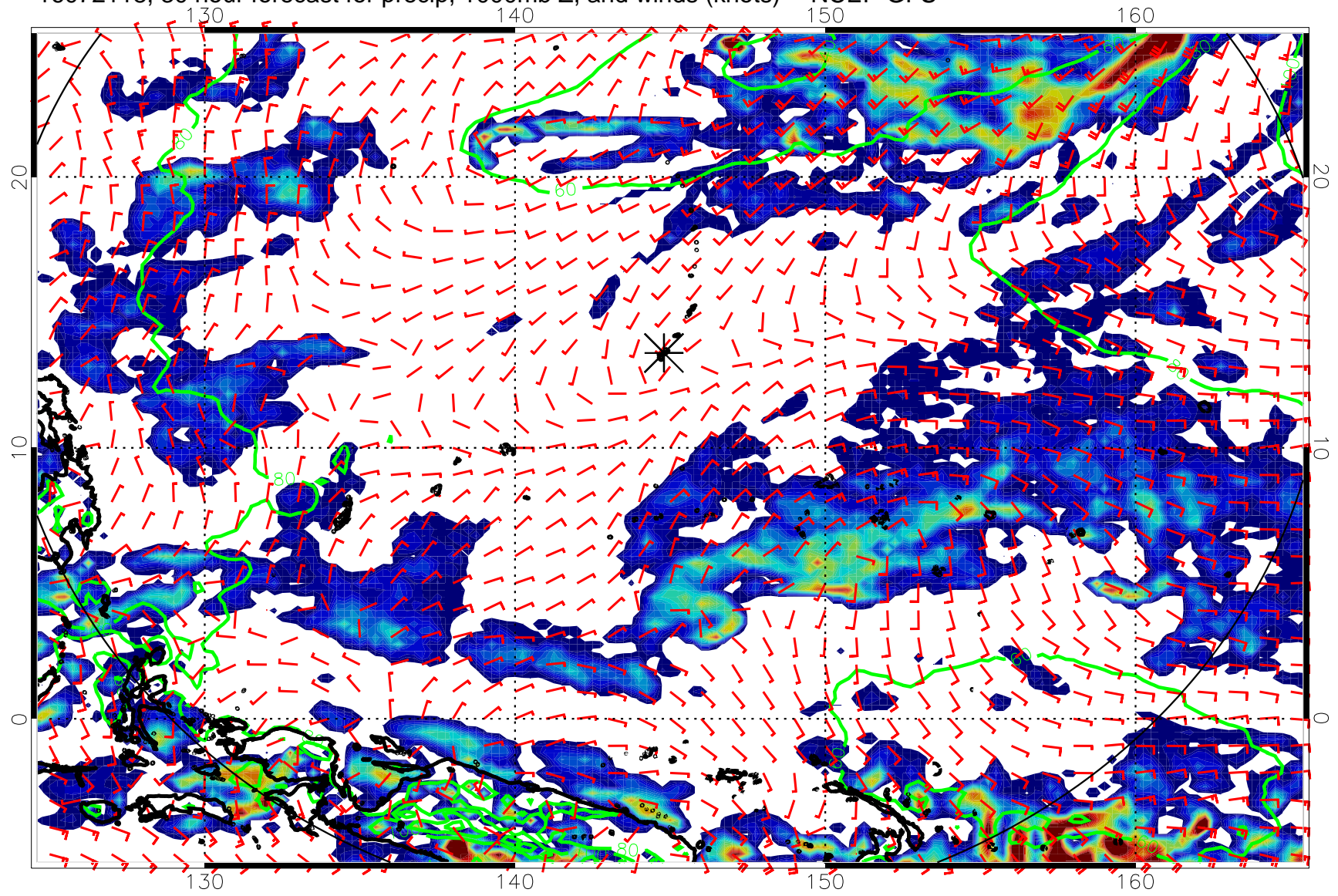
16072118, 30 hour forecast for precip, 1000mb Z, and winds (knots) -- NCEP GFS
