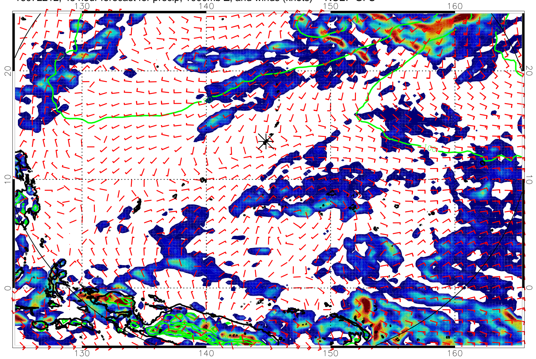
16072212, 48 hour forecast for precip, 1000mb Z, and winds (knots) -- NCEP GFS
