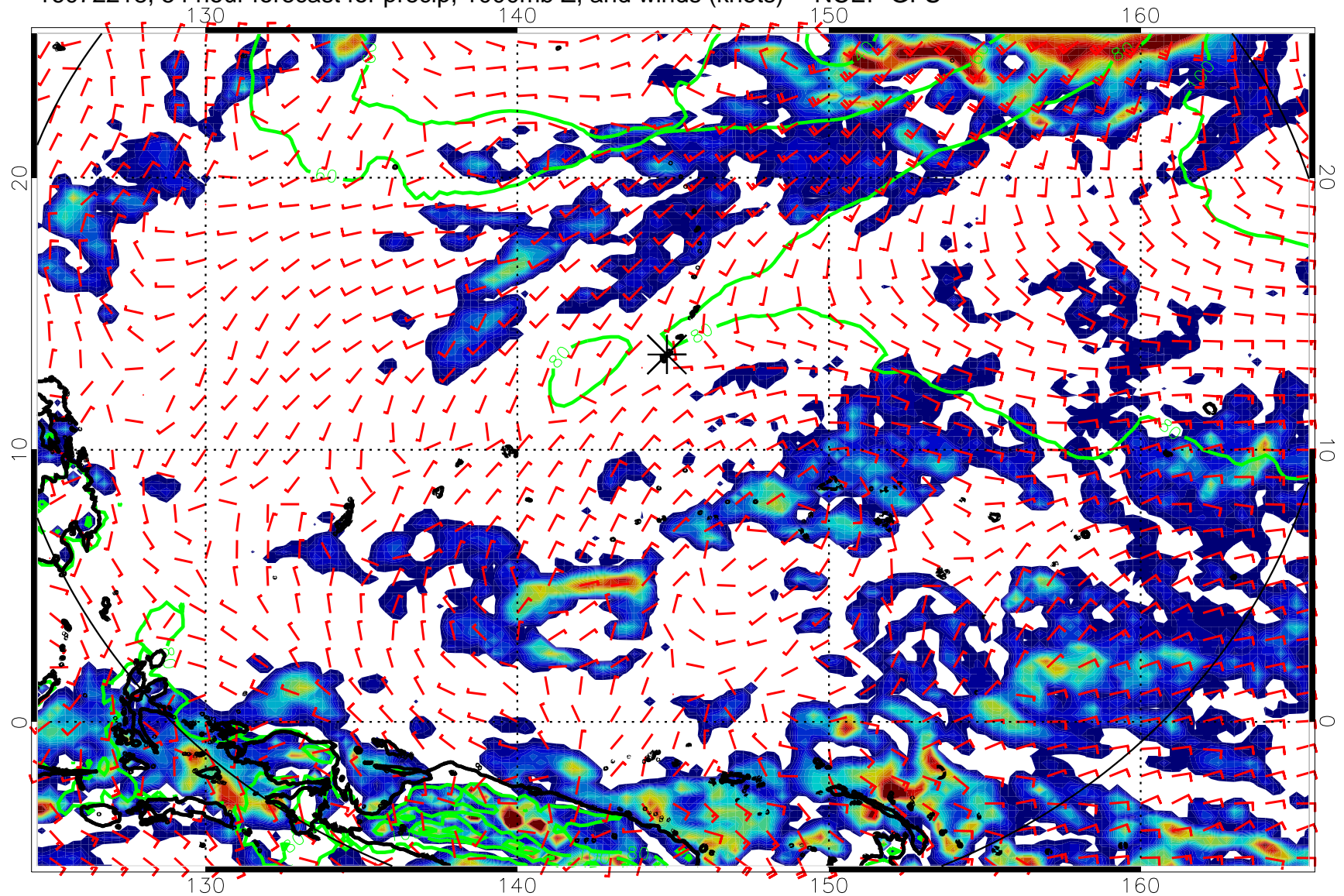
16072218, 54 hour forecast for precip, 1000mb Z, and winds (knots) -- NCEP GFS
