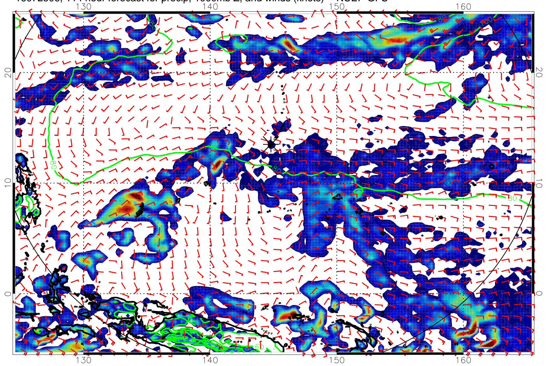
16072506, 114 hour forecast for precip, 1000mb Z, and winds (knots) -- NCEP GFS
