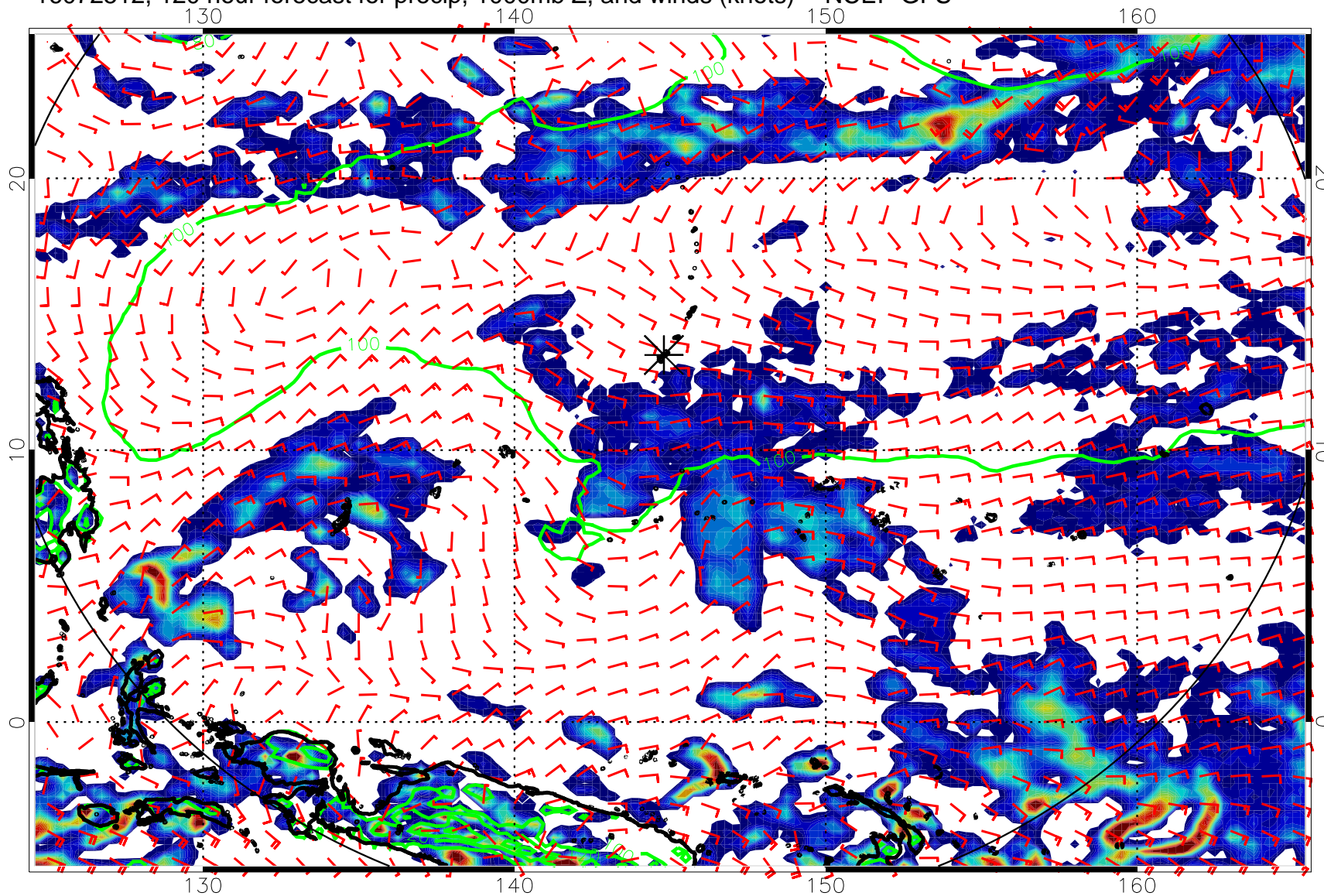
16072512, 120 hour forecast for precip, 1000mb Z, and winds (knots) -- NCEP GFS
