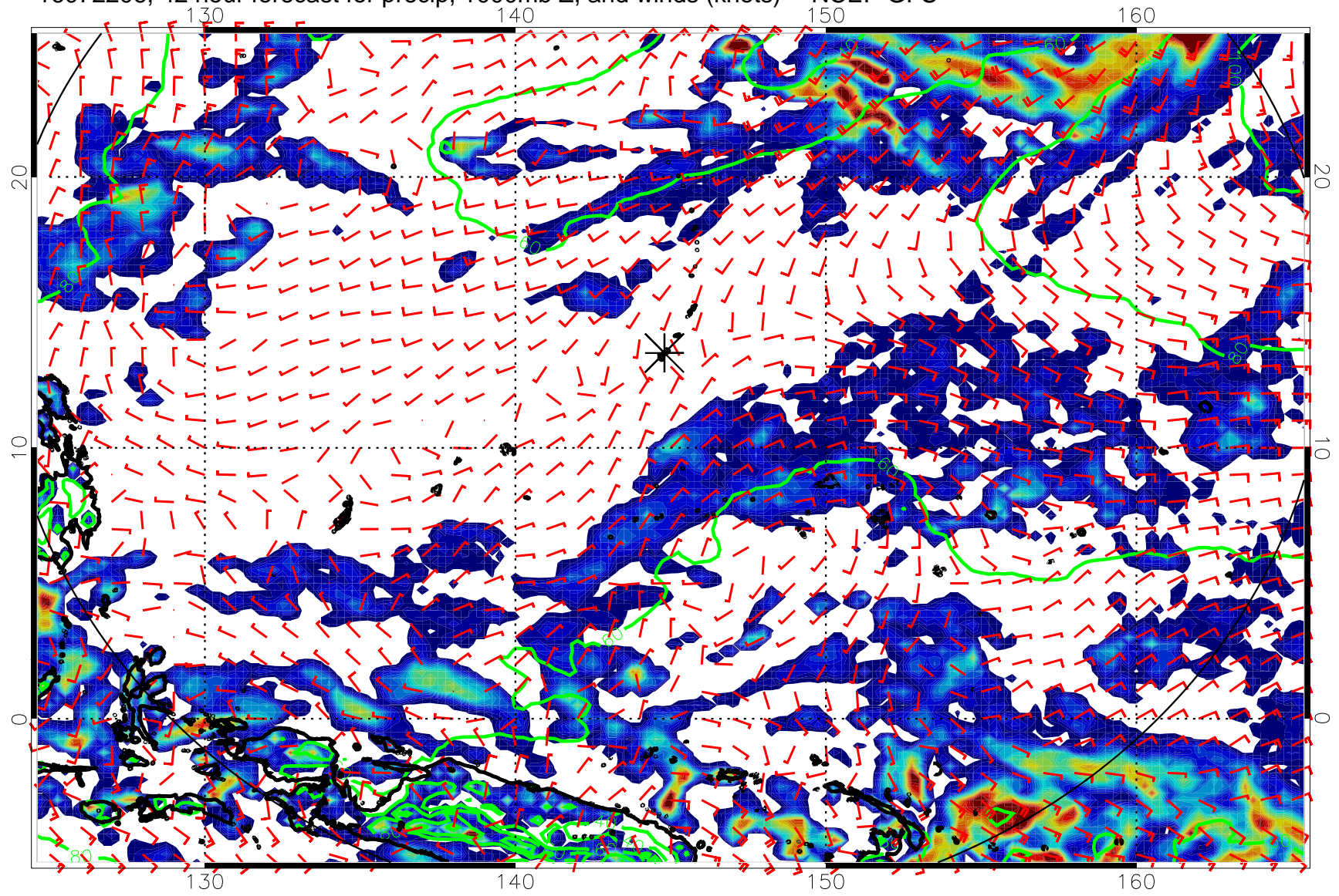
16072206, 42 hour forecast for precip, 1000mb Z, and winds (knots) -- NCEP GFS
