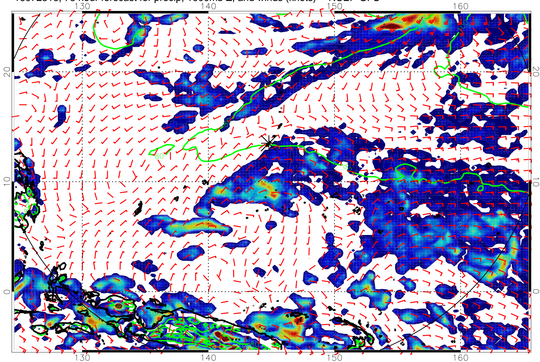
16072318, 78 hour forecast for precip, 1000mb Z, and winds (knots) -- NCEP GFS
