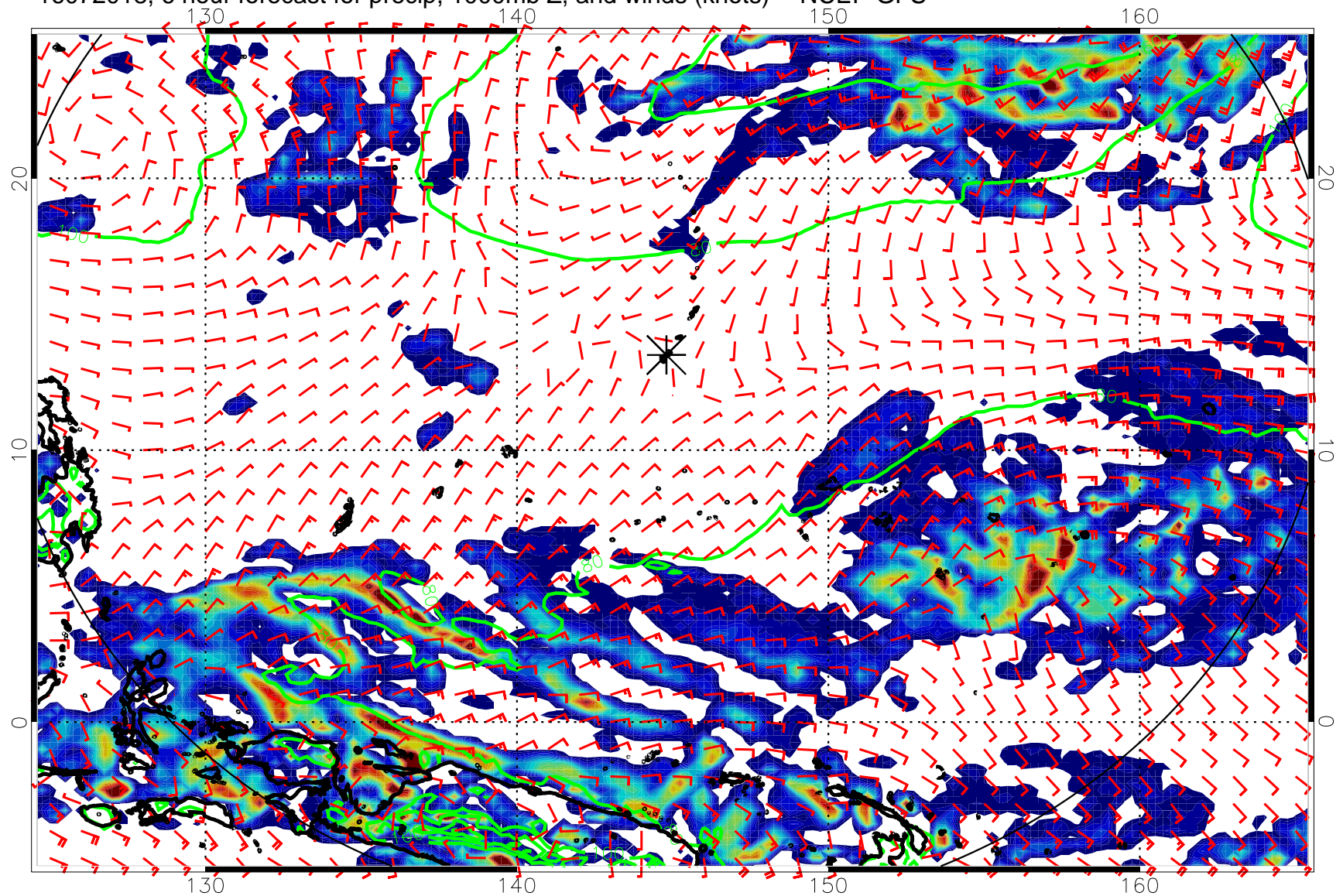
16072018, 6 hour forecast for precip, 1000mb Z, and winds (knots) -- NCEP GFS
