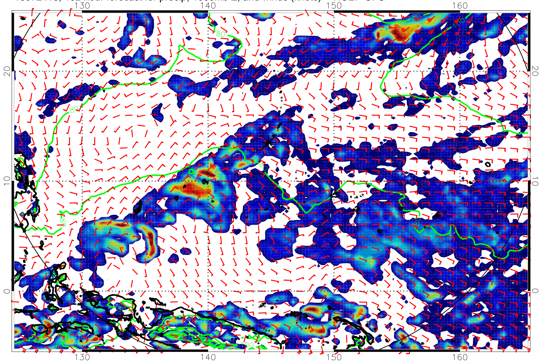
16072418, 102 hour forecast for precip, 1000mb Z, and winds (knots) -- NCEP GFS
