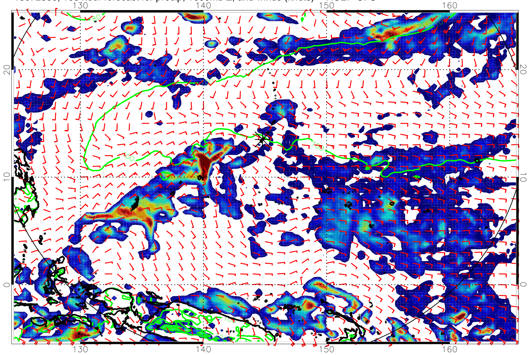
16072500, 108 hour forecast for precip, 1000mb Z, and winds (knots) -- NCEP GFS
