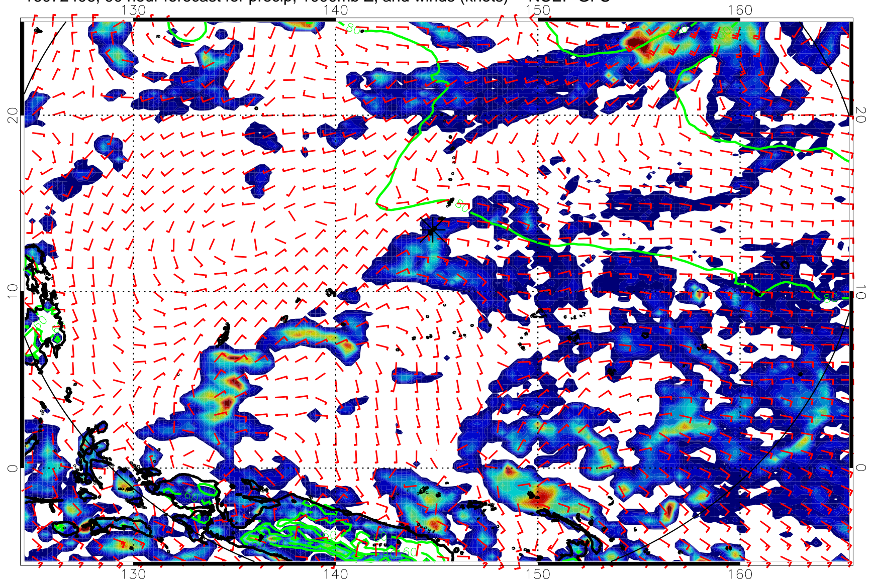
16072406, 90 hour forecast for precip, 1000mb Z, and winds (knots) -- NCEP GFS
