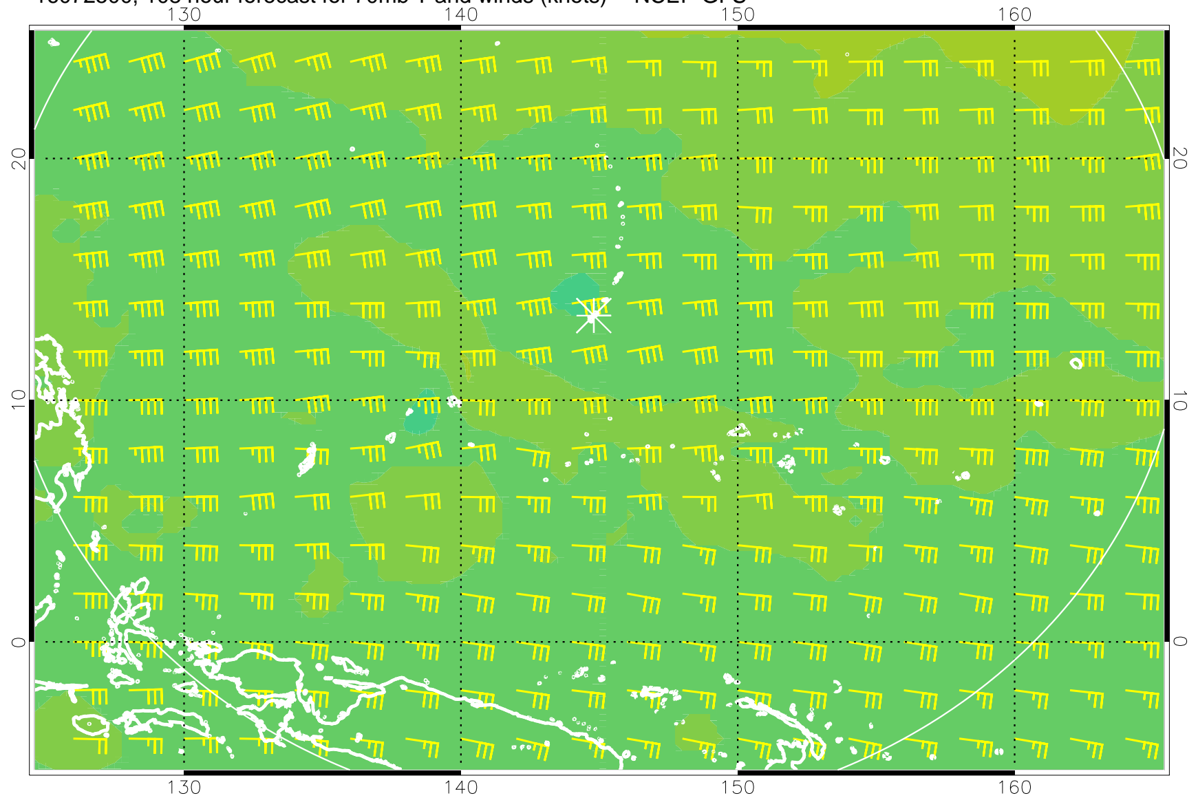
16072500, 108 hour forecast for 70mb T and winds (knots) -- NCEP GFS
