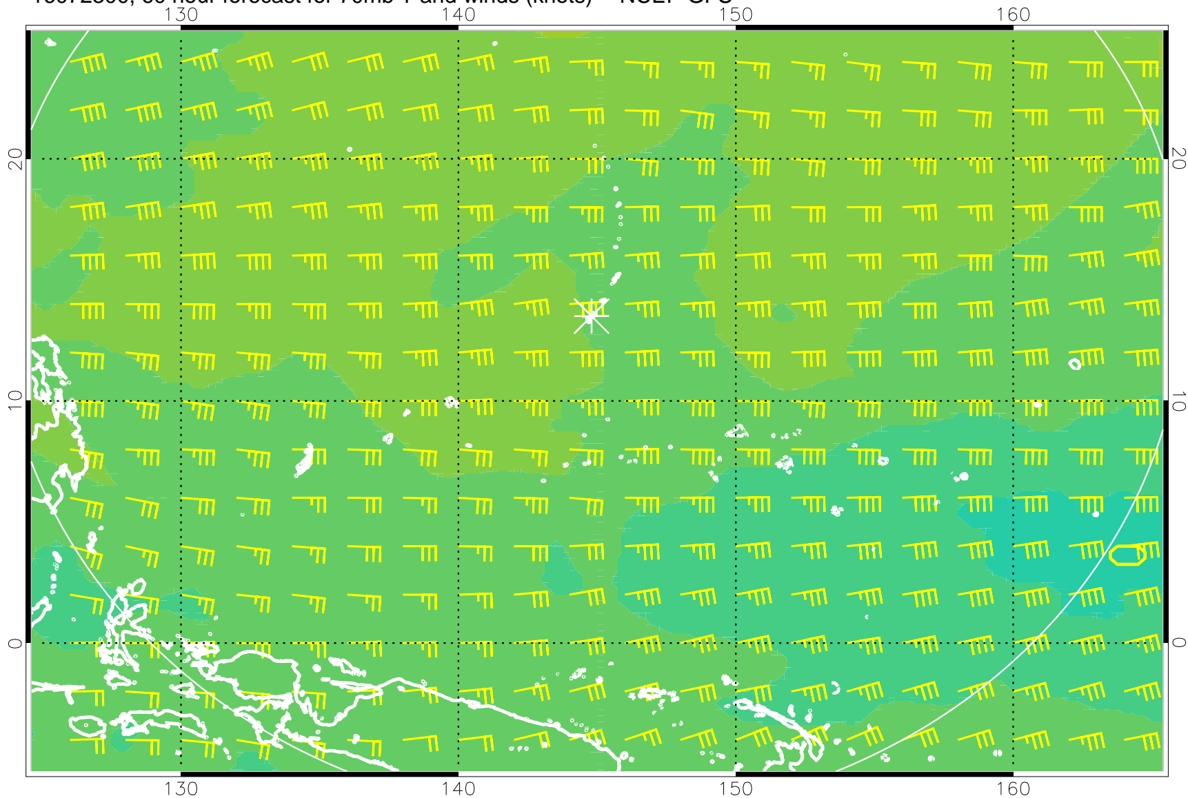
16072300, 60 hour forecast for 70mb T and winds (knots) -- NCEP GFS
