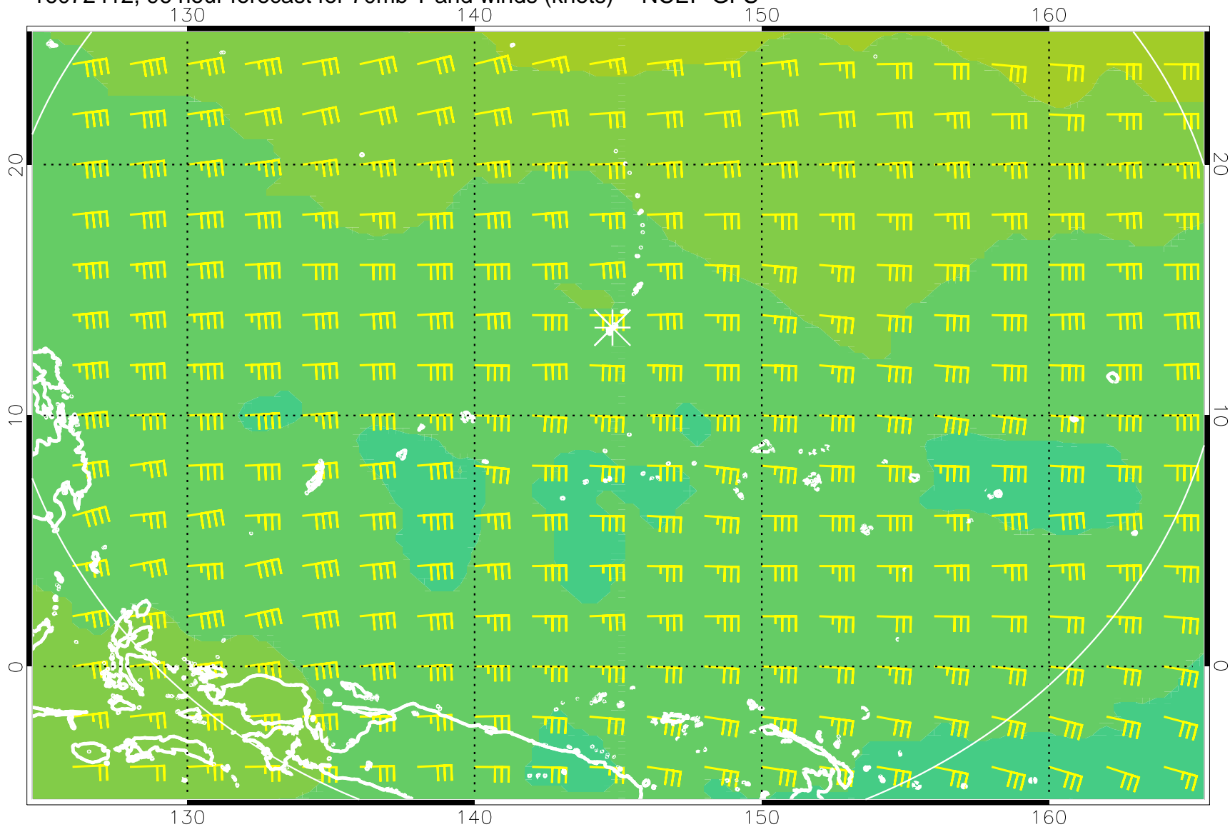
16072412, 96 hour forecast for 70mb T and winds (knots) -- NCEP GFS
