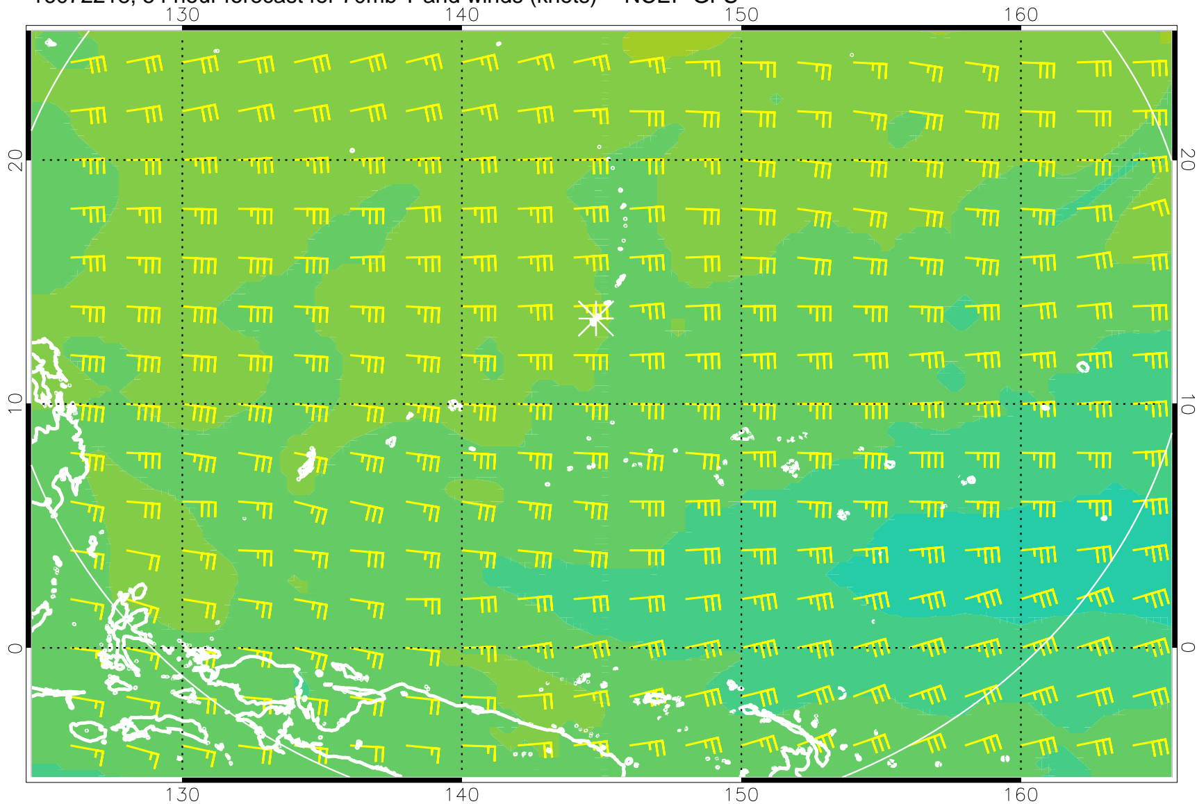
16072218, 54 hour forecast for 70mb T and winds (knots) -- NCEP GFS
