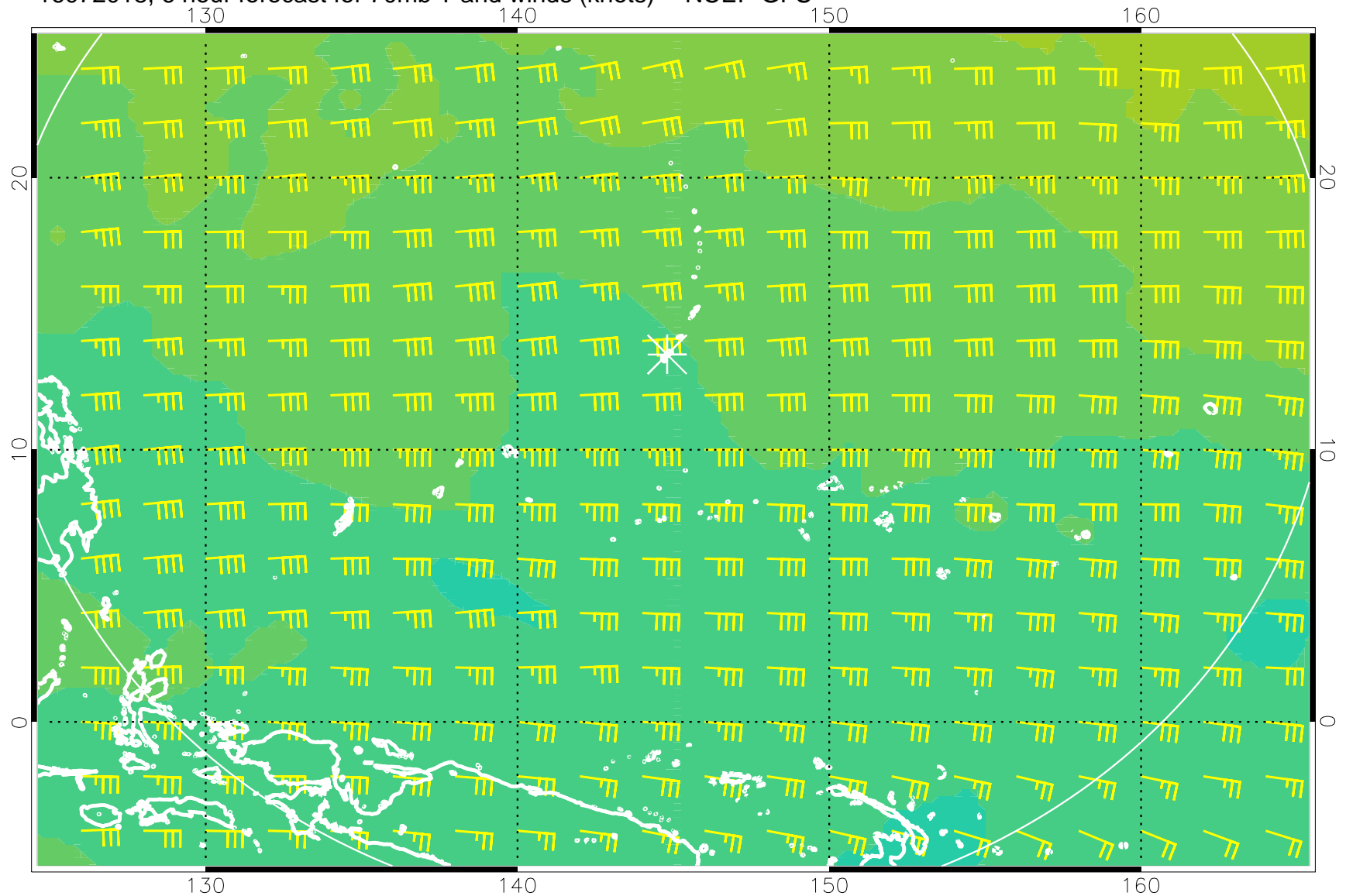
16072018, 6 hour forecast for 70mb T and winds (knots) -- NCEP GFS
