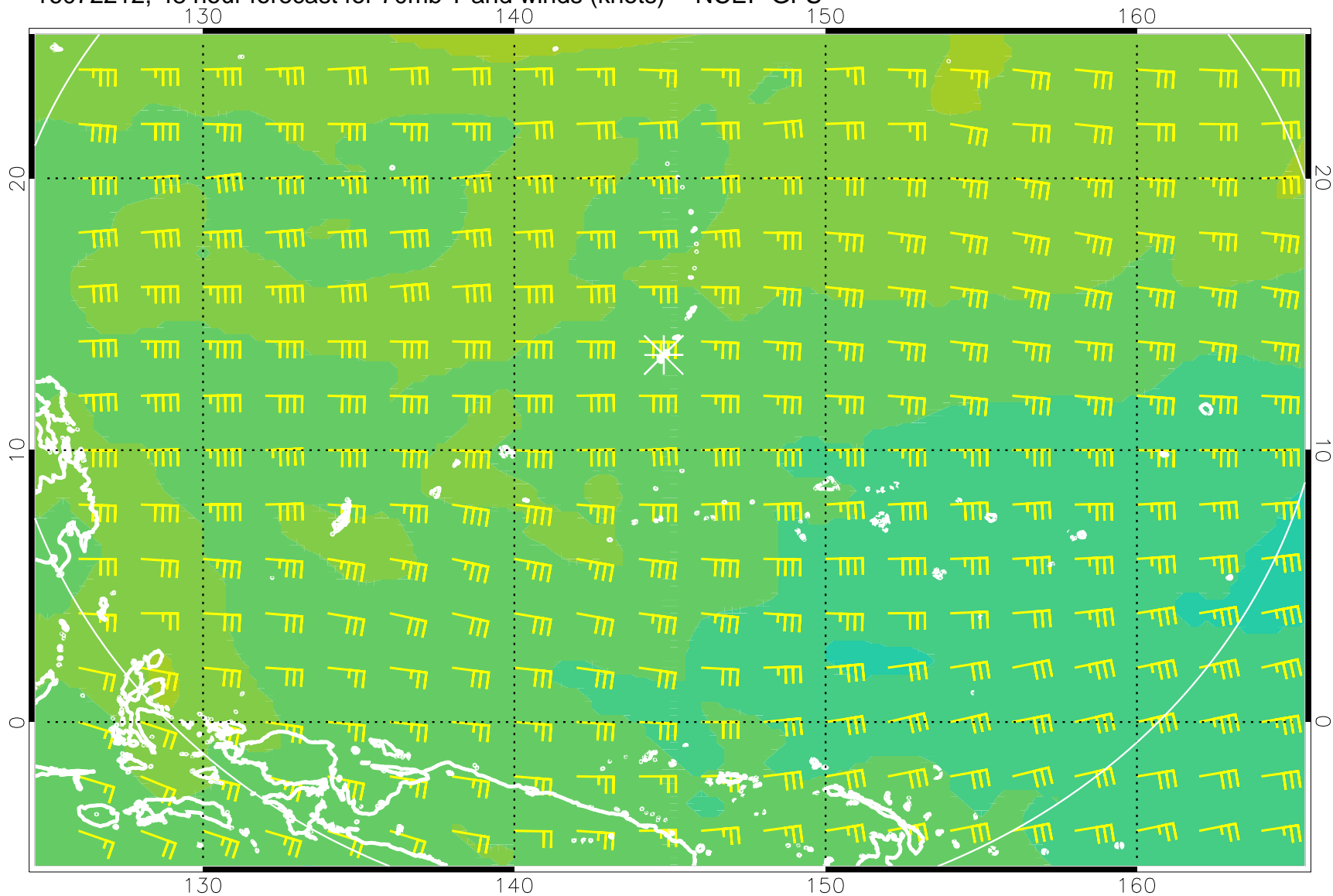
16072212, 48 hour forecast for 70mb T and winds (knots) -- NCEP GFS
