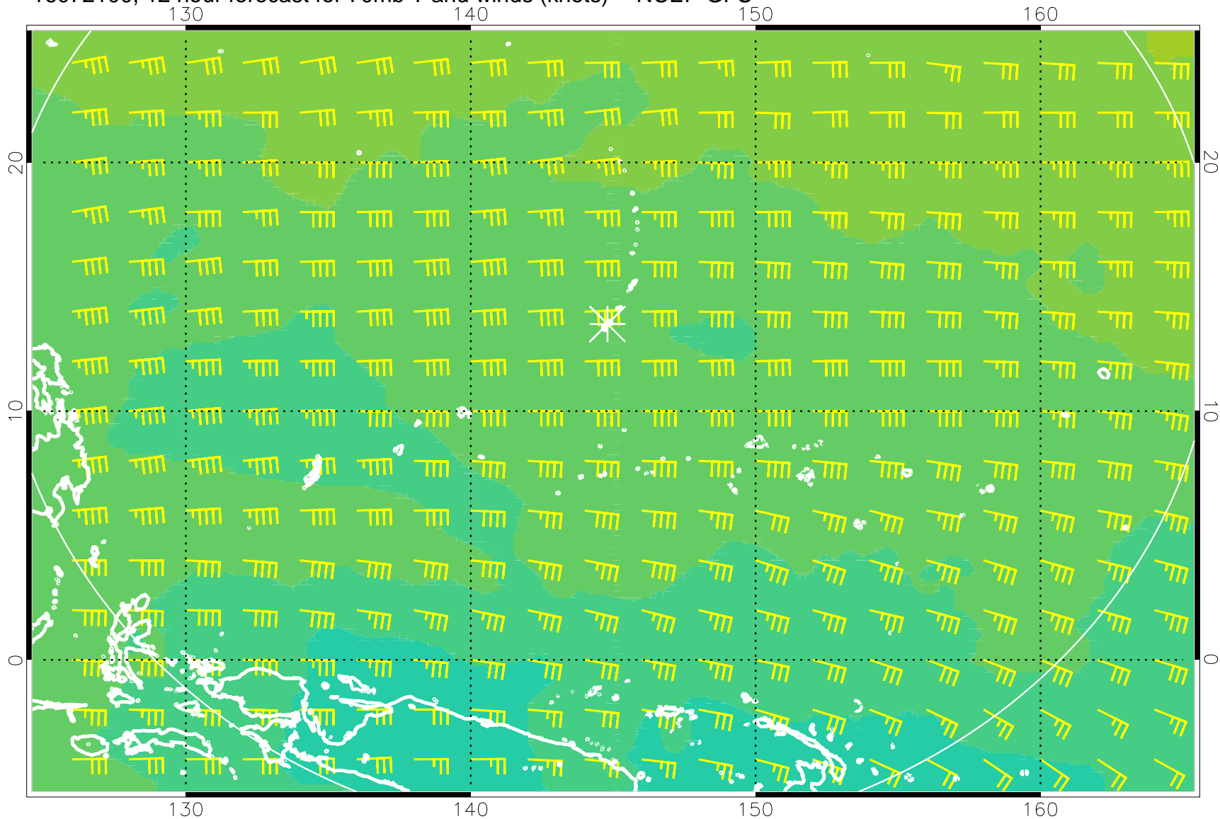
16072100, 12 hour forecast for 70mb T and winds (knots) -- NCEP GFS
