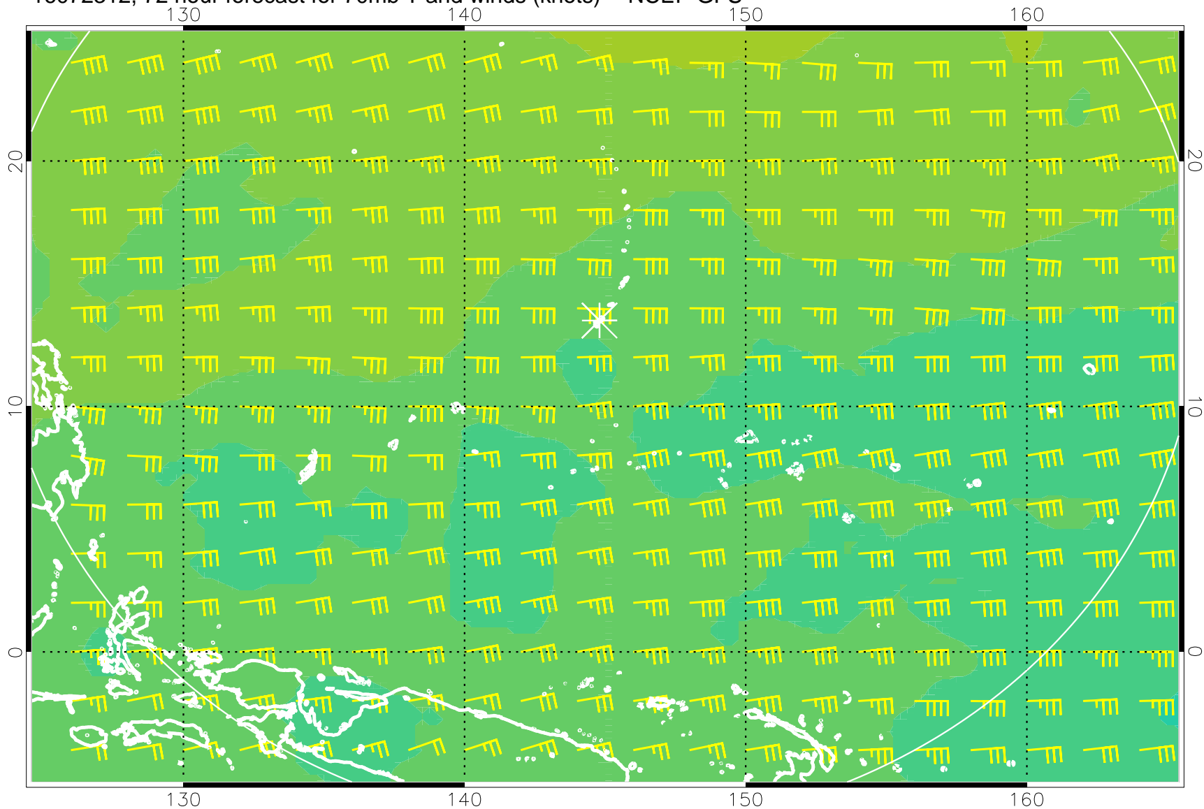
16072312, 72 hour forecast for 70mb T and winds (knots) -- NCEP GFS
