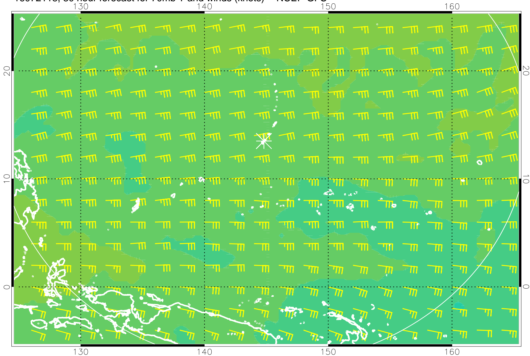
16072118, 30 hour forecast for 70mb T and winds (knots) -- NCEP GFS
