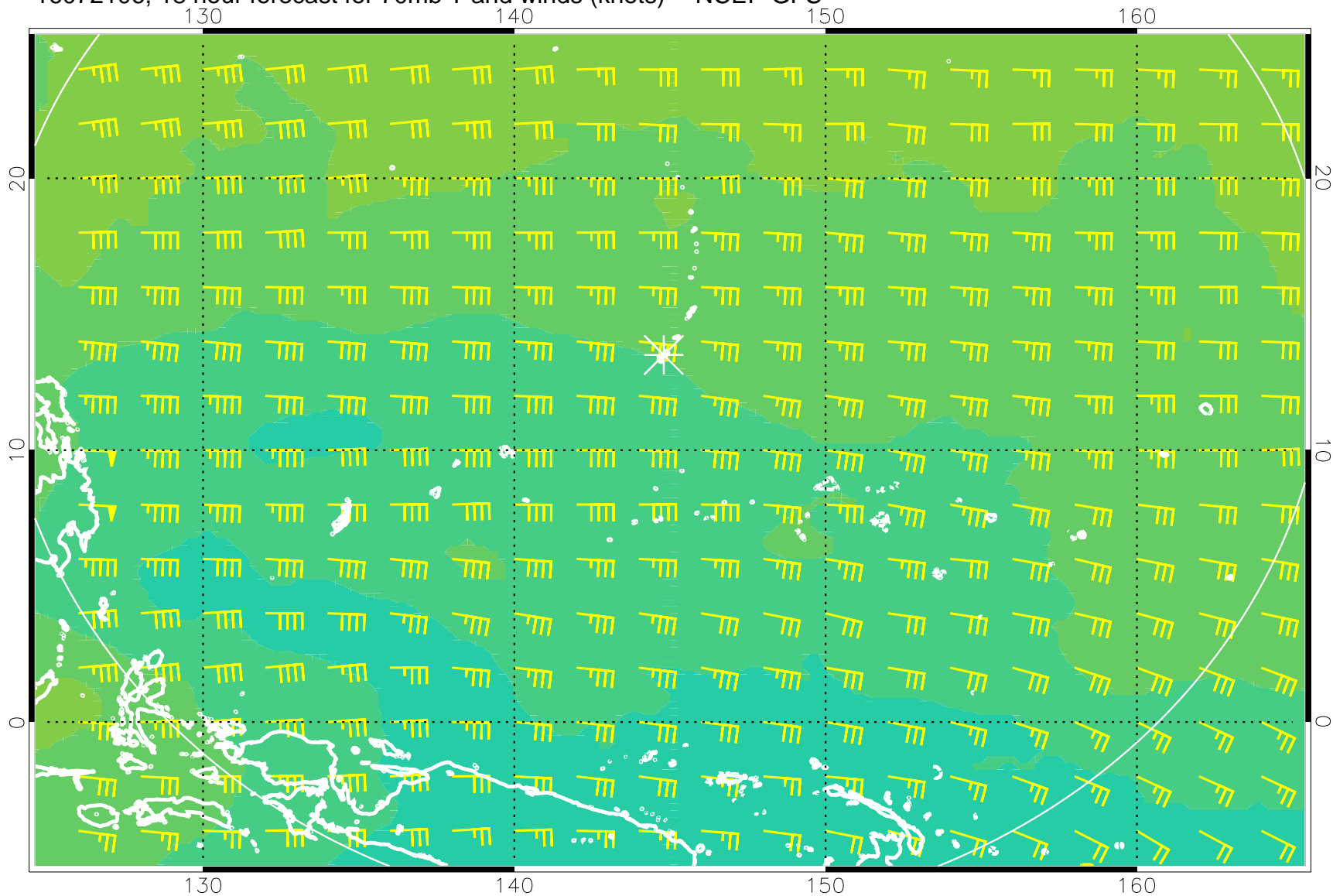
16072106, 18 hour forecast for 70mb T and winds (knots) -- NCEP GFS
