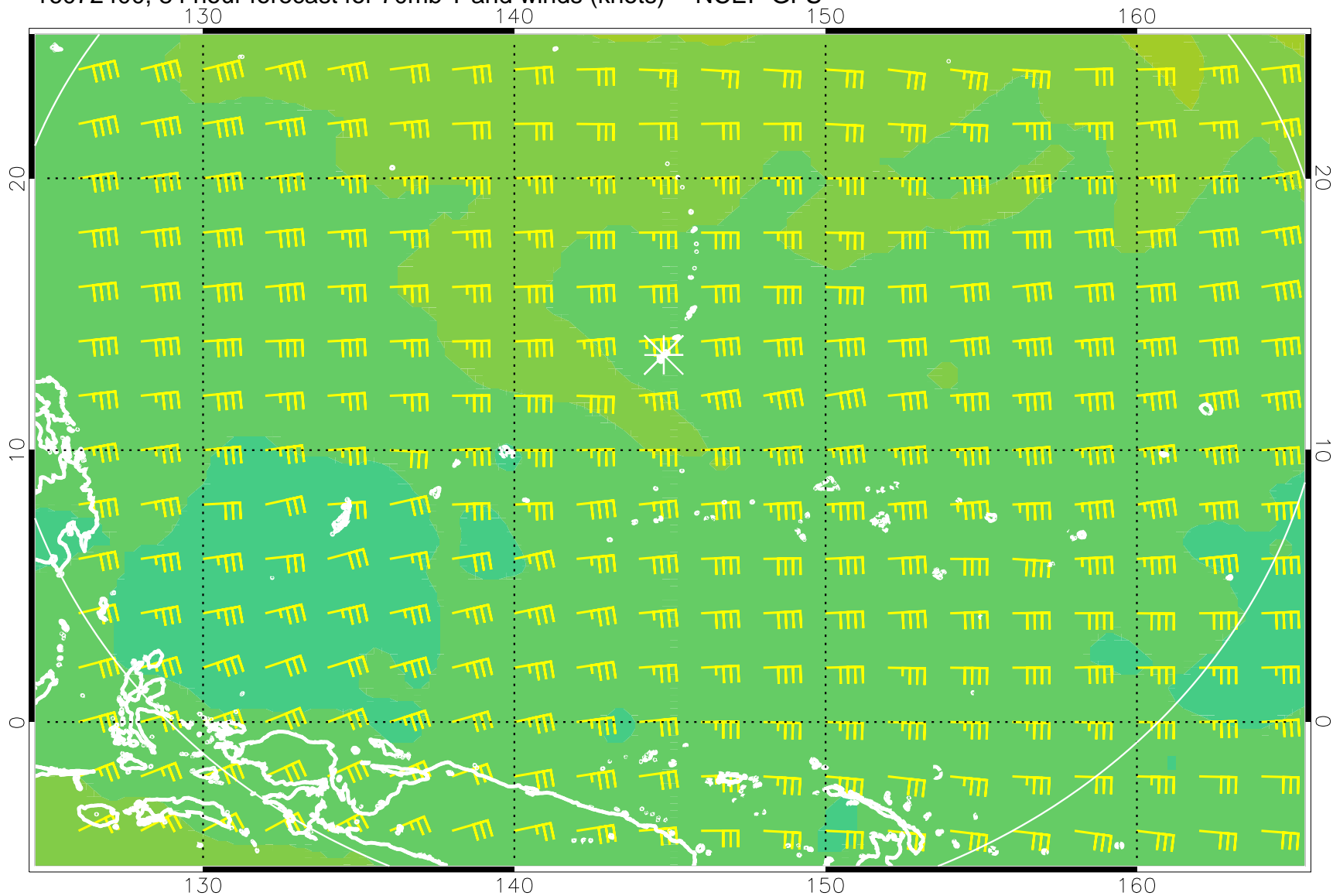
16072400, 84 hour forecast for 70mb T and winds (knots) -- NCEP GFS
