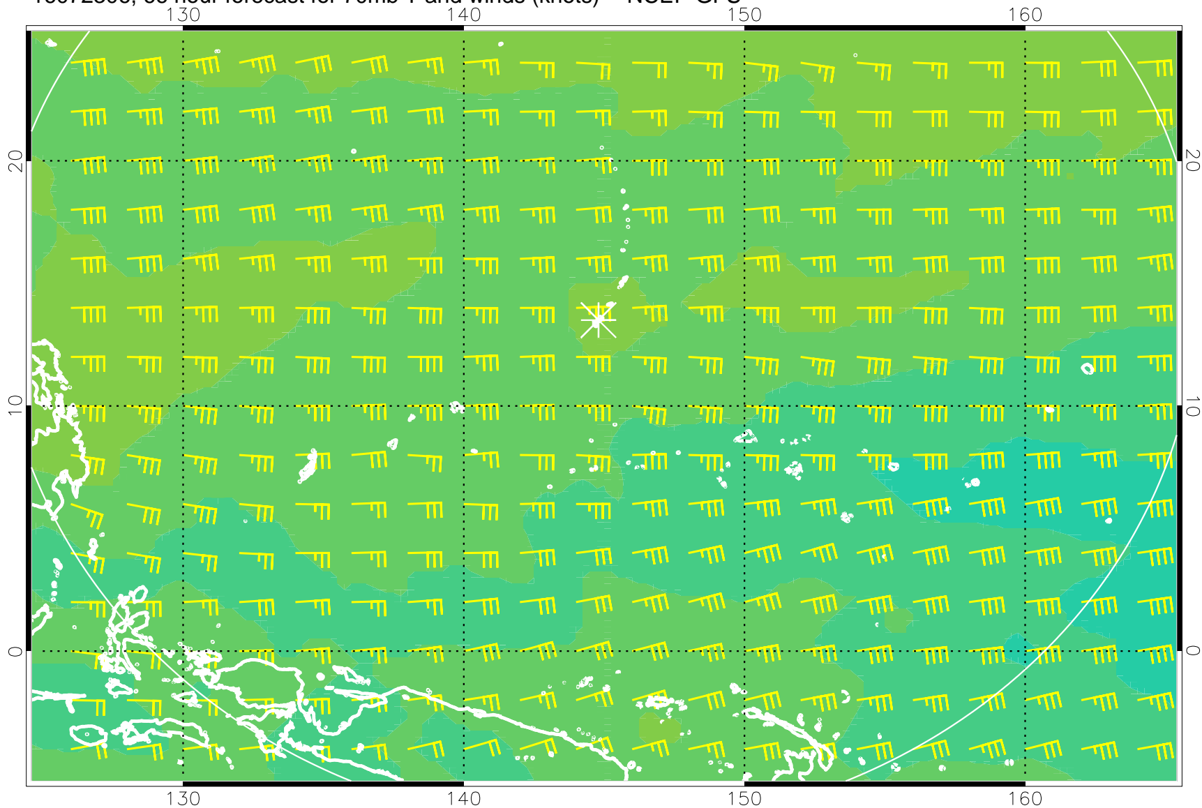
16072306, 66 hour forecast for 70mb T and winds (knots) -- NCEP GFS
