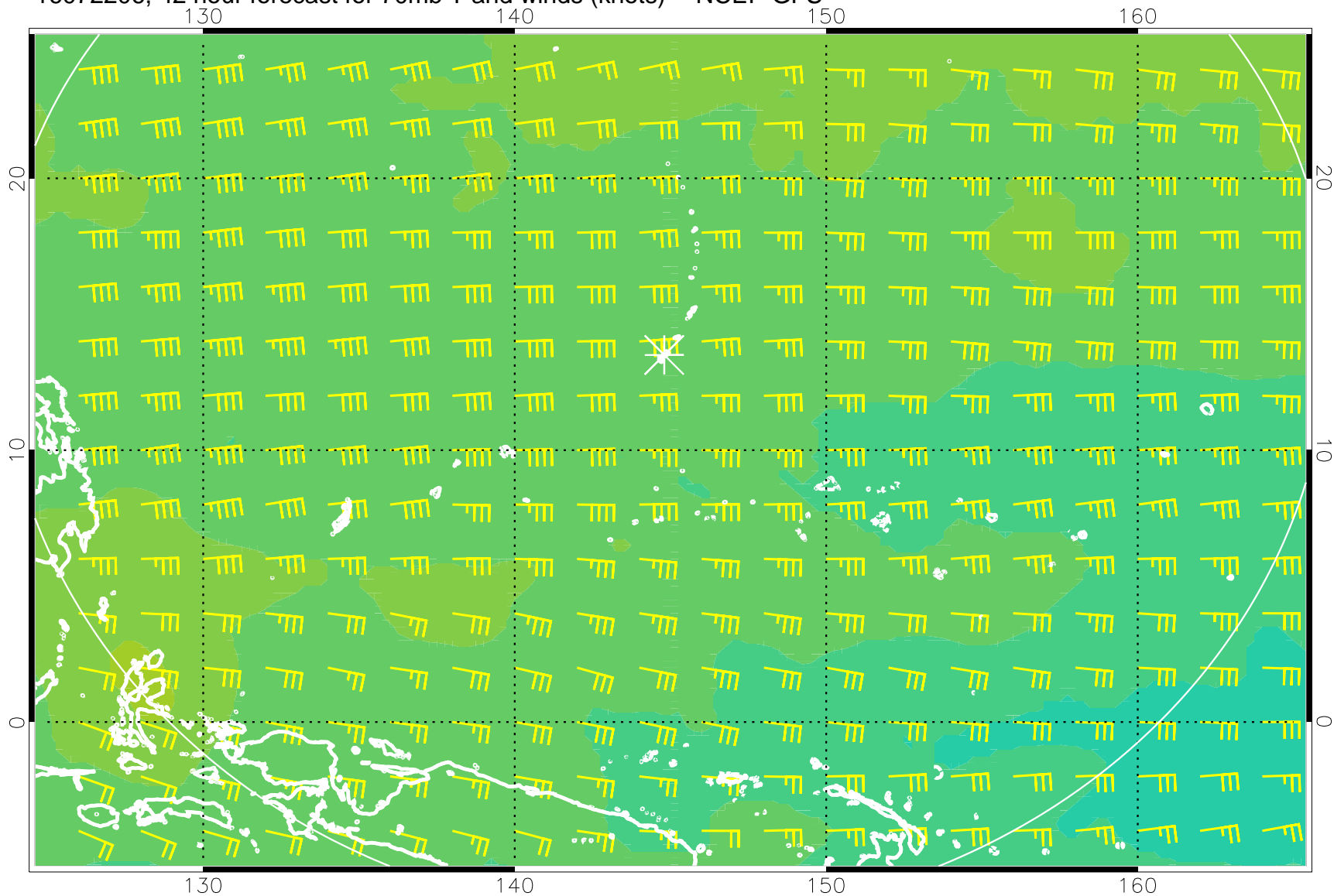
16072206, 42 hour forecast for 70mb T and winds (knots) -- NCEP GFS
