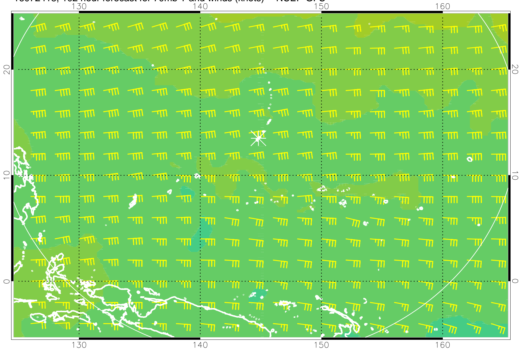
16072418, 102 hour forecast for 70mb T and winds (knots) -- NCEP GFS
