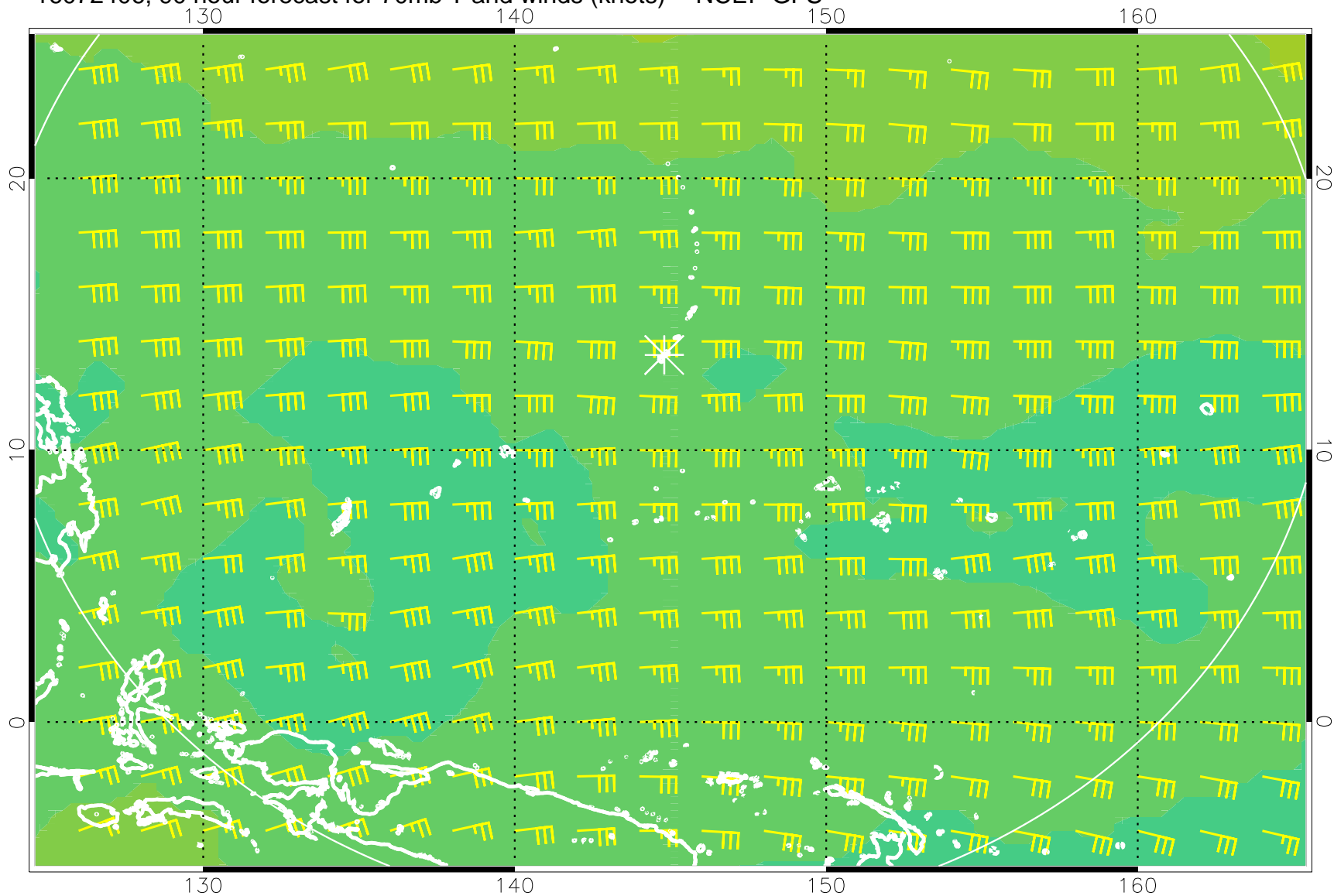
16072406, 90 hour forecast for 70mb T and winds (knots) -- NCEP GFS
