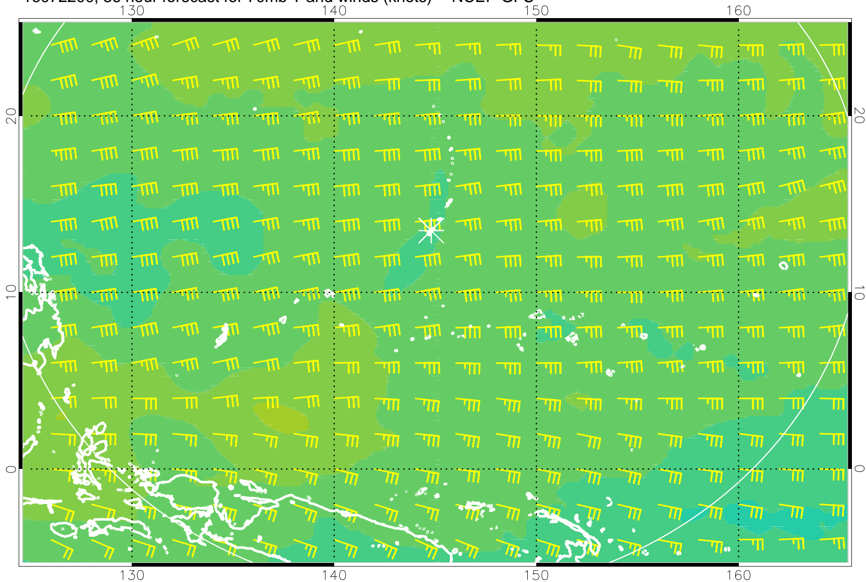
16072200, 36 hour forecast for 70mb T and winds (knots) -- NCEP GFS
