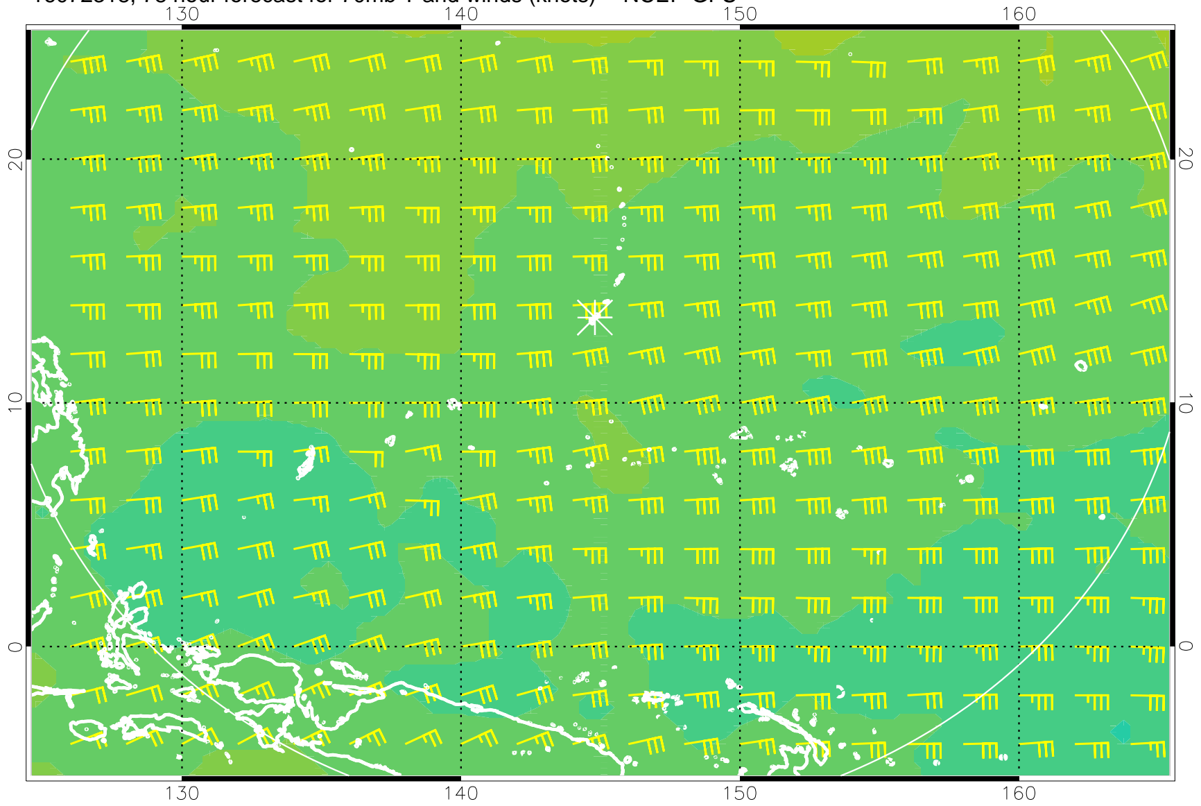
16072318, 78 hour forecast for 70mb T and winds (knots) -- NCEP GFS
