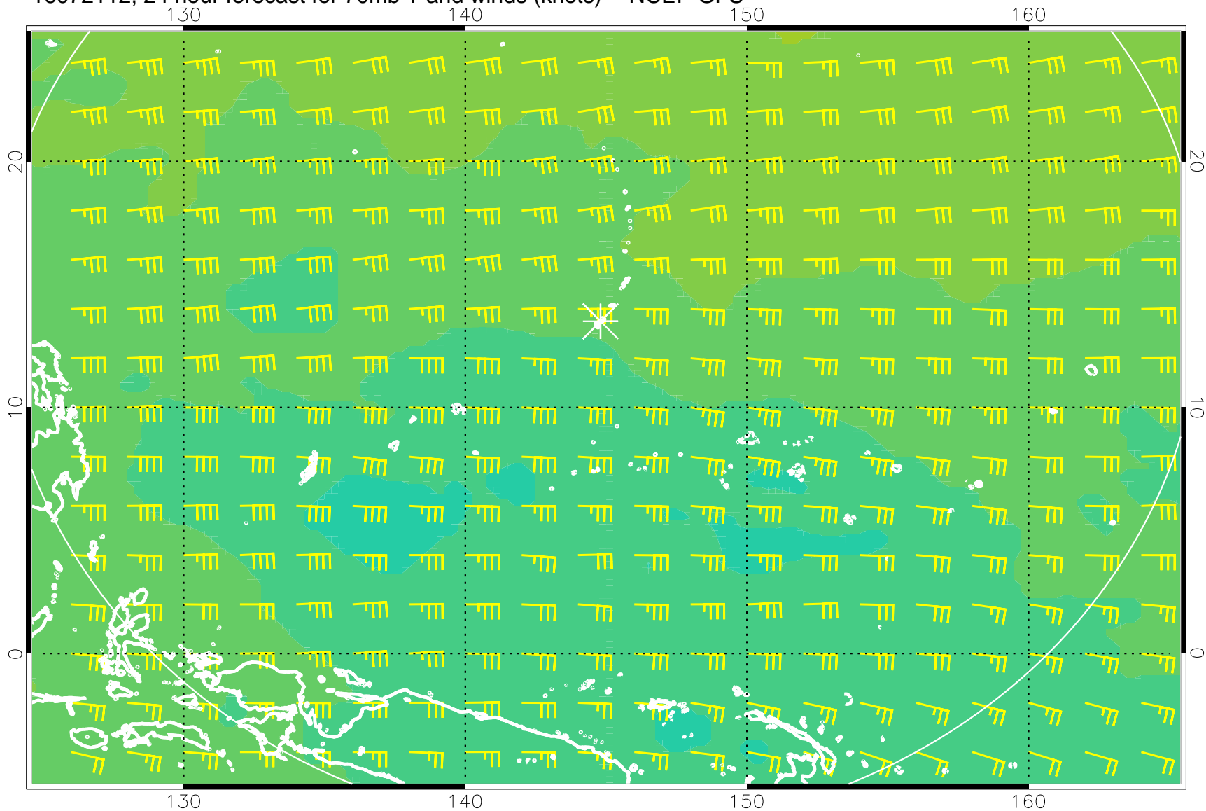
16072112, 24 hour forecast for 70mb T and winds (knots) -- NCEP GFS
