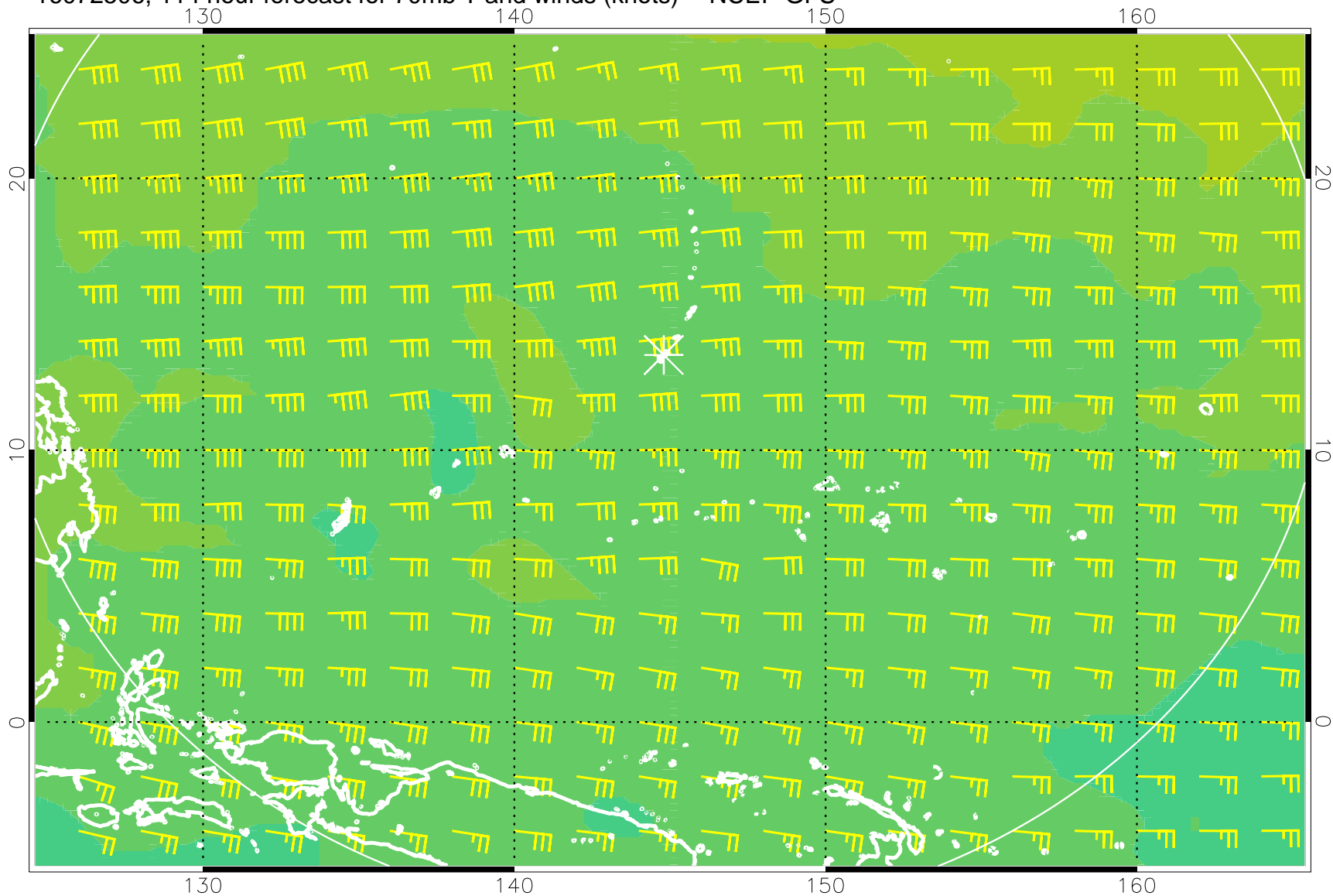
16072506, 114 hour forecast for 70mb T and winds (knots) -- NCEP GFS
