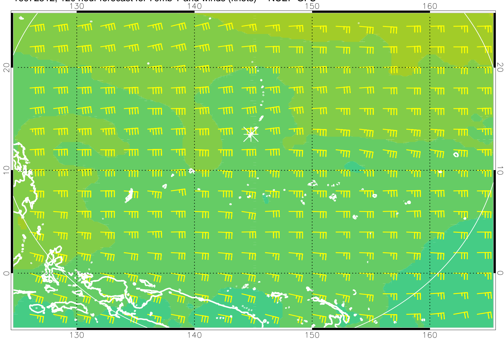
16072512, 120 hour forecast for 70mb T and winds (knots) -- NCEP GFS
