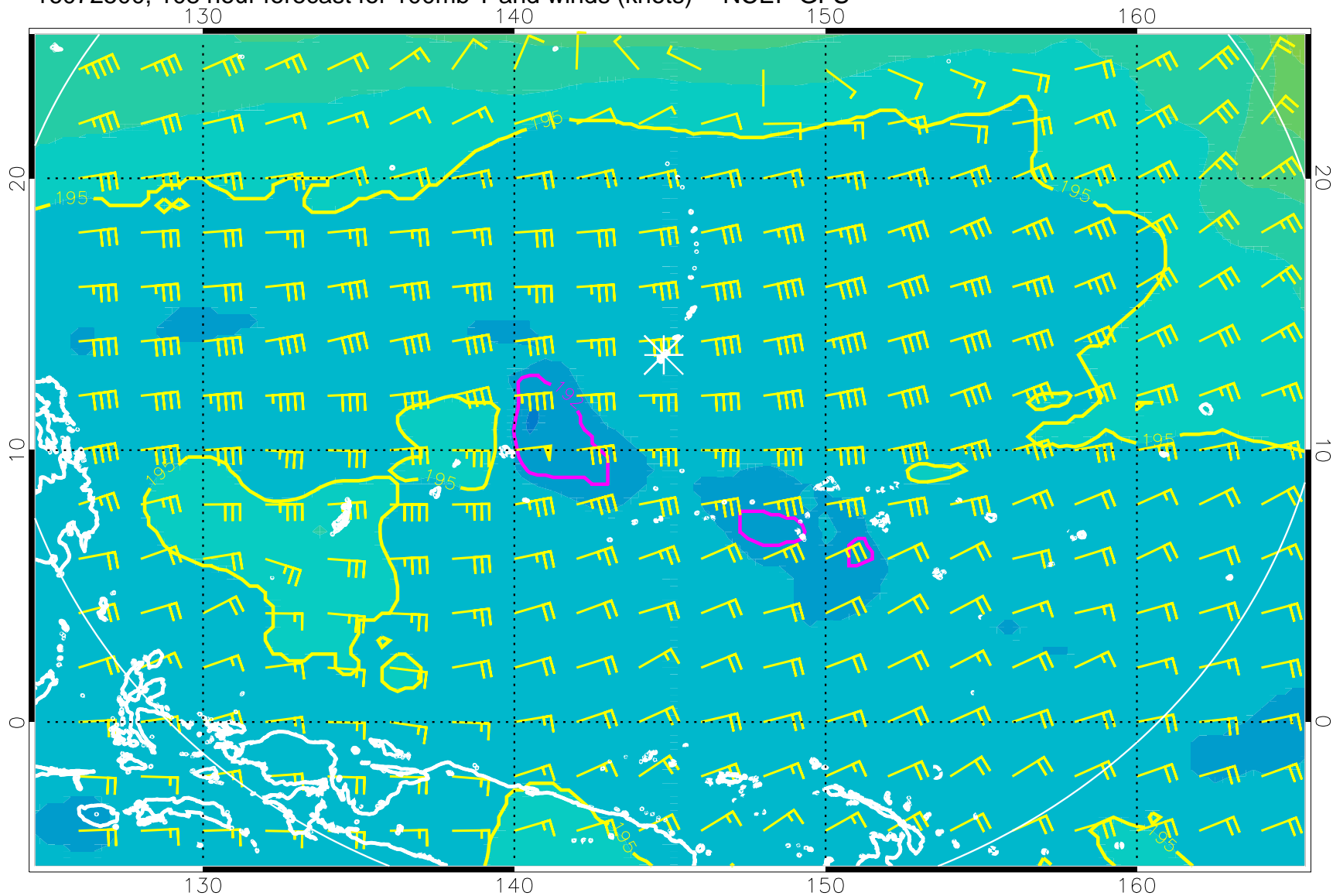
16072500, 108 hour forecast for 100mb T and winds (knots) -- NCEP GFS
