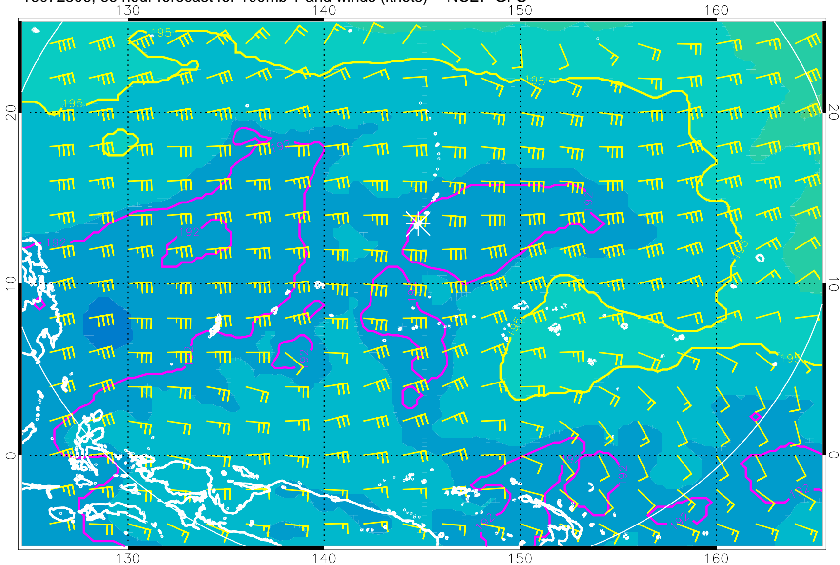
16072306, 66 hour forecast for 100mb T and winds (knots) -- NCEP GFS
