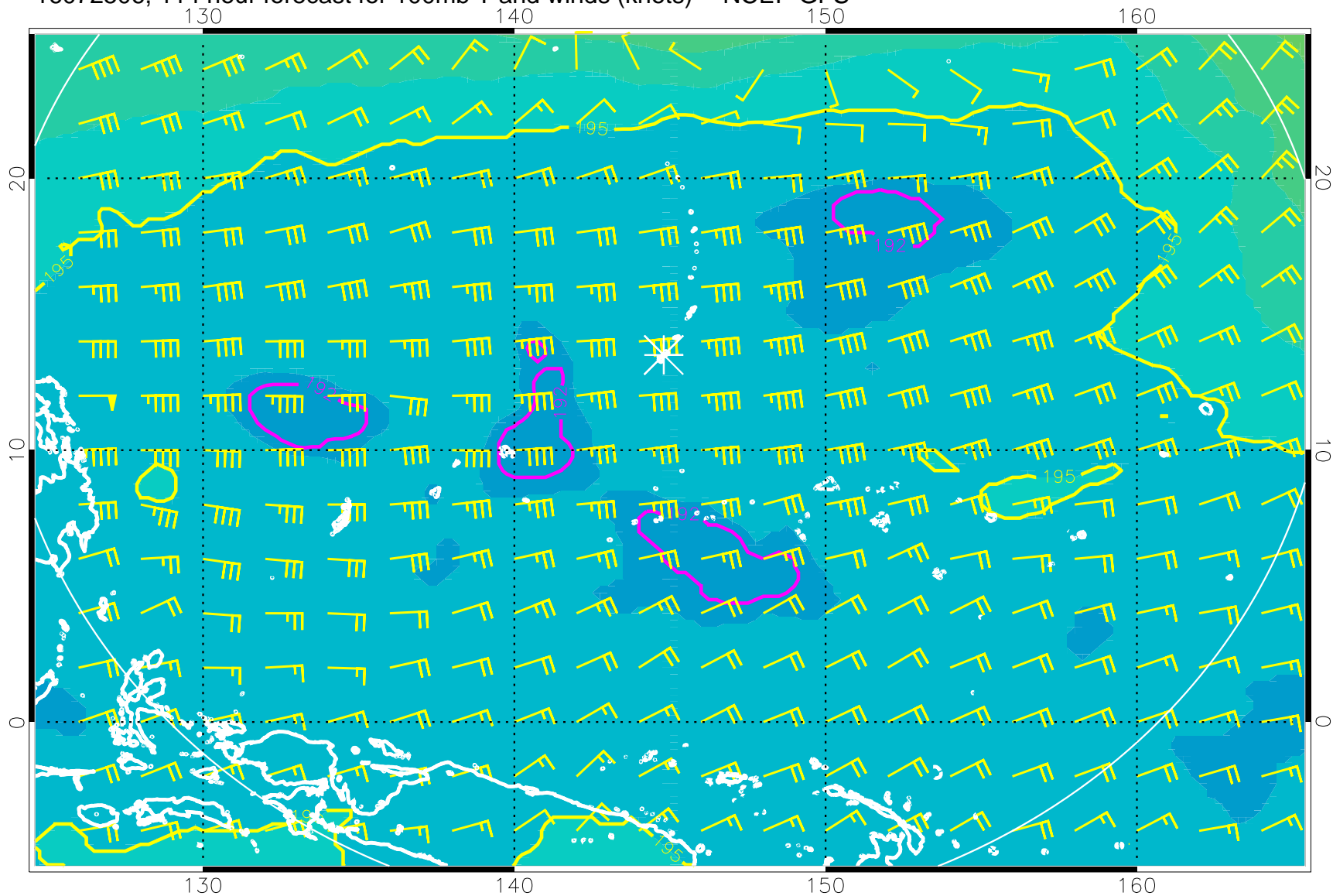
16072506, 114 hour forecast for 100mb T and winds (knots) -- NCEP GFS
