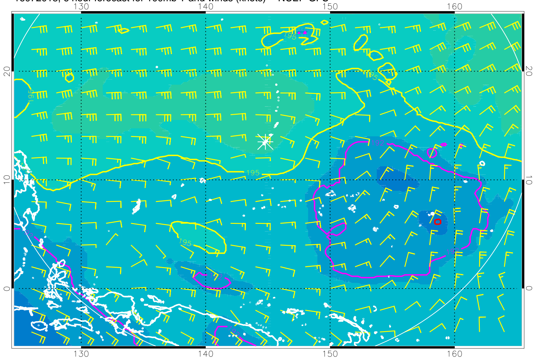
16072018, 6 hour forecast for 100mb T and winds (knots) -- NCEP GFS
