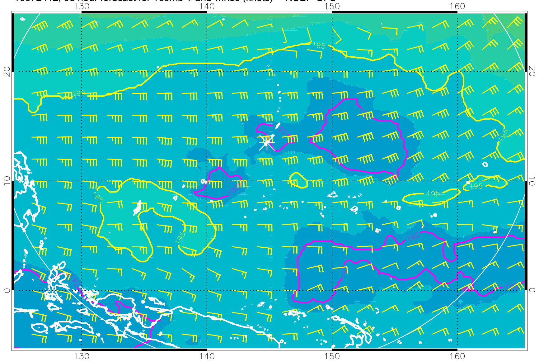
16072412, 96 hour forecast for 100mb T and winds (knots) -- NCEP GFS
