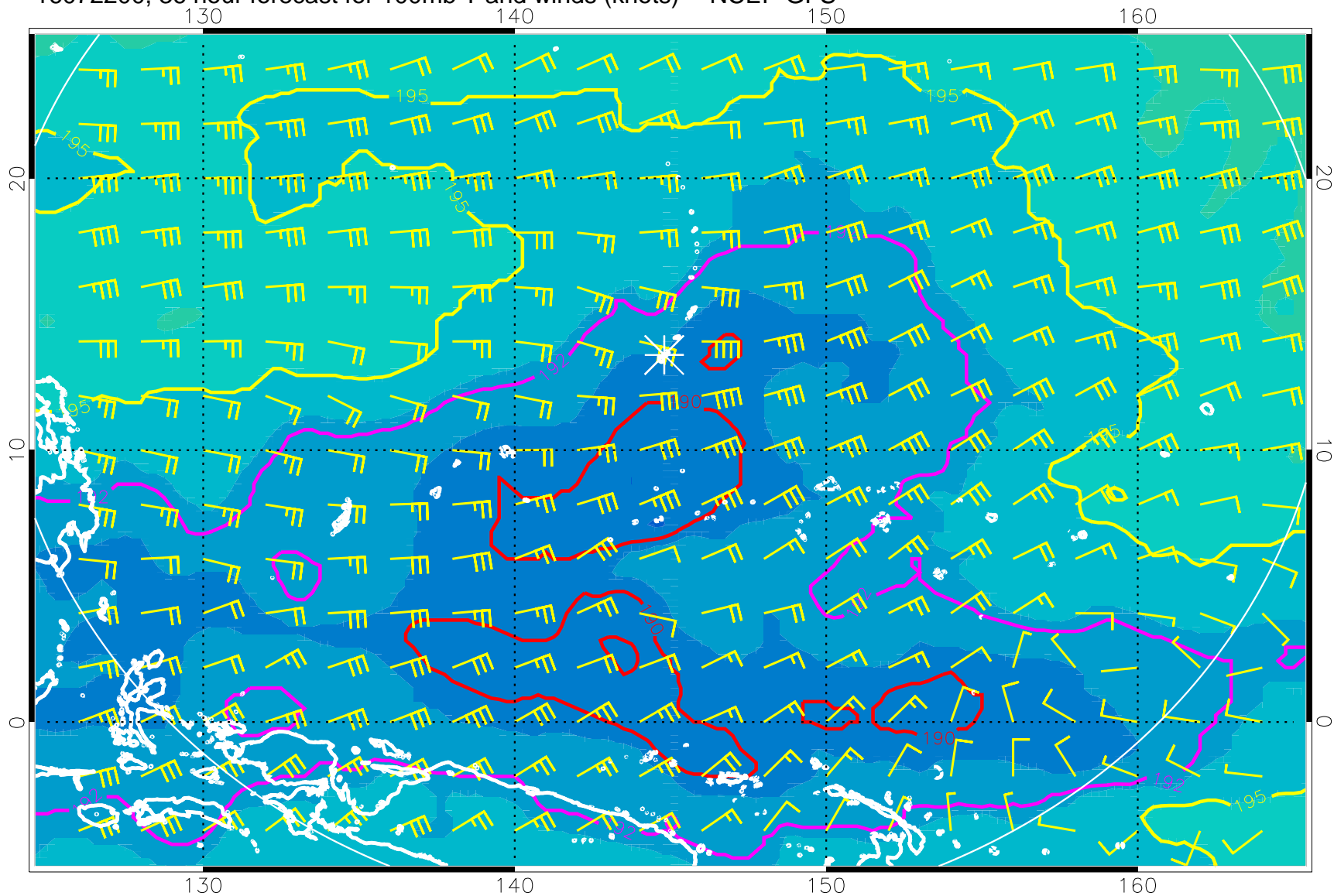
16072200, 36 hour forecast for 100mb T and winds (knots) -- NCEP GFS
