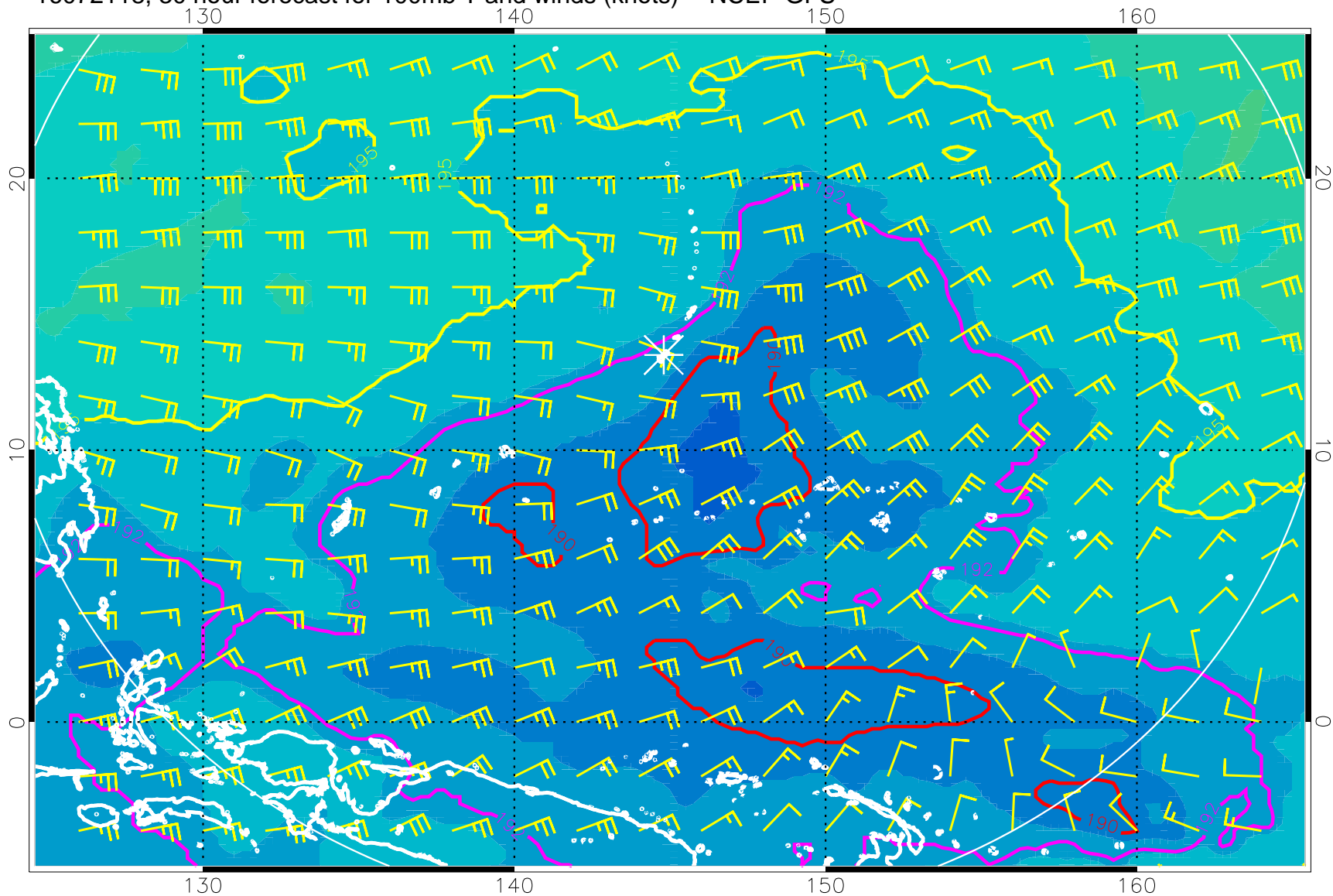
16072118, 30 hour forecast for 100mb T and winds (knots) -- NCEP GFS
