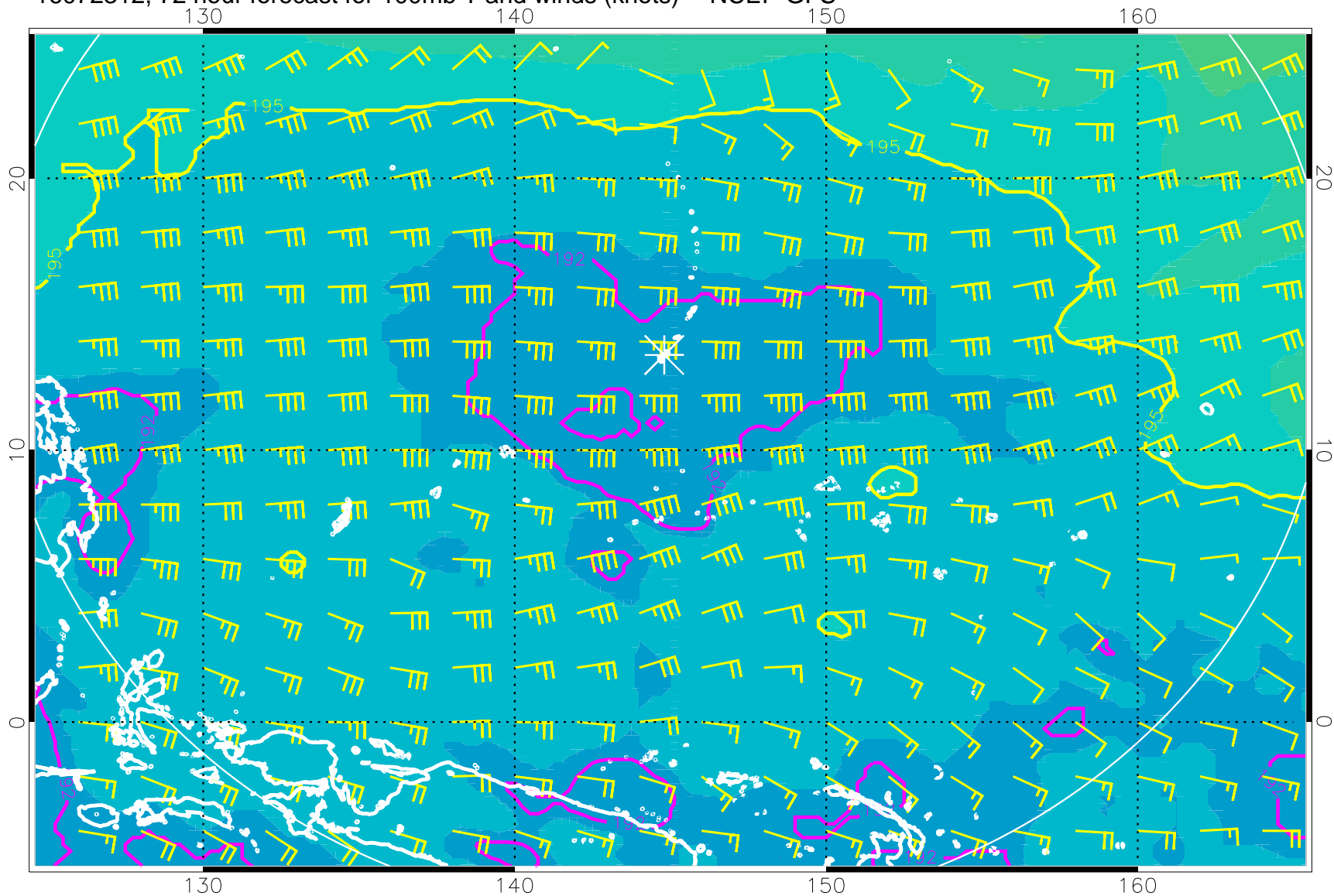
16072312, 72 hour forecast for 100mb T and winds (knots) -- NCEP GFS
