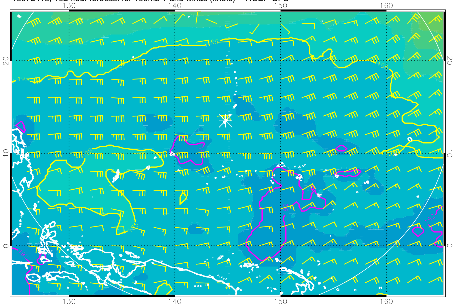
16072418, 102 hour forecast for 100mb T and winds (knots) -- NCEP GFS
