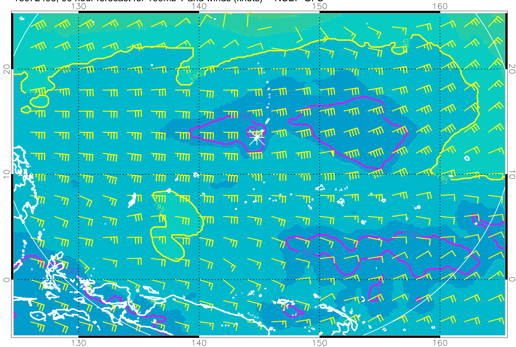
16072406, 90 hour forecast for 100mb T and winds (knots) -- NCEP GFS
