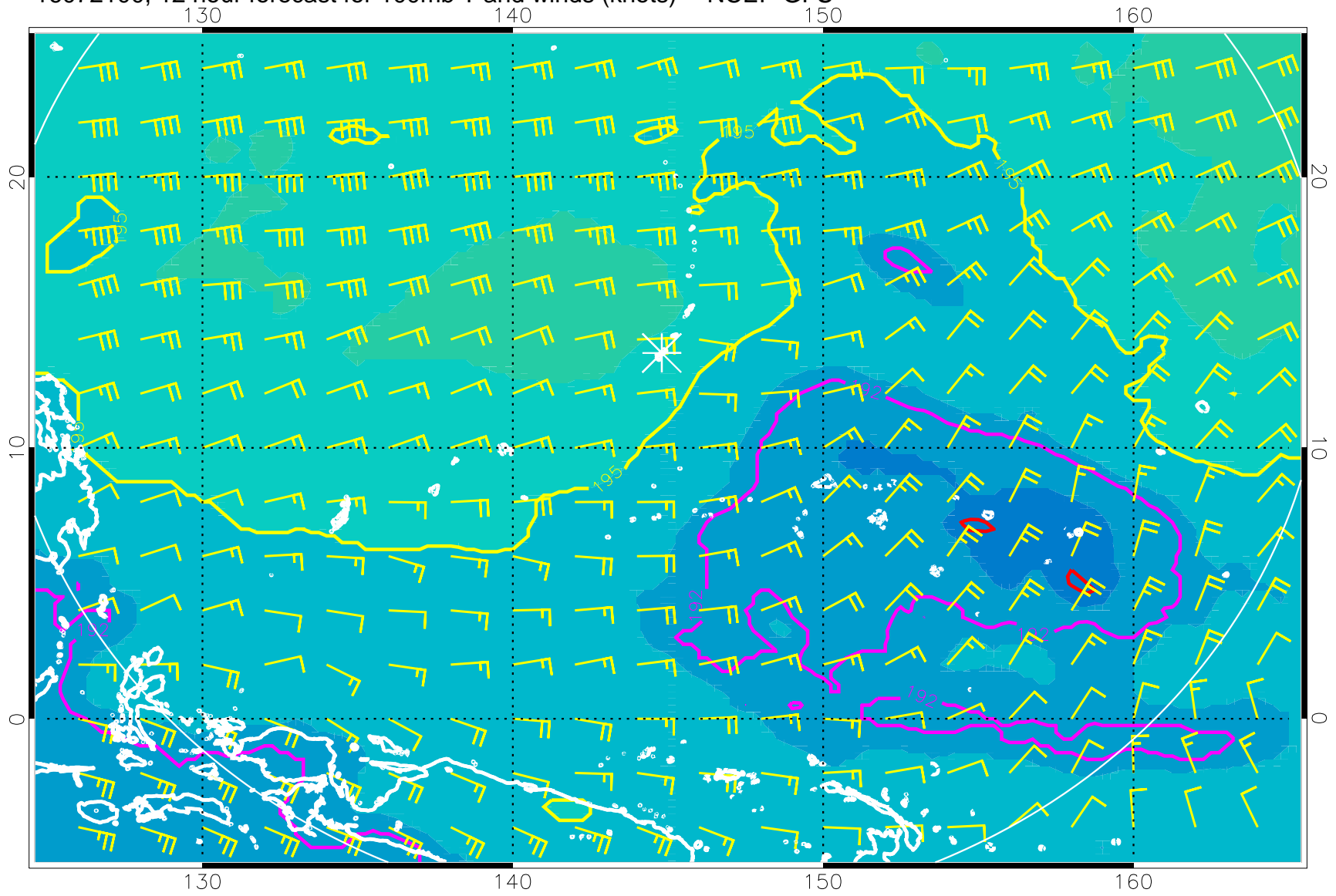
16072100, 12 hour forecast for 100mb T and winds (knots) -- NCEP GFS
