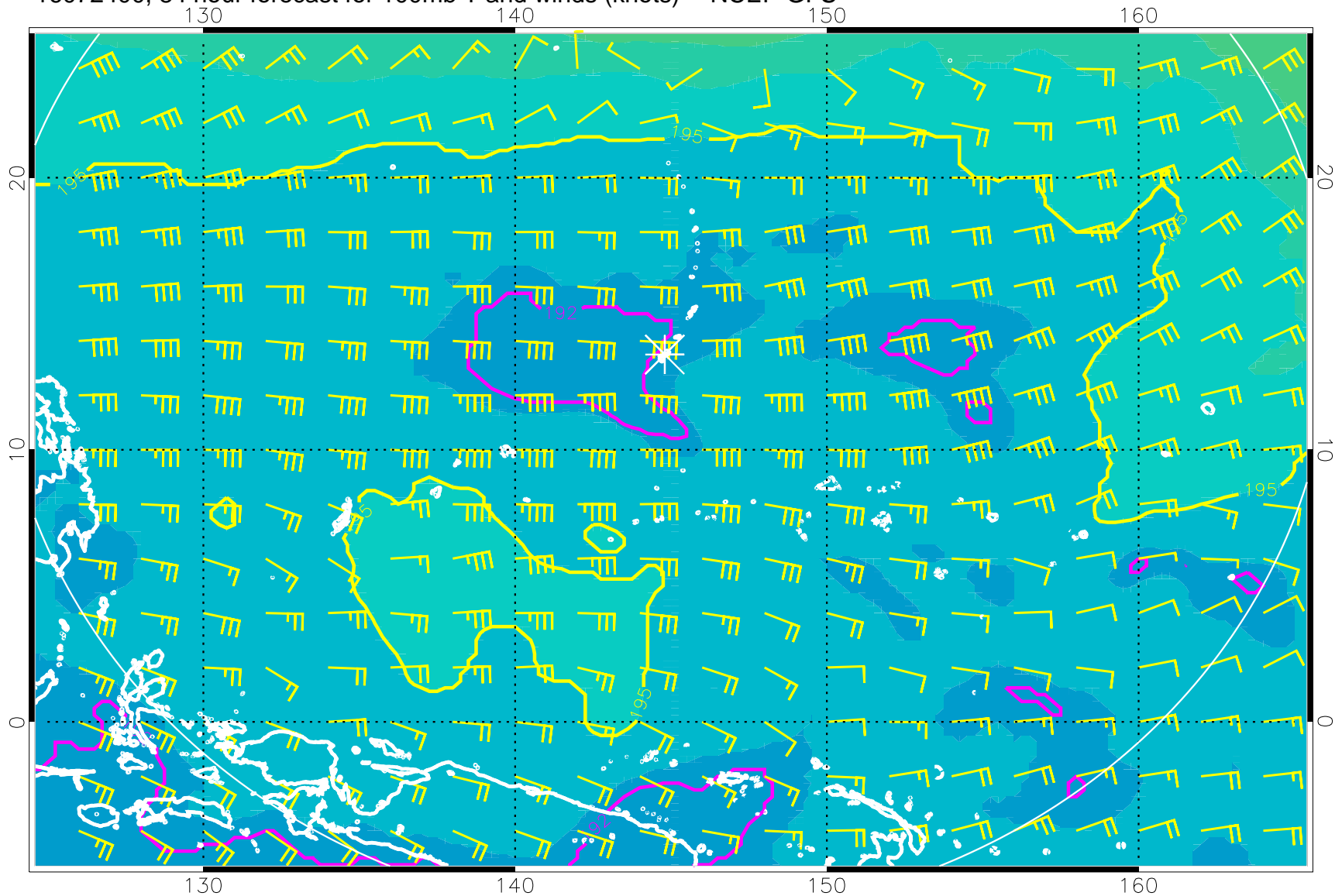
16072400, 84 hour forecast for 100mb T and winds (knots) -- NCEP GFS
