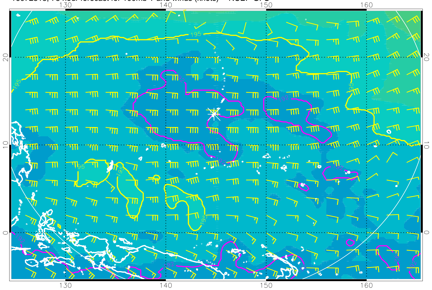
16072318, 78 hour forecast for 100mb T and winds (knots) -- NCEP GFS
