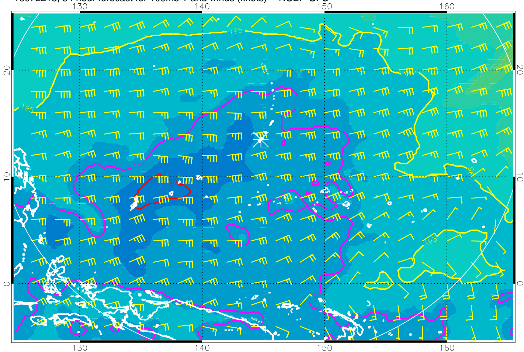
16072218, 54 hour forecast for 100mb T and winds (knots) -- NCEP GFS
