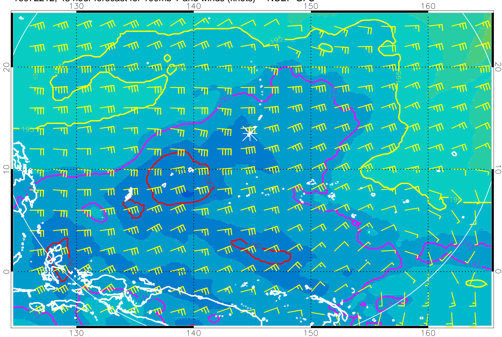
16072212, 48 hour forecast for 100mb T and winds (knots) -- NCEP GFS
