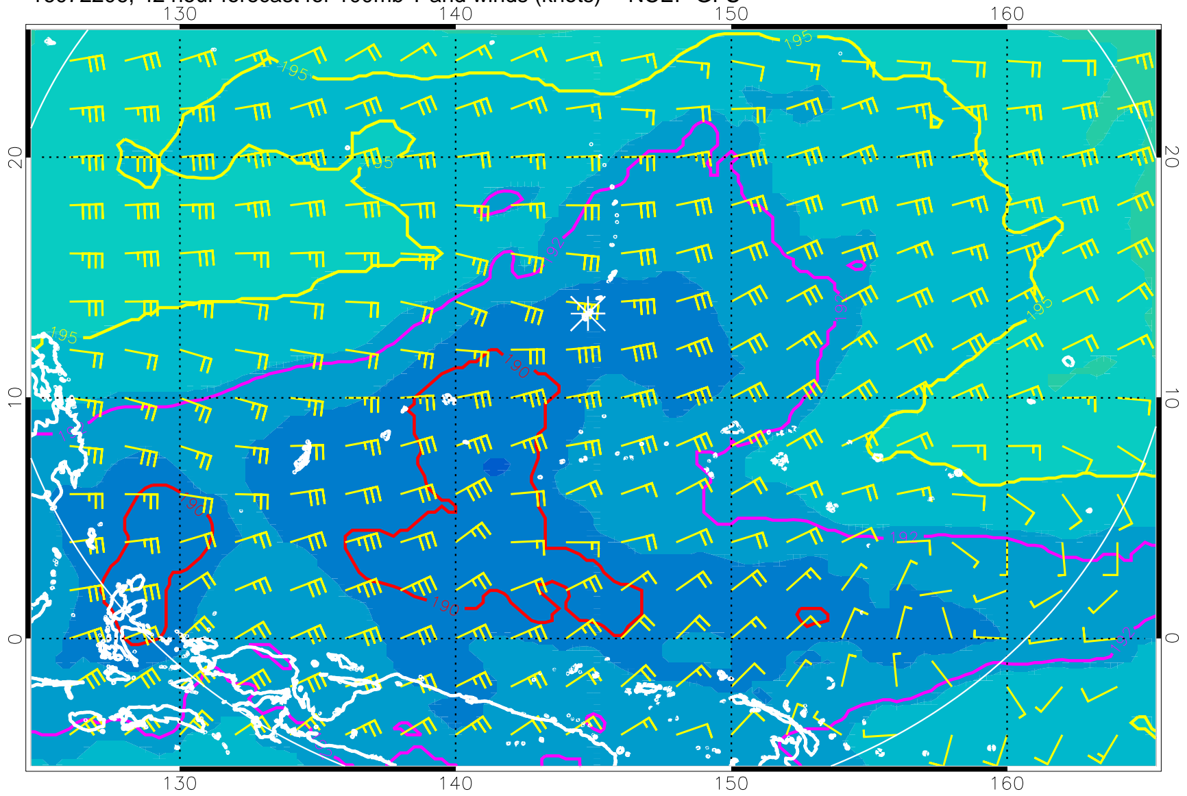
16072206, 42 hour forecast for 100mb T and winds (knots) -- NCEP GFS
