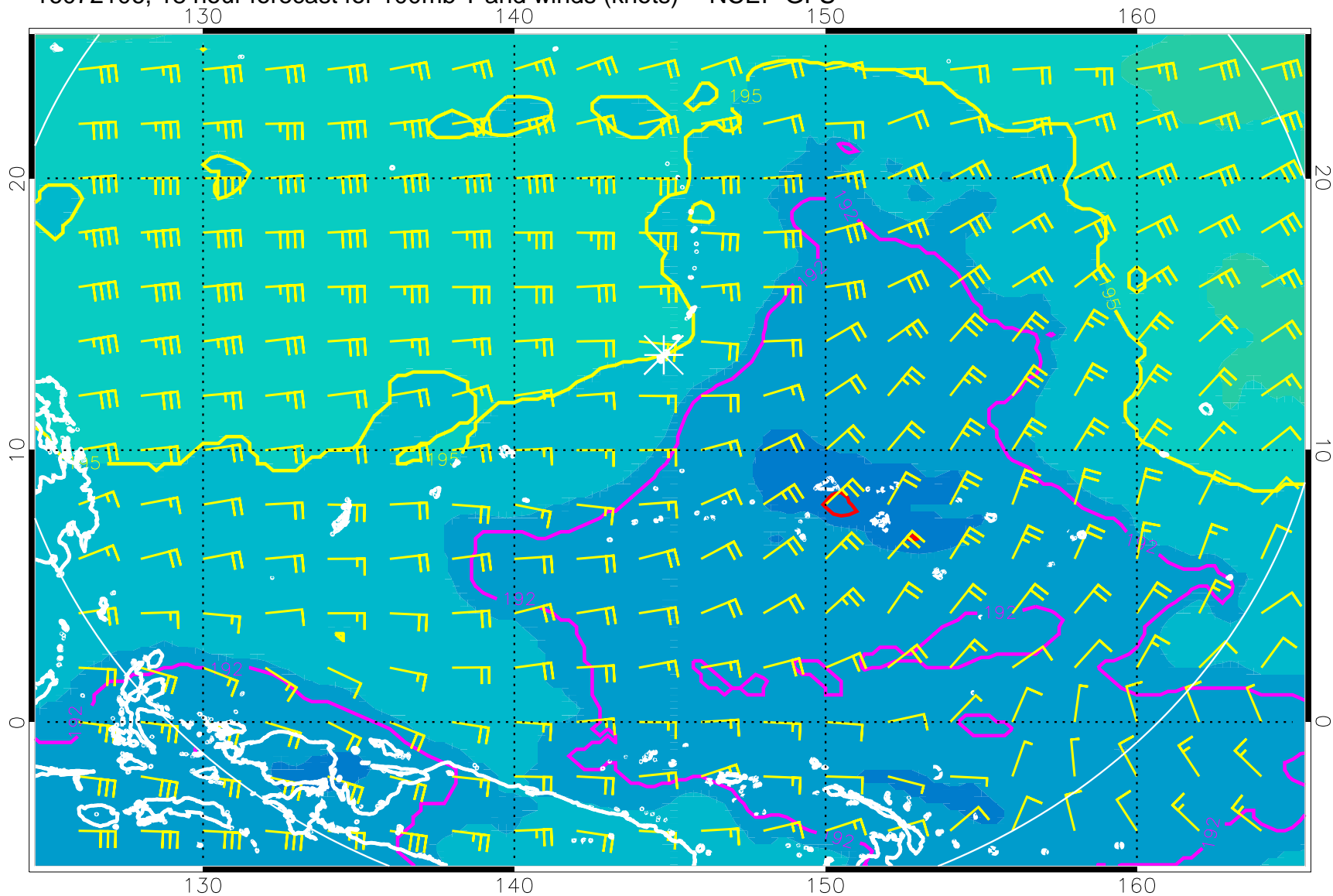
16072106, 18 hour forecast for 100mb T and winds (knots) -- NCEP GFS
