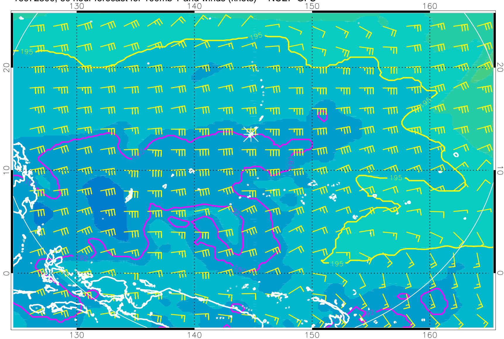
16072300, 60 hour forecast for 100mb T and winds (knots) -- NCEP GFS
