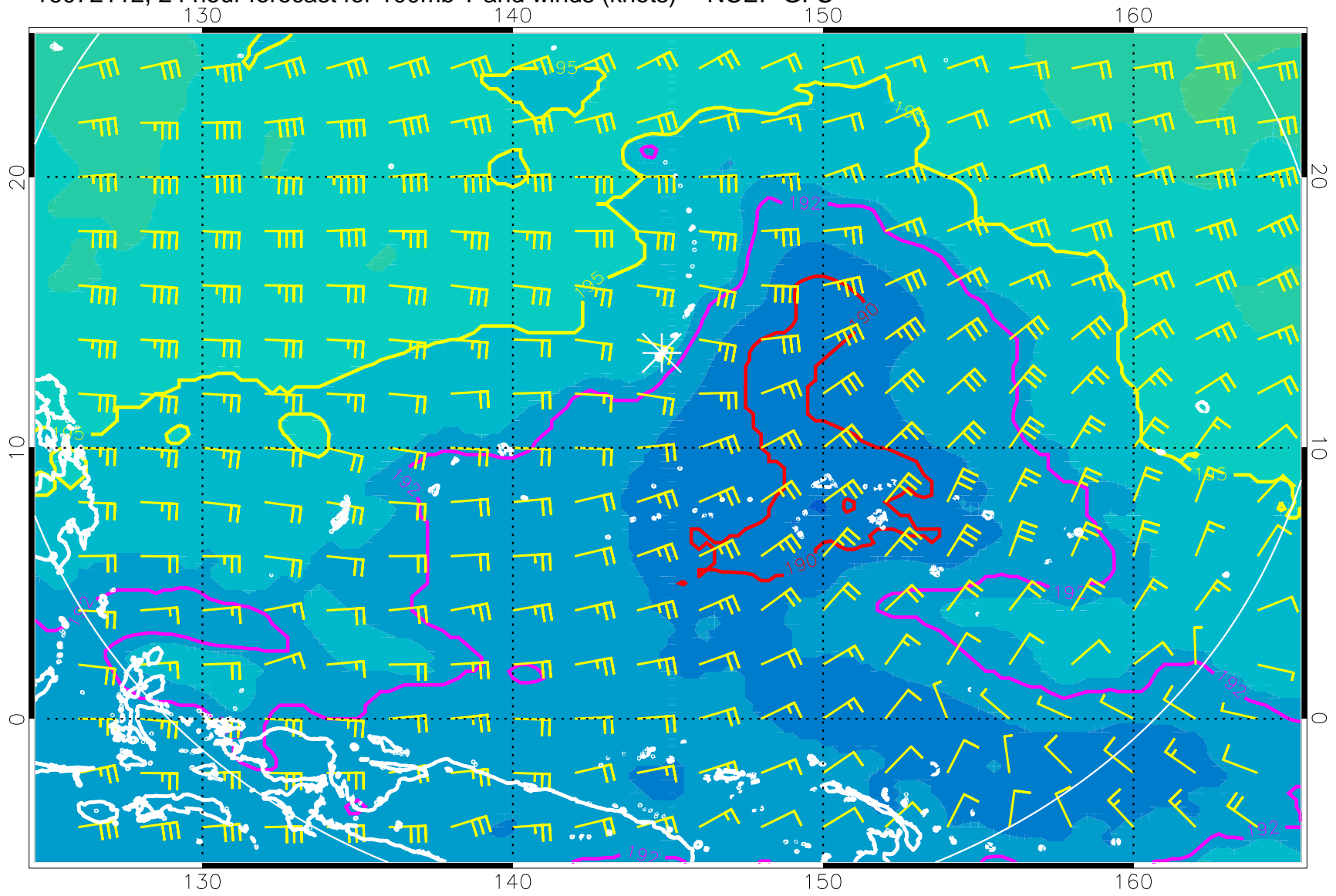
16072112, 24 hour forecast for 100mb T and winds (knots) -- NCEP GFS
