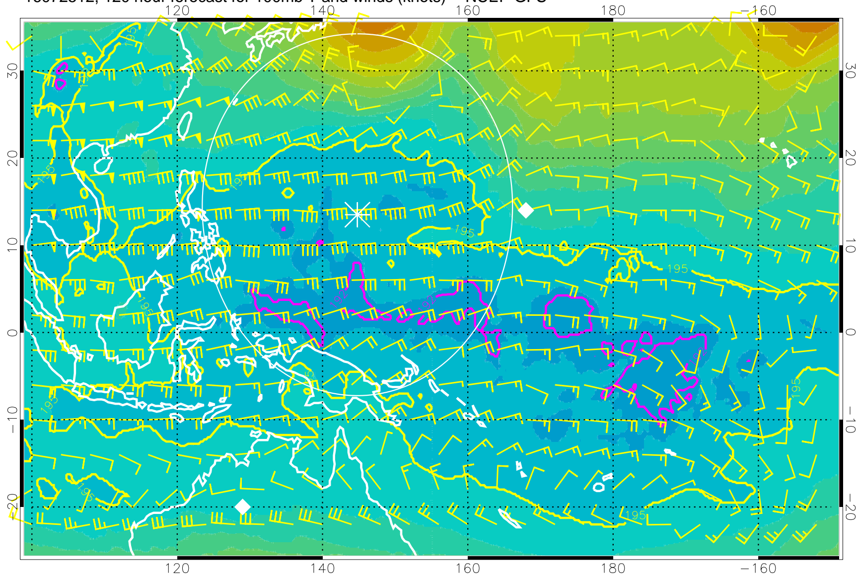
16072512, 120 hour forecast for 100mb T and winds (knots) -- NCEP GFS
