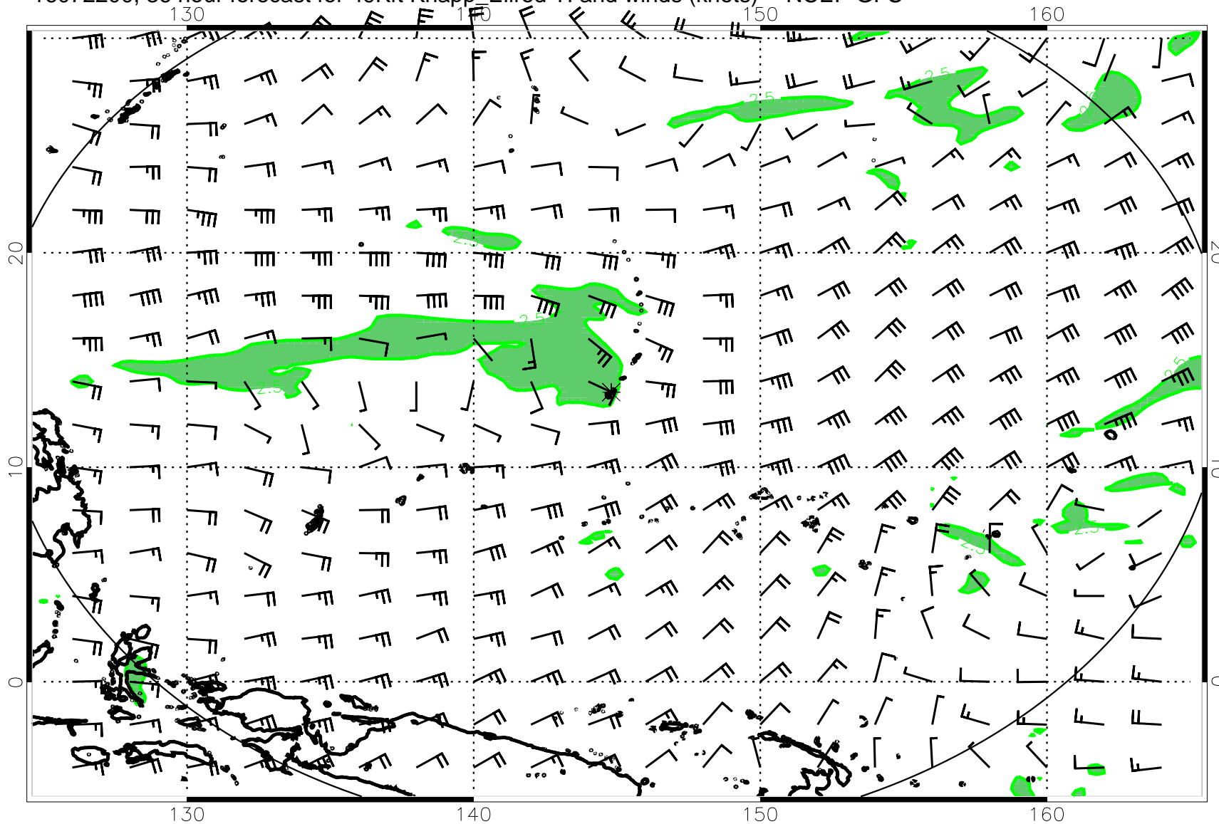
16072200, 36 hour forecast for 49Kft Knapp_Ellrod TI and winds (knots) -- NCEP GFS
