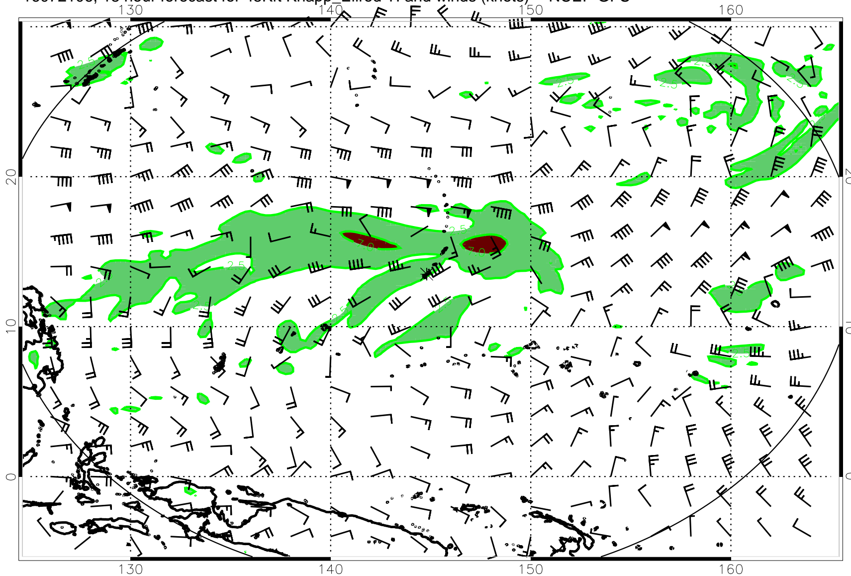
16072106, 18 hour forecast for 45Kft Knapp_Ellrod TI and winds (knots) -- NCEP GFS
