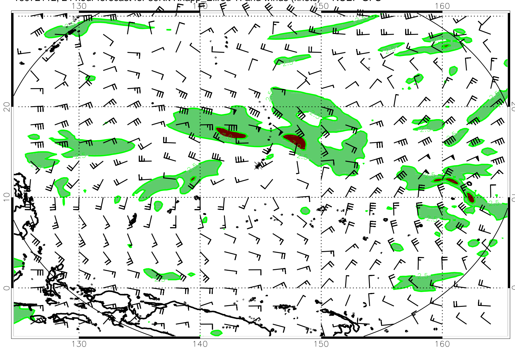
16072112, 24 hour forecast for 39Kft Knapp_Ellrod TI and winds (knots) -- NCEP GFS
