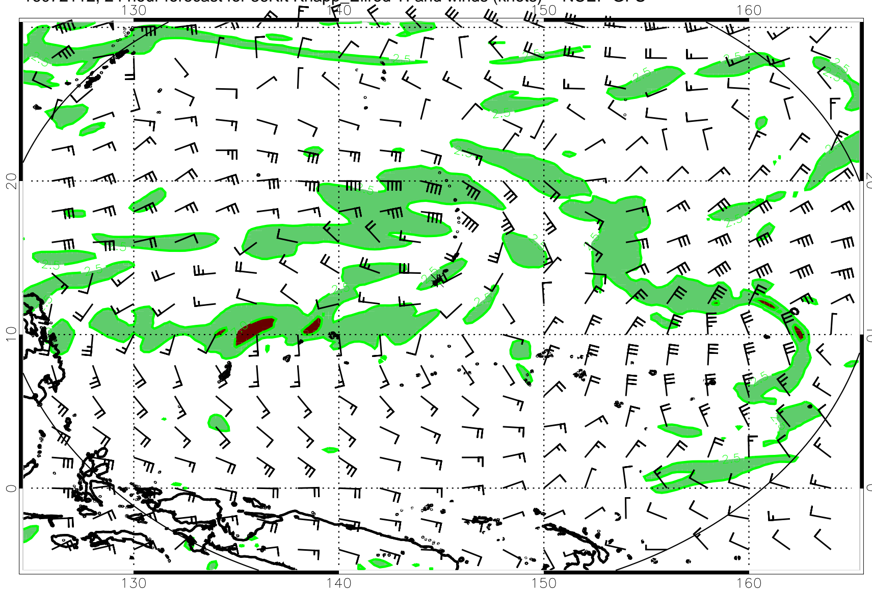
16072112, 24 hour forecast for 36Kft Knapp Ellrod TI and winds (knots) -- NCEP GFS
