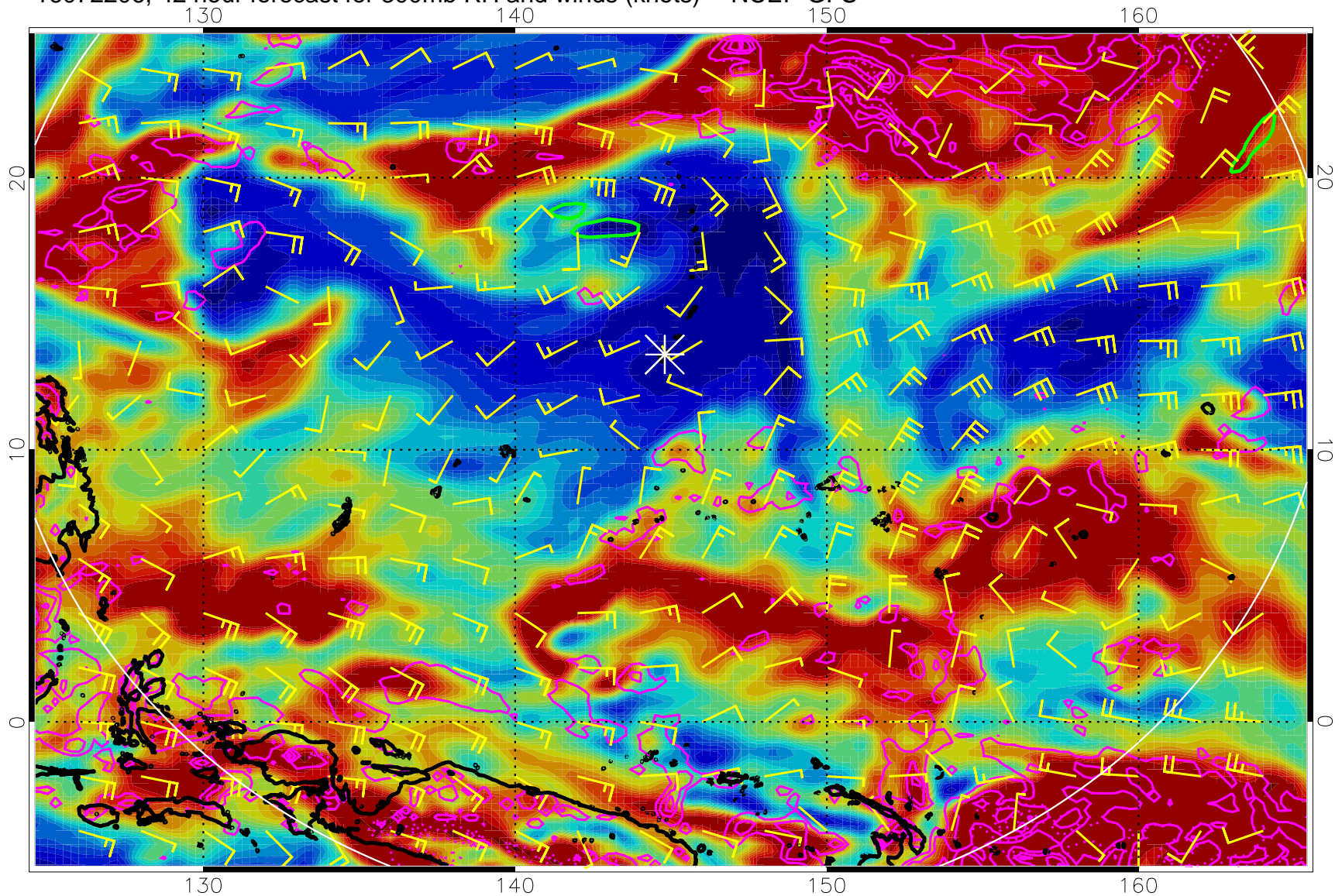
16072206, 42 hour forecast for 300mb RH and winds (knots) -- NCEP GFS
