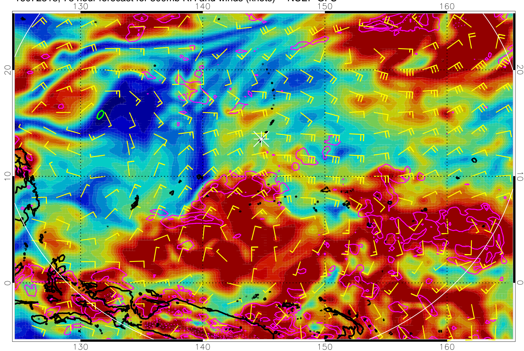
16072318, 78 hour forecast for 300mb RH and winds (knots) -- NCEP GFS
