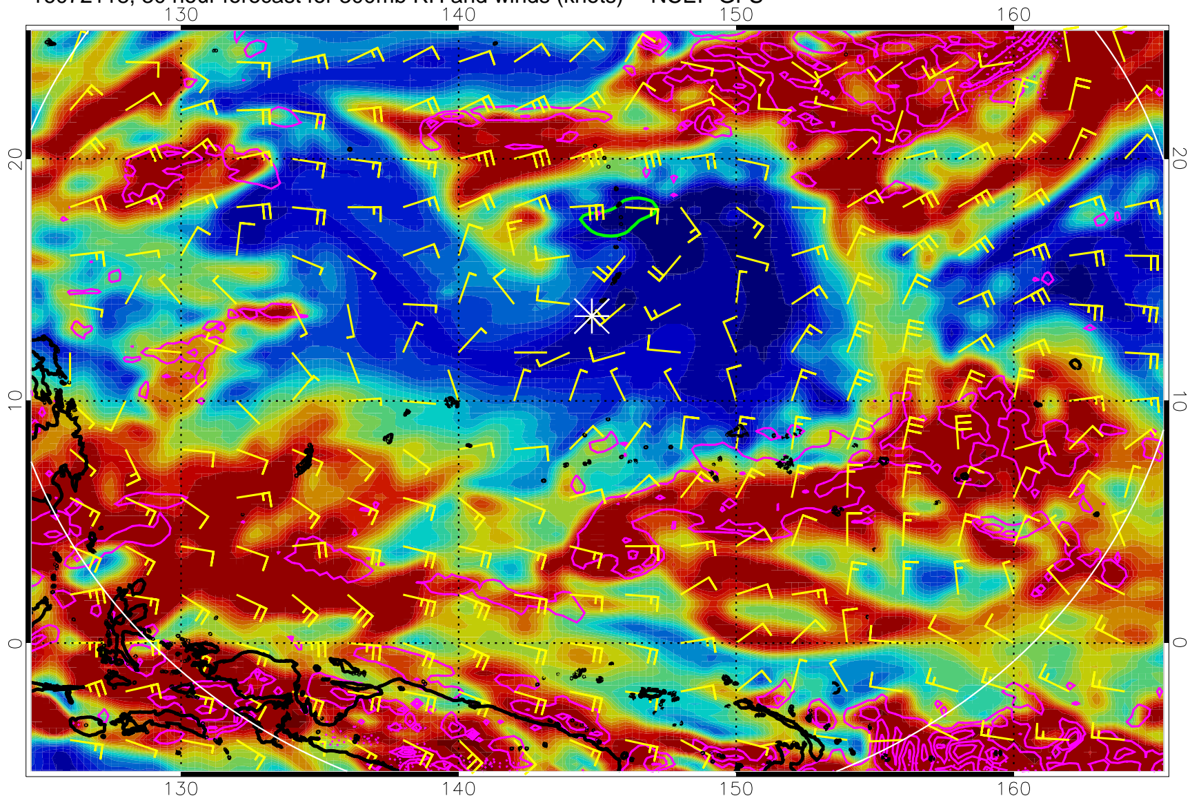
16072118, 30 hour forecast for 300mb RH and winds (knots) -- NCEP GFS
