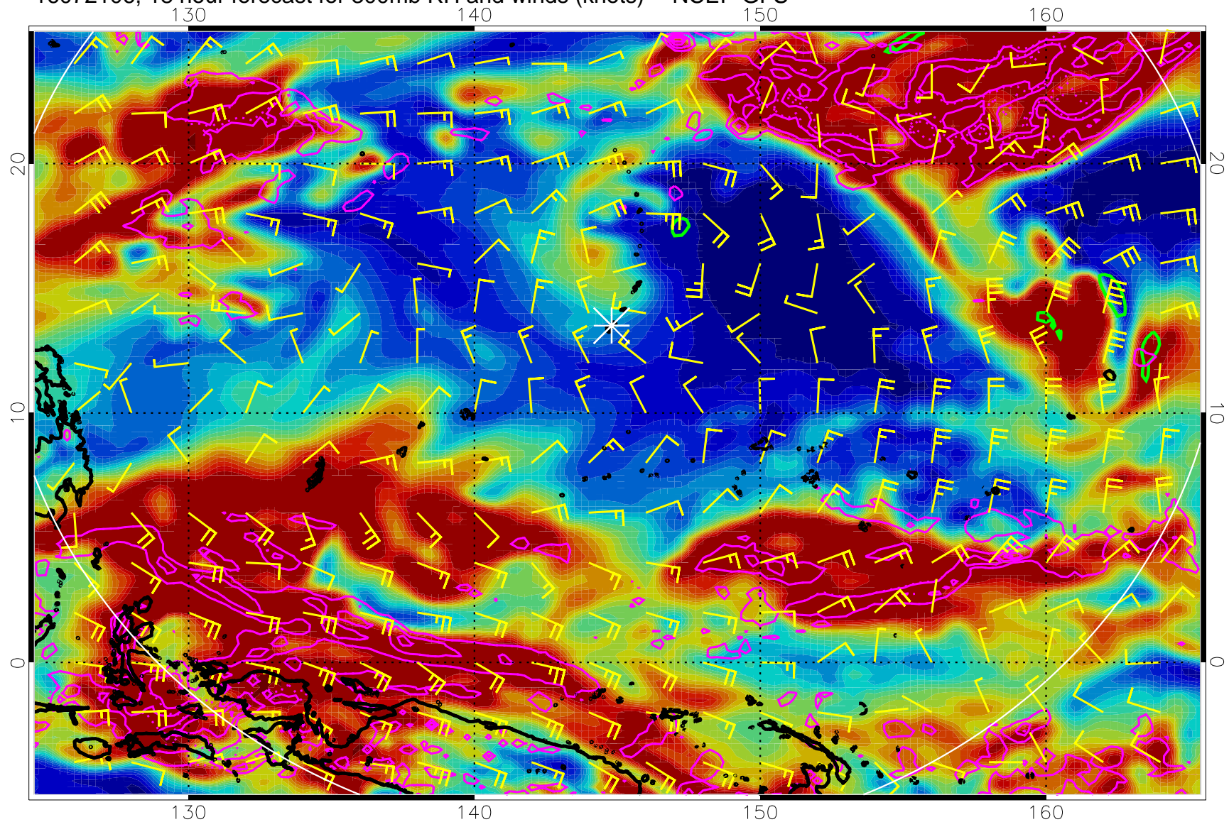
16072106, 18 hour forecast for 300mb RH and winds (knots) -- NCEP GFS
