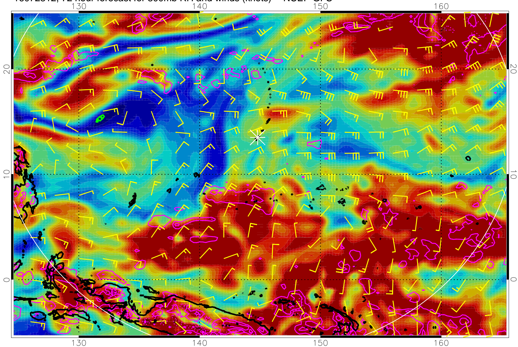
16072312, 72 hour forecast for 300mb RH and winds (knots) -- NCEP GFS
