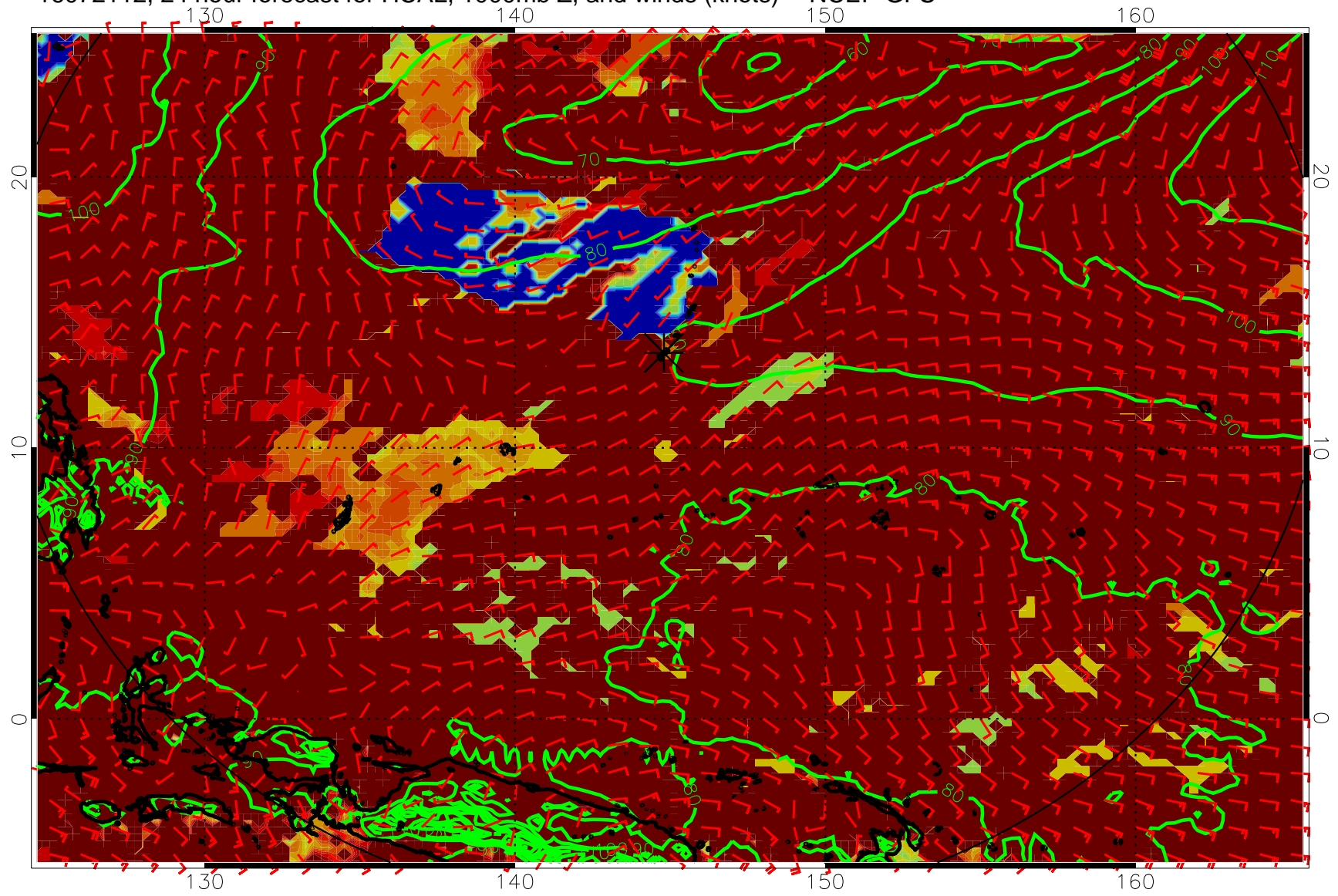
16072112, 24 hour forecast for HCAL, 1000mb Z, and winds (knots) -- NCEP GFS
