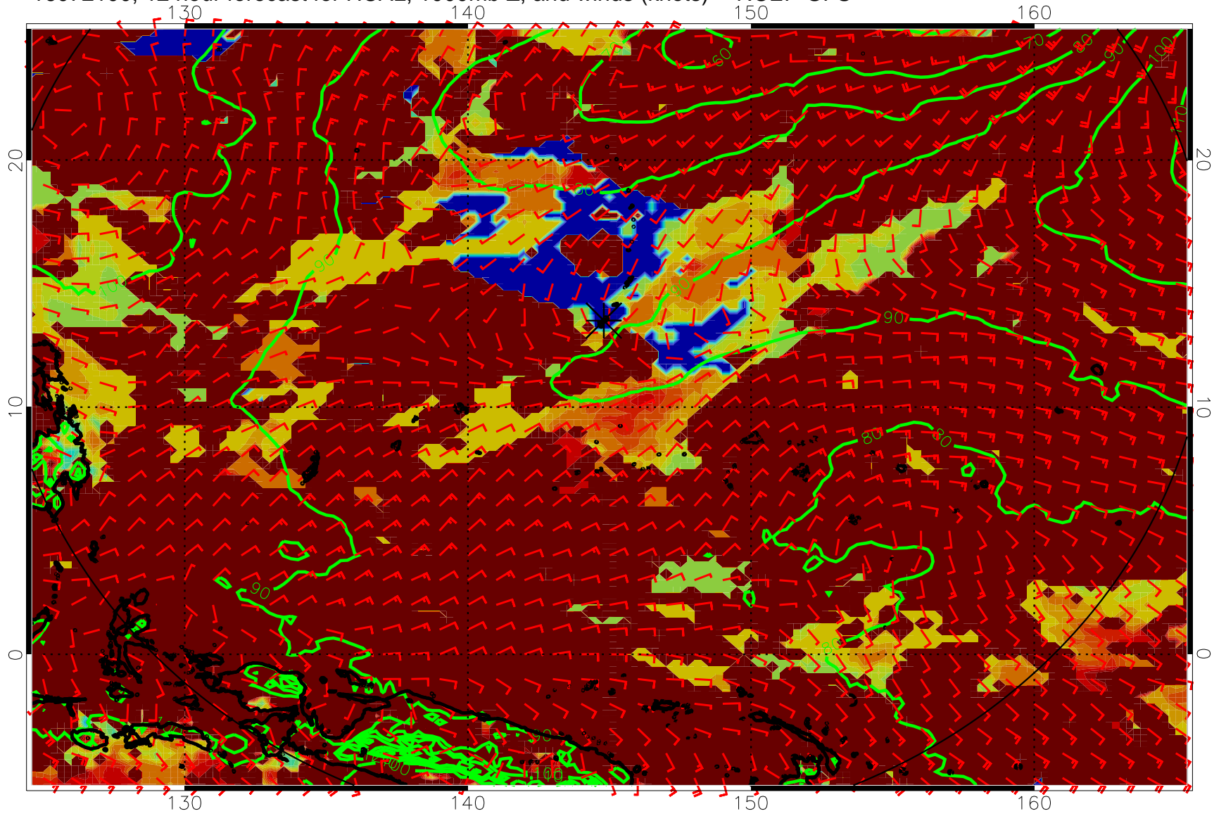
16072100, 12 hour forecast for HCAL, 1000mb Z, and winds (knots) -- NCEP GFS
