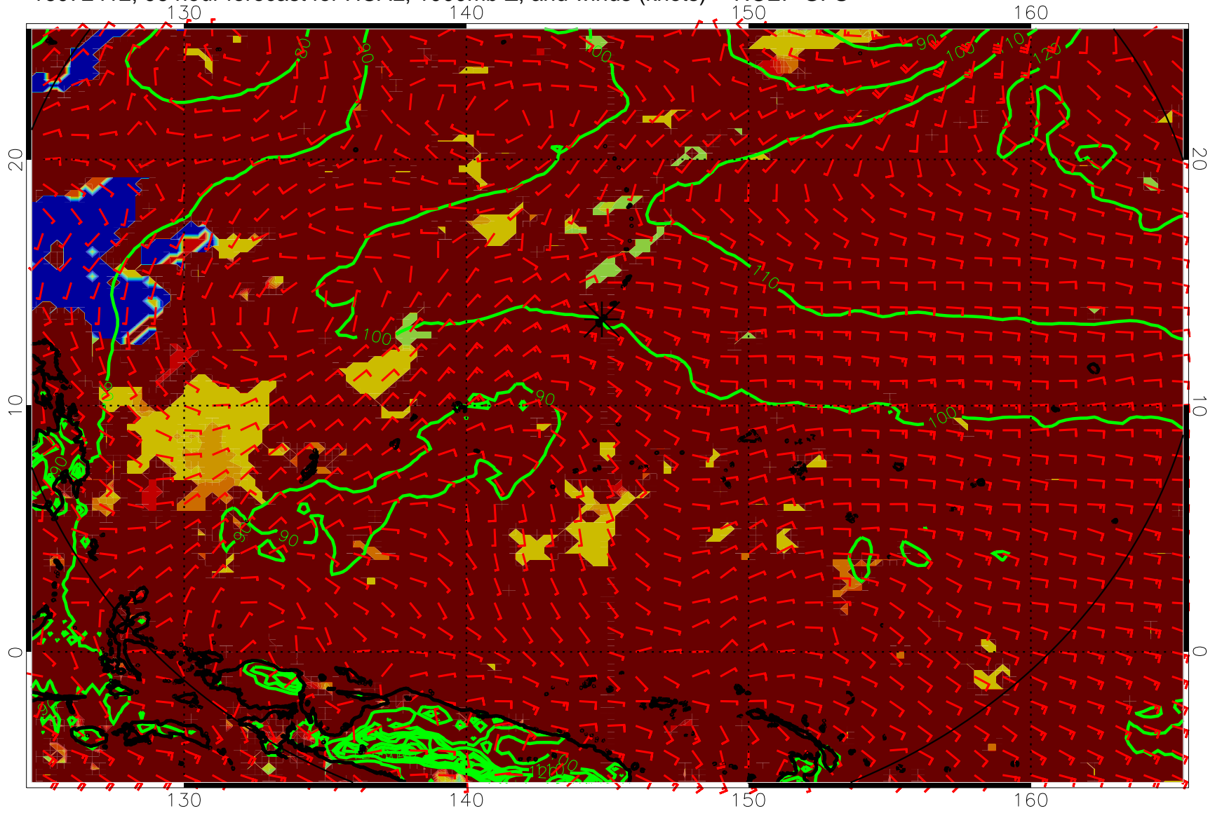
16072412, 96 hour forecast for HCAL, 1000mb Z, and winds (knots) -- NCEP GFS
