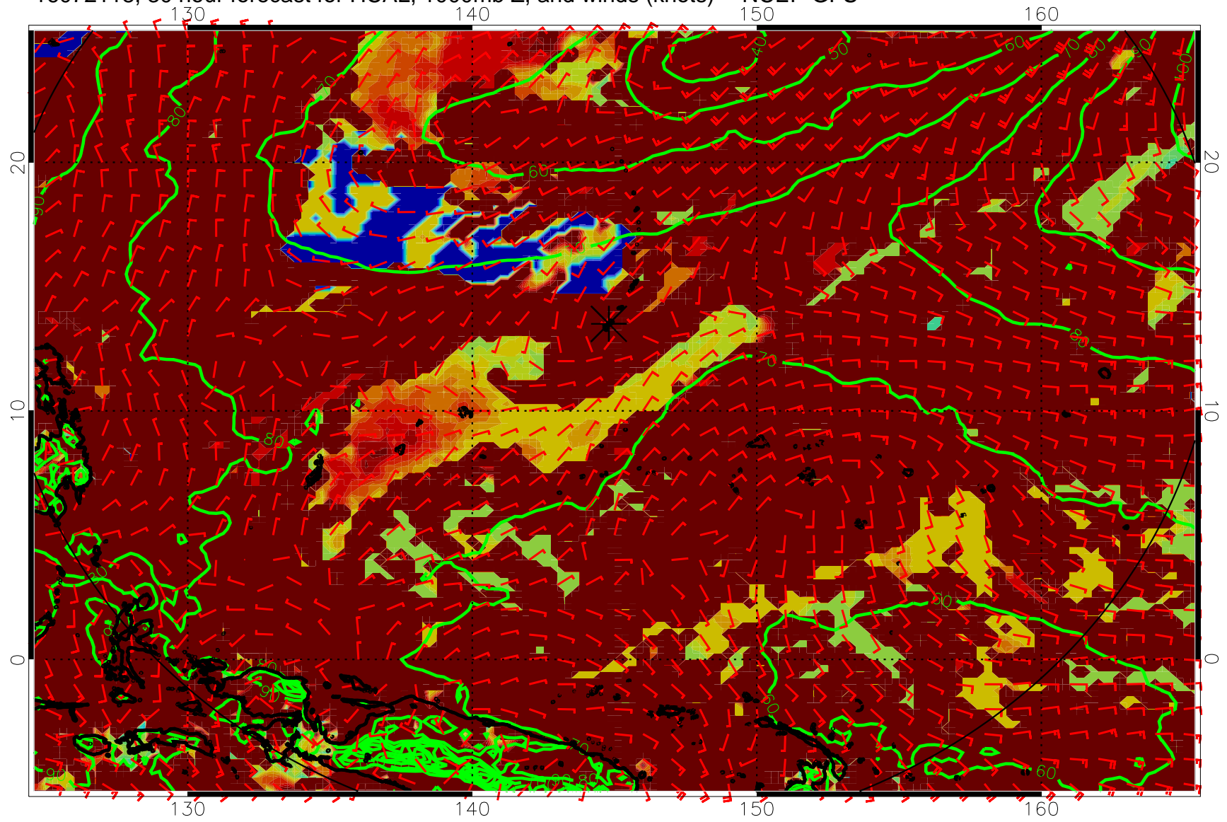
16072118, 30 hour forecast for HCAL, 1000mb Z, and winds (knots) -- NCEP GFS
