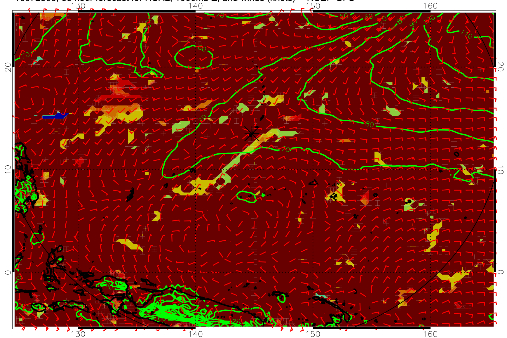
16072306, 66 hour forecast for HCAL, 1000mb Z, and winds (knots) -- NCEP GFS
