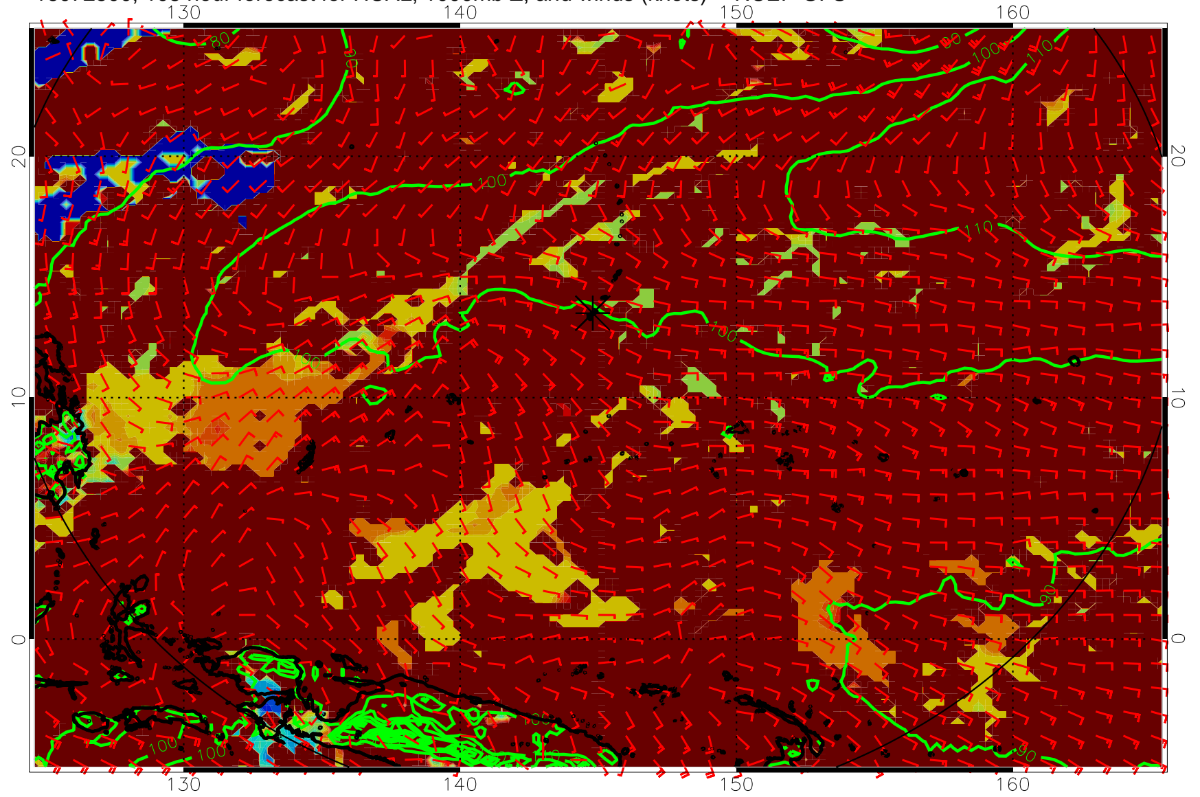
16072500, 108 hour forecast for HCAL, 1000mb Z, and winds (knots) -- NCEP GFS
