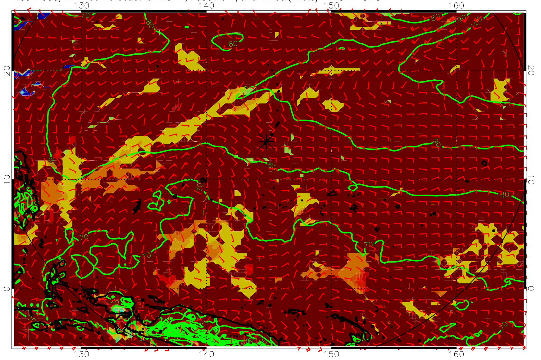
16072506, 114 hour forecast for HCAL, 1000mb Z, and winds (knots) -- NCEP GFS
