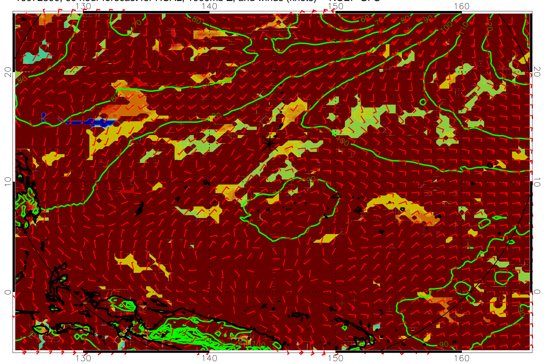
16072300, 60 hour forecast for HCAL, 1000mb Z, and winds (knots) -- NCEP GFS
