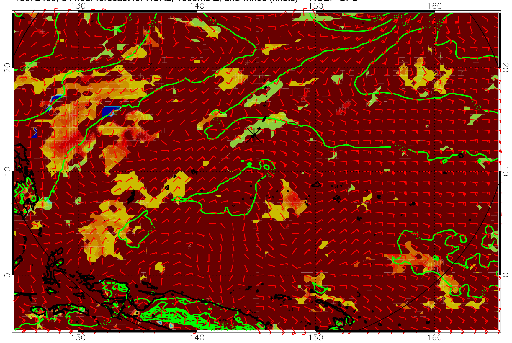
16072400, 84 hour forecast for HCAL, 1000mb Z, and winds (knots) -- NCEP GFS
