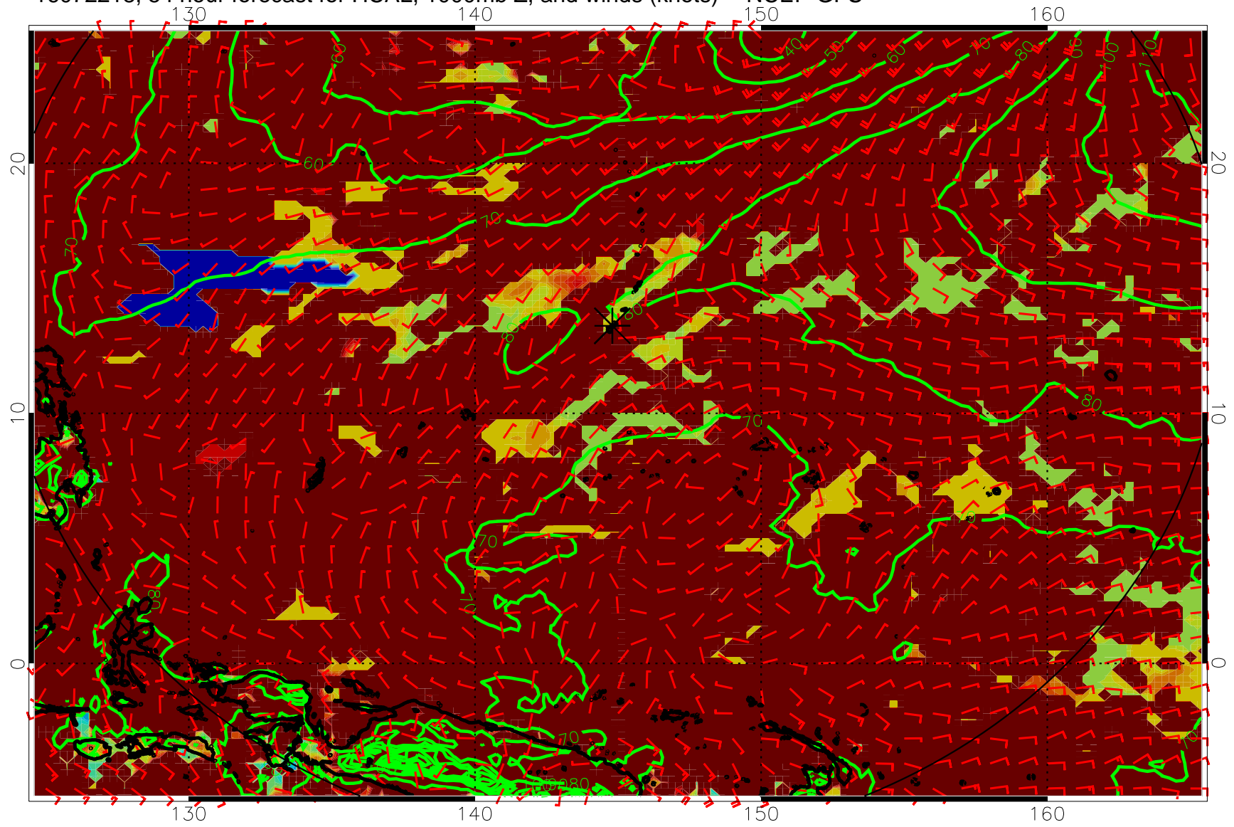
16072218, 54 hour forecast for HCAL, 1000mb Z, and winds (knots) -- NCEP GFS
