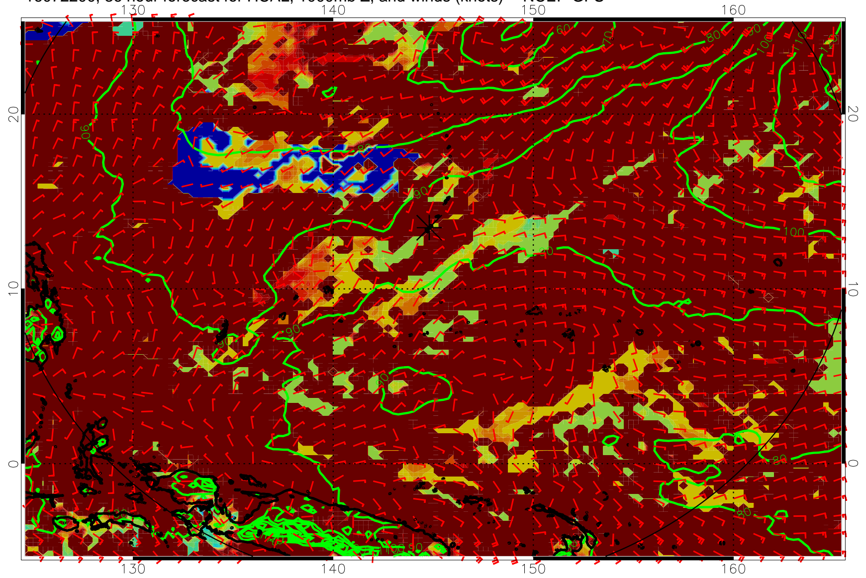
16072200, 36 hour forecast for HCAL, 1000mb Z, and winds (knots) -- NCEP GFS
