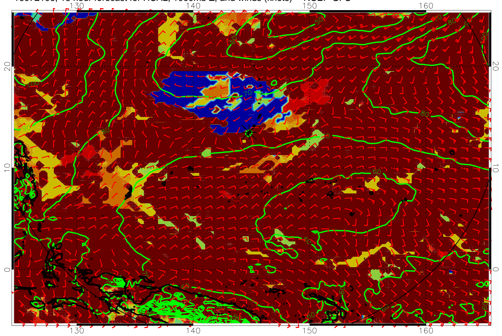
16072106, 18 hour forecast for HCAL, 1000mb Z, and winds (knots) -- NCEP GFS
