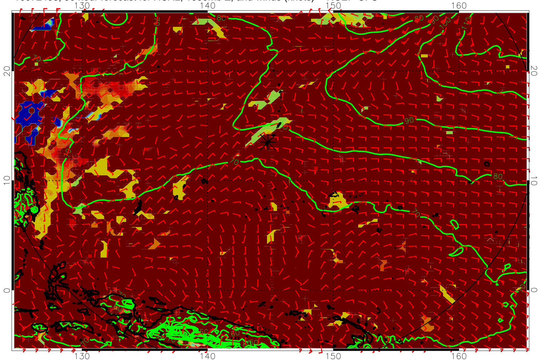
16072406, 90 hour forecast for HCAL, 1000mb Z, and winds (knots) -- NCEP GFS
