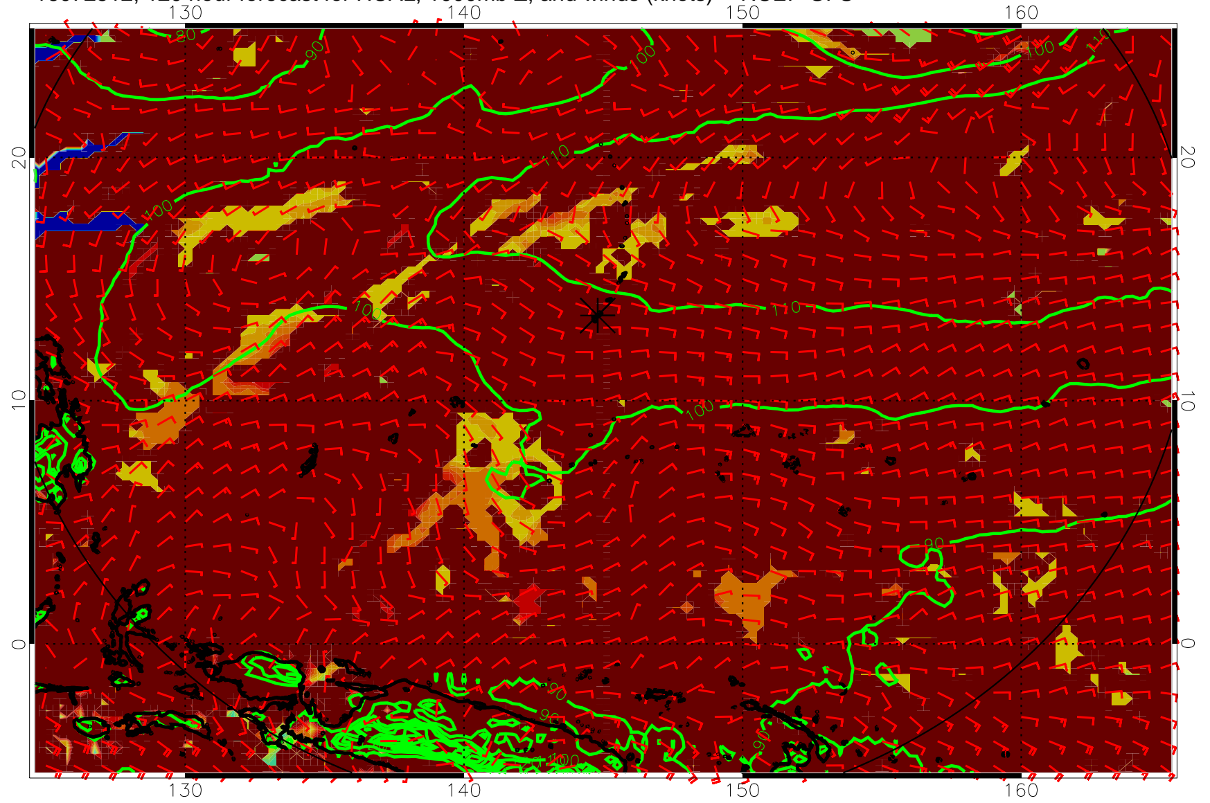
16072512, 120 hour forecast for HCAL, 1000mb Z, and winds (knots) -- NCEP GFS
