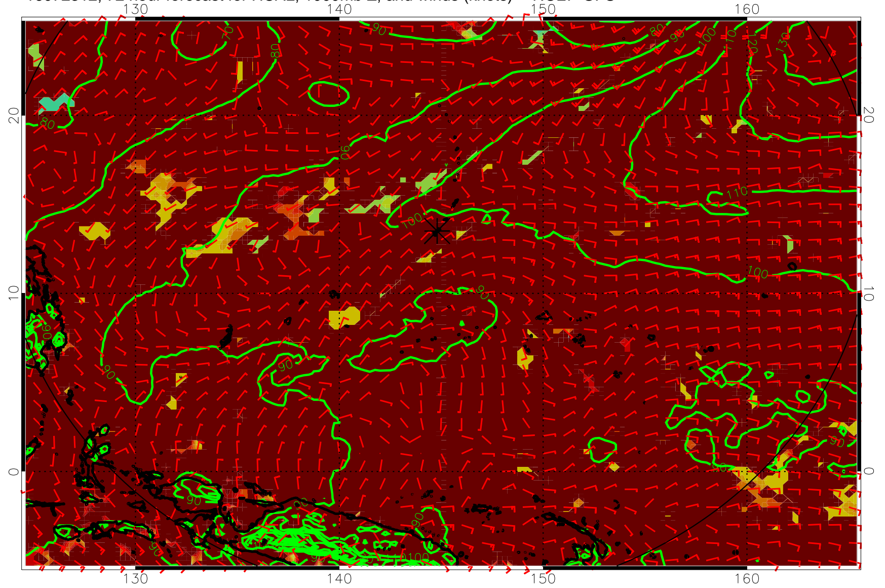
16072312, 72 hour forecast for HCAL, 1000mb Z, and winds (knots) -- NCEP GFS
