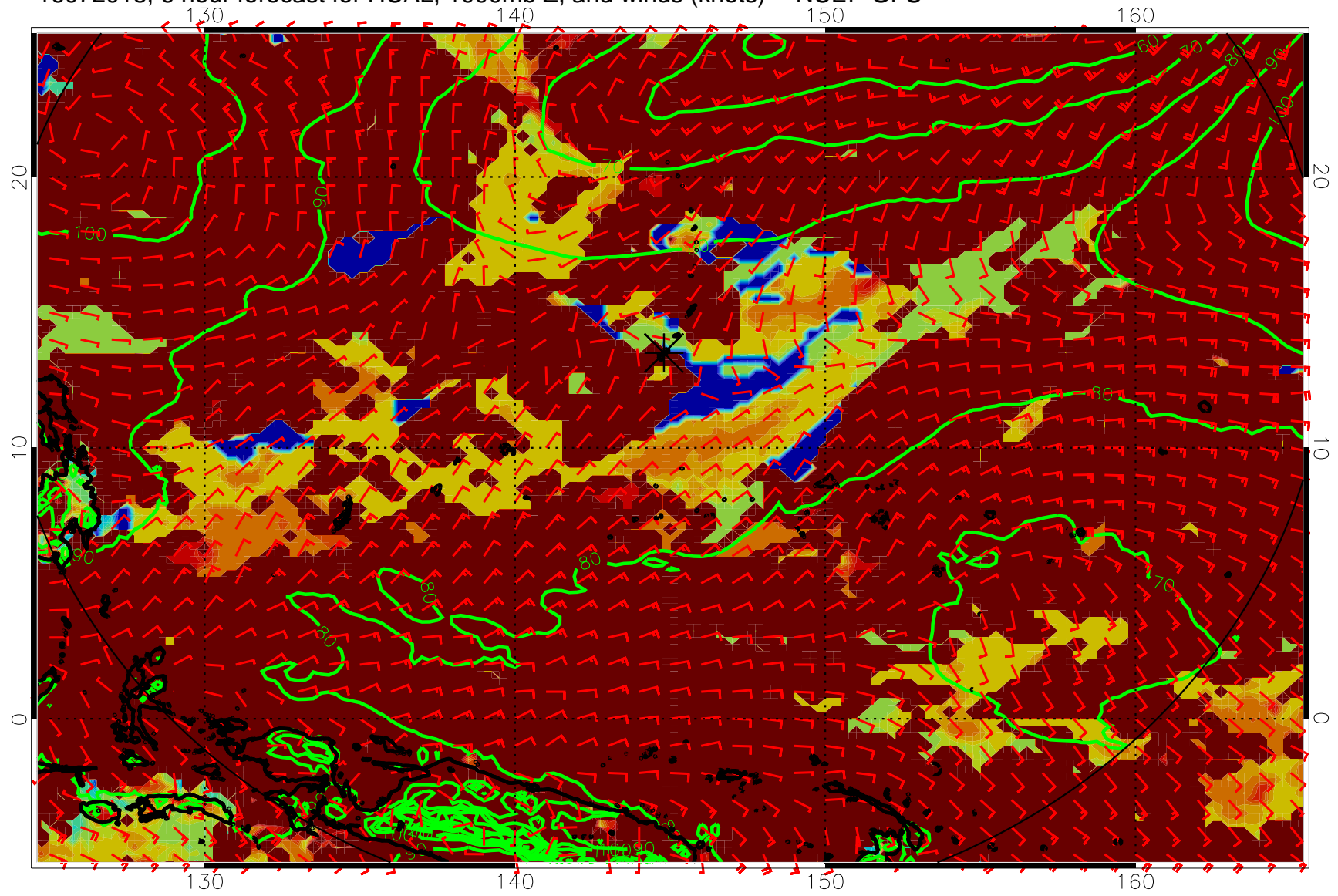
16072018, 6 hour forecast for HCAL, 1000mb Z, and winds (knots) -- NCEP GFS
