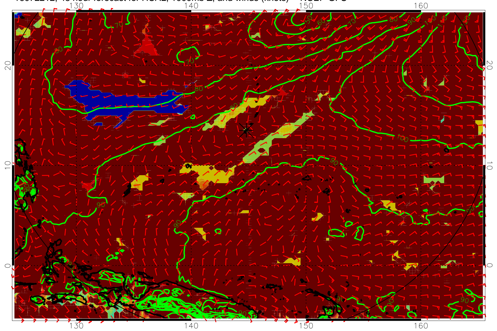
16072212, 48 hour forecast for HCAL, 1000mb Z, and winds (knots) -- NCEP GFS
