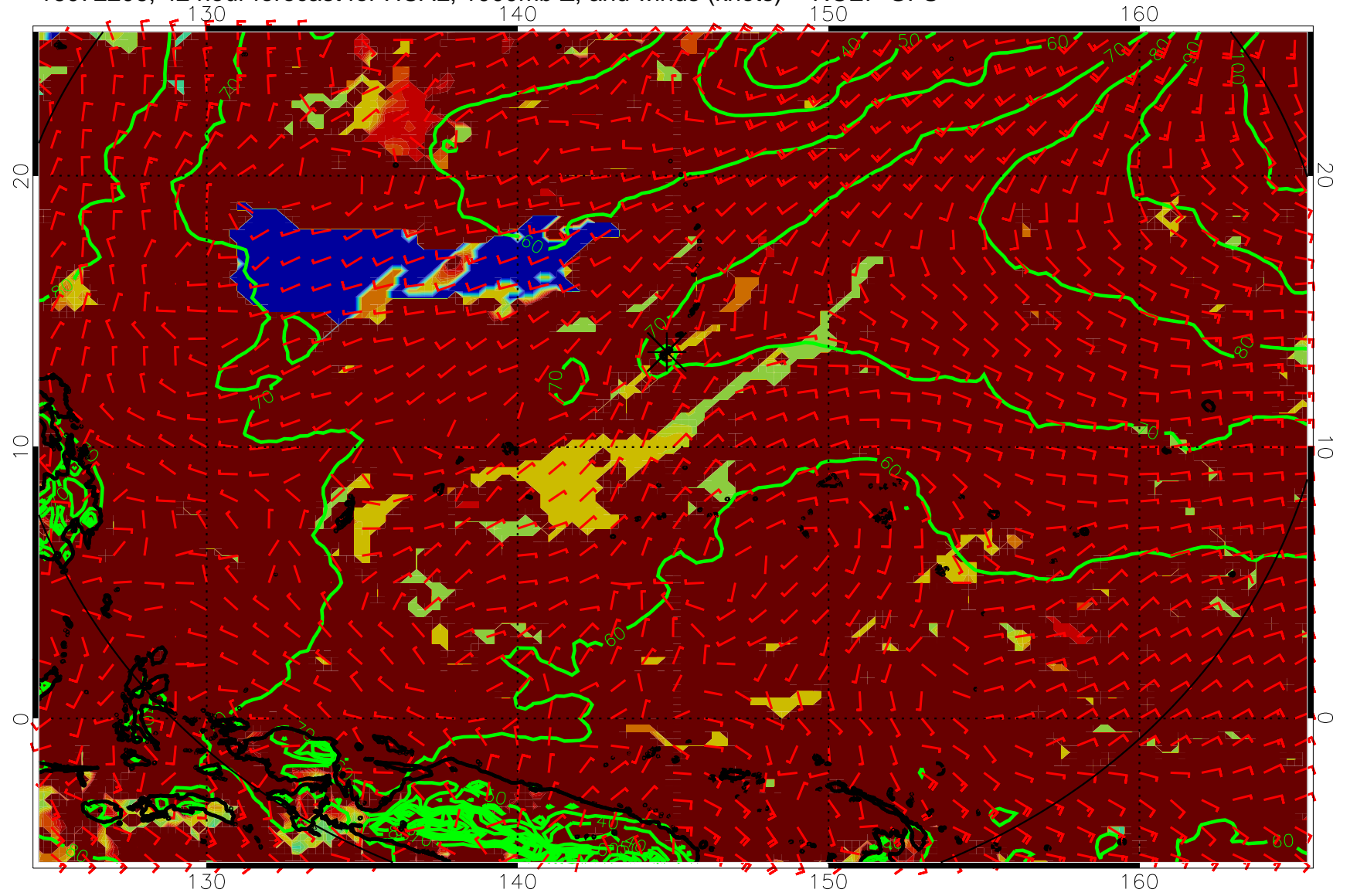
16072206, 42 hour forecast for HCAL, 1000mb Z, and winds (knots) -- NCEP GFS
