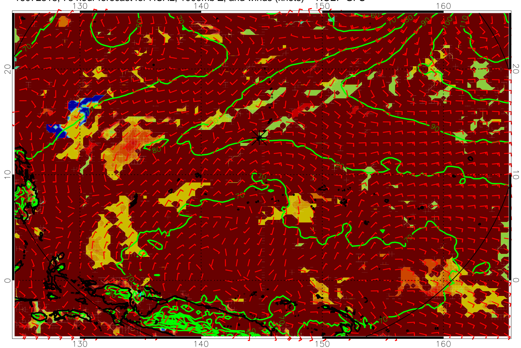
16072318, 78 hour forecast for HCAL, 1000mb Z, and winds (knots) -- NCEP GFS
