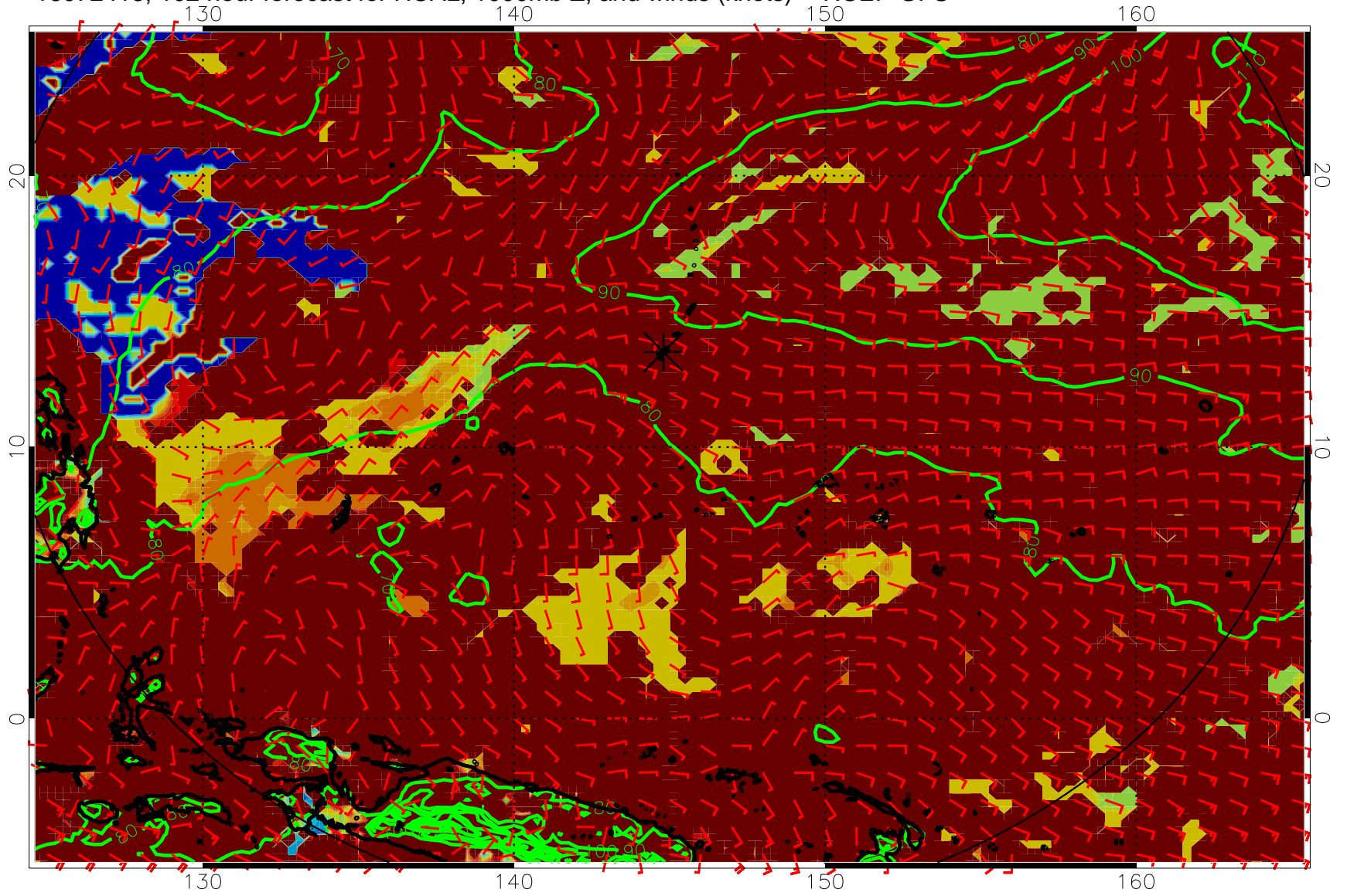
16072418, 102 hour forecast for HCAL, 1000mb Z, and winds (knots) -- NCEP GFS
