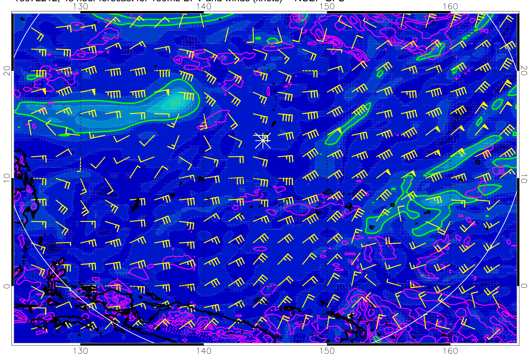
16072212, 48 hour forecast for 150mb EPV and winds (knots) -- NCEP GFS
