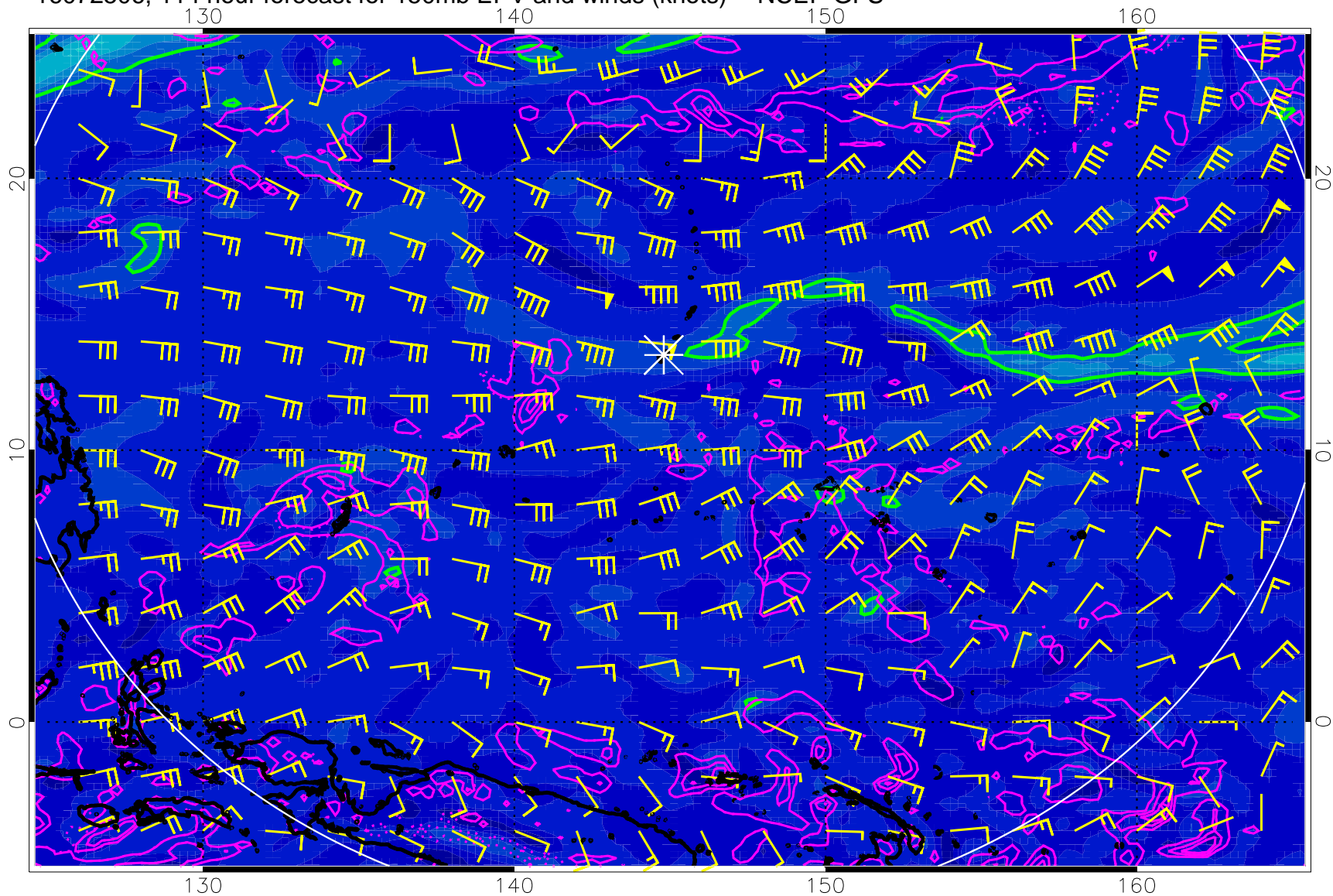
16072506, 114 hour forecast for 150mb EPV and winds (knots) -- NCEP GFS
