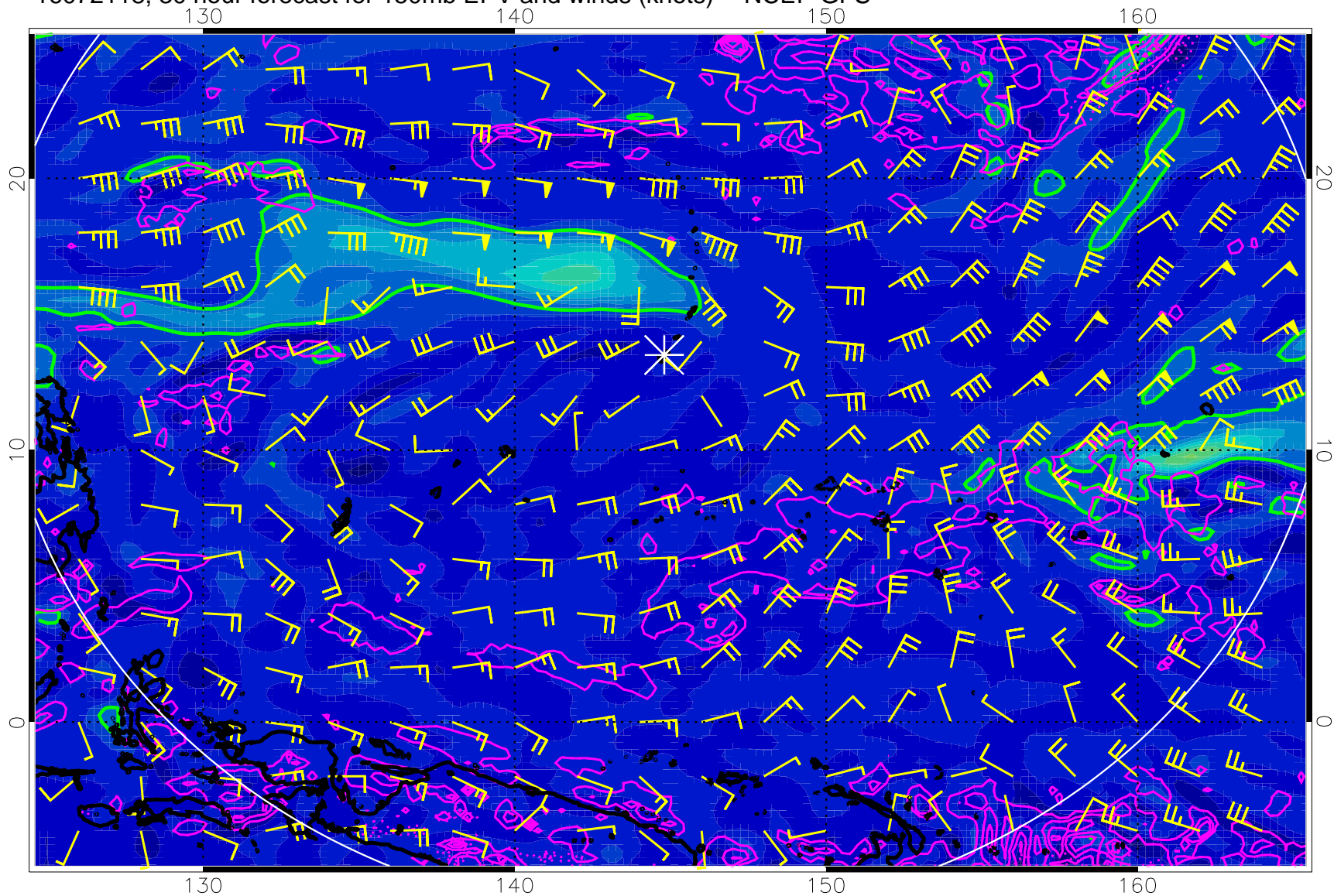
16072118, 30 hour forecast for 150mb EPV and winds (knots) -- NCEP GFS
