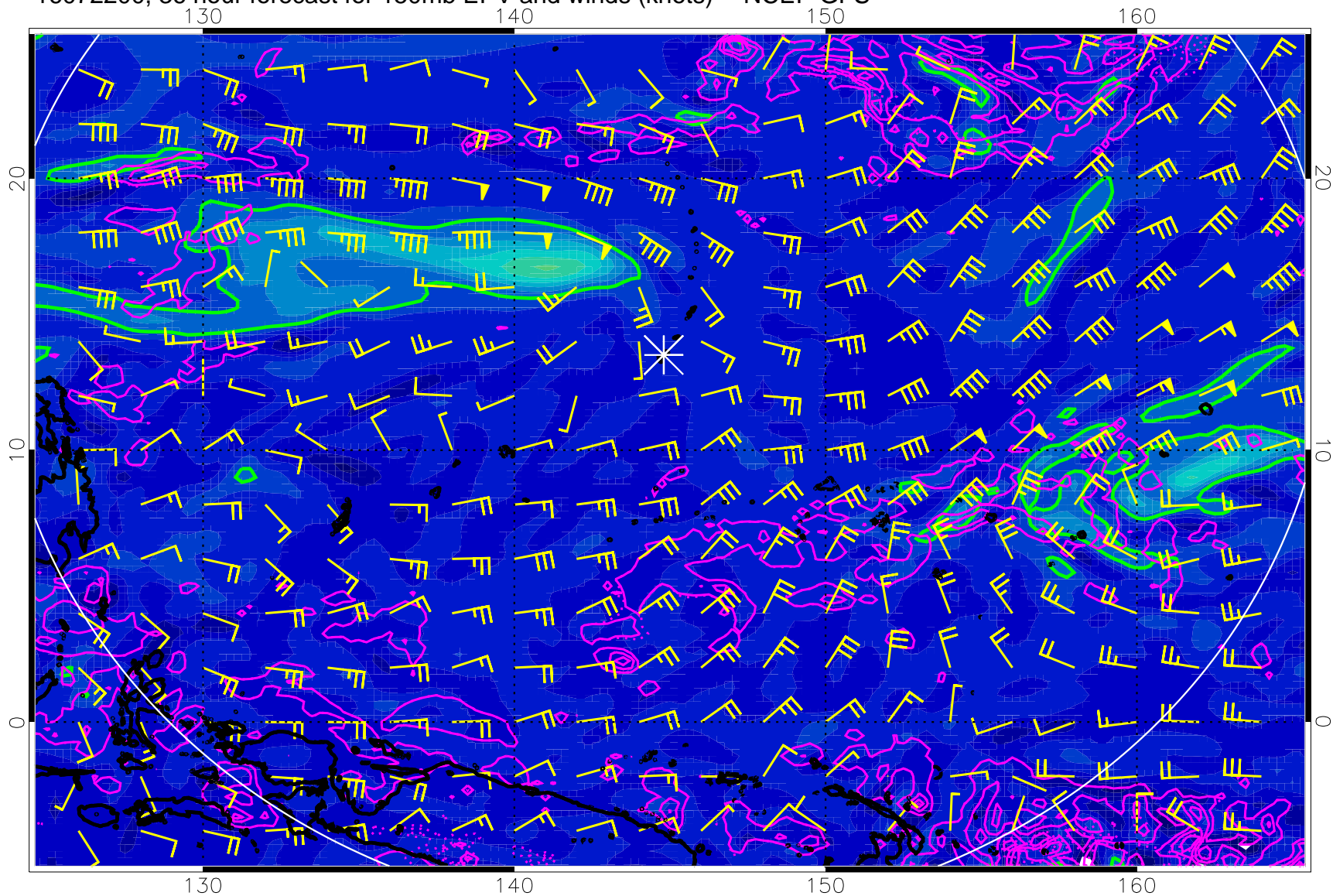
16072200, 36 hour forecast for 150mb EPV and winds (knots) -- NCEP GFS
