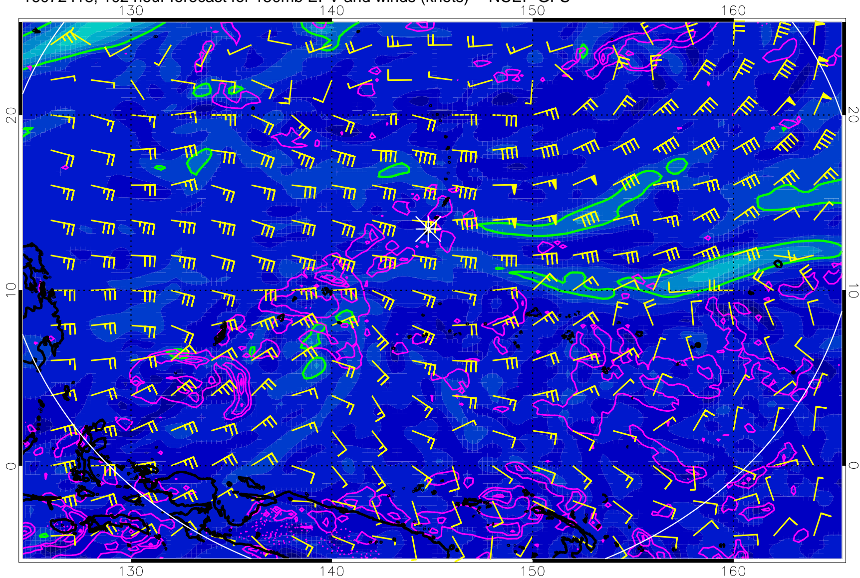
16072418, 102 hour forecast for 150mb EPV and winds (knots) -- NCEP GFS
