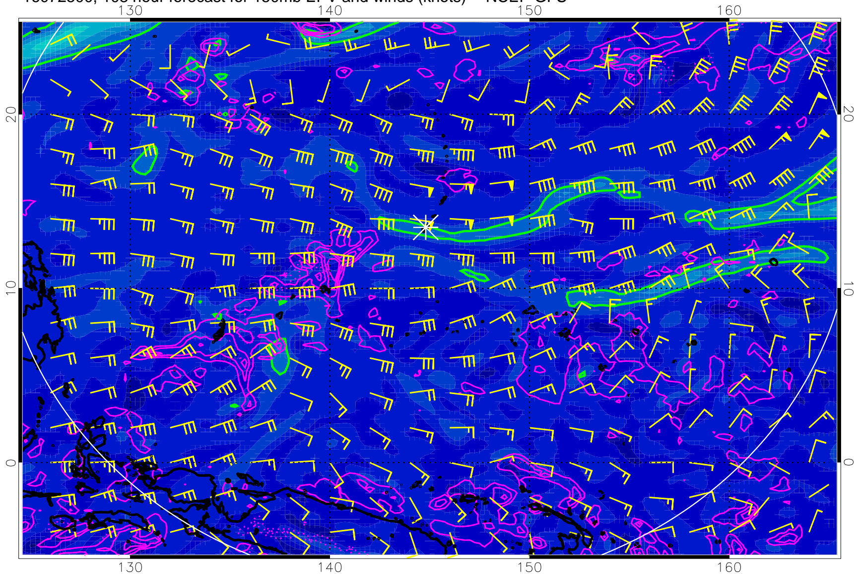
16072500, 108 hour forecast for 150mb EPV and winds (knots) -- NCEP GFS
