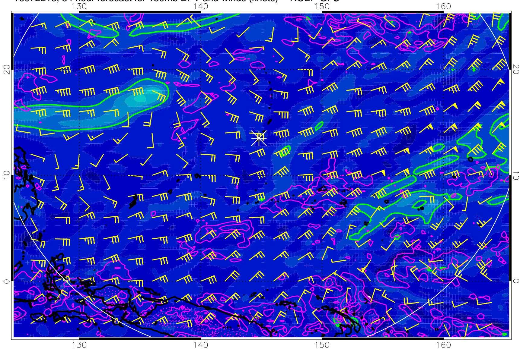
16072218, 54 hour forecast for 150mb EPV and winds (knots) -- NCEP GFS
