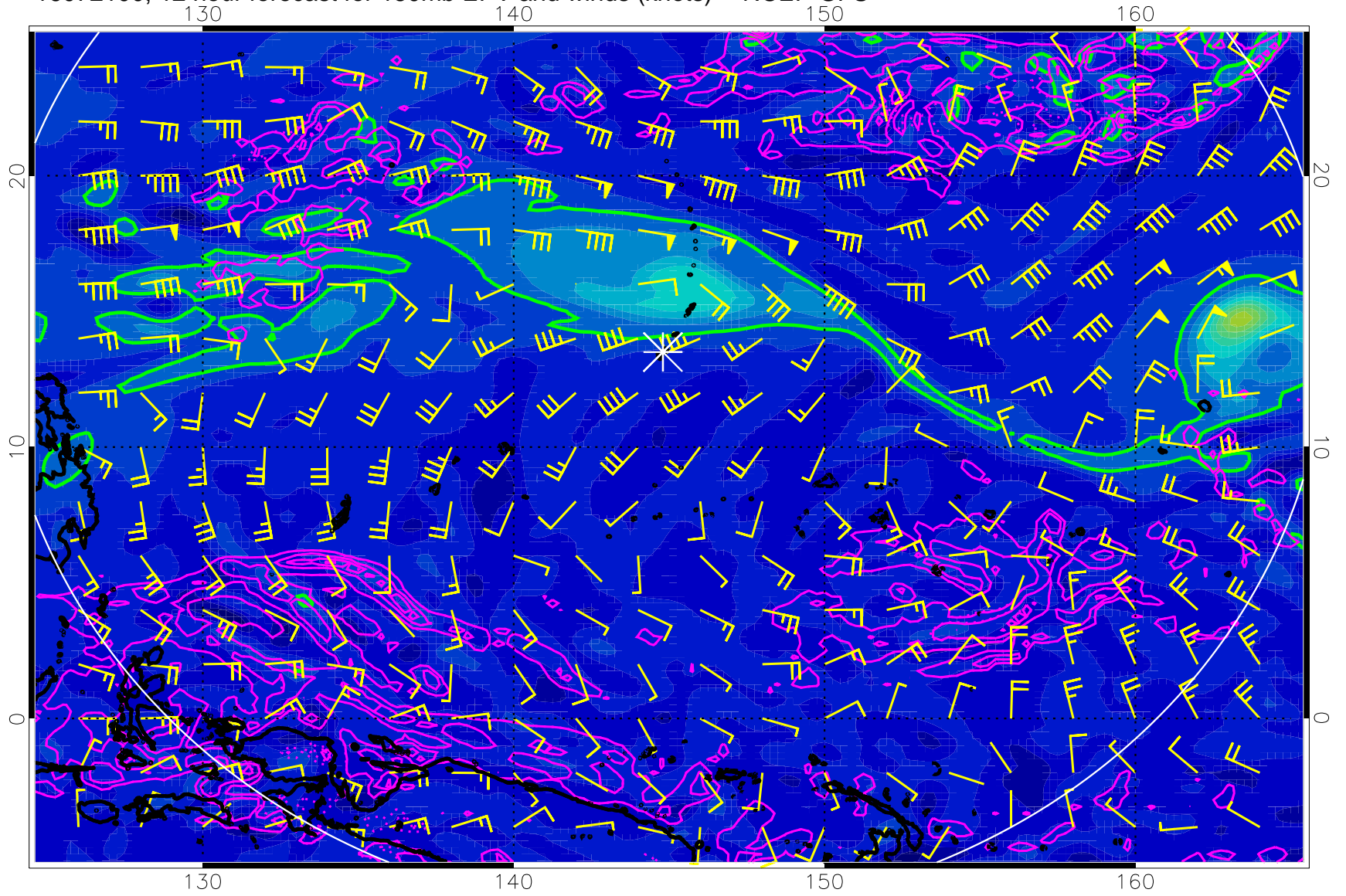
16072100, 12 hour forecast for 150mb EPV and winds (knots) -- NCEP GFS
