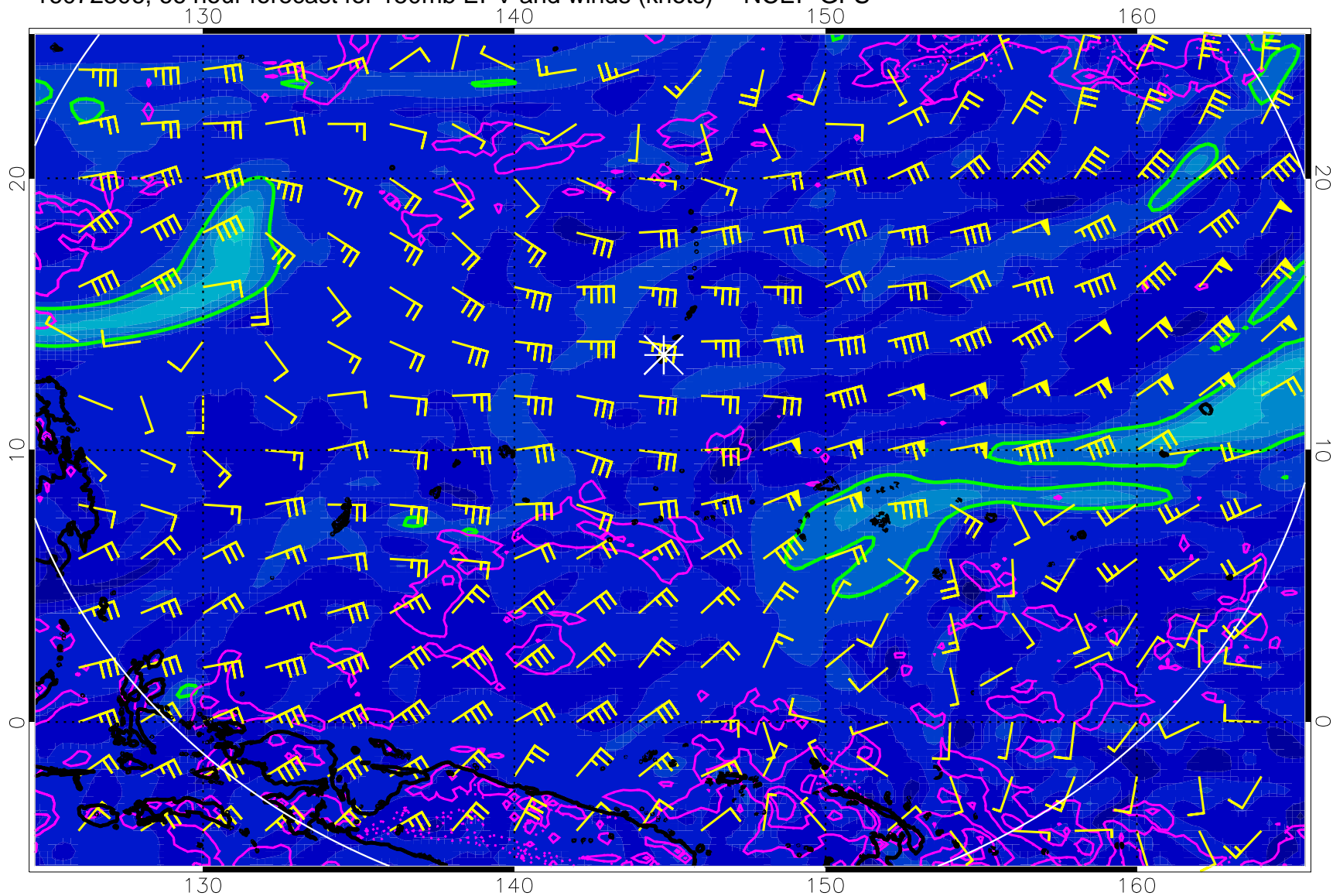
16072306, 66 hour forecast for 150mb EPV and winds (knots) -- NCEP GFS
