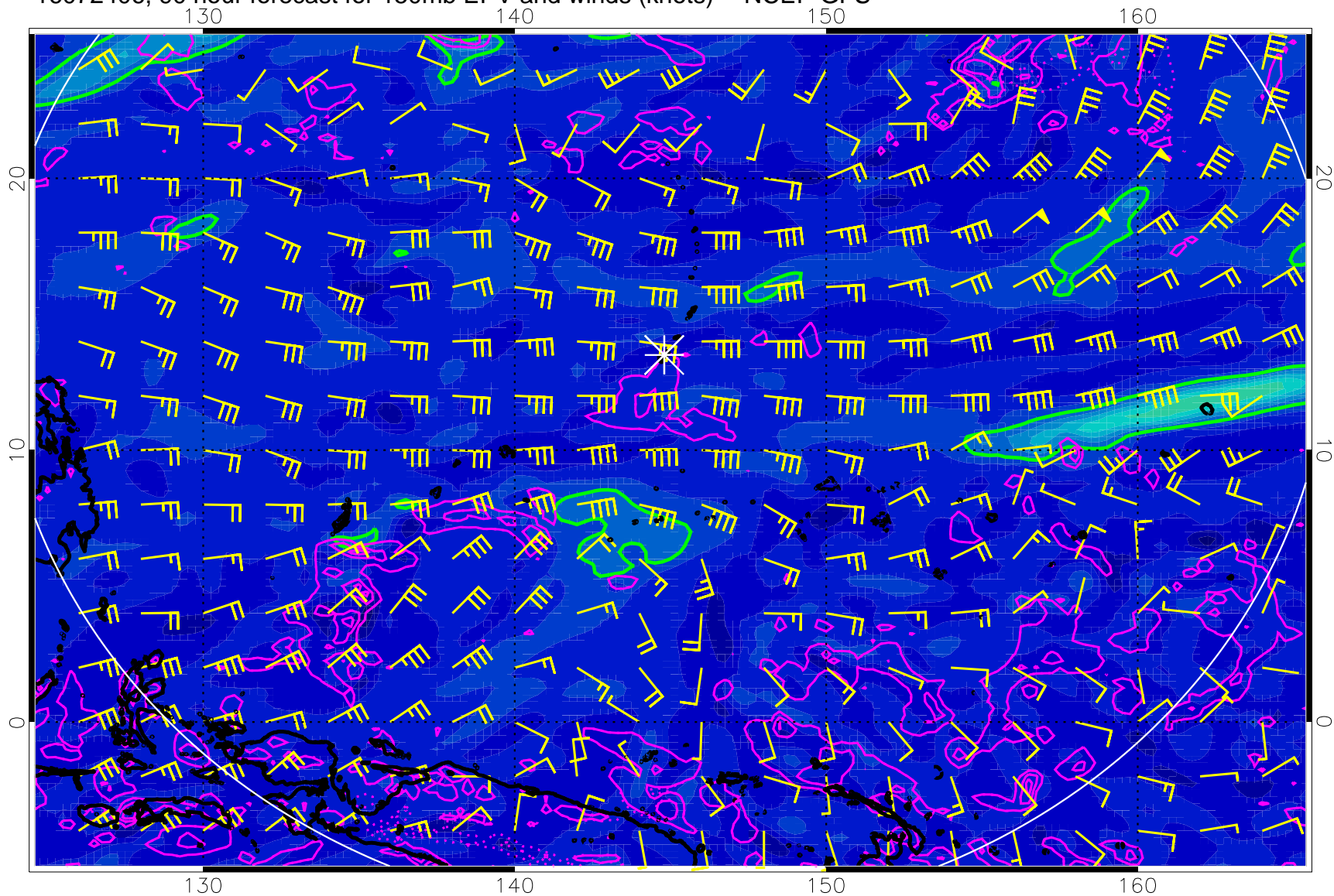
16072406, 90 hour forecast for 150mb EPV and winds (knots) -- NCEP GFS
