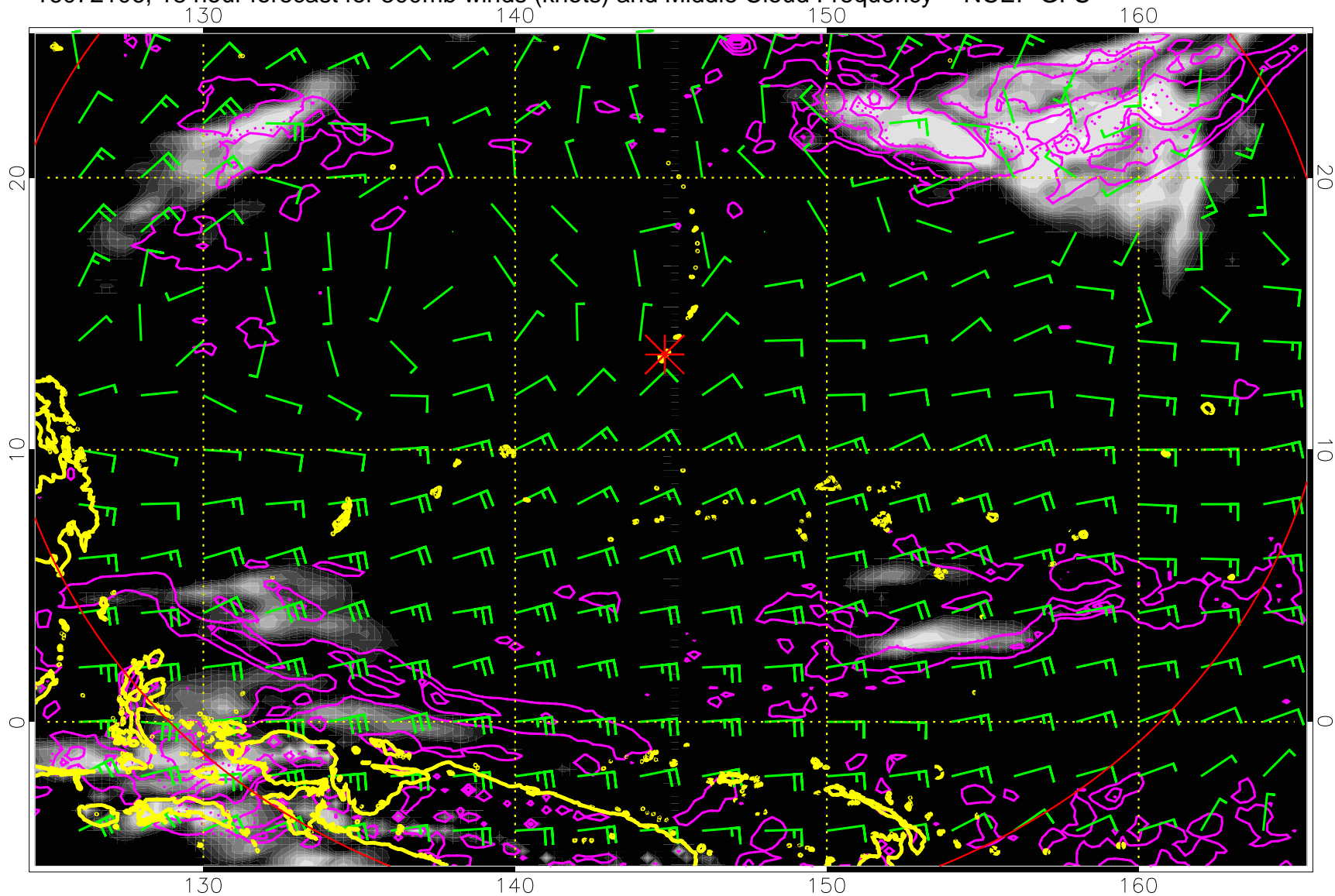
16072106, 18 hour forecast for 500mb winds (knots) and Middle Cloud Frequency -- NCEP GFS
