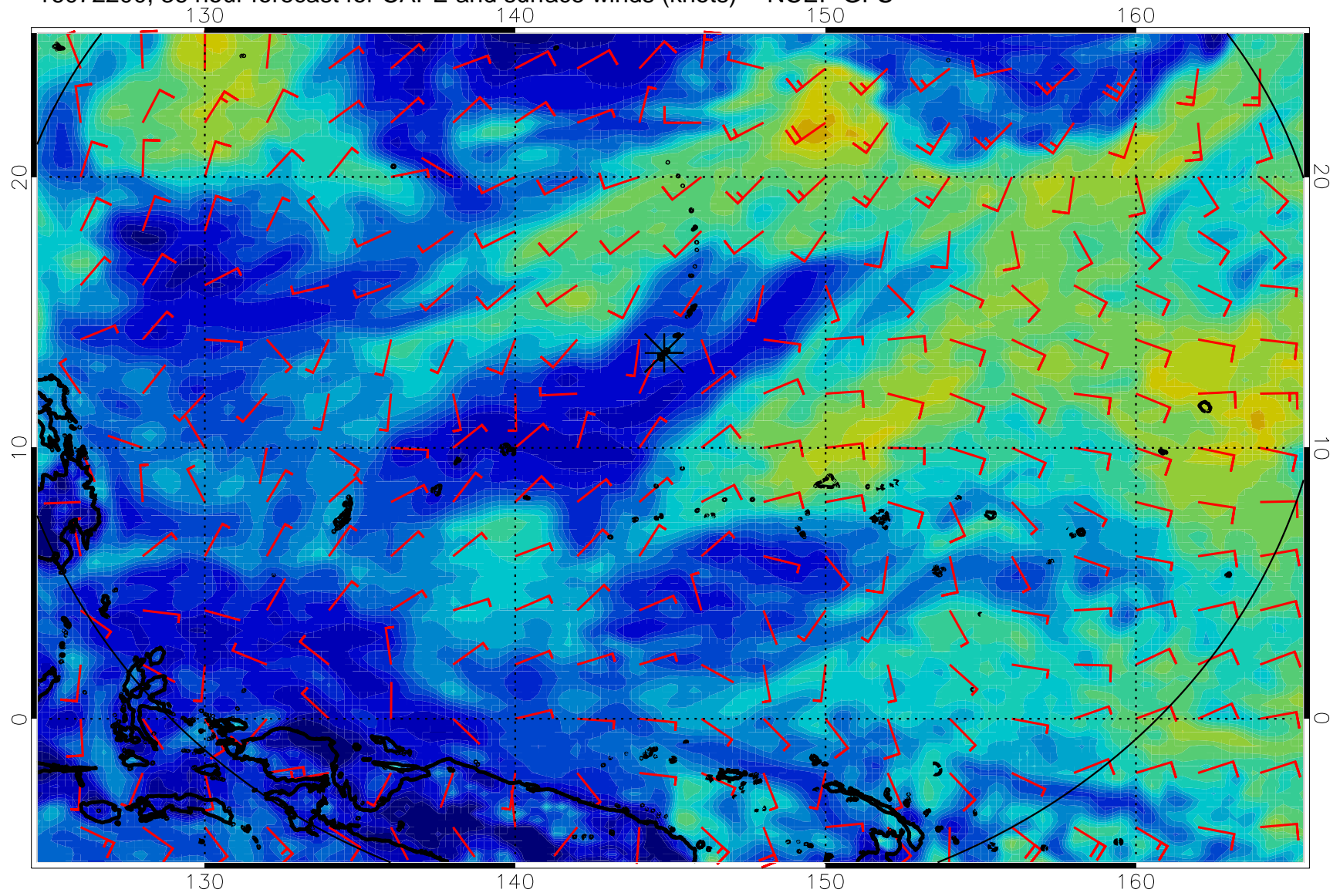
16072200, 36 hour forecast for CAPE and surface winds (knots) -- NCEP GFS
