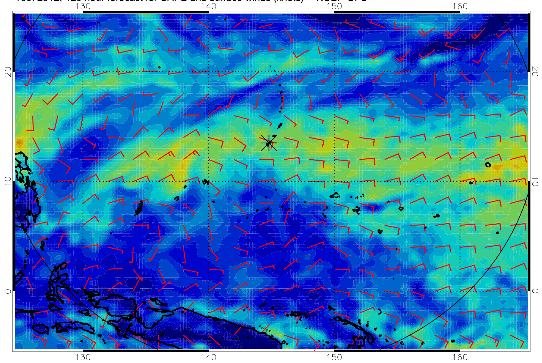
16072512, 120 hour forecast for CAPE and surface winds (knots) -- NCEP GFS
