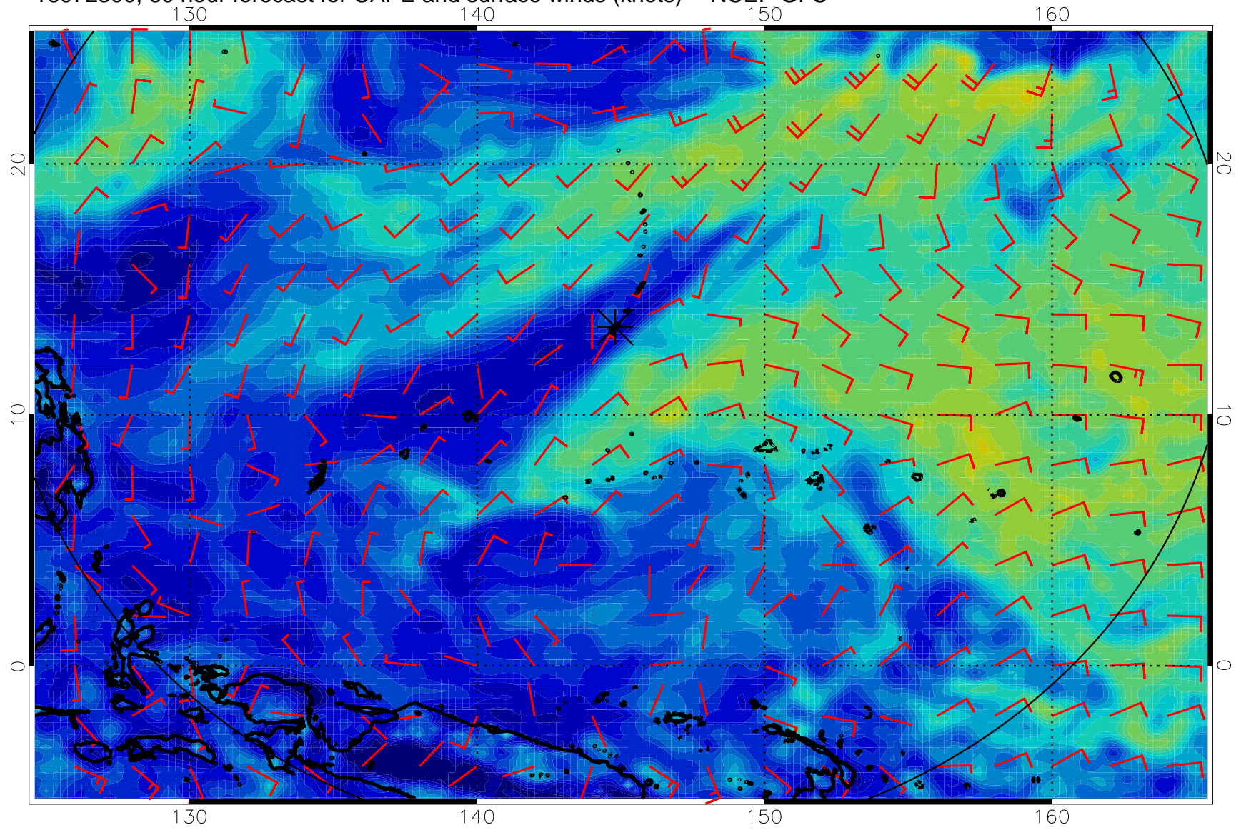
16072300, 60 hour forecast for CAPE and surface winds (knots) -- NCEP GFS
