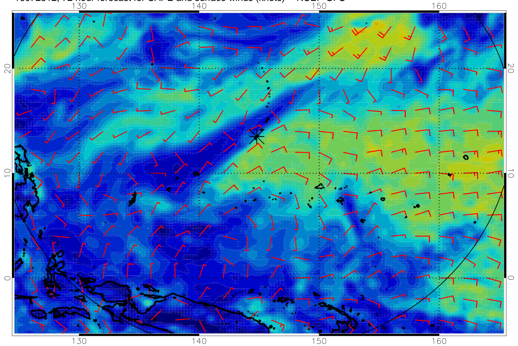
16072312, 72 hour forecast for CAPE and surface winds (knots) -- NCEP GFS
