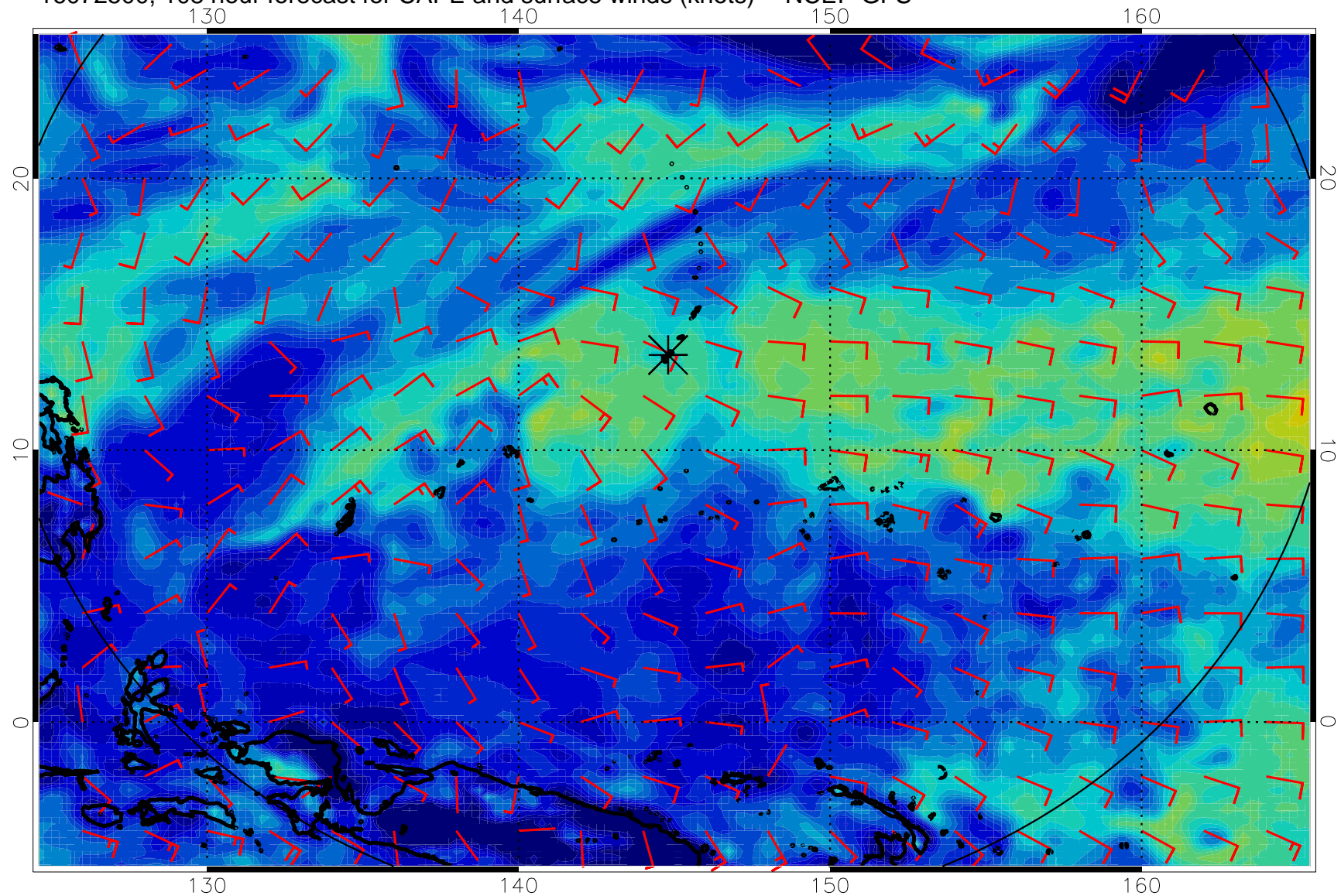
16072500, 108 hour forecast for CAPE and surface winds (knots) -- NCEP GFS
