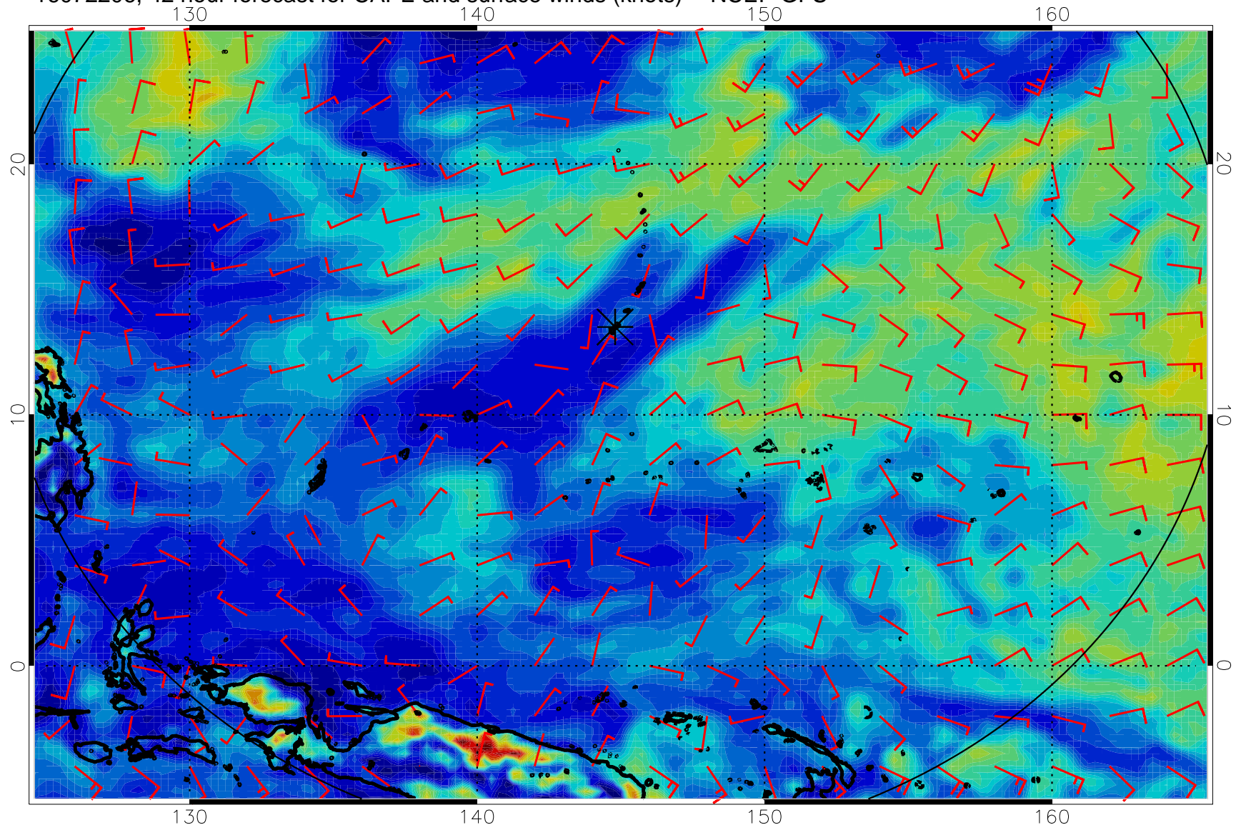
16072206, 42 hour forecast for CAPE and surface winds (knots) -- NCEP GFS
