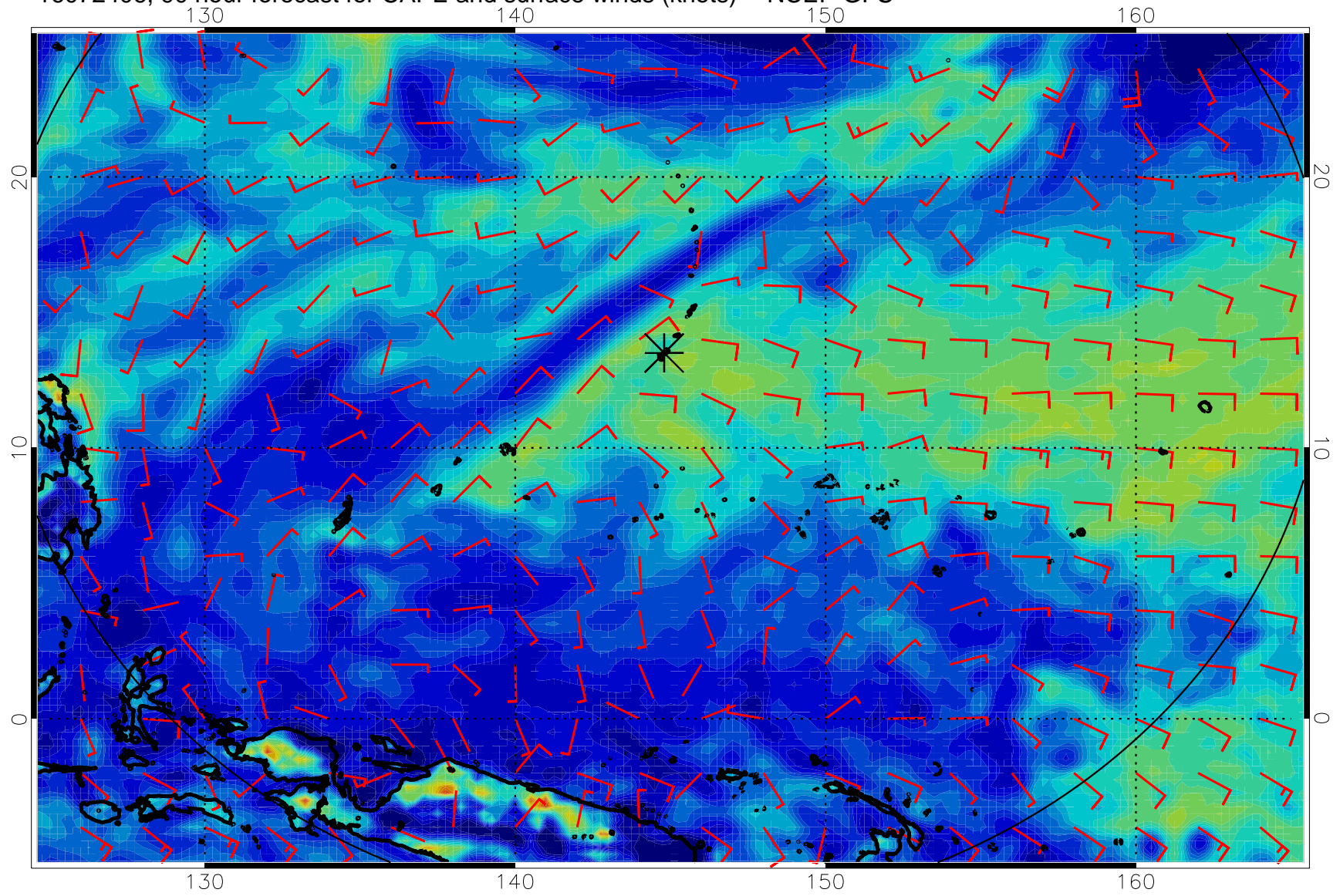
16072406, 90 hour forecast for CAPE and surface winds (knots) -- NCEP GFS
