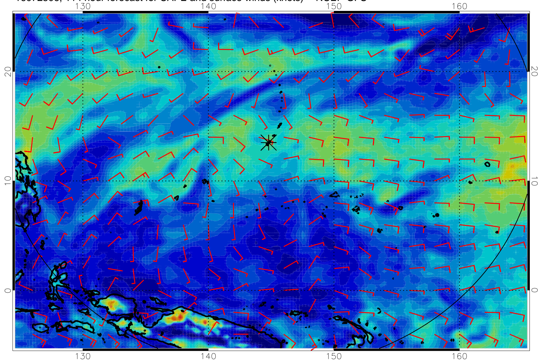
16072506, 114 hour forecast for CAPE and surface winds (knots) -- NCEP GFS
