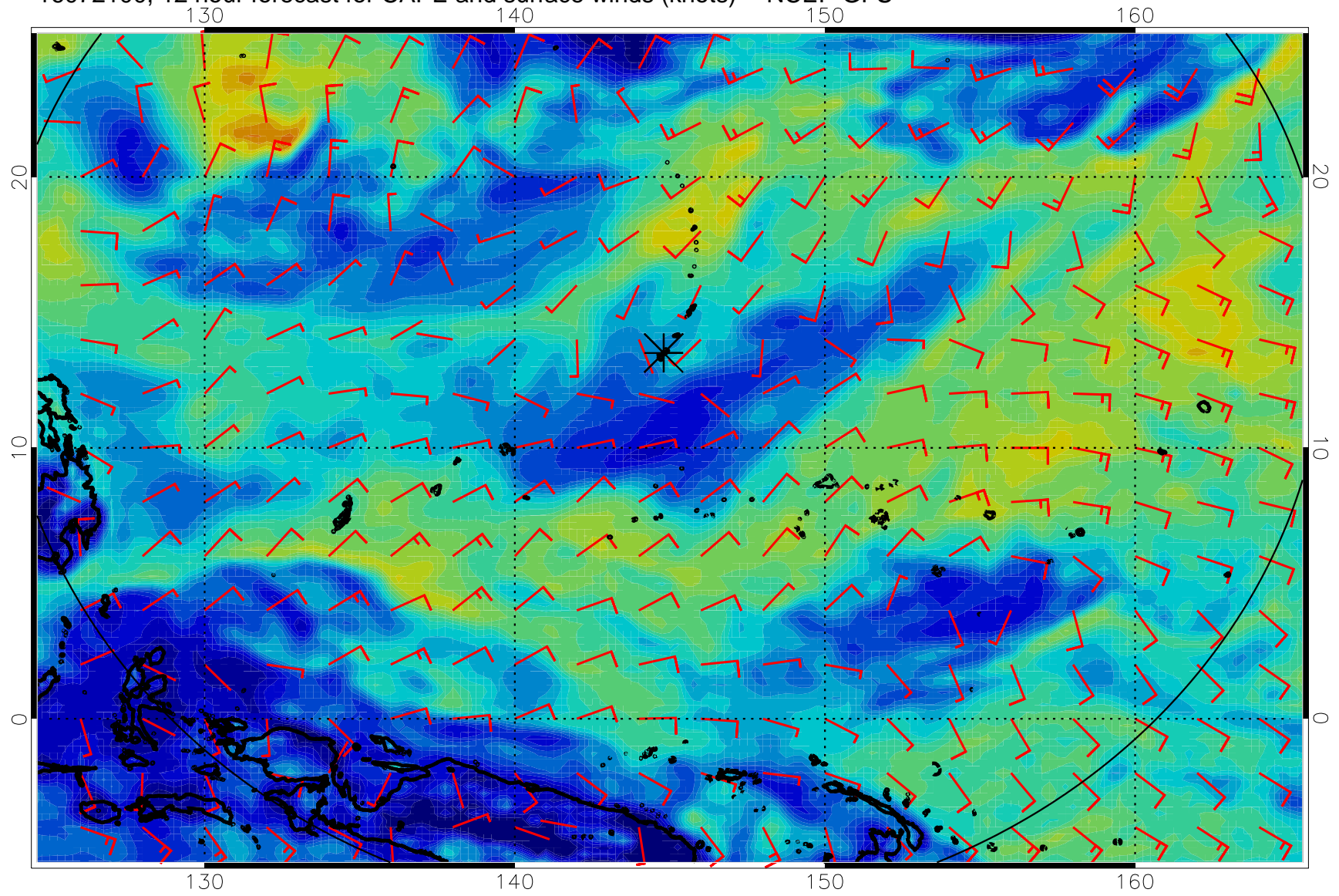
16072100, 12 hour forecast for CAPE and surface winds (knots) -- NCEP GFS
