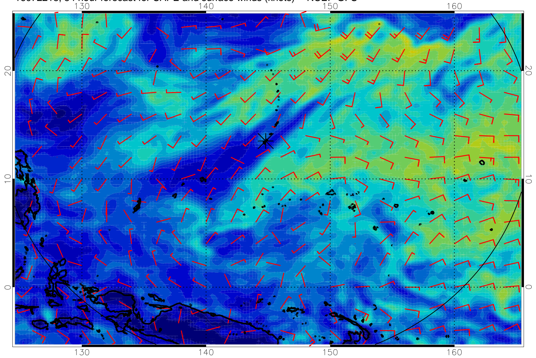
16072218, 54 hour forecast for CAPE and surface winds (knots) -- NCEP GFS
