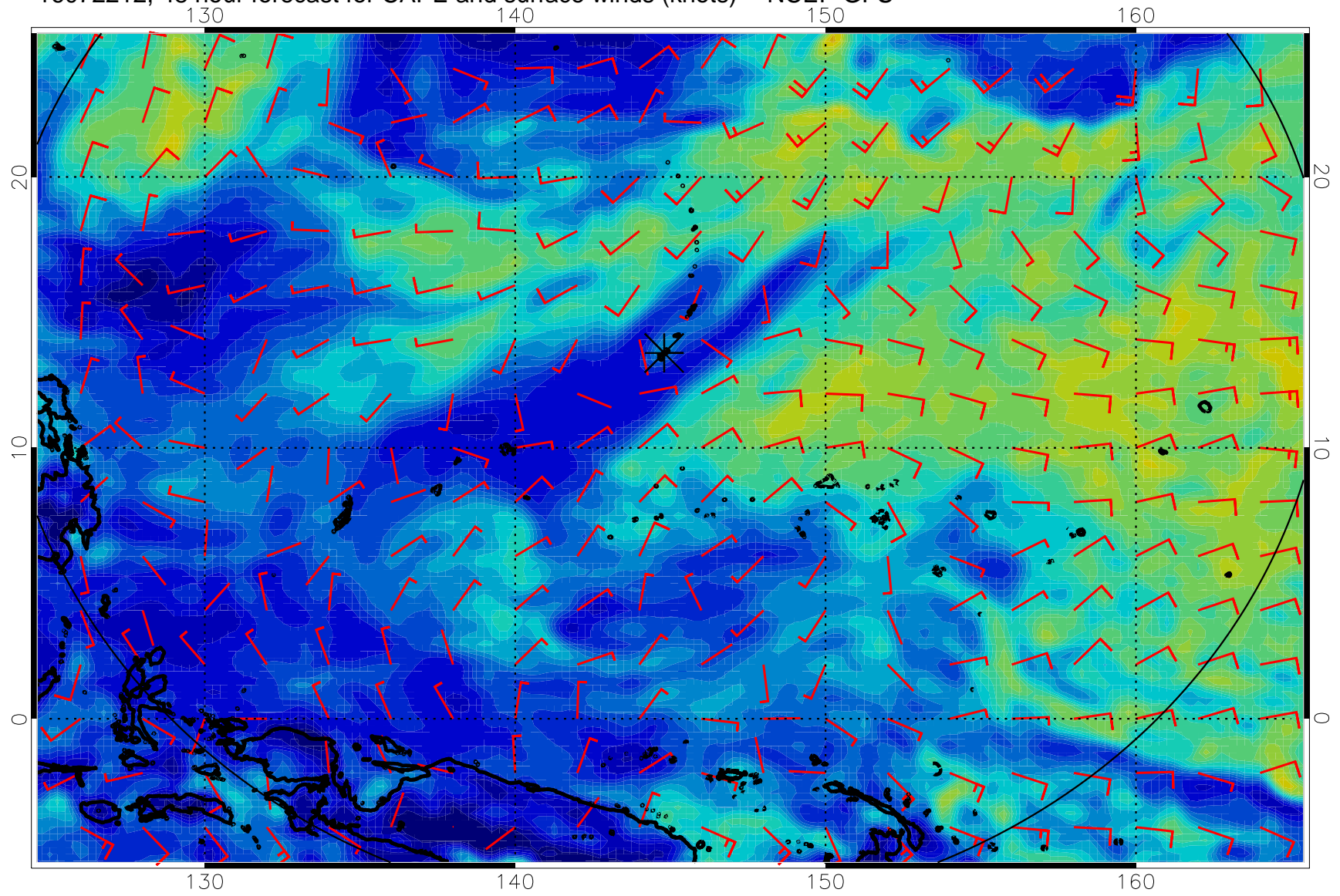
16072212, 48 hour forecast for CAPE and surface winds (knots) -- NCEP GFS
