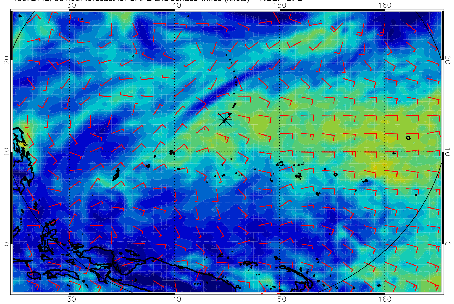
16072412, 96 hour forecast for CAPE and surface winds (knots) -- NCEP GFS
