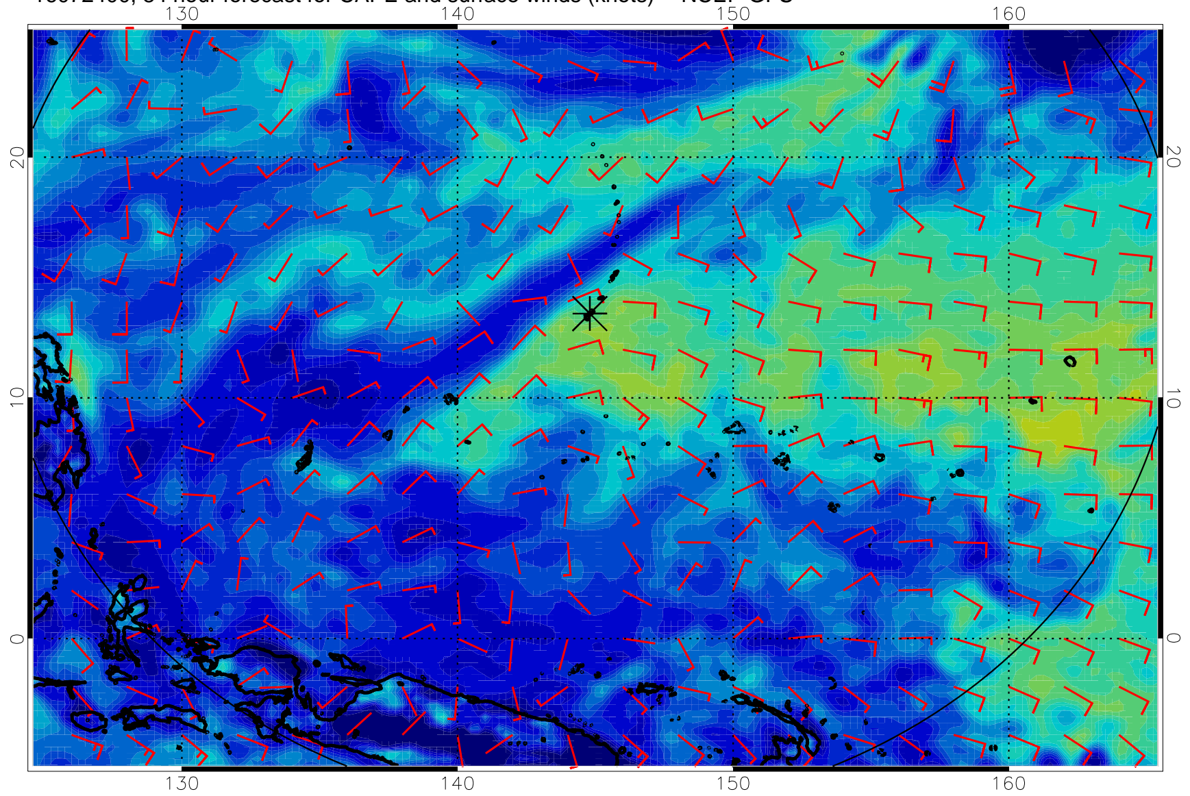
16072400, 84 hour forecast for CAPE and surface winds (knots) -- NCEP GFS
