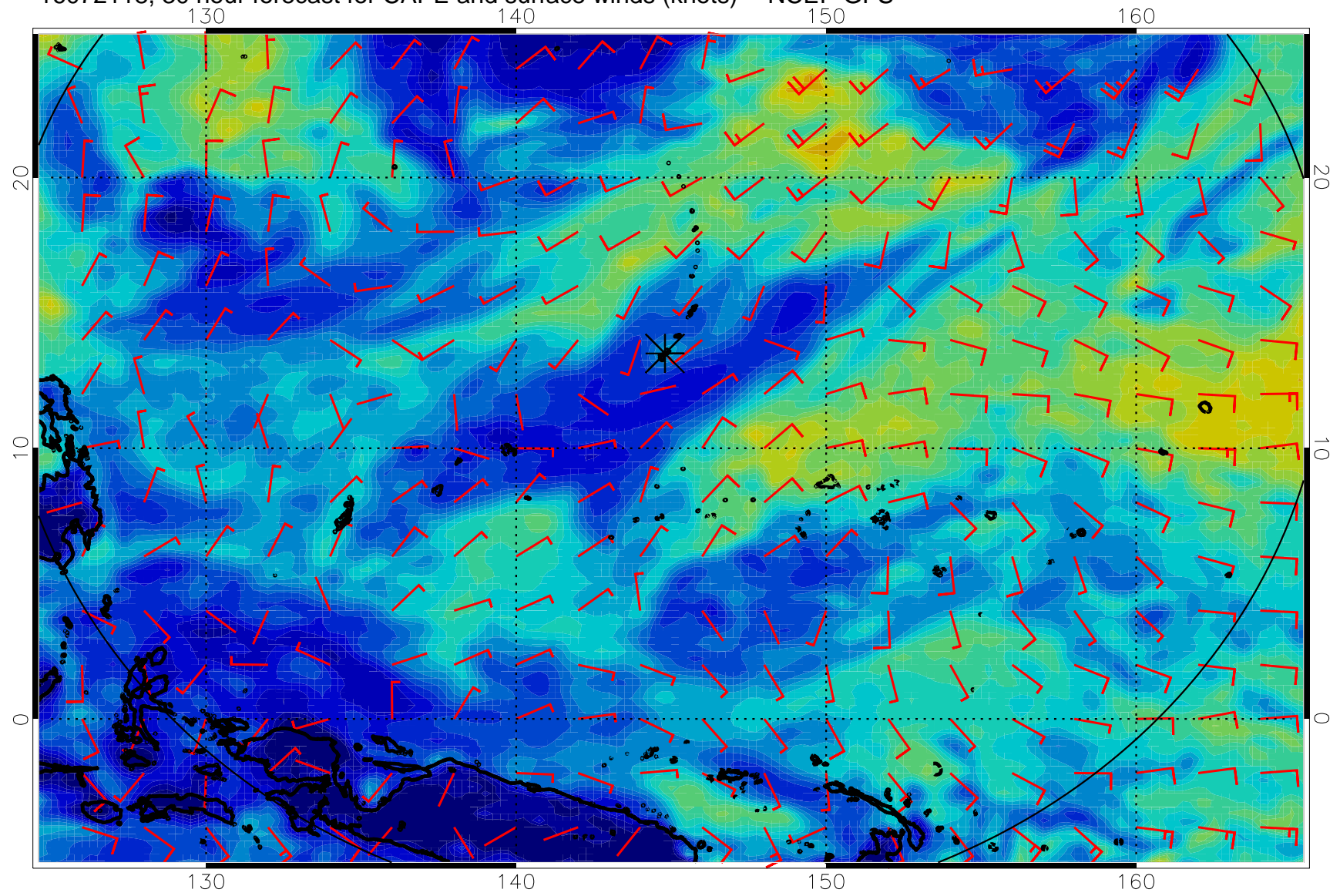
16072118, 30 hour forecast for CAPE and surface winds (knots) -- NCEP GFS
