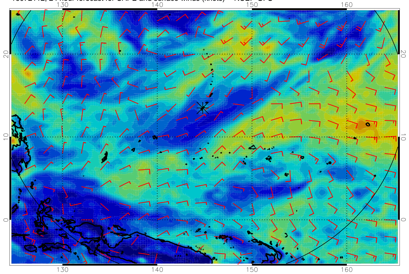
16072112, 24 hour forecast for CAPE and surface winds (knots) -- NCEP GFS
