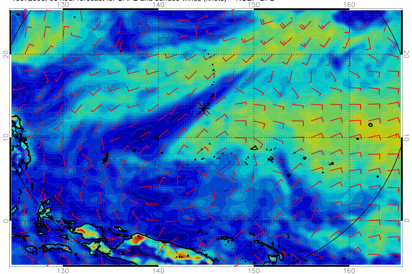
16072306, 66 hour forecast for CAPE and surface winds (knots) -- NCEP GFS
