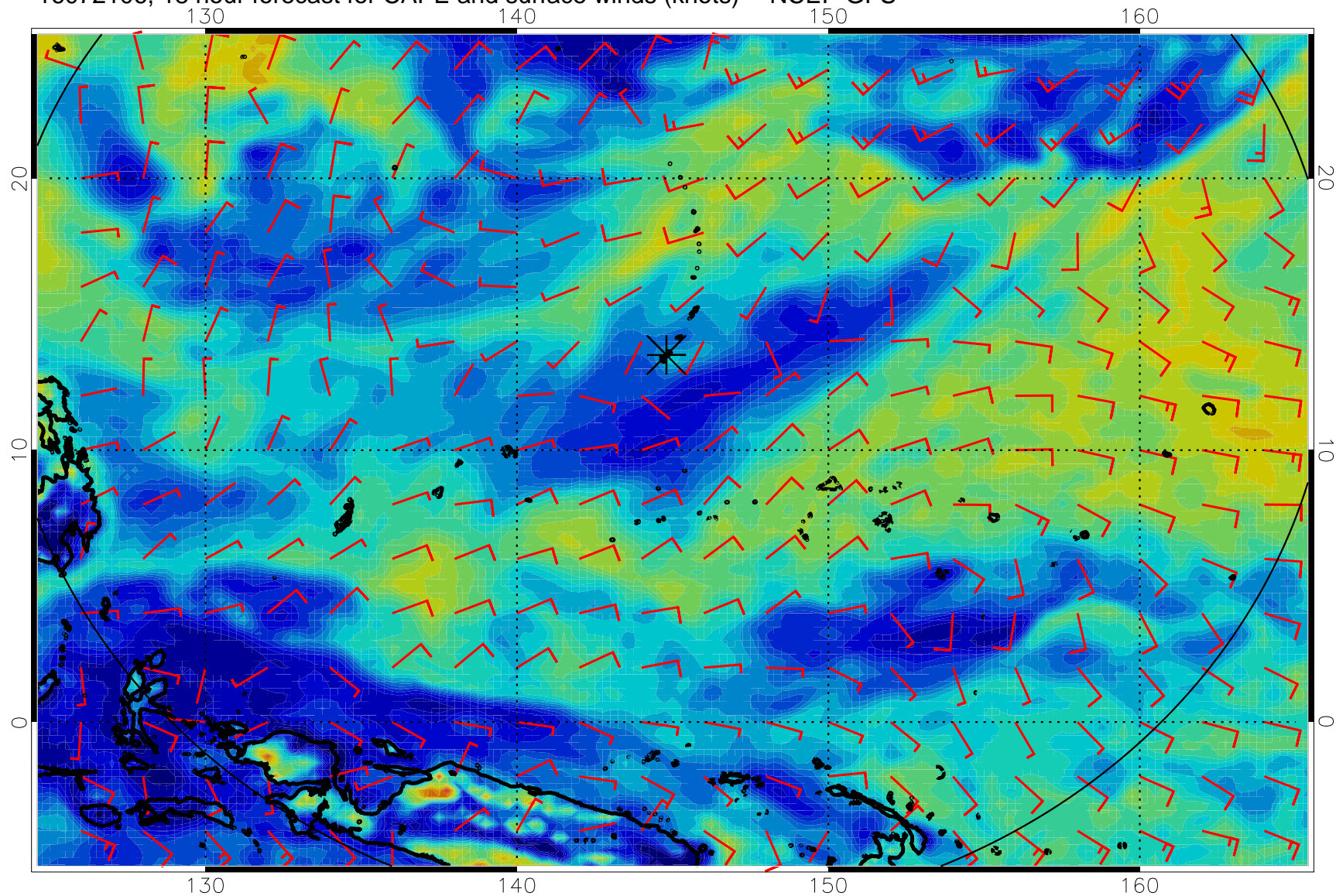
16072106, 18 hour forecast for CAPE and surface winds (knots) -- NCEP GFS
