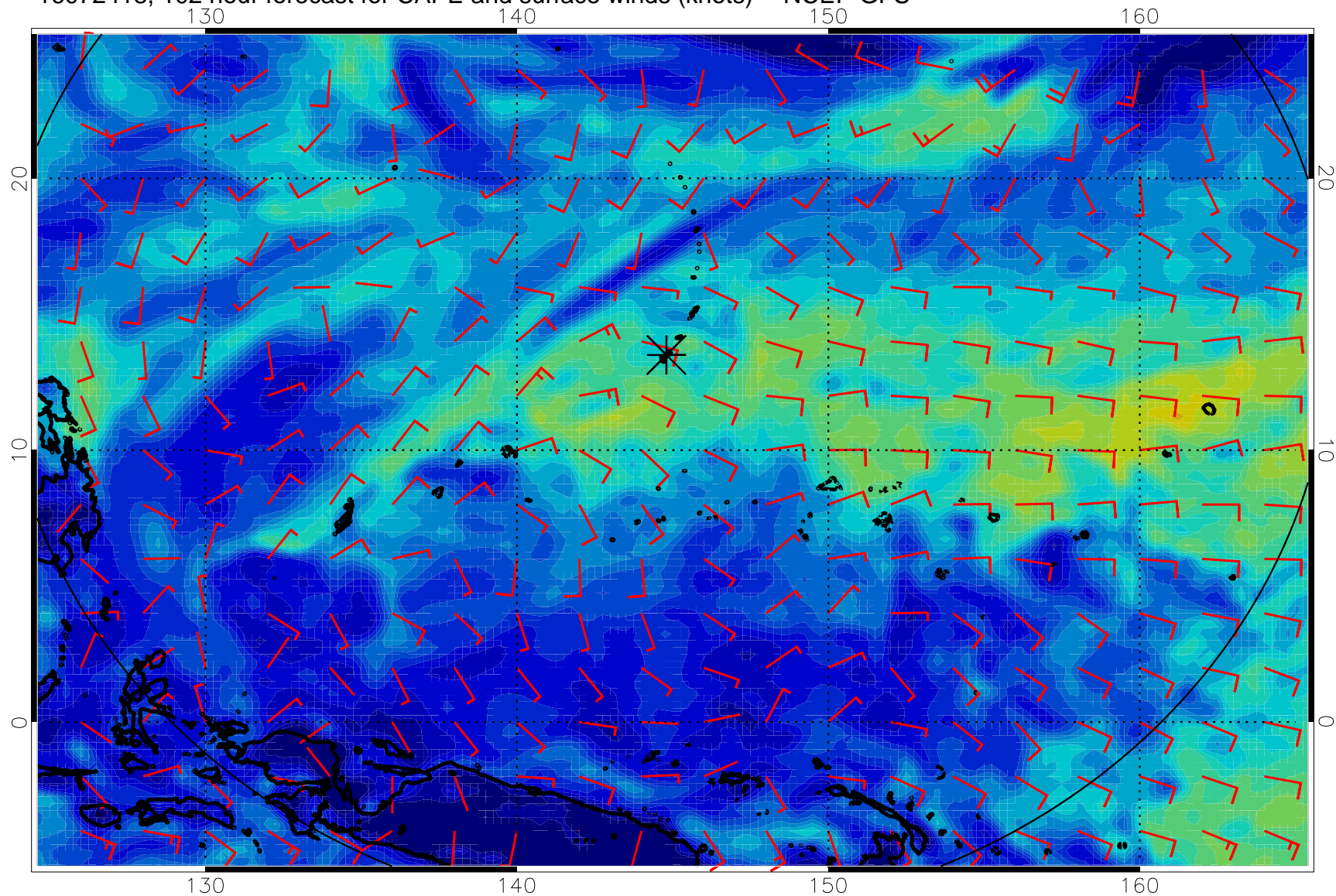
16072418, 102 hour forecast for CAPE and surface winds (knots) -- NCEP GFS
