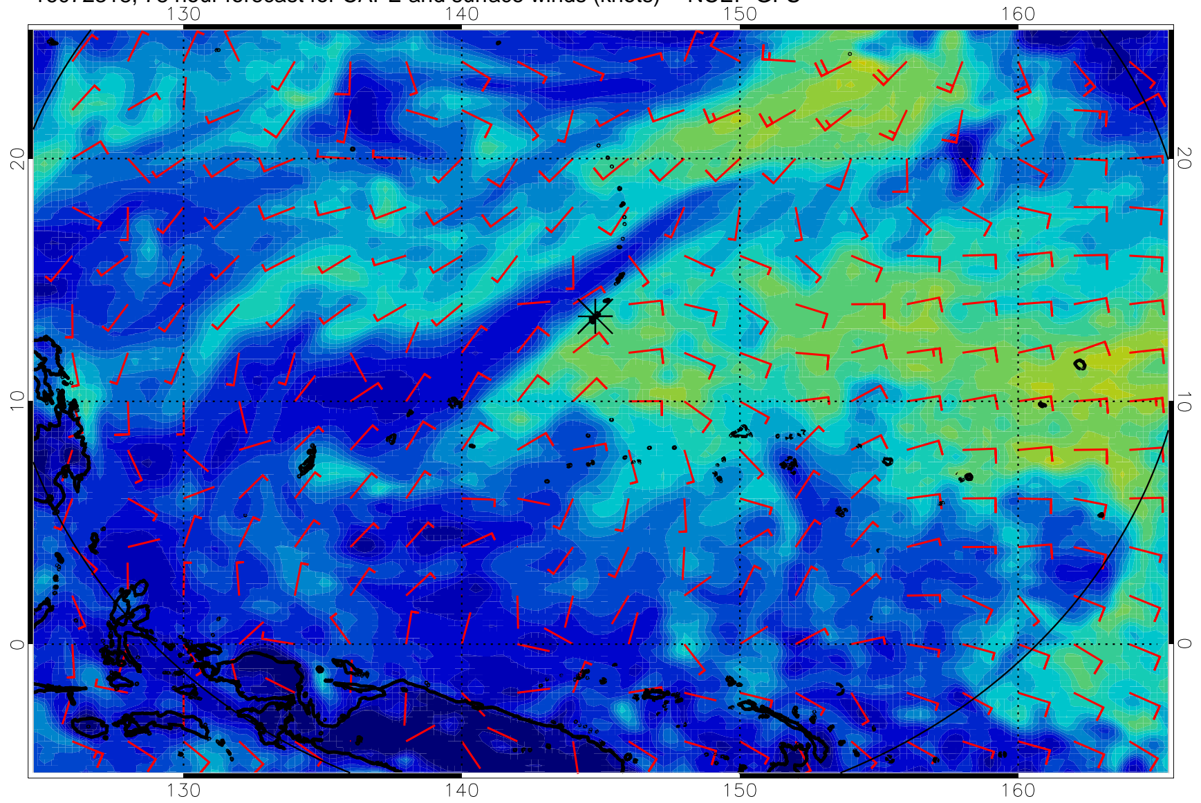
16072318, 78 hour forecast for CAPE and surface winds (knots) -- NCEP GFS
