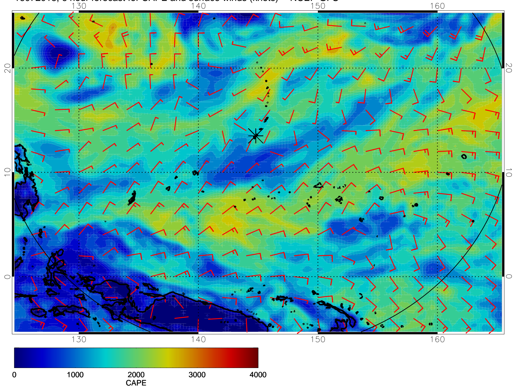
16072018, 6 hour forecast for CAPE and surface winds (knots) -- NCEP GFS
