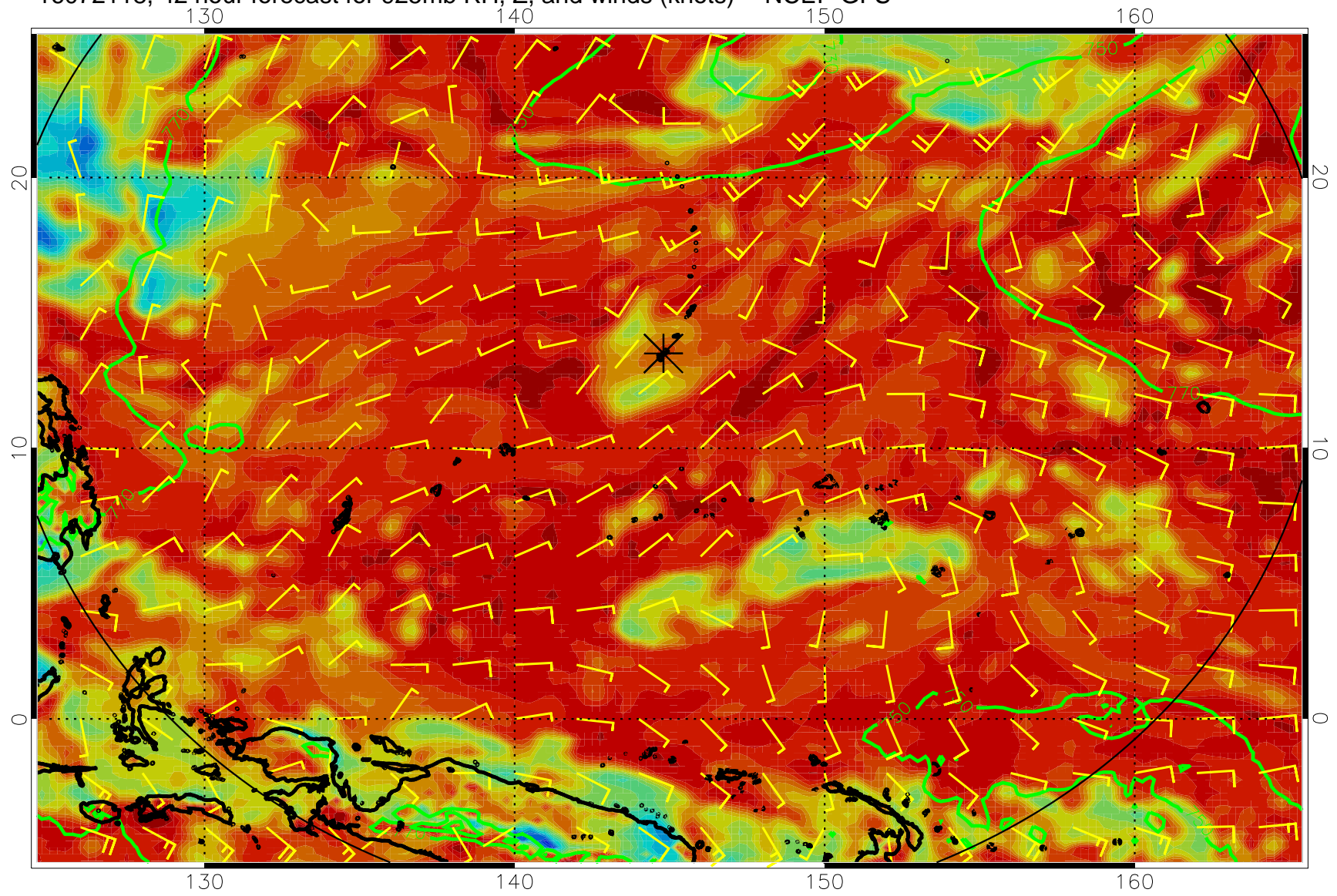
16072118, 42 hour forecast for 925mb RH, Z, and winds (knots) -- NCEP GFS
