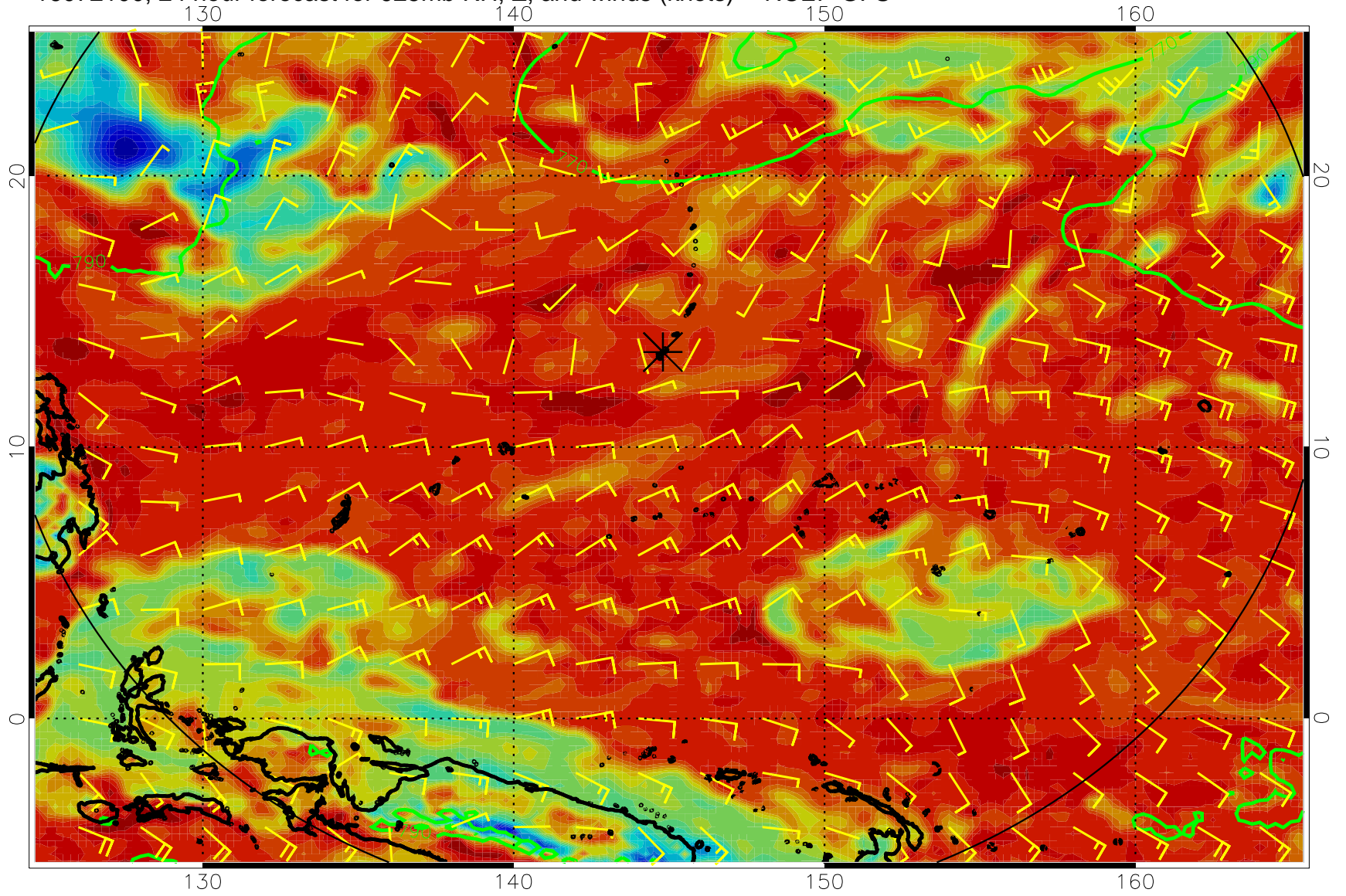
16072100, 24 hour forecast for 925mb RH, Z, and winds (knots) -- NCEP GFS
