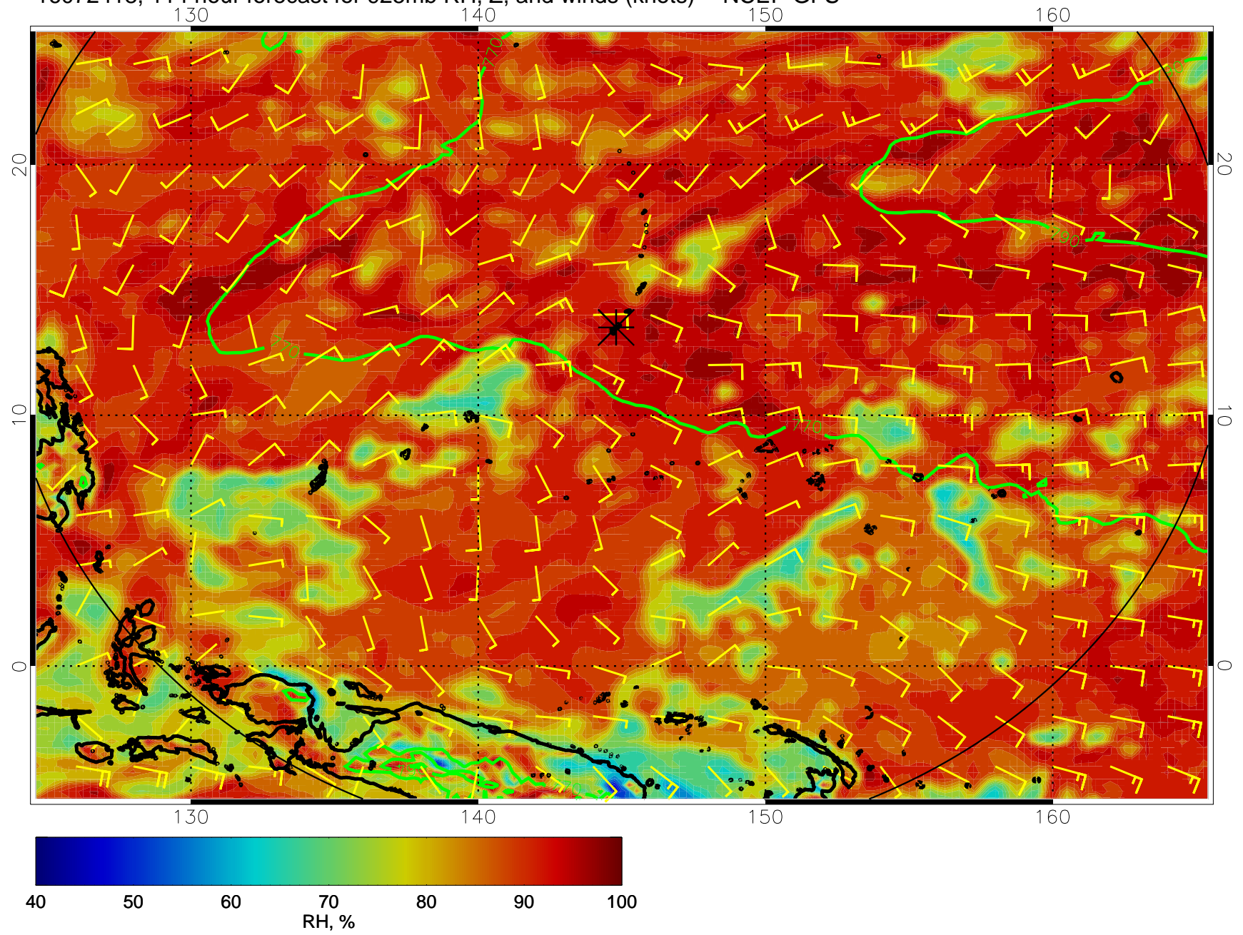
16072418, 114 hour forecast for 925mb RH, Z, and winds (knots) -- NCEP GFS
