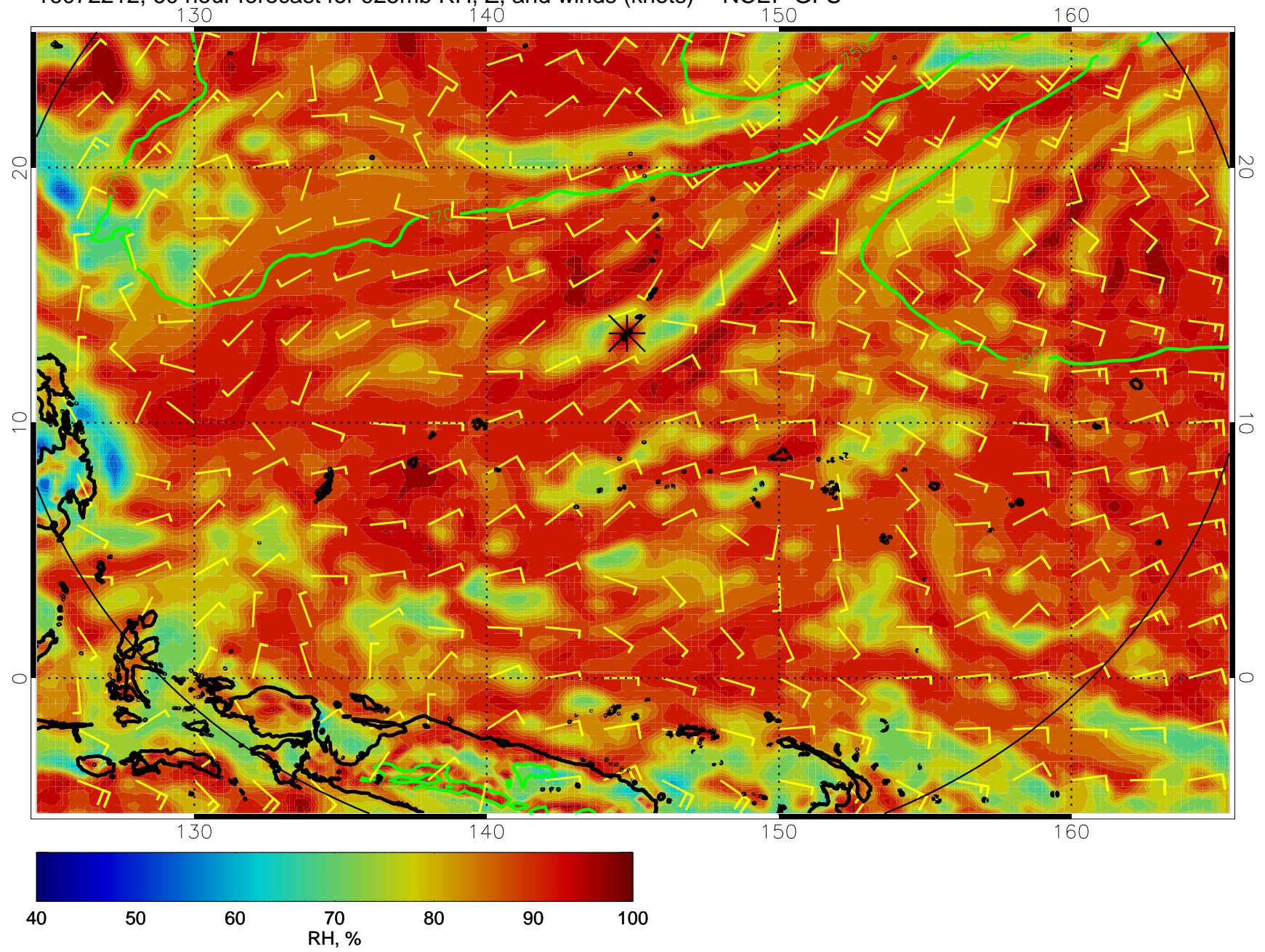
16072212, 60 hour forecast for 925mb RH, Z, and winds (knots) -- NCEP GFS
