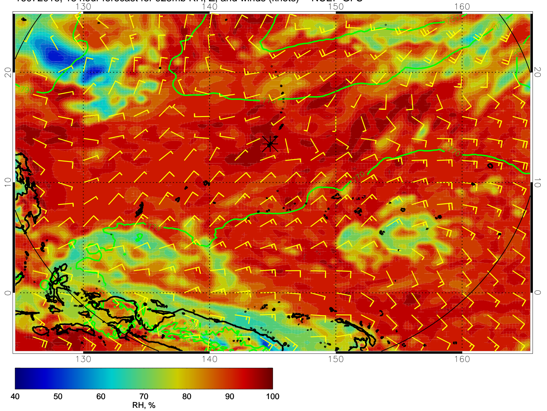
16072018, 18 hour forecast for 925mb RH, Z, and winds (knots) -- NCEP GFS
