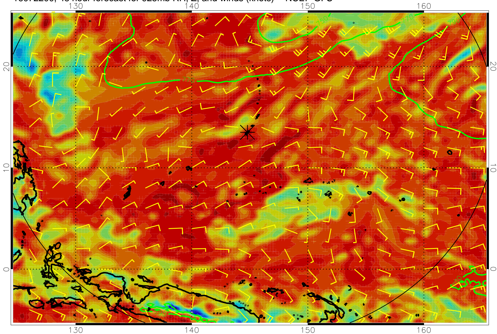
16072200, 48 hour forecast for 925mb RH, Z, and winds (knots) -- NCEP GFS
