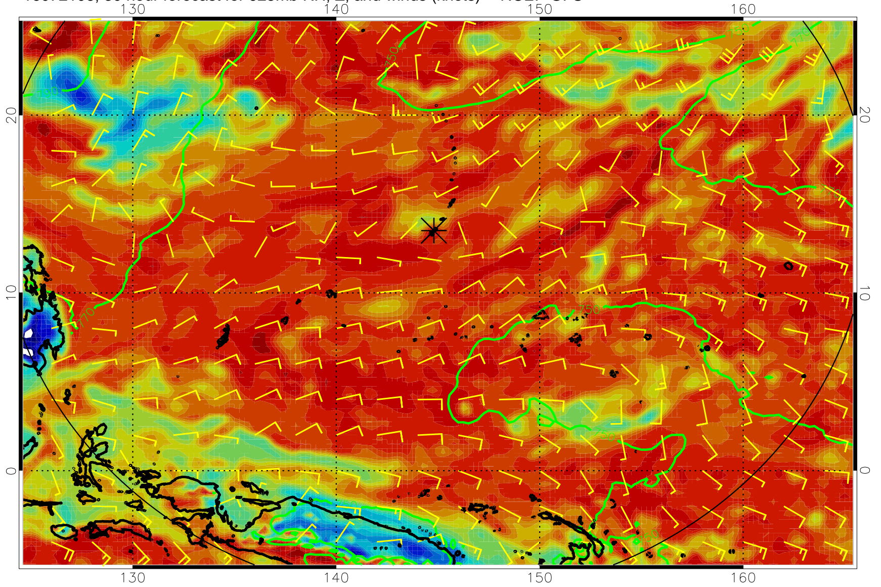
16072106, 30 hour forecast for 925mb RH, Z, and winds (knots) -- NCEP GFS
