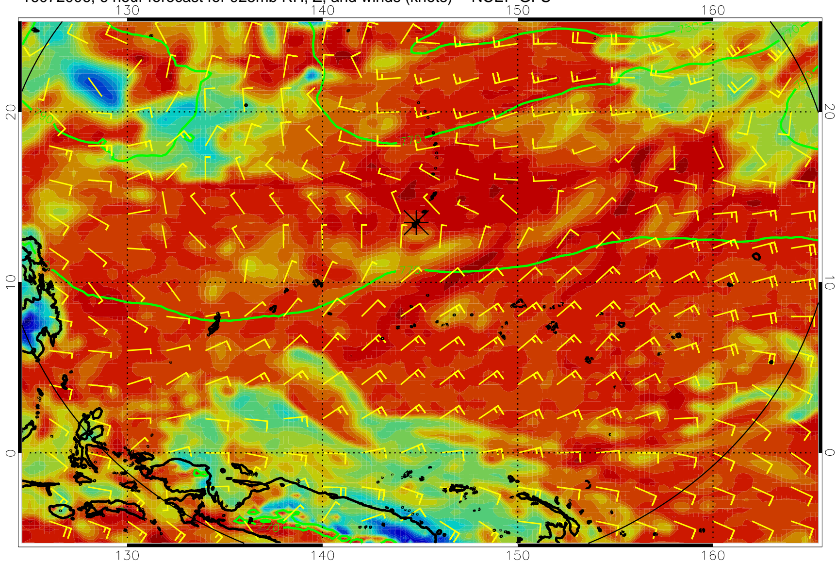
16072006, 6 hour forecast for 925mb RH, Z, and winds (knots) -- NCEP GFS
