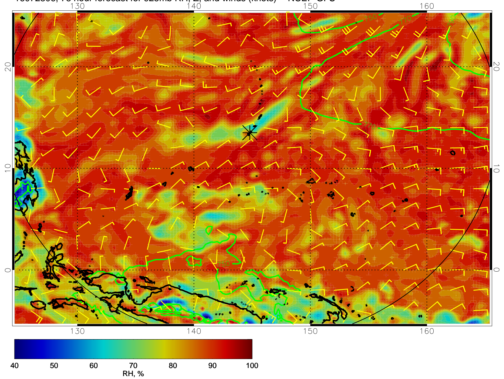
16072306, 78 hour forecast for 925mb RH, Z, and winds (knots) -- NCEP GFS
