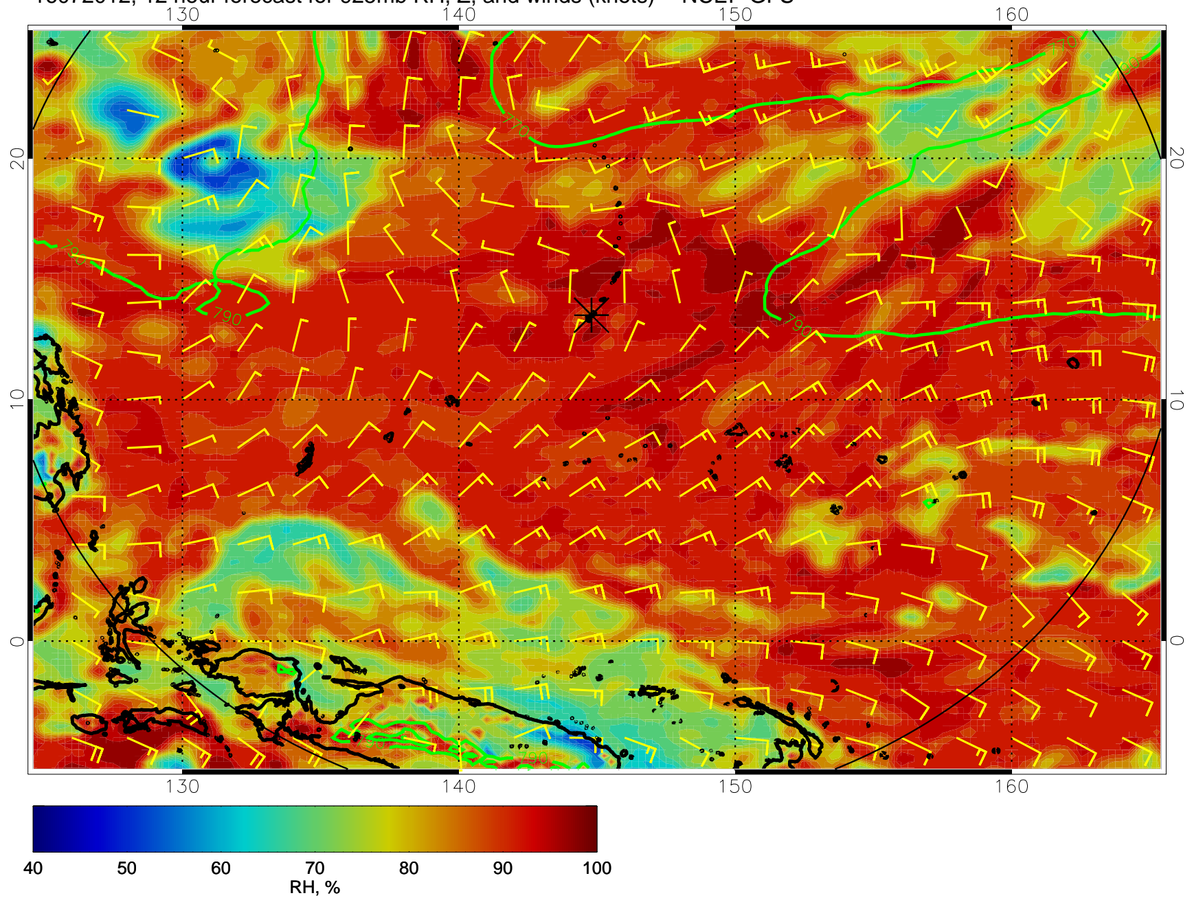
16072012, 12 hour forecast for 925mb RH, Z, and winds (knots) -- NCEP GFS
