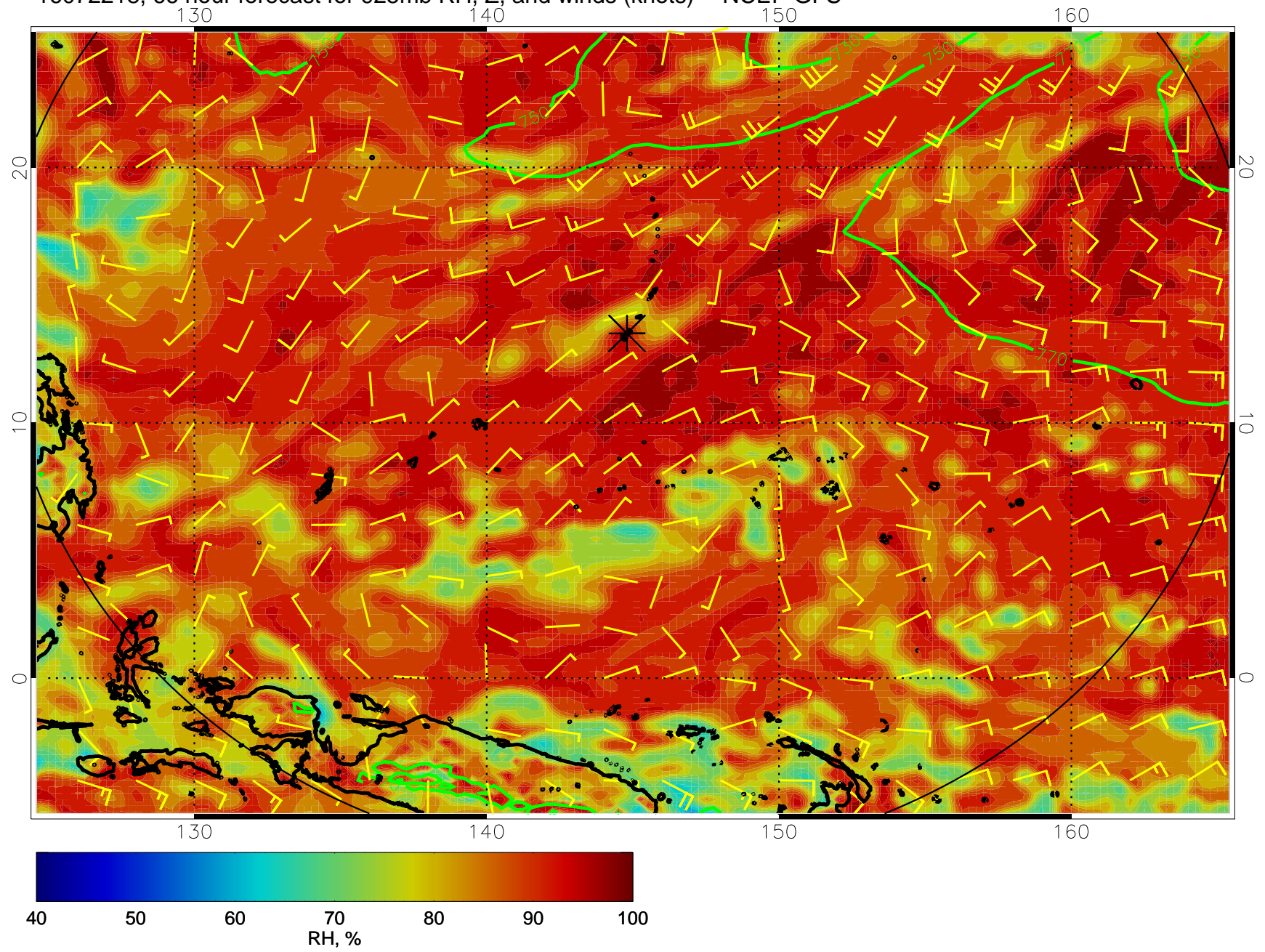
16072218, 66 hour forecast for 925mb RH, Z, and winds (knots) -- NCEP GFS
