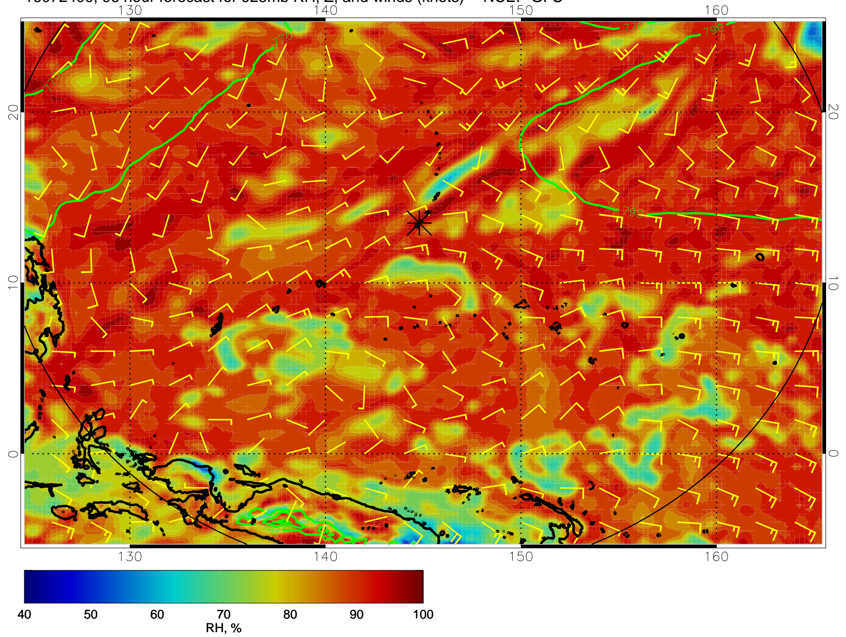
16072400, 96 hour forecast for 925mb RH, Z, and winds (knots) -- NCEP GFS
