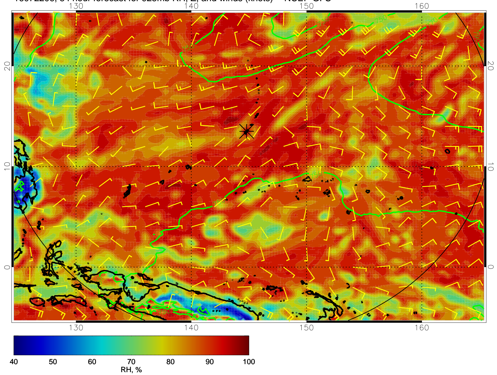
16072206, 54 hour forecast for 925mb RH, Z, and winds (knots) -- NCEP GFS
