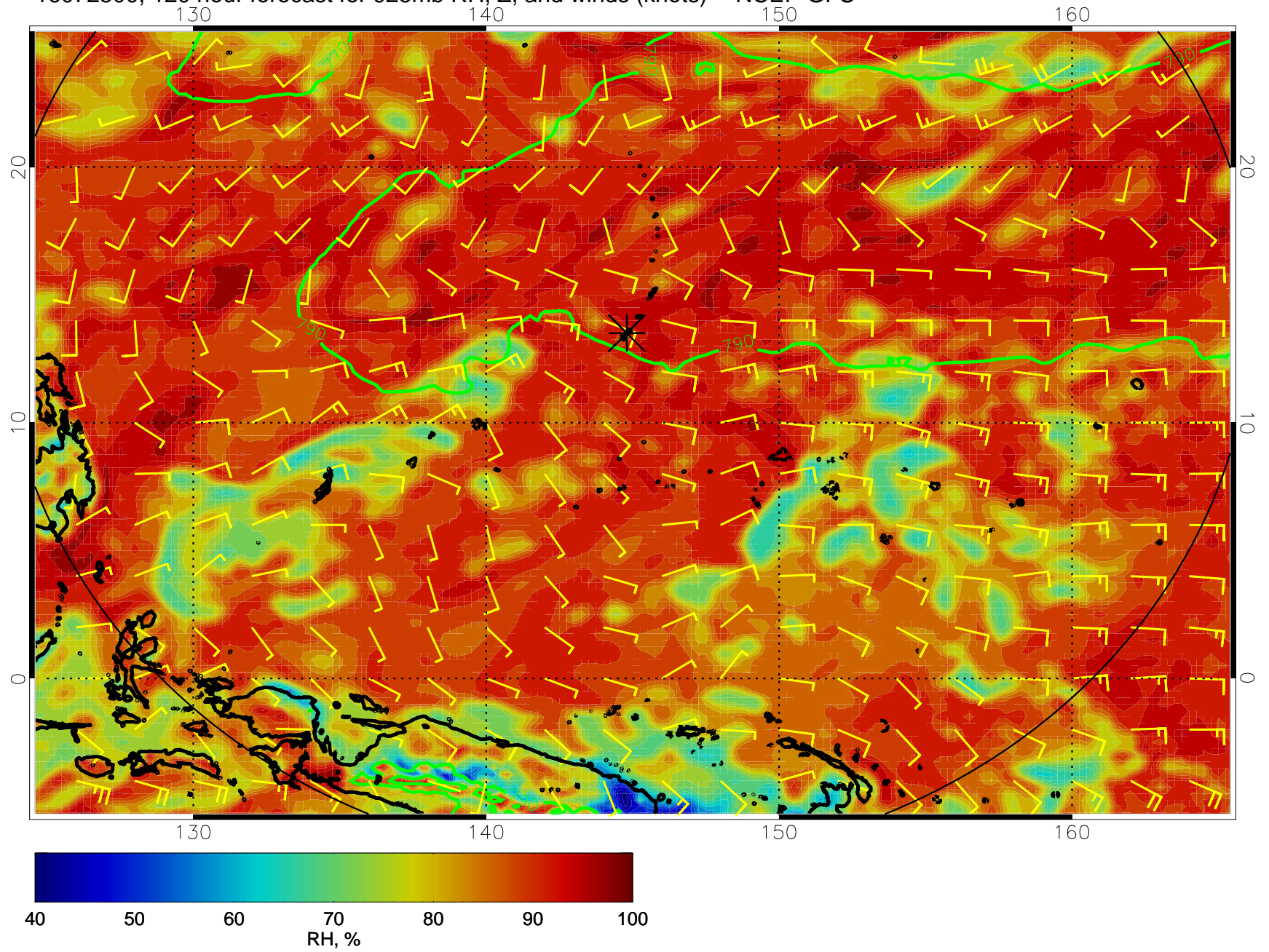
16072500, 120 hour forecast for 925mb RH, Z, and winds (knots) -- NCEP GFS
