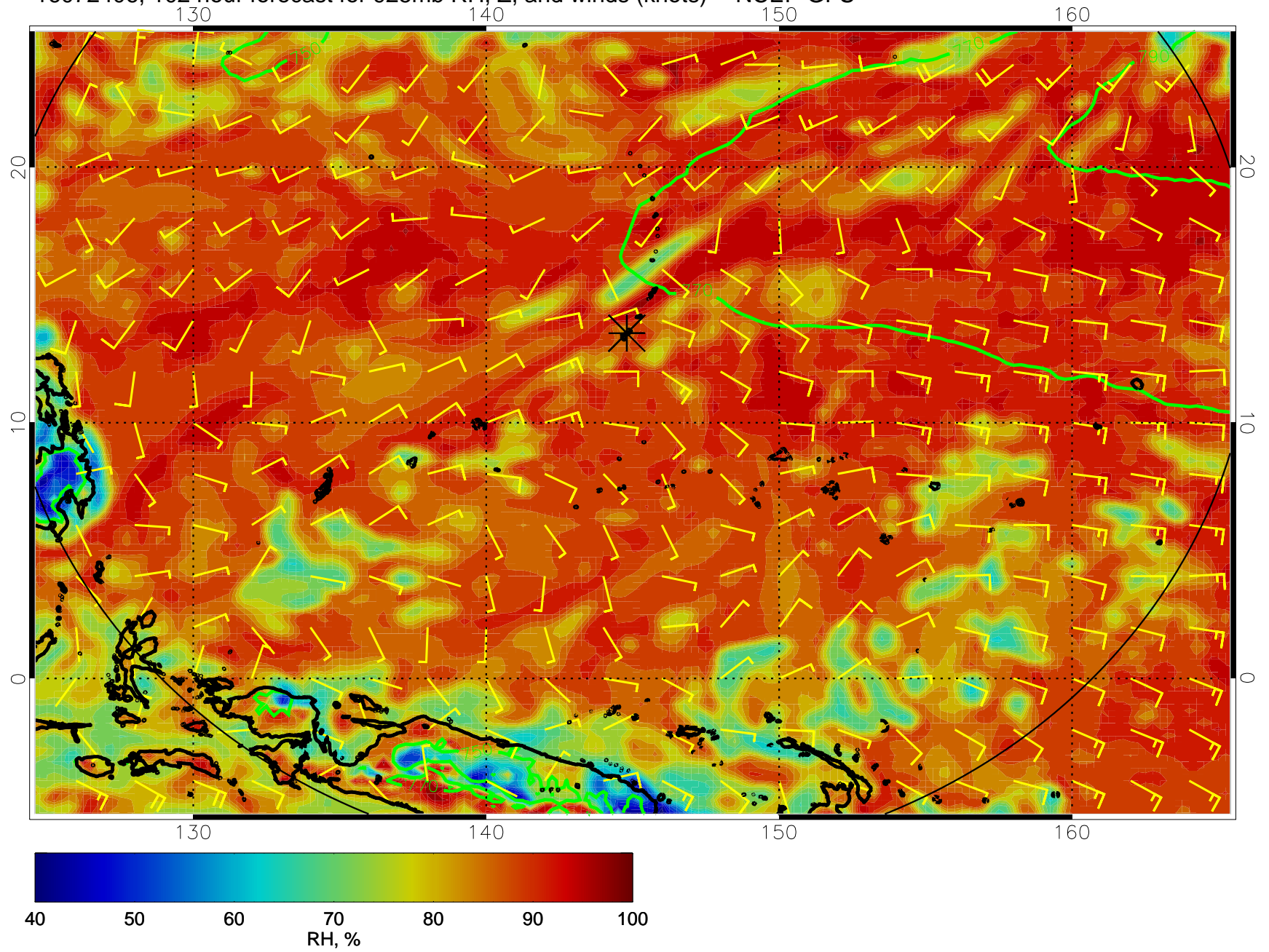
16072406, 102 hour forecast for 925mb RH, Z, and winds (knots) -- NCEP GFS
