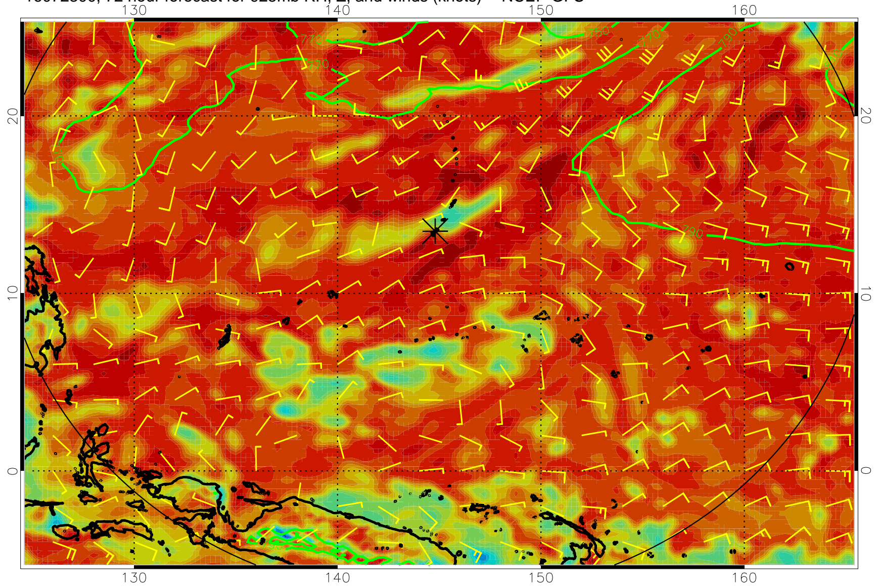
16072300, 72 hour forecast for 925mb RH, Z, and winds (knots) -- NCEP GFS
