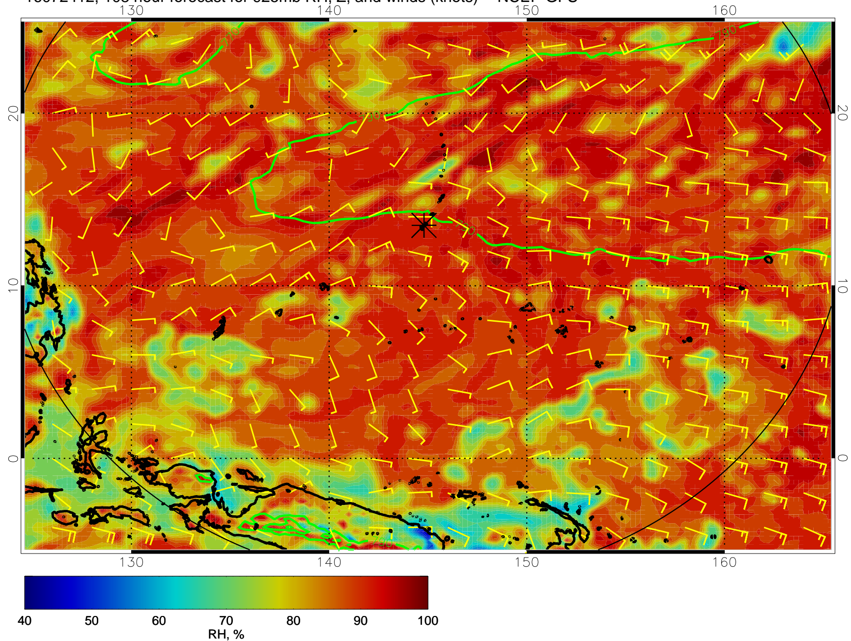
16072412, 108 hour forecast for 925mb RH, Z, and winds (knots) -- NCEP GFS
