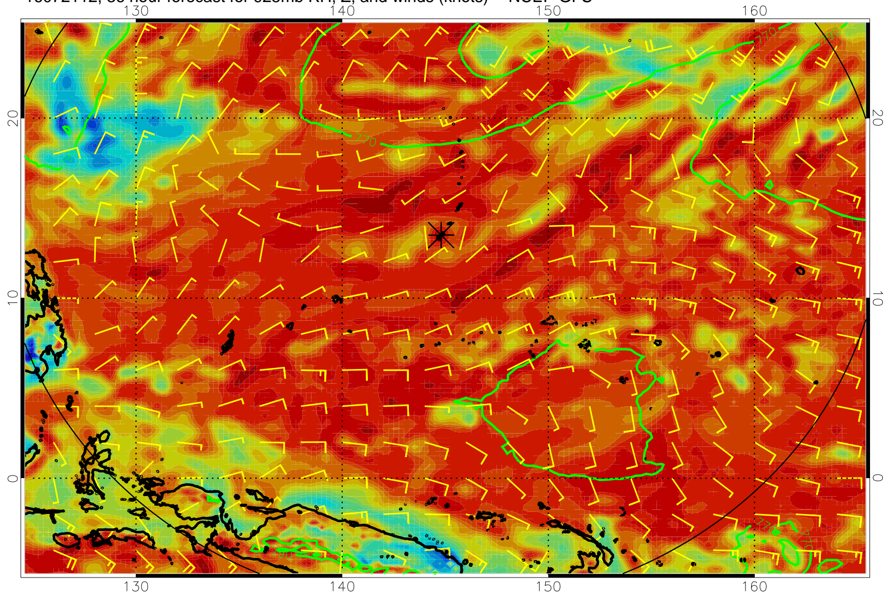
16072112, 36 hour forecast for 925mb RH, Z, and winds (knots) -- NCEP GFS
