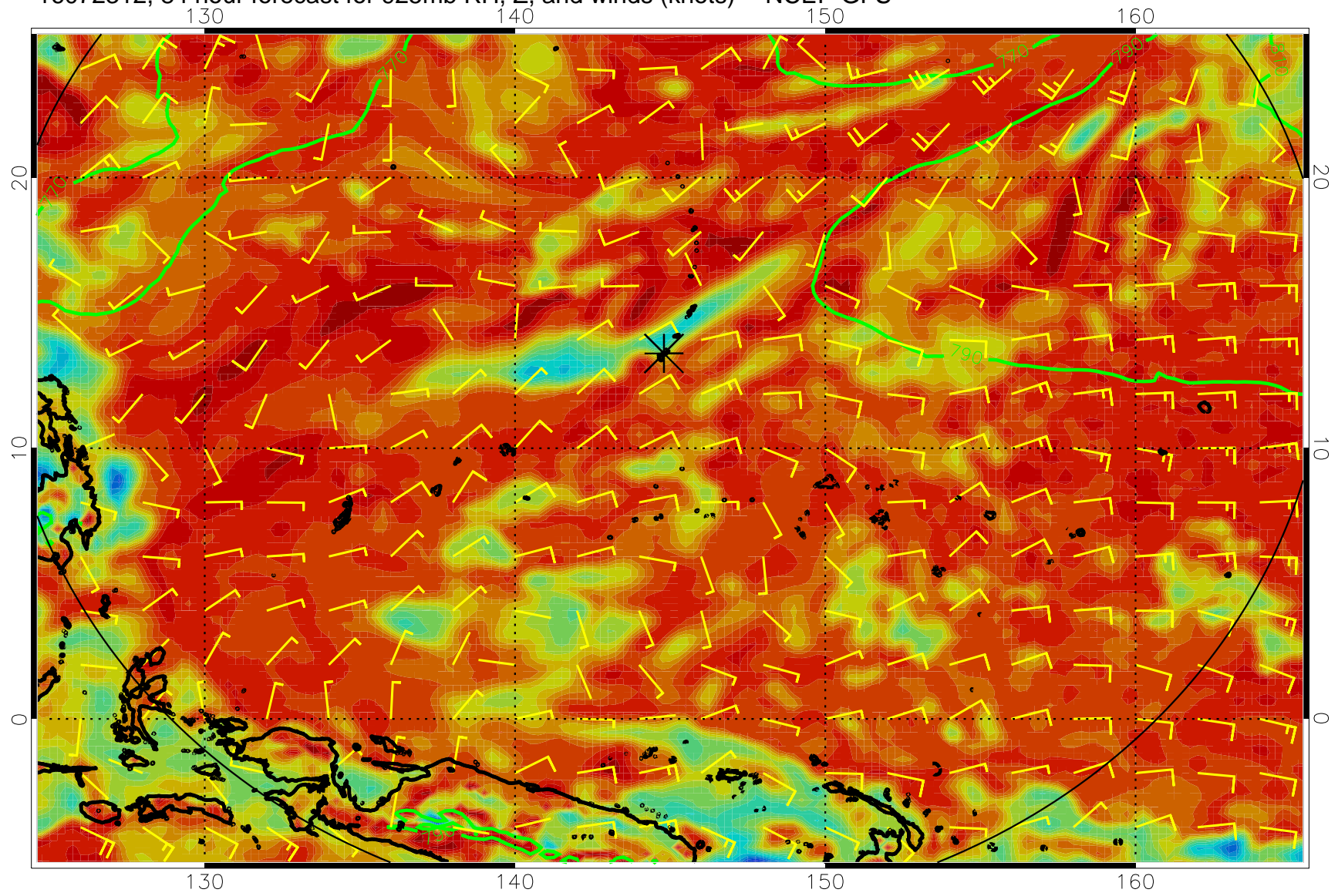
16072312, 84 hour forecast for 925mb RH, Z, and winds (knots) -- NCEP GFS
