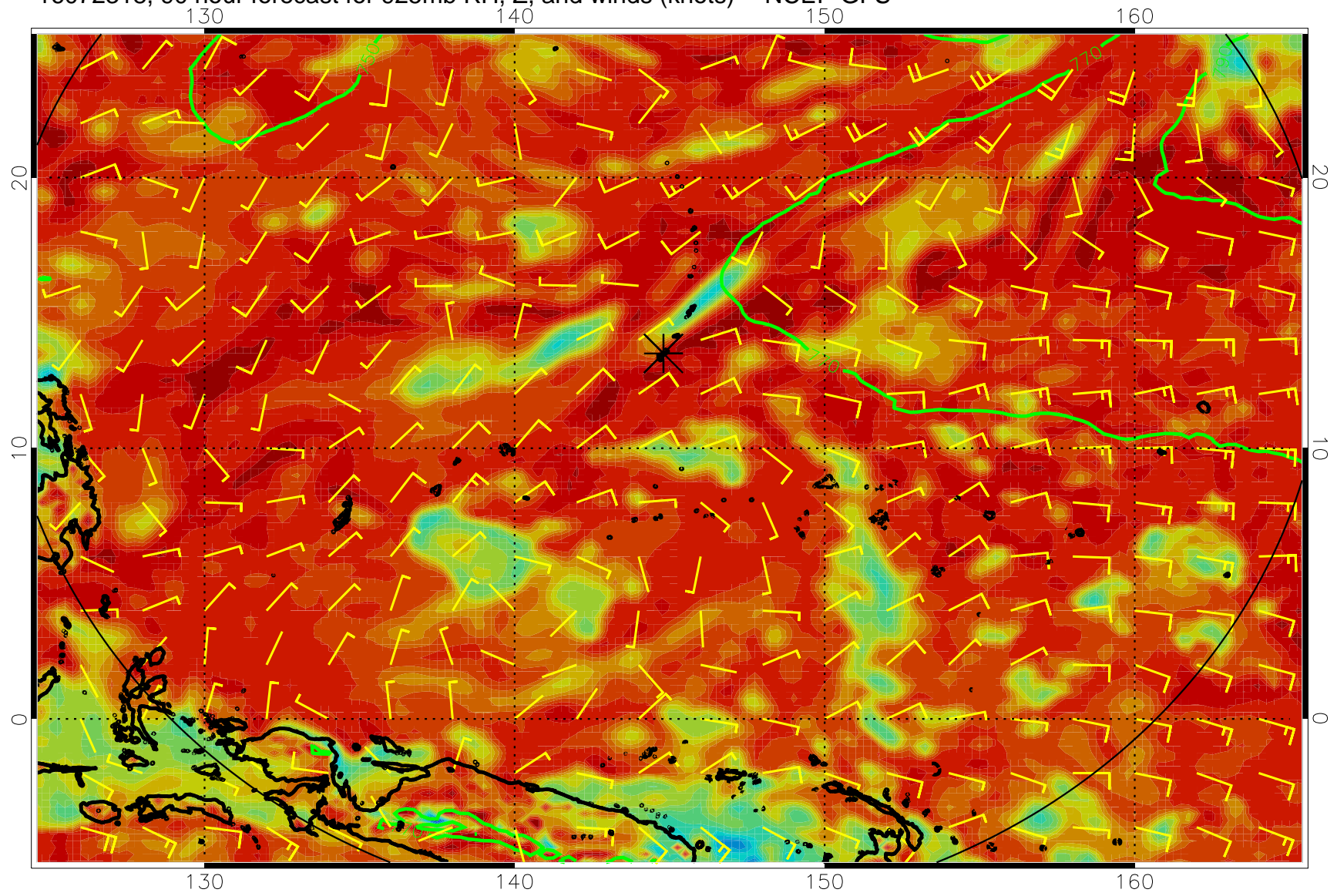
16072318, 90 hour forecast for 925mb RH, Z, and winds (knots) -- NCEP GFS
