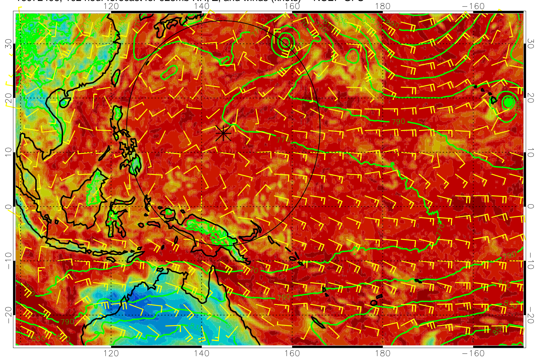
16072406, 102 hour forecast for 925mb RH, Z, and winds (knots) -- NCEP GFS
