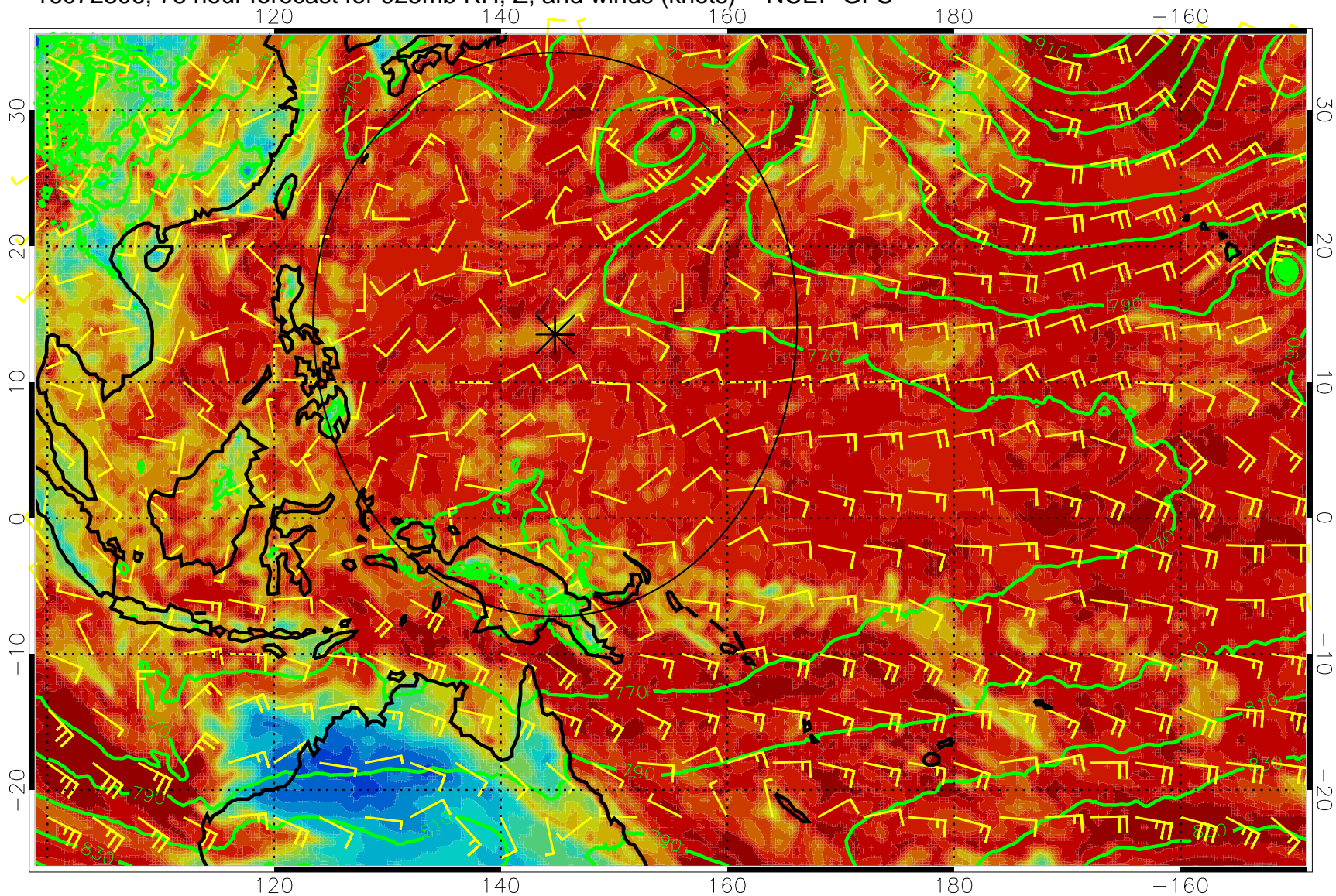
16072306, 78 hour forecast for 925mb RH, Z, and winds (knots) -- NCEP GFS
