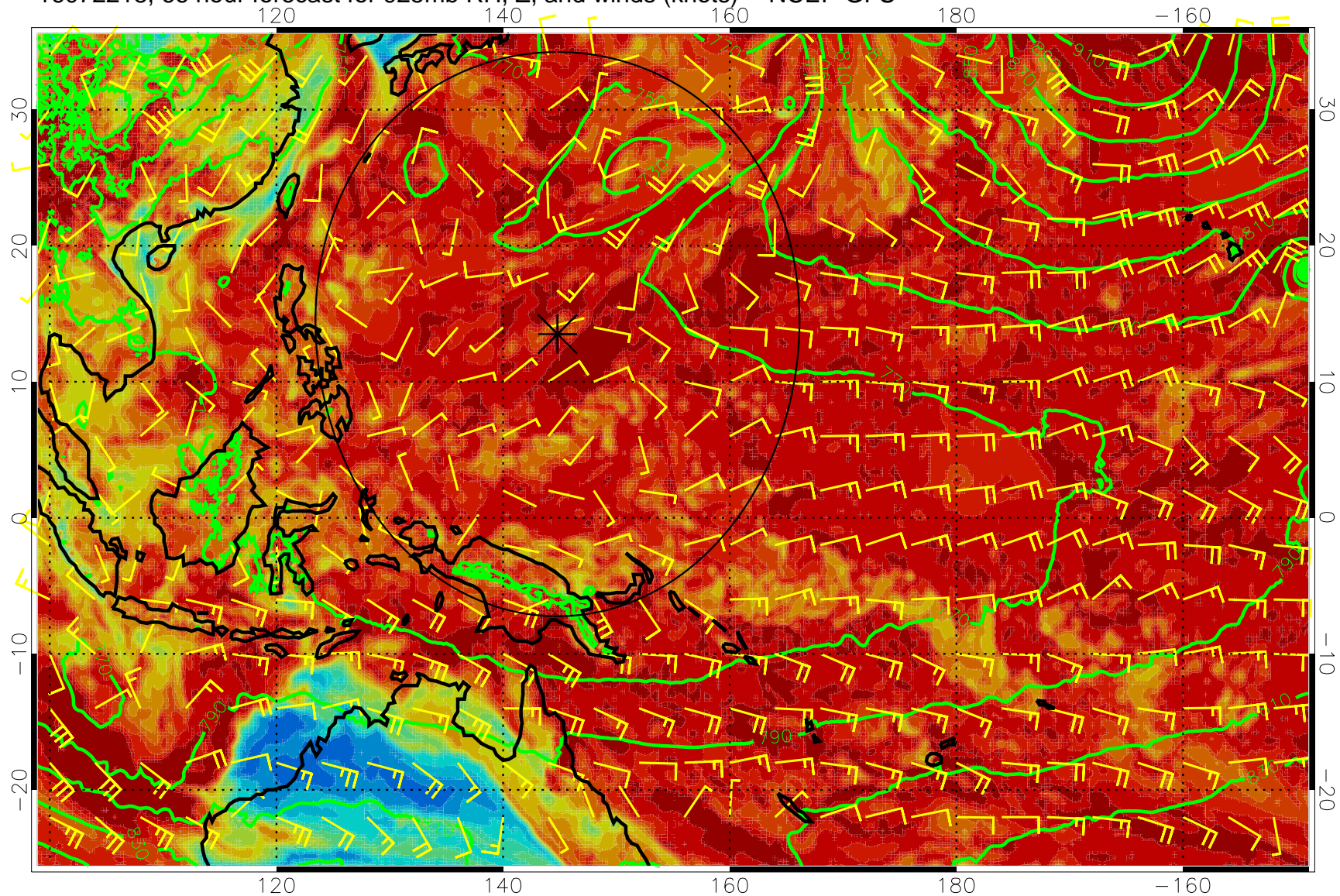
16072218, 66 hour forecast for 925mb RH, Z, and winds (knots) -- NCEP GFS
