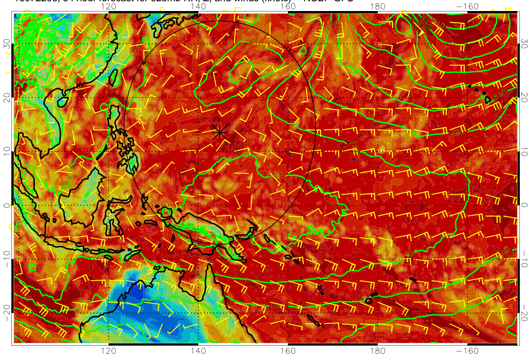
16072206, 54 hour forecast for 925mb RH, Z, and winds (knots) -- NCEP GFS
