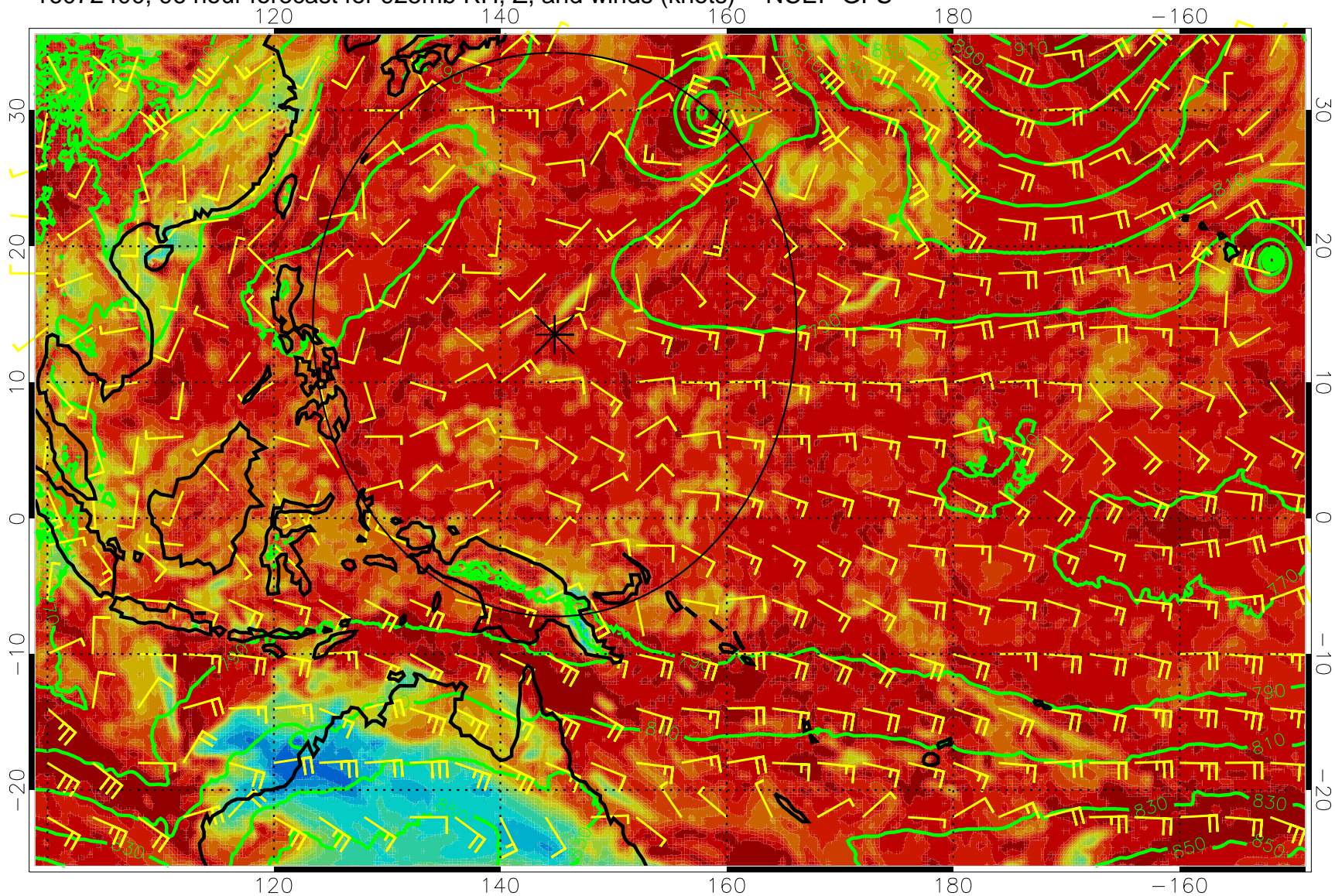
16072400, 96 hour forecast for 925mb RH, Z, and winds (knots) -- NCEP GFS
