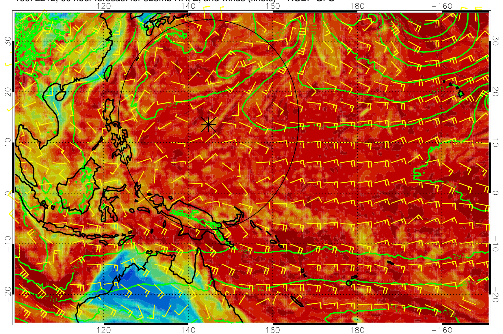
16072212, 60 hour forecast for 925mb RH, Z, and winds (knots) -- NCEP GFS
