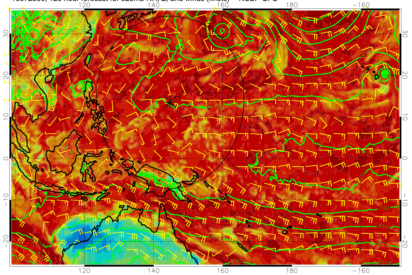
16072500, 120 hour forecast for 925mb RH, Z, and winds (knots) -- NCEP GFS
