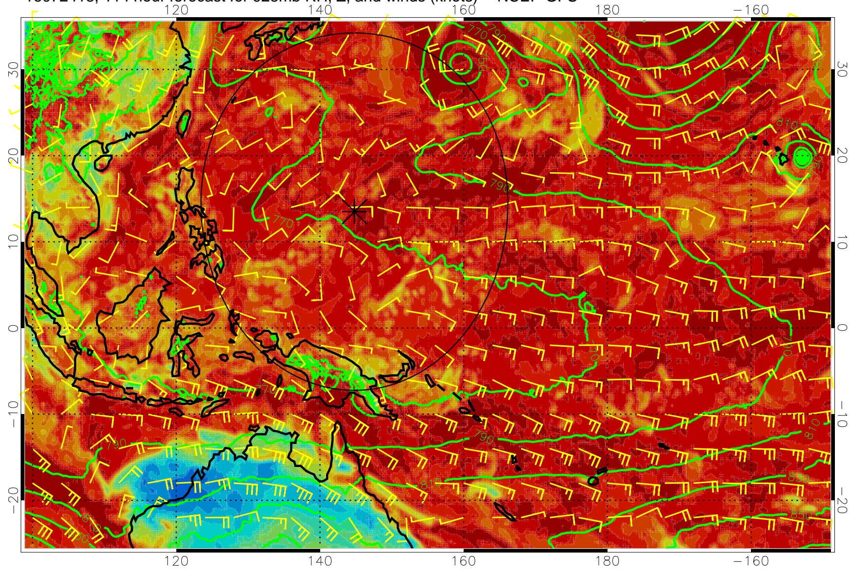
16072418, 114 hour forecast for 925mb RH, Z, and winds (knots) -- NCEP GFS
