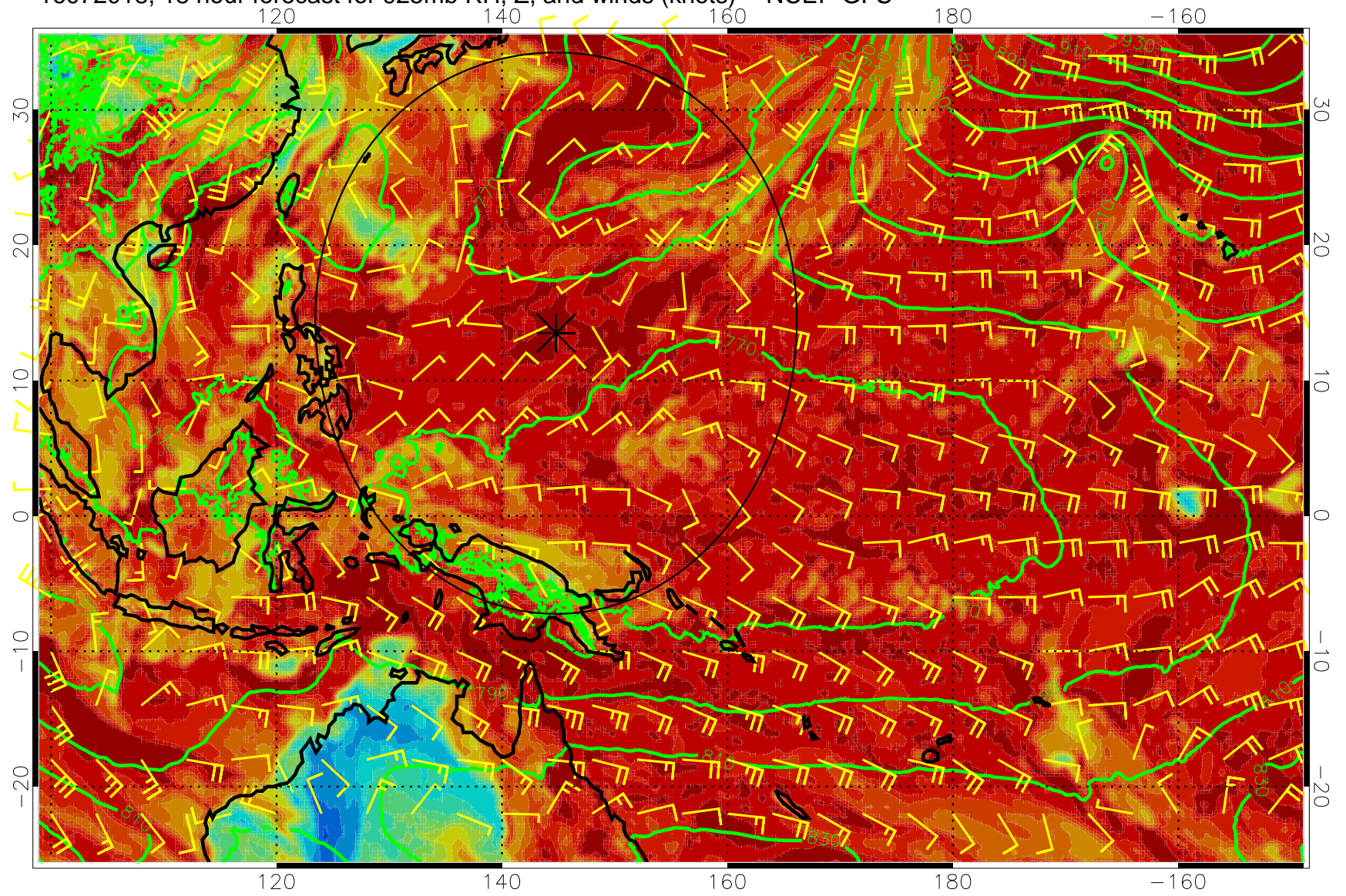
16072018, 18 hour forecast for 925mb RH, Z, and winds (knots) -- NCEP GFS
