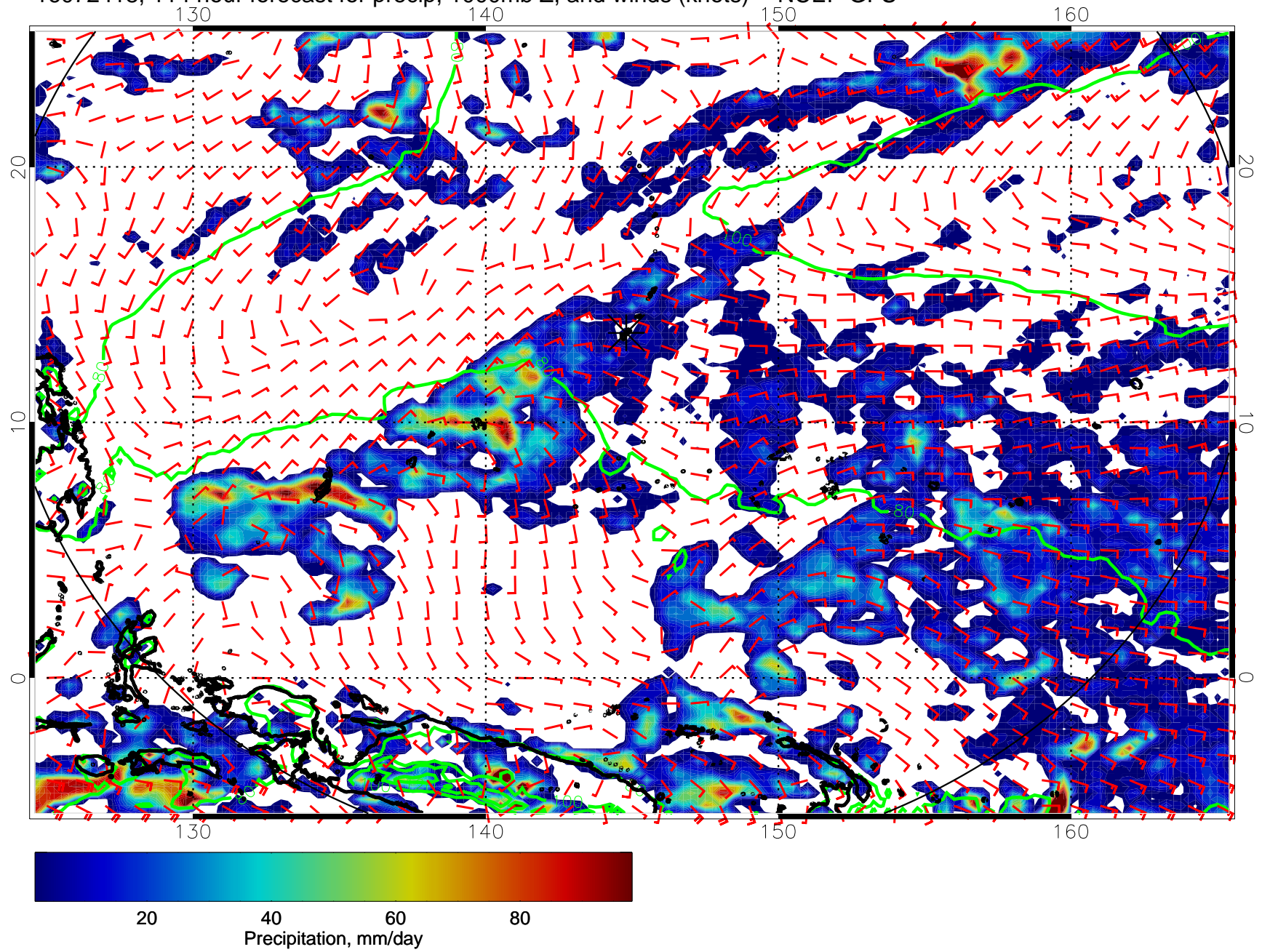
16072418, 114 hour forecast for precip, 1000mb Z, and winds (knots) -- NCEP GFS
