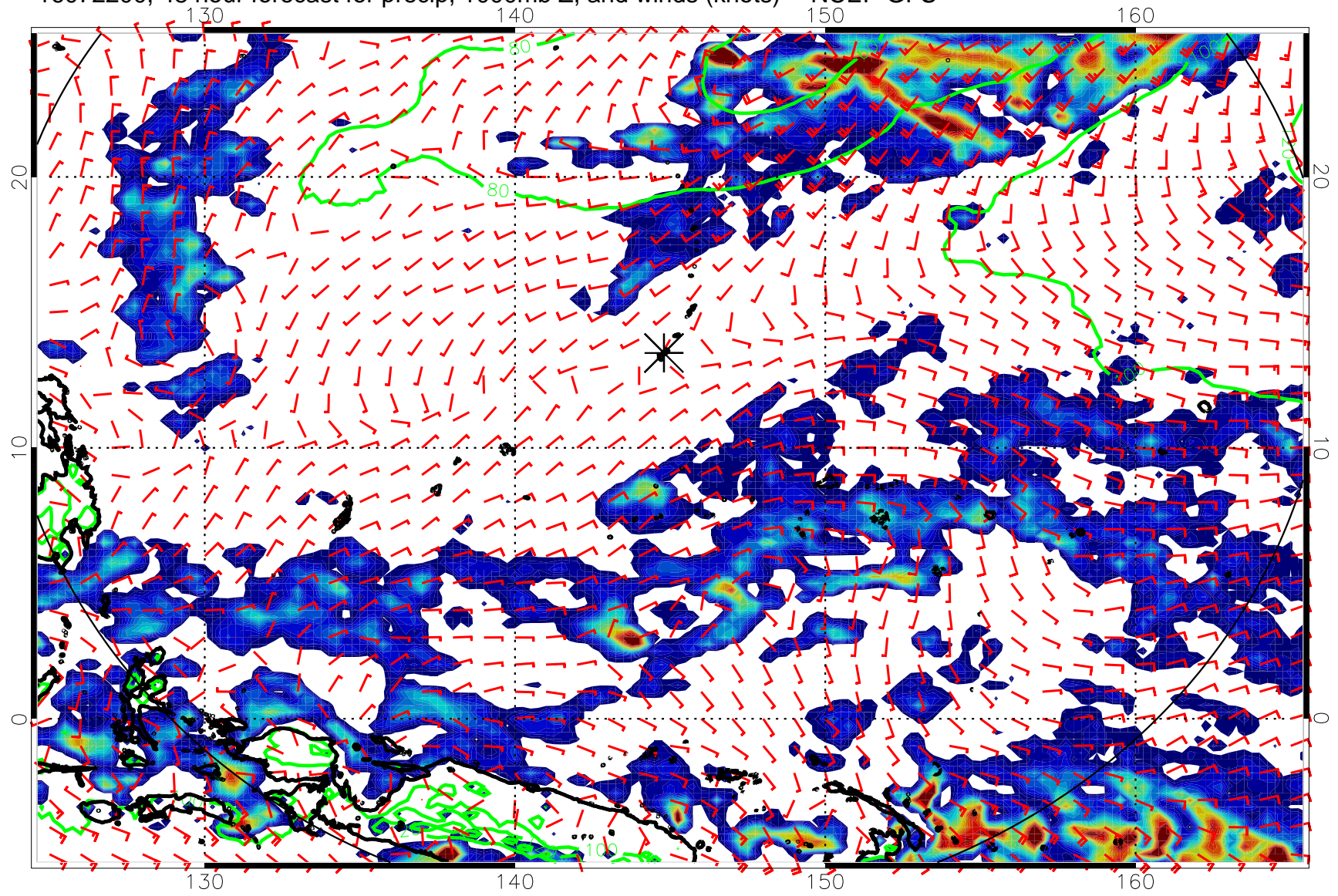
16072200, 48 hour forecast for precip, 1000mb Z, and winds (knots) -- NCEP GFS
