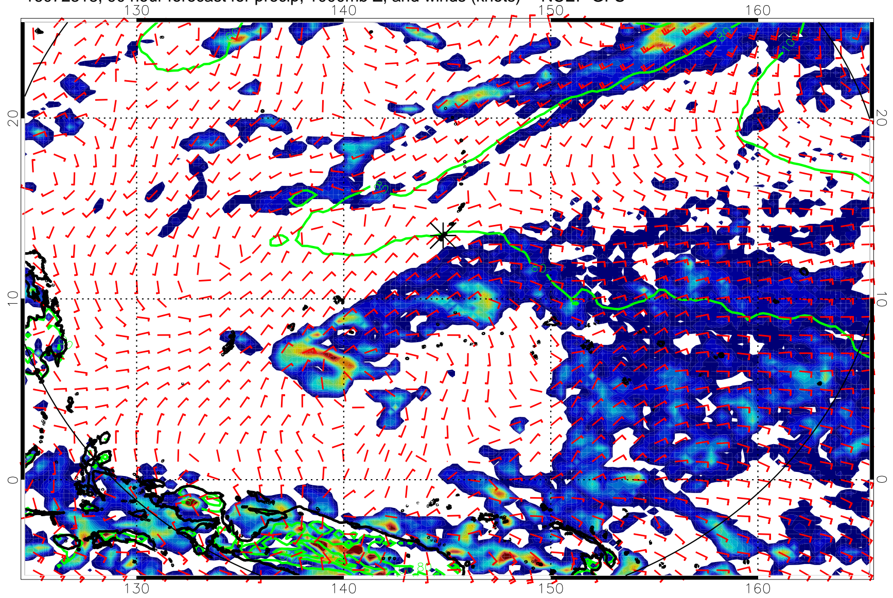
16072318, 90 hour forecast for precip, 1000mb Z, and winds (knots) -- NCEP GFS
