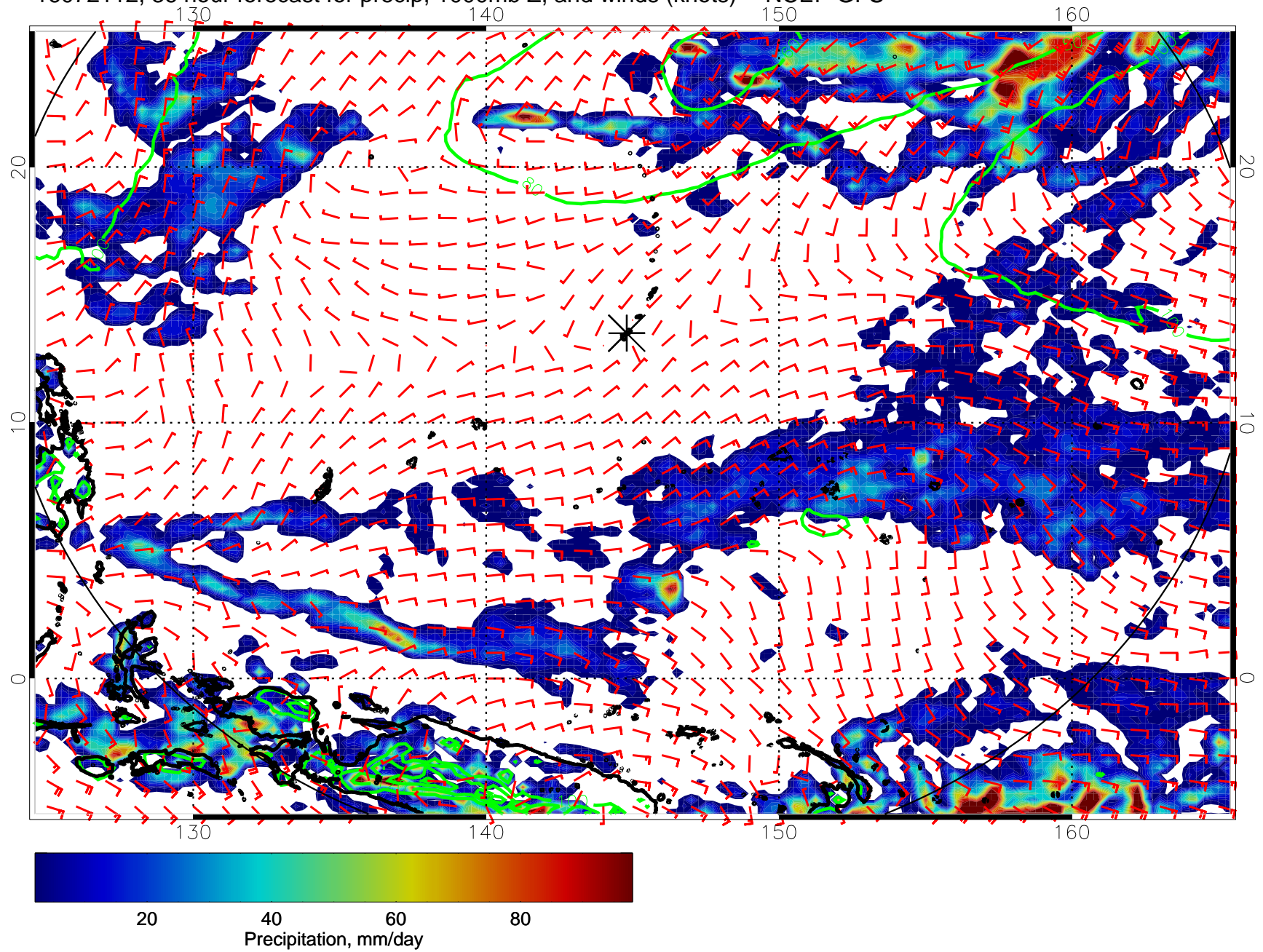
16072112, 36 hour forecast for precip, 1000mb Z, and winds (knots) -- NCEP GFS
