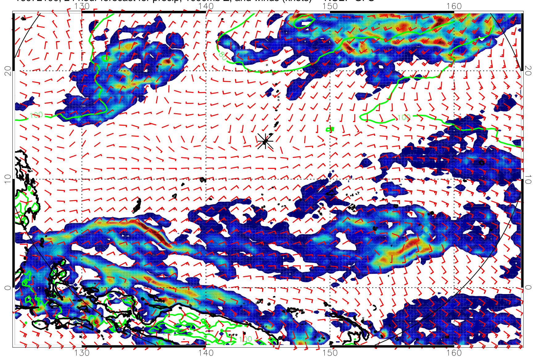
16072100, 24 hour forecast for precip, 1000mb Z, and winds (knots) -- NCEP GFS
