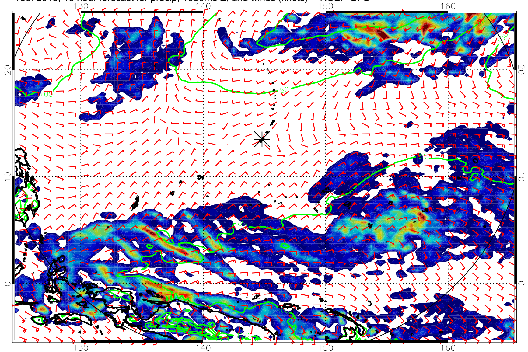
16072018, 18 hour forecast for precip, 1000mb Z, and winds (knots) -- NCEP GFS
