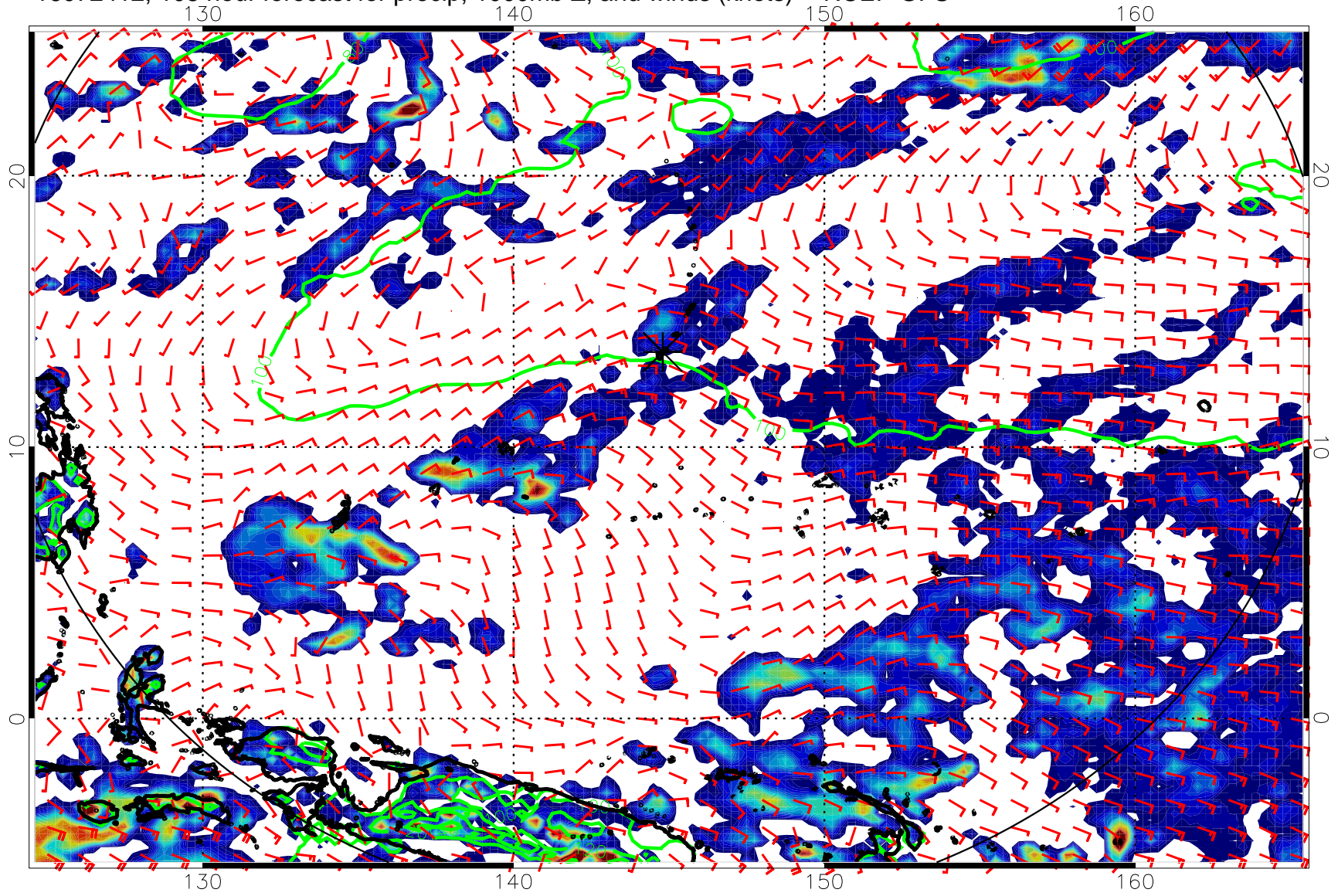
16072412, 108 hour forecast for precip, 1000mb Z, and winds (knots) -- NCEP GFS
