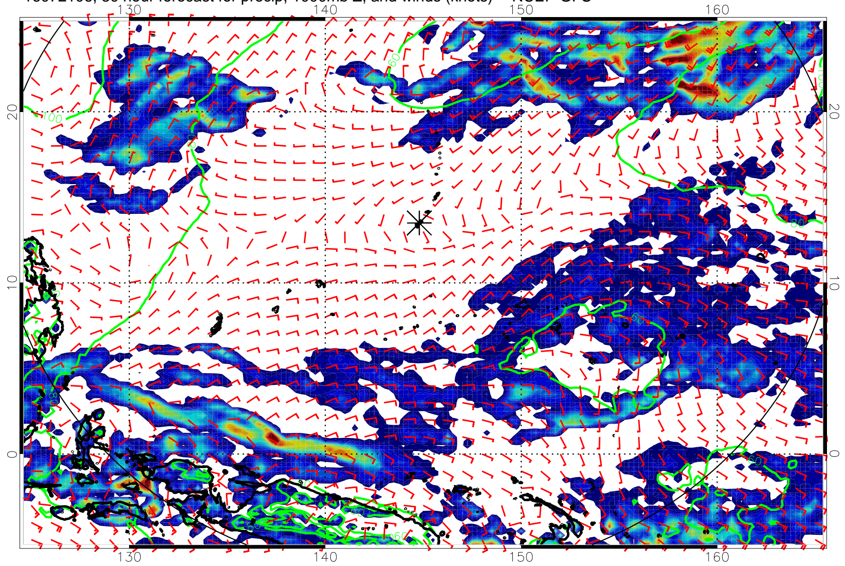
16072106, 30 hour forecast for precip, 1000mb Z, and winds (knots) -- NCEP GFS
