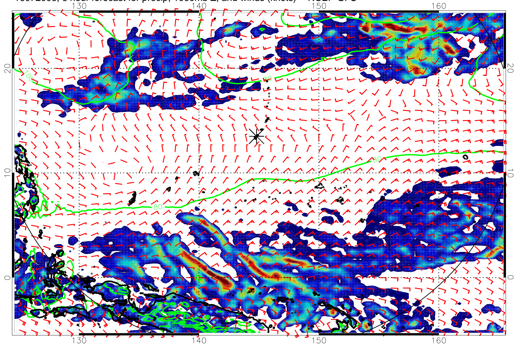
16072006, 6 hour forecast for precip, 1000mb Z, and winds (knots) -- NCEP GFS
