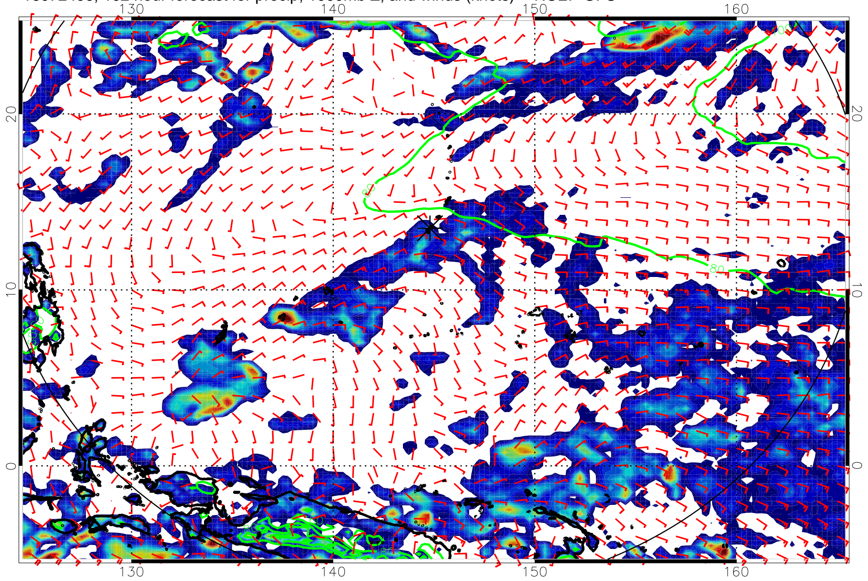
16072406, 102 hour forecast for precip, 1000mb Z, and winds (knots) -- NCEP GFS
