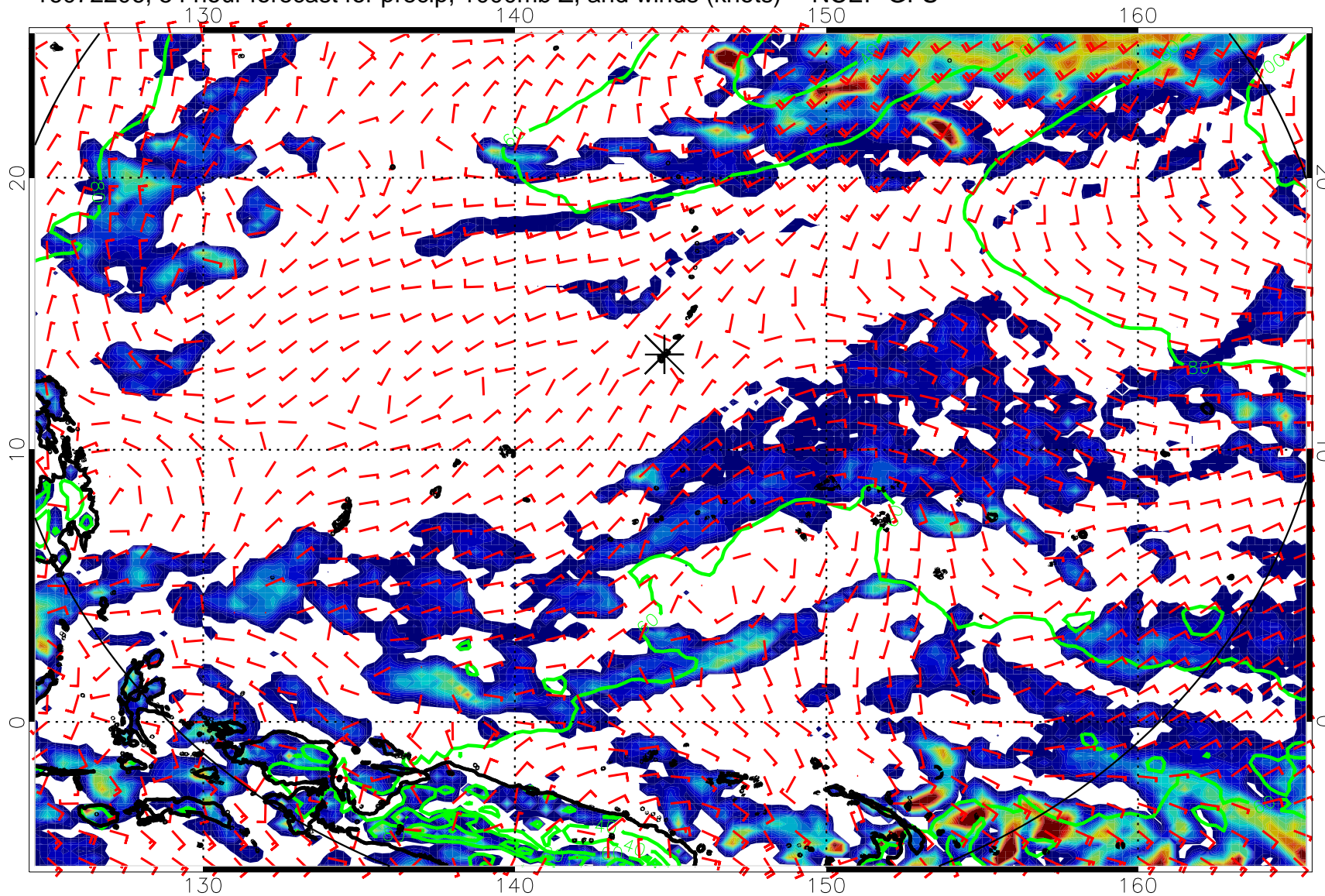
16072206, 54 hour forecast for precip, 1000mb Z, and winds (knots) -- NCEP GFS
