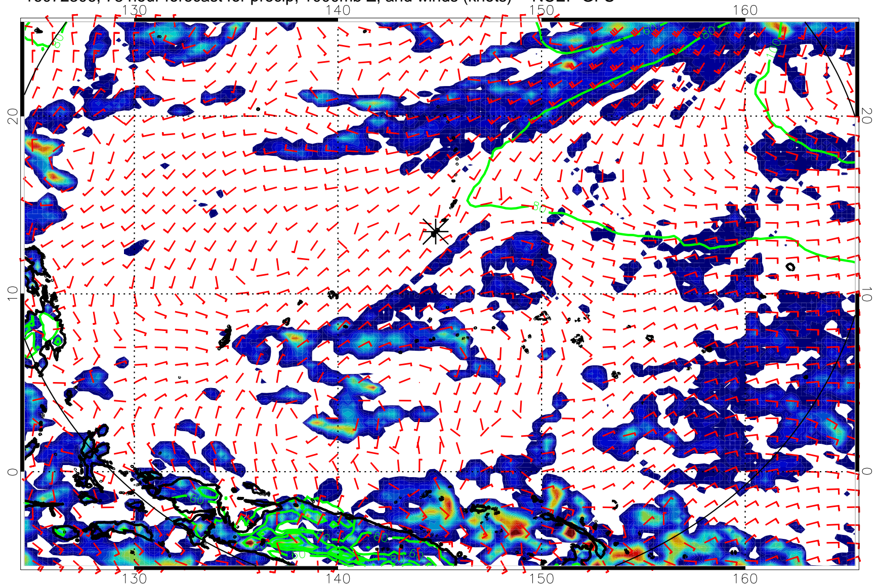
16072306, 78 hour forecast for precip, 1000mb Z, and winds (knots) -- NCEP GFS
