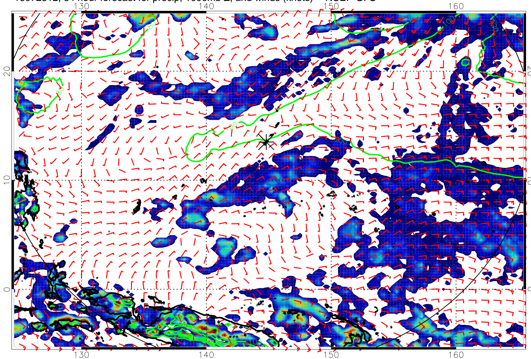
16072312, 84 hour forecast for precip, 1000mb Z, and winds (knots) -- NCEP GFS
