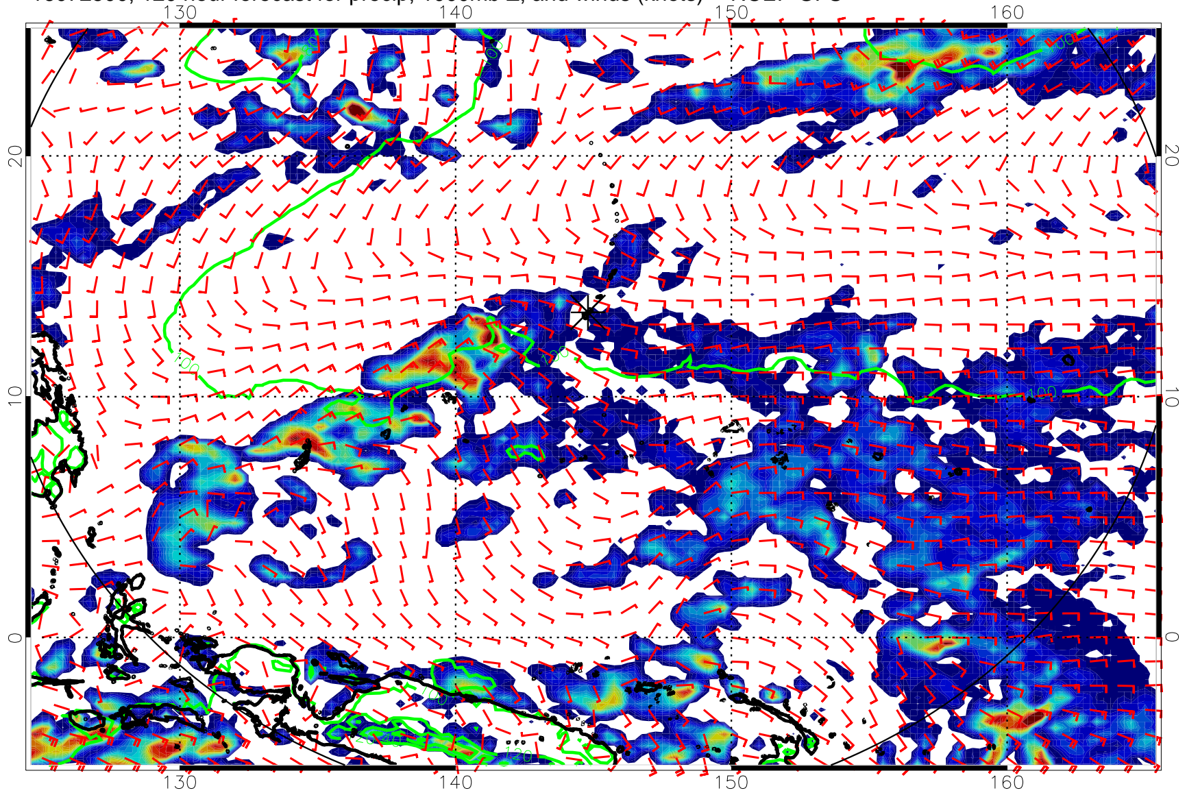
16072500, 120 hour forecast for precip, 1000mb Z, and winds (knots) -- NCEP GFS
