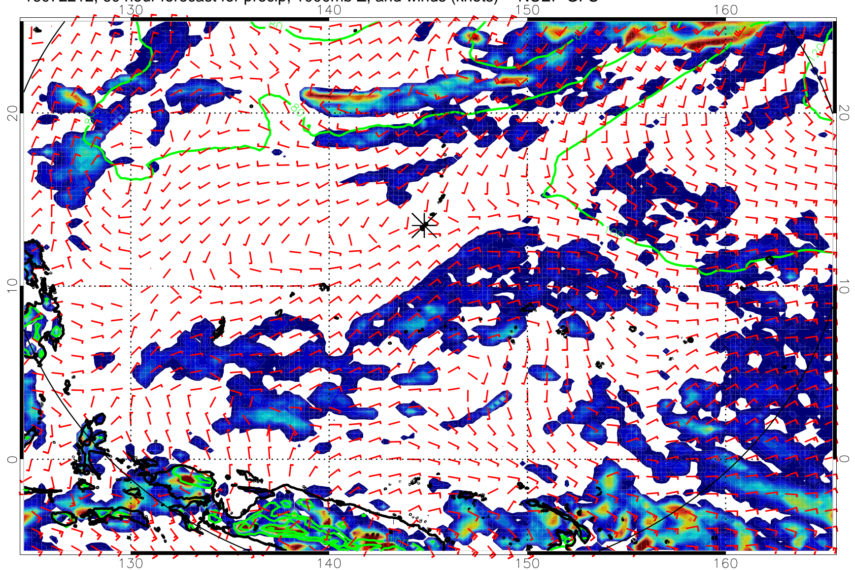
16072212, 60 hour forecast for precip, 1000mb Z, and winds (knots) -- NCEP GFS
