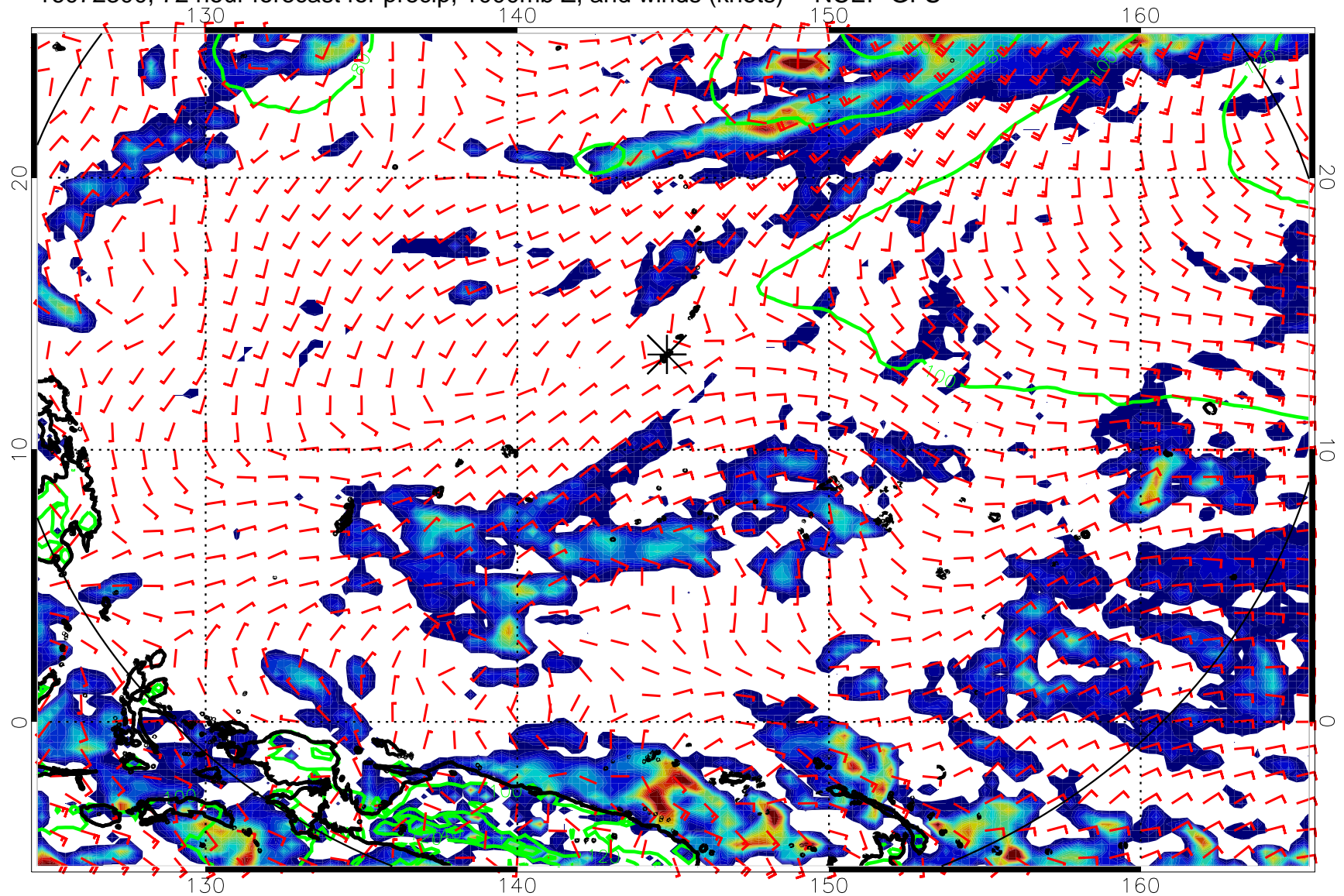
16072300, 72 hour forecast for precip, 1000mb Z, and winds (knots) -- NCEP GFS
