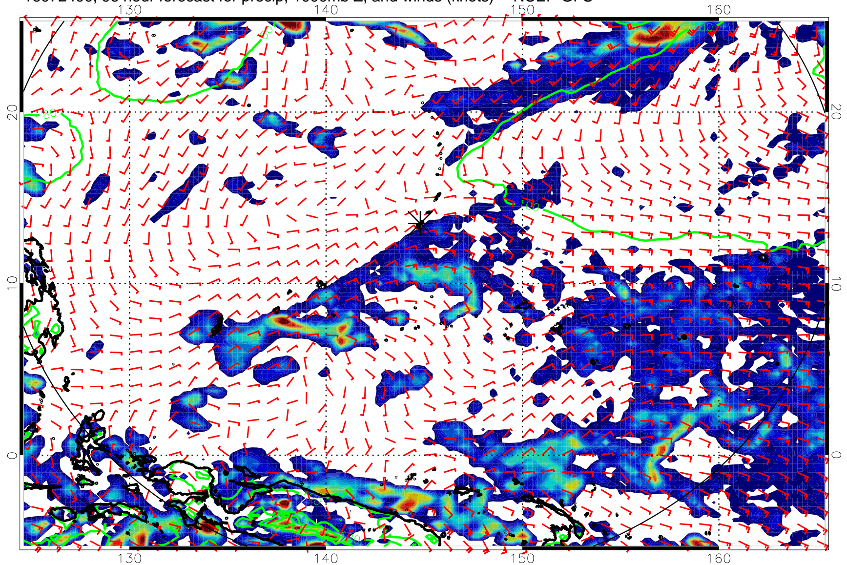
16072400, 96 hour forecast for precip, 1000mb Z, and winds (knots) -- NCEP GFS
