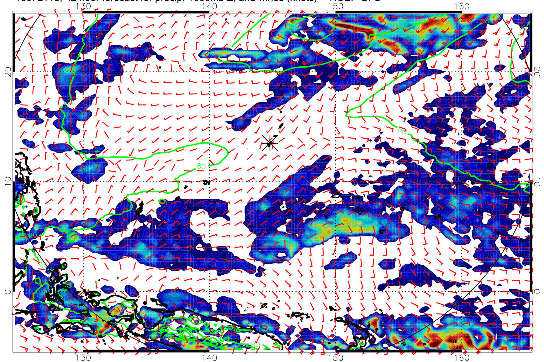
16072118, 42 hour forecast for precip, 1000mb Z, and winds (knots) -- NCEP GFS
