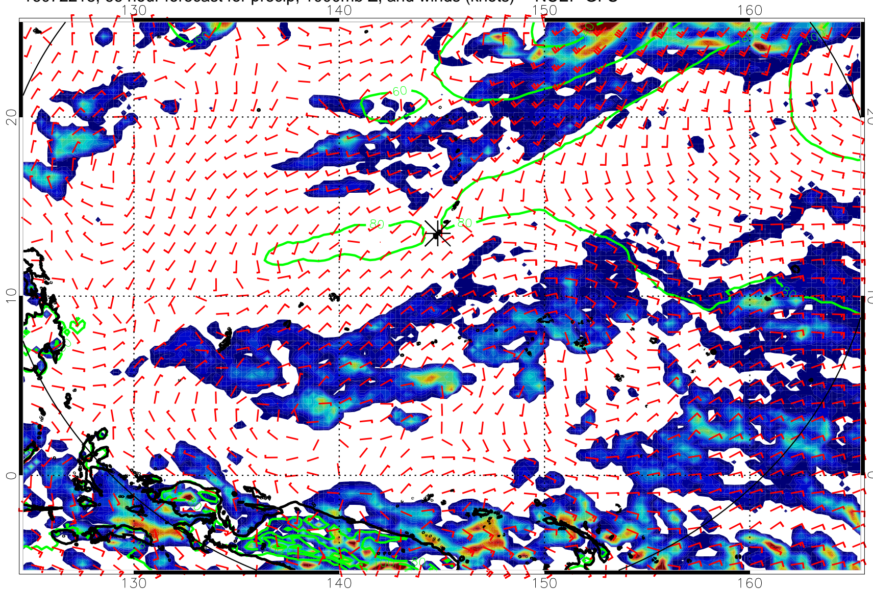
16072218, 66 hour forecast for precip, 1000mb Z, and winds (knots) -- NCEP GFS
