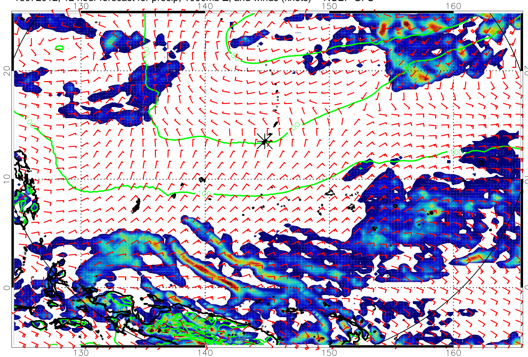
16072012, 12 hour forecast for precip, 1000mb Z, and winds (knots) -- NCEP GFS
