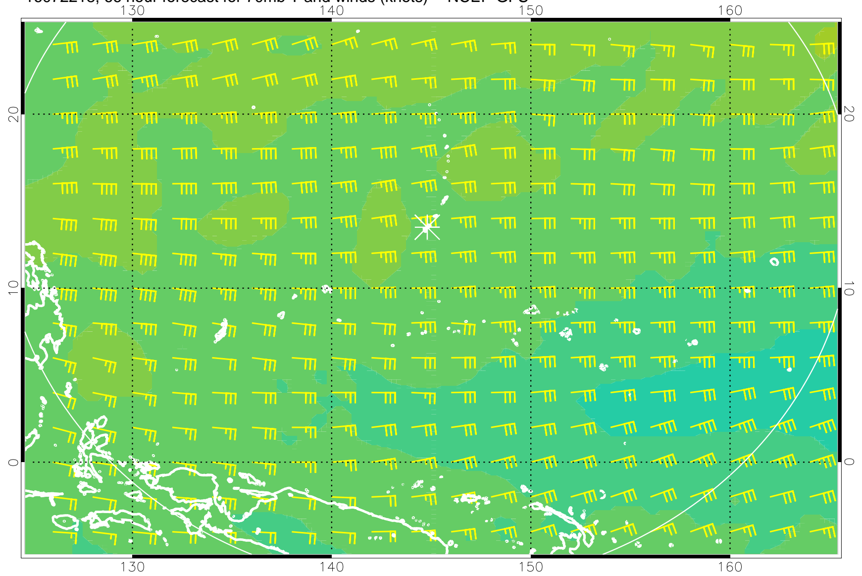
16072218, 66 hour forecast for 70mb T and winds (knots) -- NCEP GFS
