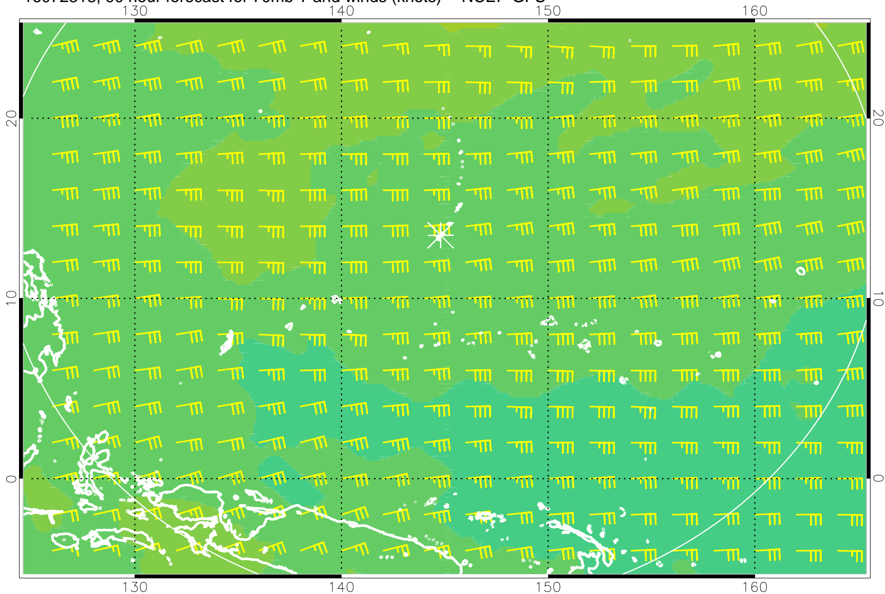
16072318, 90 hour forecast for 70mb T and winds (knots) -- NCEP GFS
