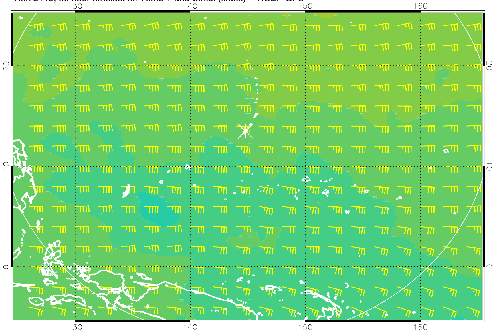
16072112, 36 hour forecast for 70mb T and winds (knots) -- NCEP GFS
