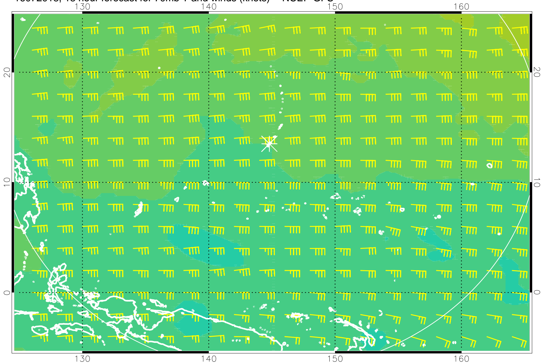
16072018, 18 hour forecast for 70mb T and winds (knots) -- NCEP GFS
