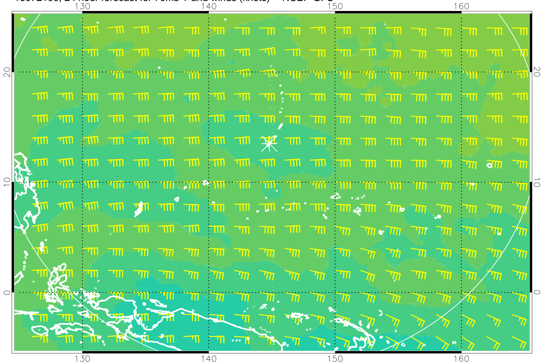
16072100, 24 hour forecast for 70mb T and winds (knots) -- NCEP GFS
