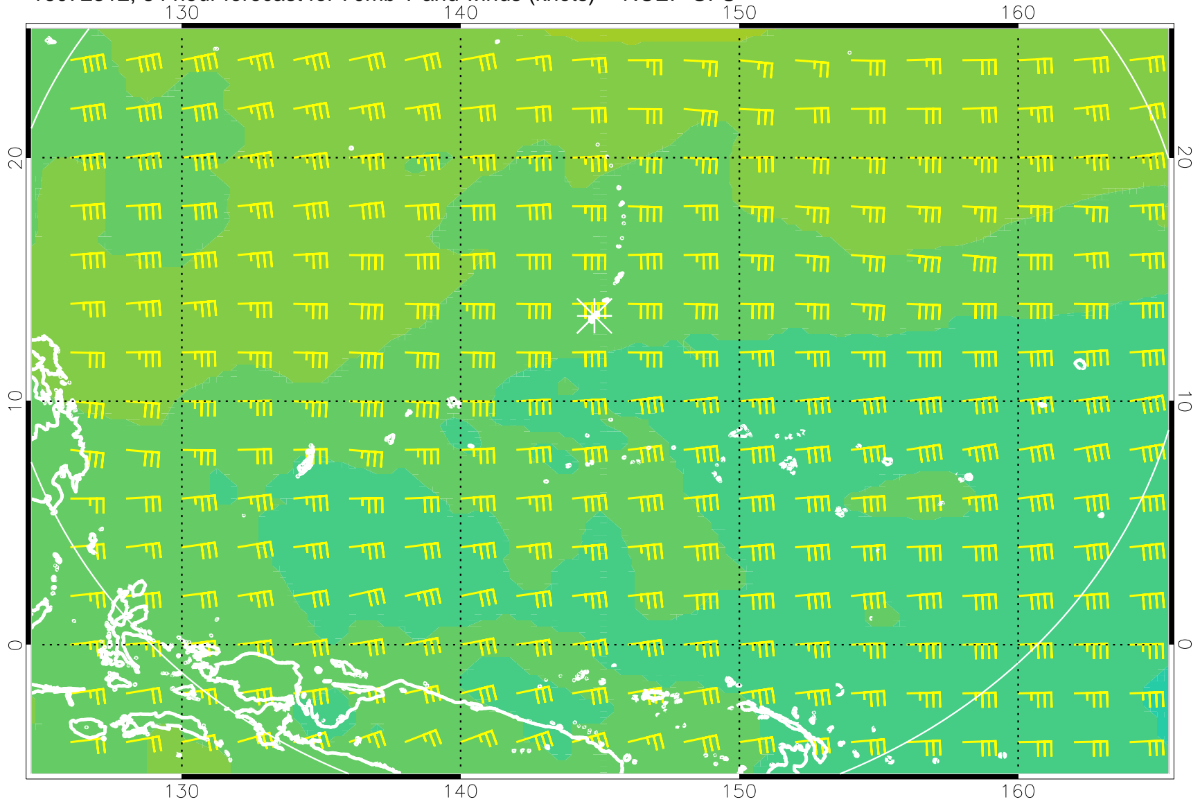
16072312, 84 hour forecast for 70mb T and winds (knots) -- NCEP GFS
