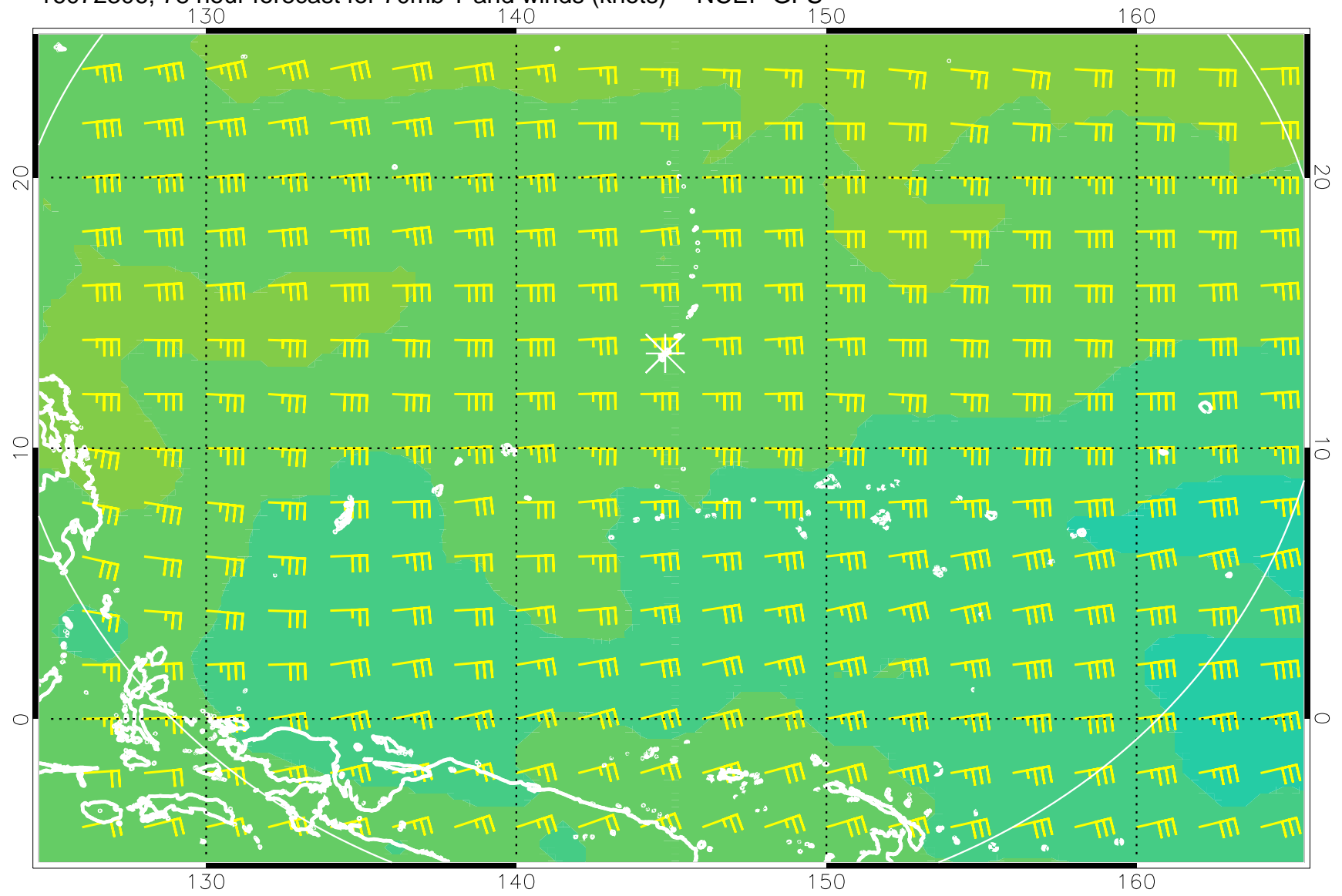
16072306, 78 hour forecast for 70mb T and winds (knots) -- NCEP GFS
