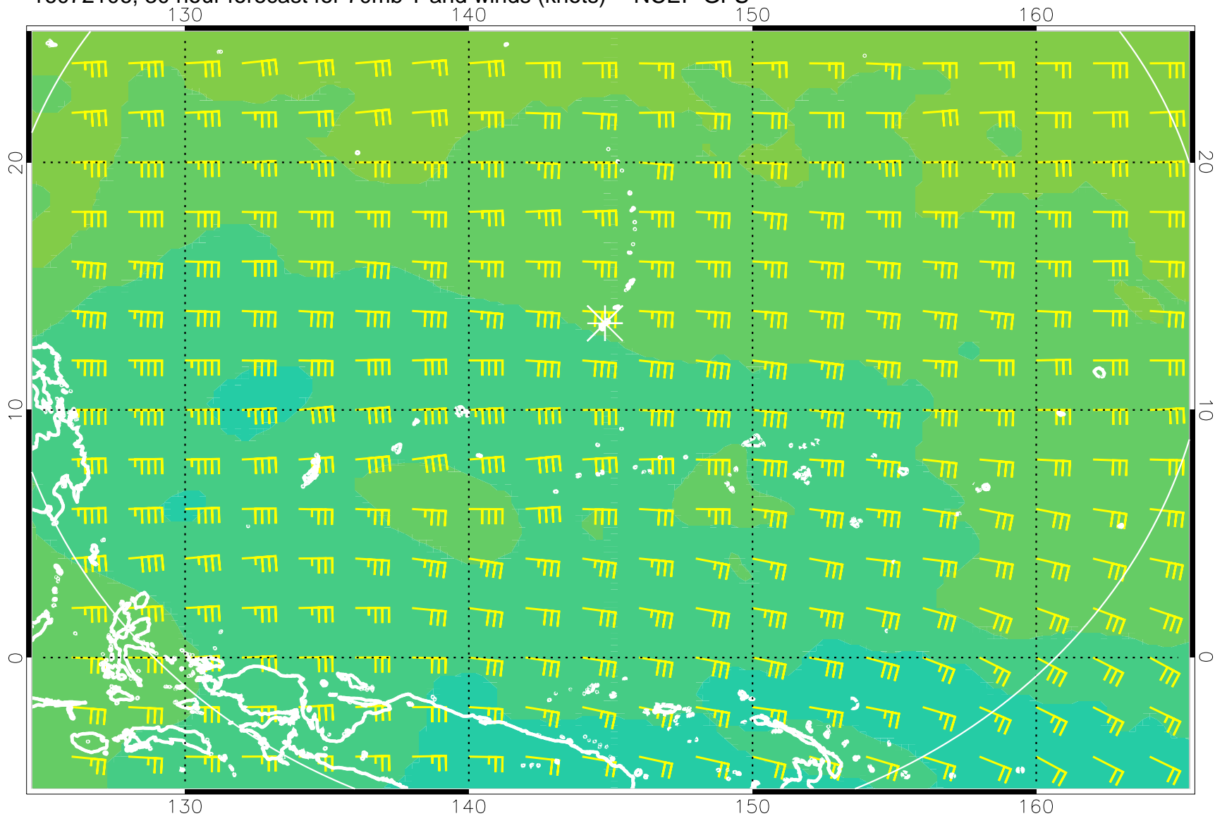
16072106, 30 hour forecast for 70mb T and winds (knots) -- NCEP GFS
