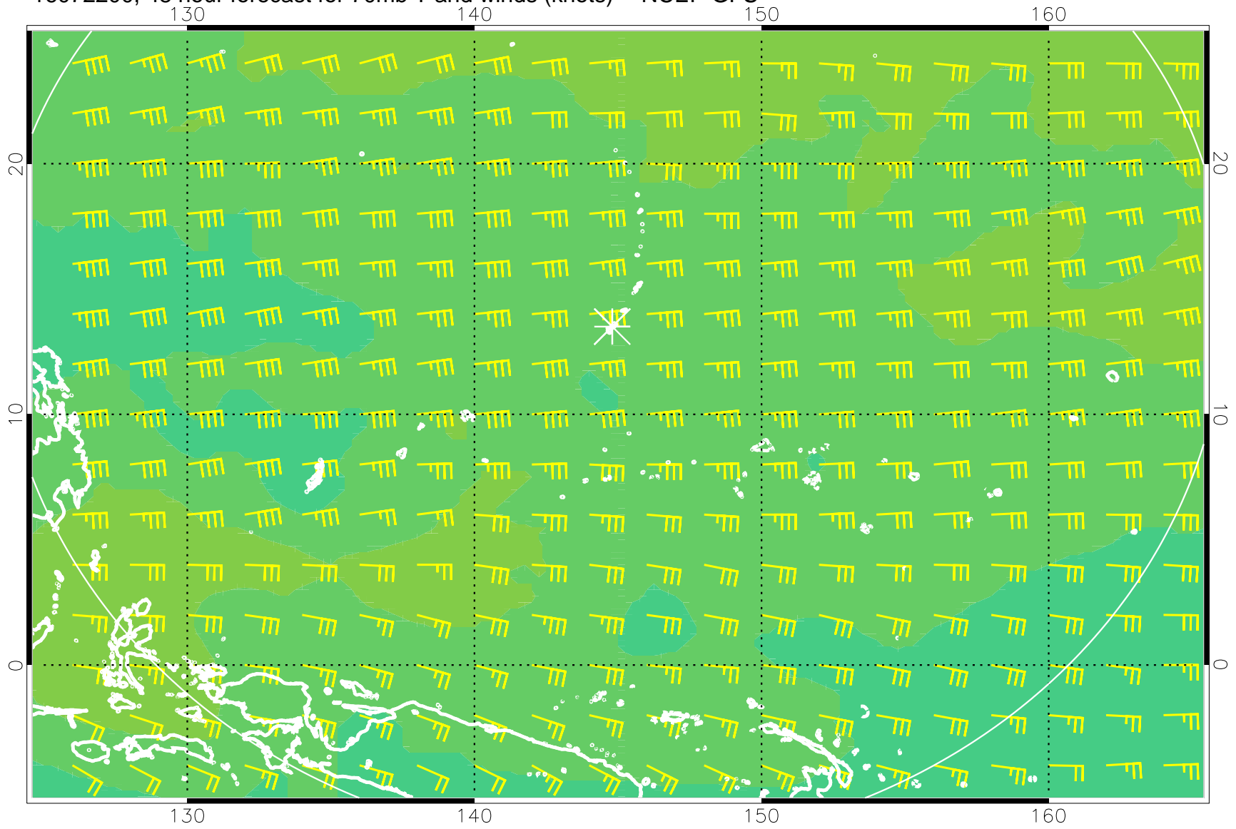
16072200, 48 hour forecast for 70mb T and winds (knots) -- NCEP GFS
