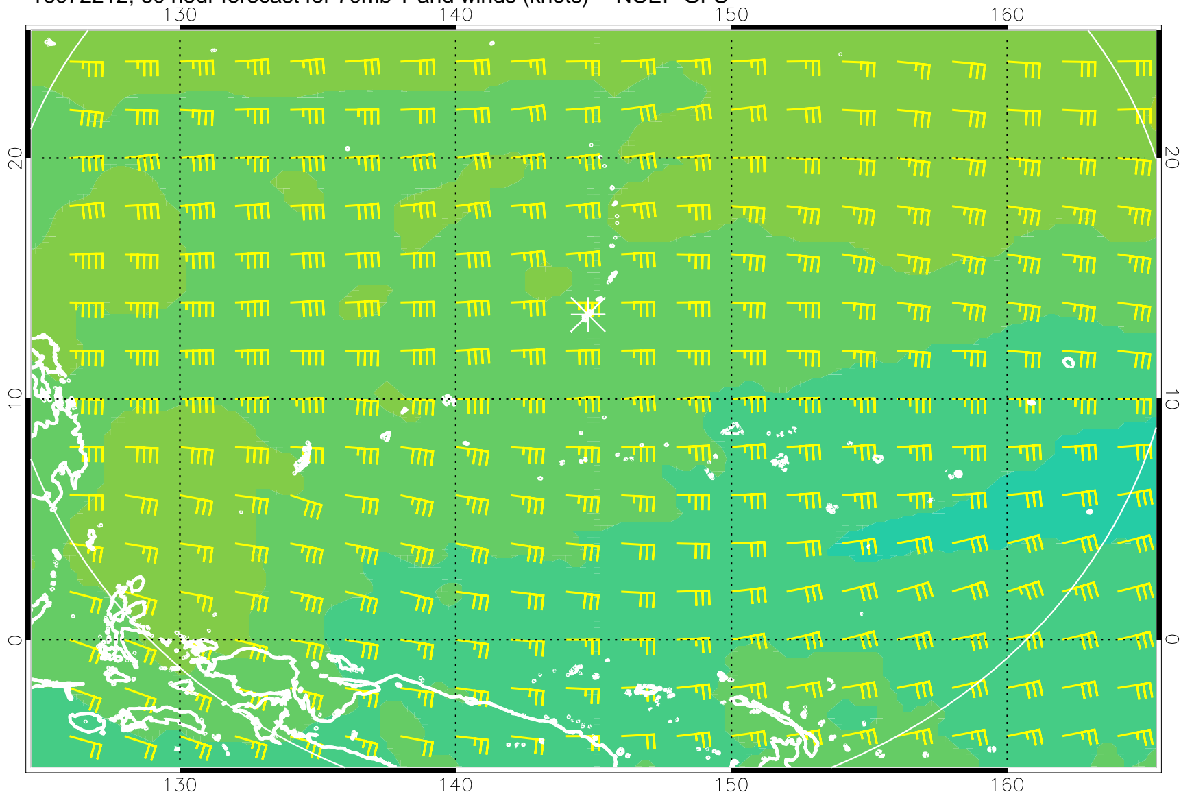
16072212, 60 hour forecast for 70mb T and winds (knots) -- NCEP GFS
