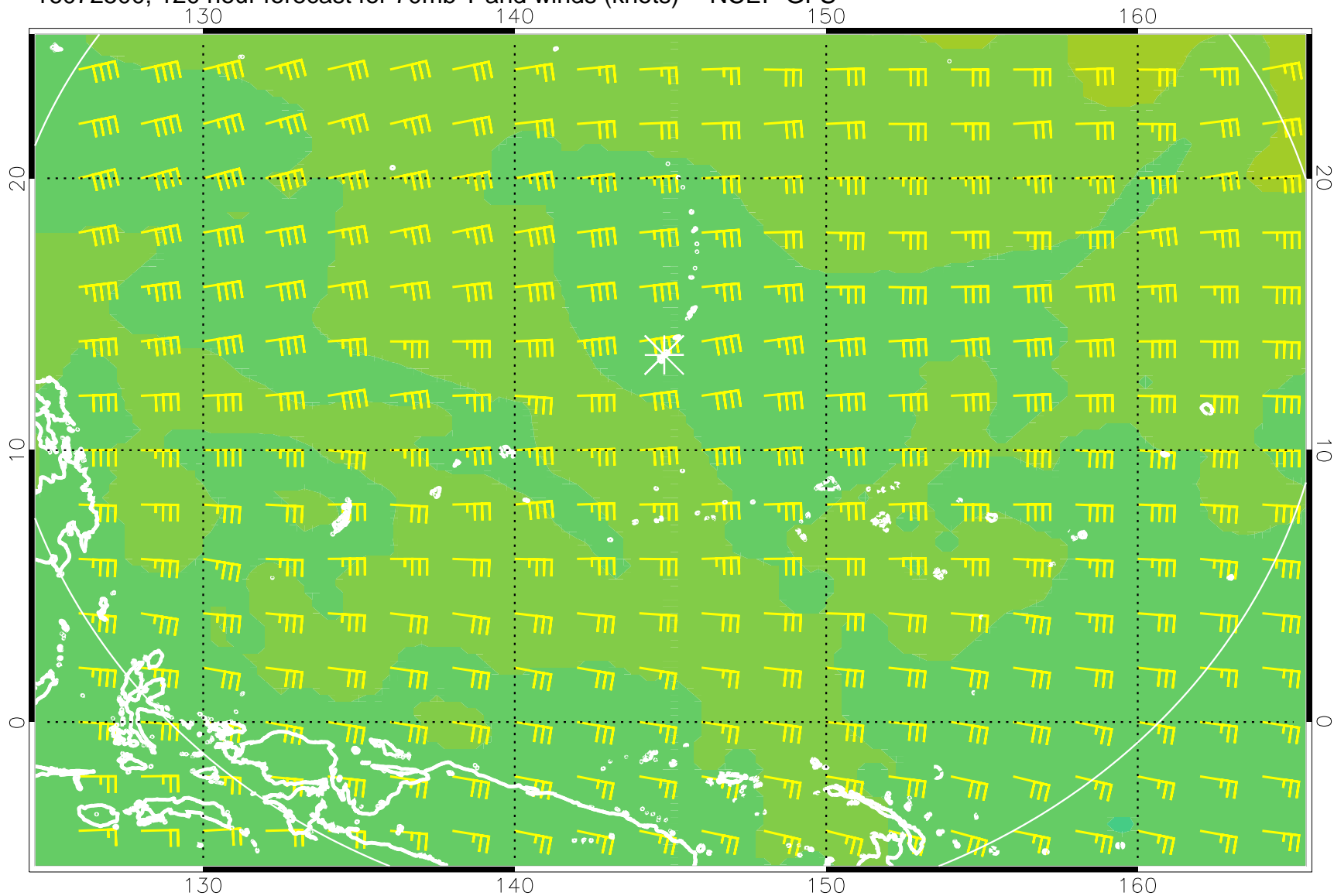
16072500, 120 hour forecast for 70mb T and winds (knots) -- NCEP GFS
