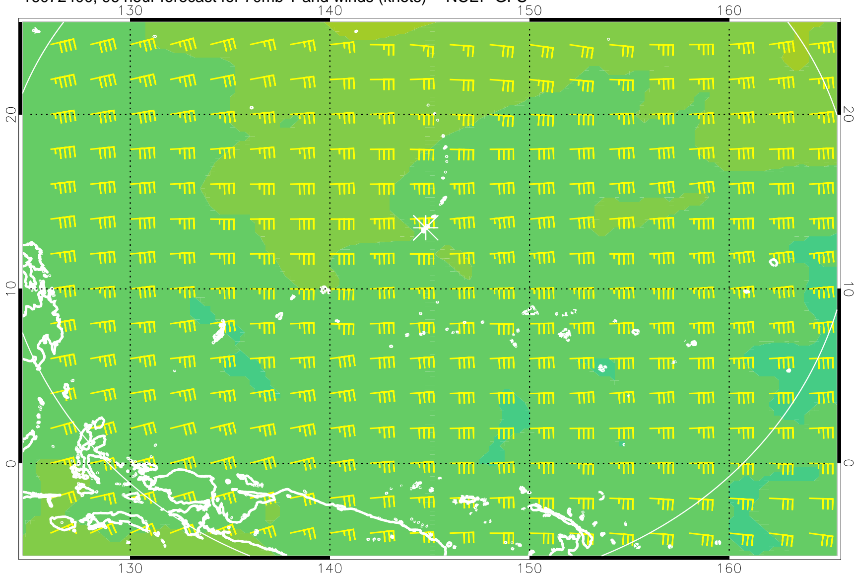
16072400, 96 hour forecast for 70mb T and winds (knots) -- NCEP GFS
