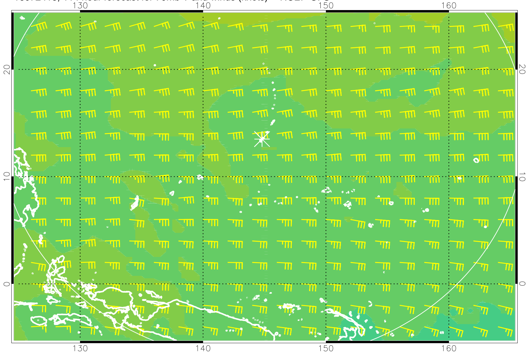
16072418, 114 hour forecast for 70mb T and winds (knots) -- NCEP GFS
