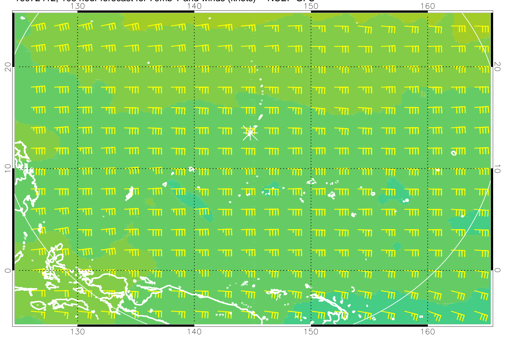
16072412, 108 hour forecast for 70mb T and winds (knots) -- NCEP GFS
