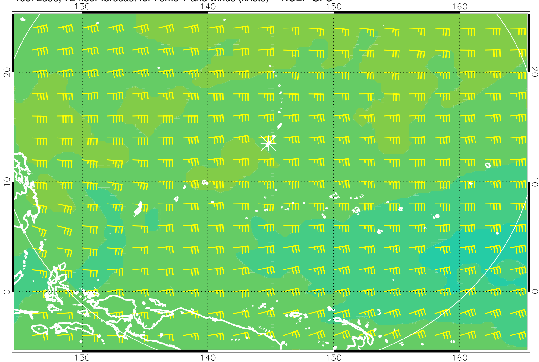
16072300, 72 hour forecast for 70mb T and winds (knots) -- NCEP GFS
