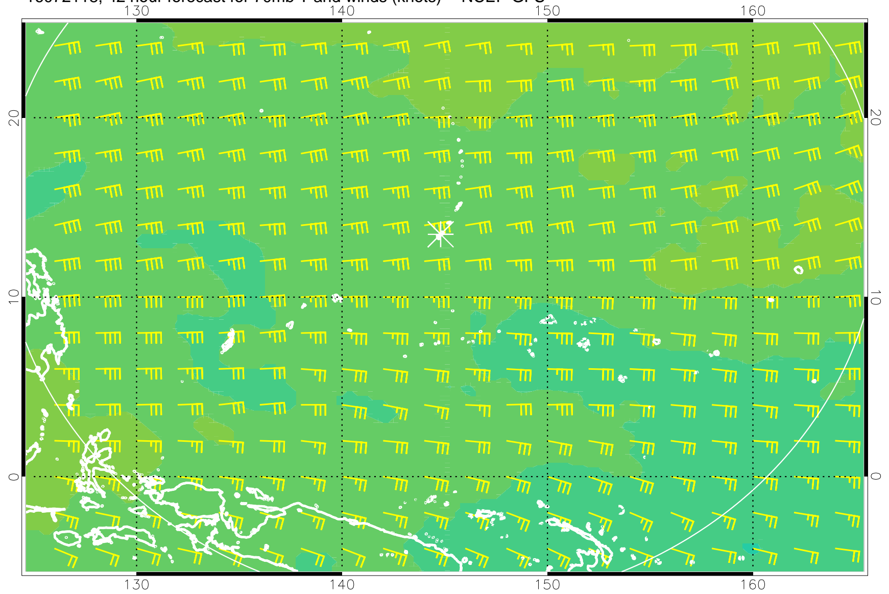
16072118, 42 hour forecast for 70mb T and winds (knots) -- NCEP GFS
