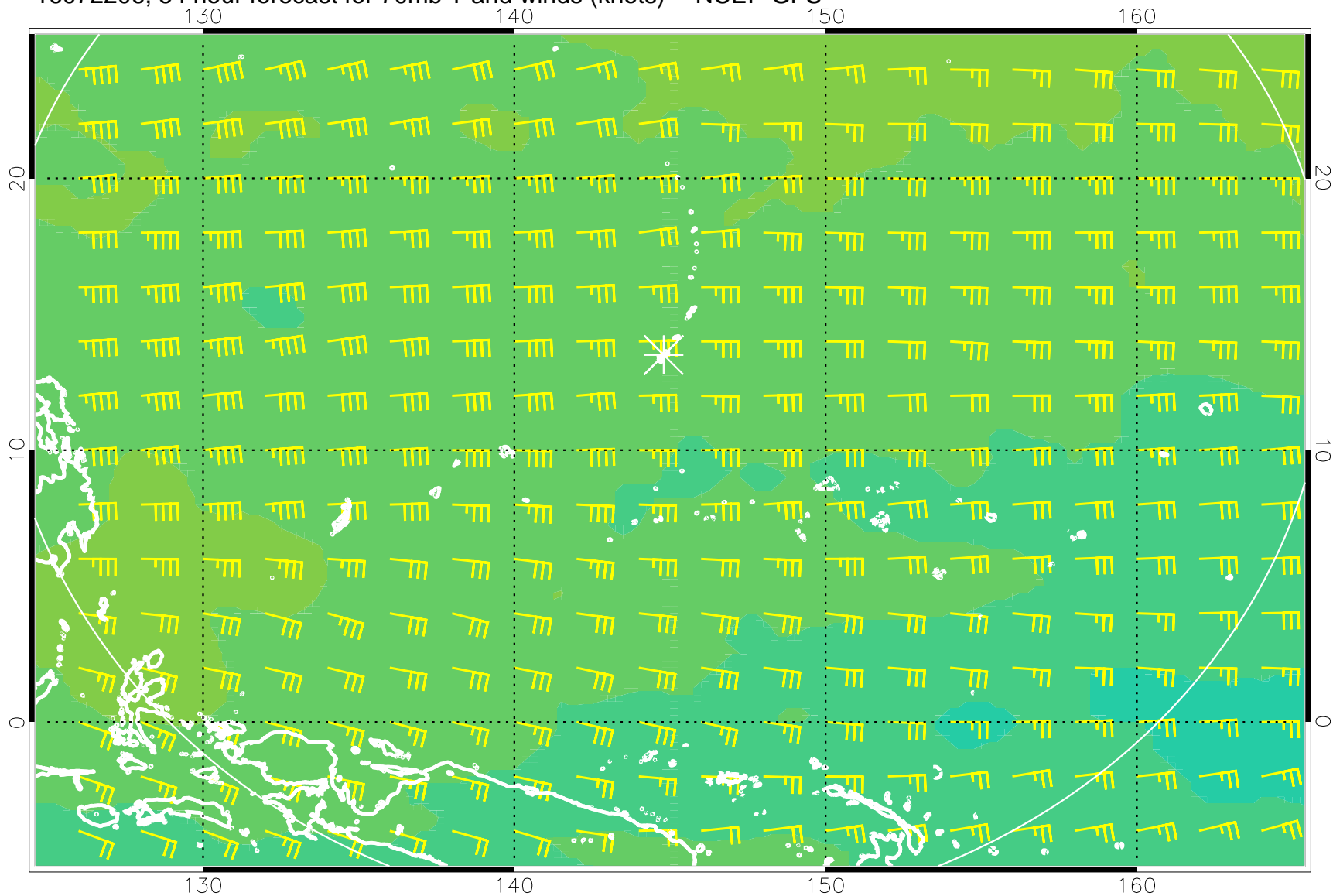
16072206, 54 hour forecast for 70mb T and winds (knots) -- NCEP GFS
