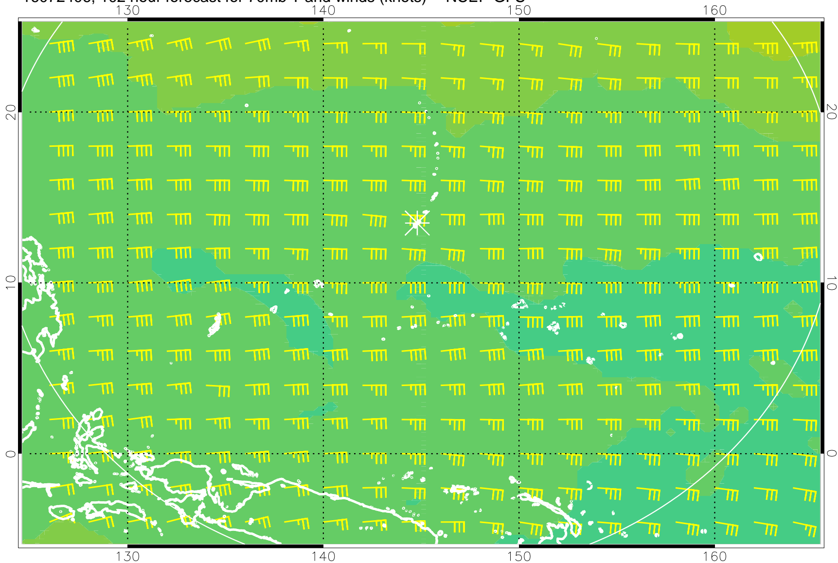
16072406, 102 hour forecast for 70mb T and winds (knots) -- NCEP GFS
