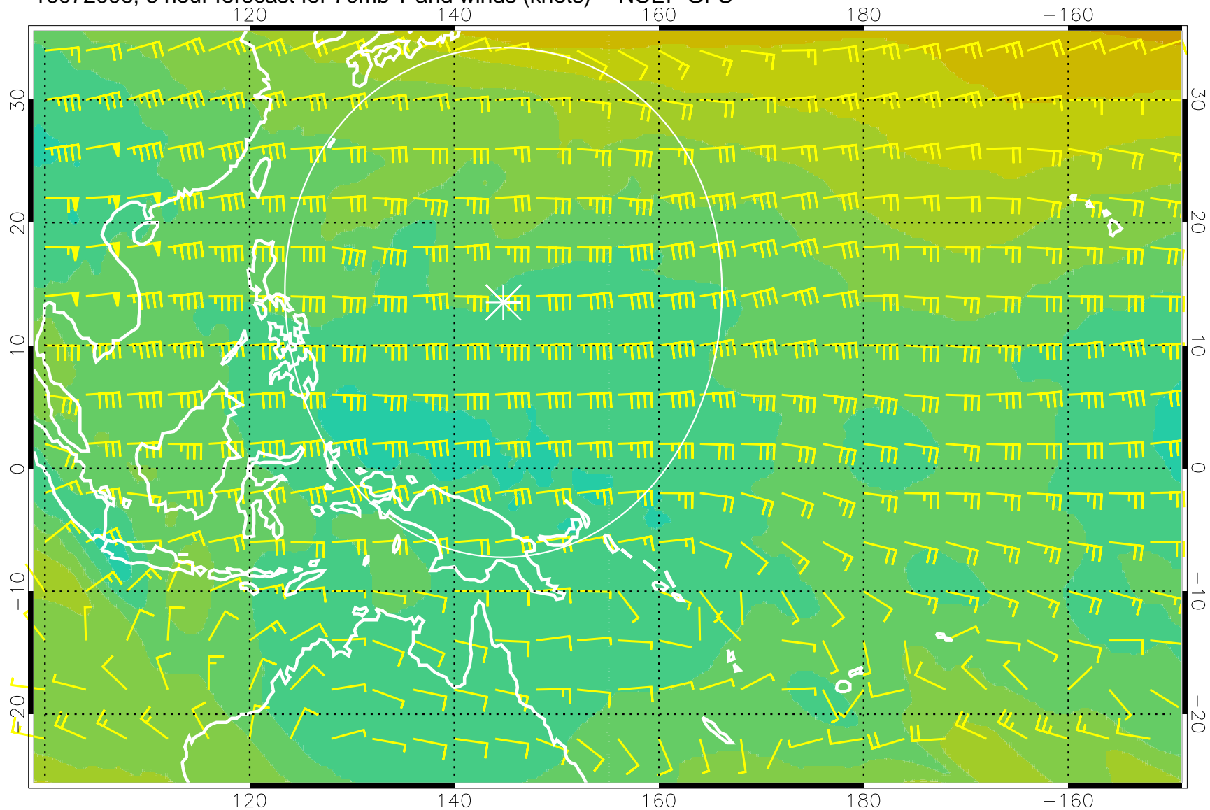
16072006, 6 hour forecast for 70mb T and winds (knots) -- NCEP GFS
