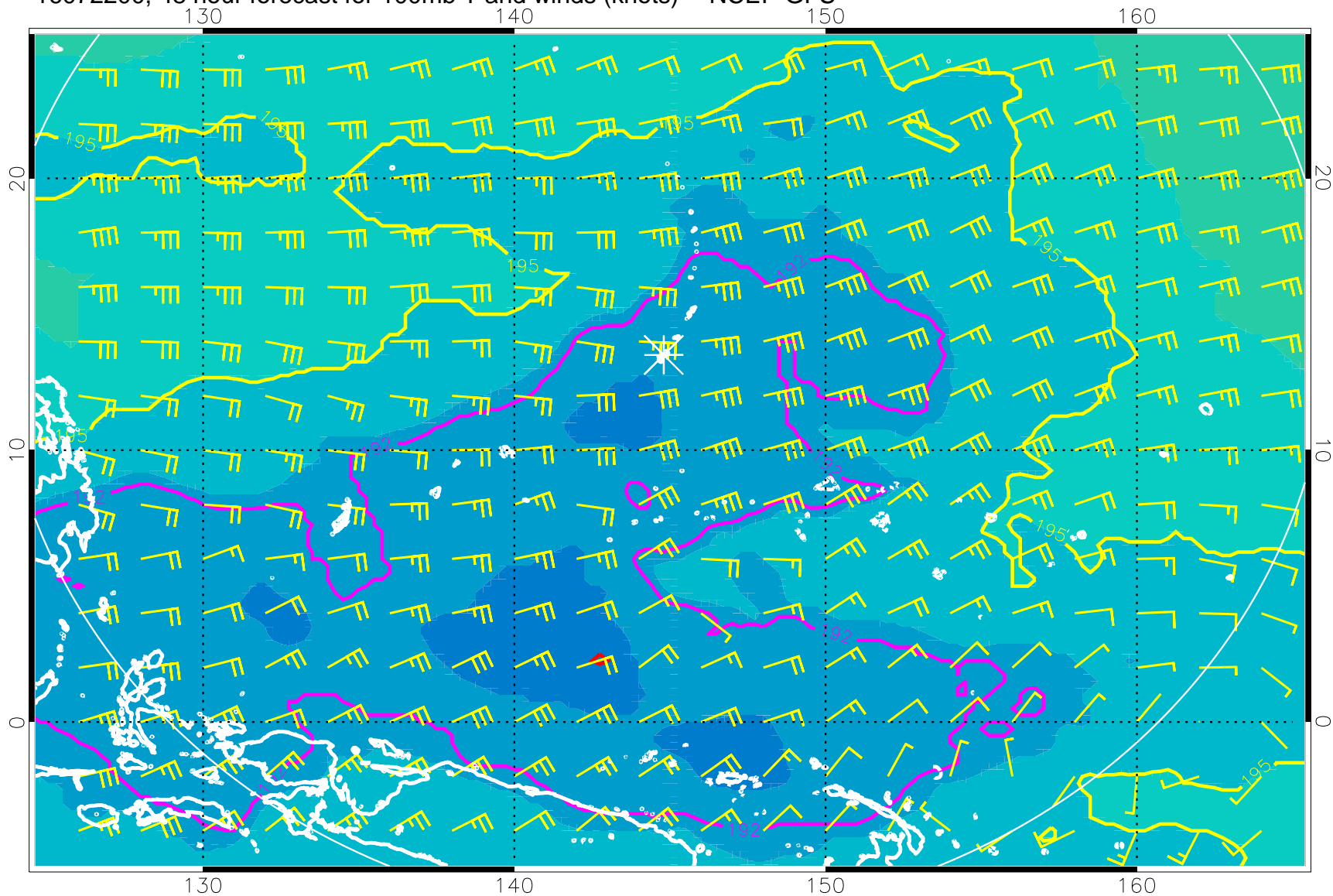
16072200, 48 hour forecast for 100mb T and winds (knots) -- NCEP GFS
