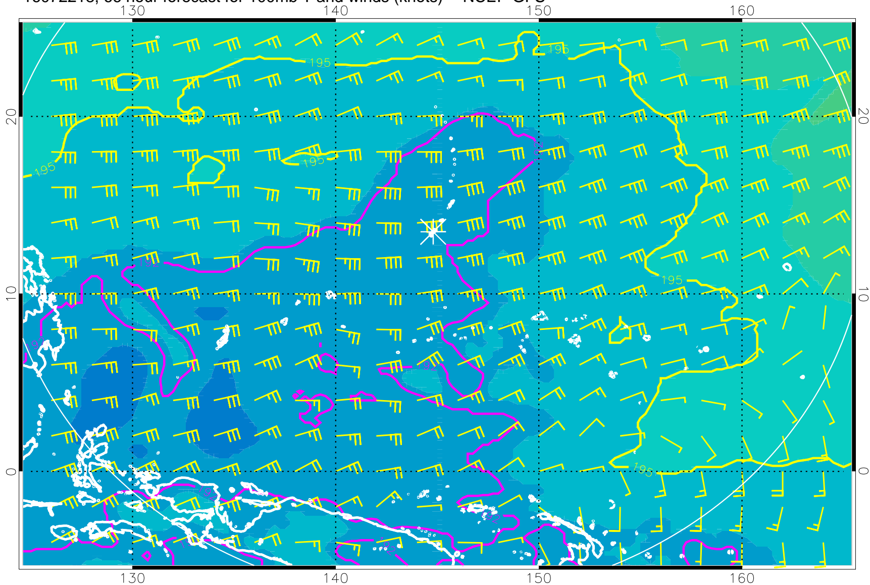
16072218, 66 hour forecast for 100mb T and winds (knots) -- NCEP GFS
