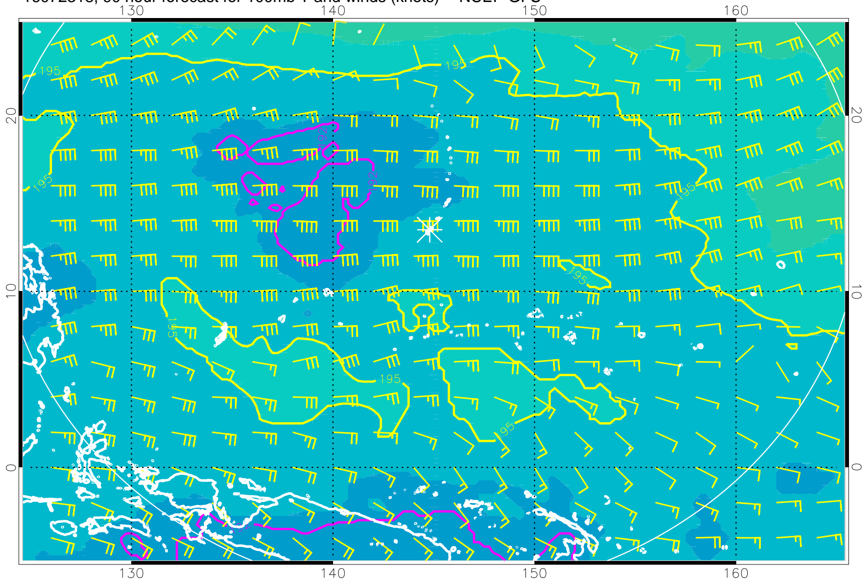
16072318, 90 hour forecast for 100mb T and winds (knots) -- NCEP GFS
