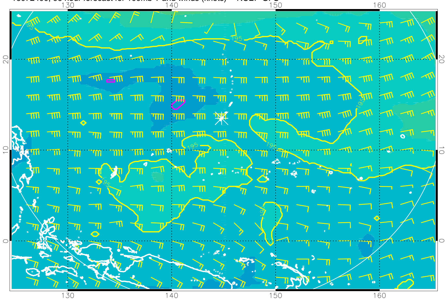
16072400, 96 hour forecast for 100mb T and winds (knots) -- NCEP GFS
