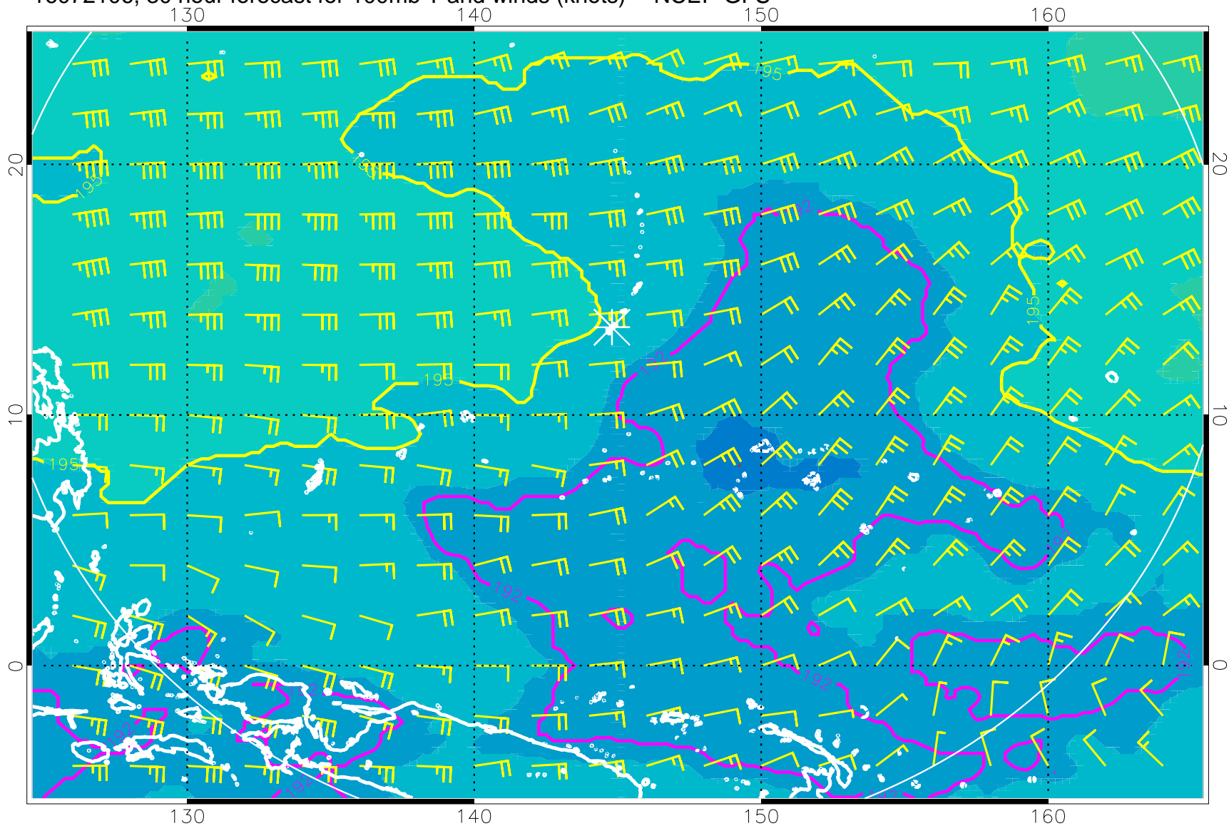
16072106, 30 hour forecast for 100mb T and winds (knots) -- NCEP GFS
