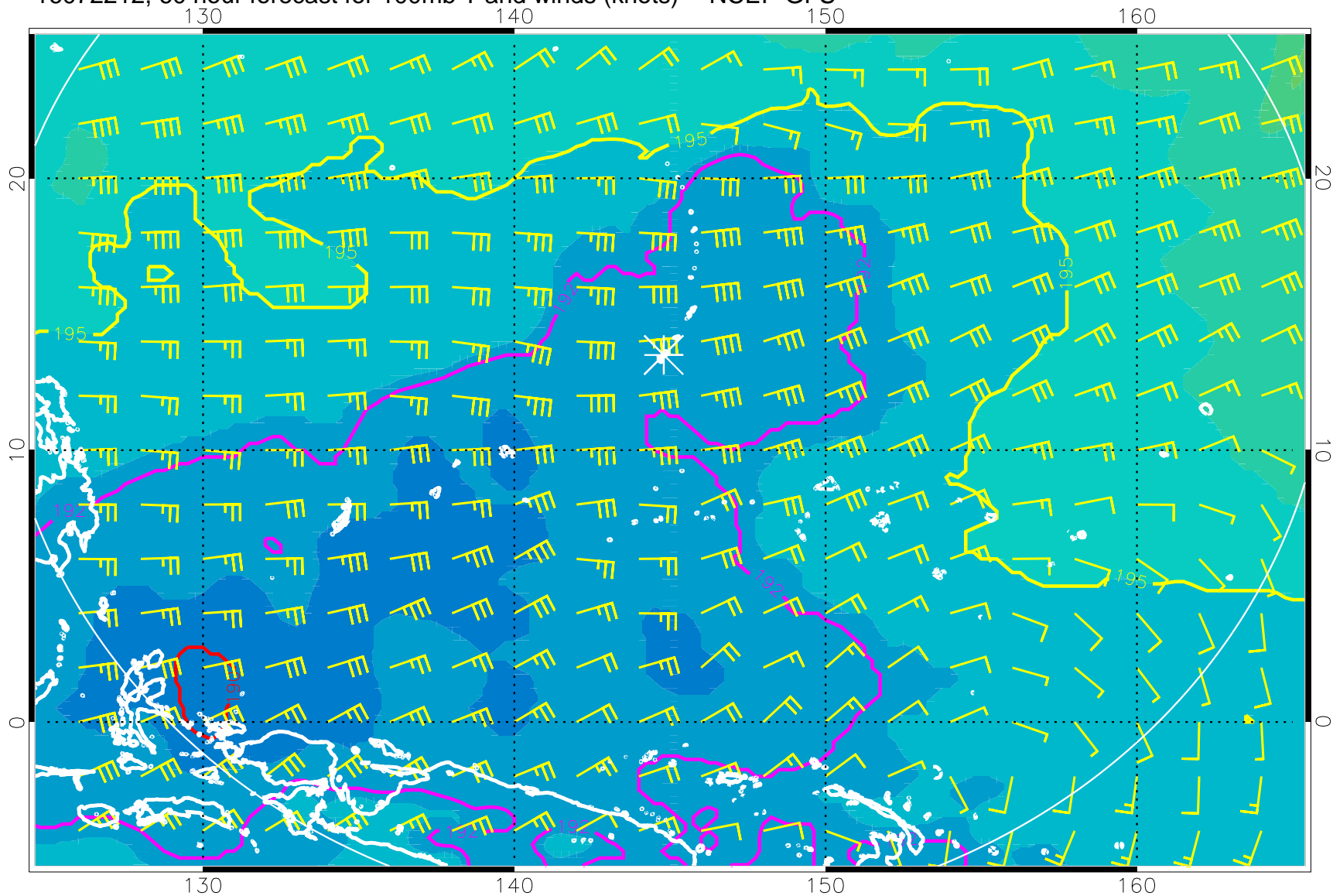
16072212, 60 hour forecast for 100mb T and winds (knots) -- NCEP GFS
