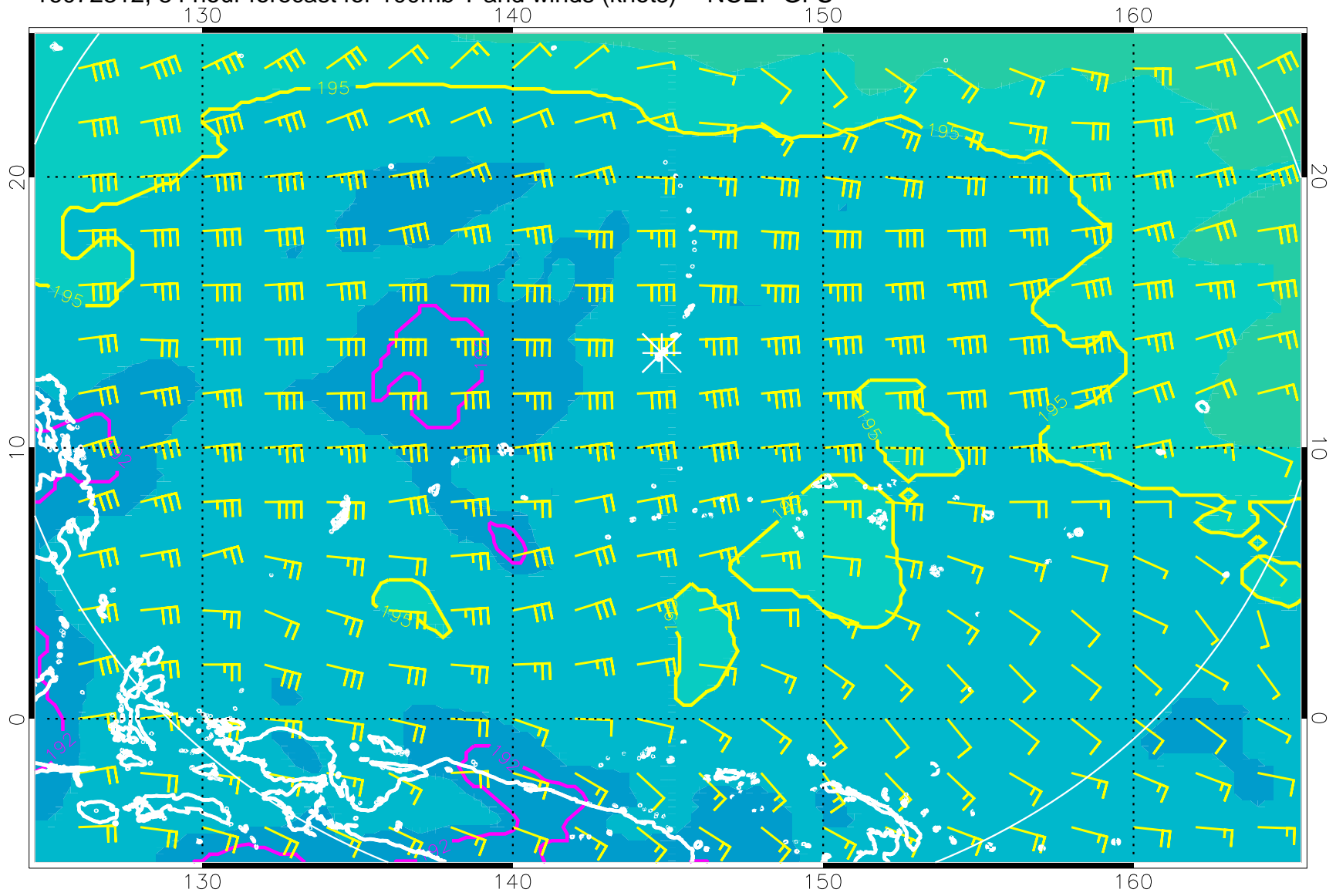
16072312, 84 hour forecast for 100mb T and winds (knots) -- NCEP GFS
