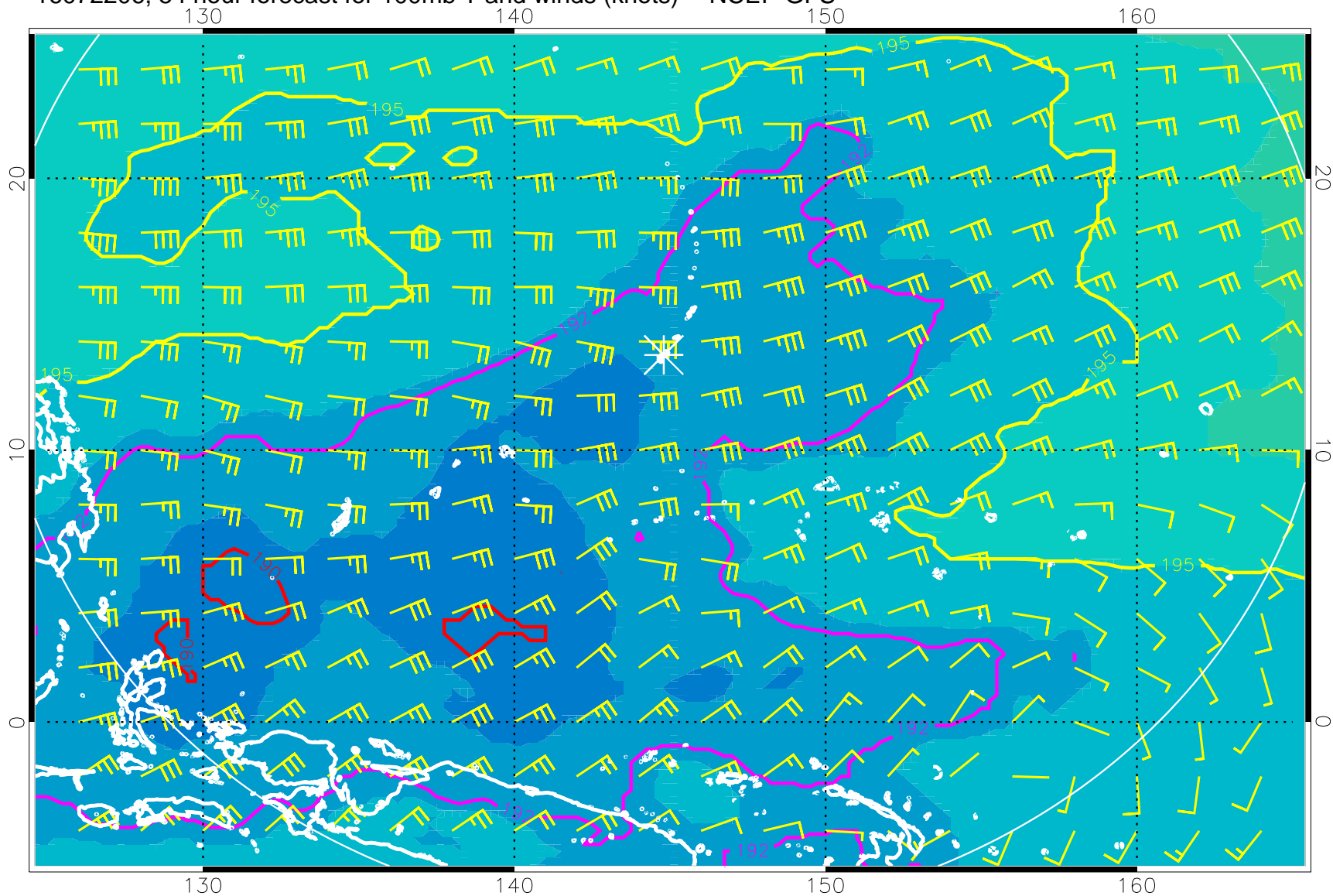
16072206, 54 hour forecast for 100mb T and winds (knots) -- NCEP GFS
