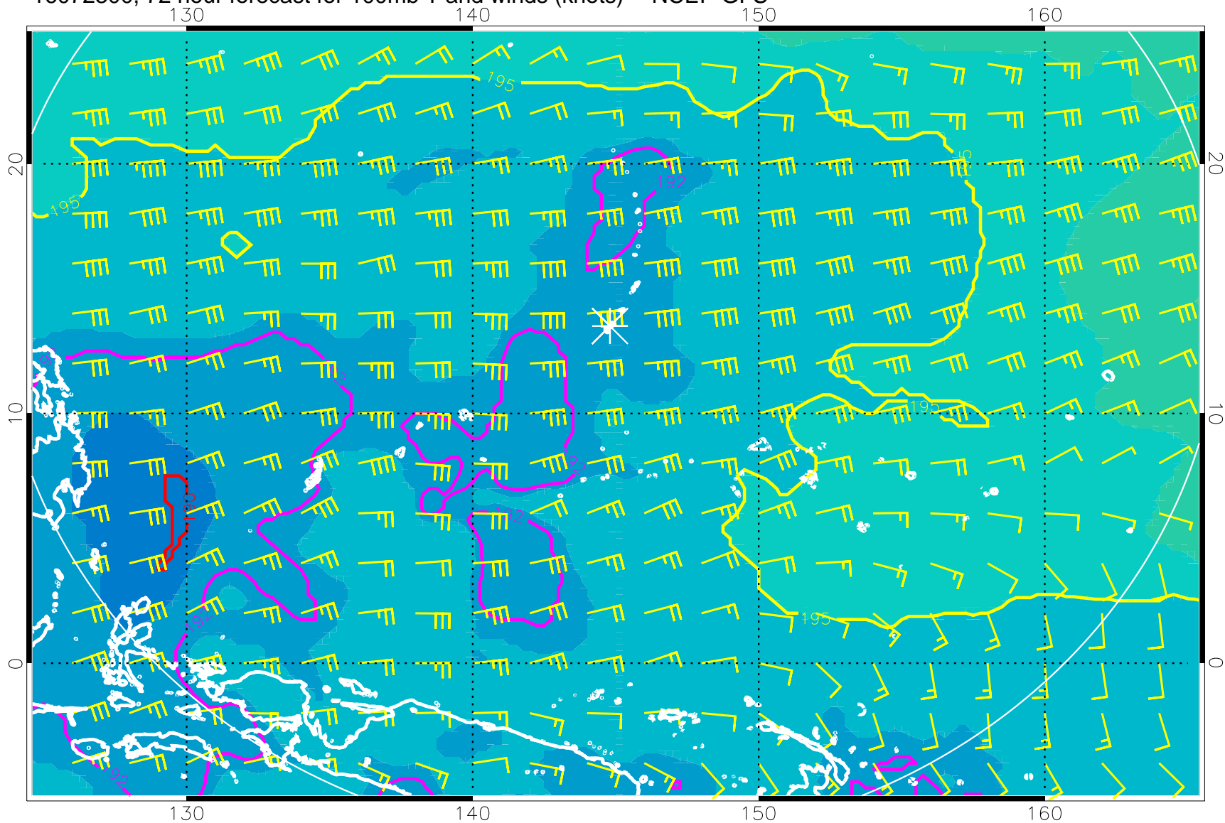
16072300, 72 hour forecast for 100mb T and winds (knots) -- NCEP GFS
