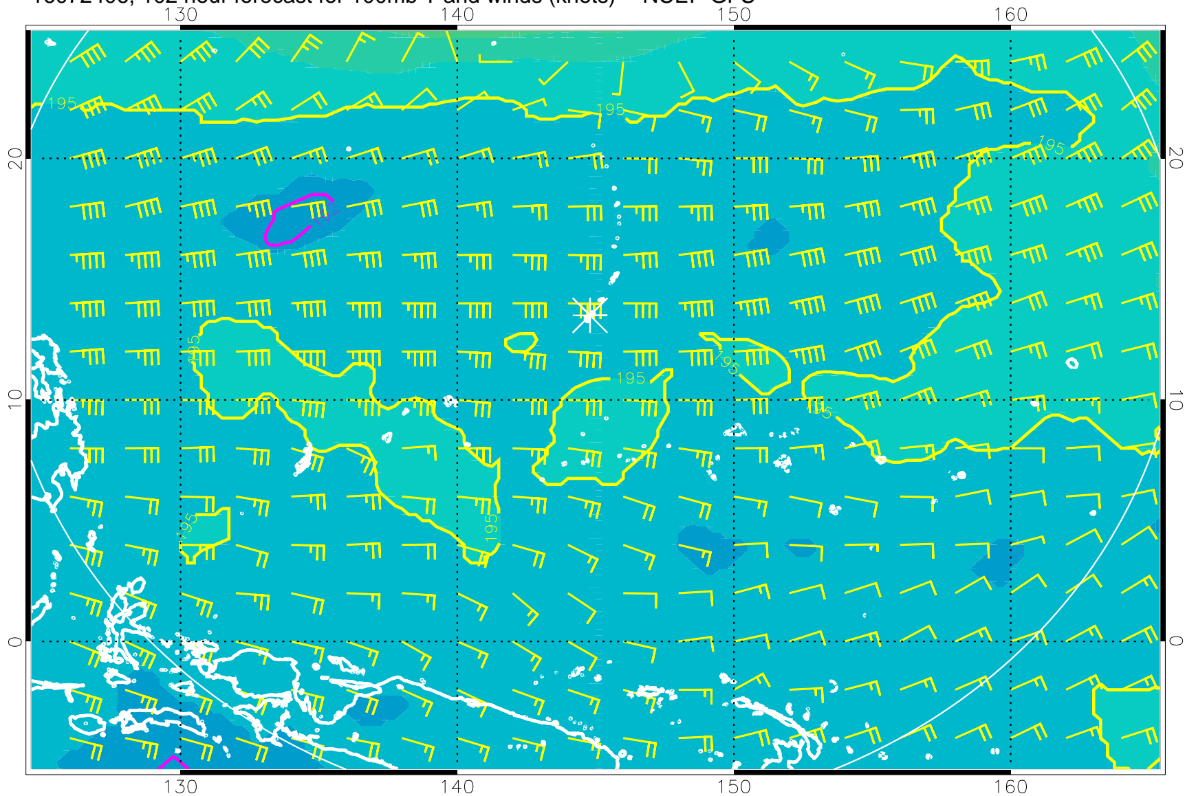
16072406, 102 hour forecast for 100mb T and winds (knots) -- NCEP GFS
