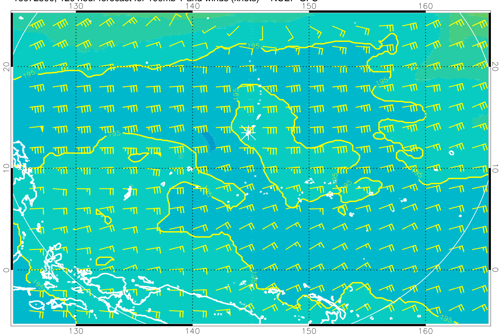
16072500, 120 hour forecast for 100mb T and winds (knots) -- NCEP GFS
