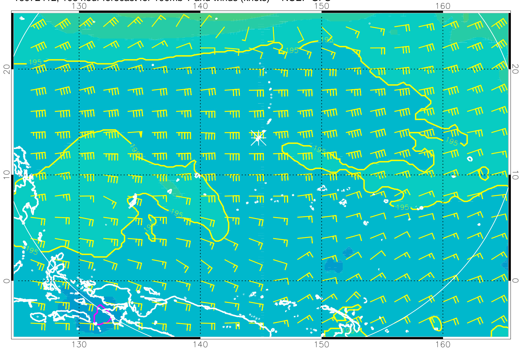
16072412, 108 hour forecast for 100mb T and winds (knots) -- NCEP GFS
