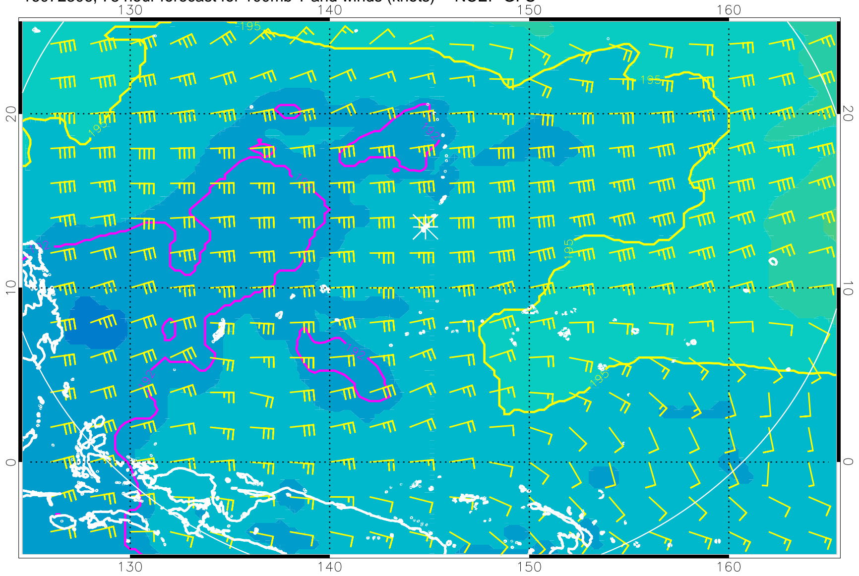
16072306, 78 hour forecast for 100mb T and winds (knots) -- NCEP GFS
