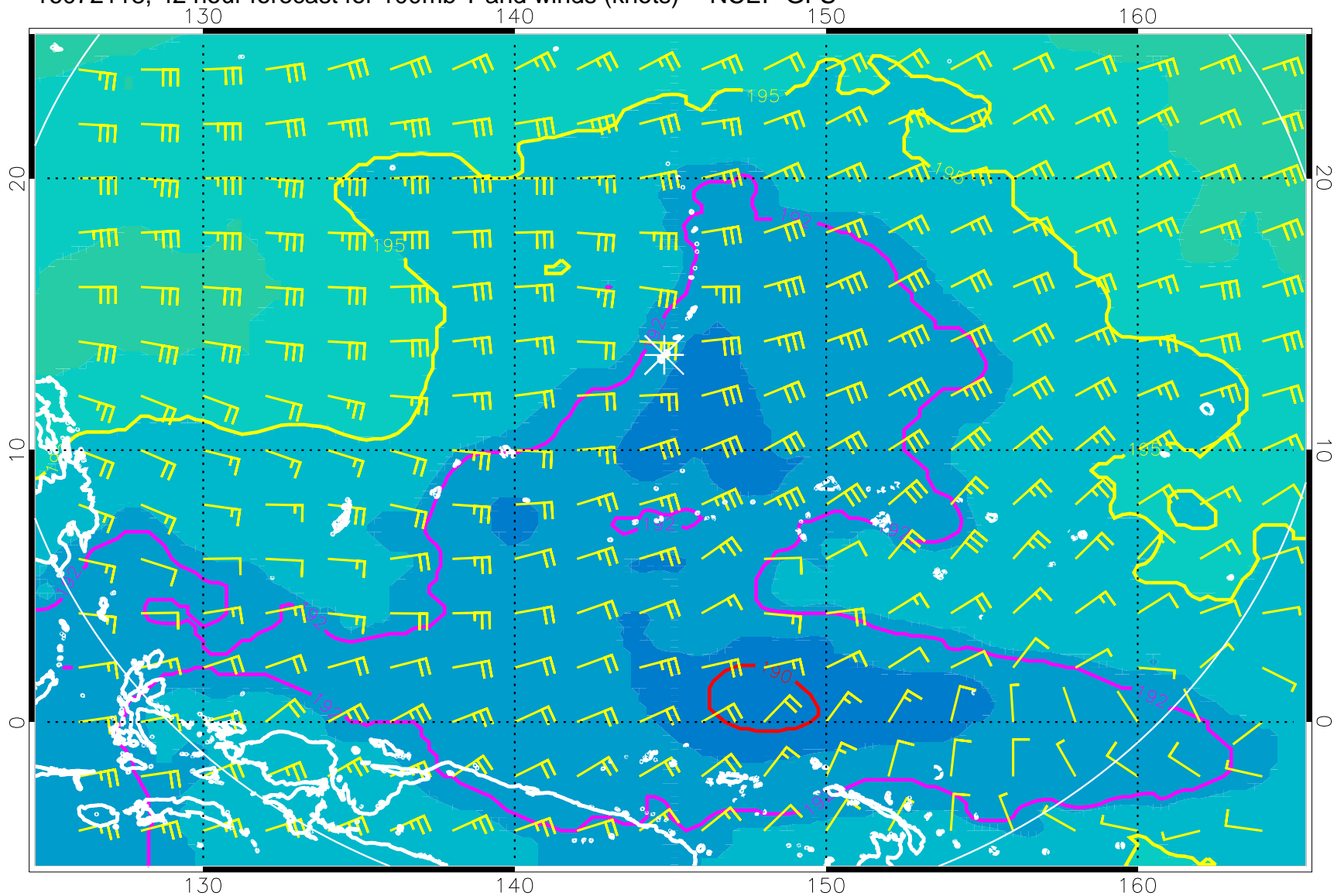
16072118, 42 hour forecast for 100mb T and winds (knots) -- NCEP GFS
