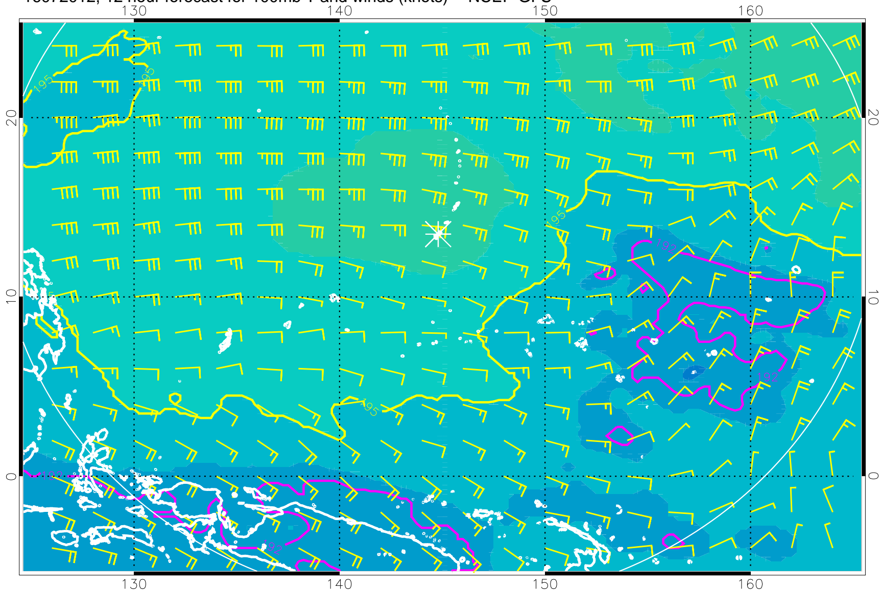
16072012, 12 hour forecast for 100mb T and winds (knots) -- NCEP GFS
