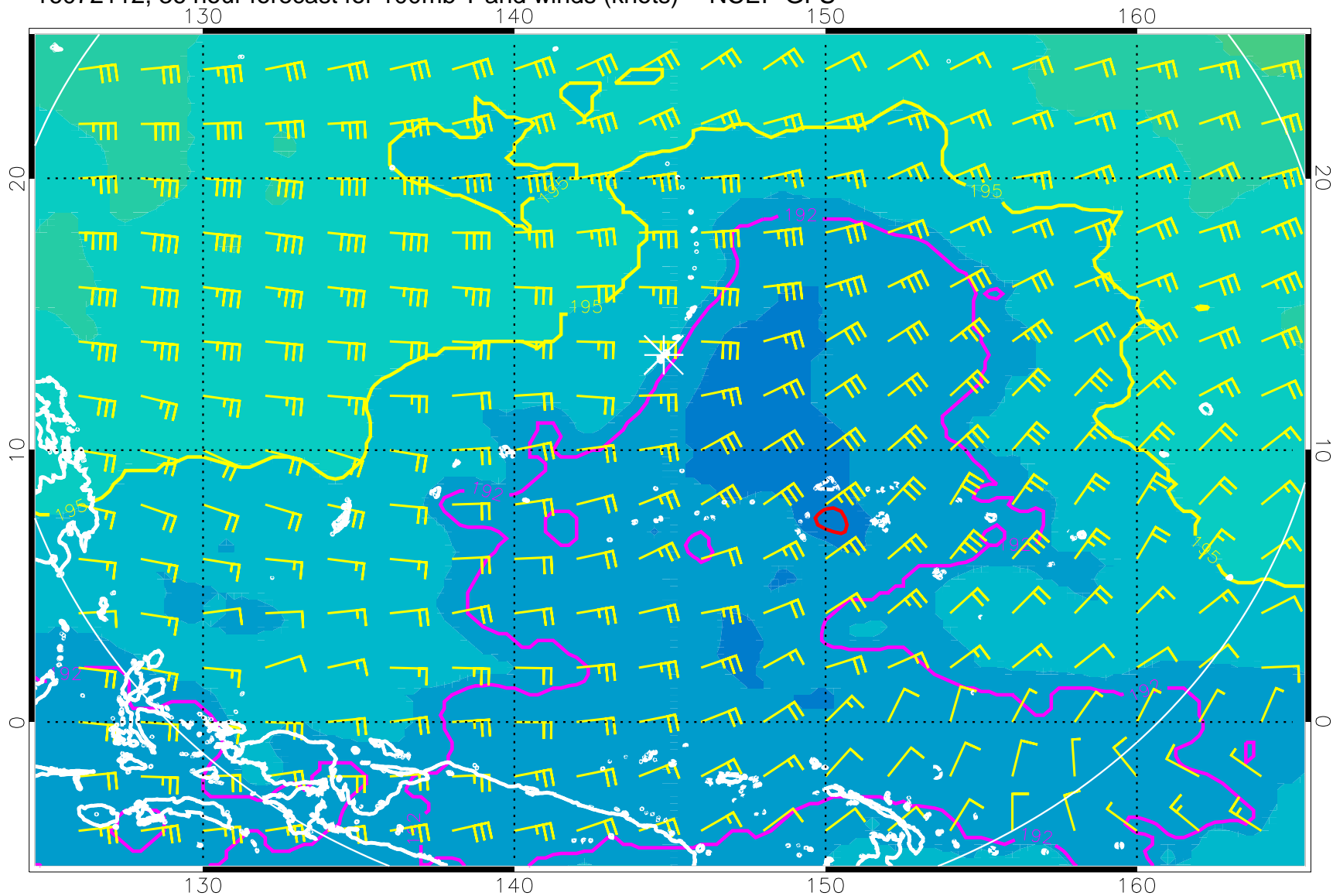
16072112, 36 hour forecast for 100mb T and winds (knots) -- NCEP GFS
