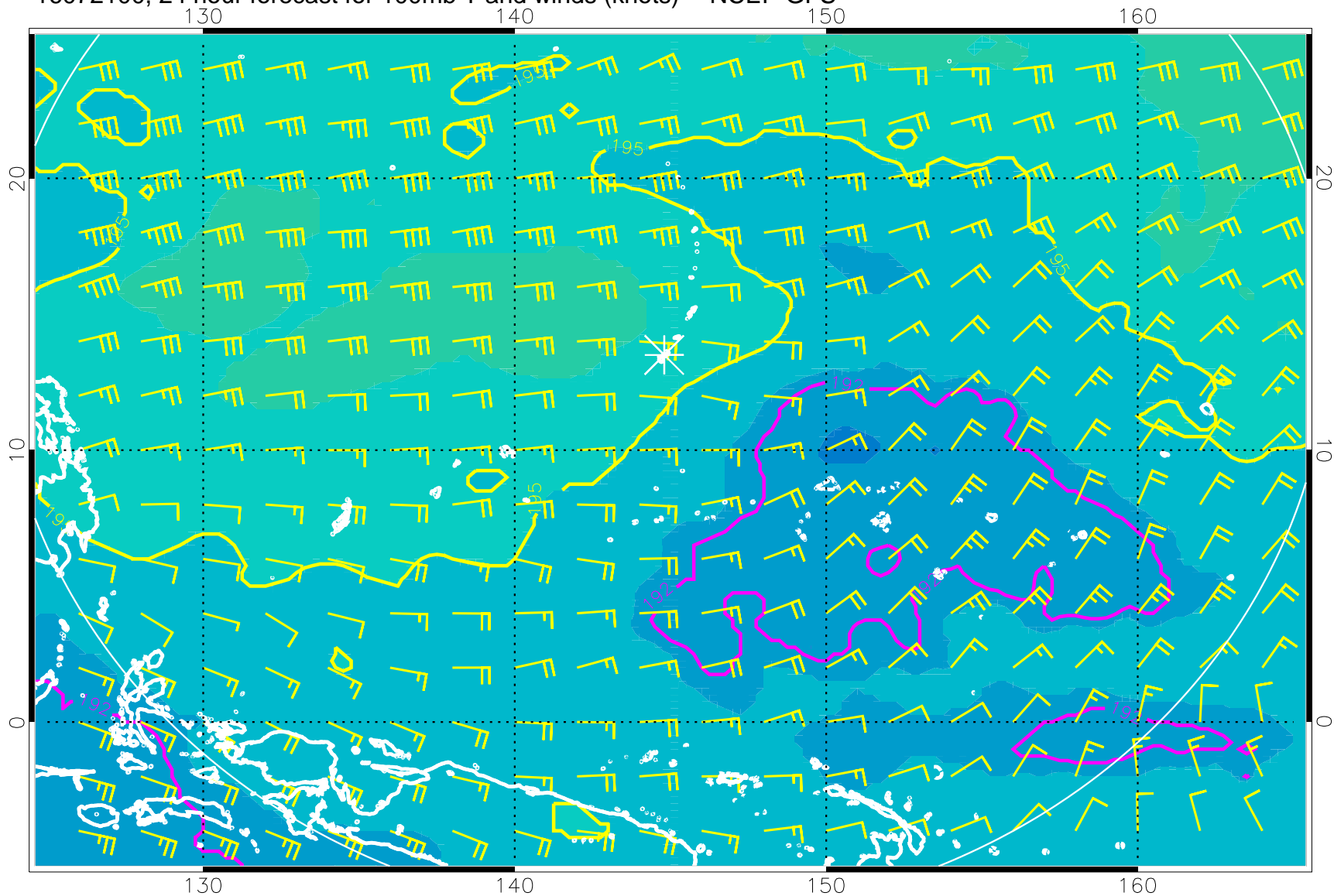
16072100, 24 hour forecast for 100mb T and winds (knots) -- NCEP GFS
