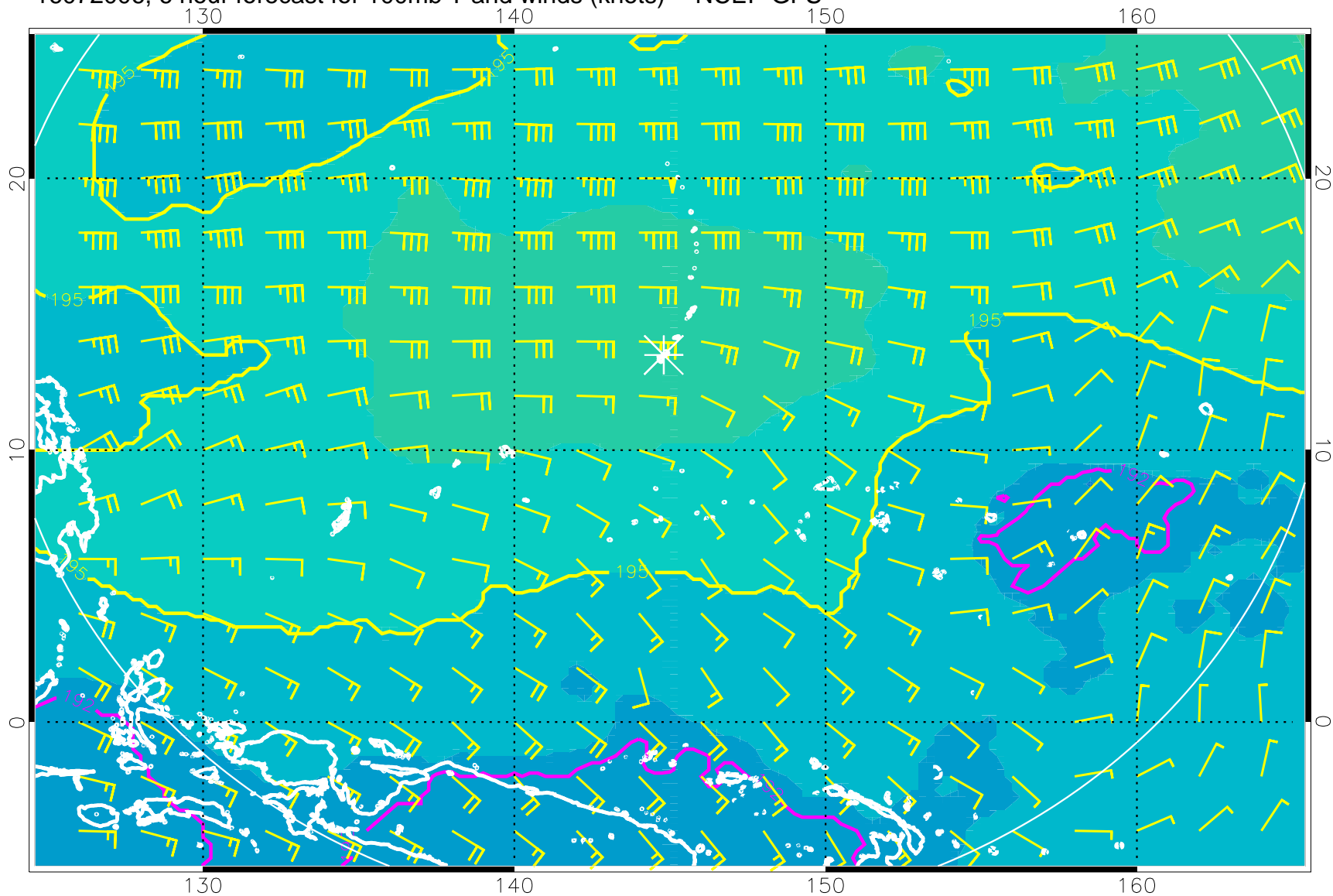
16072006, 6 hour forecast for 100mb T and winds (knots) -- NCEP GFS
