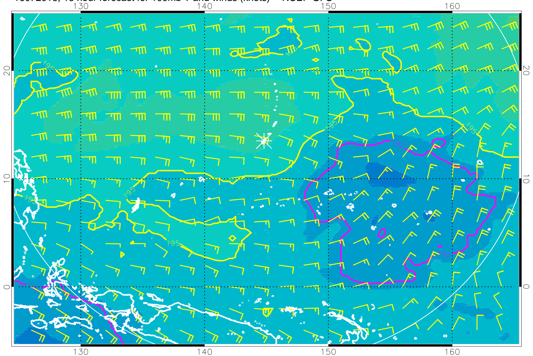
16072018, 18 hour forecast for 100mb T and winds (knots) -- NCEP GFS
