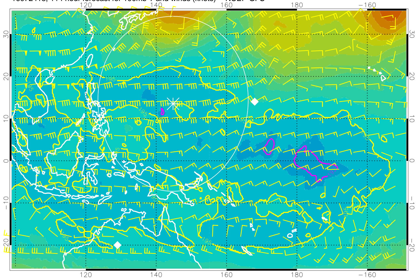
16072418, 114 hour forecast for 100mb T and winds (knots) -- NCEP GFS
