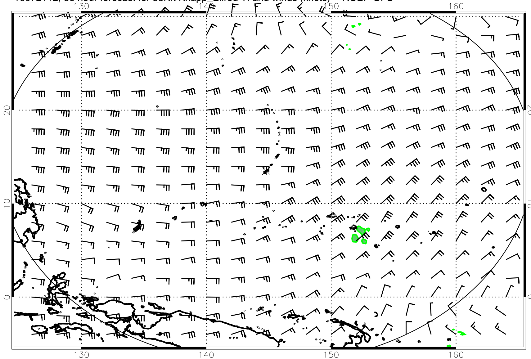
16072112, 36 hour forecast for 53Kft Knapp_Ellrod TI and winds (knots) -- NCEP GFS
