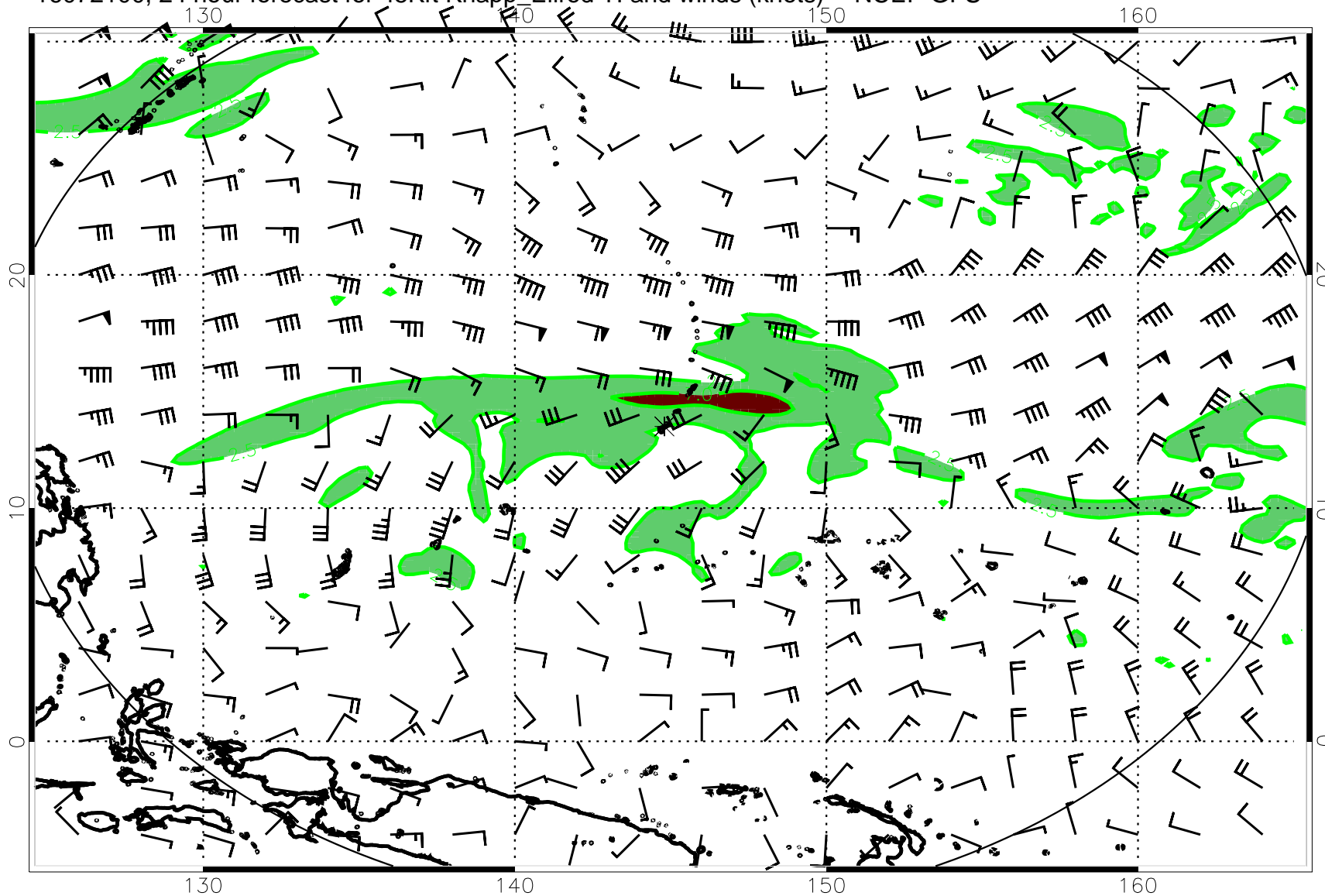
16072100, 24 hour forecast for 45Kft Knapp_Ellrod TI and winds (knots) -- NCEP GFS
