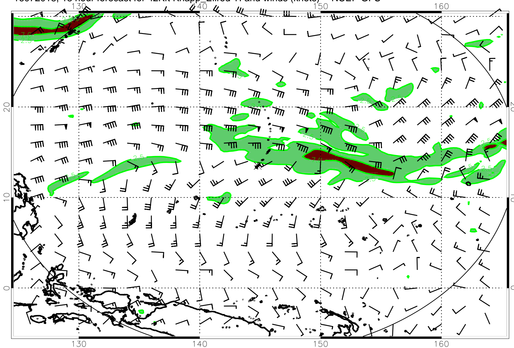
16072018, 18 hour forecast for 42Kft Knapp_Ellrod TI and winds (knots) -- NCEP GFS
