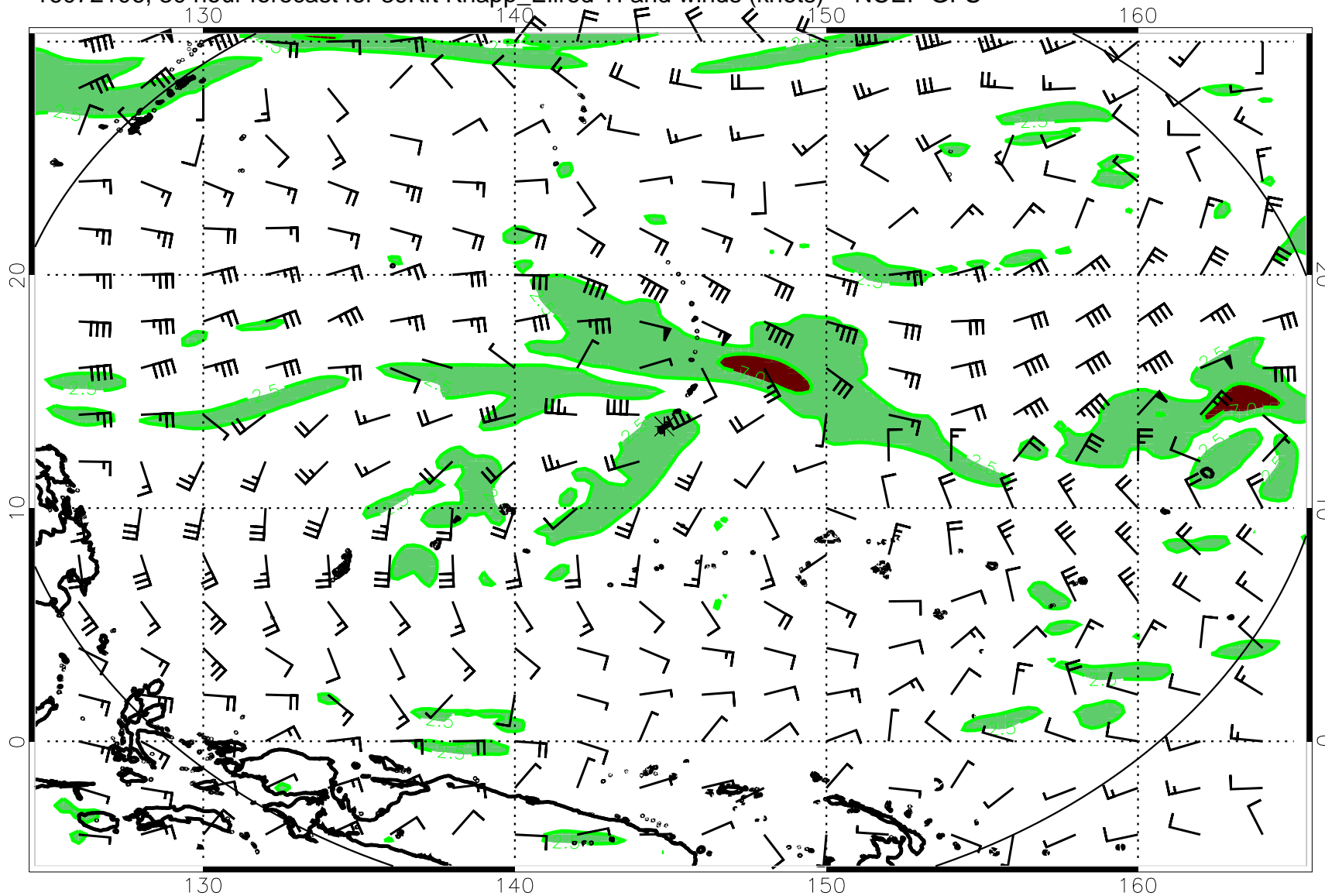
16072106, 30 hour forecast for 39Kft Knapp_Ellrod TI and winds (knots) -- NCEP GFS
