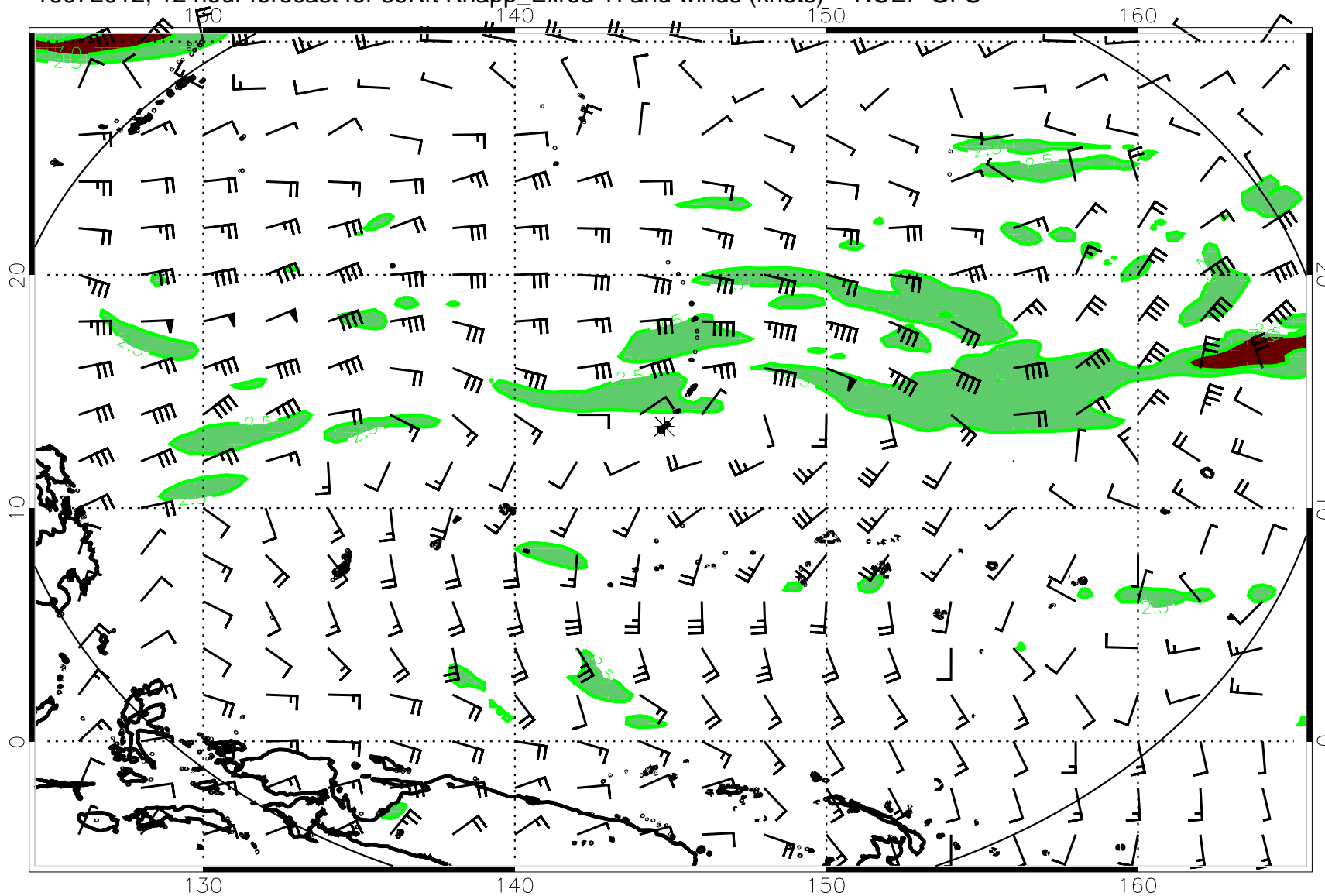
16072012, 12 hour forecast for 39Kft Knapp_Ellrod TI and winds (knots) -- NCEP GFS
