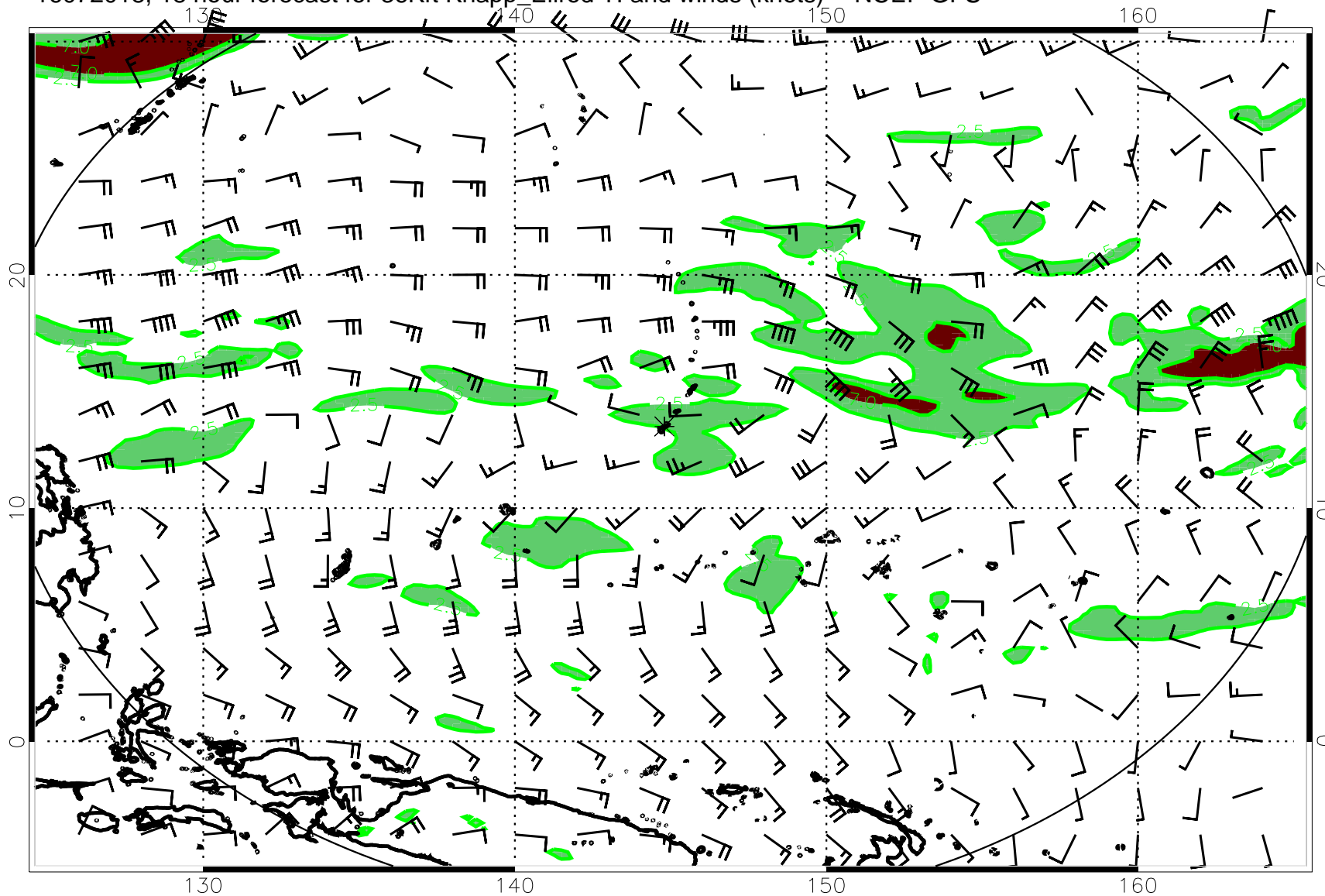
16072018, 18 hour forecast for 36Kft Knapp_Ellrod TI and winds (knots) -- NCEP GFS
