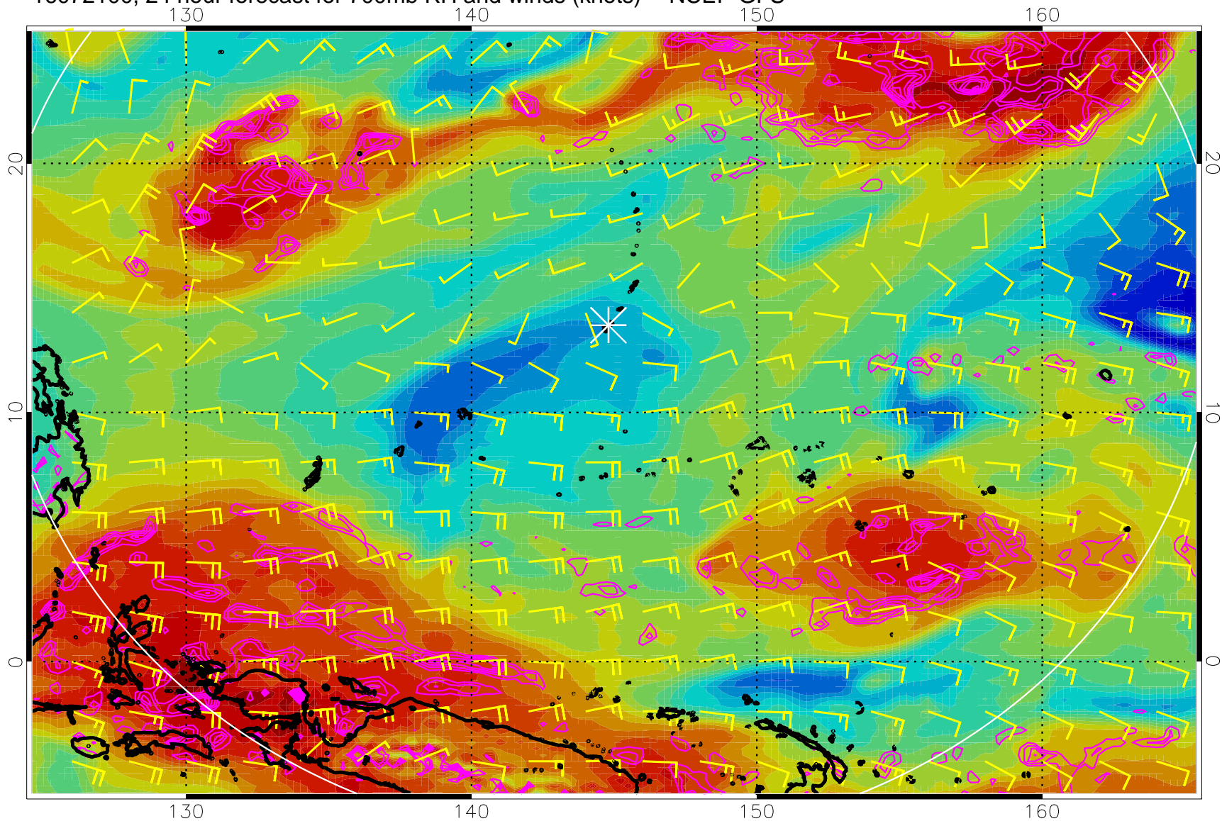
16072100, 24 hour forecast for 700mb RH and winds (knots) -- NCEP GFS
