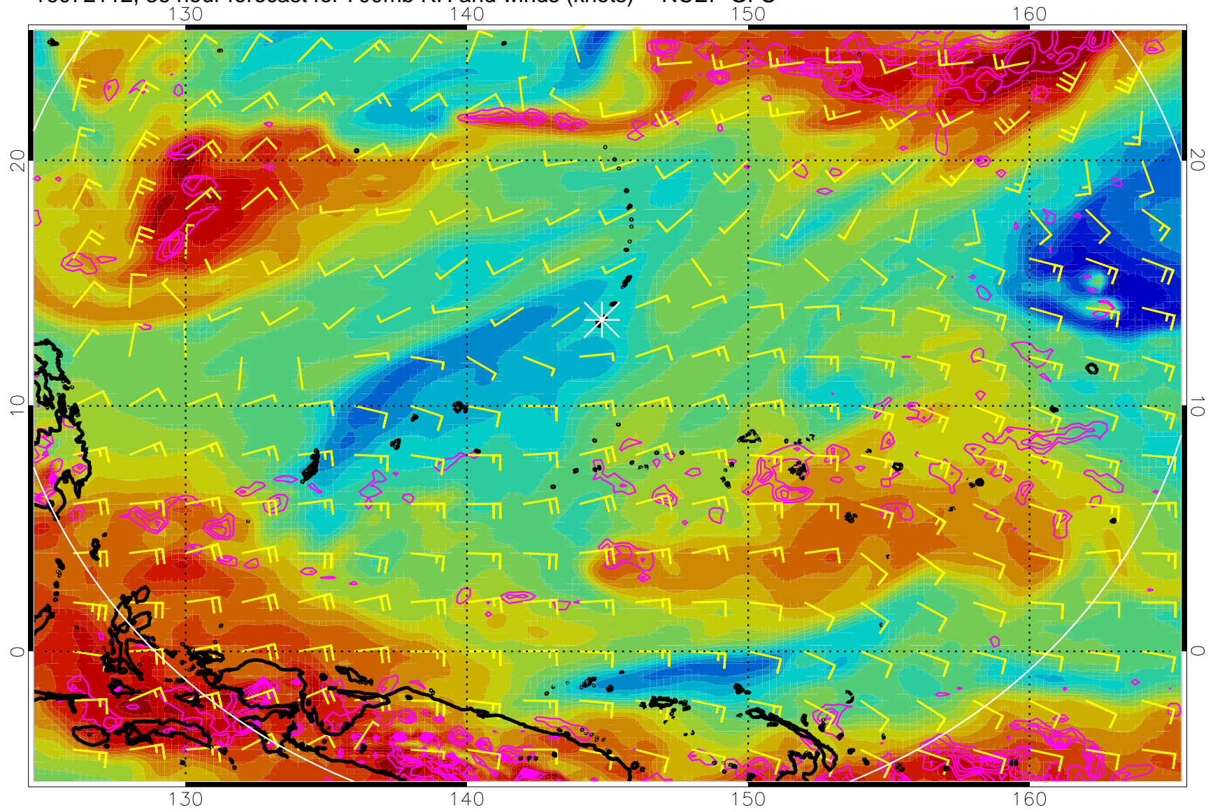
16072112, 36 hour forecast for 700mb RH and winds (knots) -- NCEP GFS
