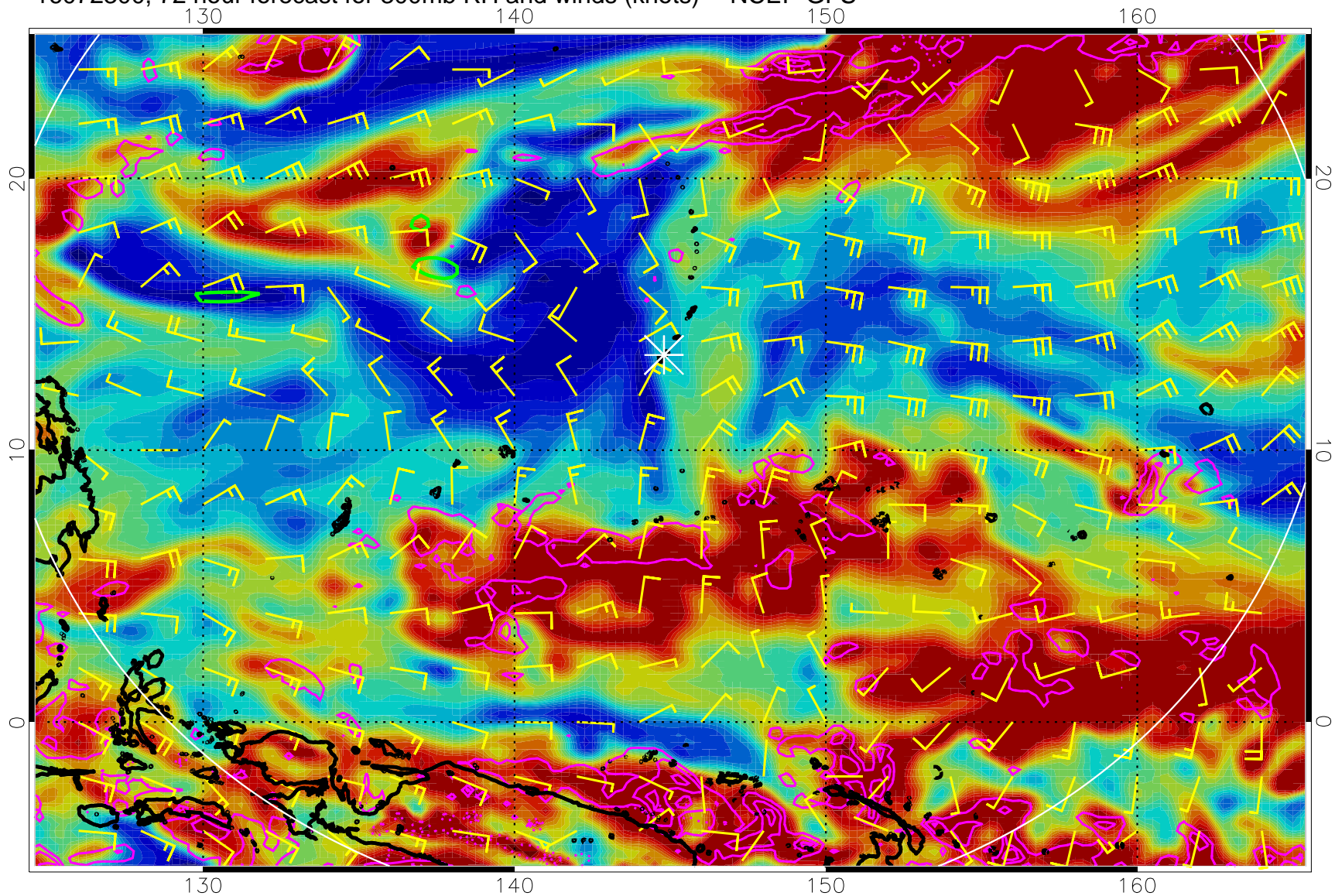
16072300, 72 hour forecast for 300mb RH and winds (knots) -- NCEP GFS
