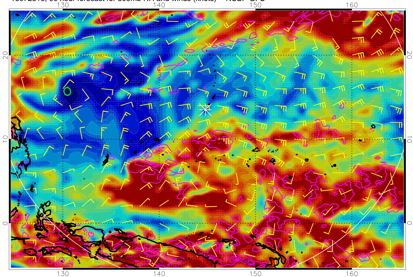
16072318, 90 hour forecast for 300mb RH and winds (knots) -- NCEP GFS
