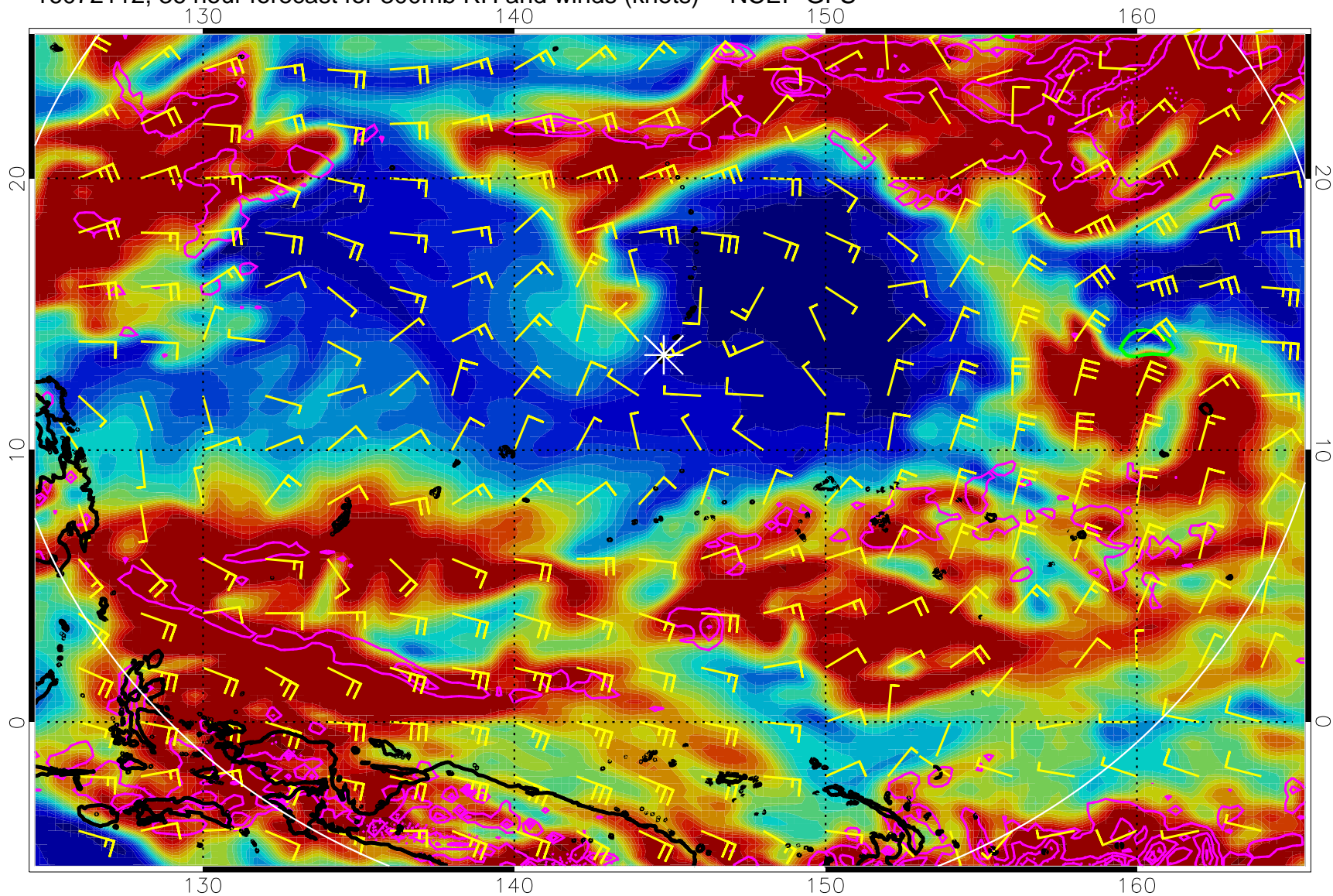
16072112, 36 hour forecast for 300mb RH and winds (knots) -- NCEP GFS
