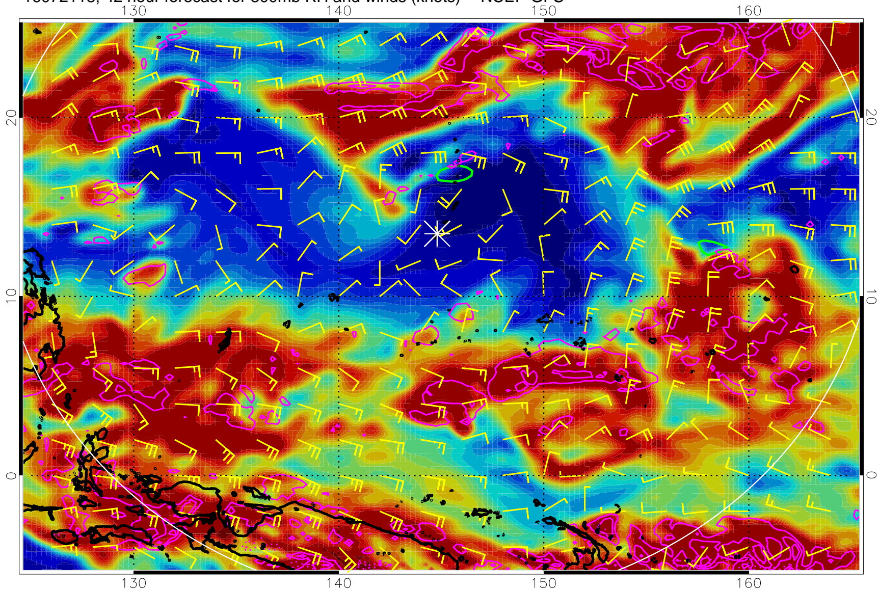
16072118, 42 hour forecast for 300mb RH and winds (knots) -- NCEP GFS
