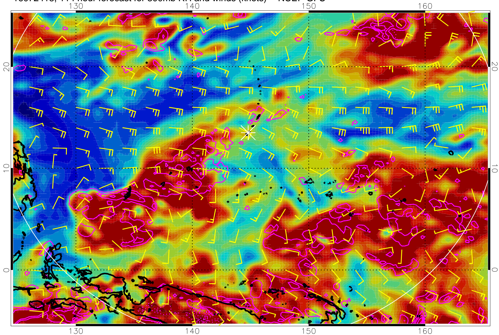
16072418, 114 hour forecast for 300mb RH and winds (knots) -- NCEP GFS
