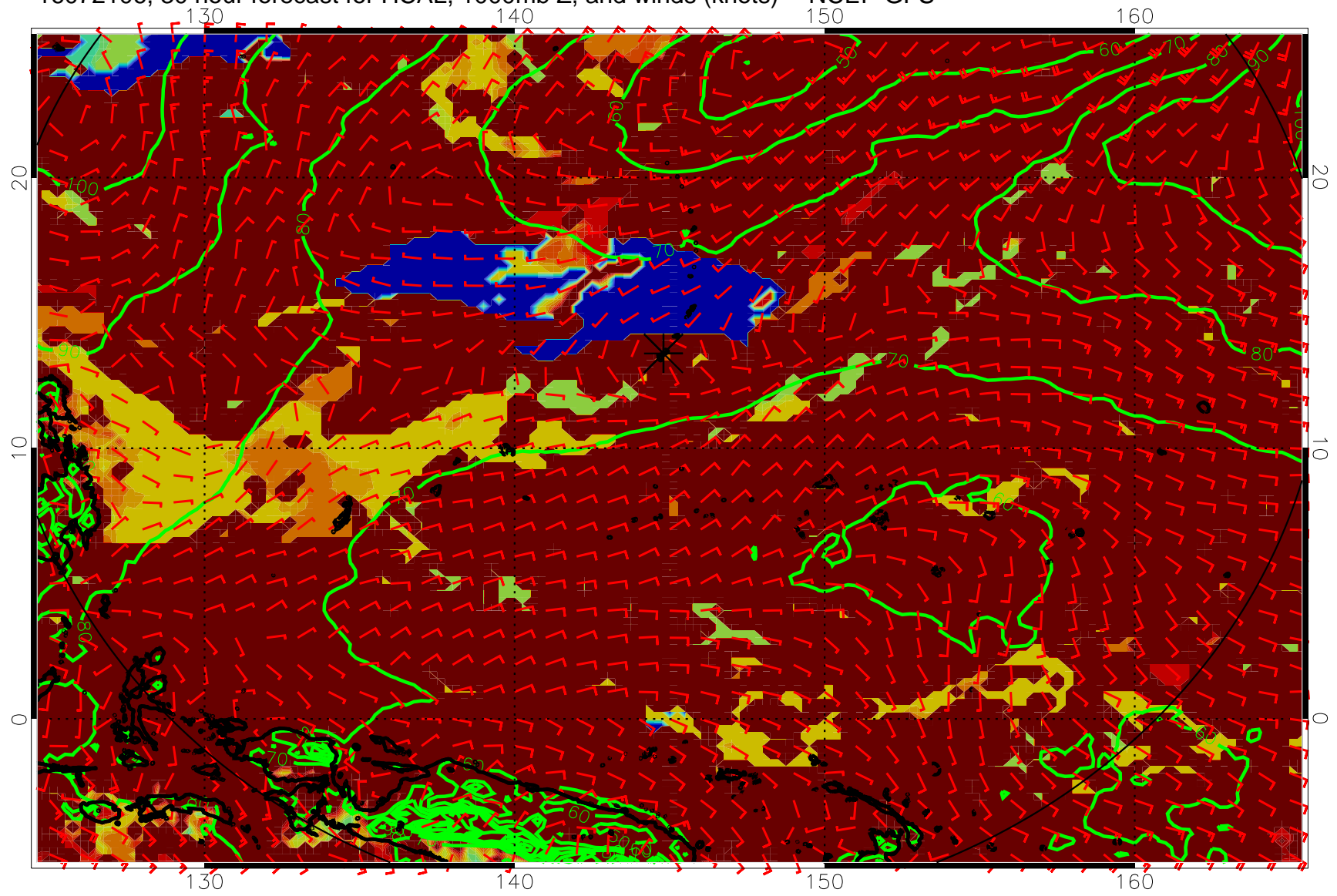
16072106, 30 hour forecast for HCAL, 1000mb Z, and winds (knots) -- NCEP GFS
