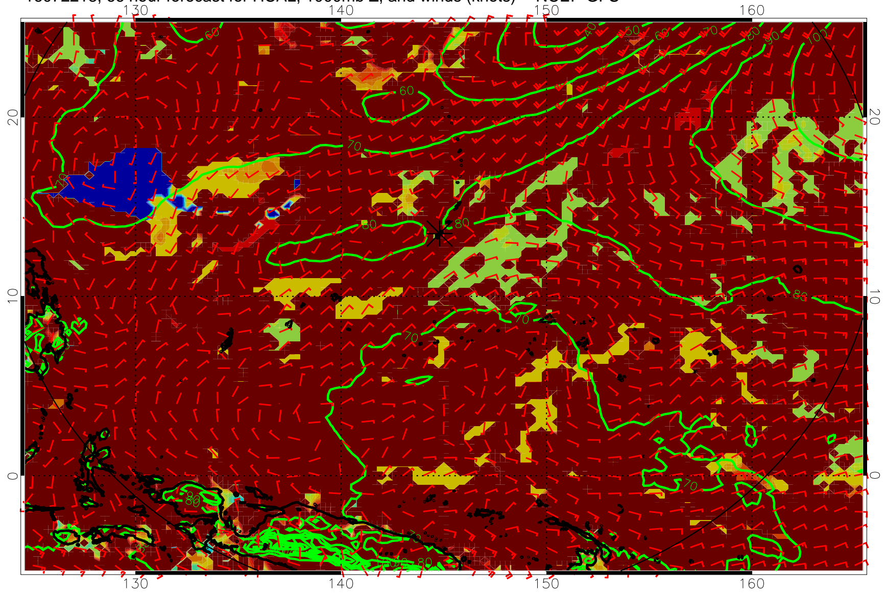
16072218, 66 hour forecast for HCAL, 1000mb Z, and winds (knots) -- NCEP GFS
