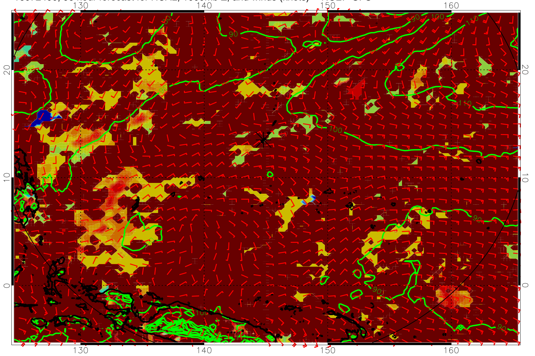
16072400, 96 hour forecast for HCAL, 1000mb Z, and winds (knots) -- NCEP GFS
