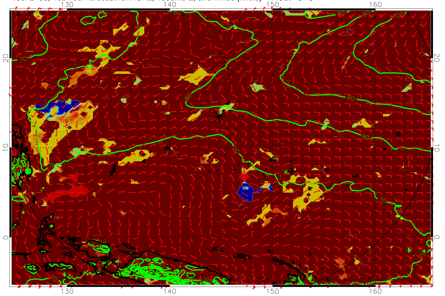
16072406, 102 hour forecast for HCAL, 1000mb Z, and winds (knots) -- NCEP GFS
