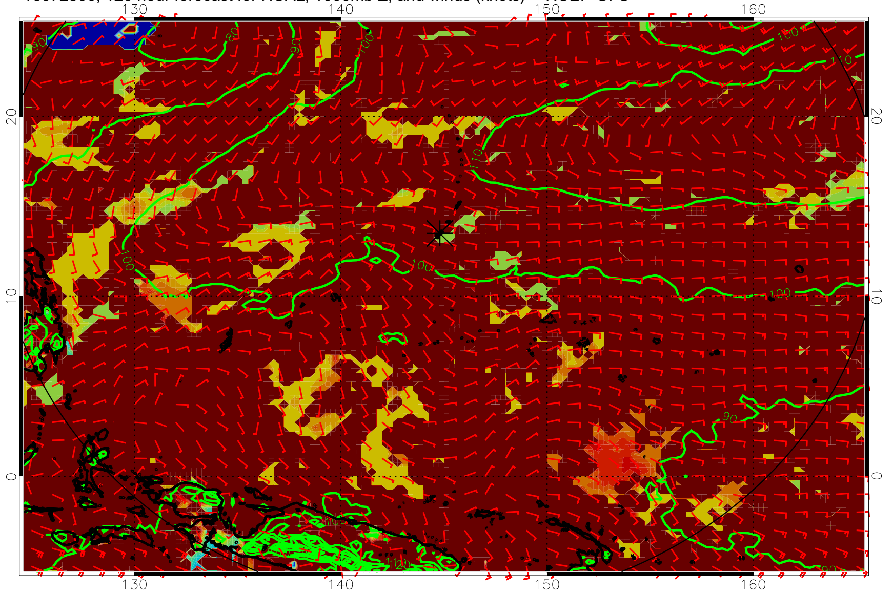
16072500, 120 hour forecast for HCAL, 1000mb Z, and winds (knots) -- NCEP GFS
