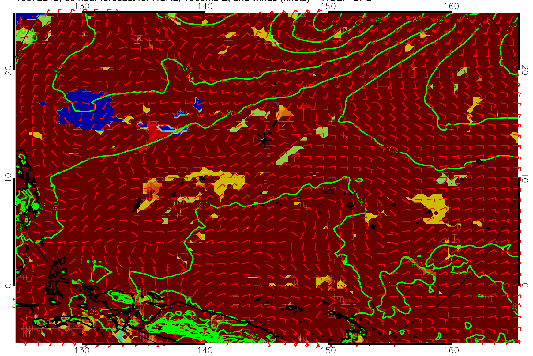
16072212, 60 hour forecast for HCAL, 1000mb Z, and winds (knots) -- NCEP GFS
