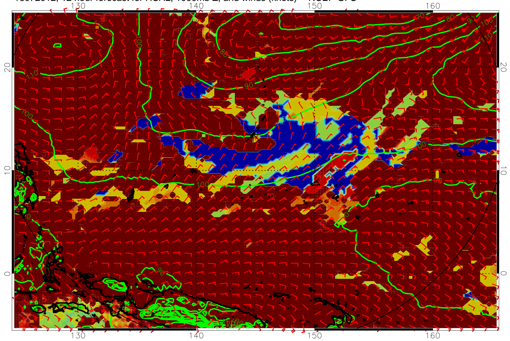
16072012, 12 hour forecast for HCAL, 1000mb Z, and winds (knots) -- NCEP GFS
