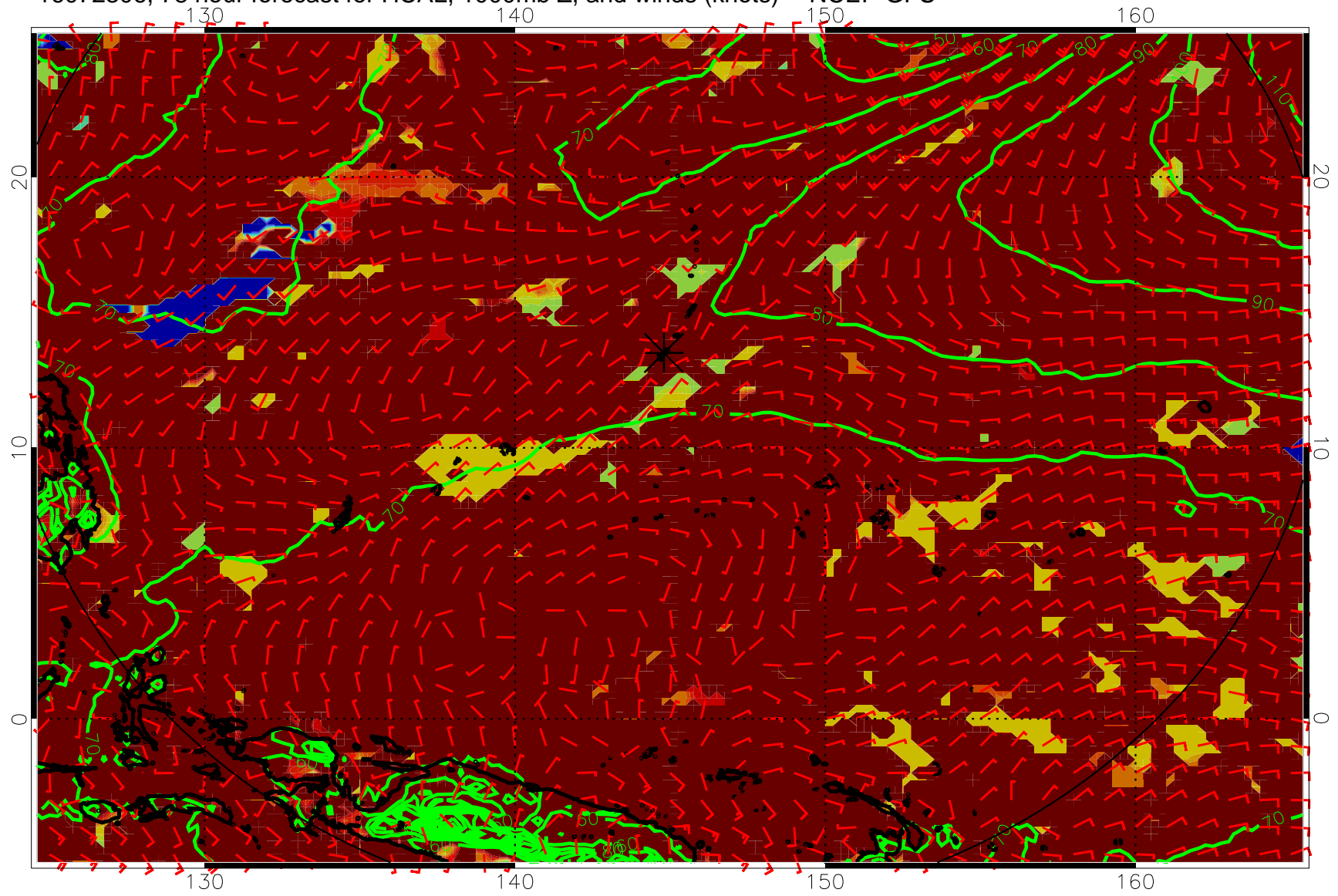
16072306, 78 hour forecast for HCAL, 1000mb Z, and winds (knots) -- NCEP GFS
