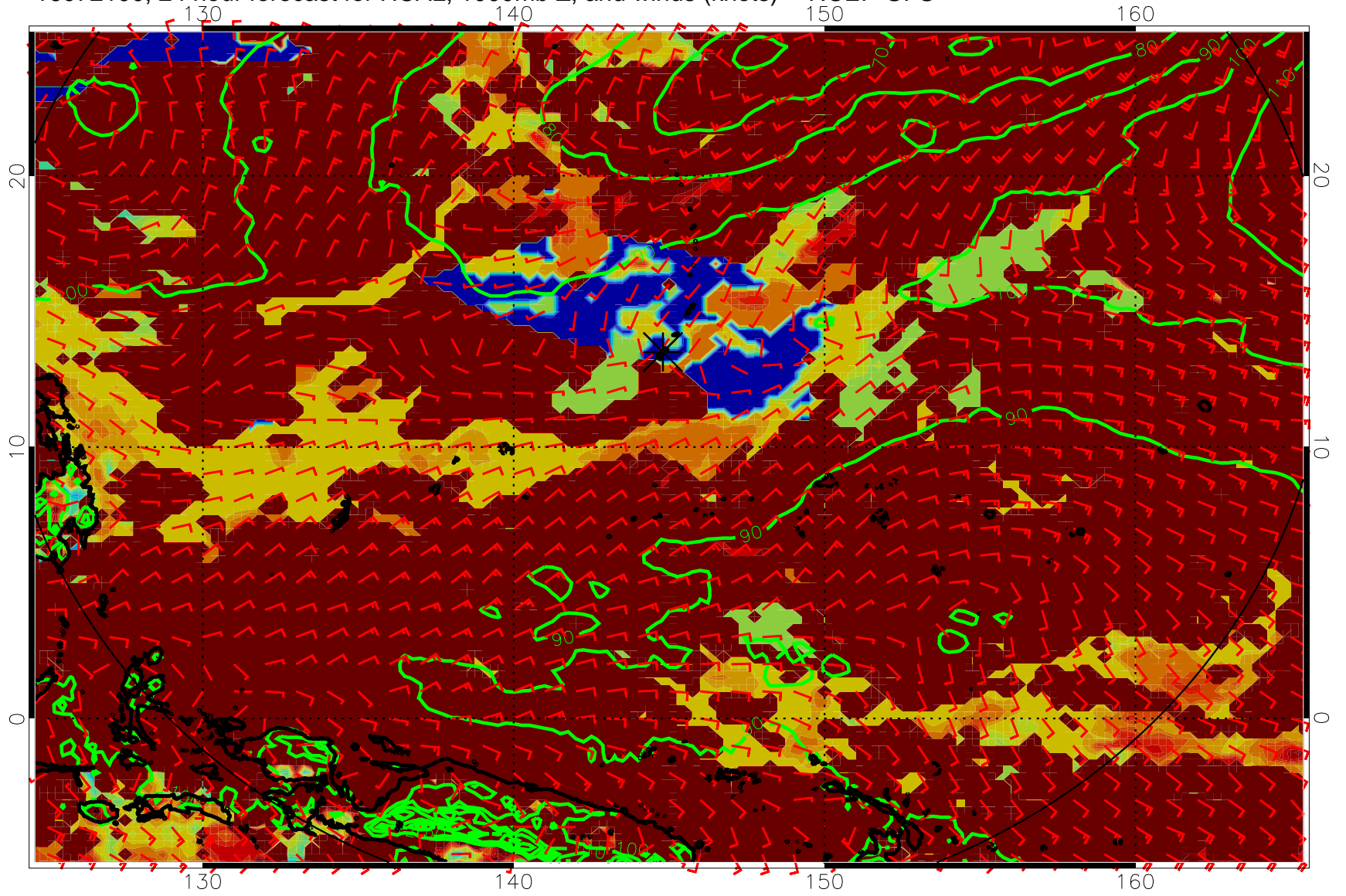
16072100, 24 hour forecast for HCAL, 1000mb Z, and winds (knots) -- NCEP GFS
