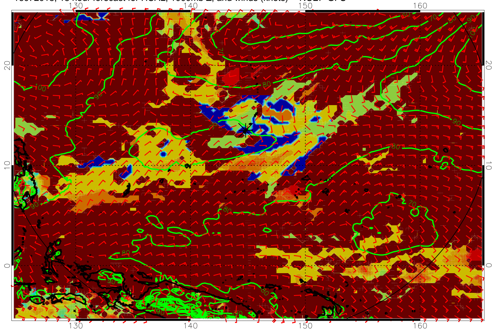
16072018, 18 hour forecast for HCAL, 1000mb Z, and winds (knots) -- NCEP GFS
