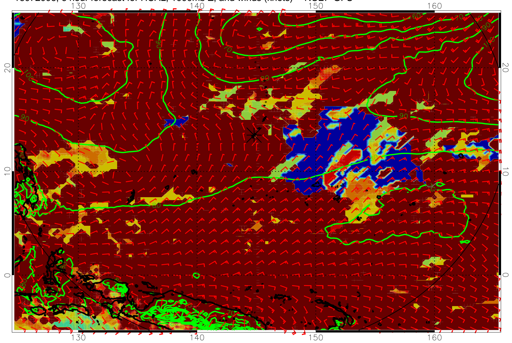
16072006, 6 hour forecast for HCAL, 1000mb Z, and winds (knots) -- NCEP GFS
