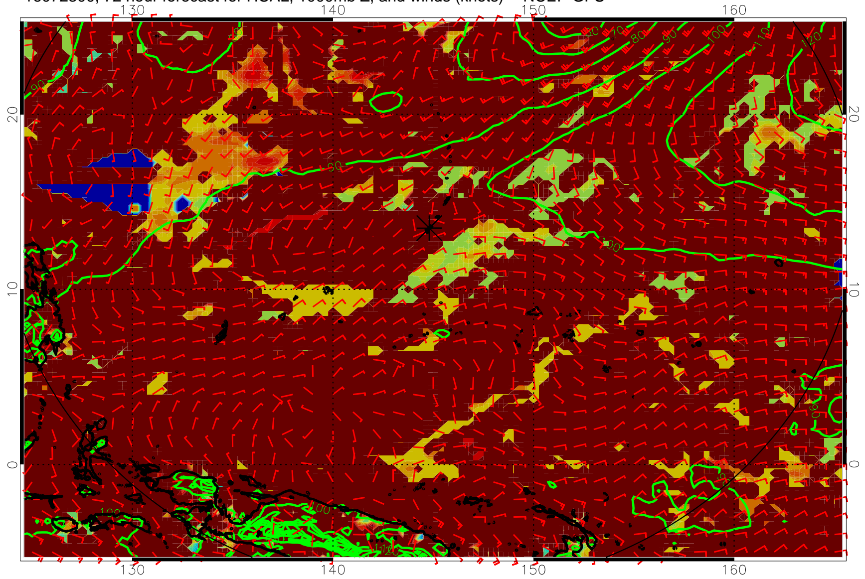
16072300, 72 hour forecast for HCAL, 1000mb Z, and winds (knots) -- NCEP GFS
