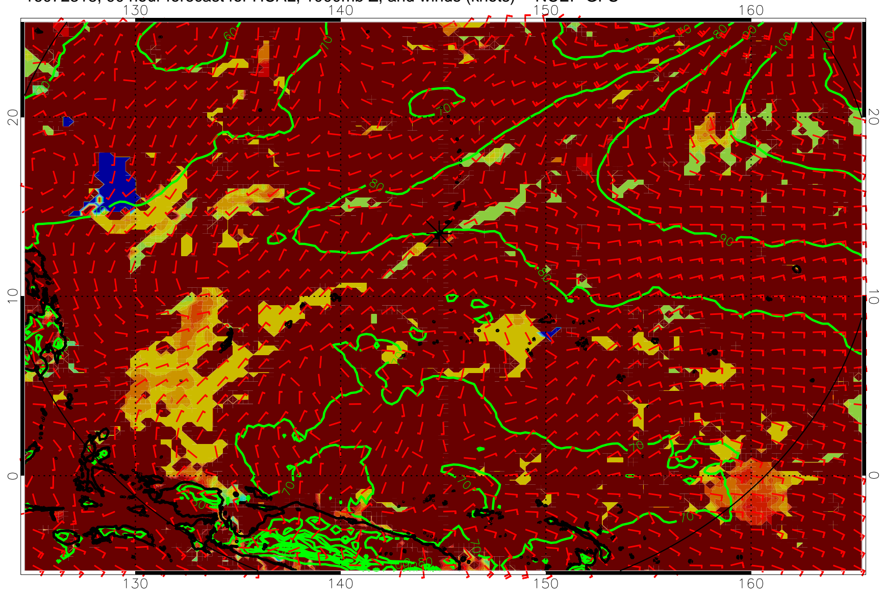
16072318, 90 hour forecast for HCAL, 1000mb Z, and winds (knots) -- NCEP GFS
