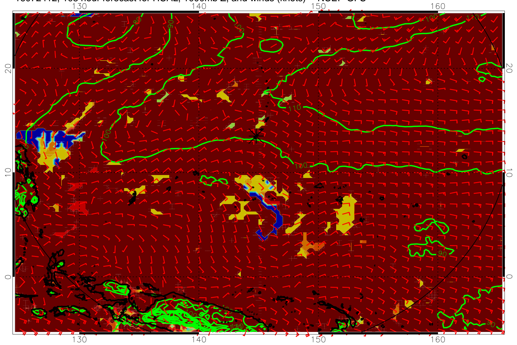
16072412, 108 hour forecast for HCAL, 1000mb Z, and winds (knots) -- NCEP GFS
