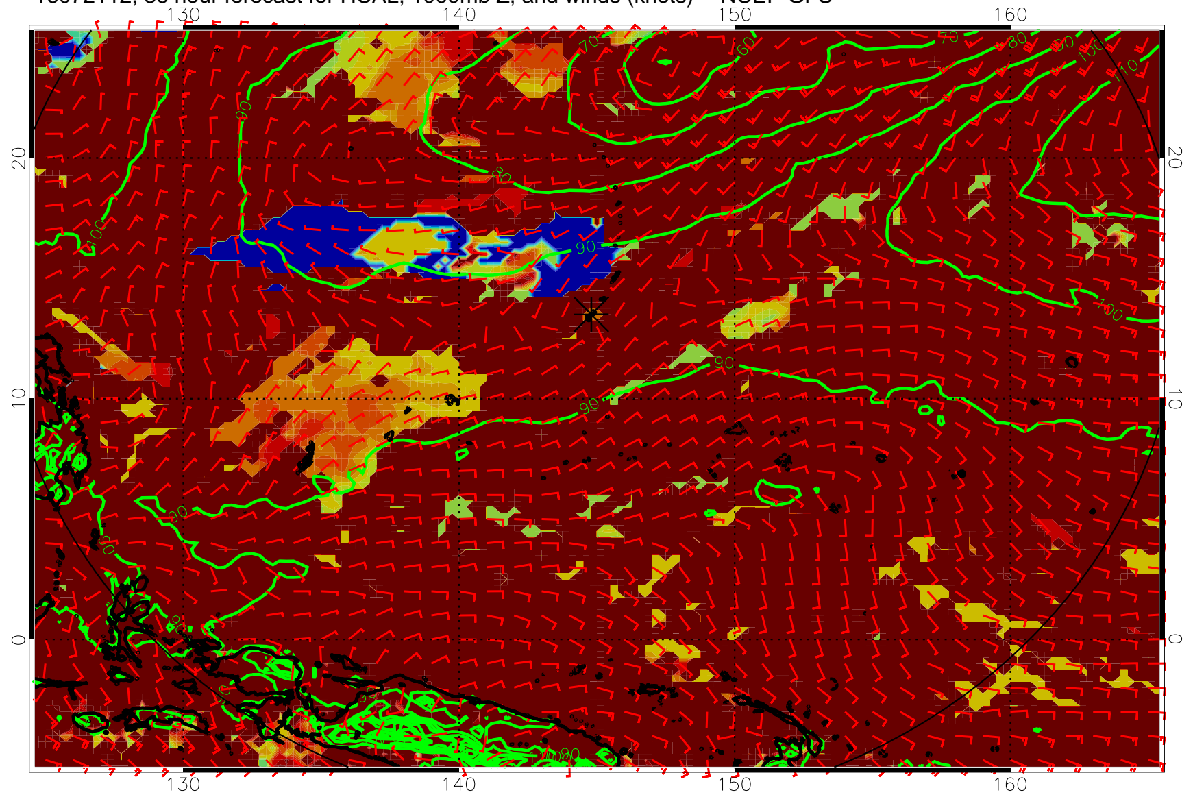
16072112, 36 hour forecast for HCAL, 1000mb Z, and winds (knots) -- NCEP GFS
