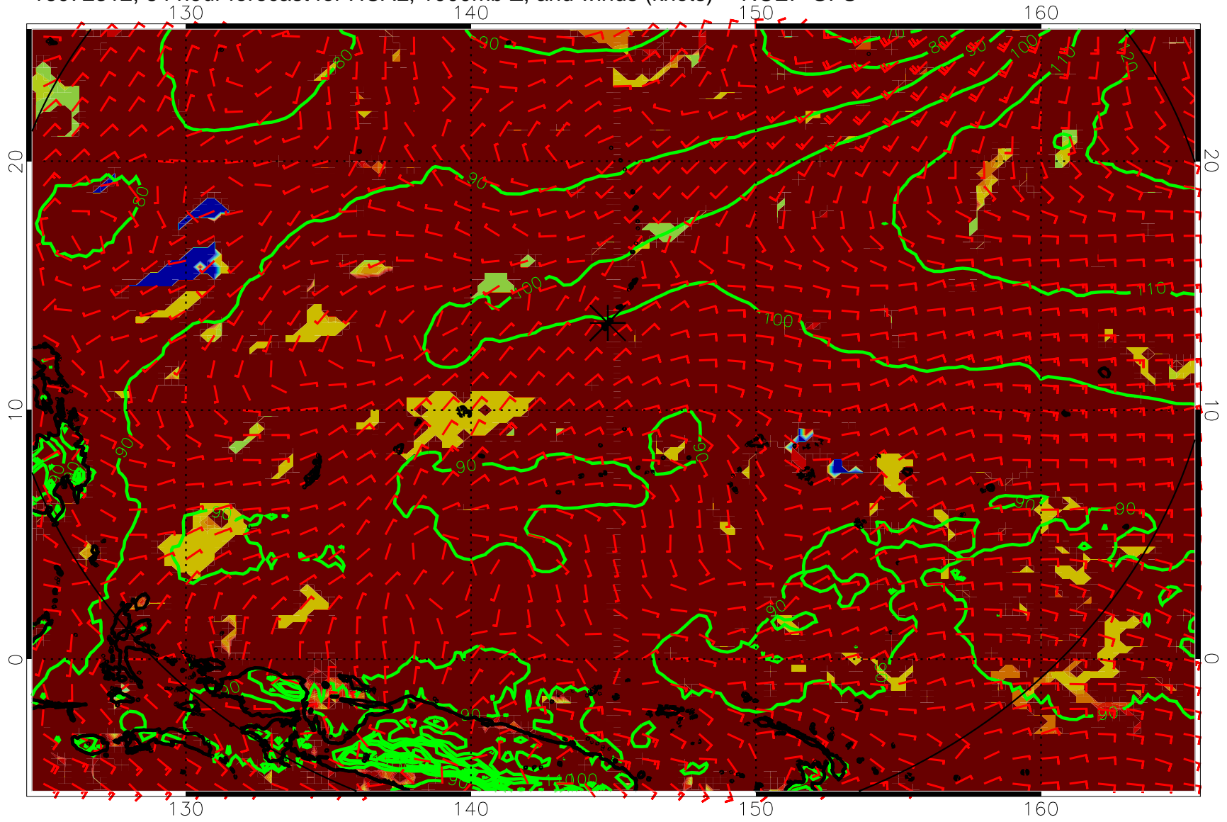
16072312, 84 hour forecast for HCAL, 1000mb Z, and winds (knots) -- NCEP GFS
