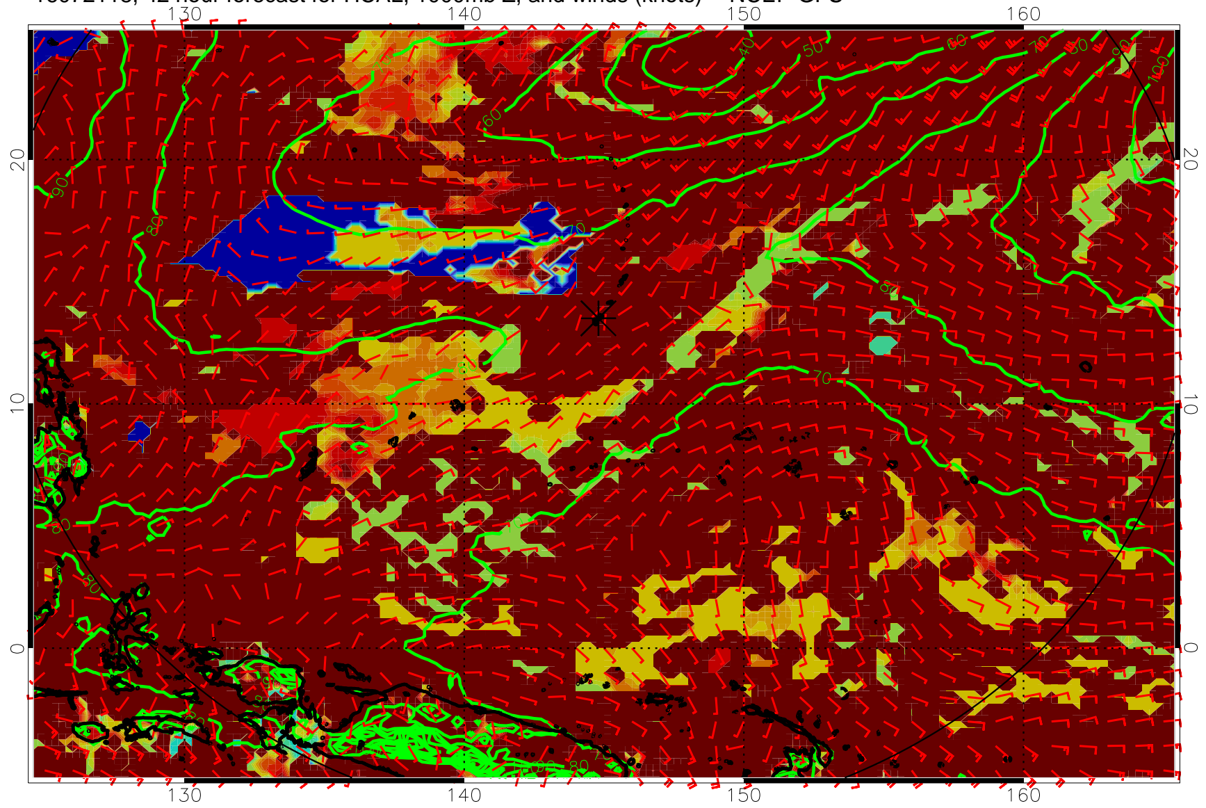
16072118, 42 hour forecast for HCAL, 1000mb Z, and winds (knots) -- NCEP GFS
