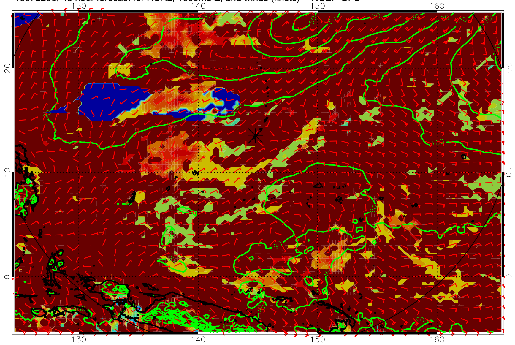
16072200, 48 hour forecast for HCAL, 1000mb Z, and winds (knots) -- NCEP GFS
