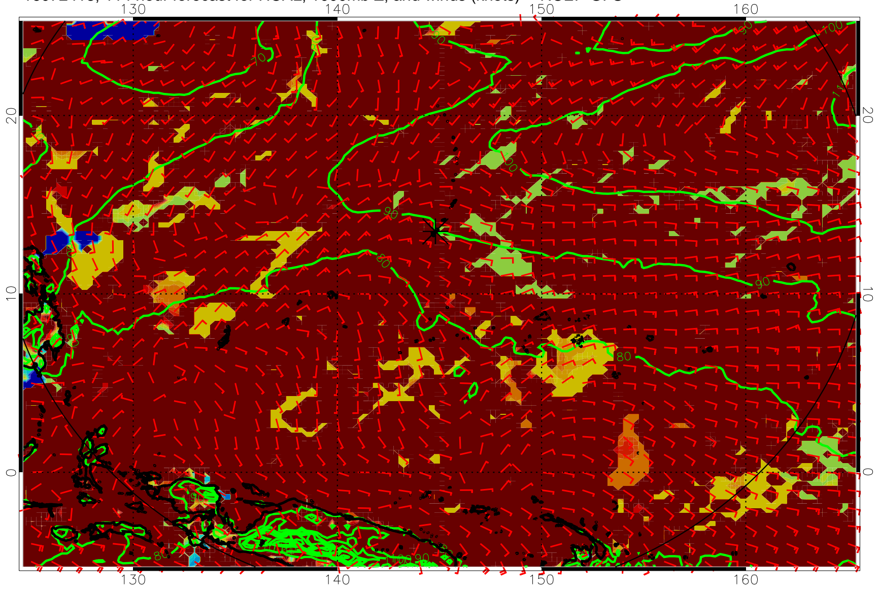
16072418, 114 hour forecast for HCAL, 1000mb Z, and winds (knots) -- NCEP GFS
