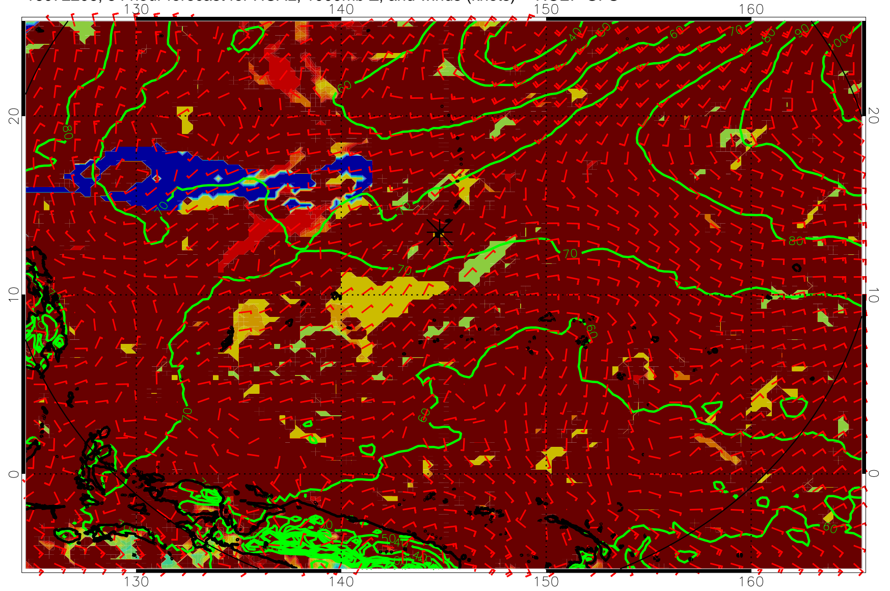
16072206, 54 hour forecast for HCAL, 1000mb Z, and winds (knots) -- NCEP GFS
