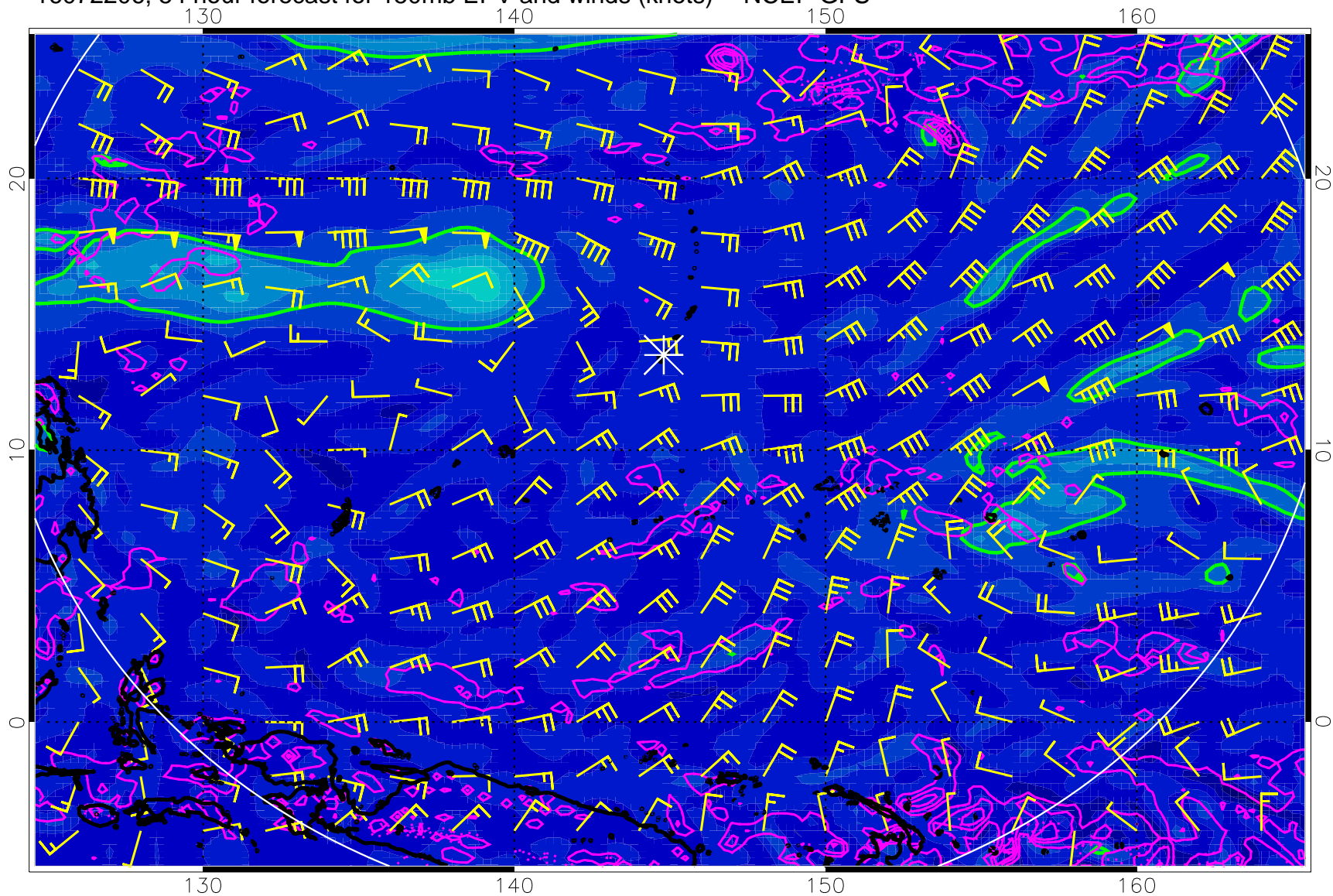
16072206, 54 hour forecast for 150mb EPV and winds (knots) -- NCEP GFS
