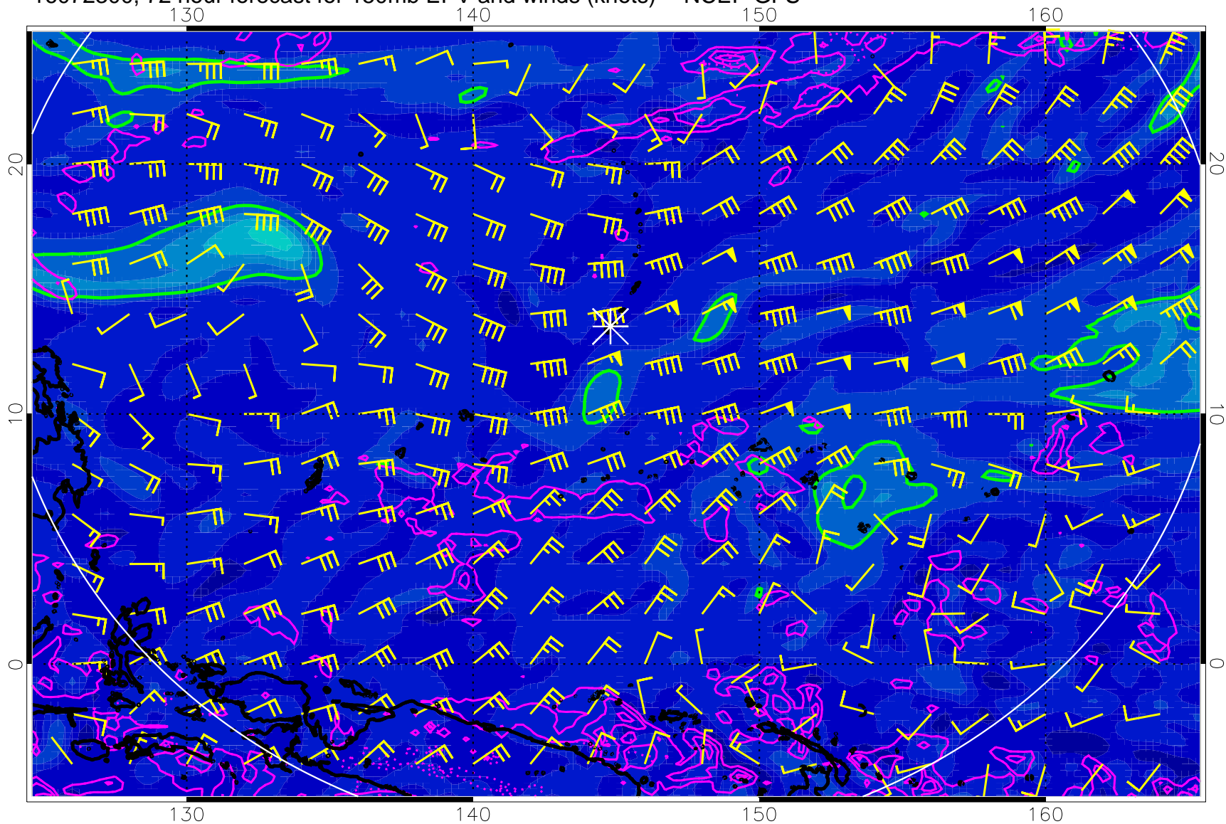
16072300, 72 hour forecast for 150mb EPV and winds (knots) -- NCEP GFS
