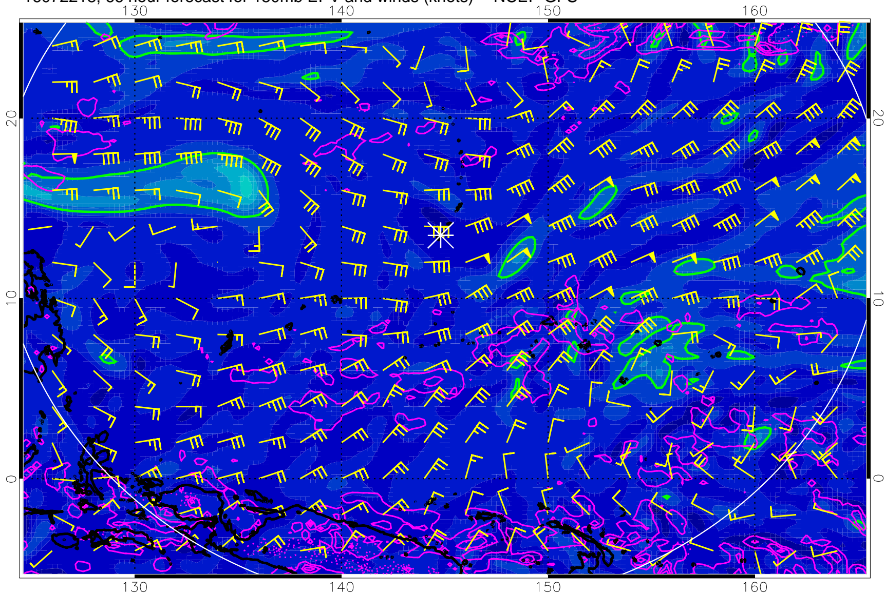
16072218, 66 hour forecast for 150mb EPV and winds (knots) -- NCEP GFS
