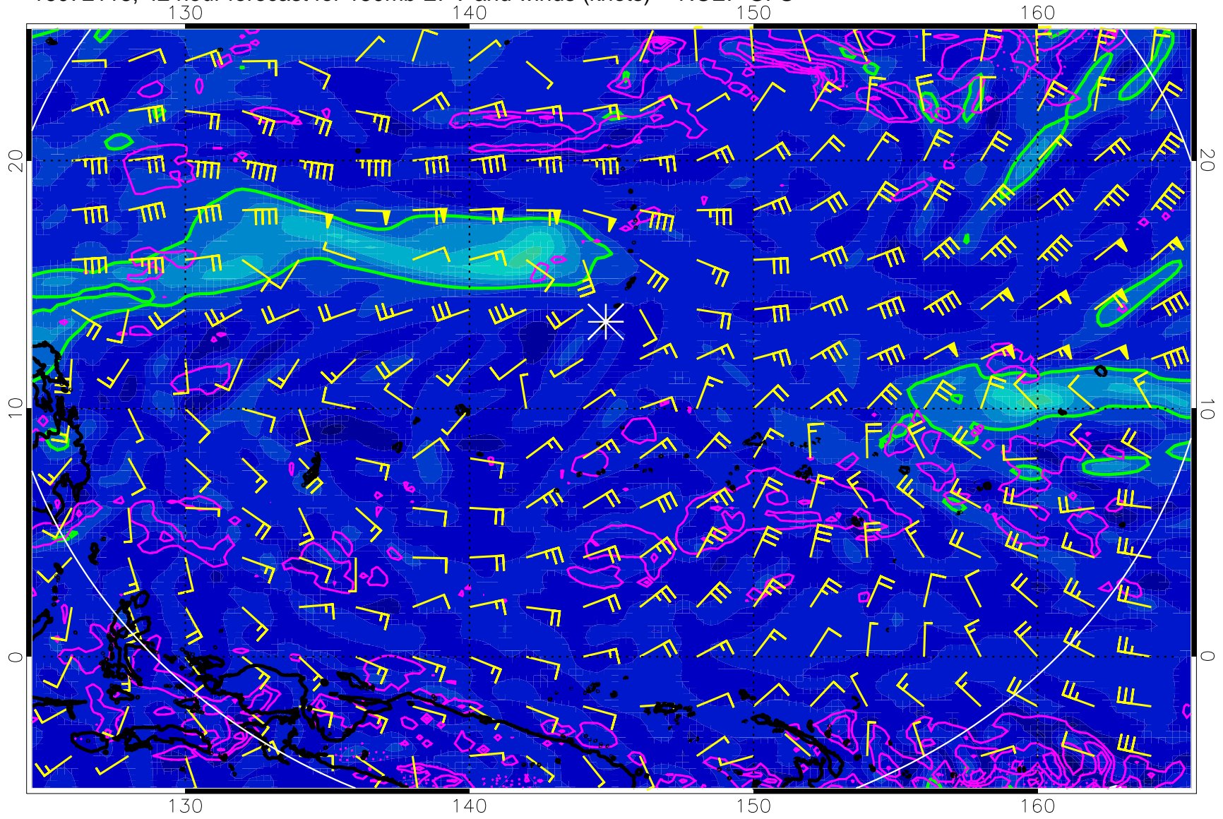
16072118, 42 hour forecast for 150mb EPV and winds (knots) -- NCEP GFS
