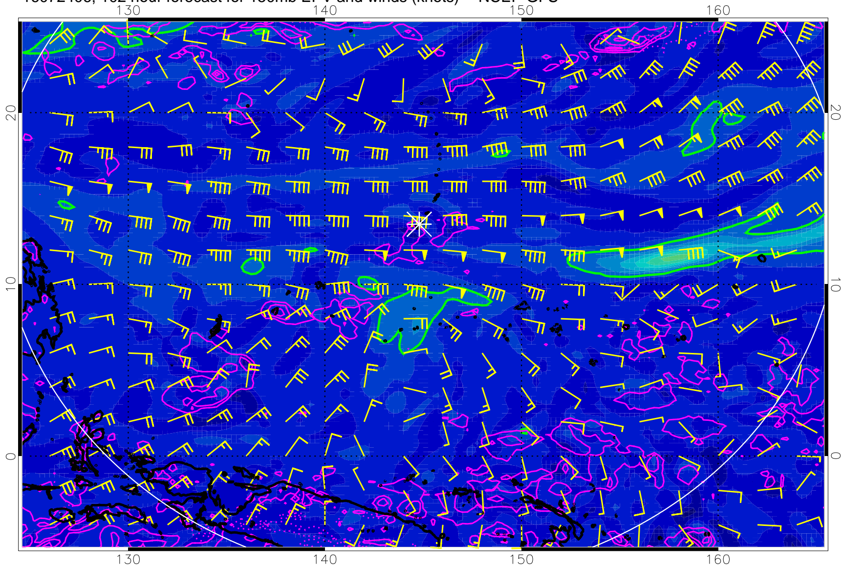
16072406, 102 hour forecast for 150mb EPV and winds (knots) -- NCEP GFS
