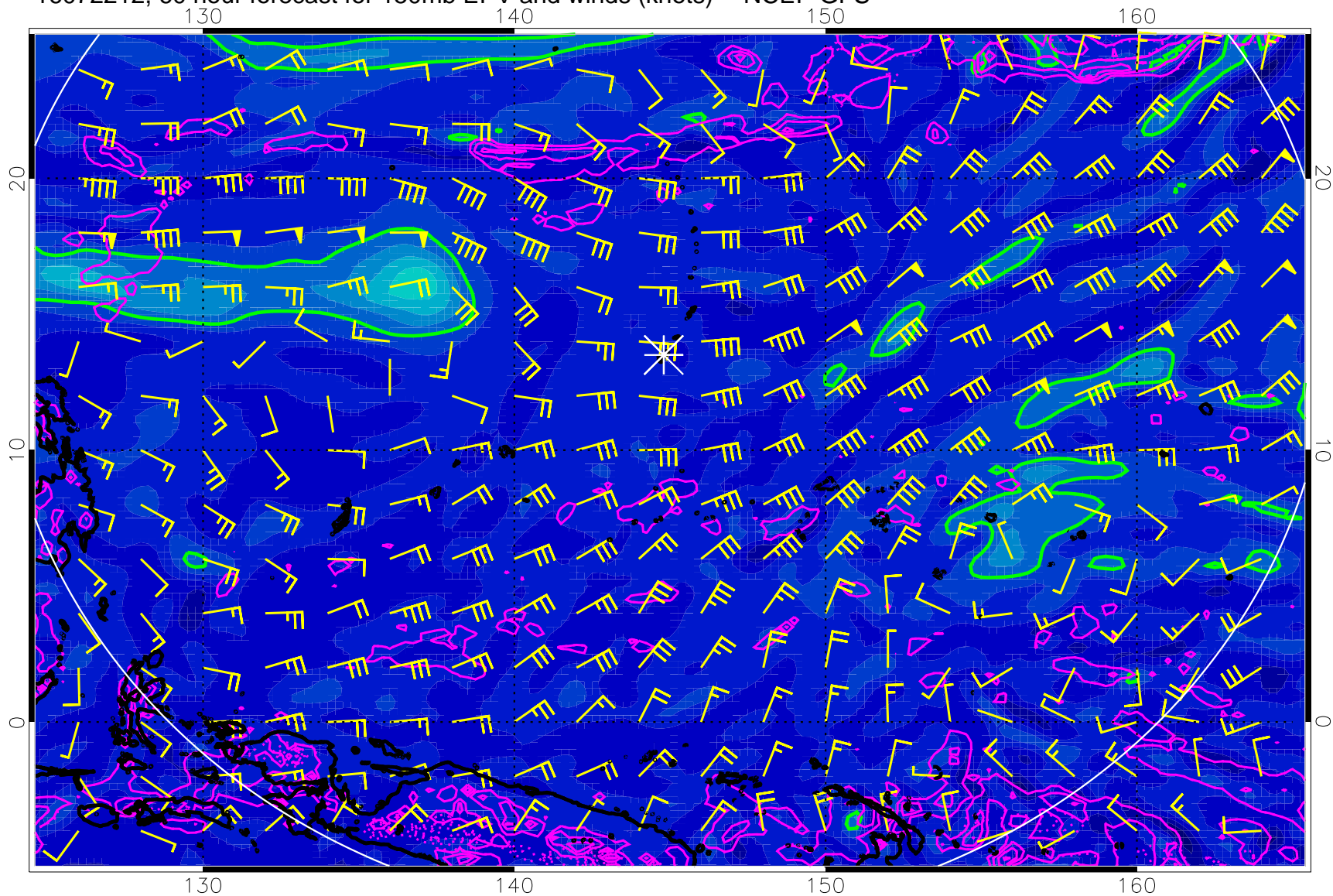
16072212, 60 hour forecast for 150mb EPV and winds (knots) -- NCEP GFS
