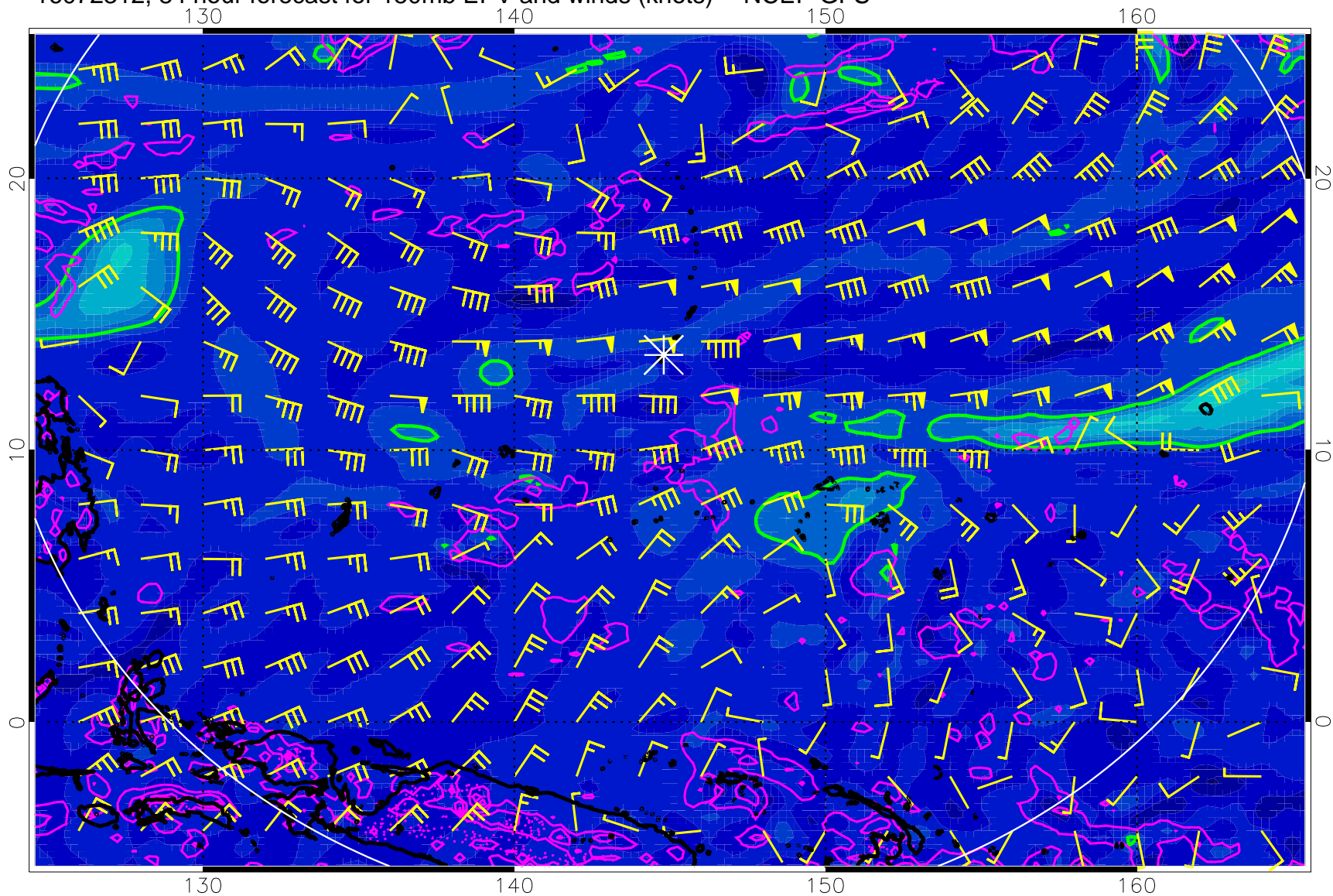
16072312, 84 hour forecast for 150mb EPV and winds (knots) -- NCEP GFS
