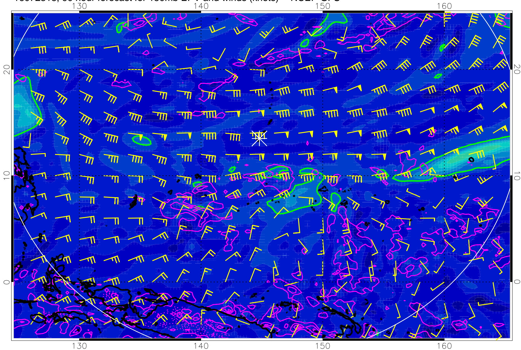
16072318, 90 hour forecast for 150mb EPV and winds (knots) -- NCEP GFS
