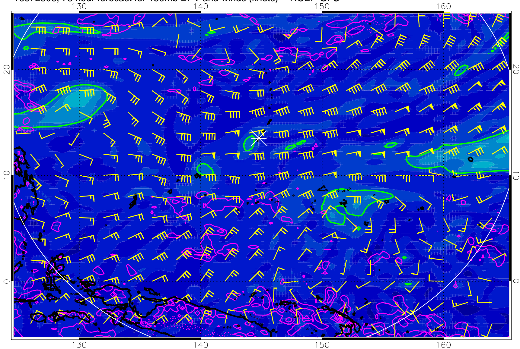
16072306, 78 hour forecast for 150mb EPV and winds (knots) -- NCEP GFS
