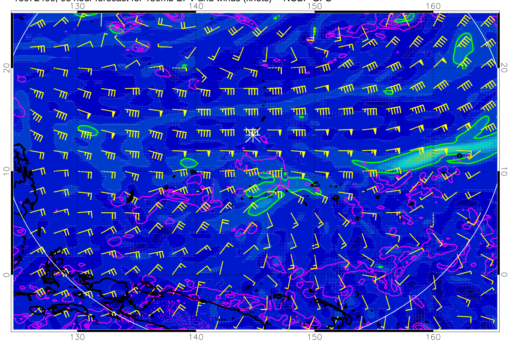
16072400, 96 hour forecast for 150mb EPV and winds (knots) -- NCEP GFS
