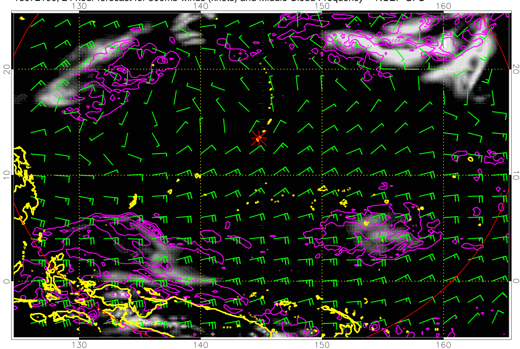
16072100, 24 hour forecast for 500mb winds (knots) and Middle Cloud Frequency -- NCEP GFS
