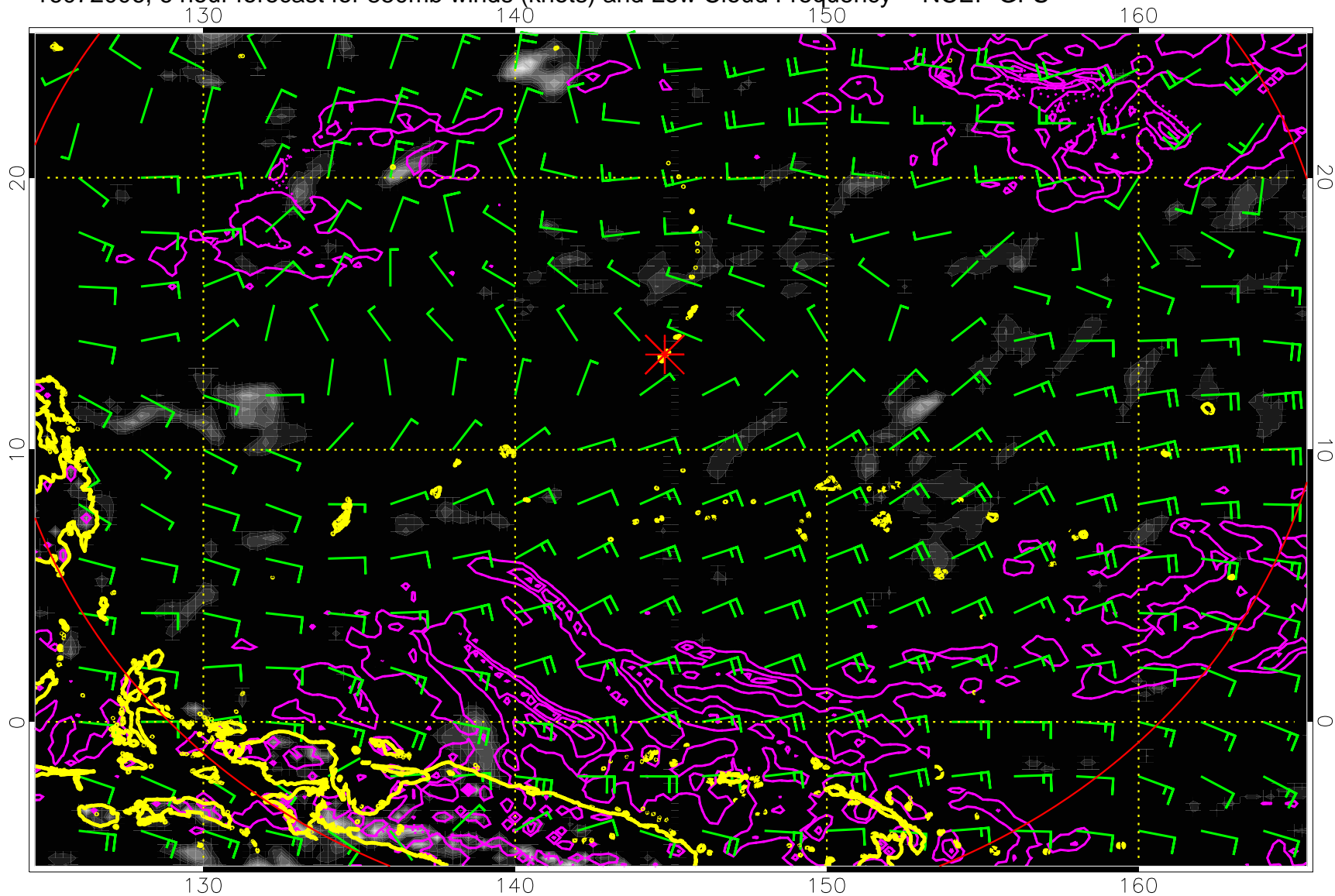
16072006, 6 hour forecast for 850mb winds (knots) and Low Cloud Frequency -- NCEP GFS
