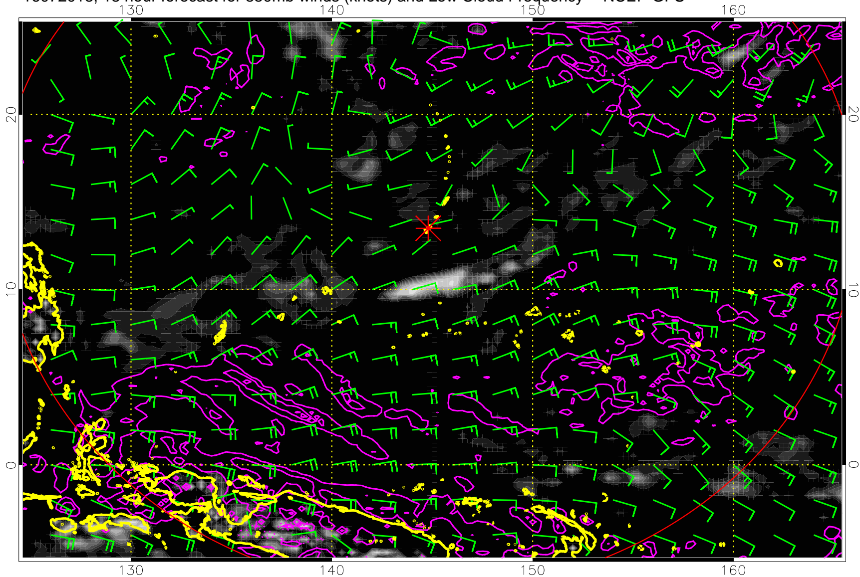
16072018, 18 hour forecast for 850mb winds (knots) and Low Cloud Frequency -- NCEP GFS
