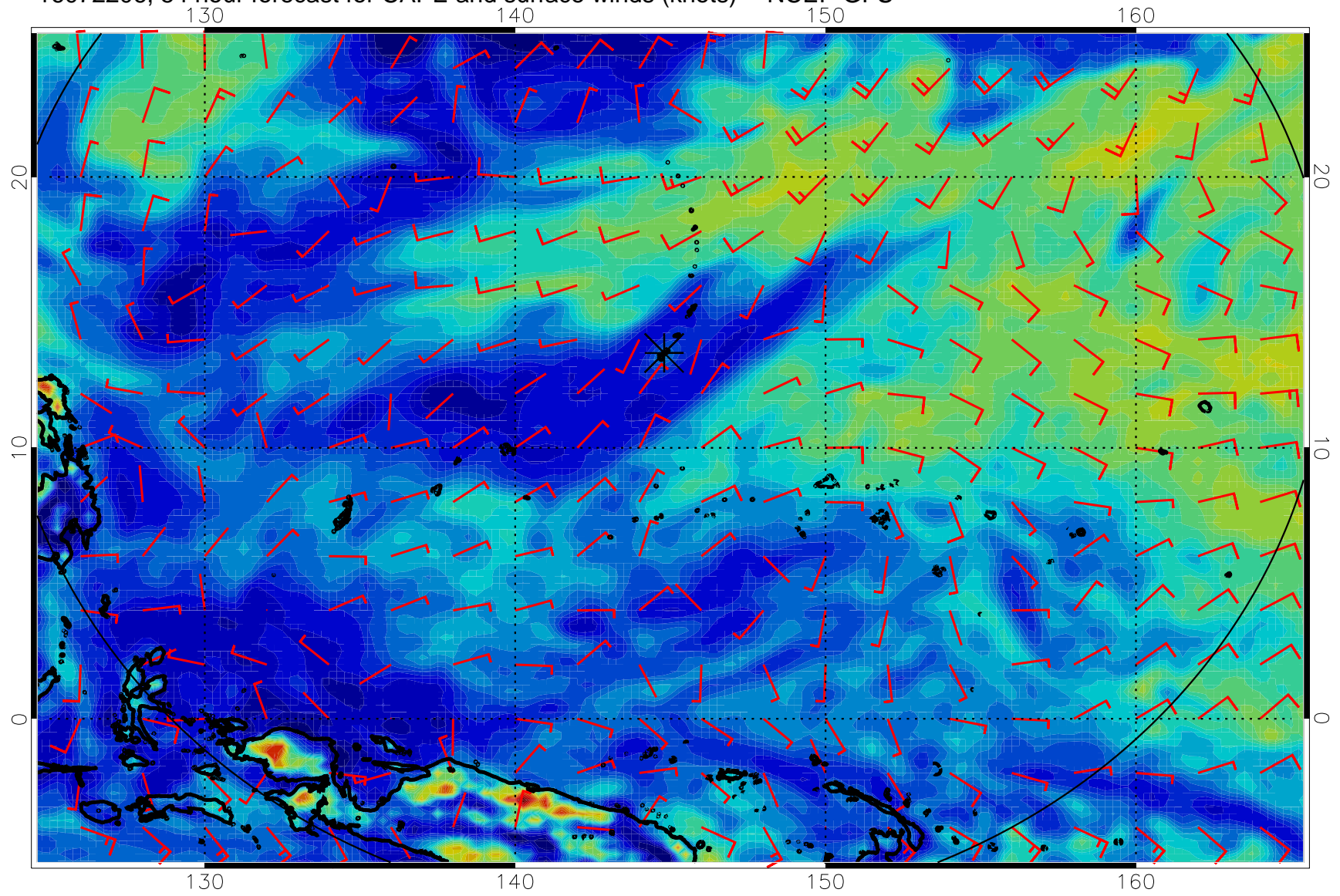
16072206, 54 hour forecast for CAPE and surface winds (knots) -- NCEP GFS
