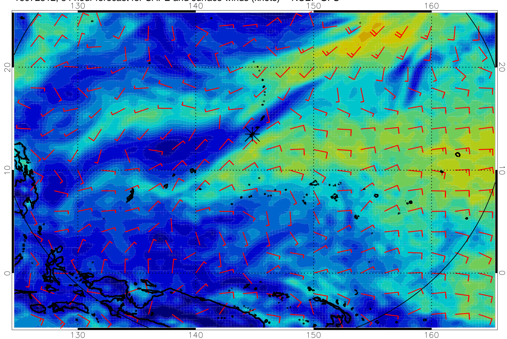
16072312, 84 hour forecast for CAPE and surface winds (knots) -- NCEP GFS
