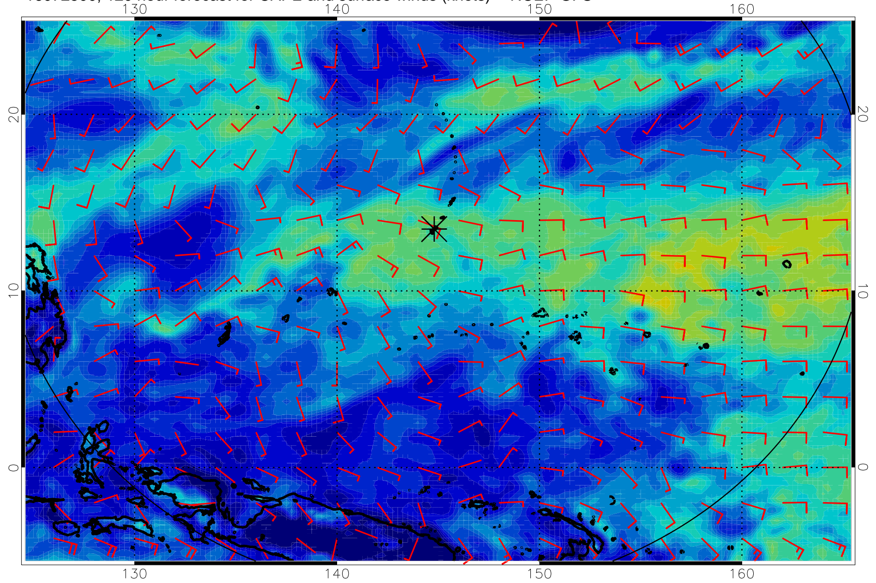
16072500, 120 hour forecast for CAPE and surface winds (knots) -- NCEP GFS
