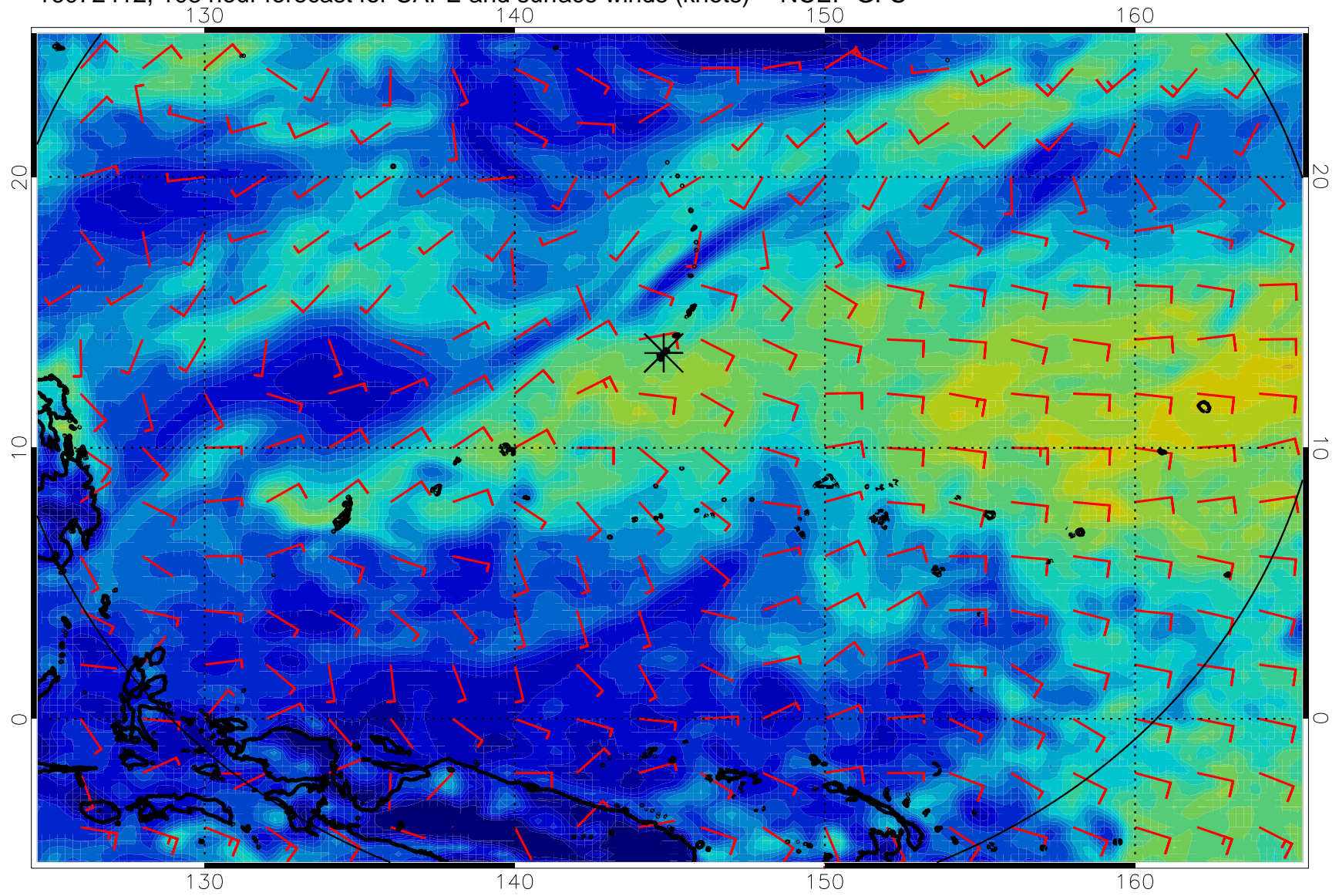
16072412, 108 hour forecast for CAPE and surface winds (knots) -- NCEP GFS
