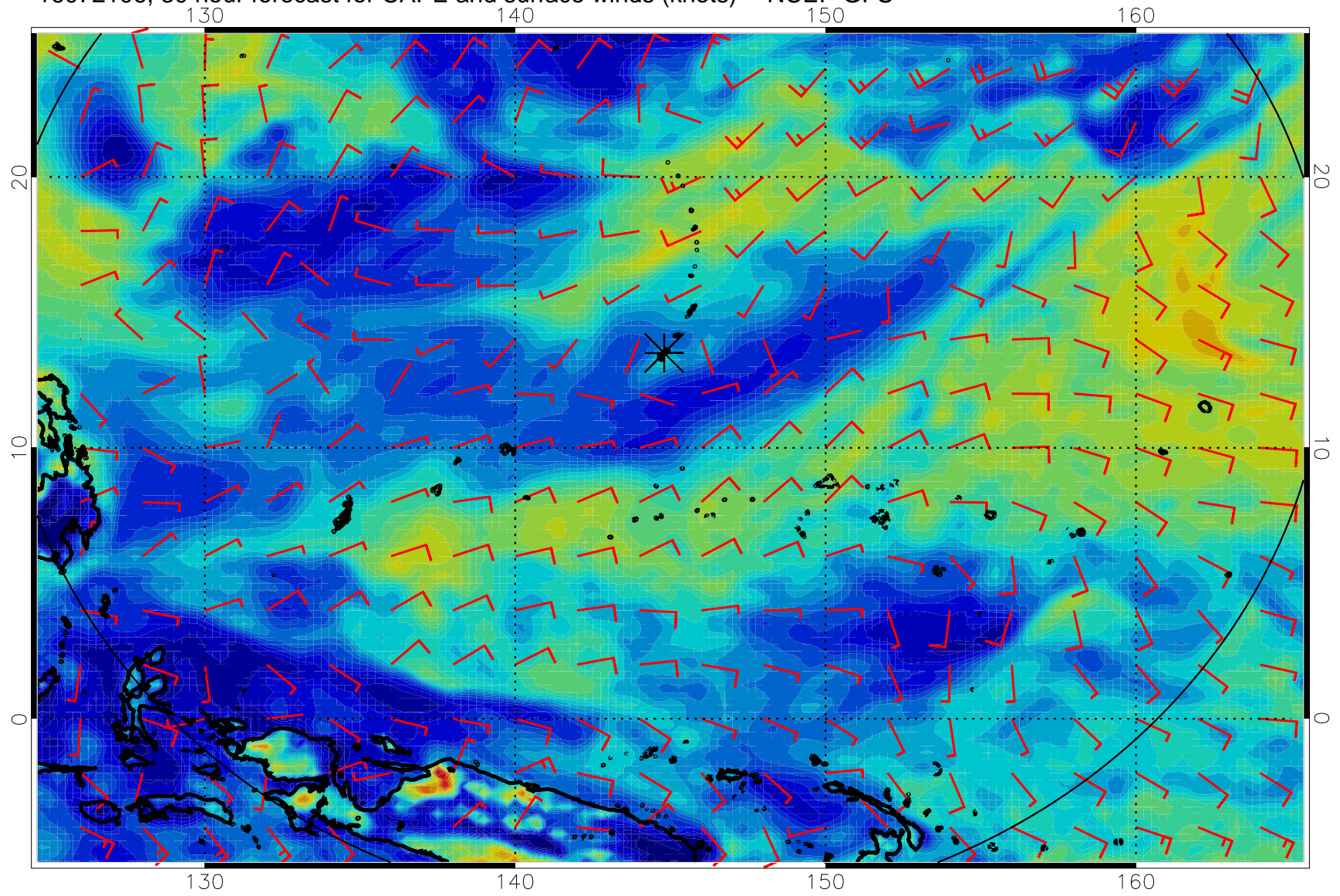
16072106, 30 hour forecast for CAPE and surface winds (knots) -- NCEP GFS
