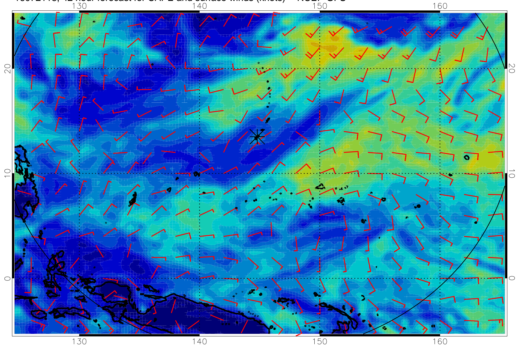
16072118, 42 hour forecast for CAPE and surface winds (knots) -- NCEP GFS
