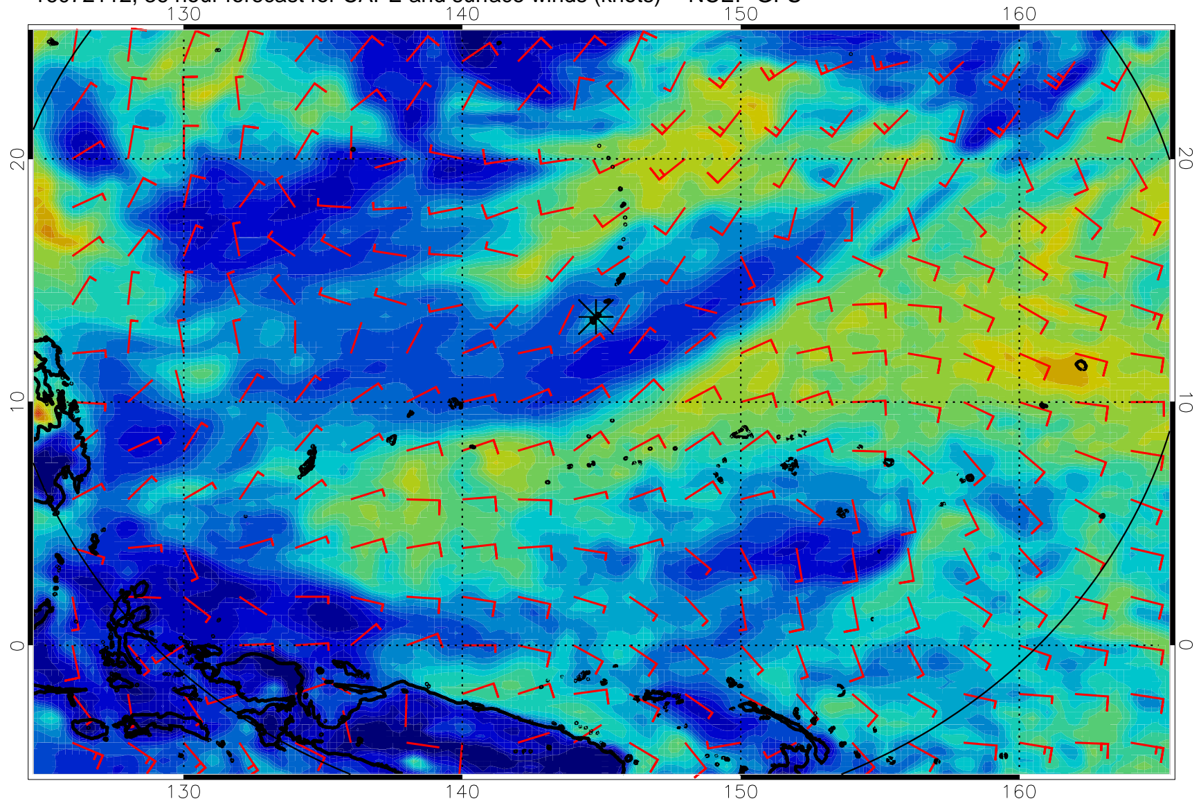
16072112, 36 hour forecast for CAPE and surface winds (knots) -- NCEP GFS
