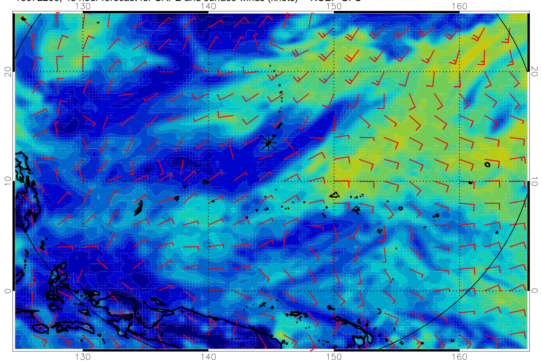
16072200, 48 hour forecast for CAPE and surface winds (knots) -- NCEP GFS
