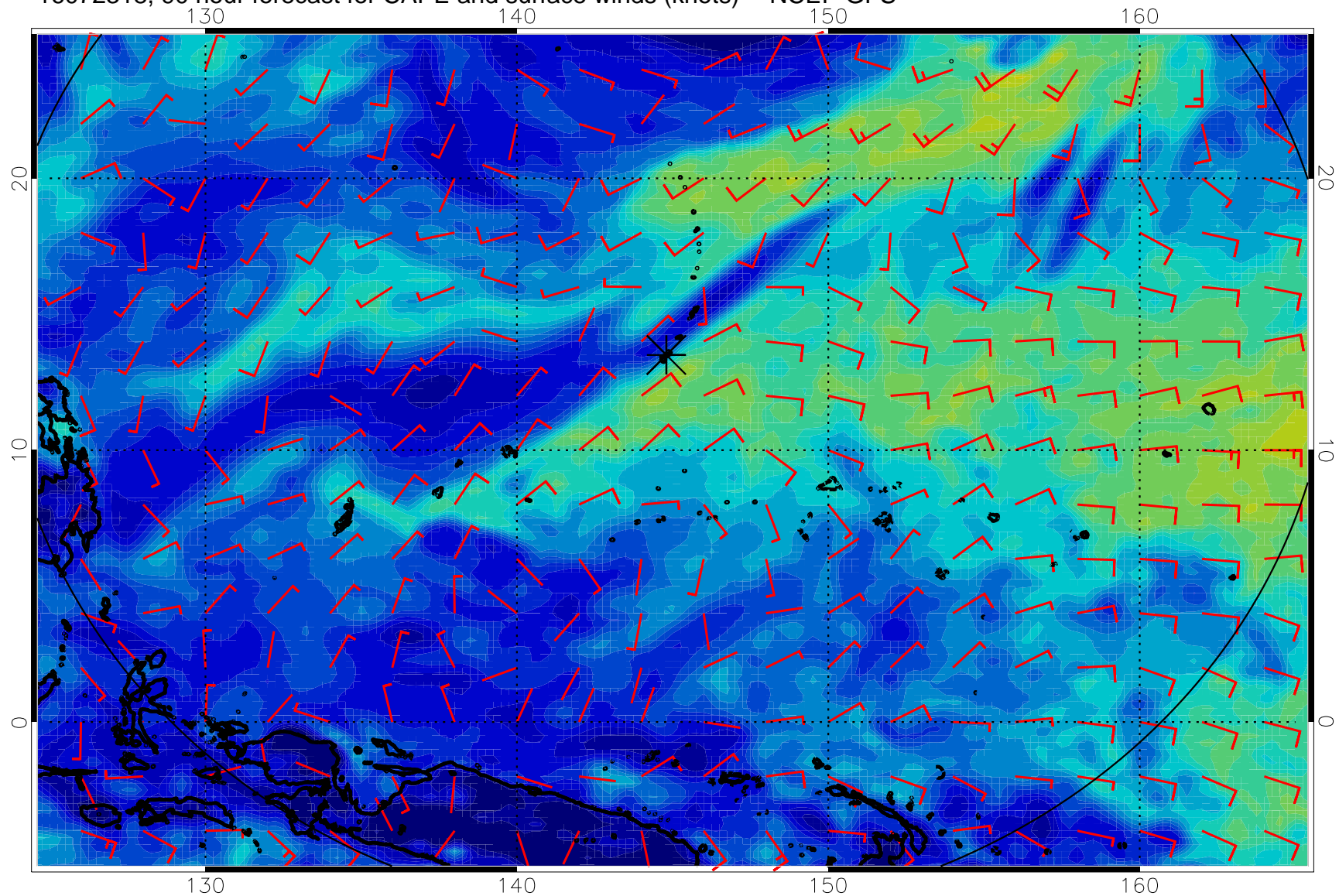
16072318, 90 hour forecast for CAPE and surface winds (knots) -- NCEP GFS
