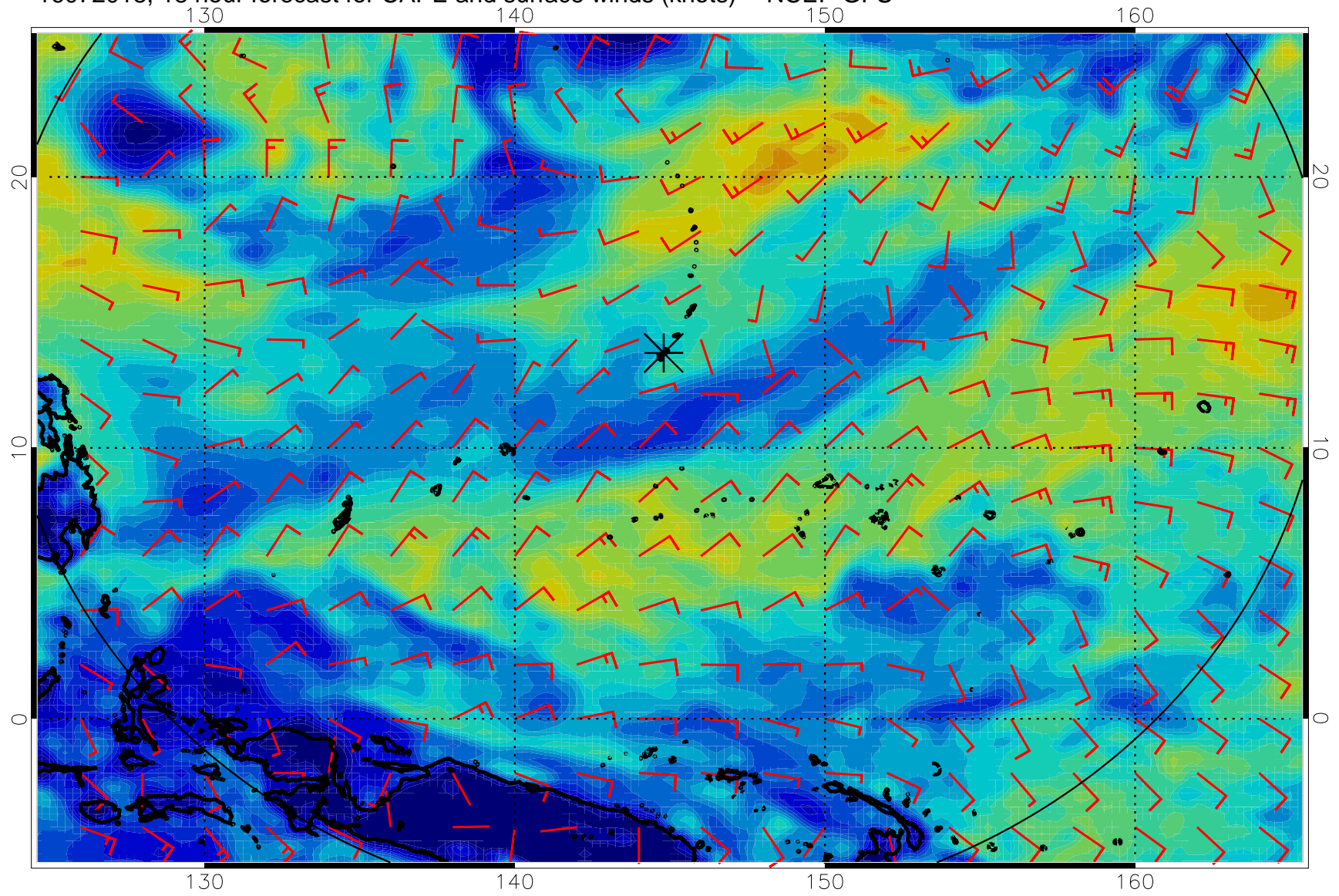
16072018, 18 hour forecast for CAPE and surface winds (knots) -- NCEP GFS
