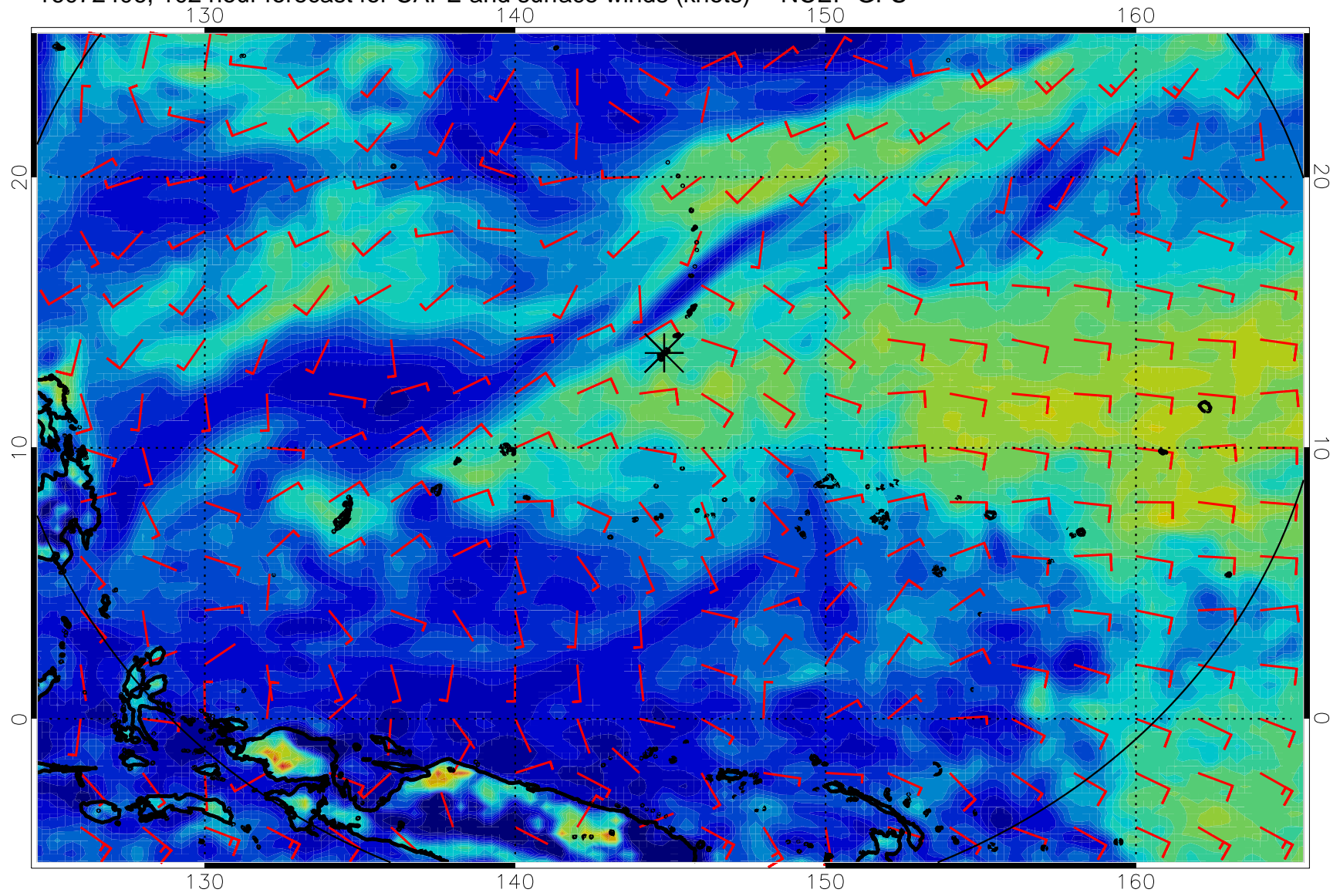
16072406, 102 hour forecast for CAPE and surface winds (knots) -- NCEP GFS
