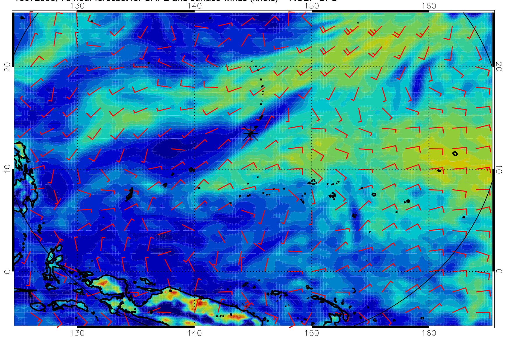
16072306, 78 hour forecast for CAPE and surface winds (knots) -- NCEP GFS
