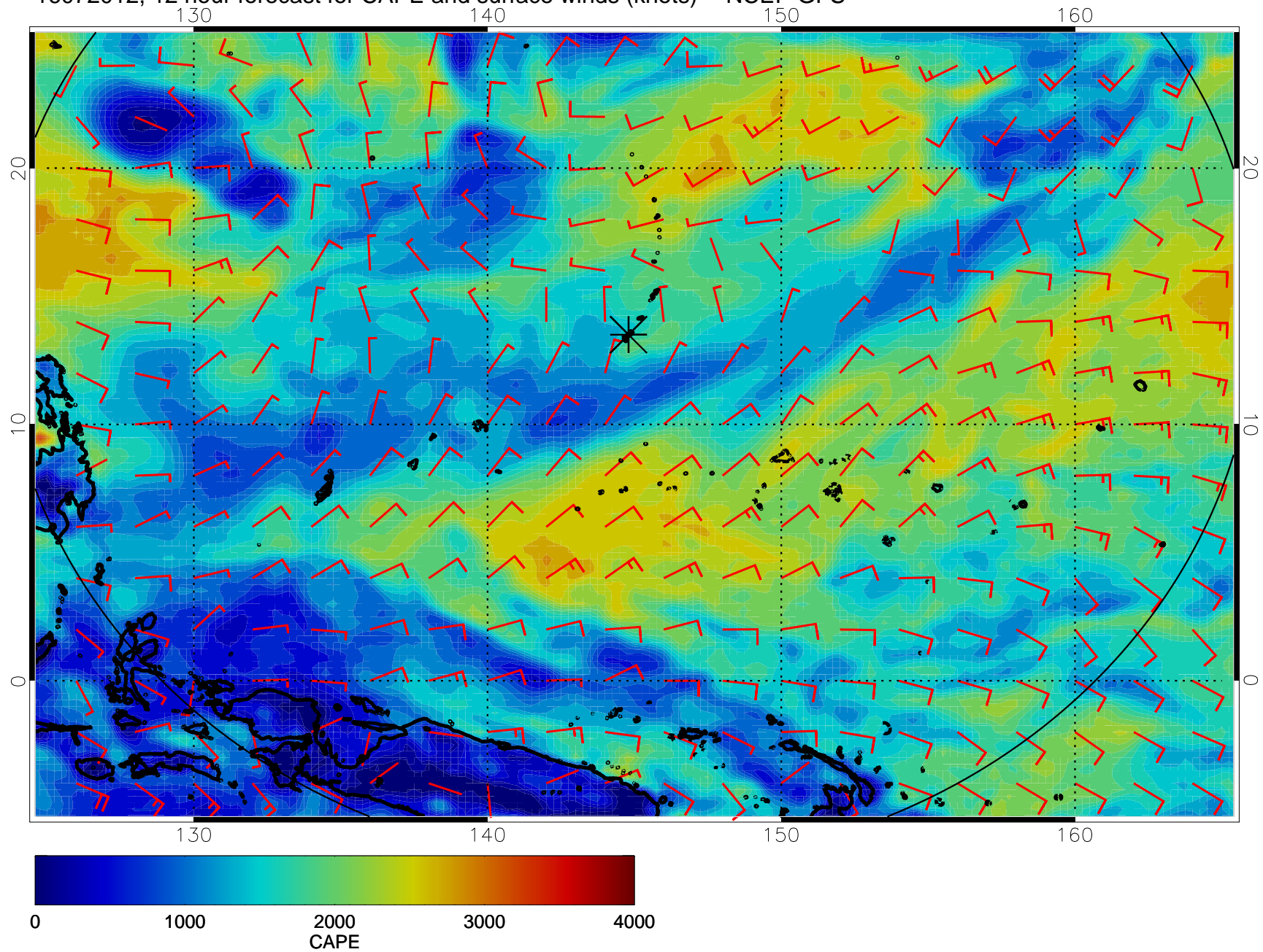
16072012, 12 hour forecast for CAPE and surface winds (knots) -- NCEP GFS
