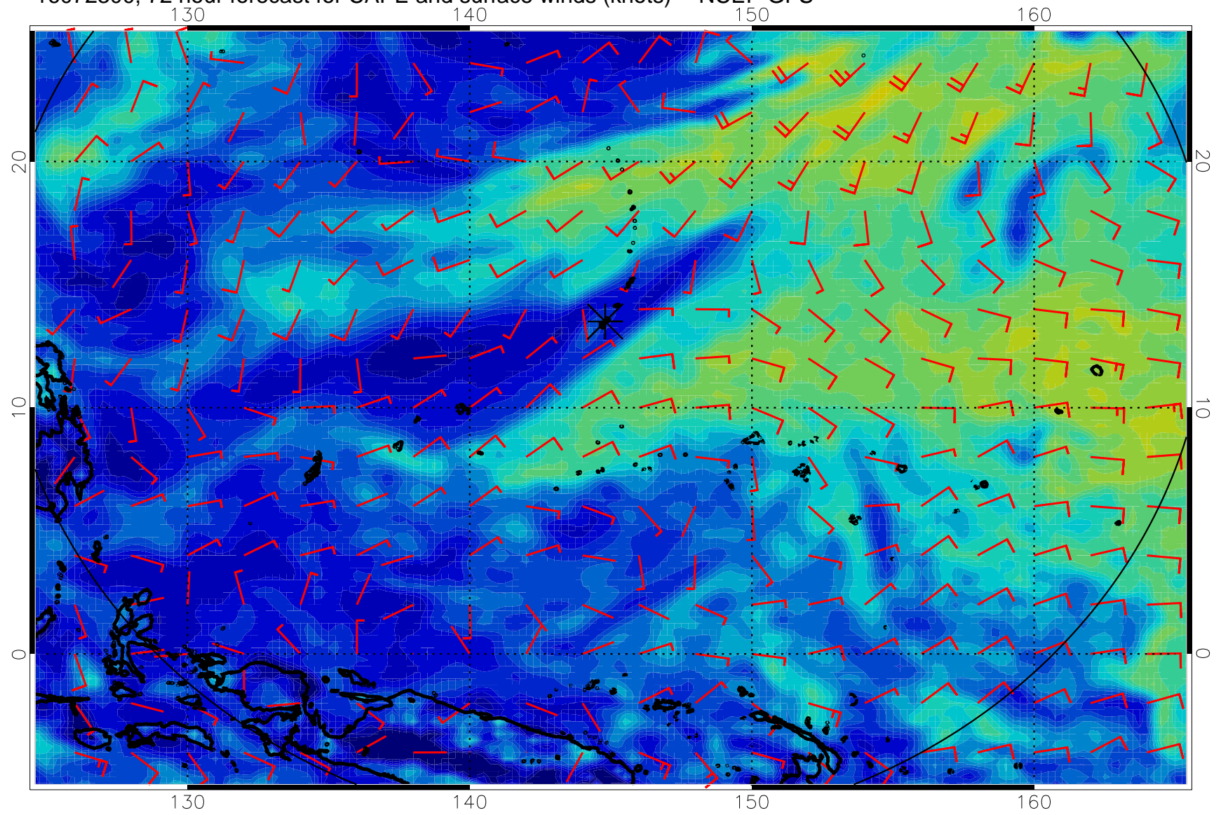
16072300, 72 hour forecast for CAPE and surface winds (knots) -- NCEP GFS
