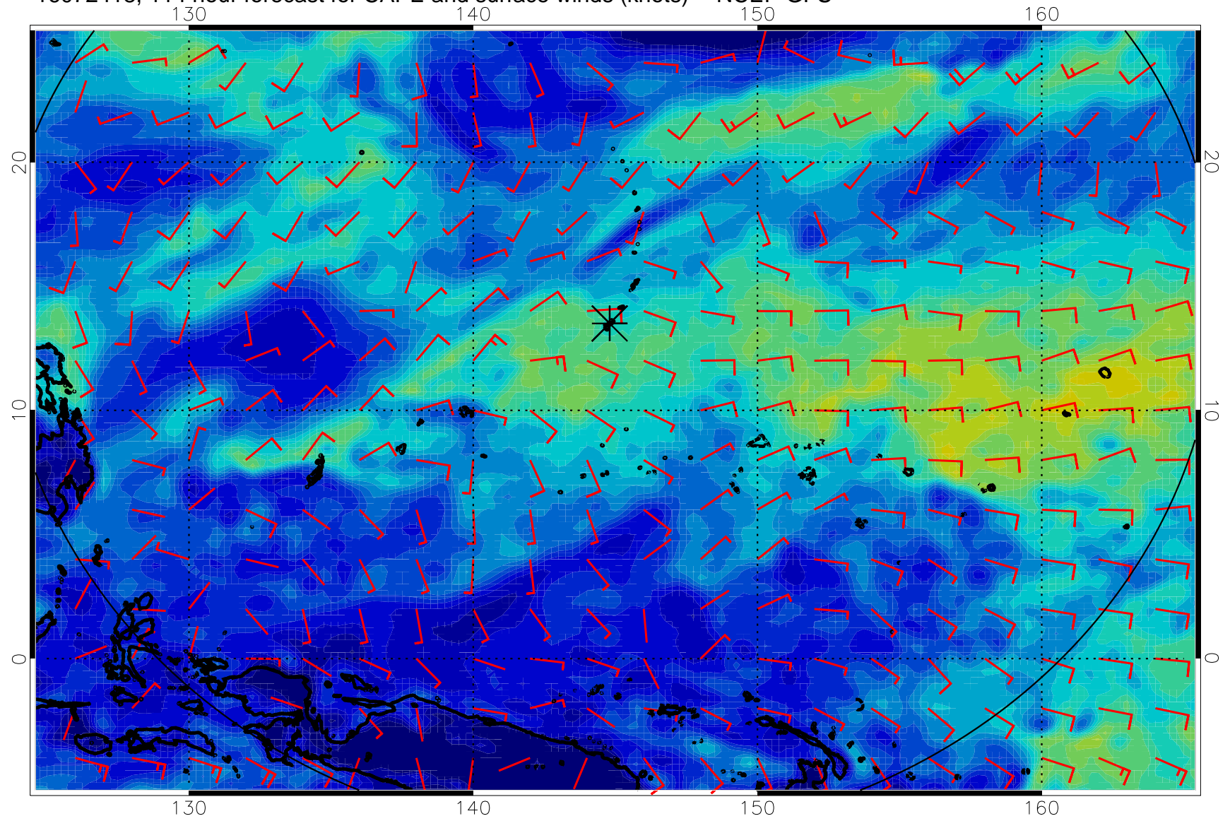
16072418, 114 hour forecast for CAPE and surface winds (knots) -- NCEP GFS
