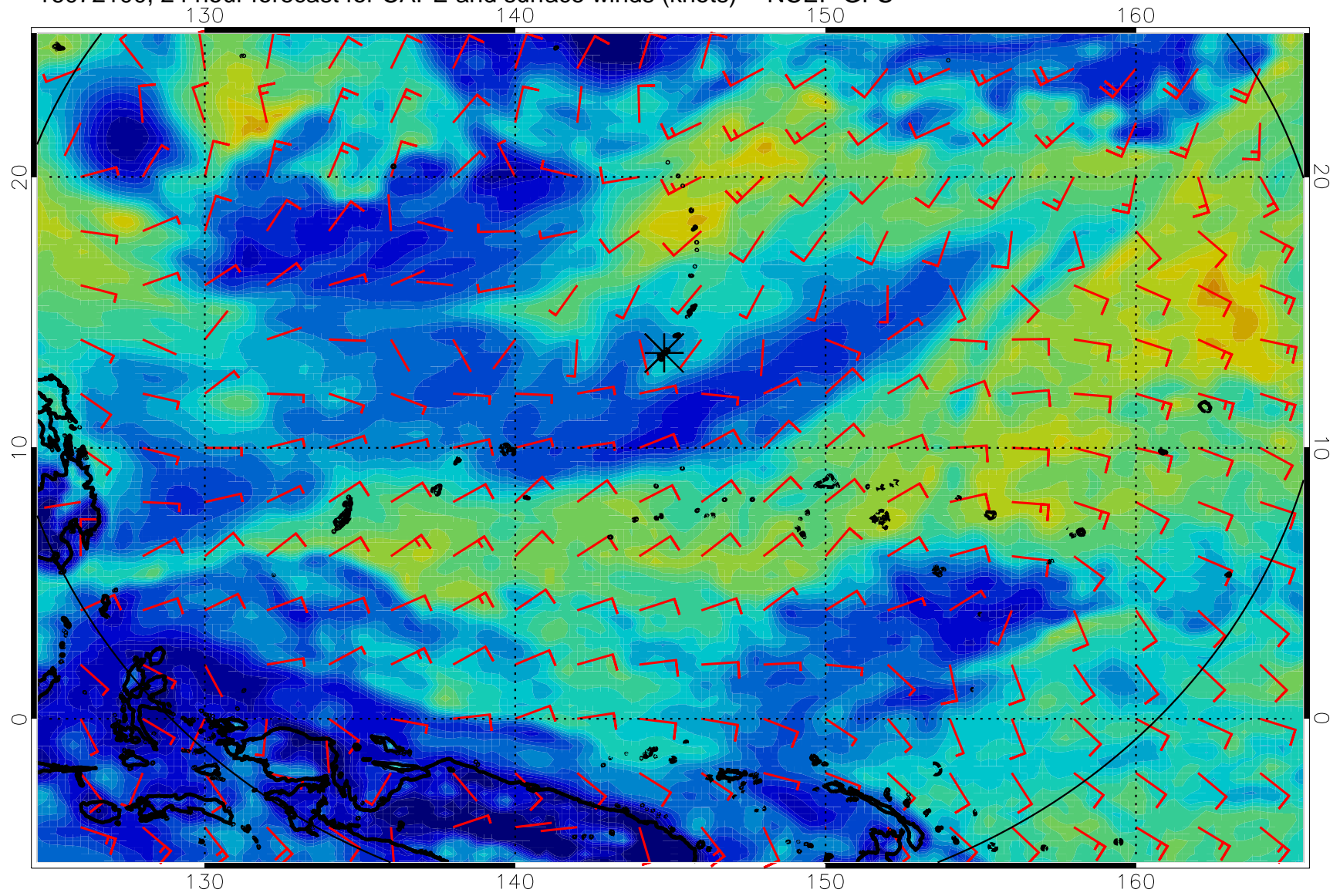
16072100, 24 hour forecast for CAPE and surface winds (knots) -- NCEP GFS
