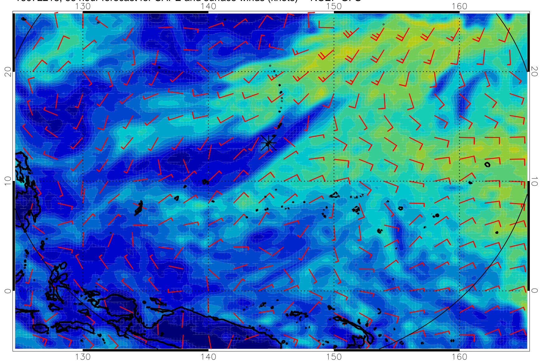
16072218, 66 hour forecast for CAPE and surface winds (knots) -- NCEP GFS
