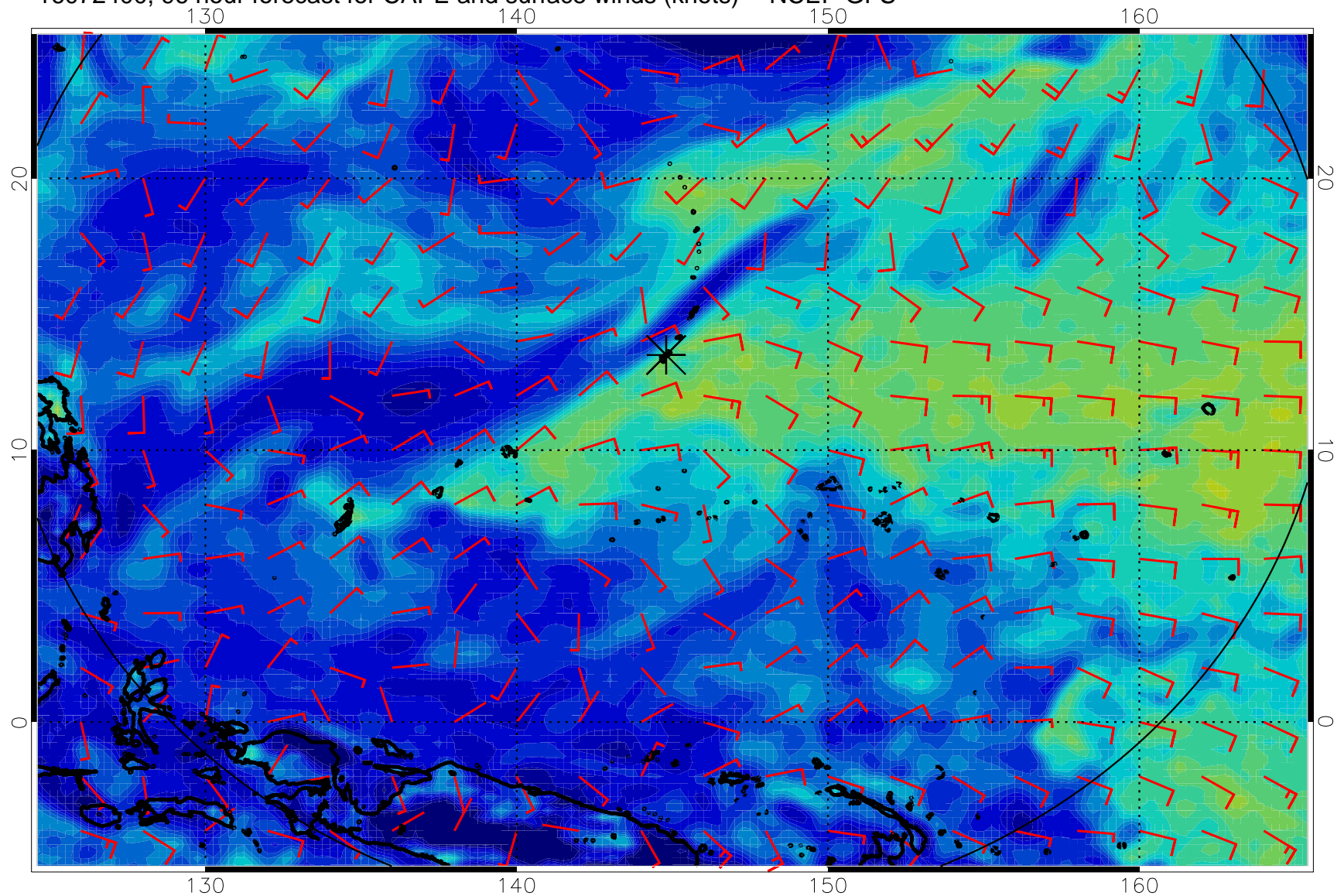
16072400, 96 hour forecast for CAPE and surface winds (knots) -- NCEP GFS
