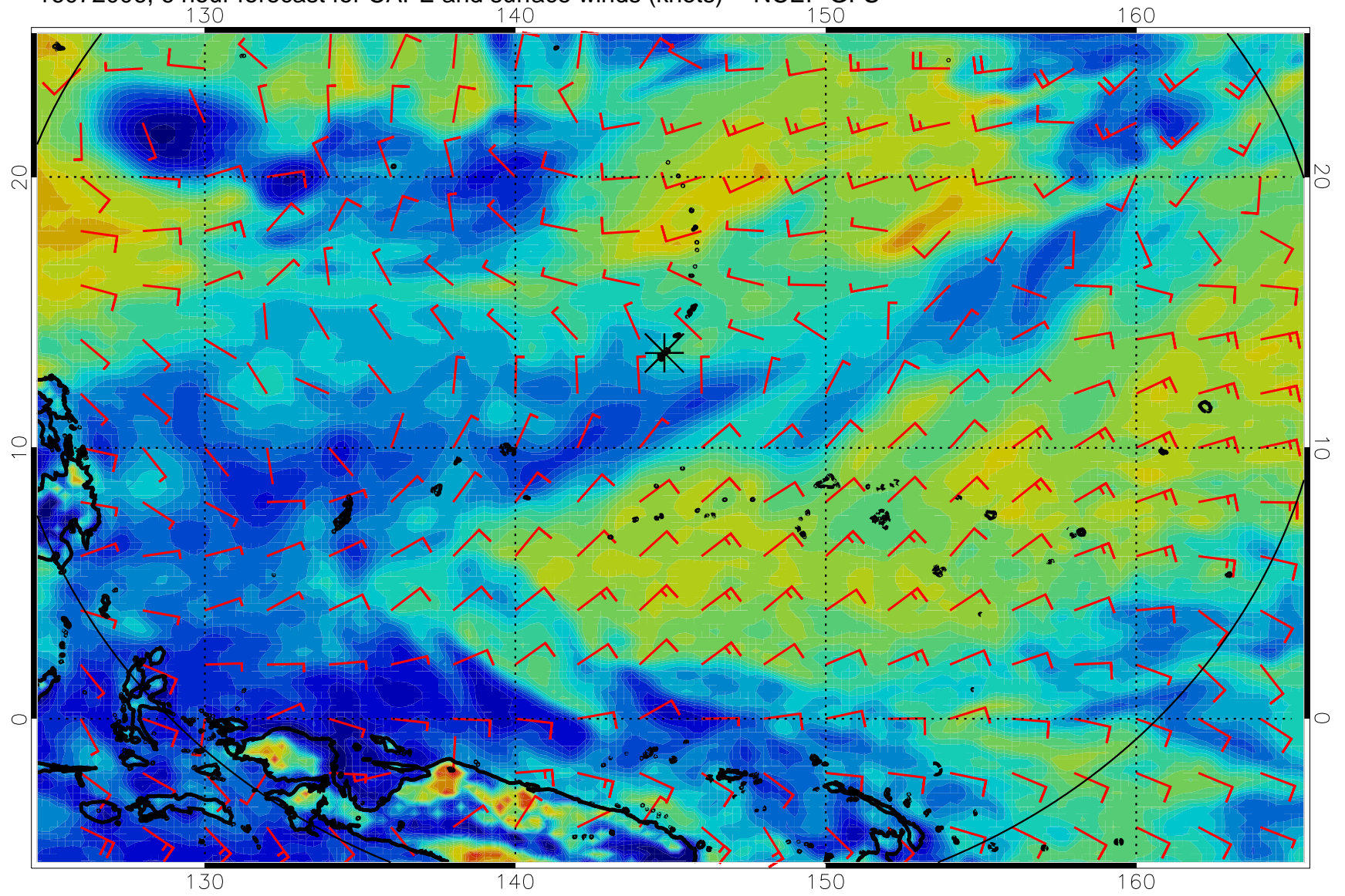
16072006, 6 hour forecast for CAPE and surface winds (knots) -- NCEP GFS
