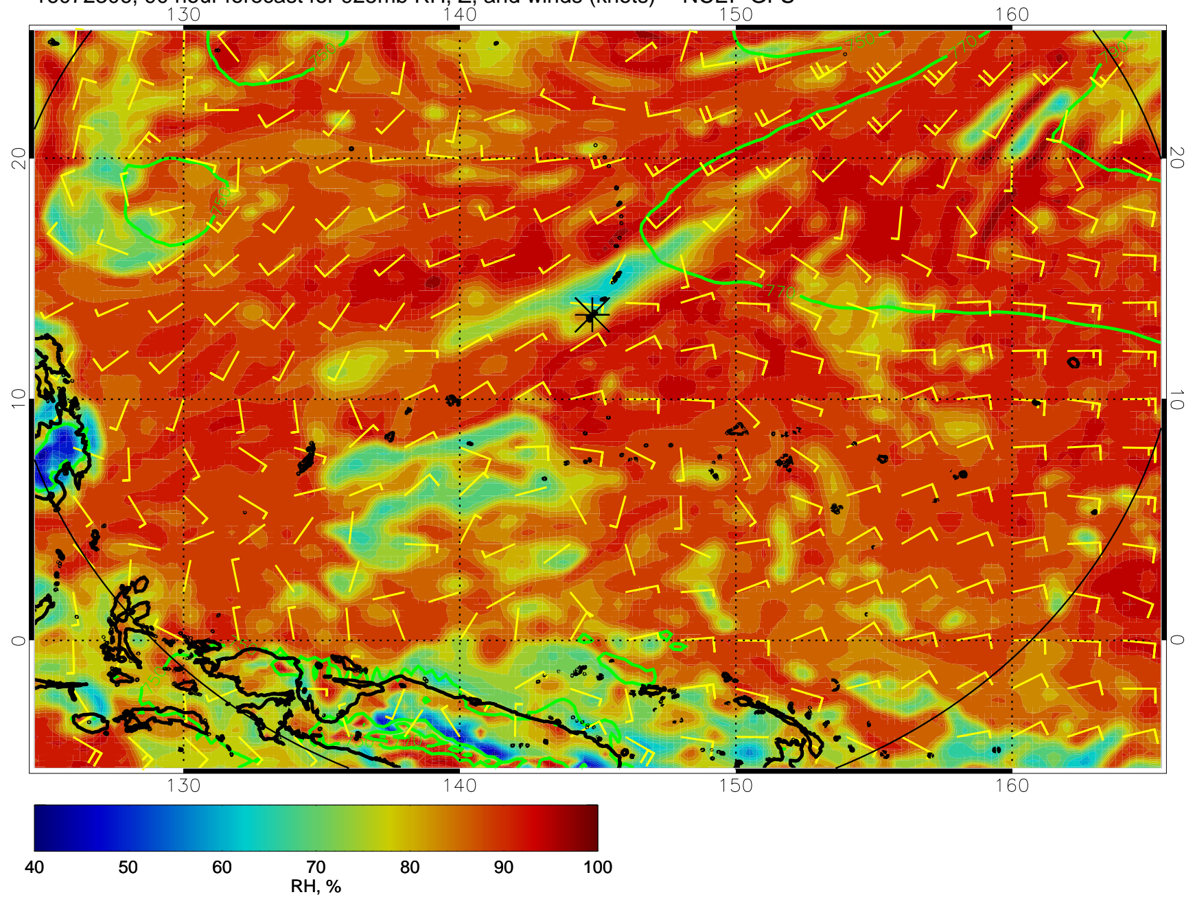
16072306, 90 hour forecast for 925mb RH, Z, and winds (knots) -- NCEP GFS
