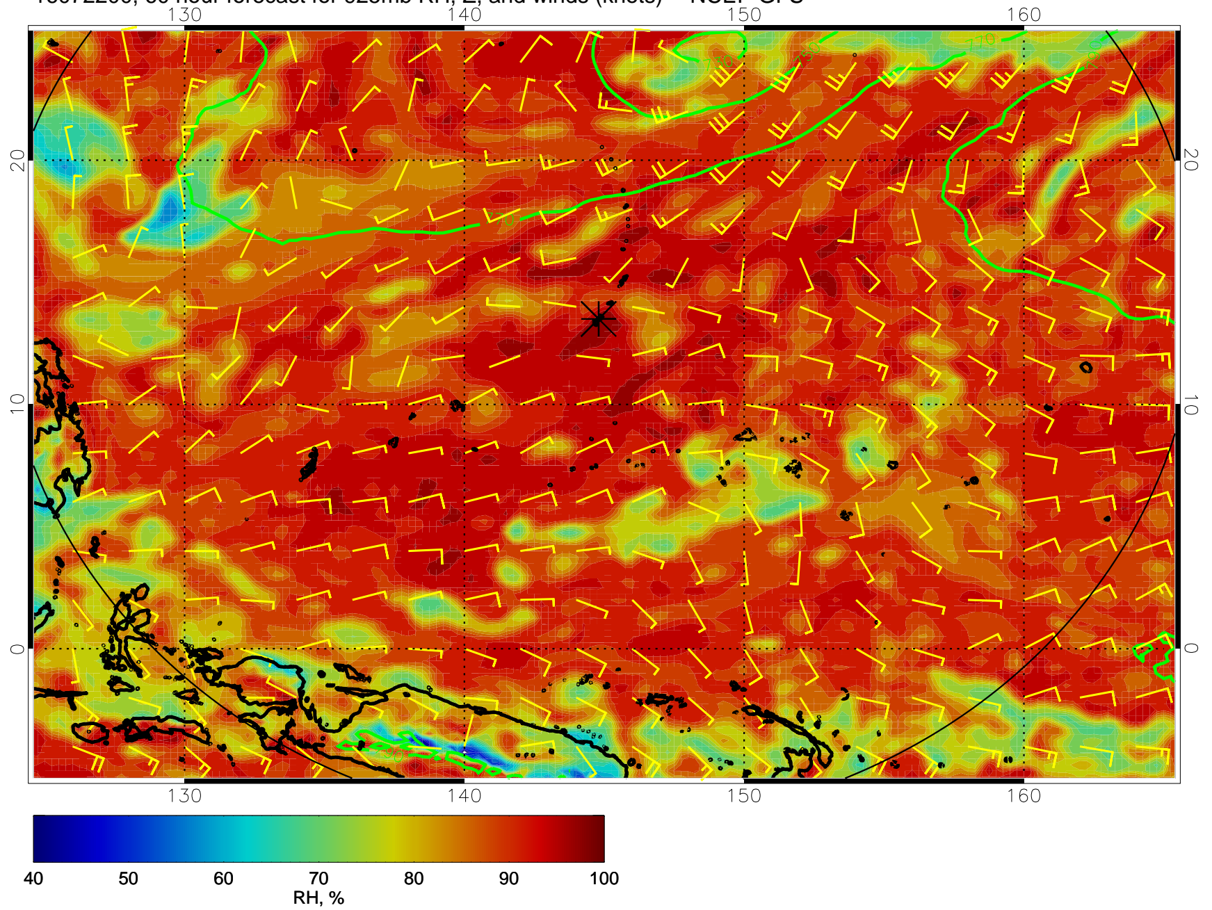
16072200, 60 hour forecast for 925mb RH, Z, and winds (knots) -- NCEP GFS
