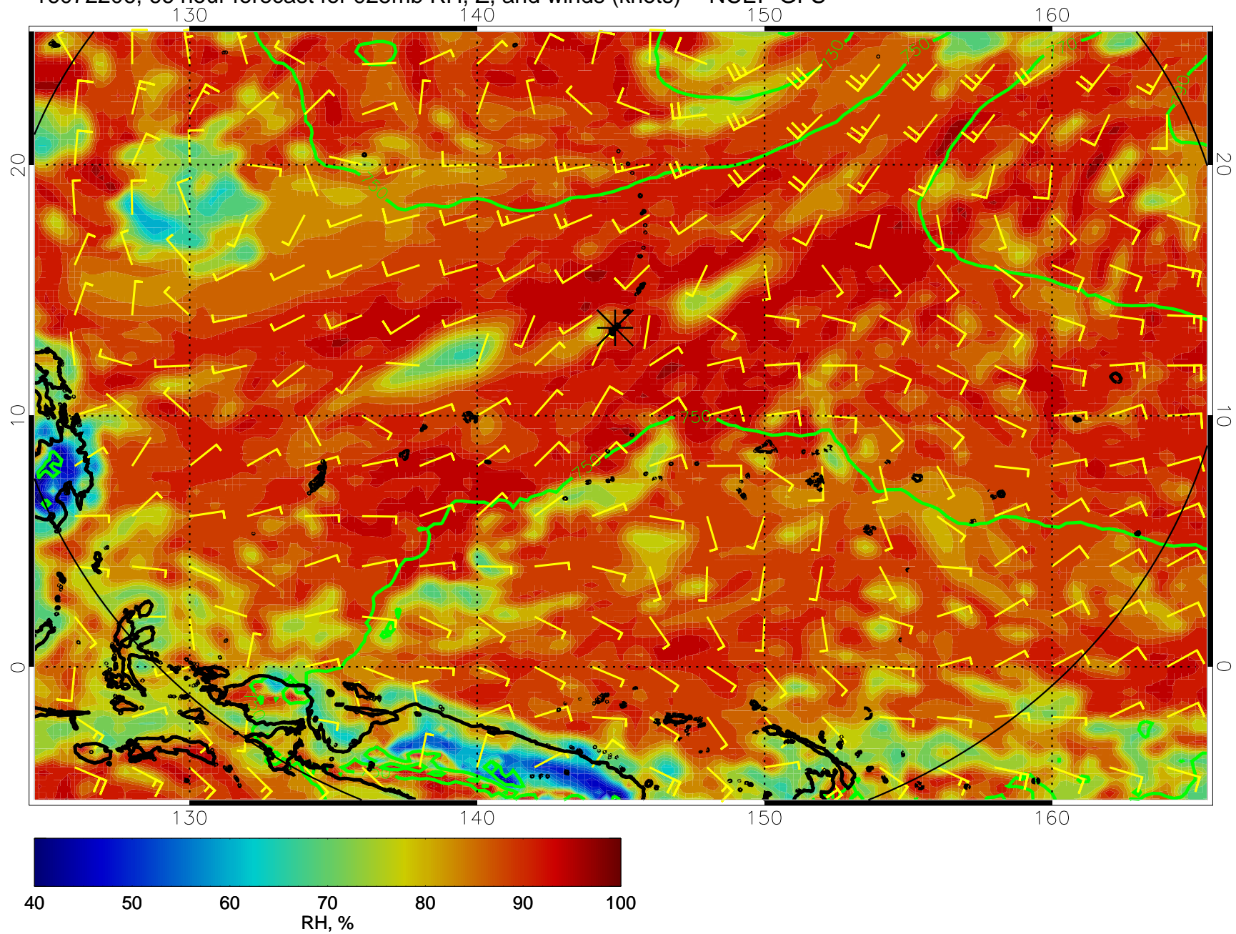
16072206, 66 hour forecast for 925mb RH, Z, and winds (knots) -- NCEP GFS
