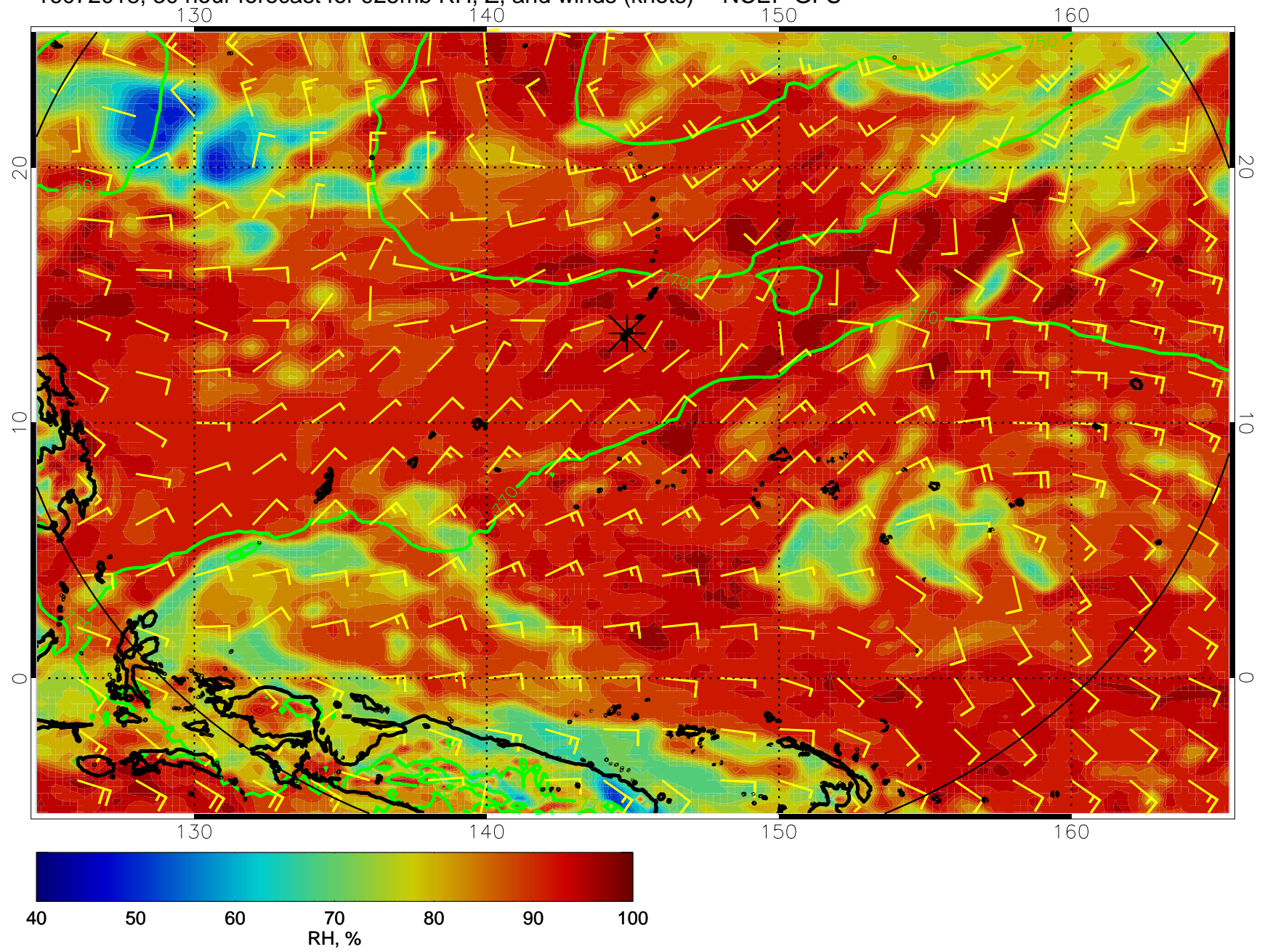
16072018, 30 hour forecast for 925mb RH, Z, and winds (knots) -- NCEP GFS
