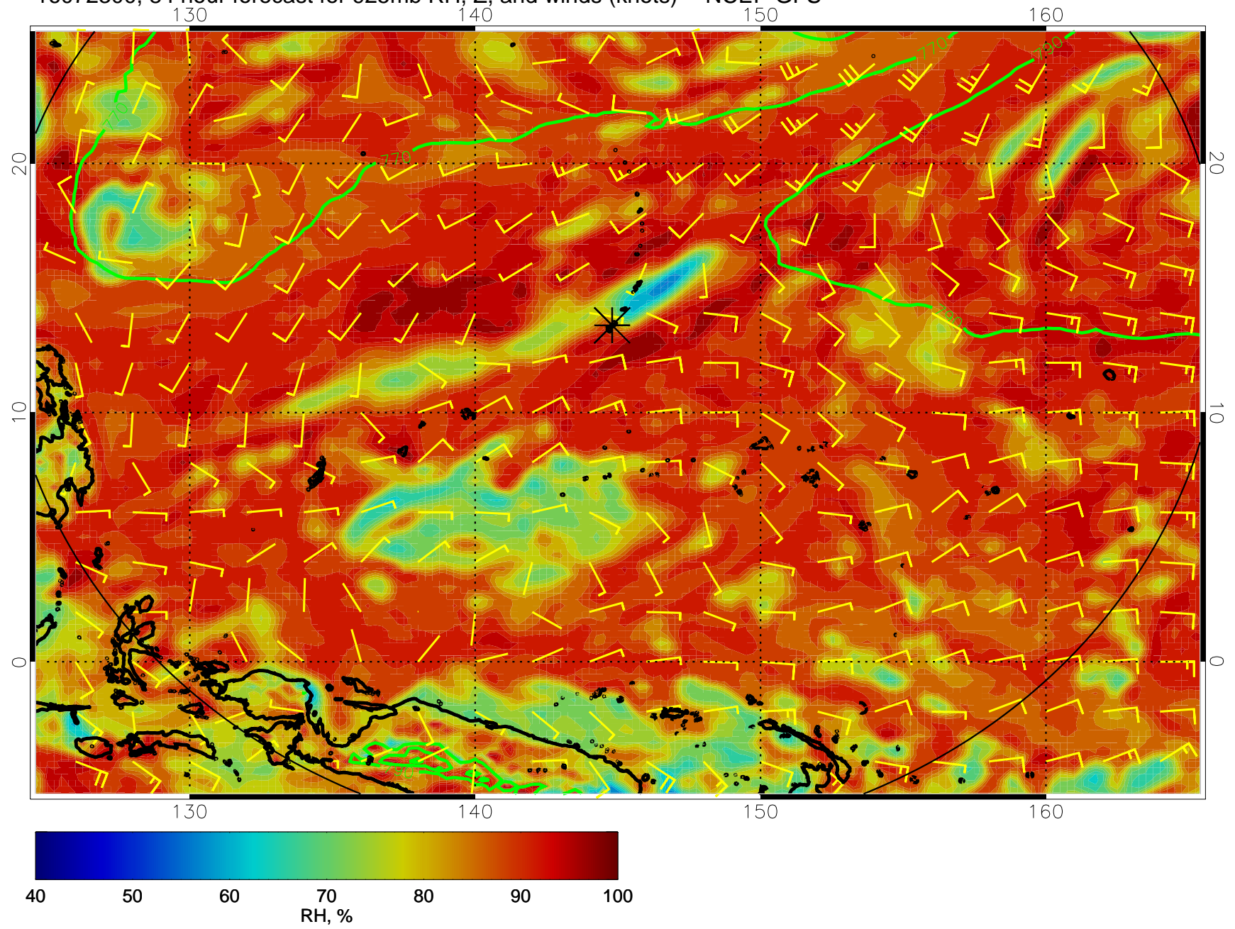
16072300, 84 hour forecast for 925mb RH, Z, and winds (knots) -- NCEP GFS
