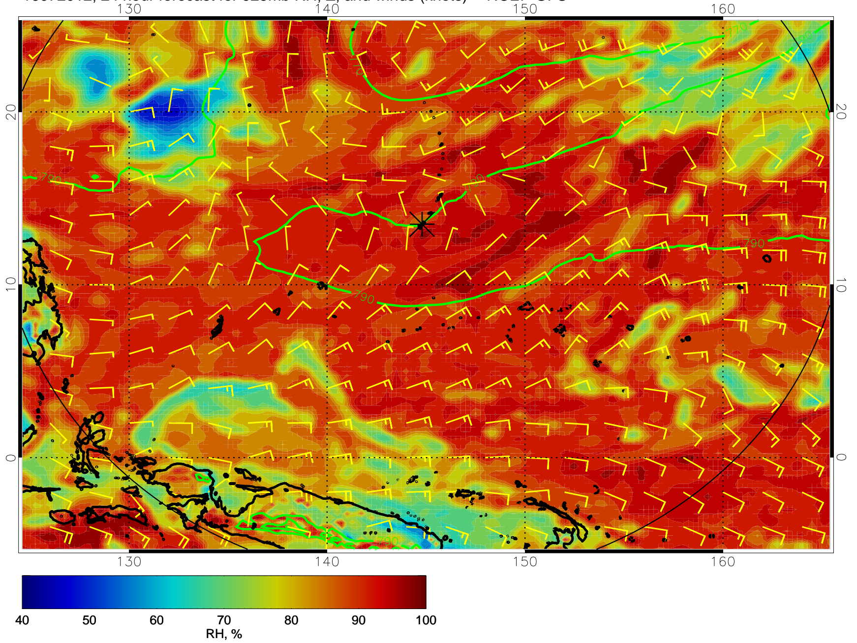
16072012, 24 hour forecast for 925mb RH, Z, and winds (knots) -- NCEP GFS
