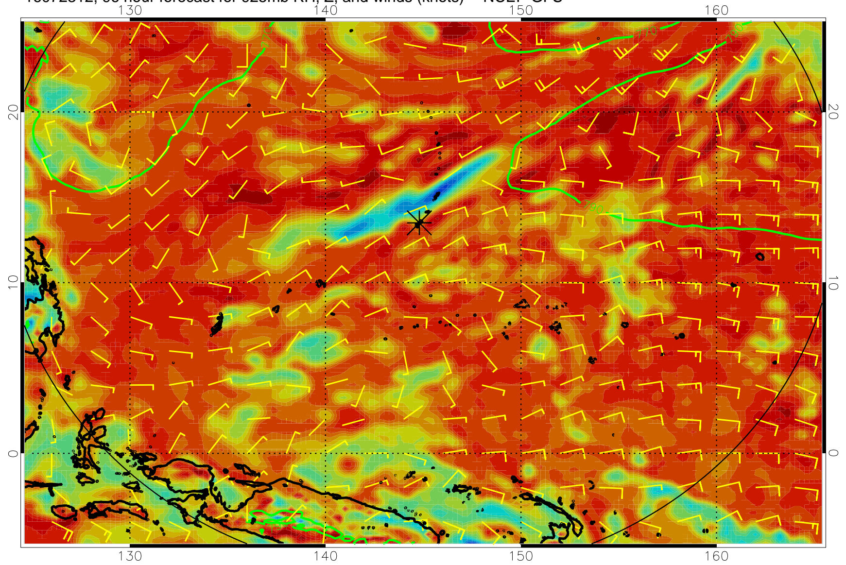
16072312, 96 hour forecast for 925mb RH, Z, and winds (knots) -- NCEP GFS
