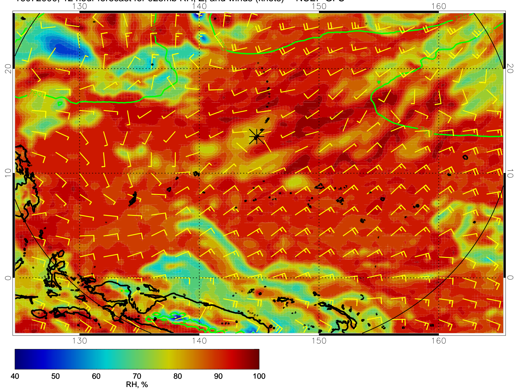
16072000, 12 hour forecast for 925mb RH, Z, and winds (knots) -- NCEP GFS
