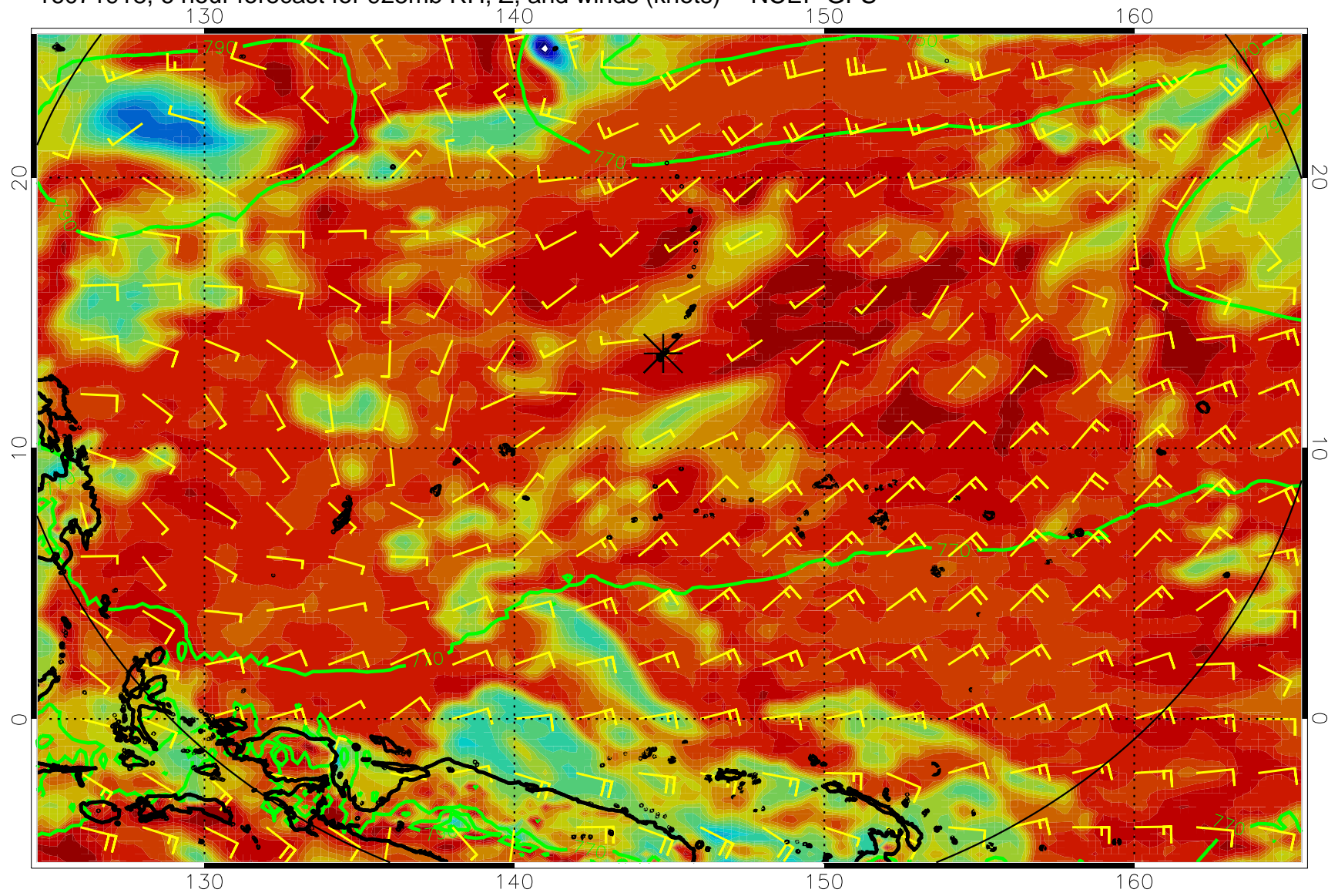
16071918, 6 hour forecast for 925mb RH, Z, and winds (knots) -- NCEP GFS
