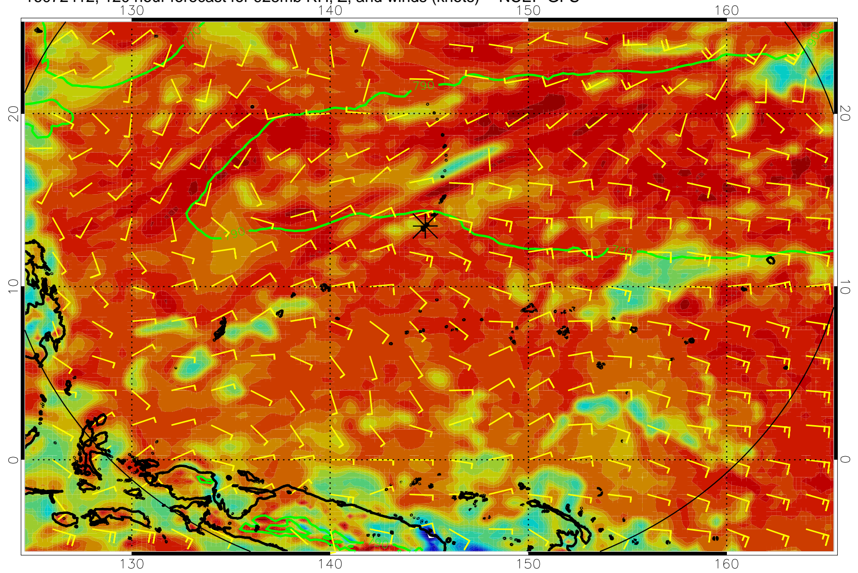
16072412, 120 hour forecast for 925mb RH, Z, and winds (knots) -- NCEP GFS
