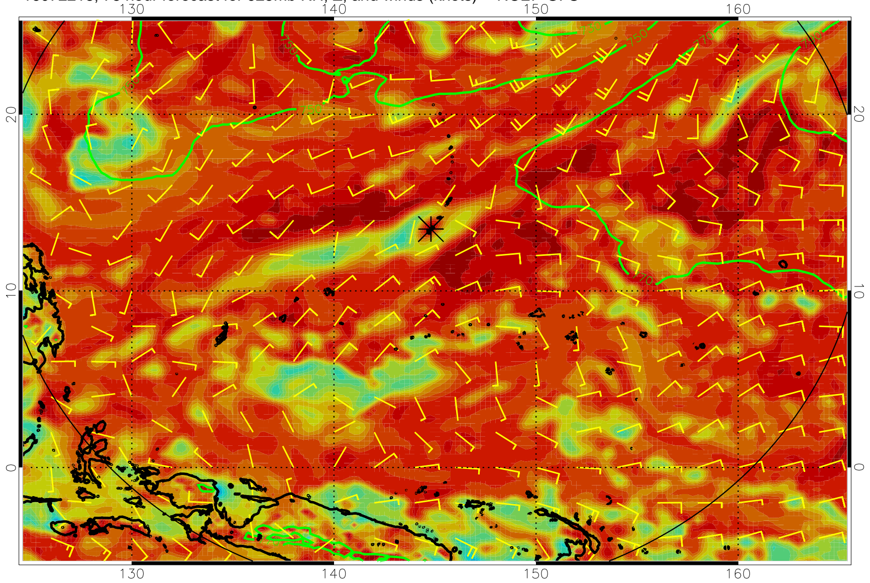
16072218, 78 hour forecast for 925mb RH, Z, and winds (knots) -- NCEP GFS
