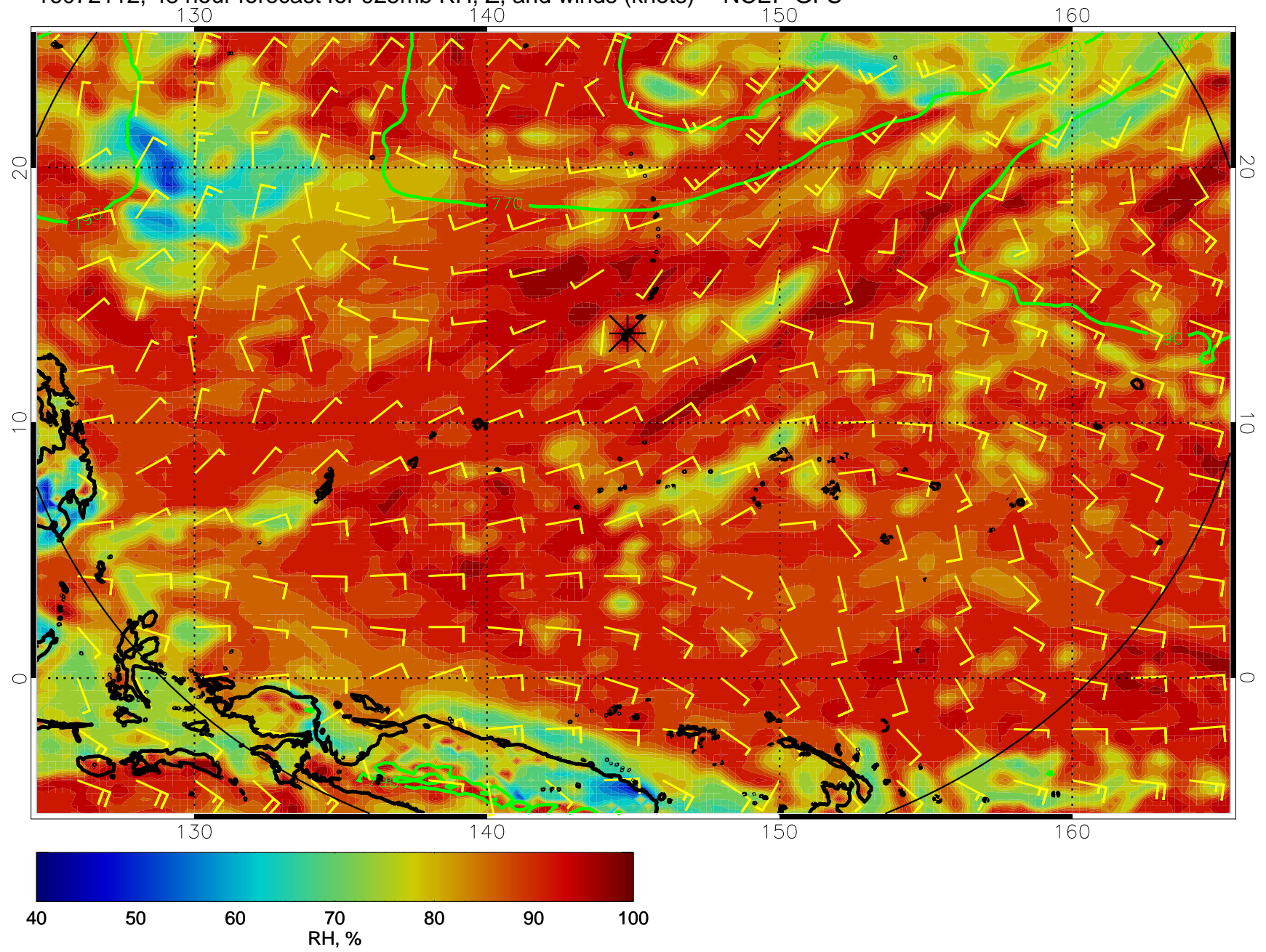
16072112, 48 hour forecast for 925mb RH, Z, and winds (knots) -- NCEP GFS
